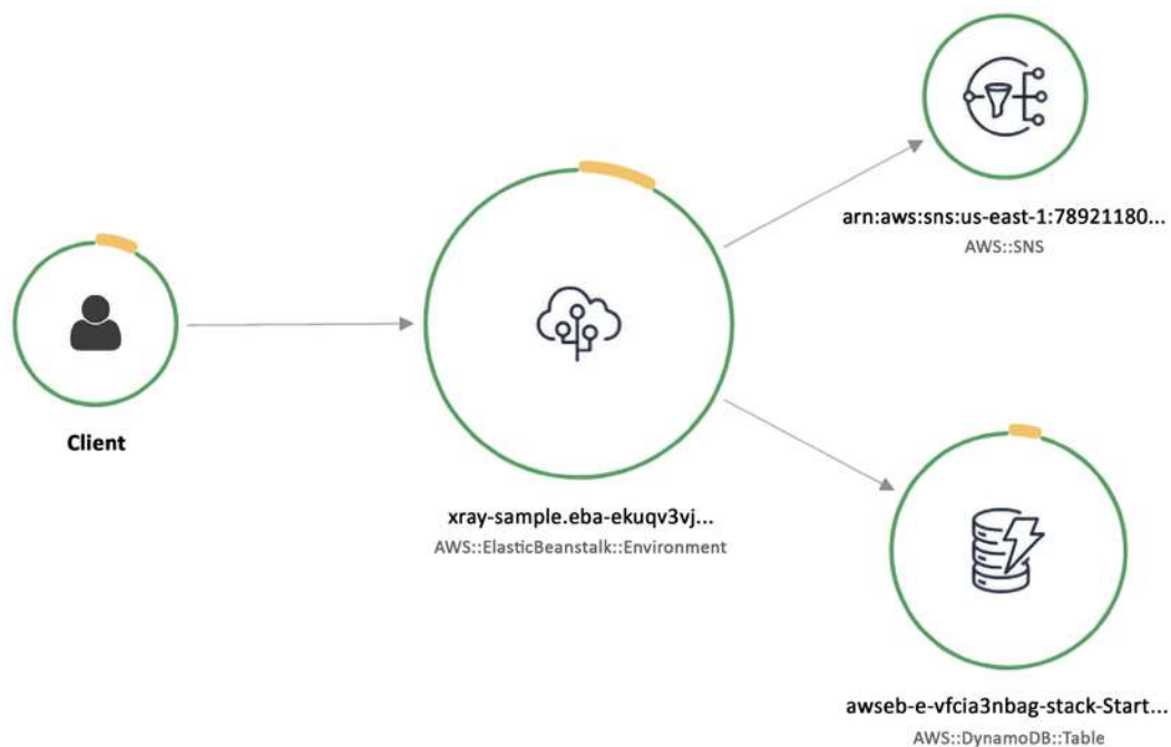
Figure 9.8: AWS X-Ray service map graph
