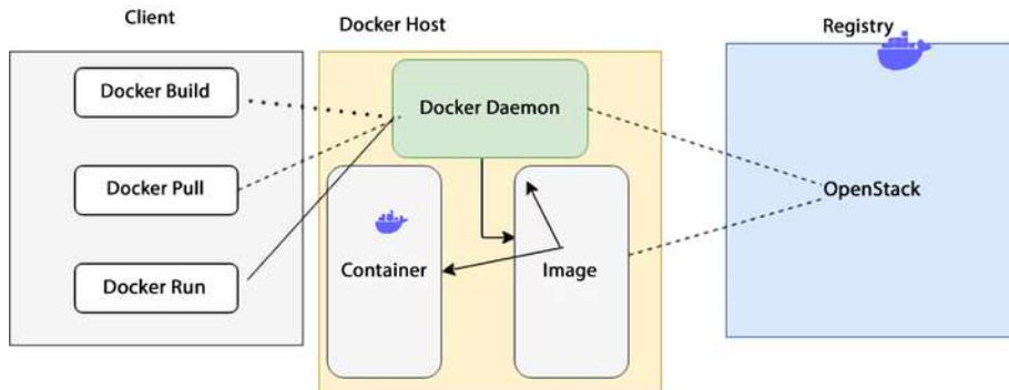
Figure 13.3: Docker architecture
