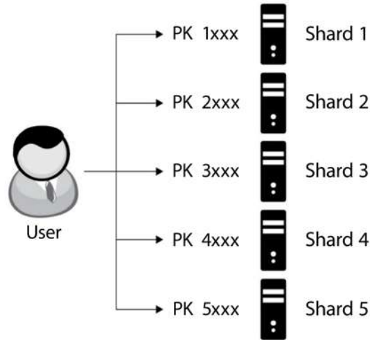
Figure 3.7: Sharding architecture
