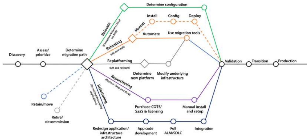
Figure 3.2: 7 Rs of AWS cloud migration
