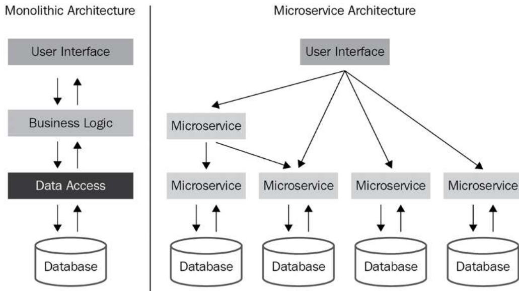
Figure 14.1: Monolithic versus microservice architectures
