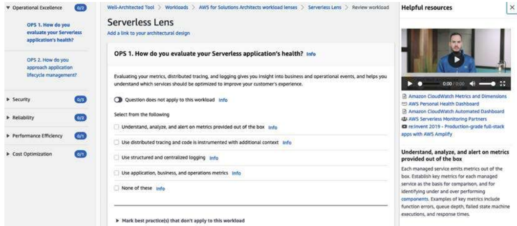
Figure 2.9: AWS Well-Architected Serverless Lens
