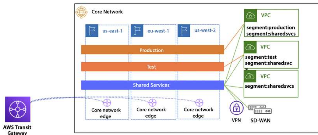
Figure 4.14: AWS Cloud WAN architecture
