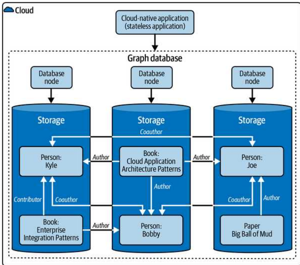
Figure 7-19. Graph Database
