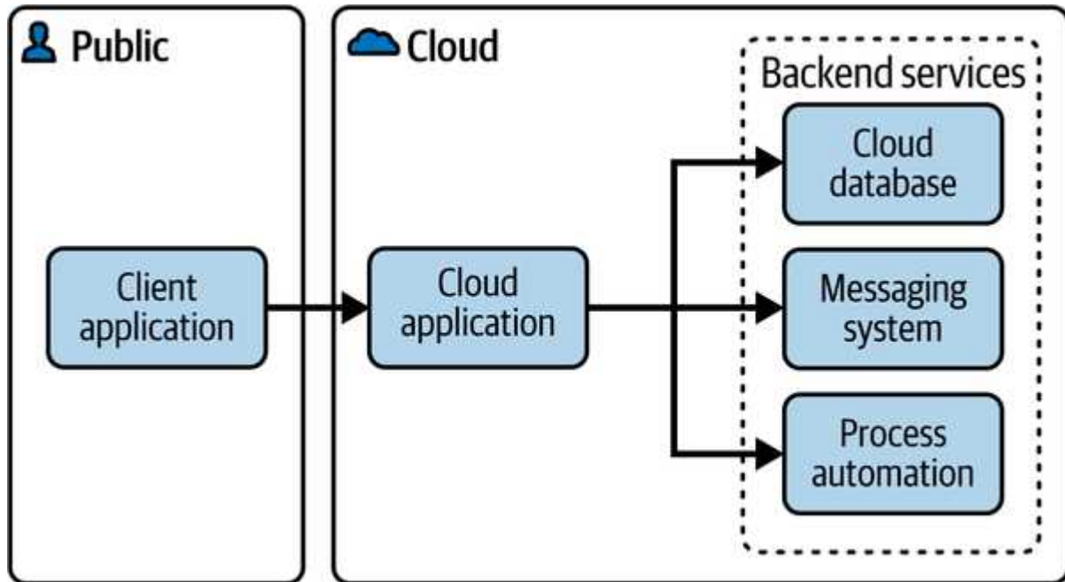
Figure 3-15. Backend Services
