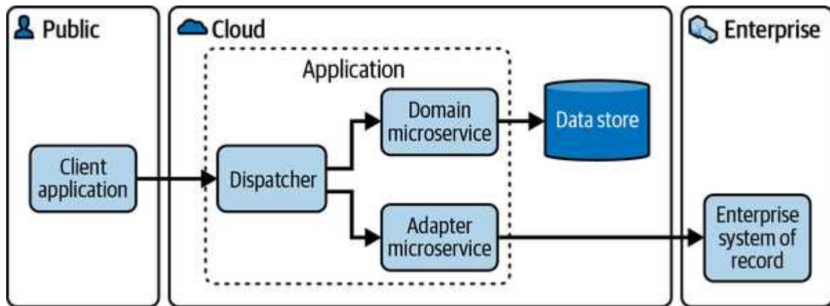
Figure 4-5. Microservices application
