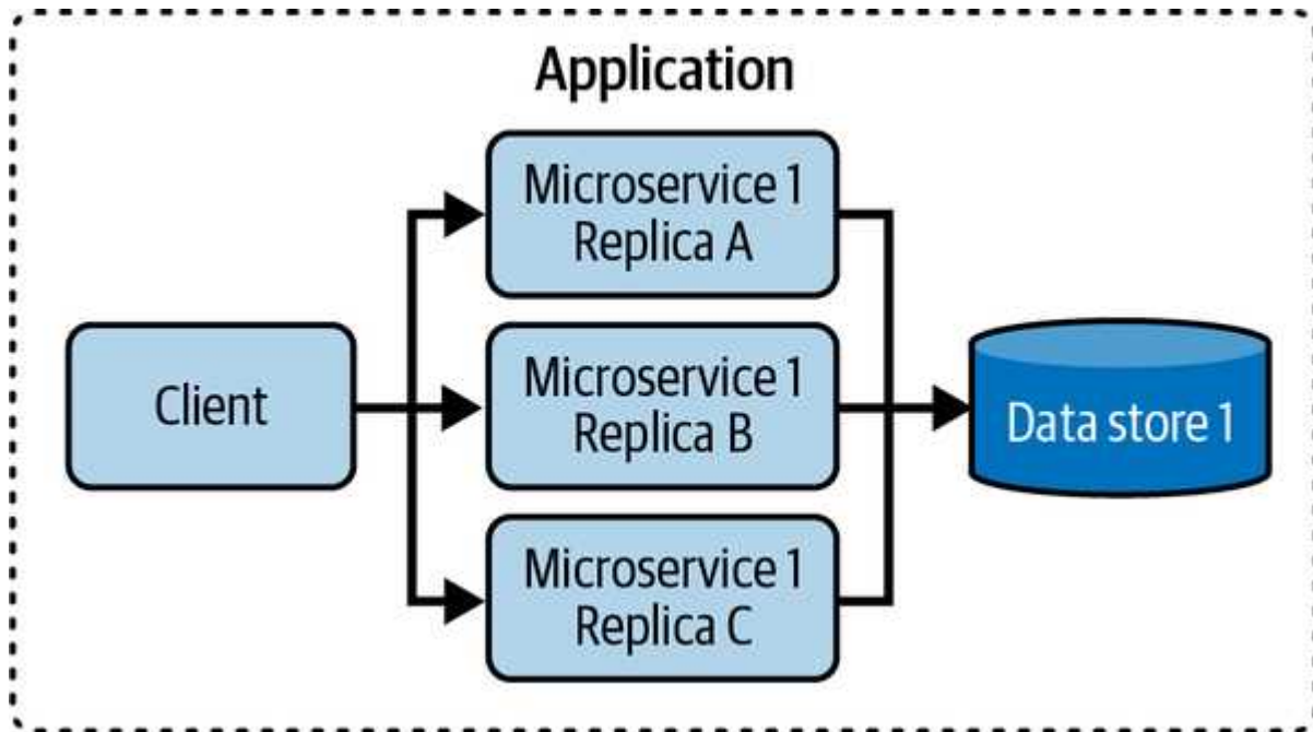
Figure 4-22. Microservice replicas share a data store
