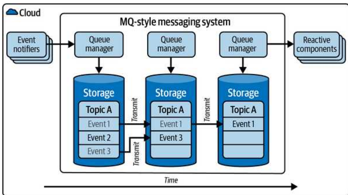
Figure 6-21. MQ-style messaging system
