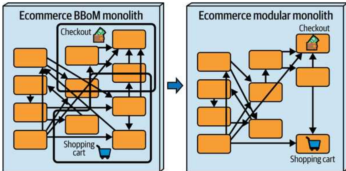
Figure 2-6. Ecommerce BBoM to Modular Monolith evolution
