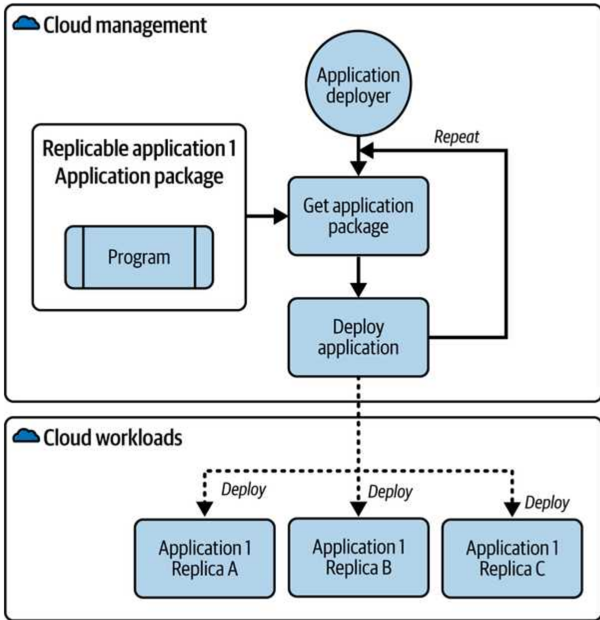
Figure 3-10. Replicable Application
