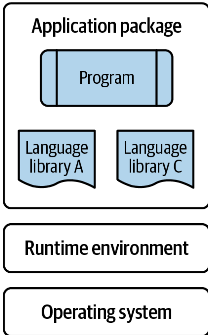
Figure 3-6. Running program
