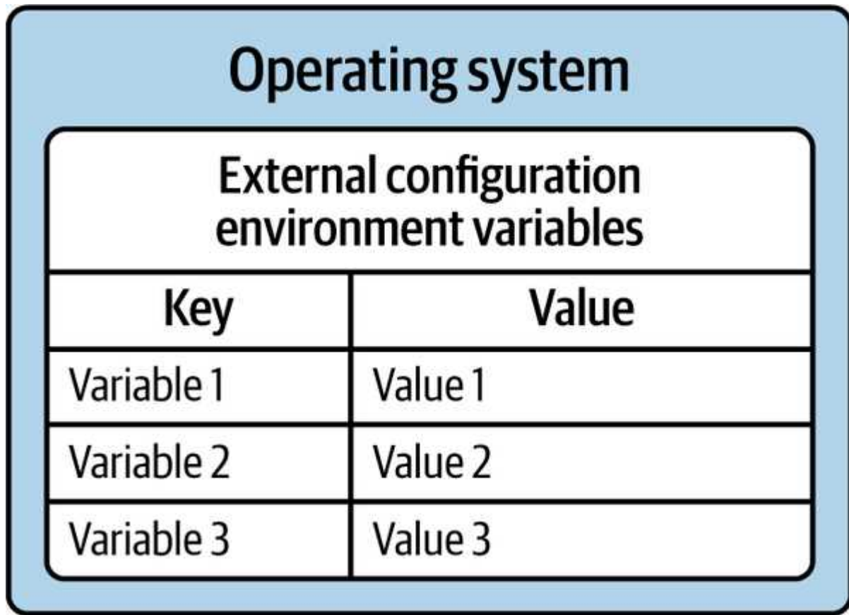
Figure 3-13. Environment variables
