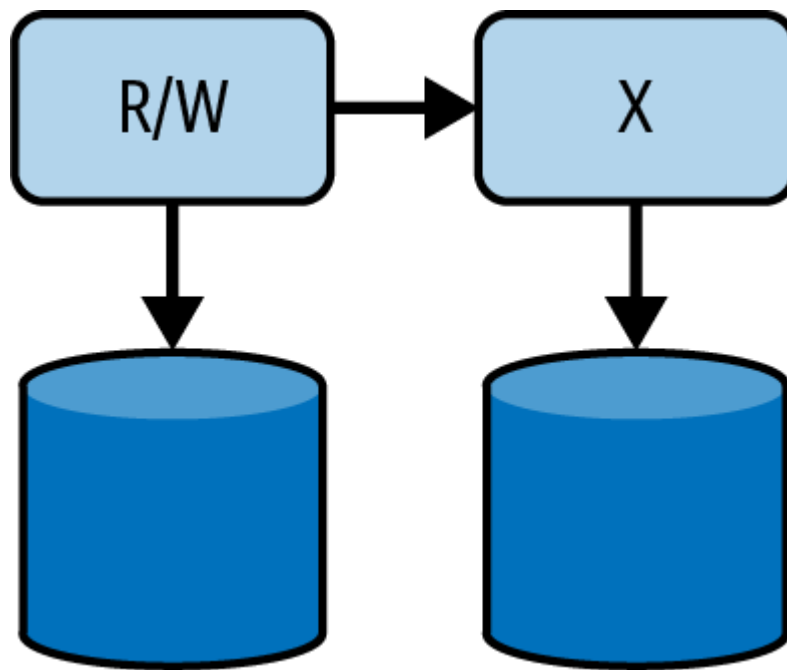
Figure 7-3. Leader-follower topology
