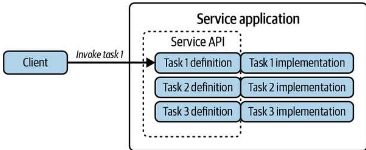
Figure 3-8. Service API
