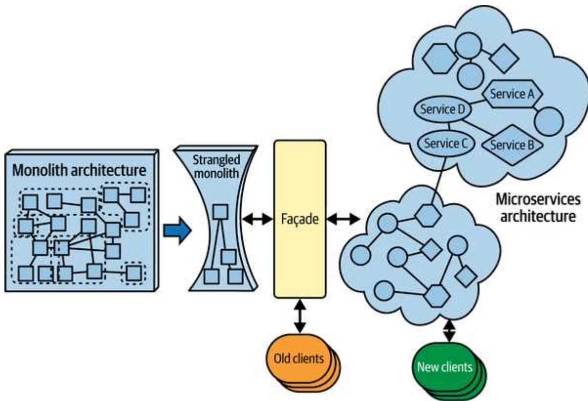
Figure 10-27. Strangled Monolith
