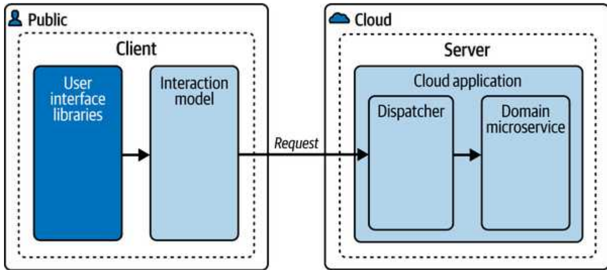
Figure 8-24. Interaction Model
