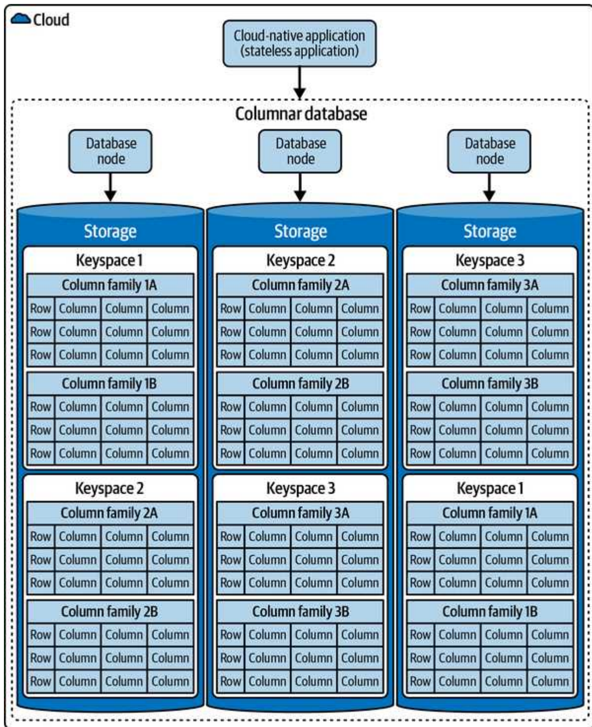
Figure 7-20. Columnar Database
