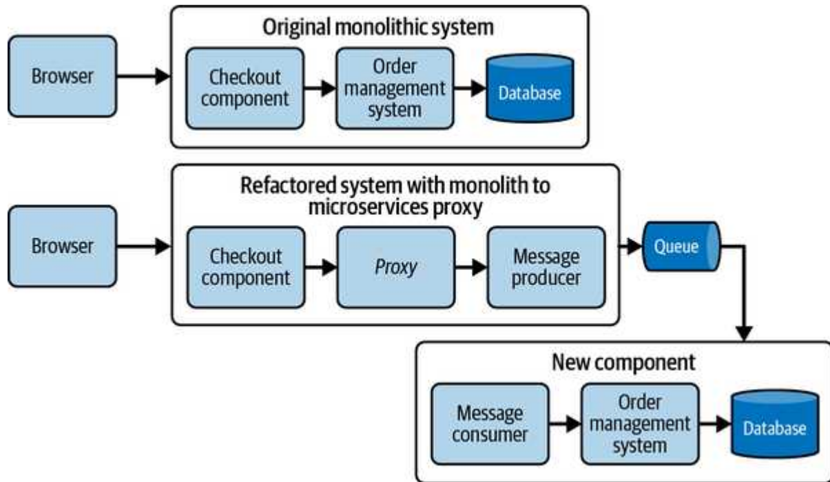
Figure 10-21. Retail example of Monolith to Microservice Proxy
