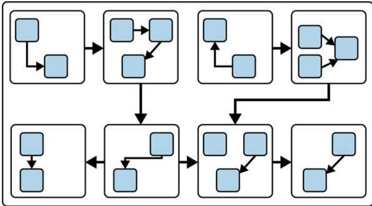
Figure 2-4. Modular Monolith
