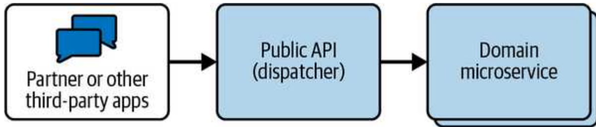
Figure 8-22. Public API
