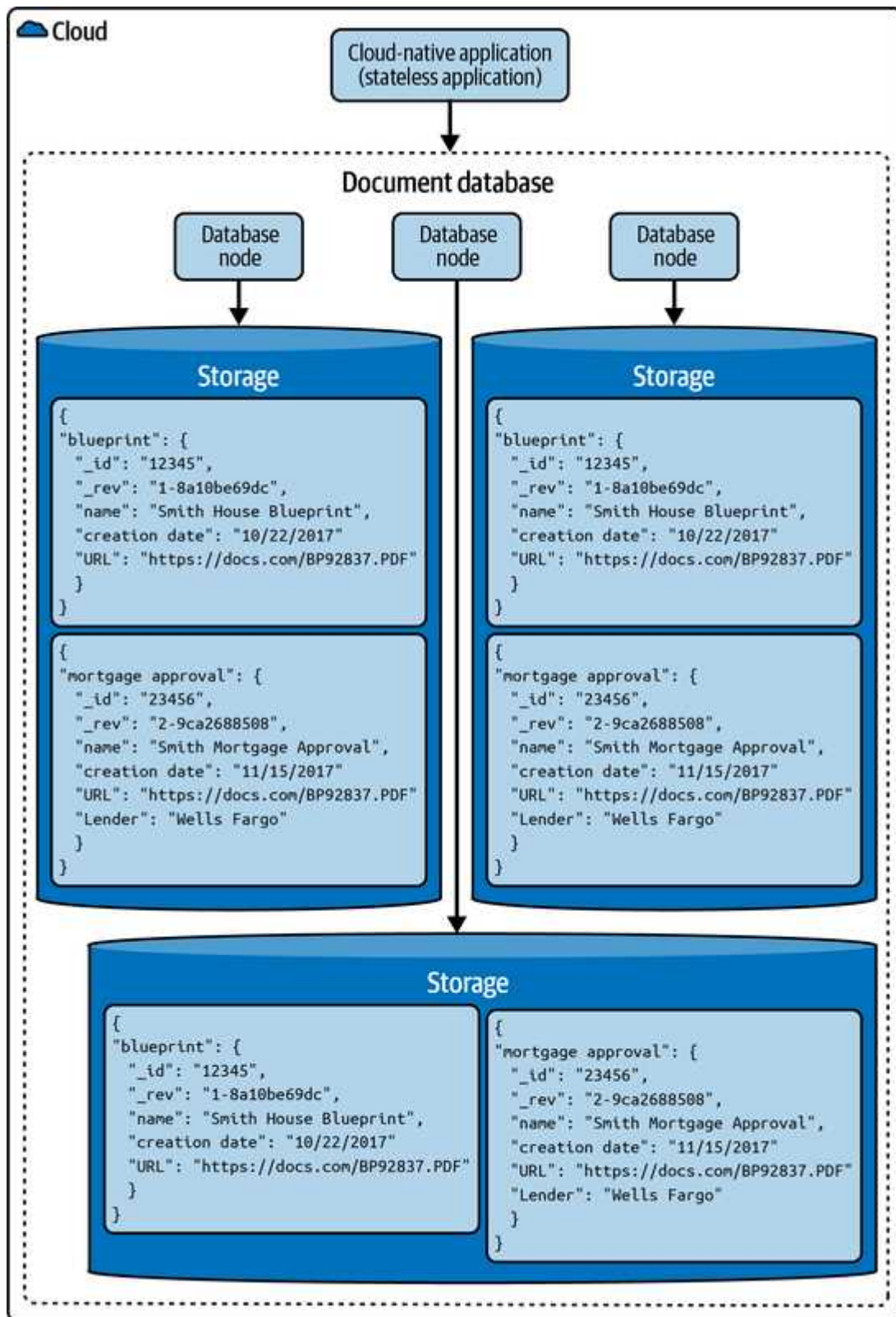
Figure 7-15. Document Database
