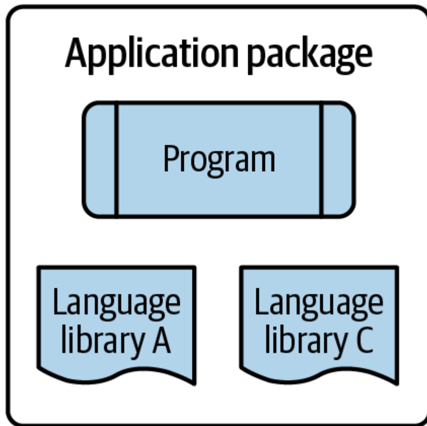
Figure 3-4. Application Package
