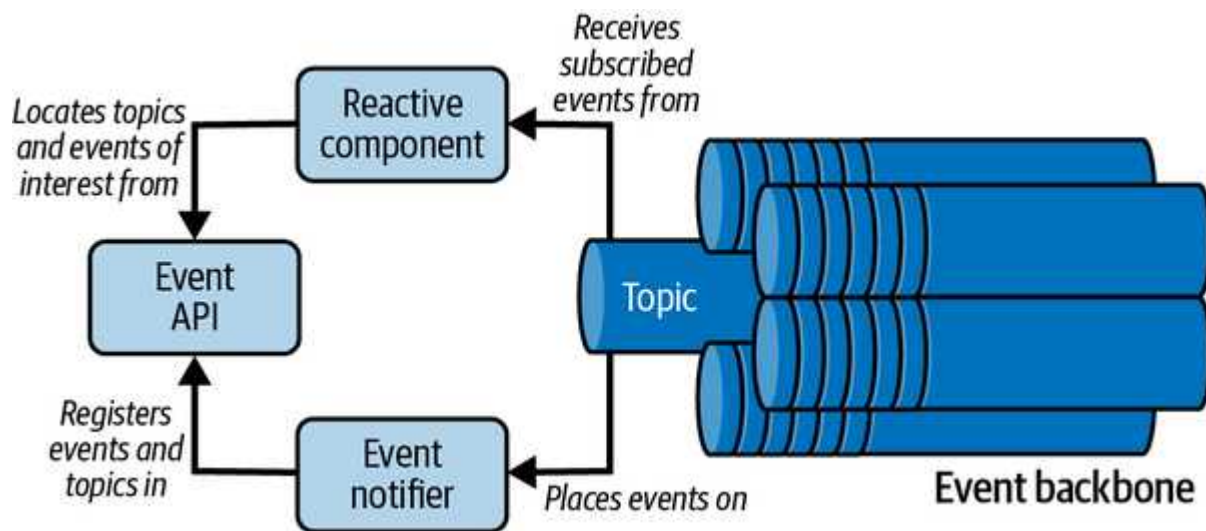
Figure 6-19. Event Backbone
