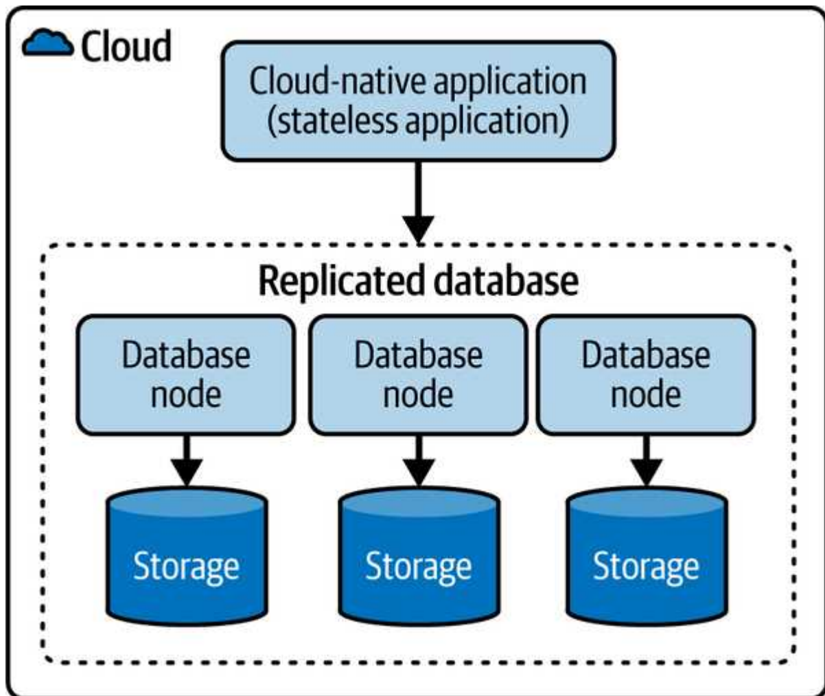
Figure 7-8. Replicated Database
