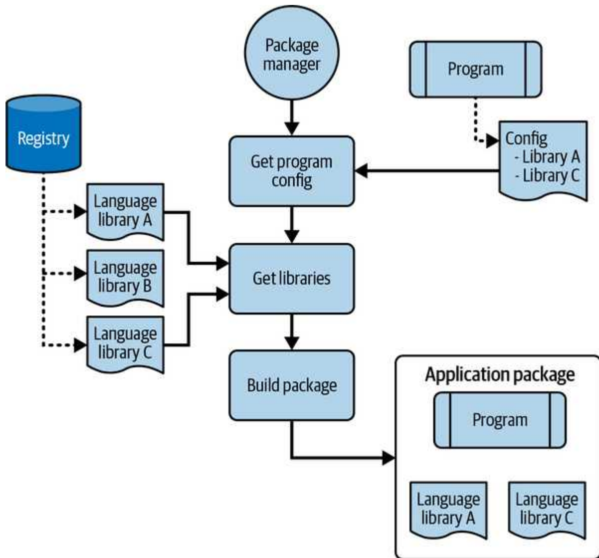
Figure 3-7. Package manager
