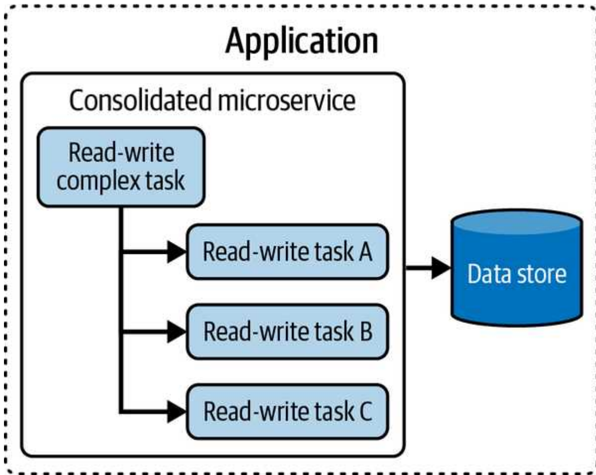
Figure 4-26. Consolidated microservice
