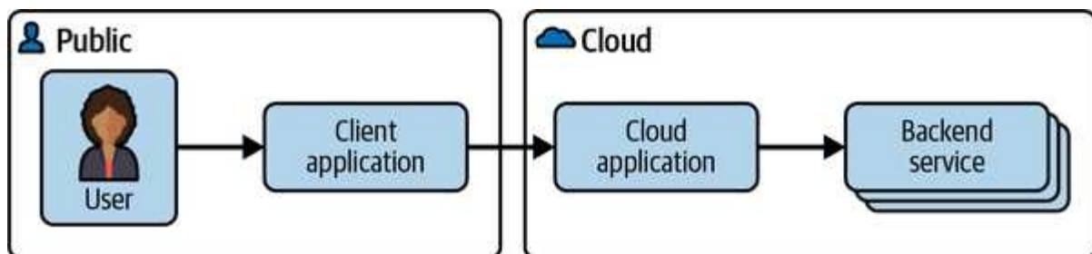
Figure 8-6. Client Application
