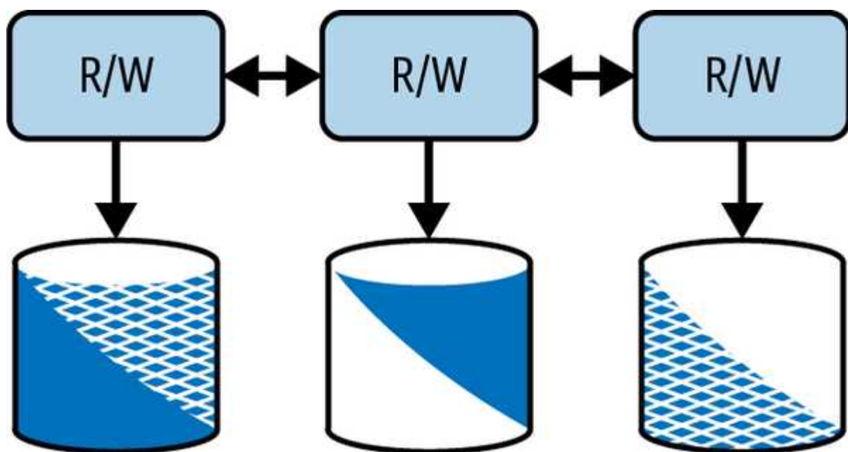
Figure 7-6. Partitioning with replication topology
