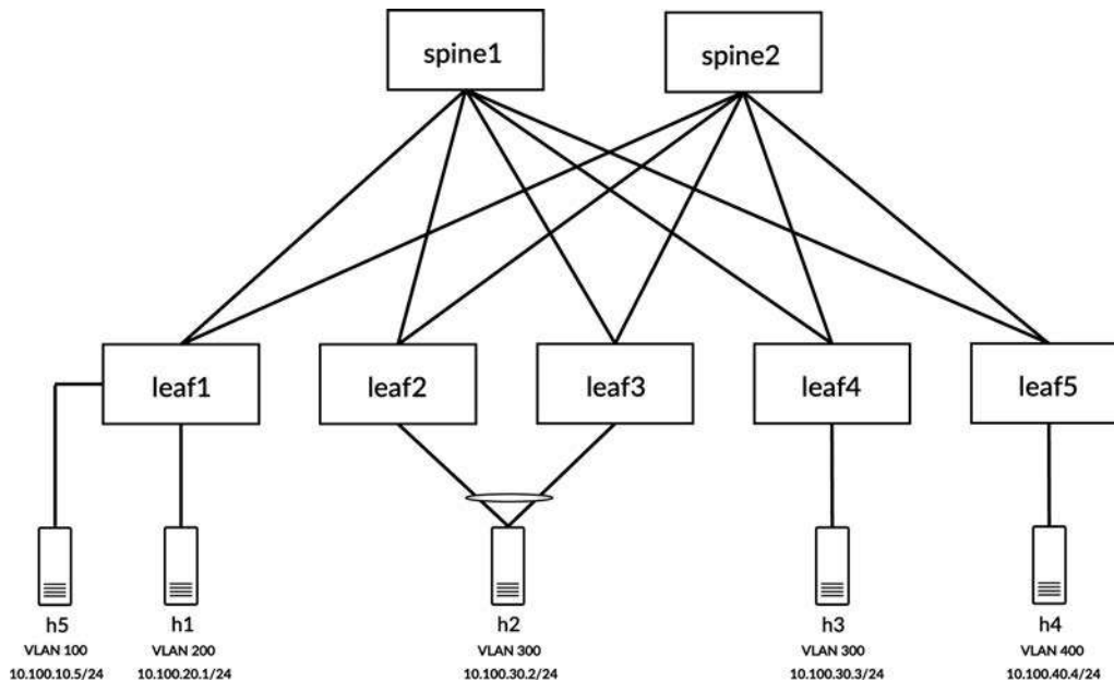
Figure 8-8 Reference topology for asymmetric IRB
