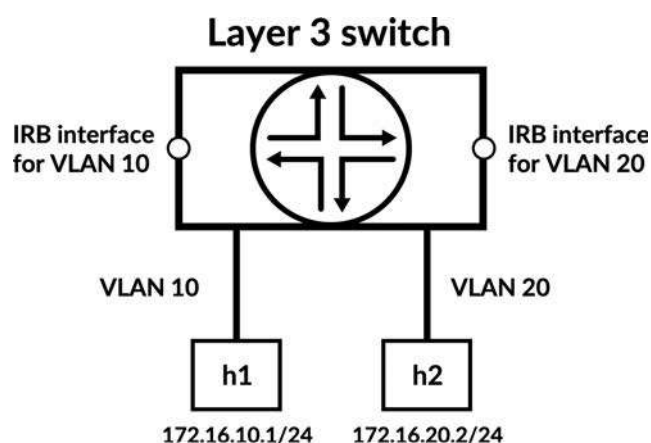
Figure 7-2 Layer 3-capable switch with IRB interfaces for routing between VLANs
