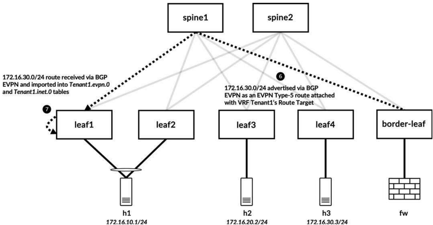
Figure 15-22 IPv4 subnet 172.16.30.0/24 received by leaf1 via BGP EVPN and imported into Tenant1's EVPN and inet.0 tables
