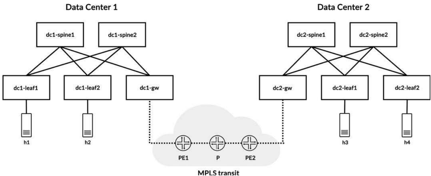
Figure 11-31 Reference topology for Integrated Interconnect with an MPLS transit
