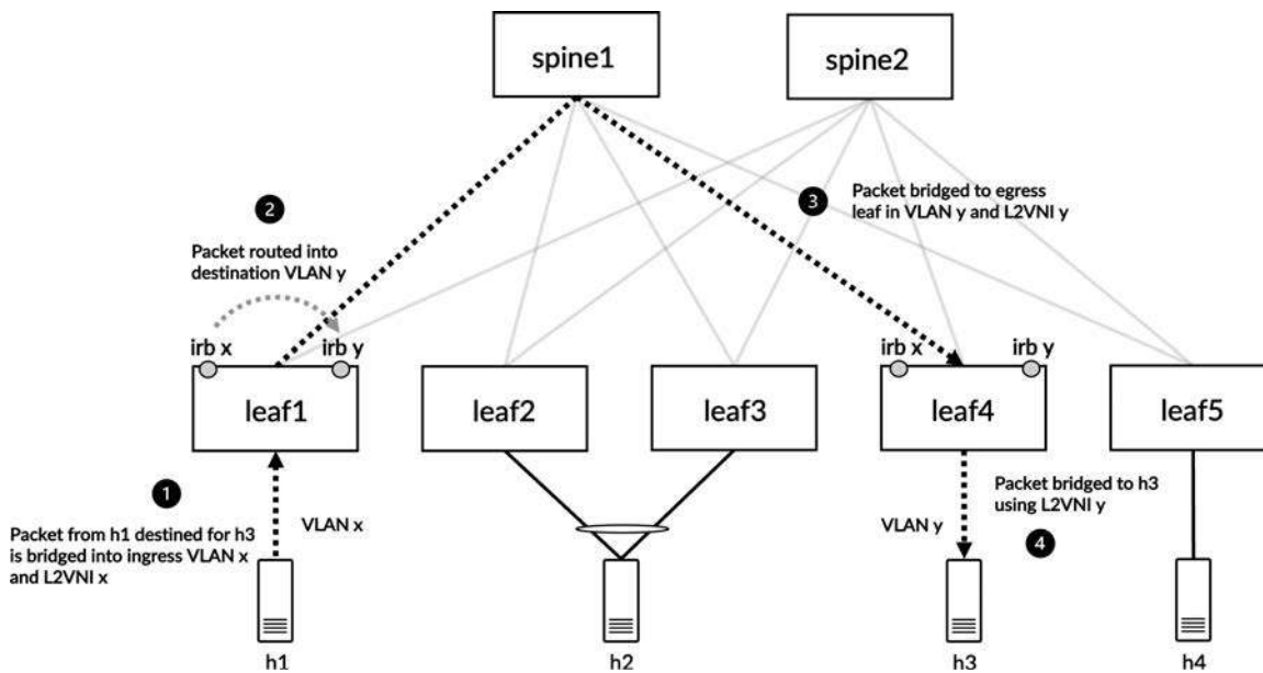
Figure 8-3 Packet flow for inter-subnet traffic with Asymmetric IRB
