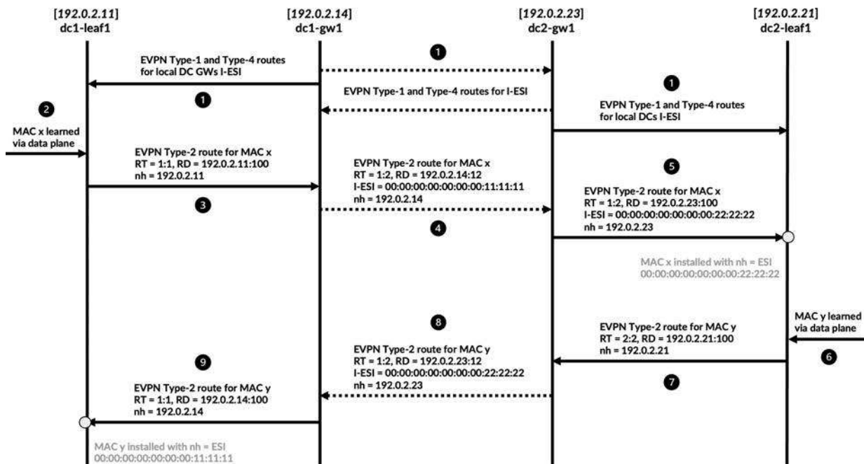
Figure 11-14 Flow diagram showing exchange of EVPN routes with VXLAN stitching
