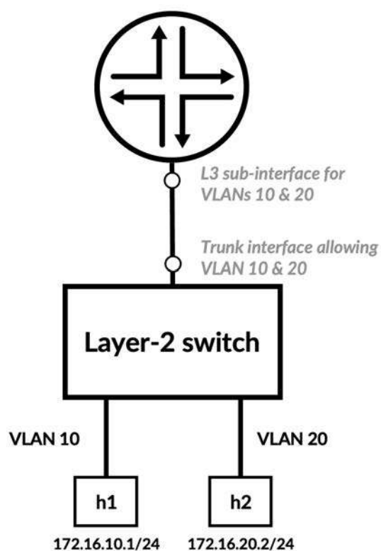
Figure 7-1 Router-on-a-stick design
