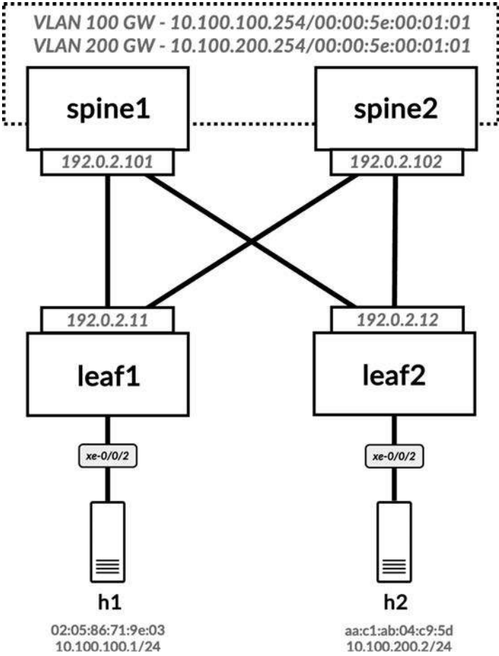
Figure 7-17 Detailed topology as a reference for the packet walk
