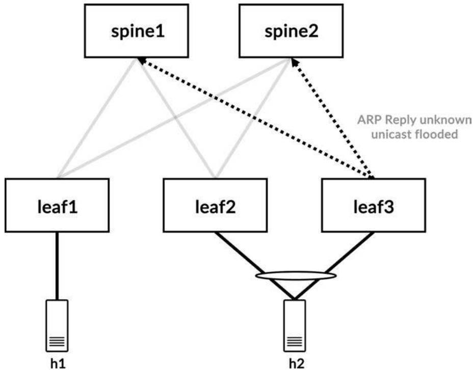
Figure 7-16 ARP reply unknown unicast flooded by leaf3 in the fabric
