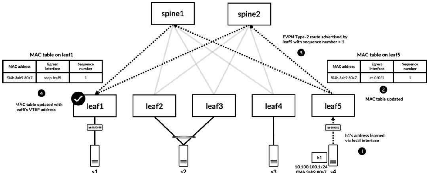
Figure 5-46 Sequence of events when h1 moves from server s1 to server 4
