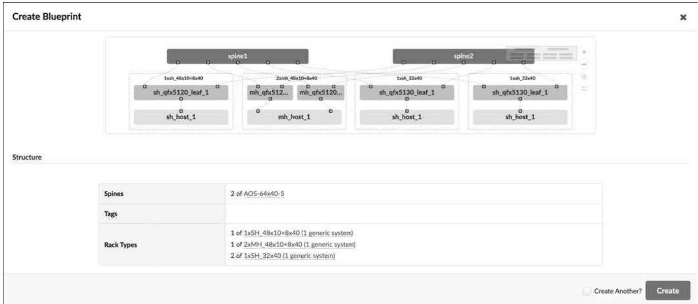
Figure 12-45 Topology preview during Blueprint creation in Apstra UI
