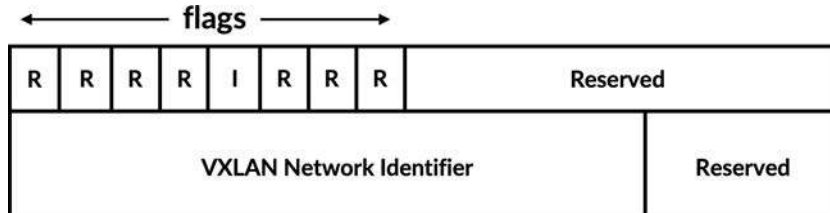
Figure 4-3 Original VXLAN header, defined in RFC 7348
