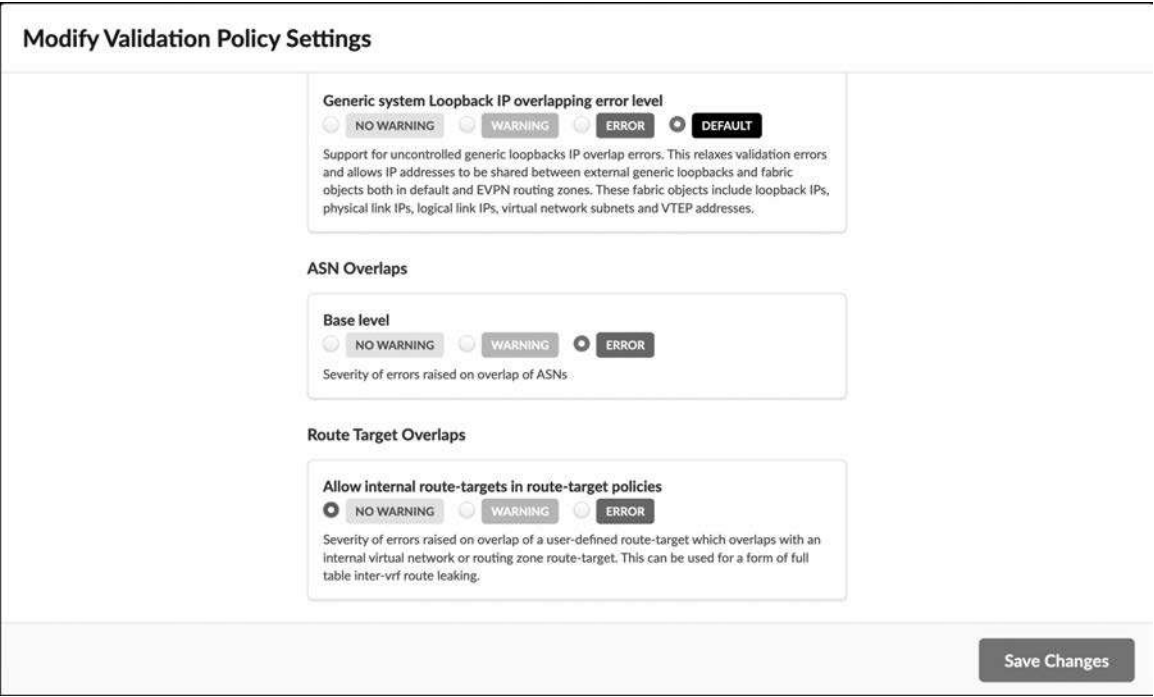
Figure 15-14 Policy change for allowing internal Route Targets in Route Target policies
