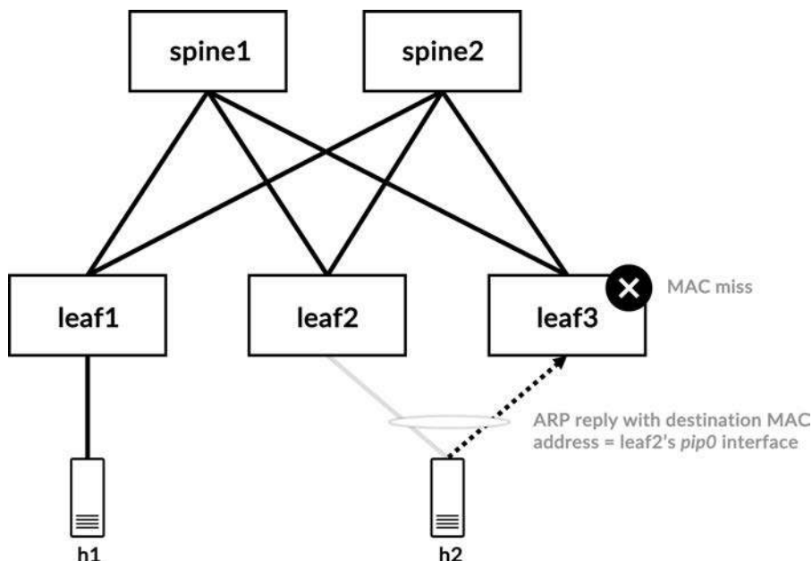
Figure 7-15 ARP reply hashed toward leaf3
