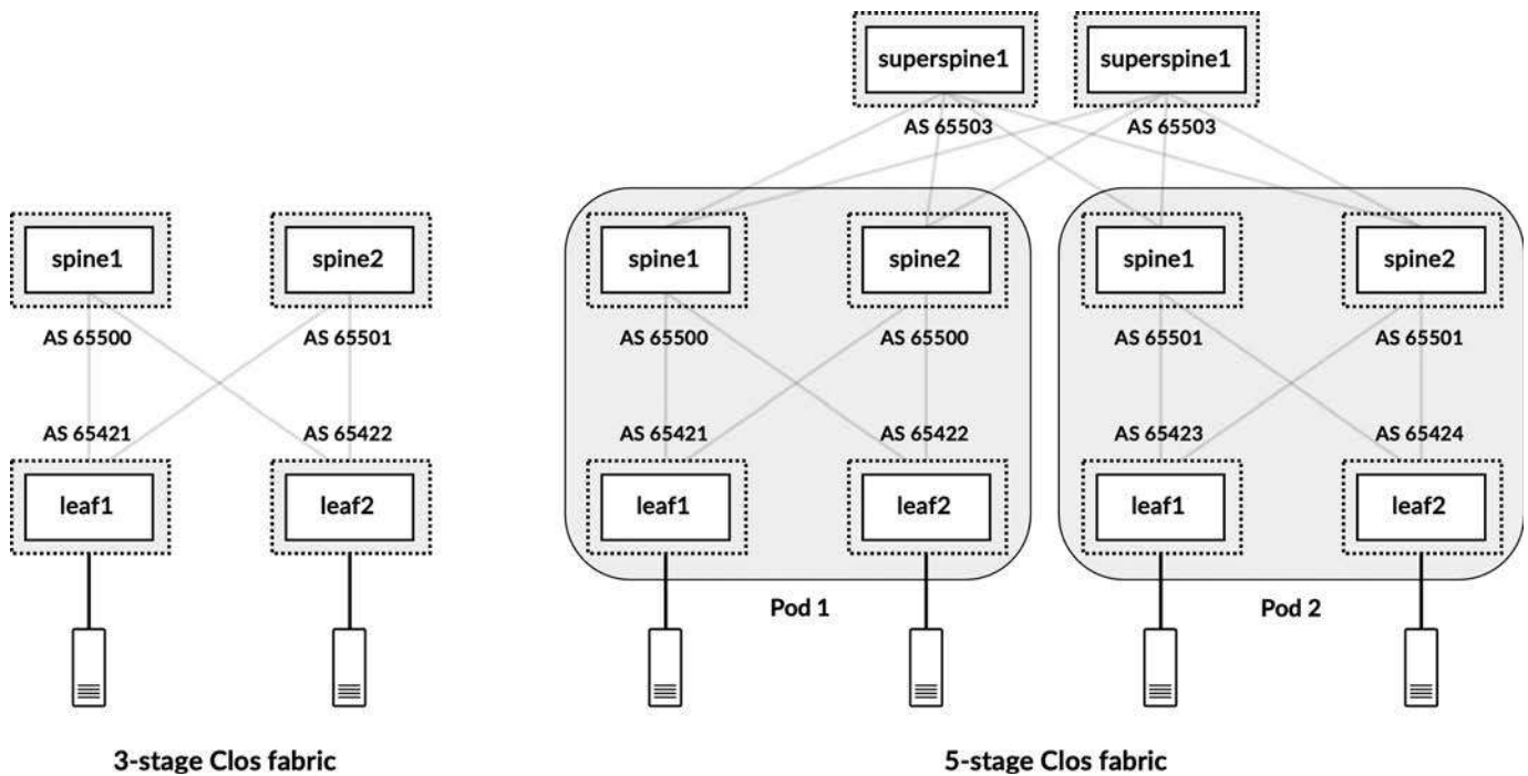
Figure 12-41 ASN schemes for a 3-stage and a 5-stage Clos fabric in Apstra
