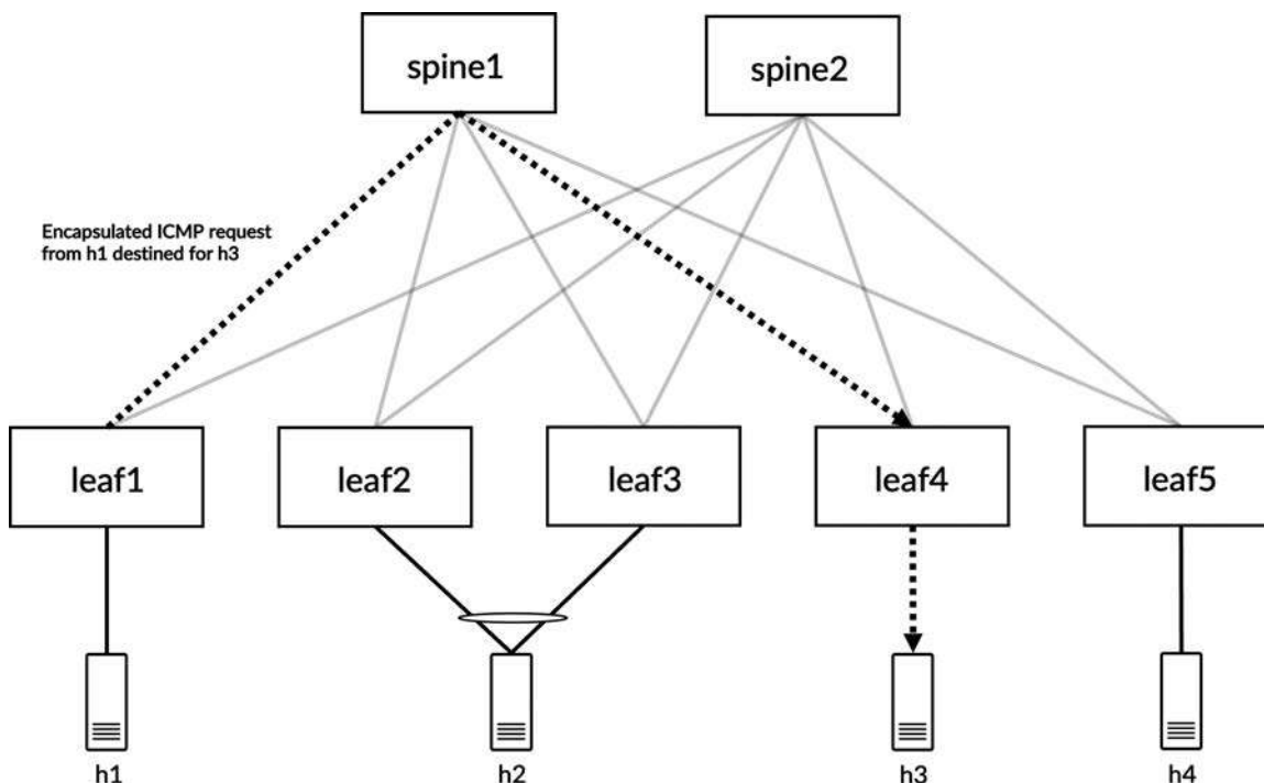
Figure 5-18 Encapsulated ICMP request destined for h3
