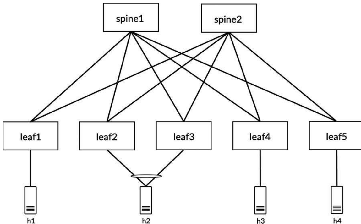
Figure 5-20 Reference topology for replication of BUM traffic
