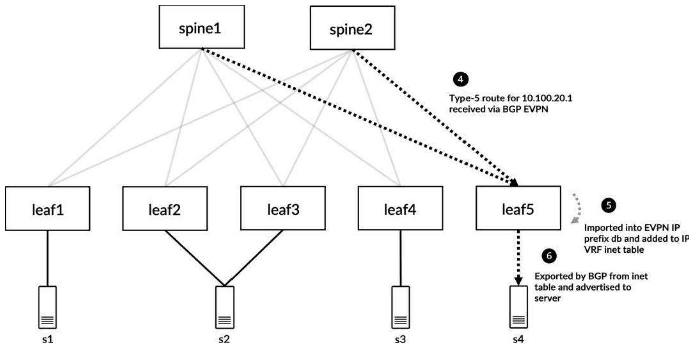
Figure 9-9 EVPN Type-5 route receive process
