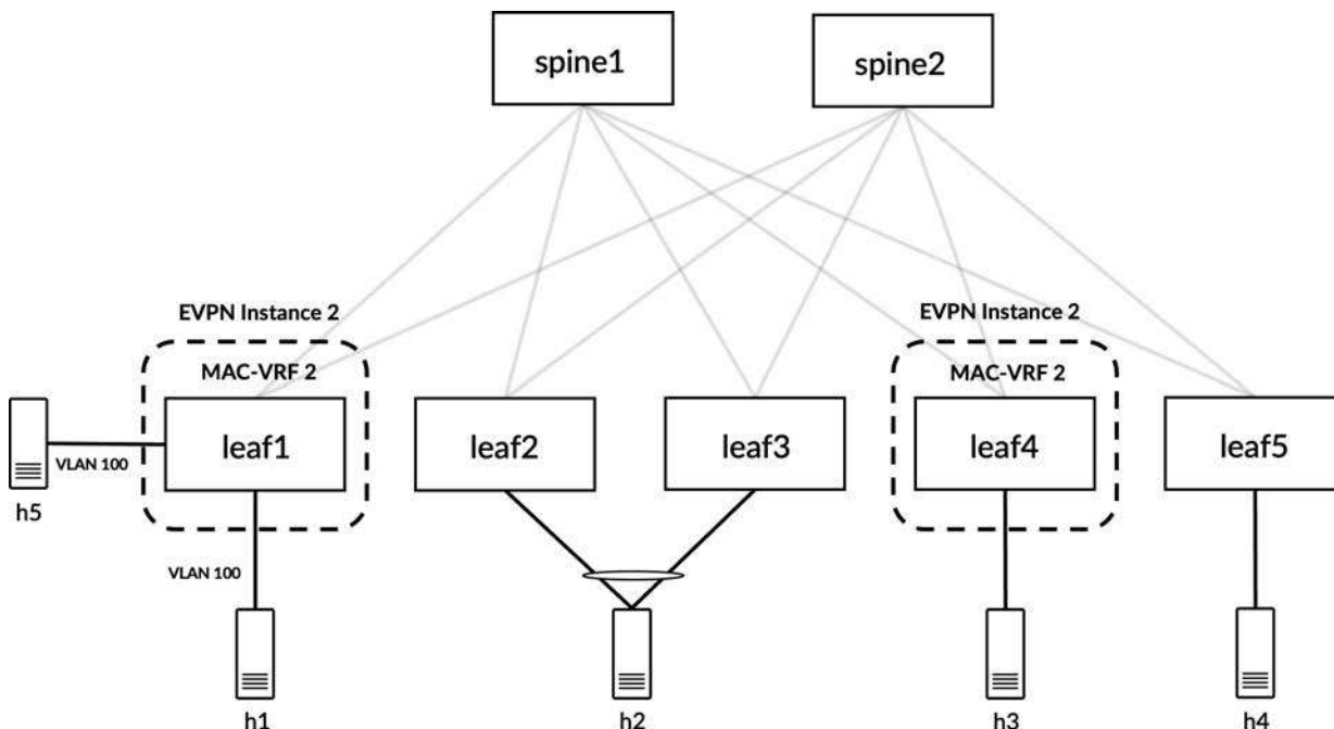
Figure 6-19 Overlapping VLANs for hosts h1 and h5 across two MAC-VRFs
