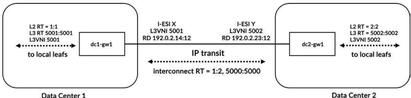
Figure 11-26 DC1 and DC2 route-target and L2VNI/L3VNI design
