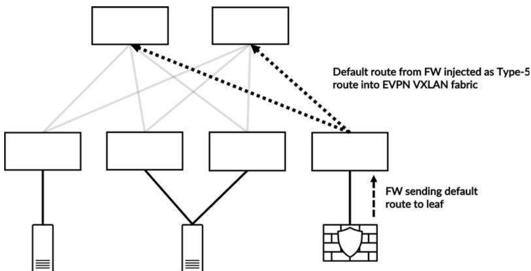
Figure 9-4 Firewall-originated default route injected into EVPN VXLAN fabric as a Type-5 route
