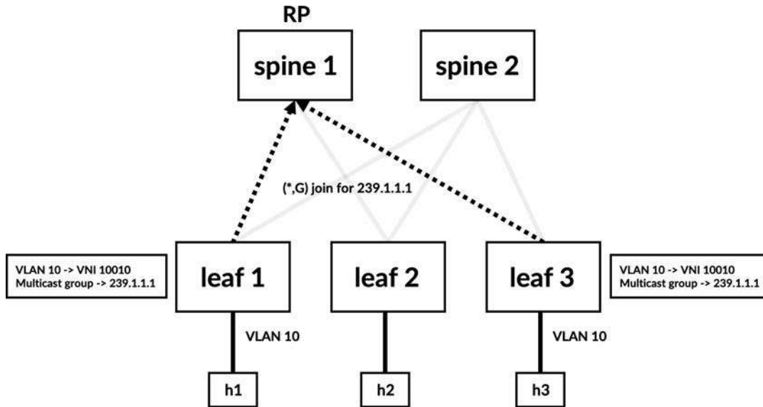
Figure 4-6 3-stage Clos fabric with multicast in the underlay for VXLAN flood-and-learn
