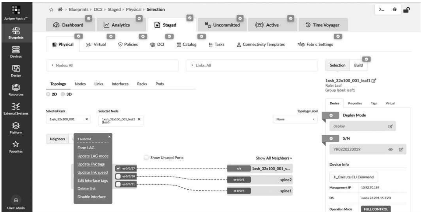
Figure 13-16 Link-specific options in Apstra UI
