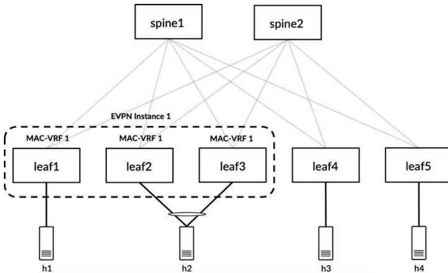
Figure 6-18 Initial reference topology for VLAN normalization
