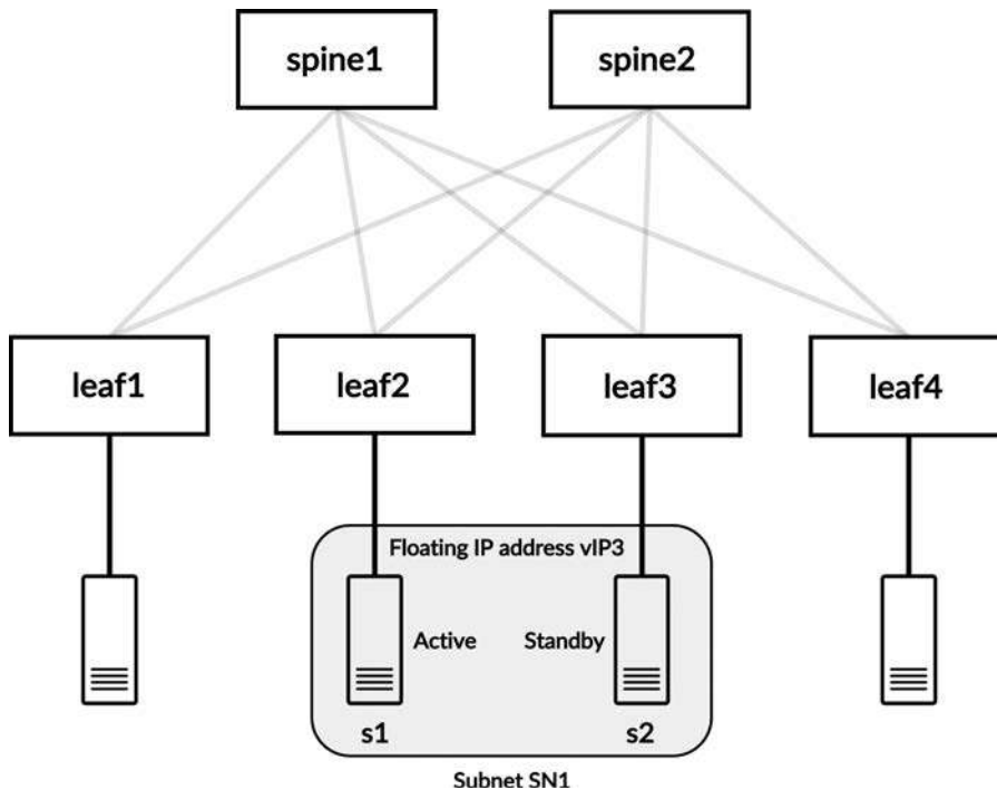
Figure 9-6 Servers with floating IP address
