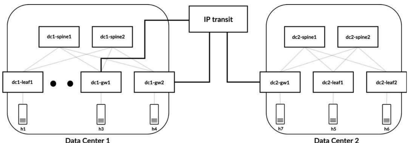
Figure 11-12 Reference topology for two VXLAN domains stitched via an IP transit
