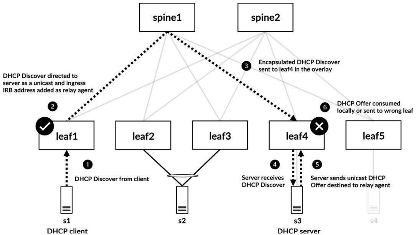
Figure 10-11 Traffic flow problem when using an anycast distributed gateway model with DHCP
