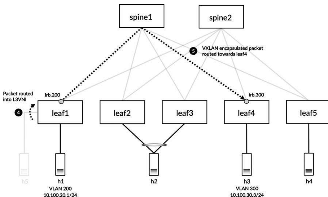
Figure 8-27 Packed routed into L3VNI and routed toward destination VTEP
