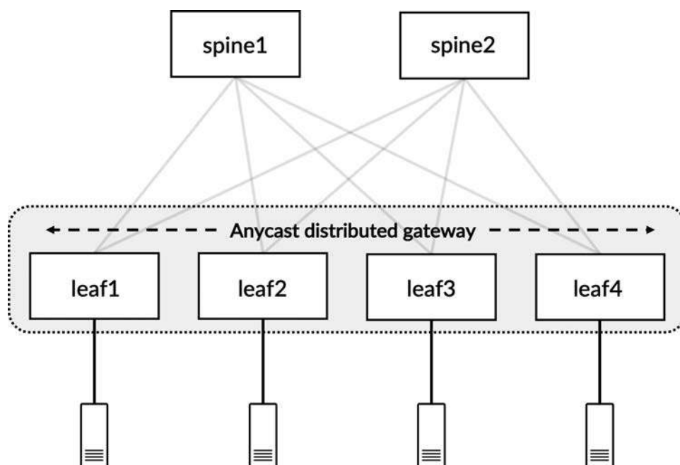
Figure 8-1 Routing on the leaves in an ERB design
