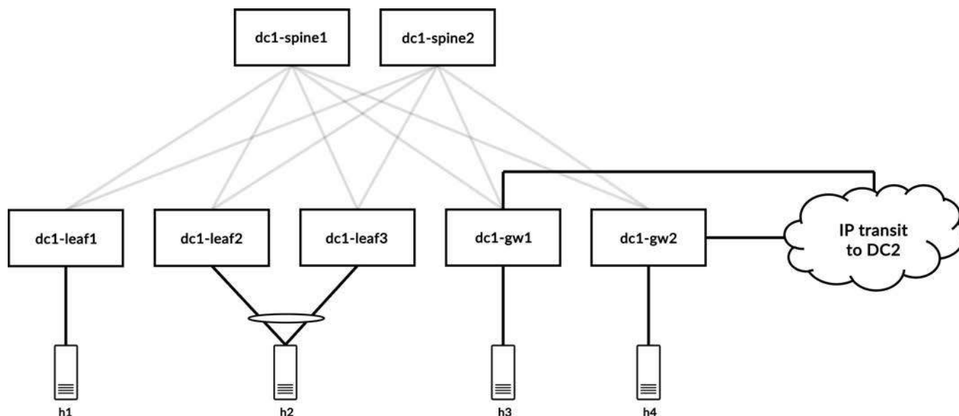
Figure 11-24 Reference topology showing details of DC1
