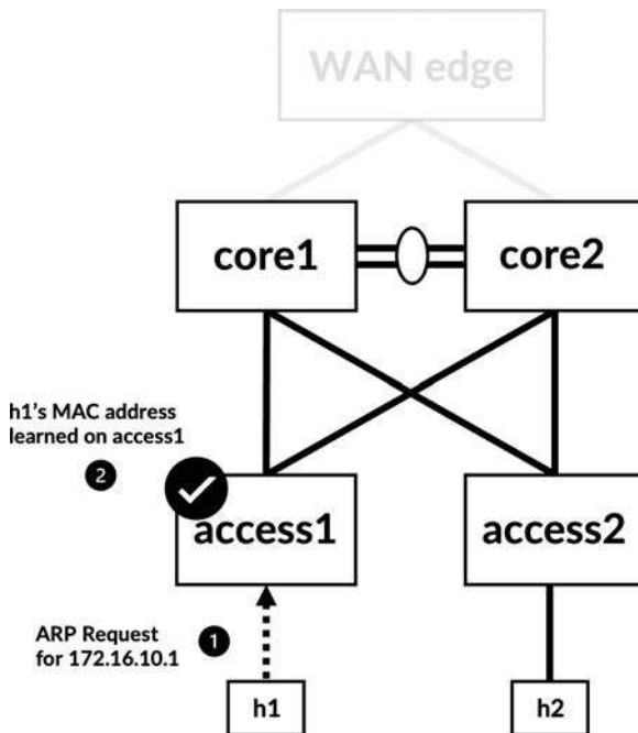
Figure 1-5 Host h1 resolving default gateway using ARP
