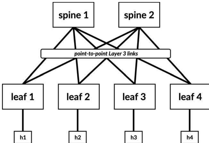
Figure 2-10 3-stage Clos fabric for data center networks with point-to-point links between leafs and spines
