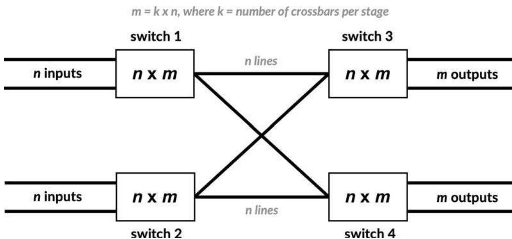
Figure 2-6 A non-blocking n \times m 2-stage crossbar interconnection
