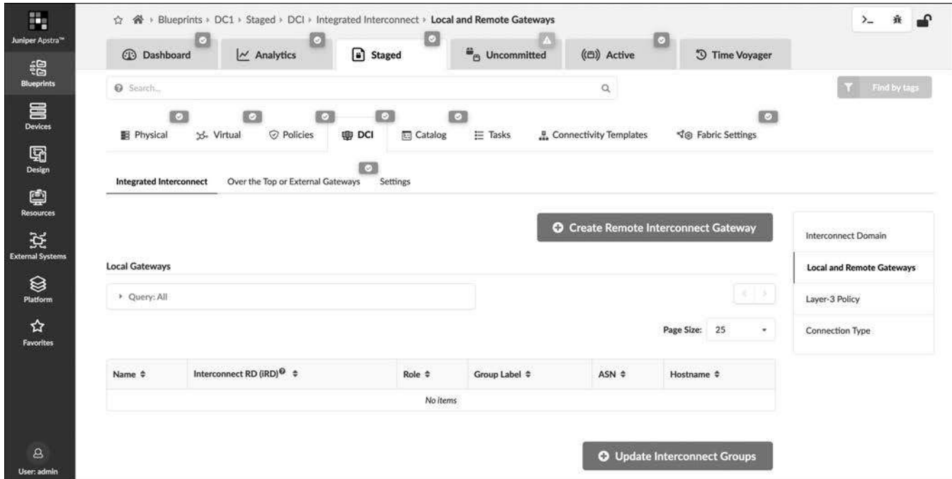
Figure 13-47 Apstra UI page to create remote BGP EVPN peers for Integrated Interconnect
