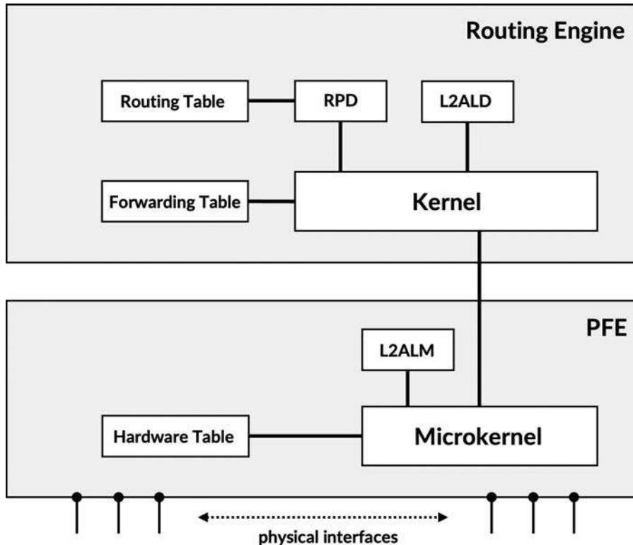
Figure 1-1 Junos OS high-level architecture
