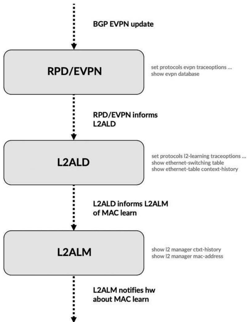
Figure 5-14 Sequence of events on a remote leaf when a BGP EVPN update is received
