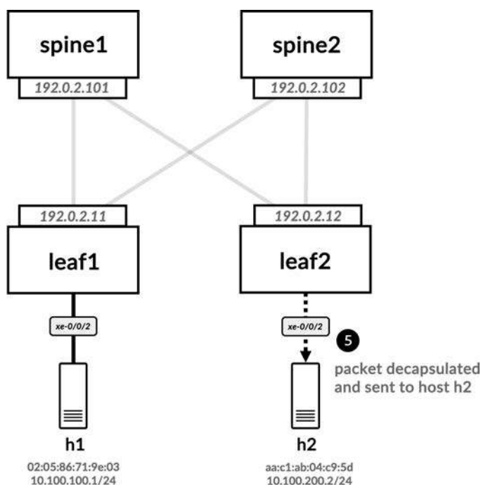
Figure 7-27 Packet decapsulated on leaf2 and bridged to host h2
