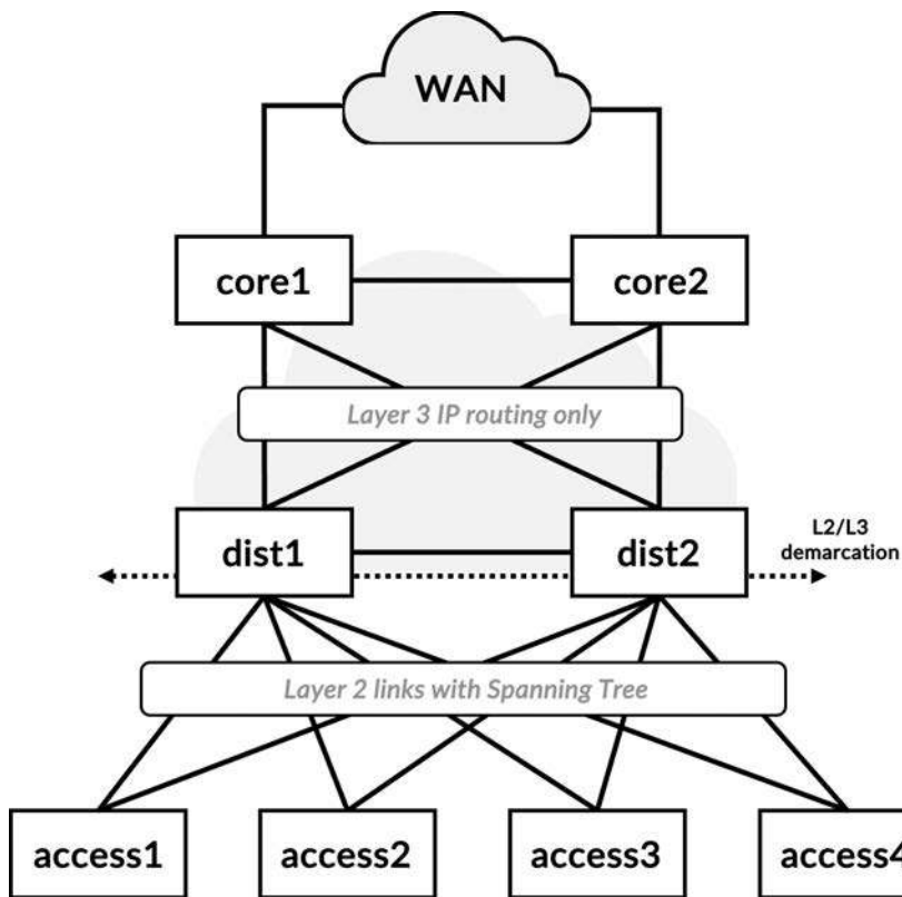
Figure 2-1 Three-tier data center architecture
