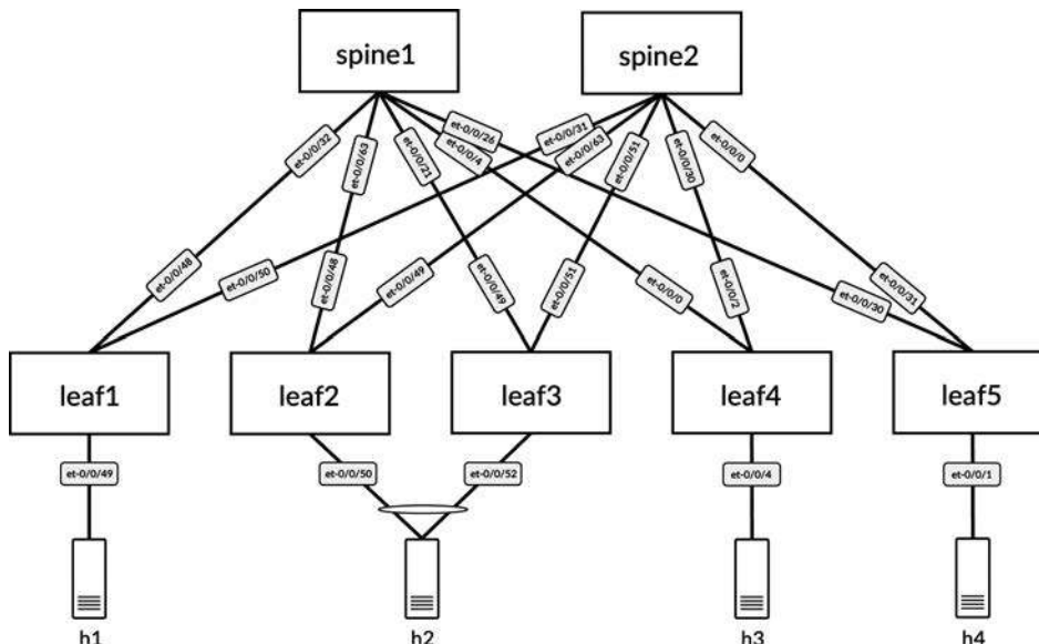
Figure 5-2 Reference topology to build a bridged overlay EVPN VXLAN fabric
