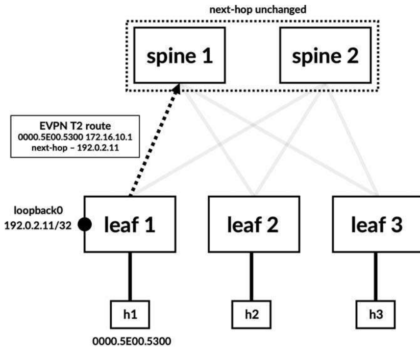
Figure 4-8 The spines, in a 3-stage Clos fabric, configured to not change the next-hop for BGP EVPN routes
