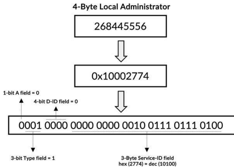
Figure 5-43 Breakdown of an auto-derived Route Target added to an EVPN Type-2 route advertised by leaf2
