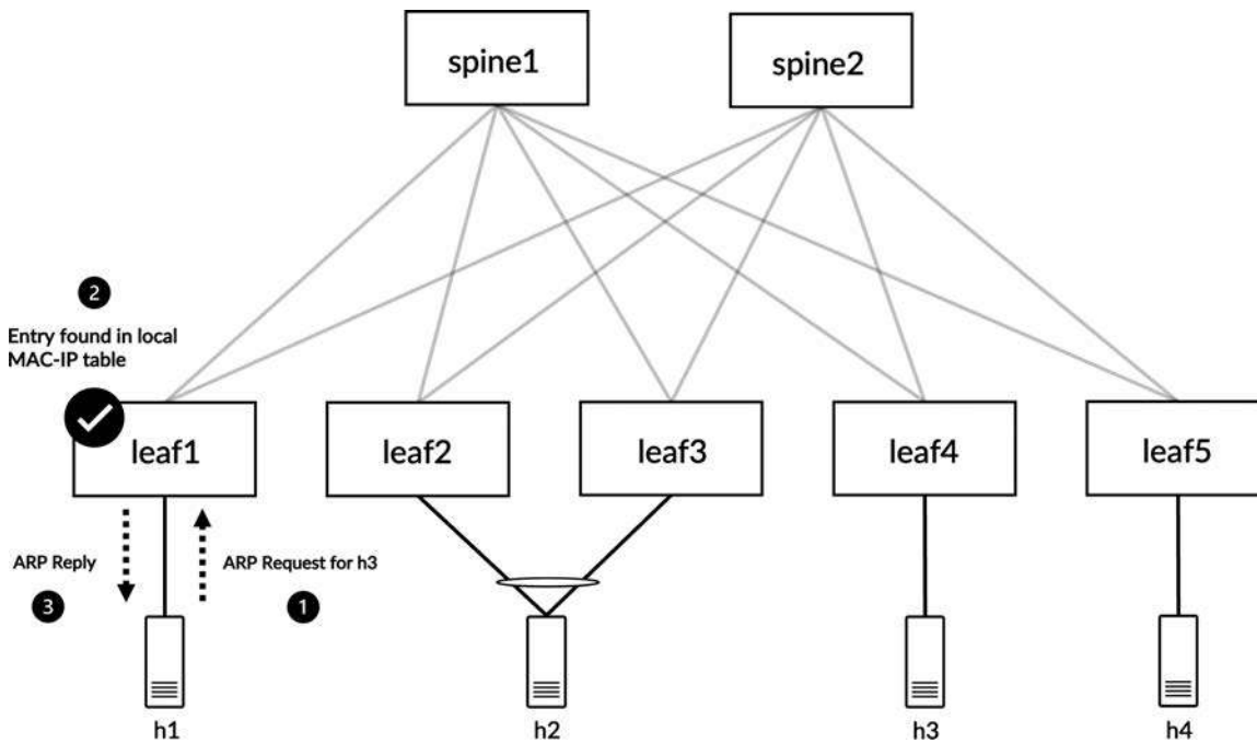
Figure 5-17 Visual representation of proxy ARP and ARP suppression from the perspective of leaf1
