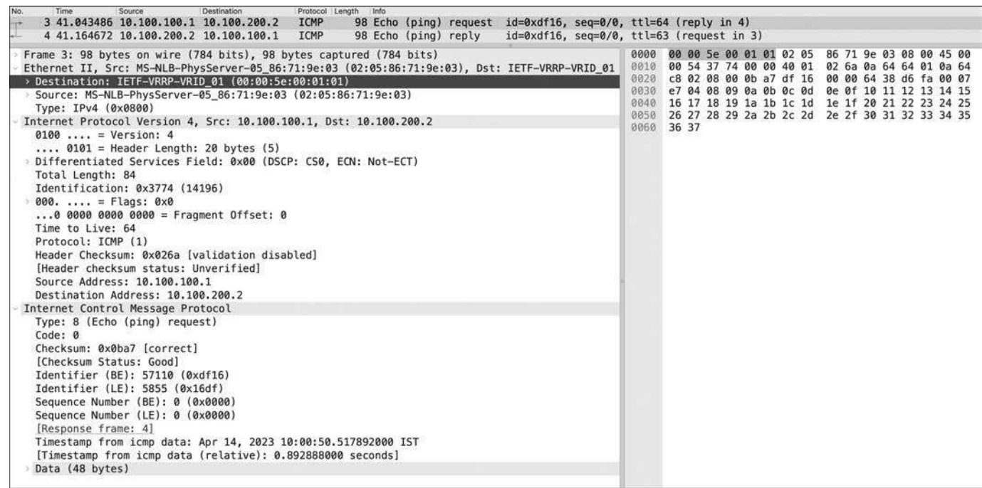
Figure 7-22 Packet capture showing ICMP request from h1 destined for h2
