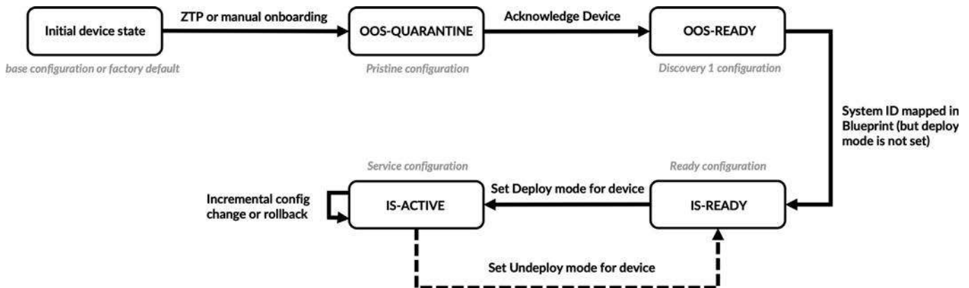
Figure 12-76 Lifecycle of a device in Apstra
