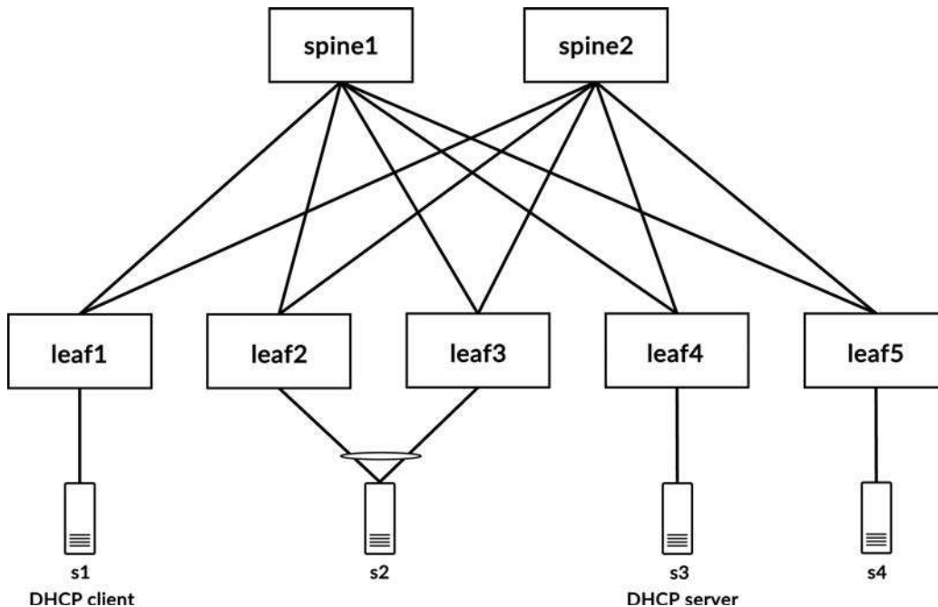
Figure 10-3 Reference topology for DHCP in a bridged overlay fabric
