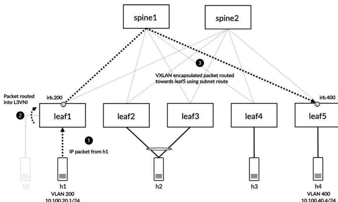
Figure 8-30 Packet routed toward egress leaf using subnet route
