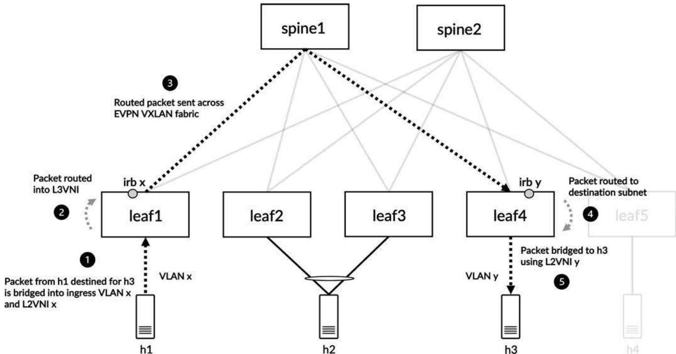
Figure 11-22 Packet flow with Symmetric IRB
