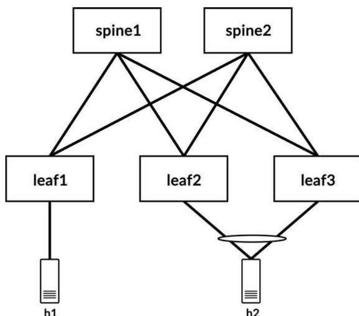
Figure 7-12 Host h2 multihomed to leaf2 and leaf3 via ESI LAG
