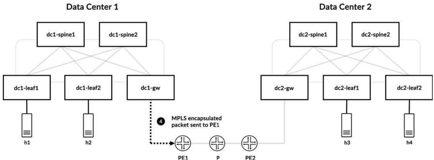
Figure 11-37 MPLS-encapsulated packet from dc1-gw to PE1
