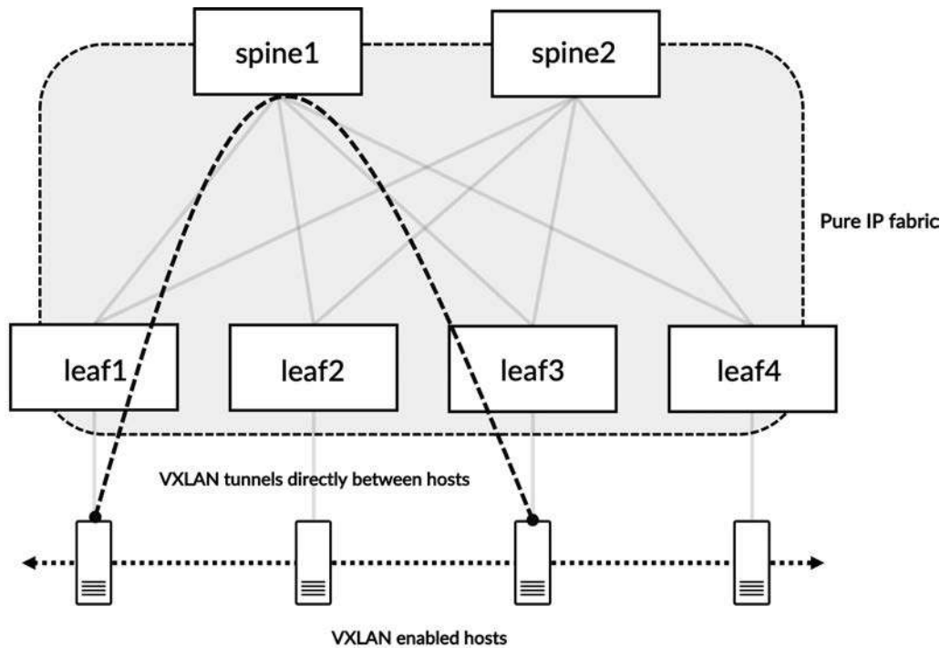
Figure 9-11 Host-routed bridging with direct VXLAN tunnels between hosts
