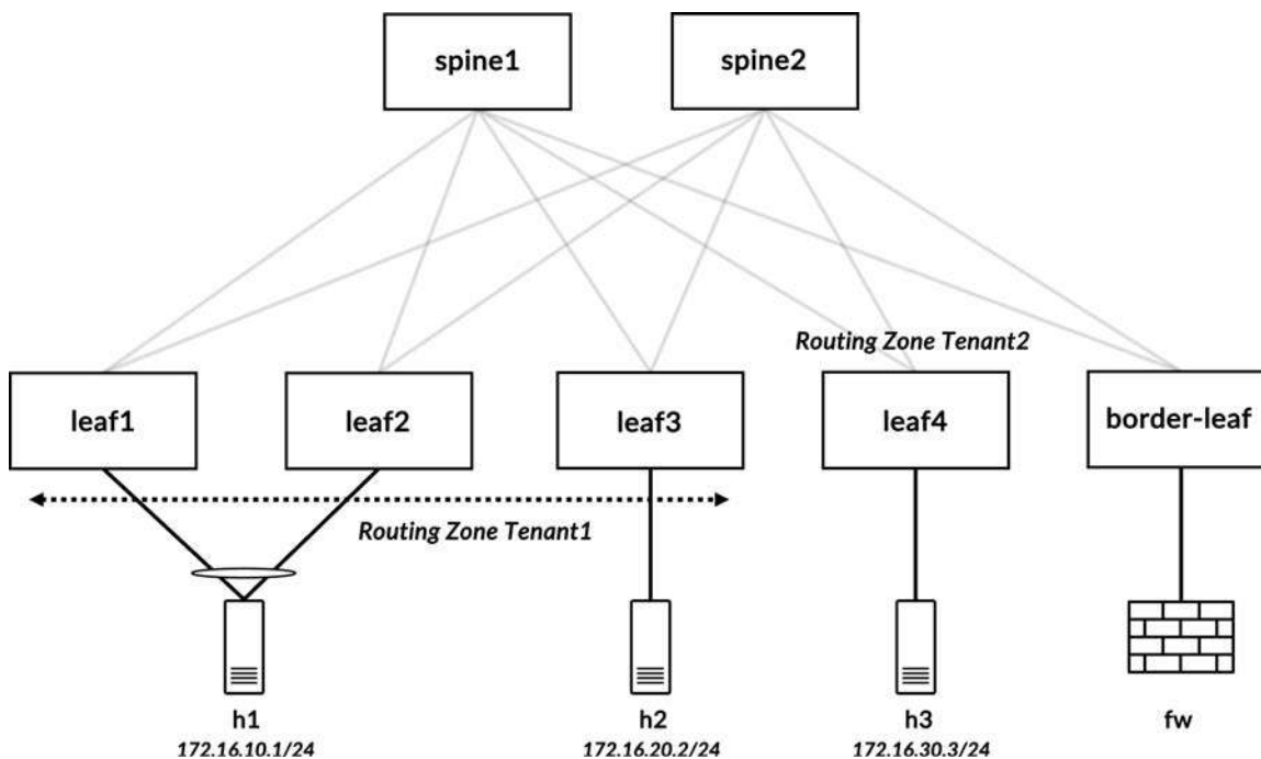
Figure 15-10 Topology for inter-VRF routing
