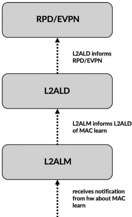
Figure 7-18 Sequence of events for a MAC learn via data plane
