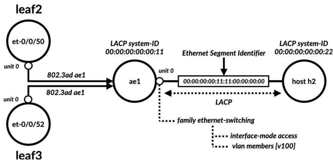
Figure 5-26 Object association for an Ethernet Segment-enabled AE interface using LACP
