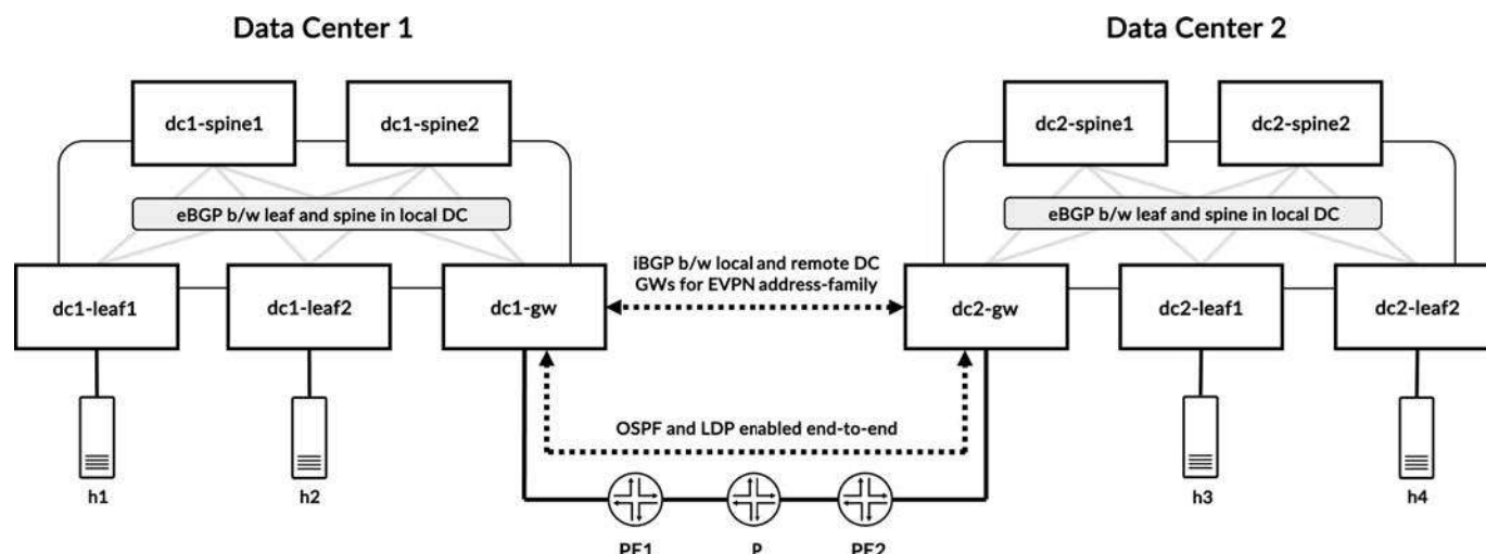
Figure 11-32 Overall design for VXLAN stitching with an MPLS transit
