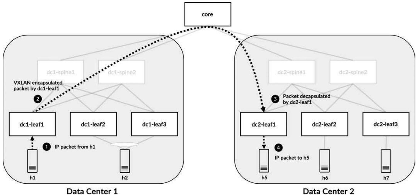
Figure 11-9 Traffic flow from DC1 to DC2 when hosts in the same subnet communicate with each other
