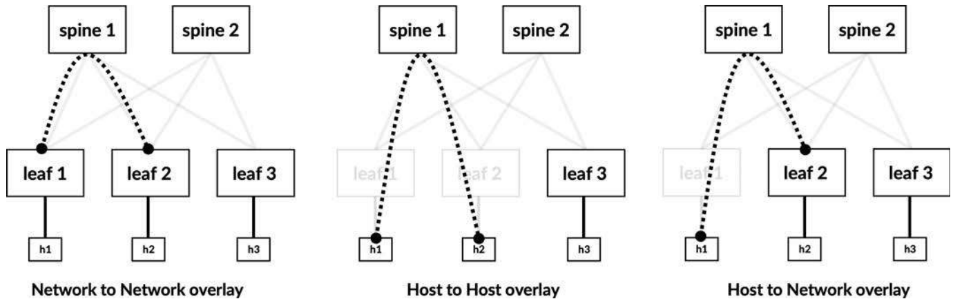
Figure 4-1 VXLAN overlay origination and termination options
