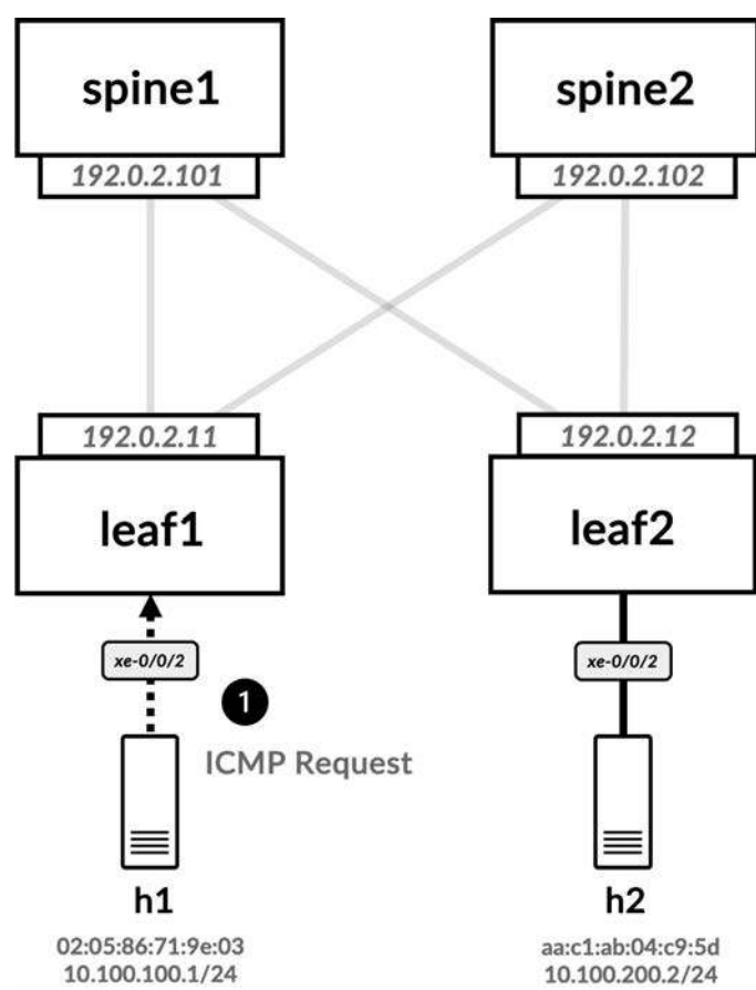
Figure 7-21 ICMP request from h1 destined for h2
