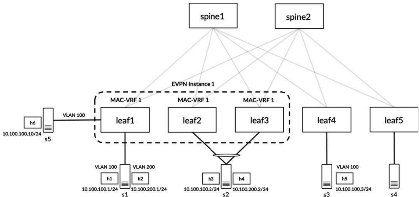
Figure 6-15 Visual representation of MAC-VRF macvrf-v100-v200-1 with new server s5 connected to leaf1
