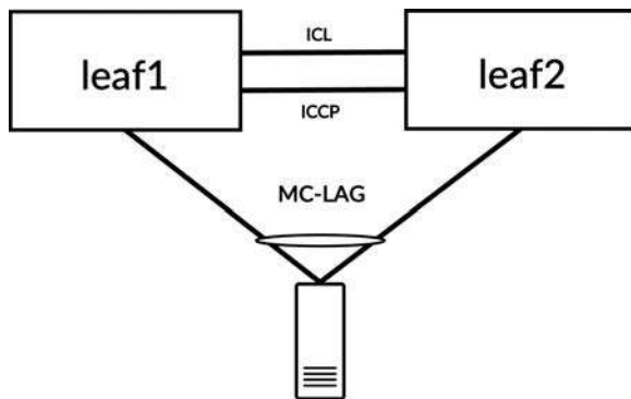
Figure 5-23 Example topology for MC-LAG
