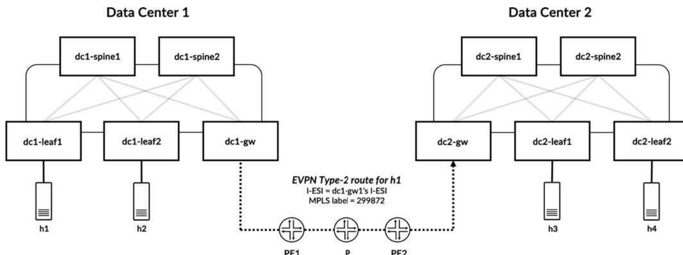
Figure 11-33 iBGP EVPN route sent from dc1-gw to dc2-gw for host h1's address
