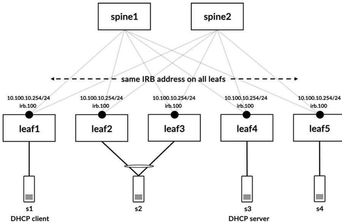
Figure 10-10 Anycast distributed gateway in an ERB fabric design
