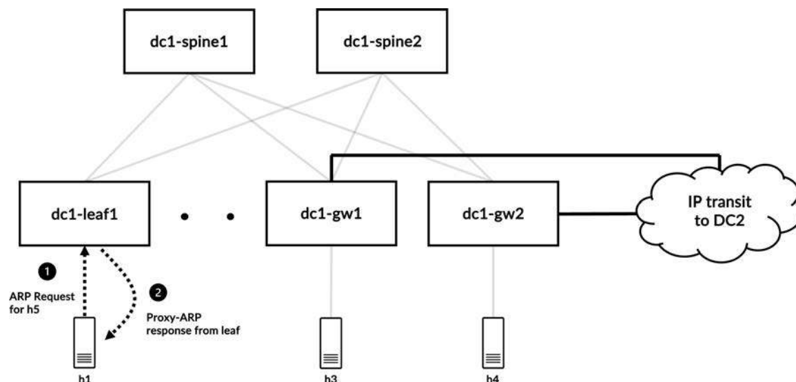
Figure 11-15 Proxy ARP response from dc1-leaf1 for an ARP request for host h5 (in DC2)
