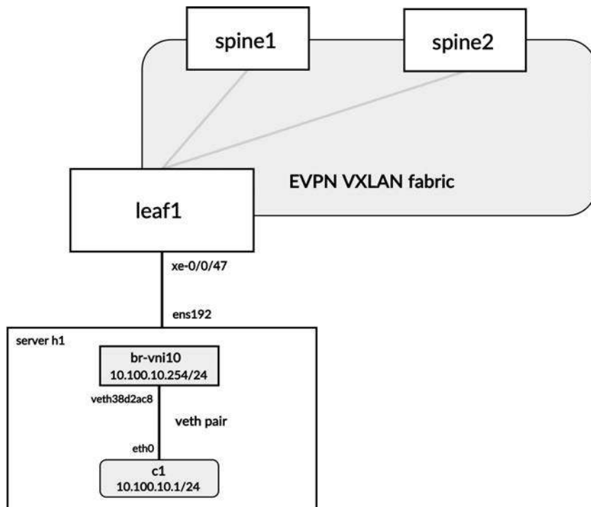
Figure 9-13 Container c1 internal connection to Docker bridge br-vni10
