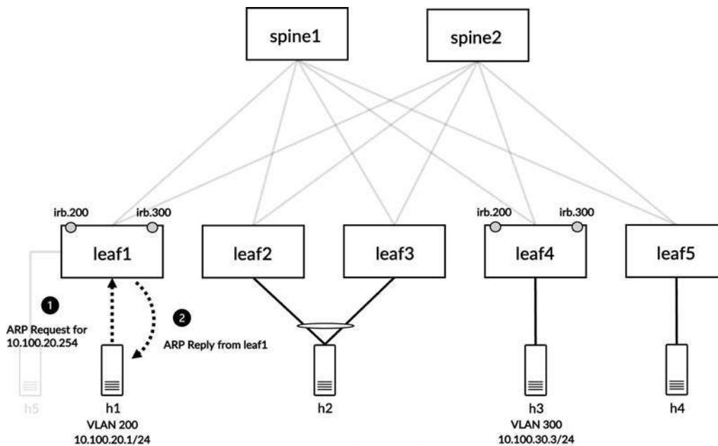
Figure 8-10 Host h1 resolving its gateway address
