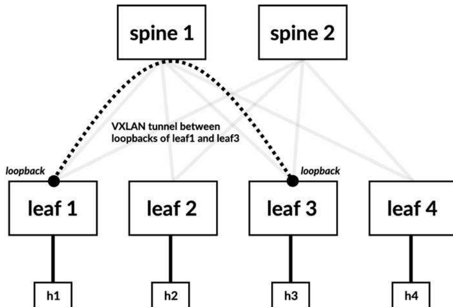
Figure 2-12 Overlay in a VXLAN 3-stage Clos fabric
