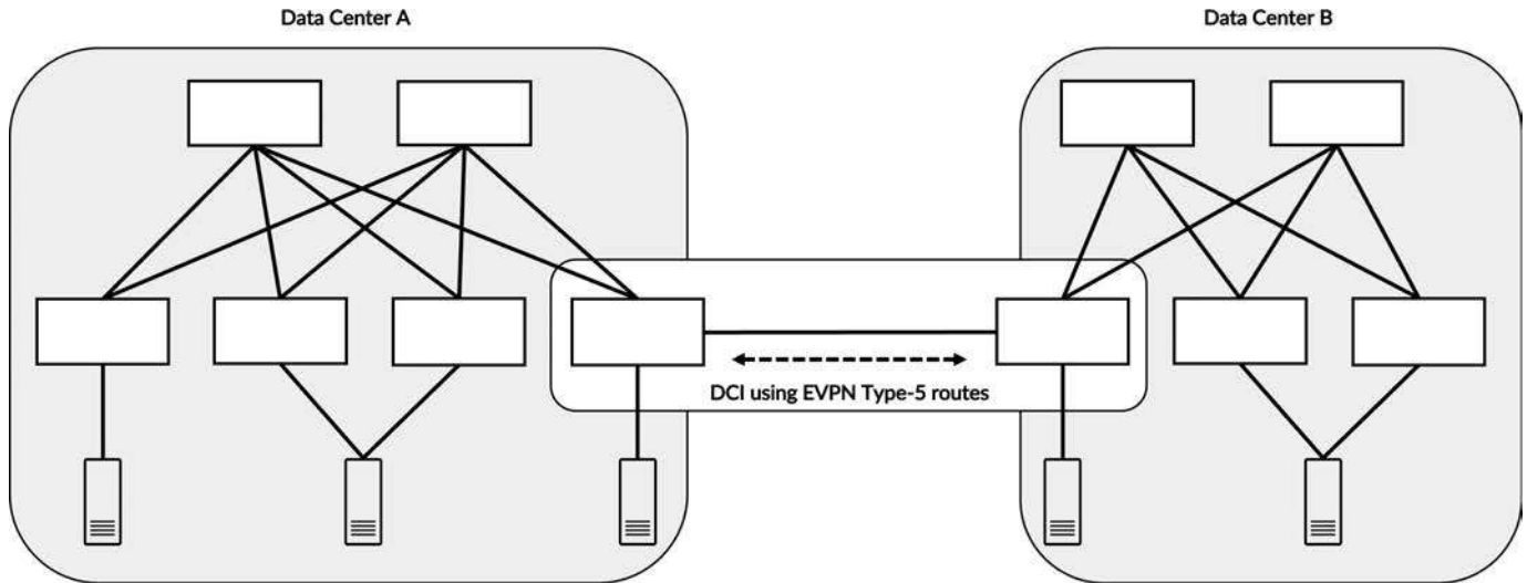
Figure 9-3 Connecting data centers using EVPN Type-5 routes
