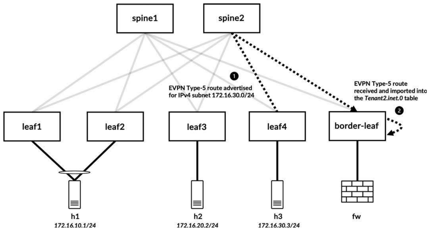
Figure 15-20 IPv4 subnet 172.16.30.0/24 advertised by leaf4, received by the border leaf, and imported into inet.0 table
