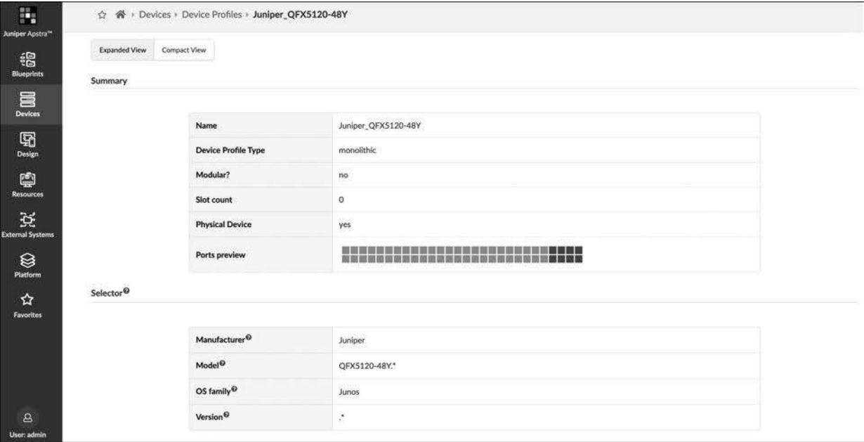
Figure 12-3 Device Profile for a Juniper QFX5120-48Y shown in the Apstra UI
