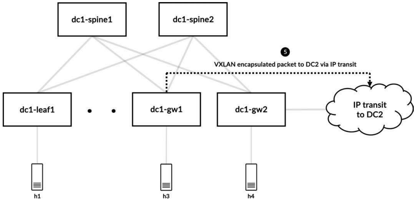
Figure 11-19 VXLAN-encapsulated packet sent toward DC2 via the IP transit
