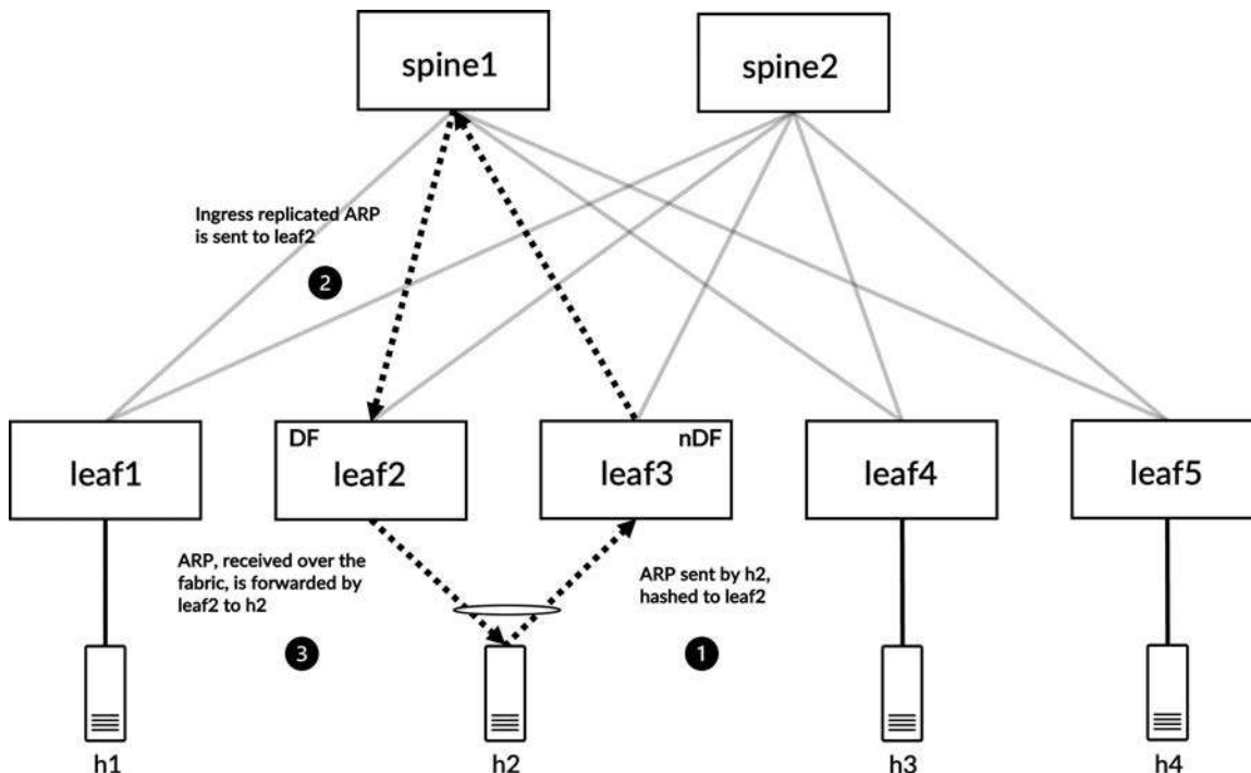
Figure 5-36 BUM traffic, originated by h2, when hashed to nDF of a segment is forwarded by leaf2 to the same host
