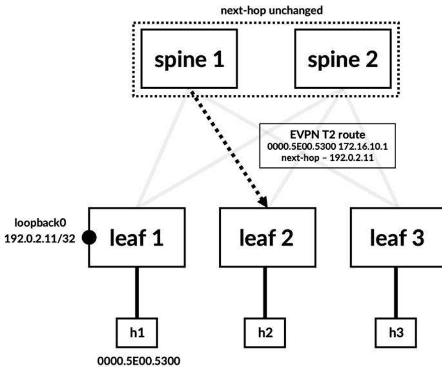
Figure 4-9 EVPN Type-2 route advertised by the spines to leaf2 without changing next-hop
