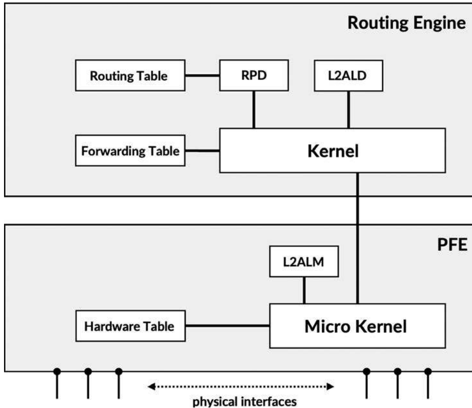
Figure 5-10 A high-level software architectural view of components involved in MAC learning
