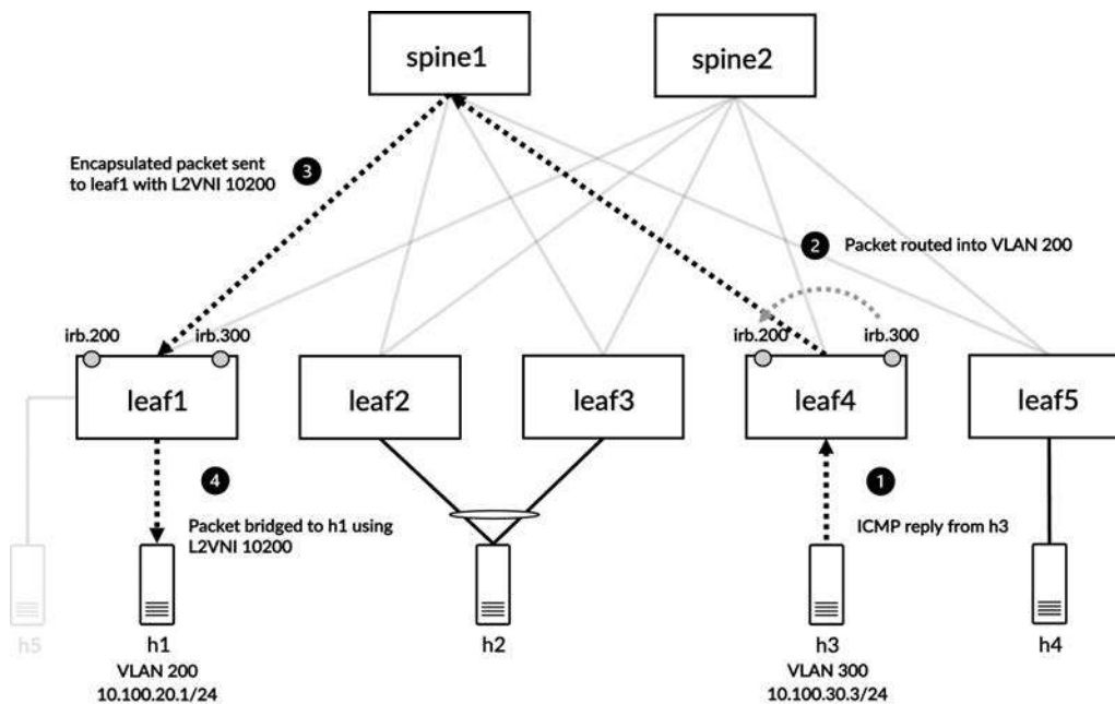
Figure 8-15 Packet flow for ICMP reply from h3 destined to h1
