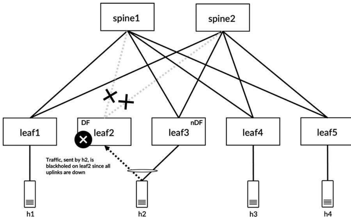
Figure 5-38 Traffic that is hashed to leaf2, from h2, is dropped since all uplinks are down
