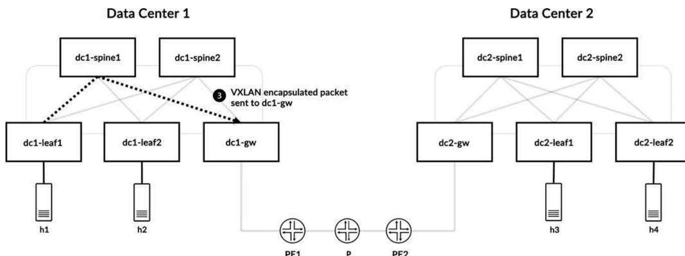
Figure 11-36 VXLAN-encapsulated packet from dc1-leaf1 to dc1-gw
