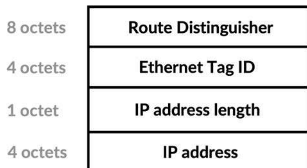
Figure 4-12 EVPN Type-3 route NLRI packet format
