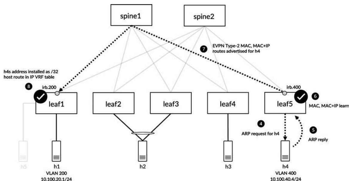
Figure 8-31 Gleaning process for silent hosts
