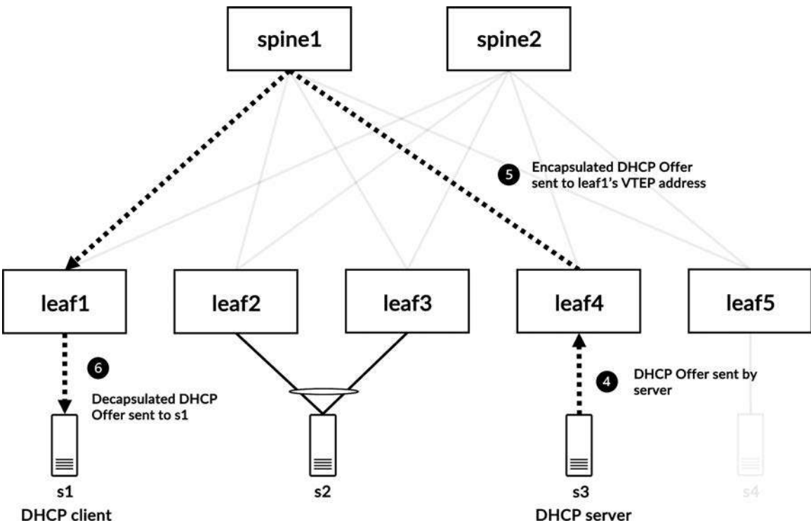
Figure 10-7 DHCP Offer sent from server to client as a unicast packet
