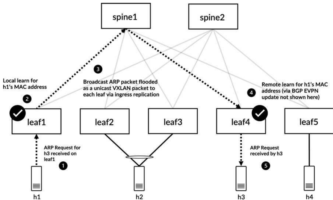
Figure 5-6 High-level packet flow for an ARP request from h1 for h3
