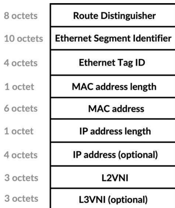
Figure 4-11 EVPN Type-2 route NLRI packet format
