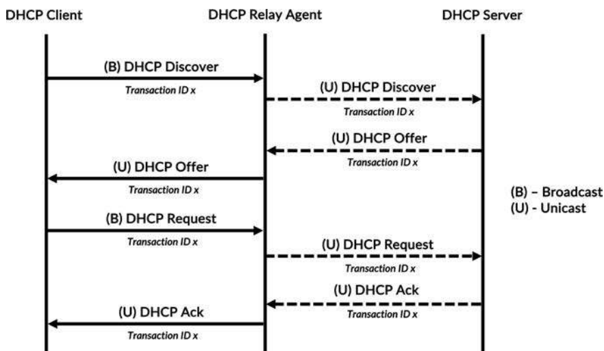
Figure 10-2 DHCP DORA process with a DHCP relay agent
