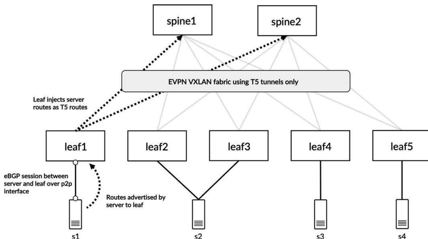
Figure 9-2 Routed overlay with EVPN VXLAN design overview
