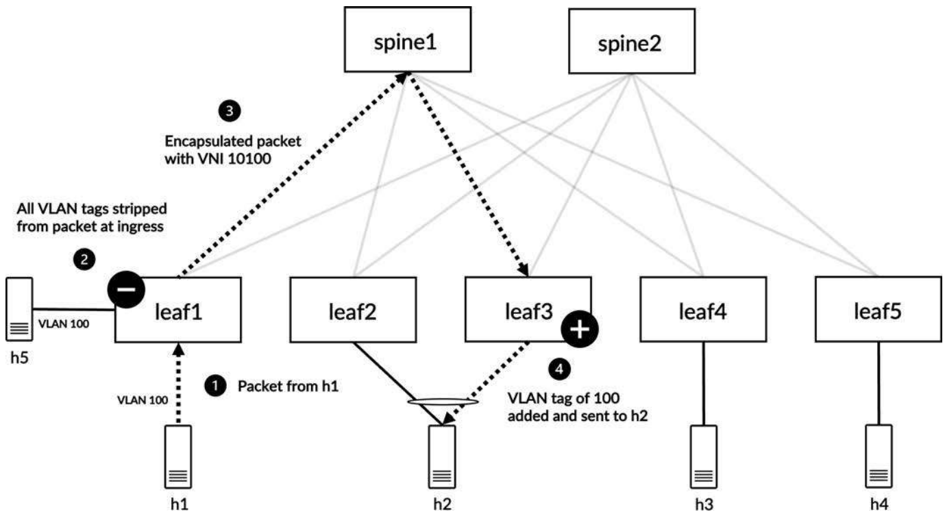
Figure 6-20 Traffic flow for a packet from host h1 to h2 with VLAN normalization to VLAN ID of none
