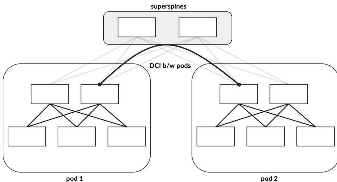
Figure 11-1 DCI between pods
