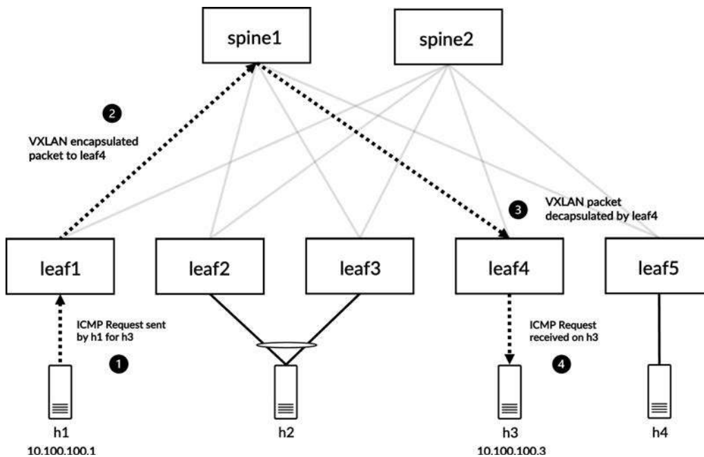
Figure 5-9 Flow of ICMP request through the EVPN VXLAN fabric
