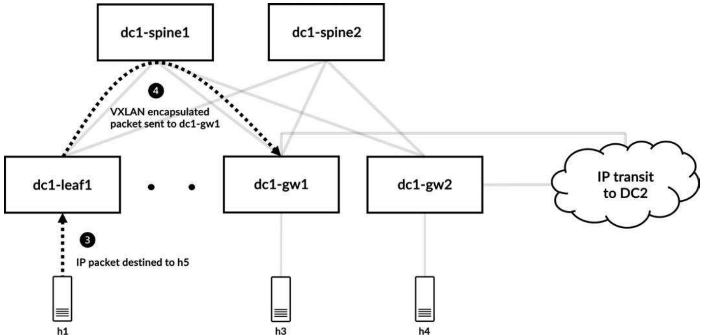
Figure 11-16 VXLAN-encapsulated packet sent to dc1-gw1 to exit toward DC2
