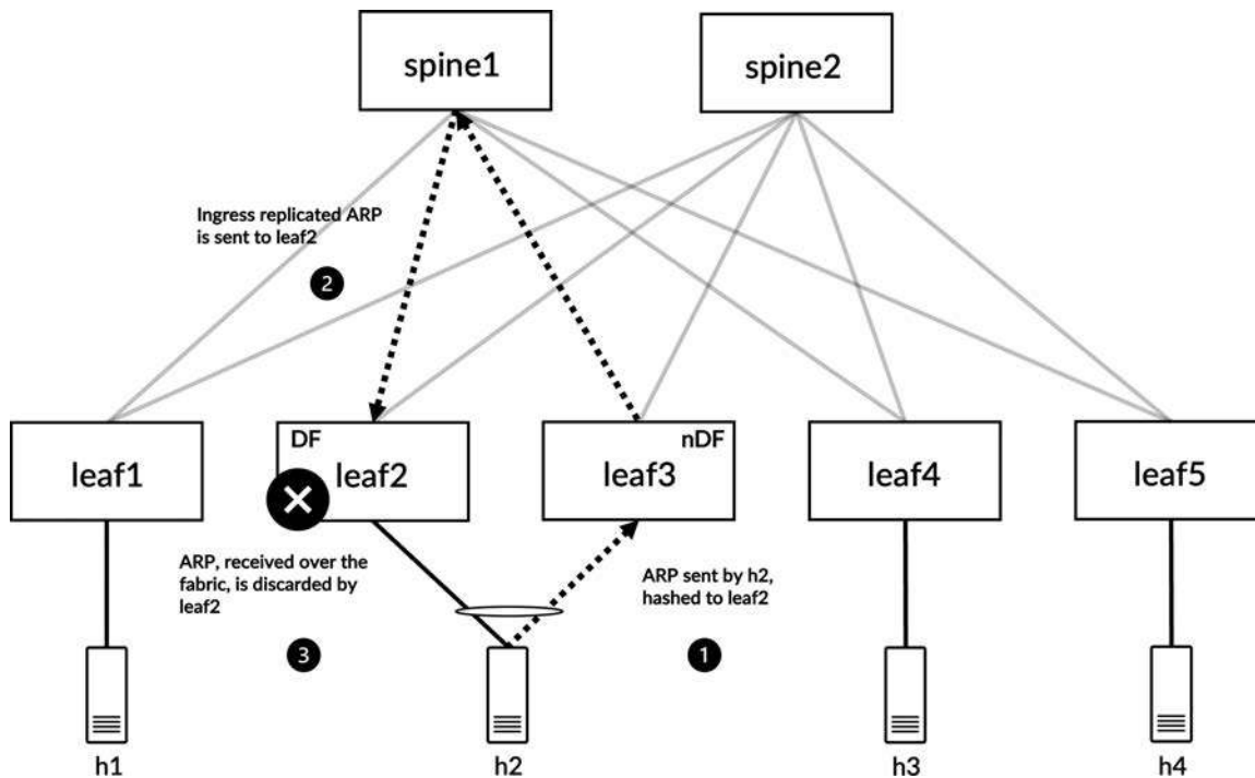
Figure 5-37 BUM traffic, originated by h2, when hashed to nDF is discarded by DF, leaf2, when received over the fabric
