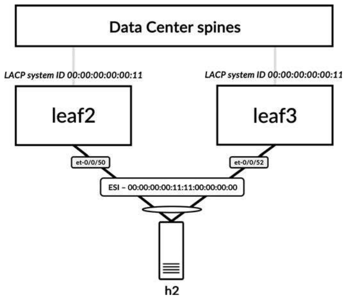
Figure 5-25 EVPN multihoming details for leaf2 and leaf3
