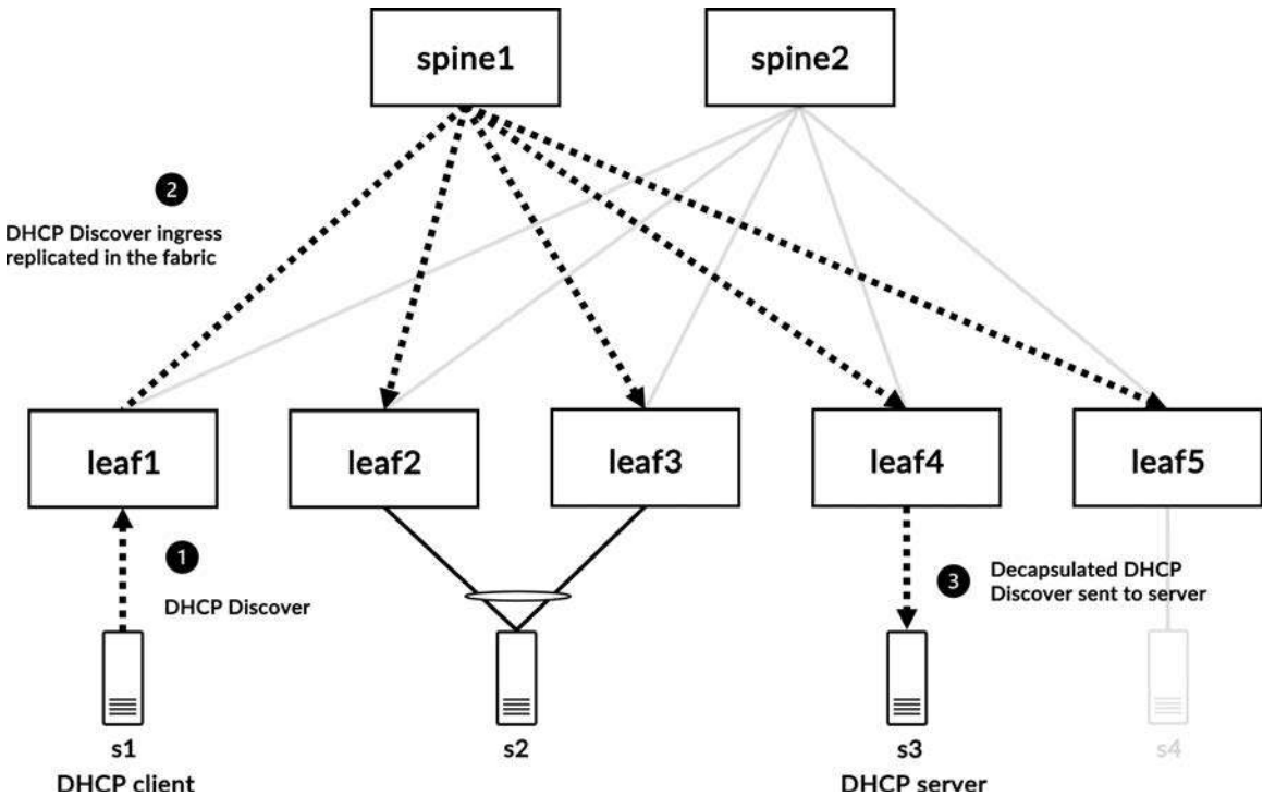
Figure 10-5 DHCP Discover flooded in the fabric
