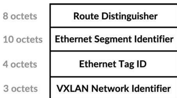
Figure 4-10 EVPN Type-1 route NLRI packet format
