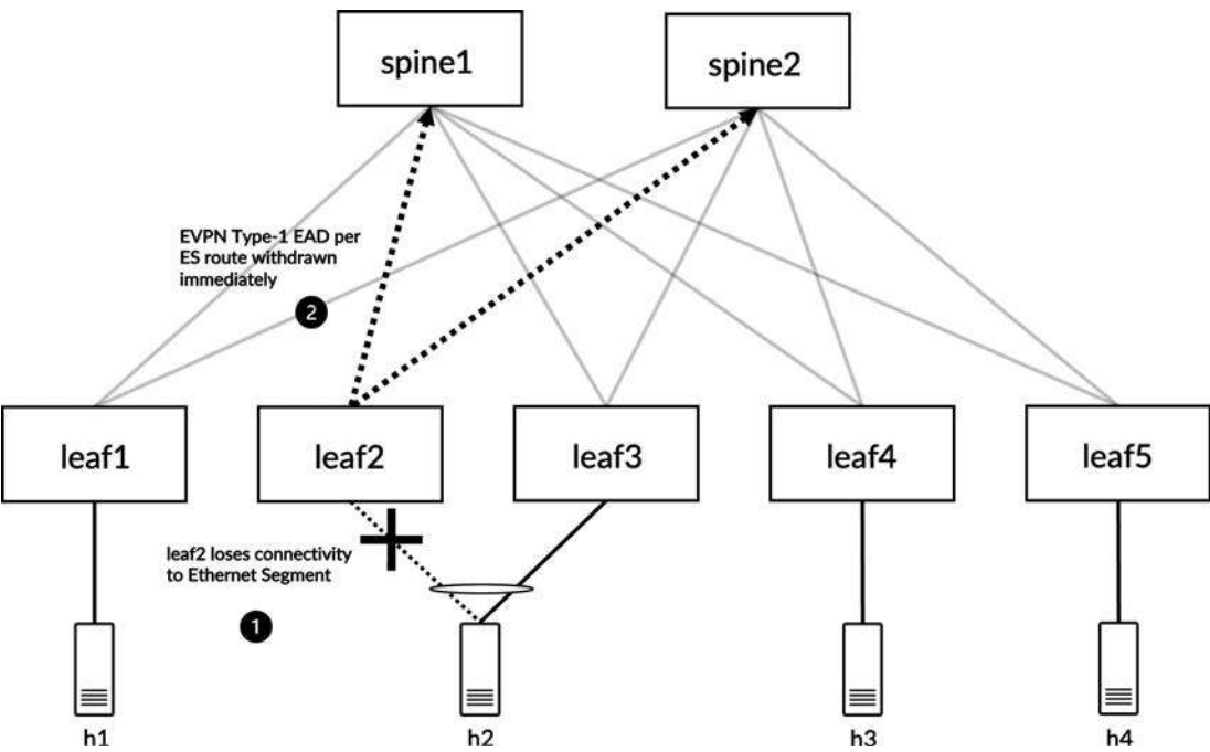
Figure 5-34 Type-1 EAD per ES route withdrawn when leaf2 loses connectivity to the Ethernet Segment
