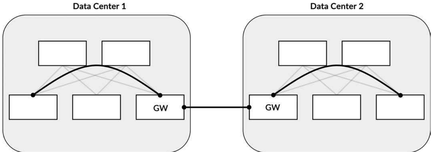
Figure 11-11 VXLAN tunnels with Integrated Interconnect
