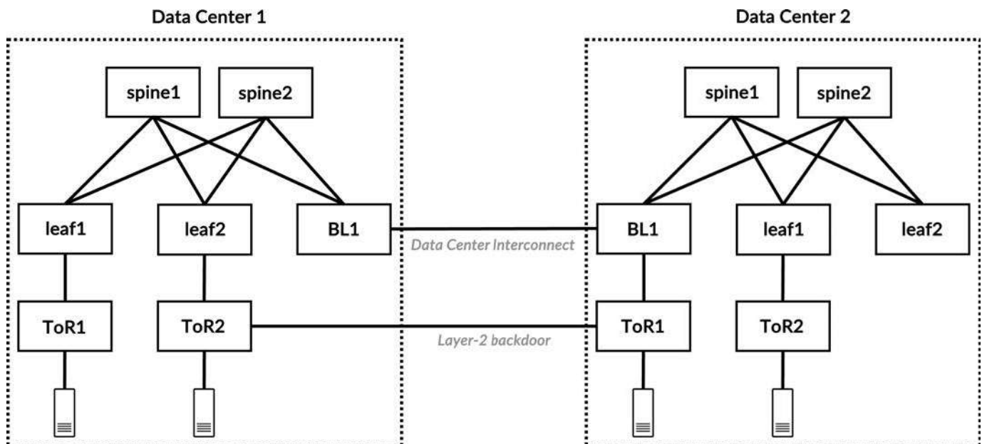
Figure 5-50 A backdoor link between two data centers causing a loop
