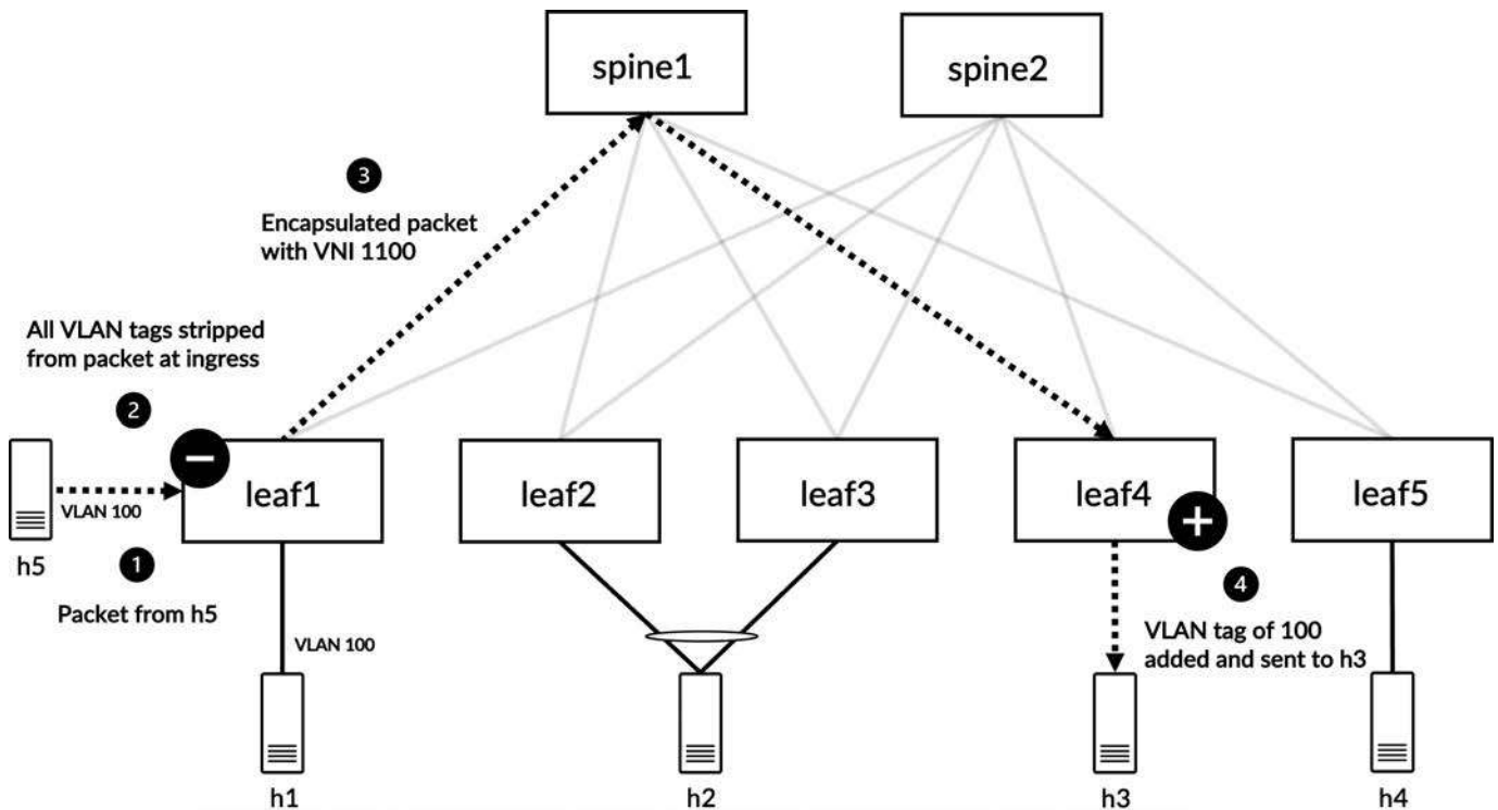
Figure 6-21 Traffic flow for a packet from host h5 to h3 with VLAN normalization to VLAN ID of none
