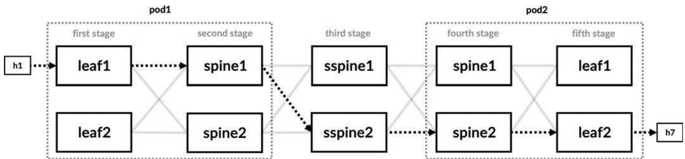
Figure 2-14 Five stages of 5-stage fabric
