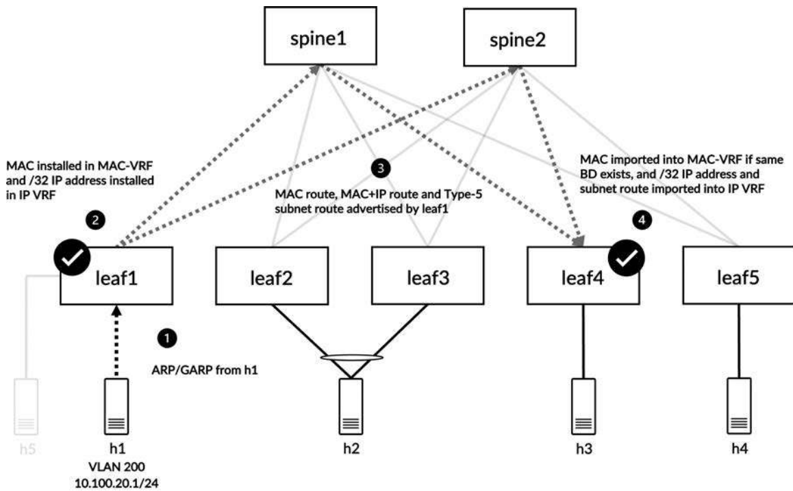
Figure 8-19 Overall view of the control plane with symmetric IRB
