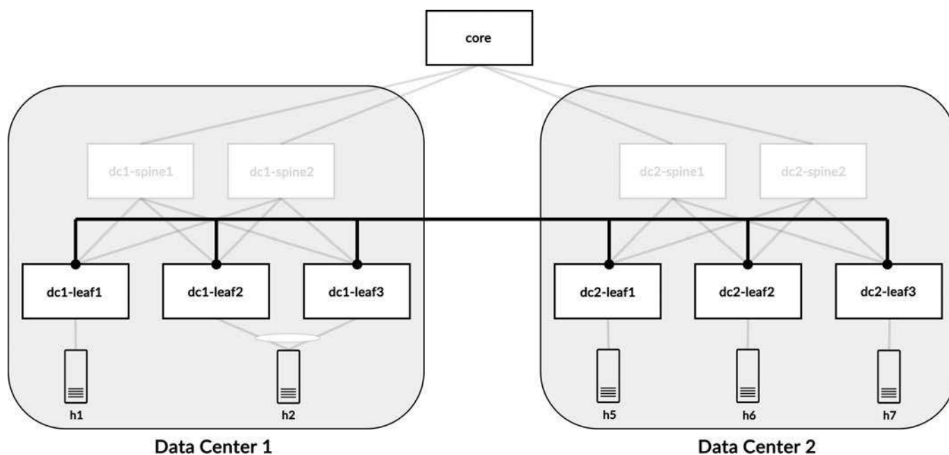
Figure 11-8 Mesh of VXLAN tunnels from one leaf in DC1
