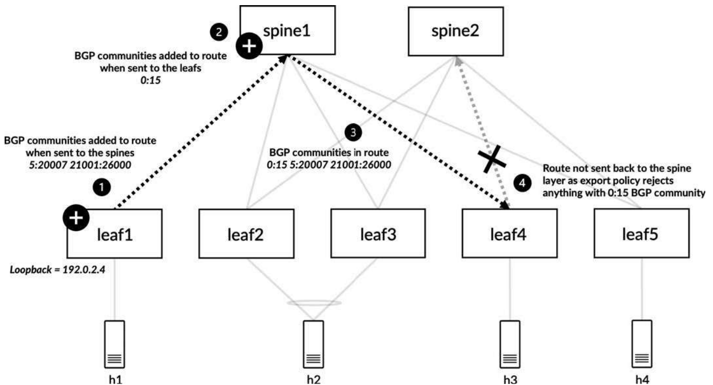
Figure 12-66 Visual representation of the prevention of BGP path hunting in an Apstra-deployed data center fabric
