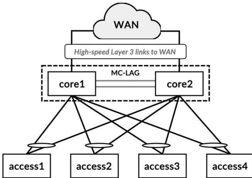
Figure 2-2 MC-LAG design in enterprise and data centers
