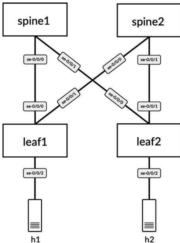
Figure 7-5 Physical connectivity for CRB design and configuration
