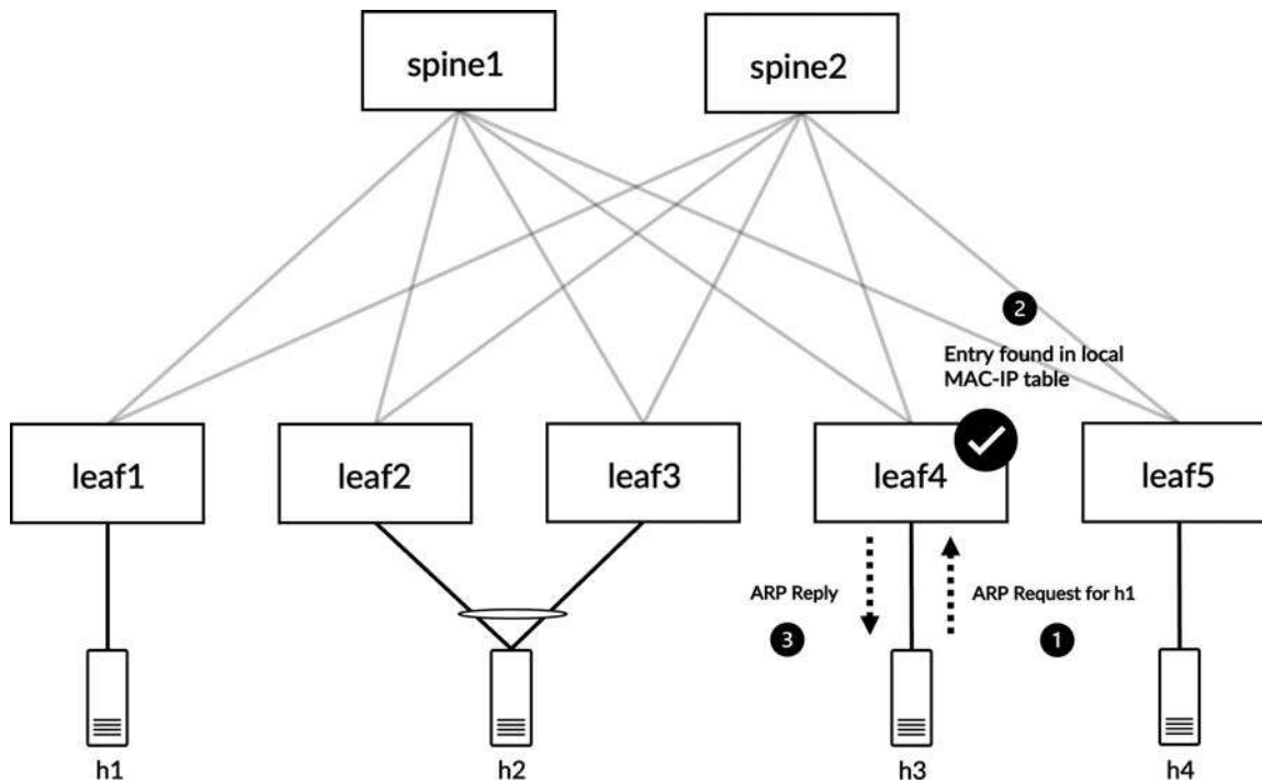
Figure 5-19 Visual representation of proxy ARP and ARP suppression from the perspective of leaf4
