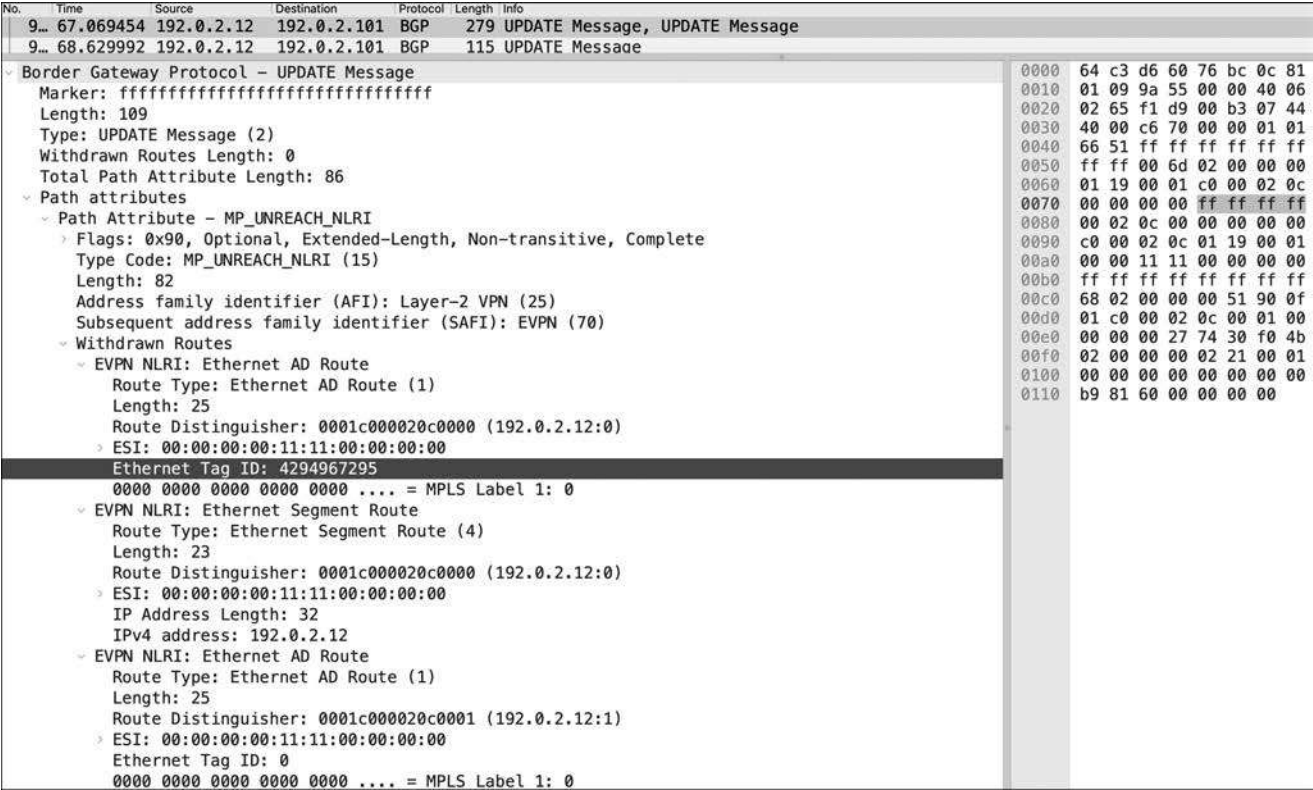
Figure 5-35 Packet capture showing withdraw of Type-1 EAD per ES route
