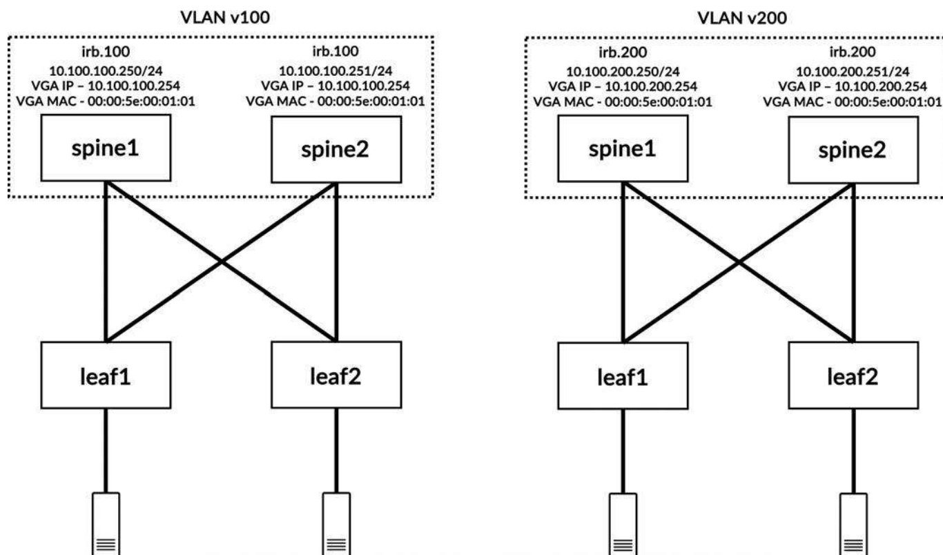
Figure 7-7 Visualizing the configuration of IRB interfaces for VLANs v100 and v200
