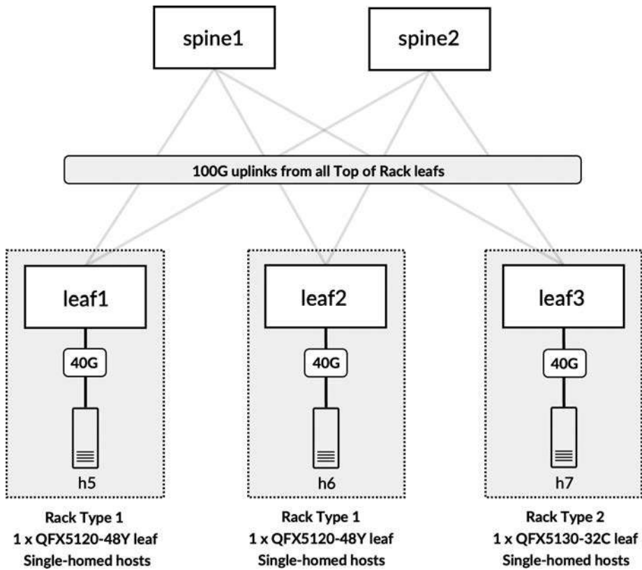
Figure 13-11 Reference topology for second data center and details of Rack Types to be designed in Apstra
