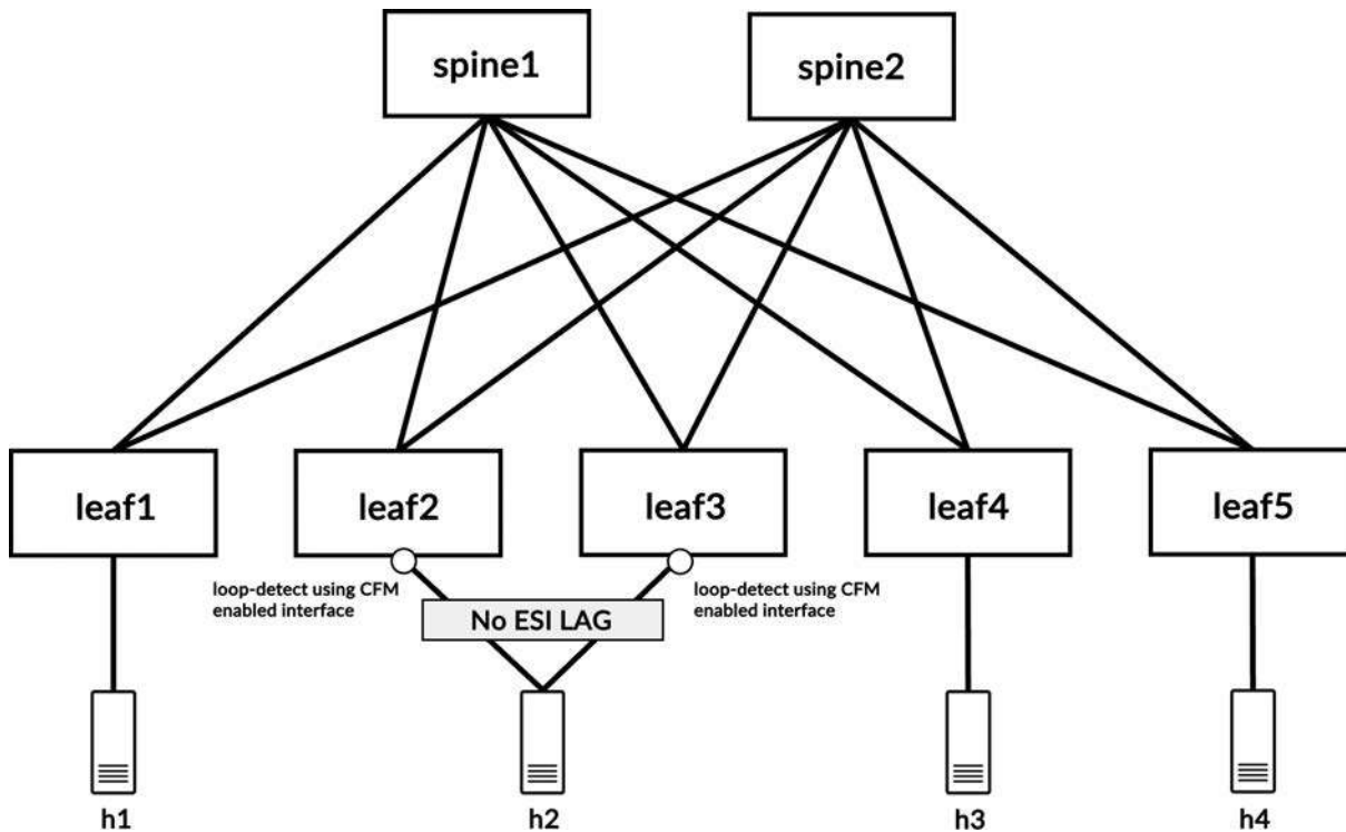
Figure 5-51 PE-to-CE interfaces configured with loop-detect using CFM
