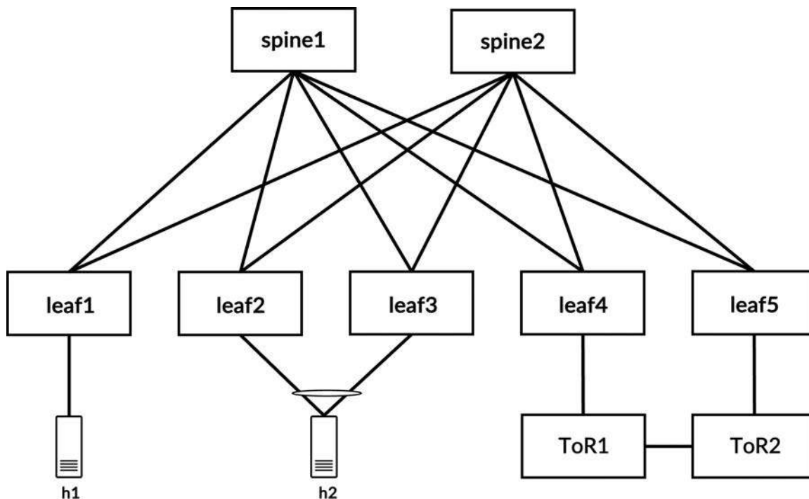
Figure 5-49 Another example topology connected downstream to an EVPN VXLAN fabric that can cause a forwarding loop
