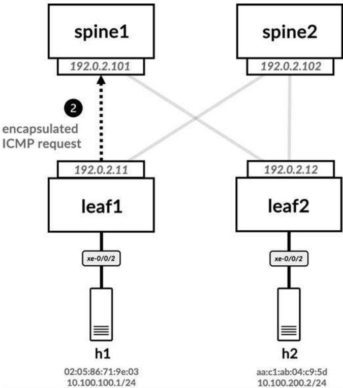
Figure 7-23 Encapsulated ICMP request sent from leaf1 to spine1
