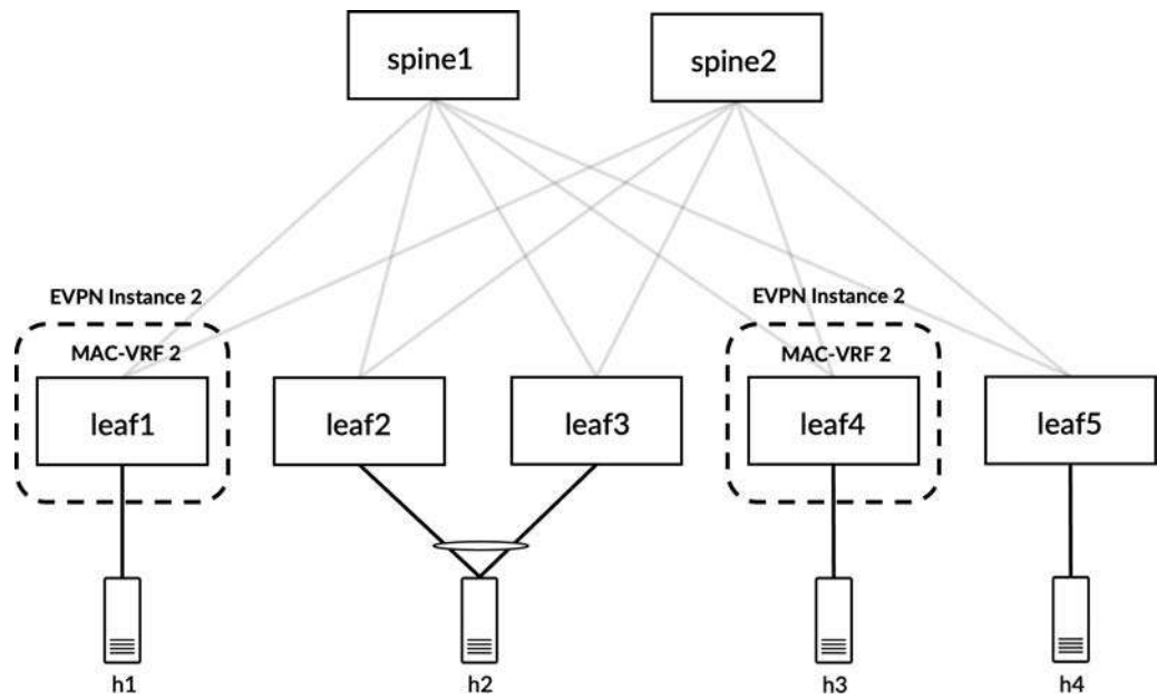
Figure 6-10 MAC-VRF macvrf-v200-1 between leaf1 and leaf4
