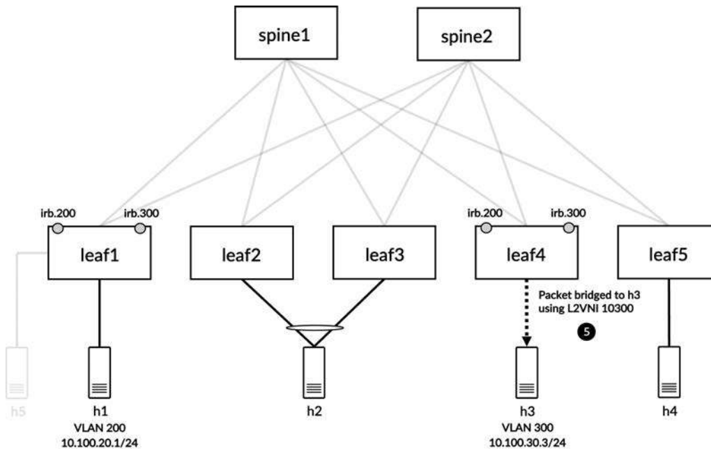
Figure 8-14 Packet bridged down to host h3 in L2VNI 10300
