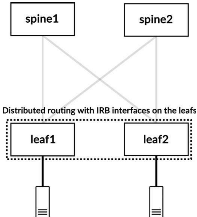
Figure 7-4 IRB placement in an ERB architecture
