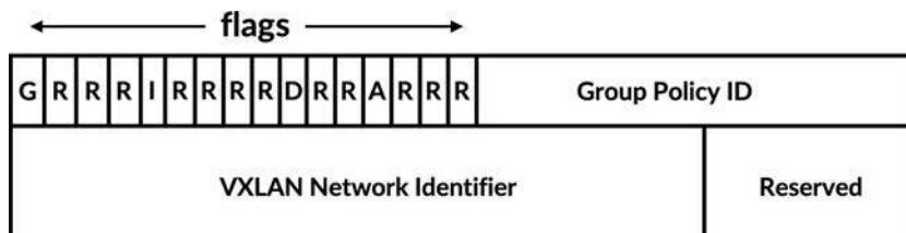
Figure 4-4 VXLAN header extension, as defined in expired VXLAN group policy IETF draft
