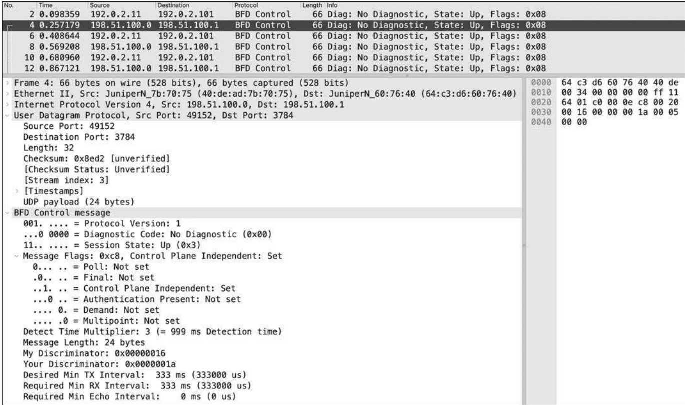
Figure 5-53 A single-hop BFD session packet capture
