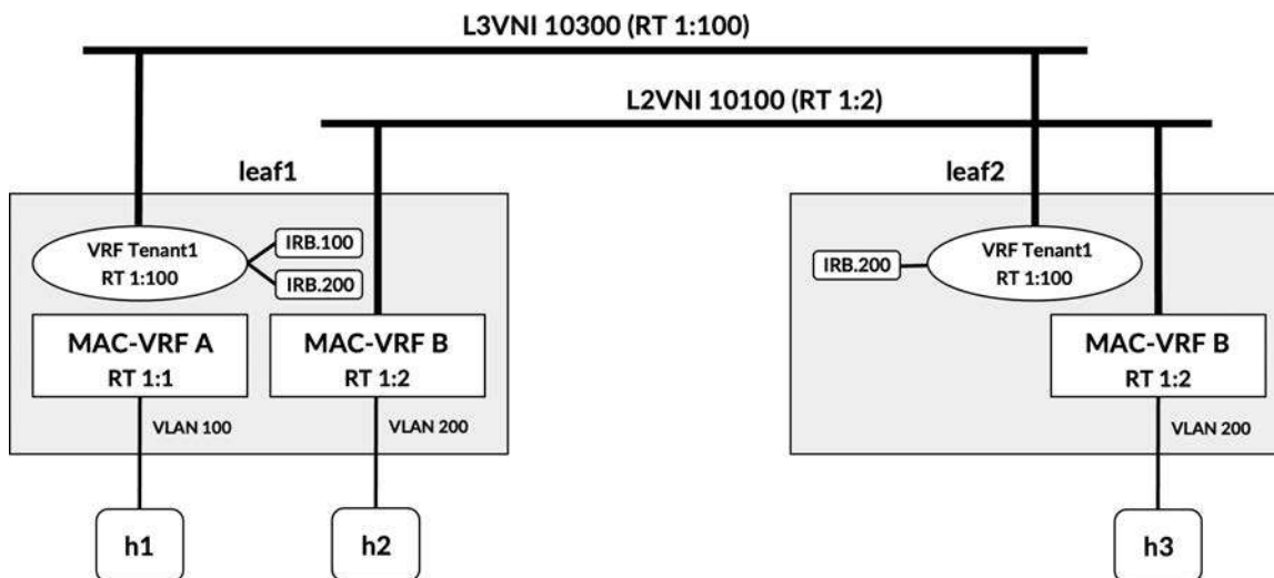
Figure 8-4 Visual representation of symmetric IRB with IP VRFs and MAC-VRFs
