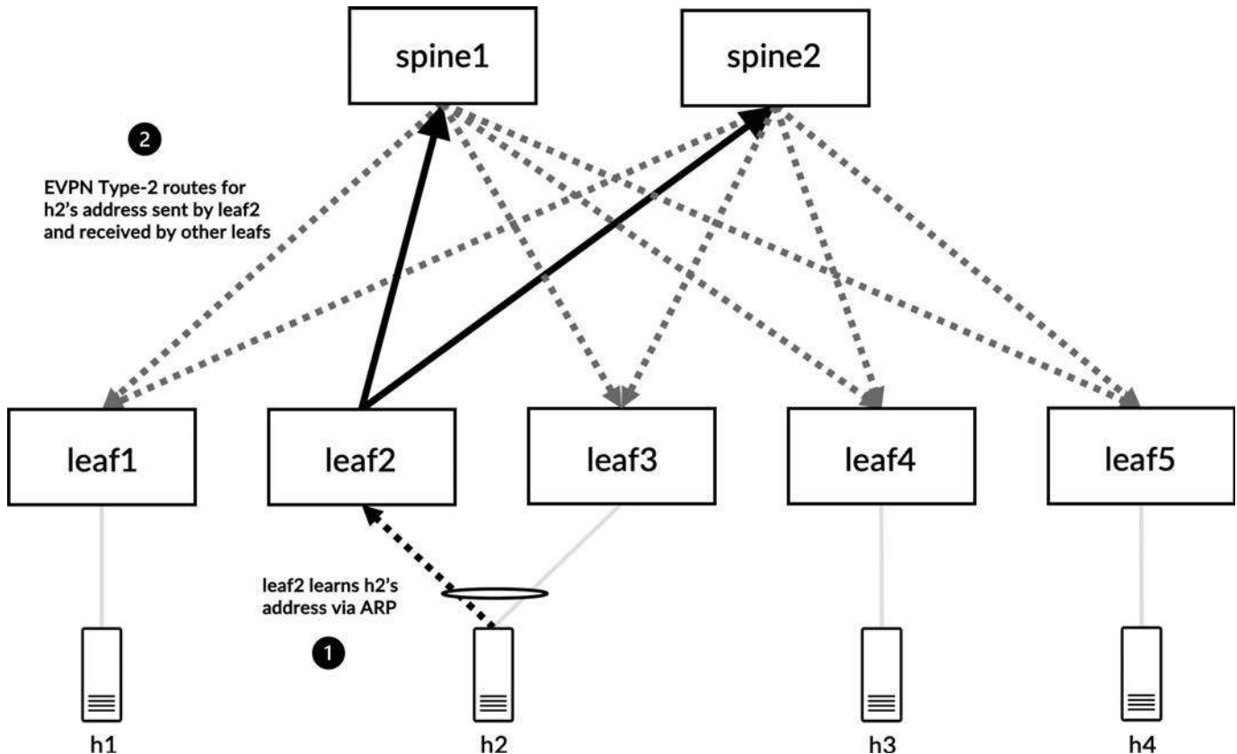
Figure 5-27 Local learn for h2 on leaf2 only, and the subsequent EVPN Type-2 route advertisement
