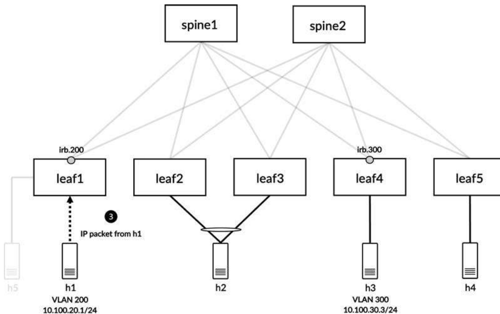
Figure 8-25 IP packet sent from host h1 destined for h3
