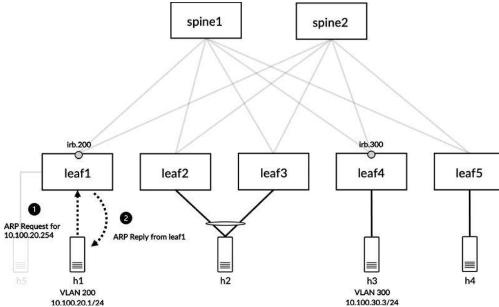
Figure 8-24 Host h1 resolving its gateway address
