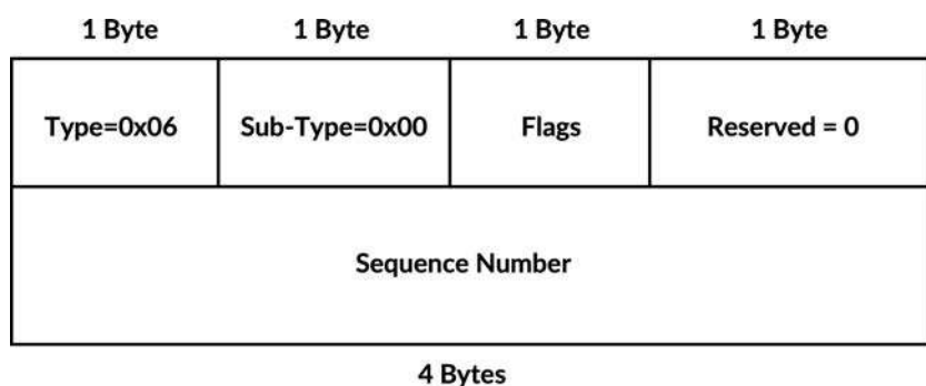
Figure 5-44 MAC Mobility extended community
