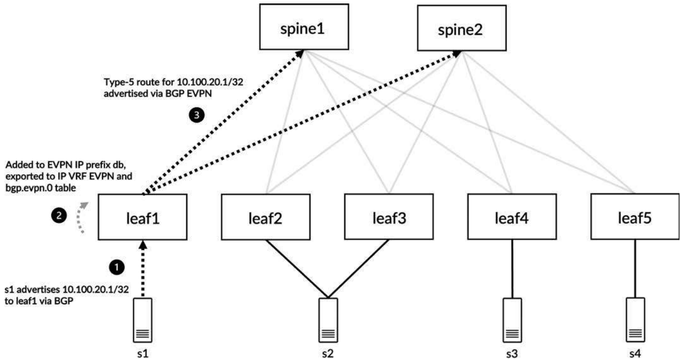
Figure 9-8 EVPN Type-5 route advertisement process
