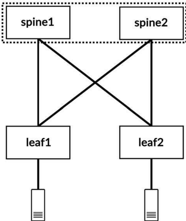
Figure 7-3 IRB placement in a CRB architecture
