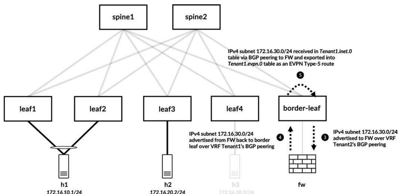
Figure 15-21 IPv4 subnet 172.16.30.0/24 advertised to FW, received back from the FW, and exported as an EVPN Type-5 route
