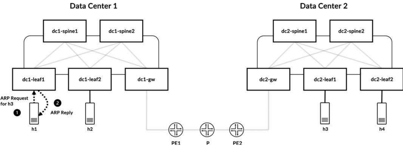
Figure 11-35 Proxy-ARP reply by dc1-leaf1 to an ARP request destined for host h3
