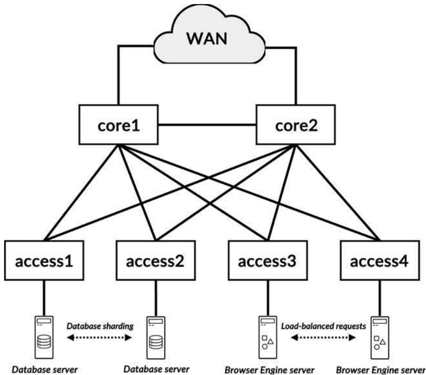
Figure 2-3 Scale-out architecture of applications
