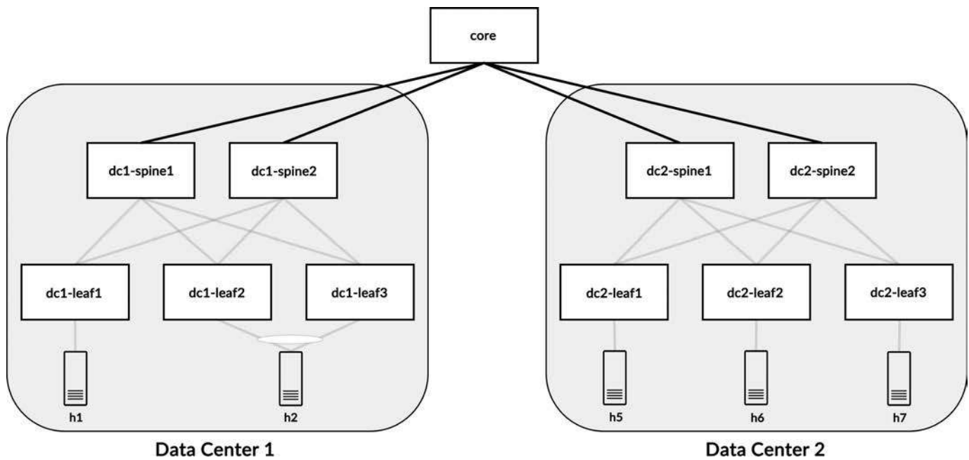
Figure 11-6 Reference topology for OTT DCI
