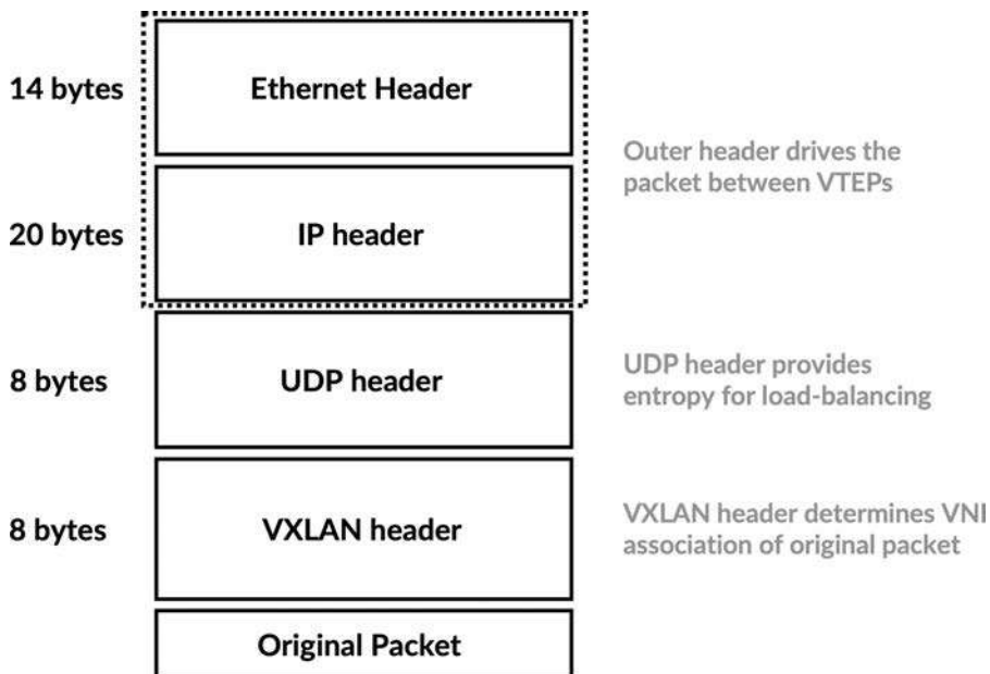
Figure 4-2 Headers added as part of VXLAN encapsulation of the original packet
