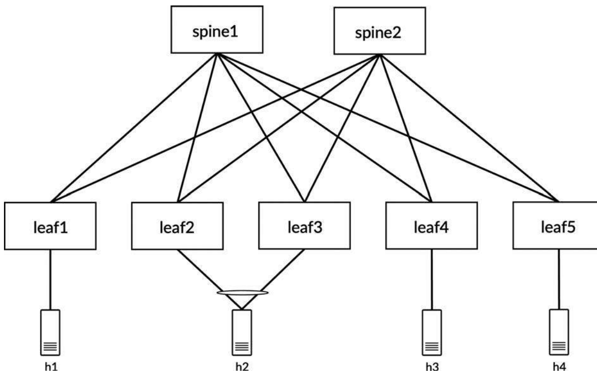
Figure 5-15 Reference topology for proxy ARP and ARP suppression
