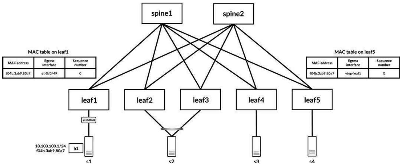
Figure 5-45 State of host h1’s MAC address during steady state, shown on leaf1 and leaf5
