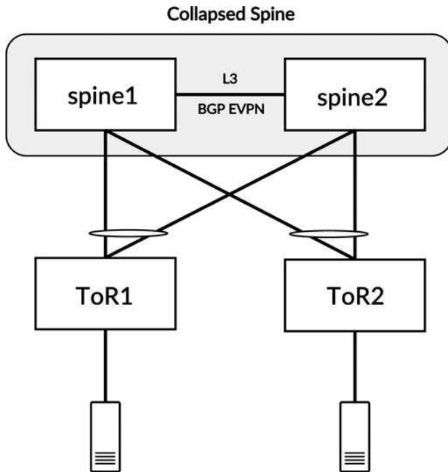
Figure 5-39 A typical collapsed spine design for EVPN VXLAN
