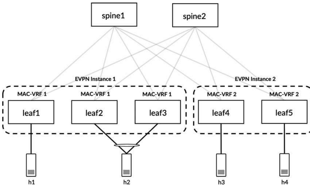
Figure 6-6 Tenant isolation with MAC-VRFs
