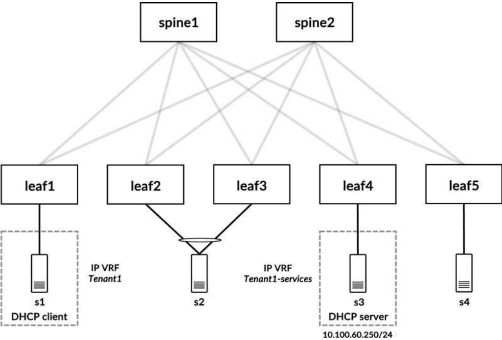
Figure 10-16 DHCP server in a dedicated services VRF
