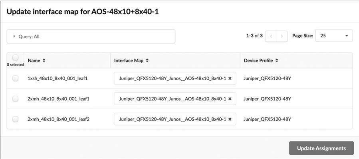
Figure 12-55 Interface Maps assigned to every instance of Logical Device AOS-48x10+8x40-1
