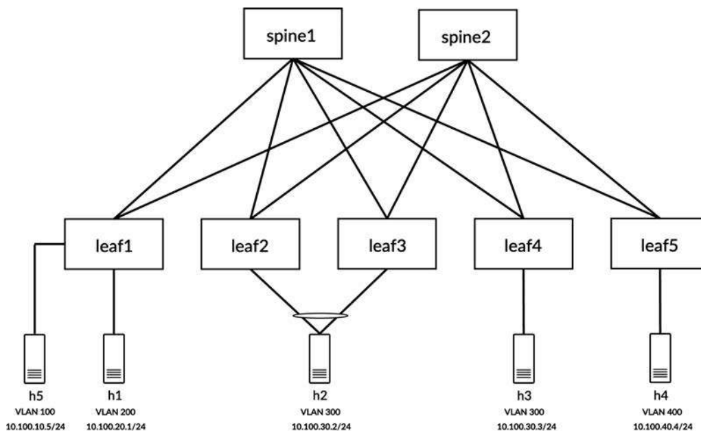
Figure 8-17 Reference topology for symmetric IRB
