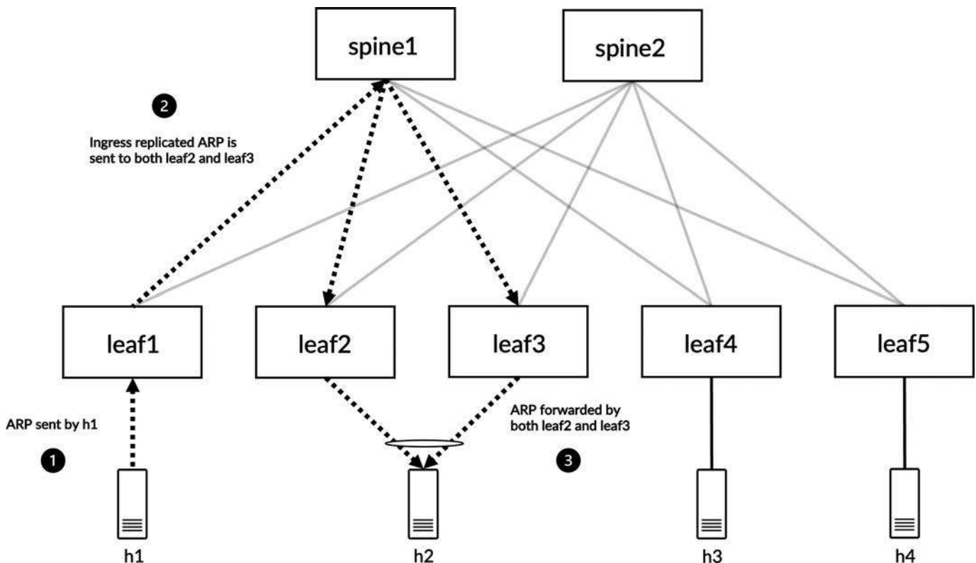
Figure 5-29 Visualization of duplicate ARP packets received on host h2
