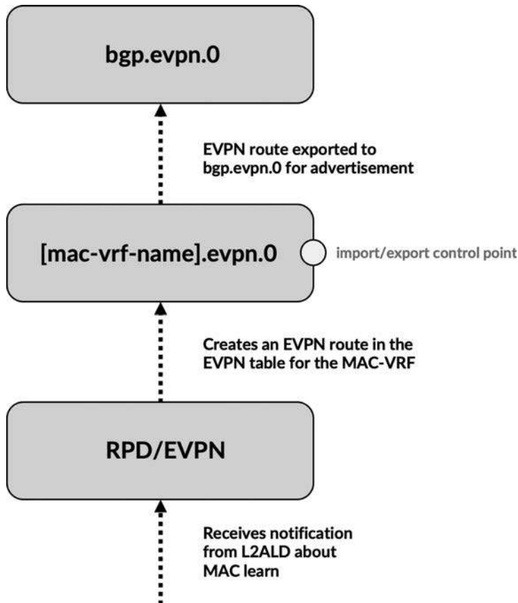
Figure 6-8 Control point and relationship of different route tables with MAC-VRFs for a locally learned address
