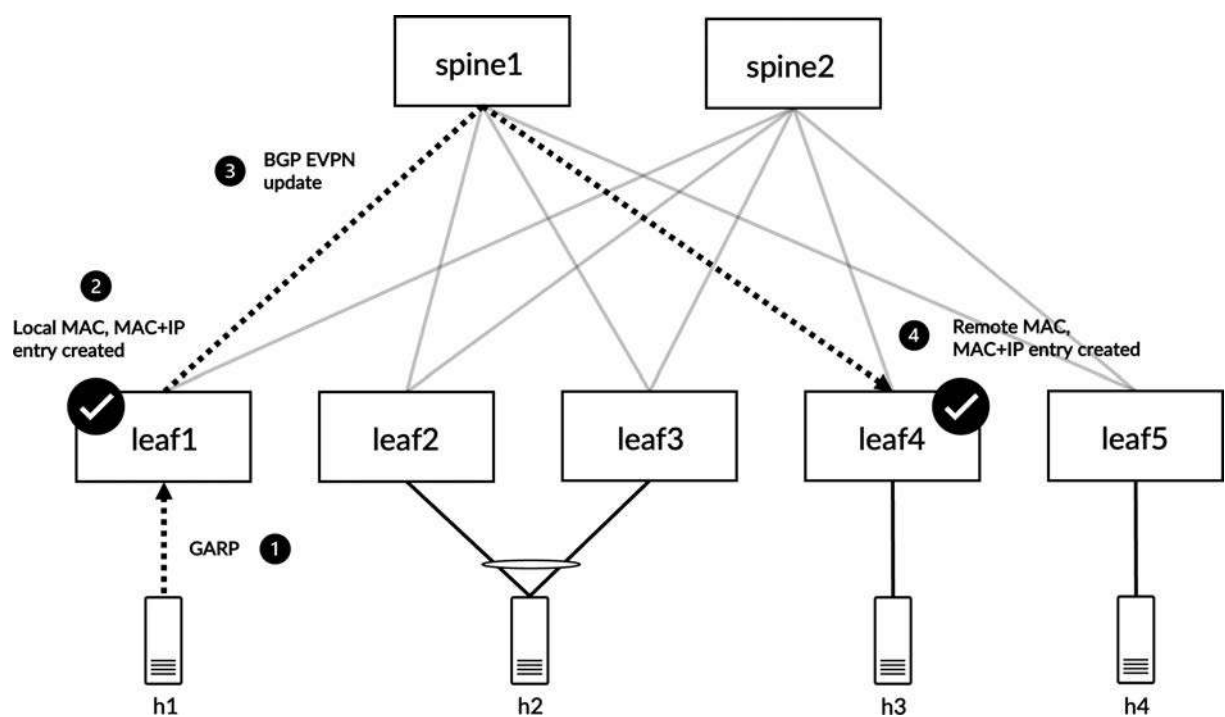
Figure 5-16 Packet walk for host h1 coming online and how its address is learned both locally and remotely
