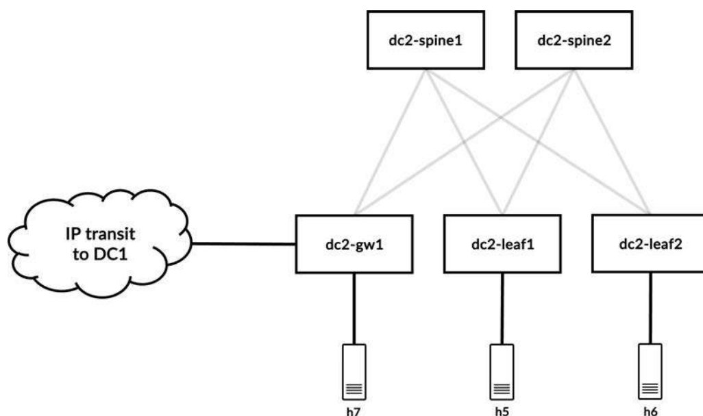
Figure 11-25 Reference topology showing details of DC2
