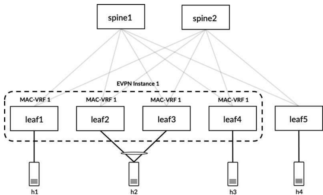
Figure 6-9 MAC-VRF macvrf-v100-1 extended to leaf4
