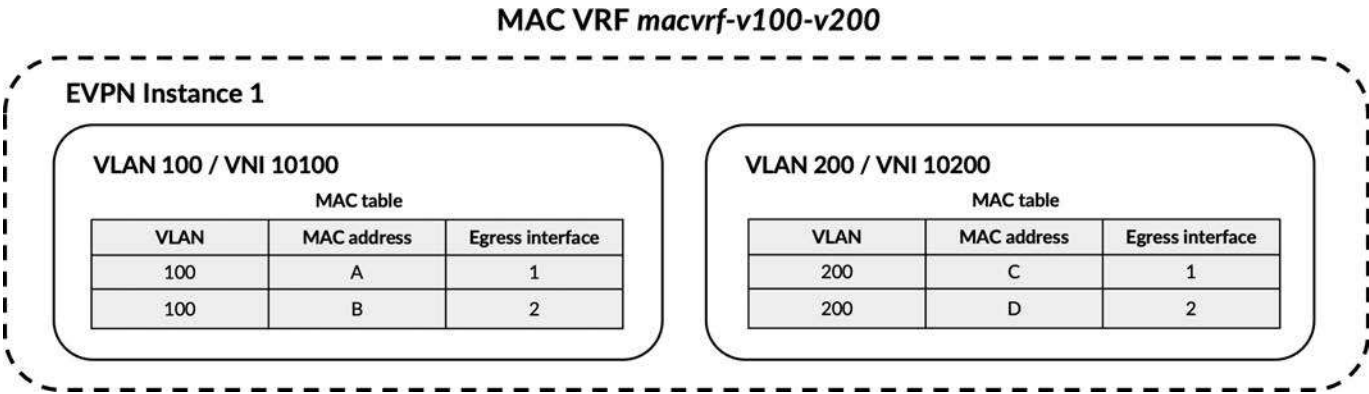
Figure 6-2 VLAN-Aware service type
