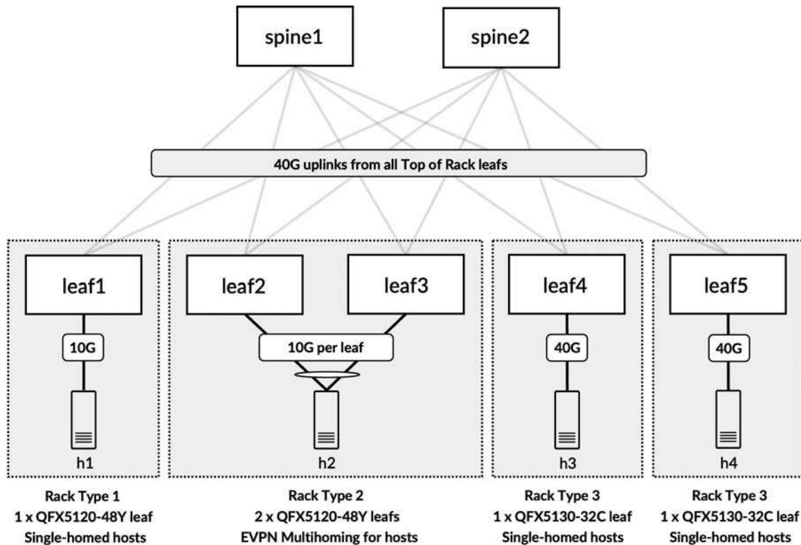
Figure 12-29 Reference topology to create a Rack Type and Template in Apstra
