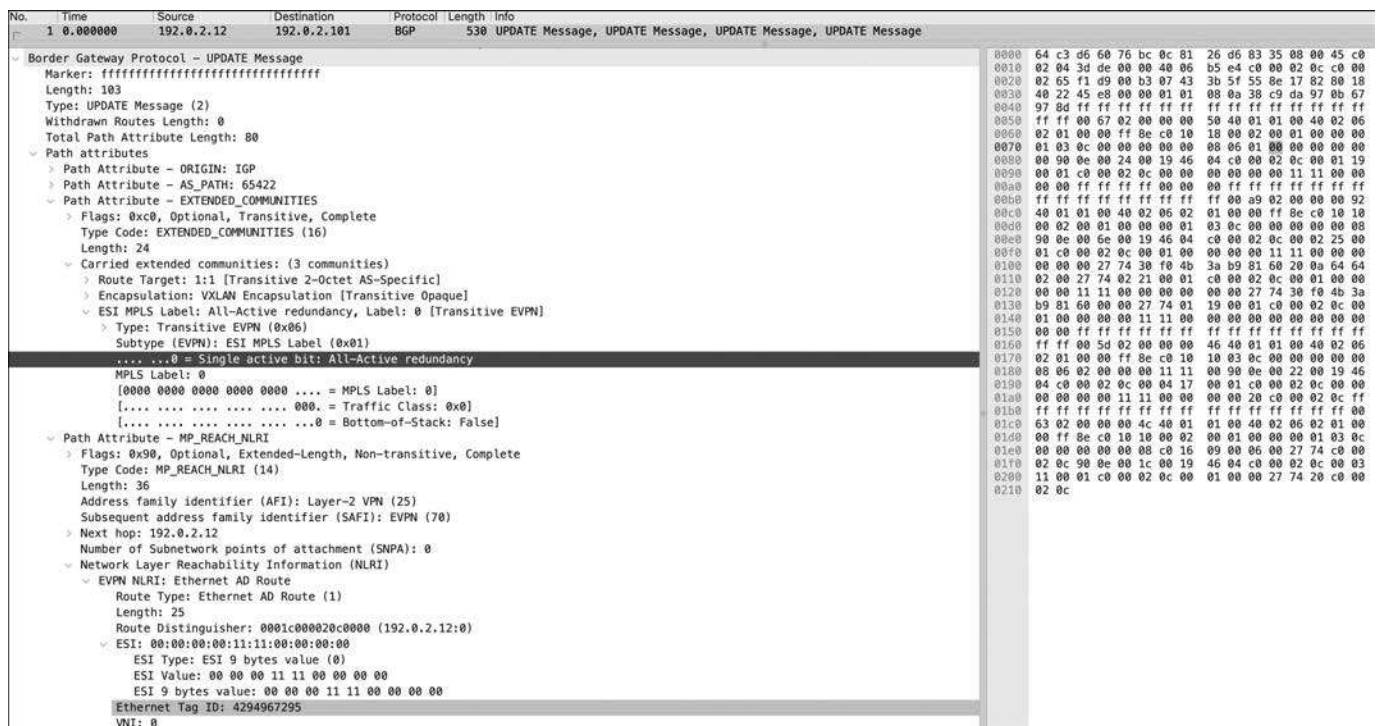
Figure 5-32 Packet capture of an EAD per ES route advertised by leaf2
