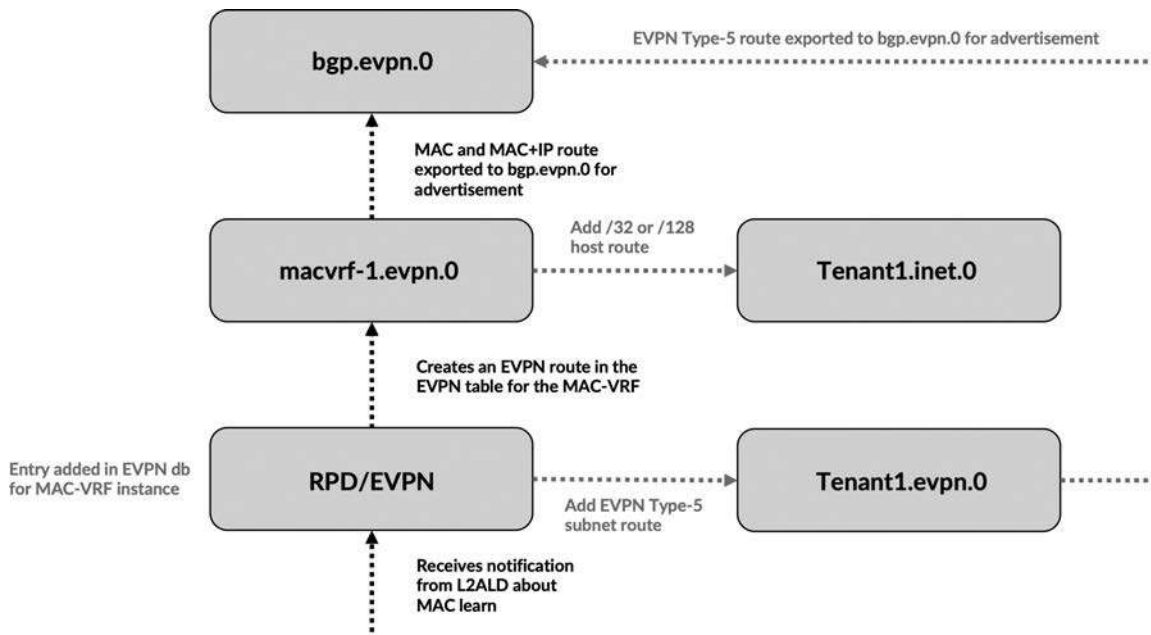
Figure 8-20 Relationship between different tables in a symmetric IRB design
