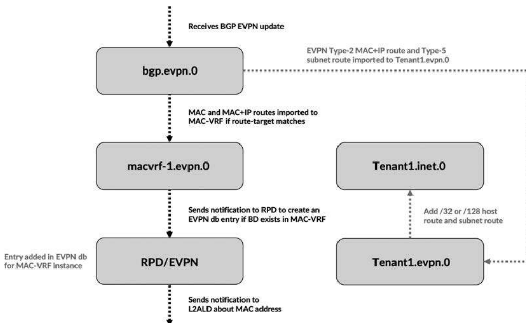
Figure 8-23 Processing of EVPN Type-2 MAC, MAC+IP, and Type-5 subnet routes with symmetric IRB
