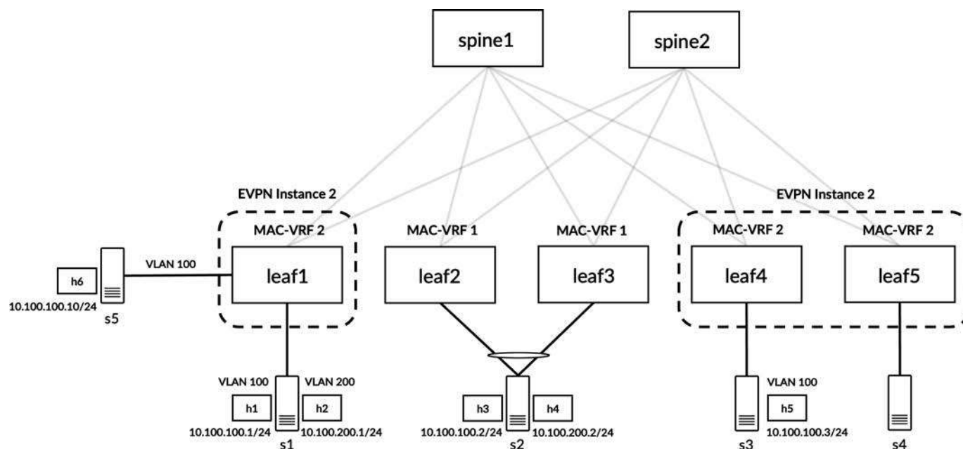
Figure 6-16 Visual representation of MAC-VRF macvrf-v100-translate with new server s5 connected to leaf1
