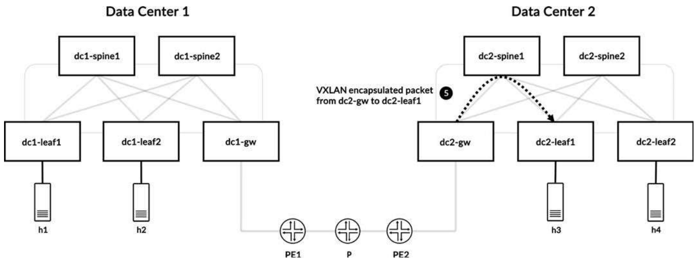
Figure 11-41 Packet capture of VXLAN-encapsulated packet from dc2-gw to dc2-leaf1
