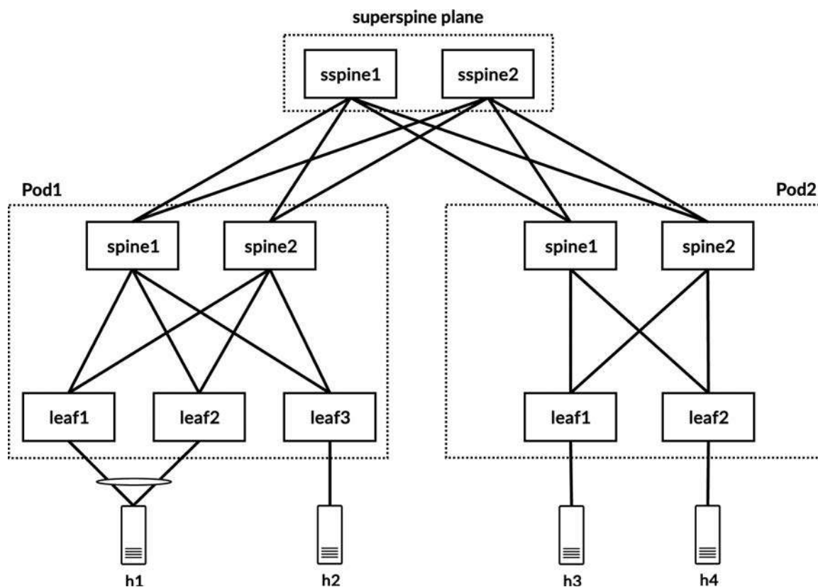
Figure 15-2 Visual representation of 5-stage Clos fabric to be deployed in Apstra
