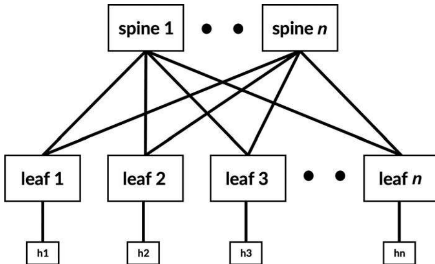
Figure 2-9 3-stage Clos fabric for data center networks
