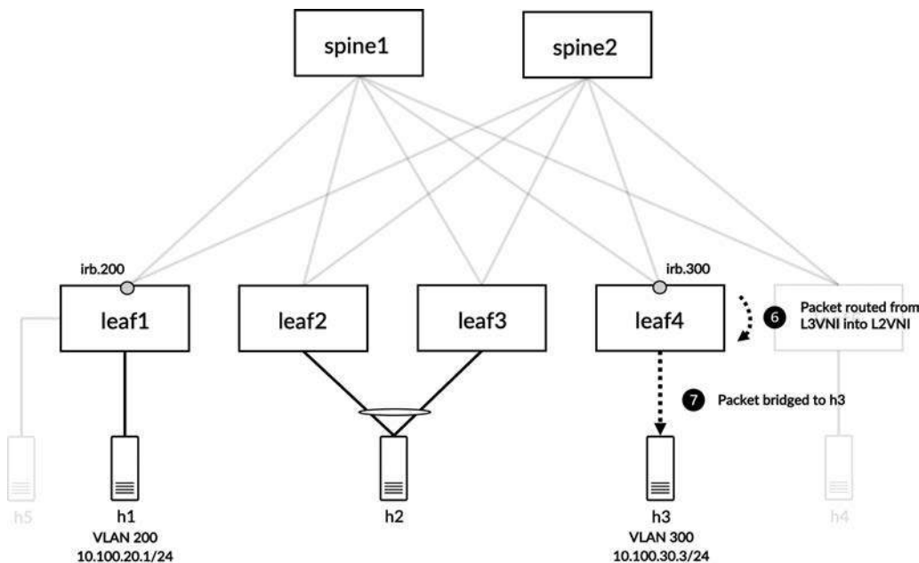
Figure 8-29 Packet routed from L3VNI to L2VNI on leaf4 and bridged to host h3
