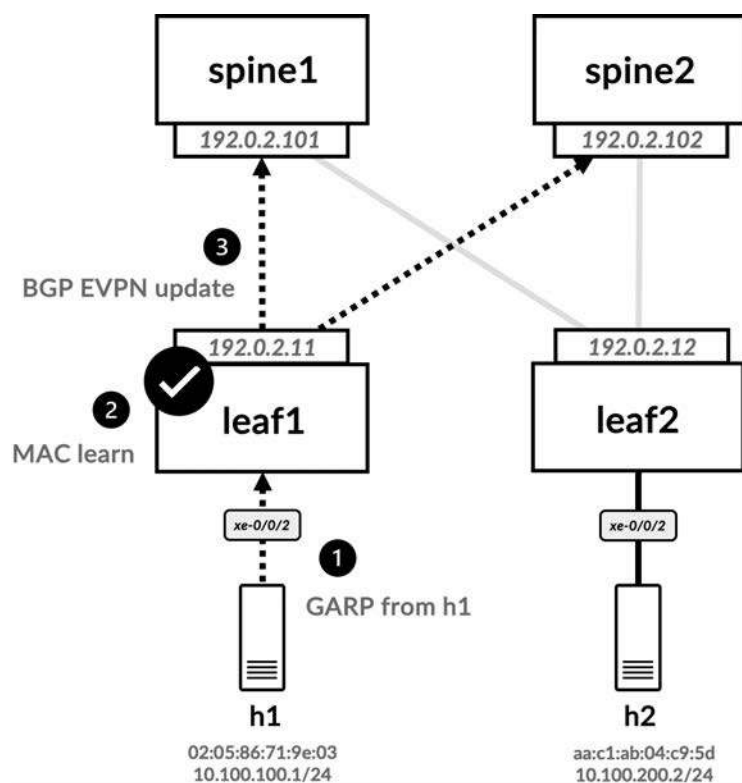
Figure 7-20 Control-plane visualization for host h1's MAC learn
