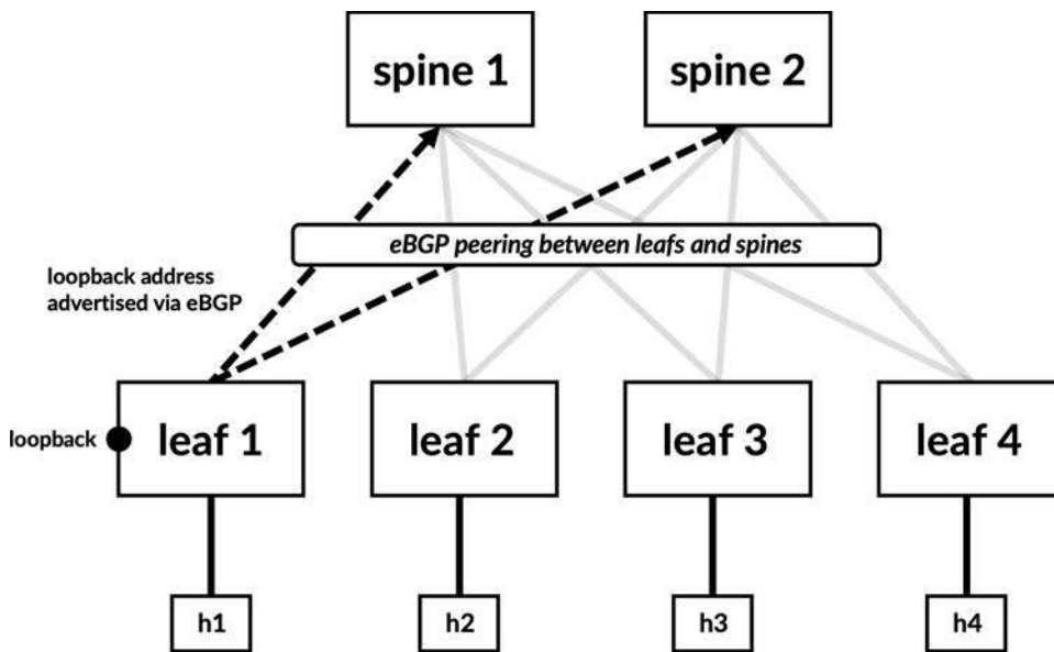
Figure 2-11 Underlay in a VXLAN 3-stage Clos fabric
