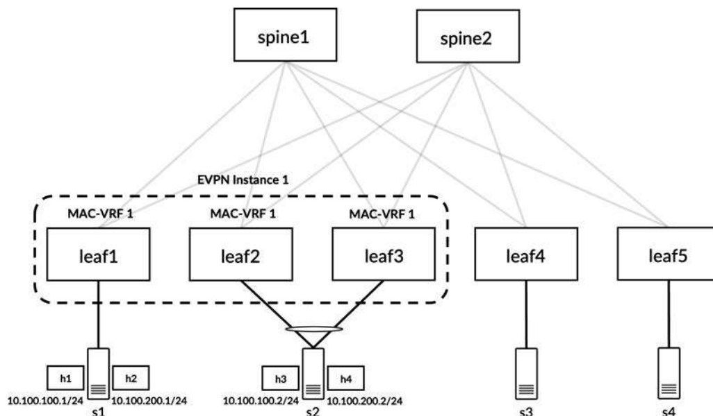
Figure 6-11 VLAN-Aware MAC-VRF for hosts h1, h2, h3, and h4
