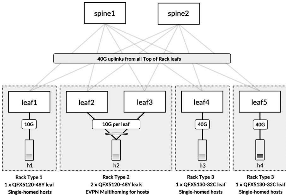
Figure 13-1 Rack Types design for ERB and Symmetric IRB deployment in Apstra
