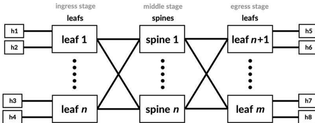
Figure 2-8 3-stage Clos network for packet-switched networks
