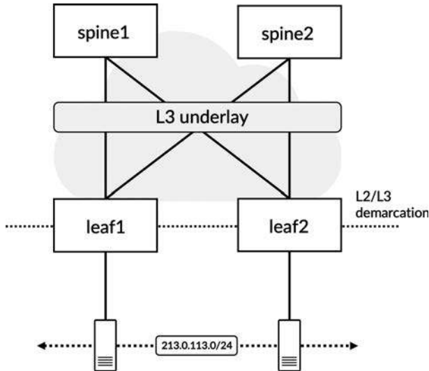
Figure 5-1 Layer 2 extended across a routed underlay
