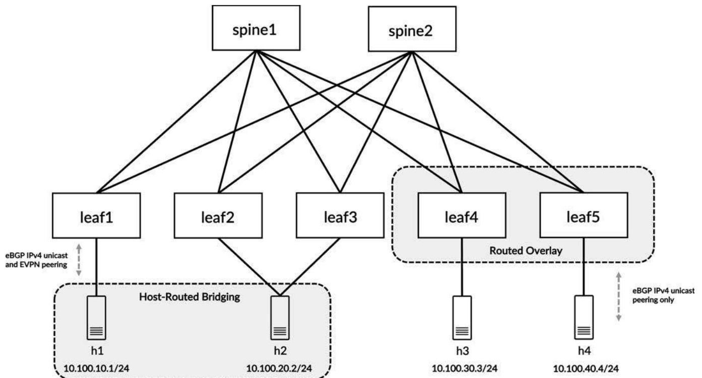
Figure 9-12 Reference topology for host-routed bridging
