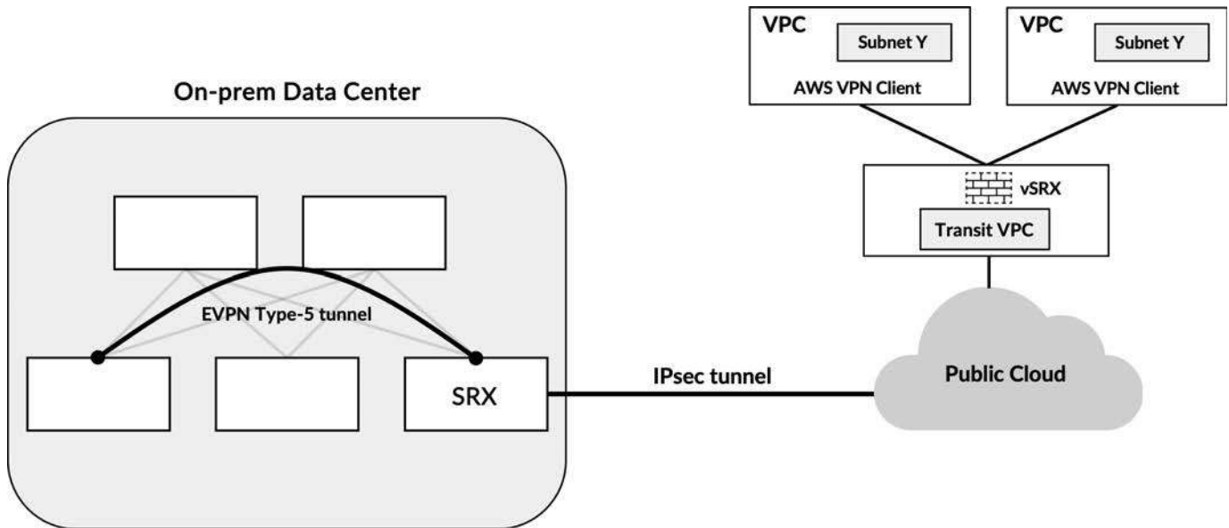
Figure 11-5 Hybrid cloud deployment with IPsec handoff to public cloud
