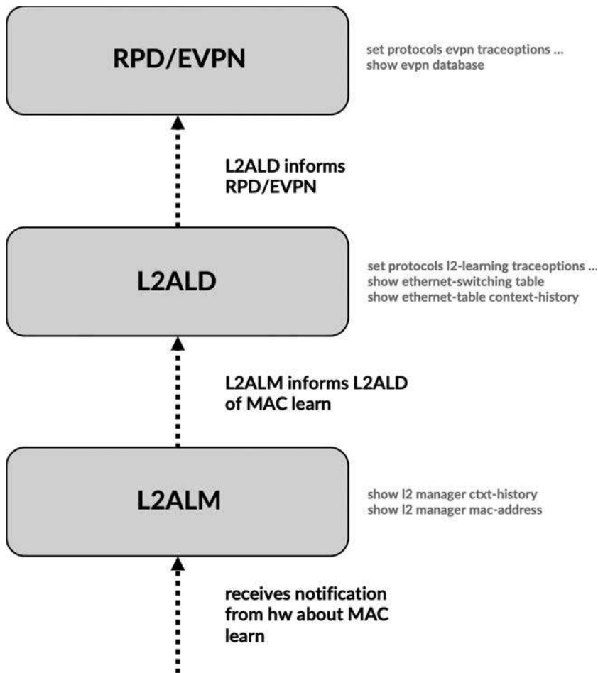
Figure 5-11 Sequence of events depicting a locally learned MAC address on a VTEP
