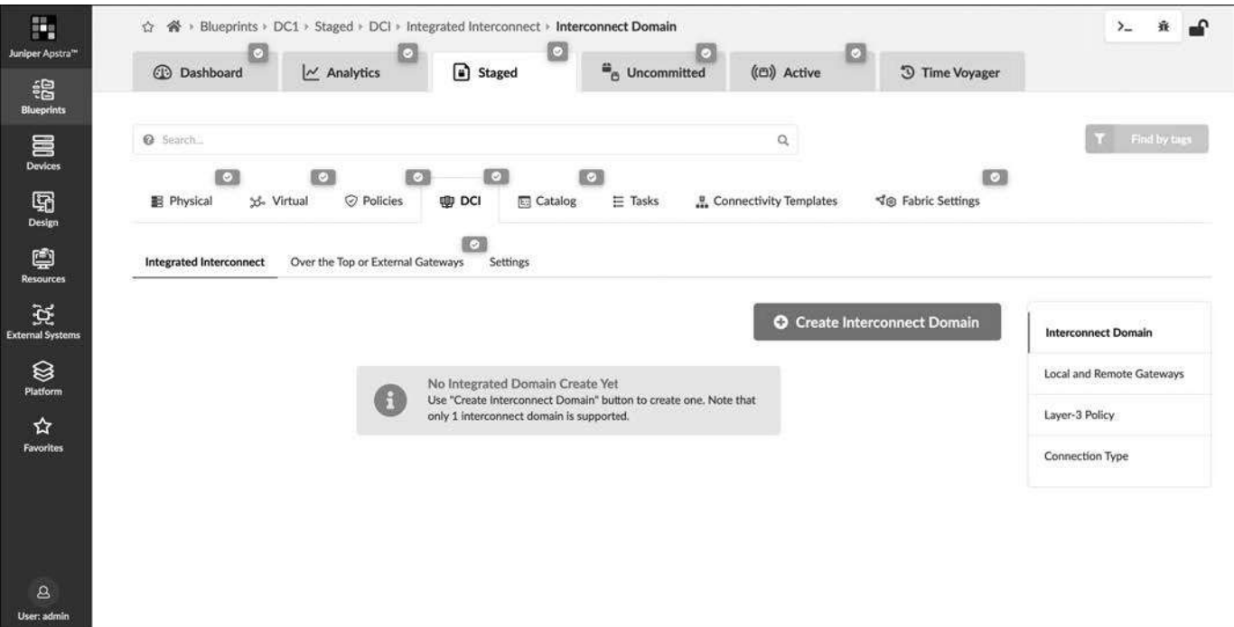
Figure 13-43 Apstra UI page for creation of Integrated Interconnect to stitch together two or more data centers
