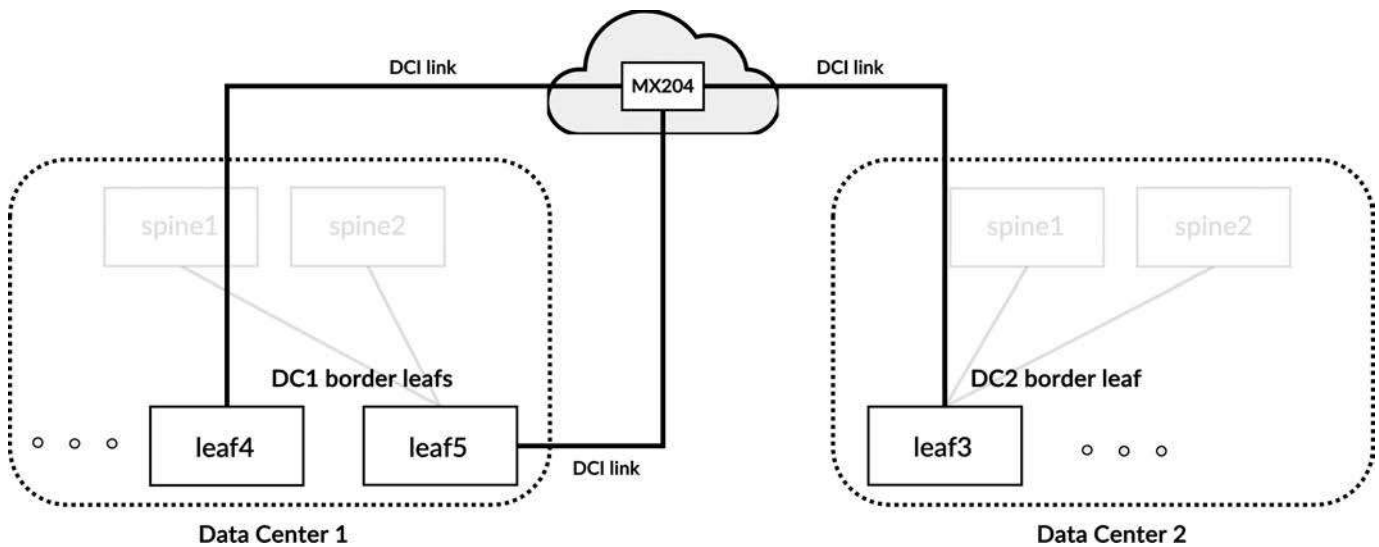
Figure 13-10 Overall topology for DCI designs, showing how the two data centers are connected
