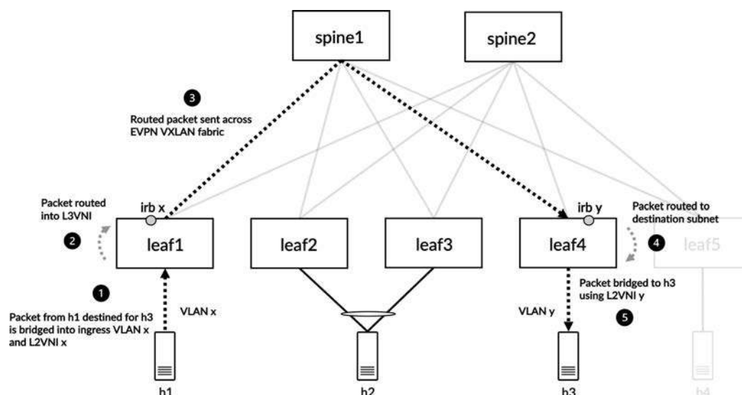
Figure 8-5 Packet flow for inter-subnet traffic with symmetric IRB
