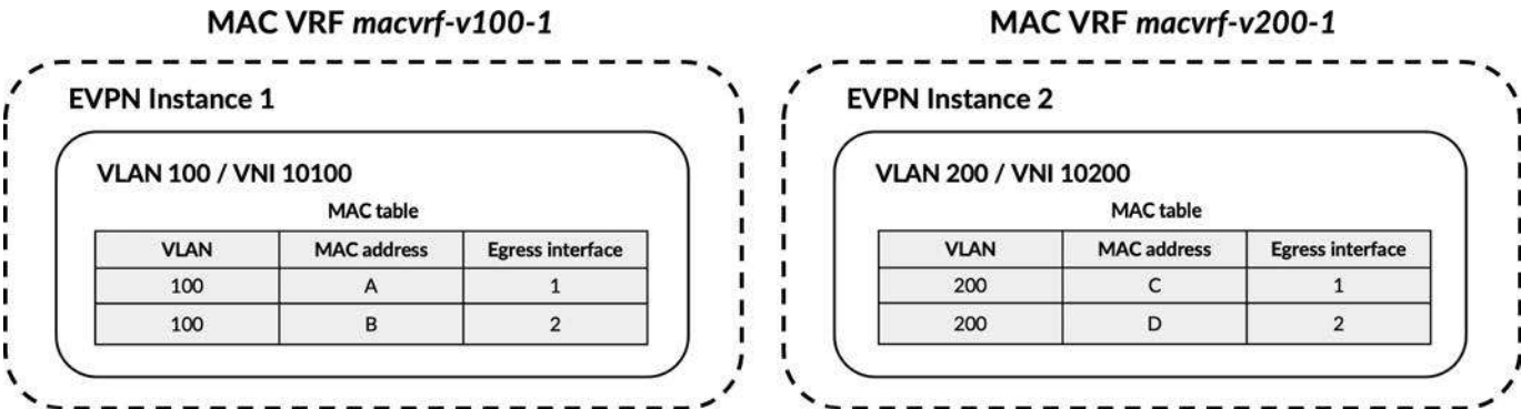
Figure 6-1 VLAN-Based service type
