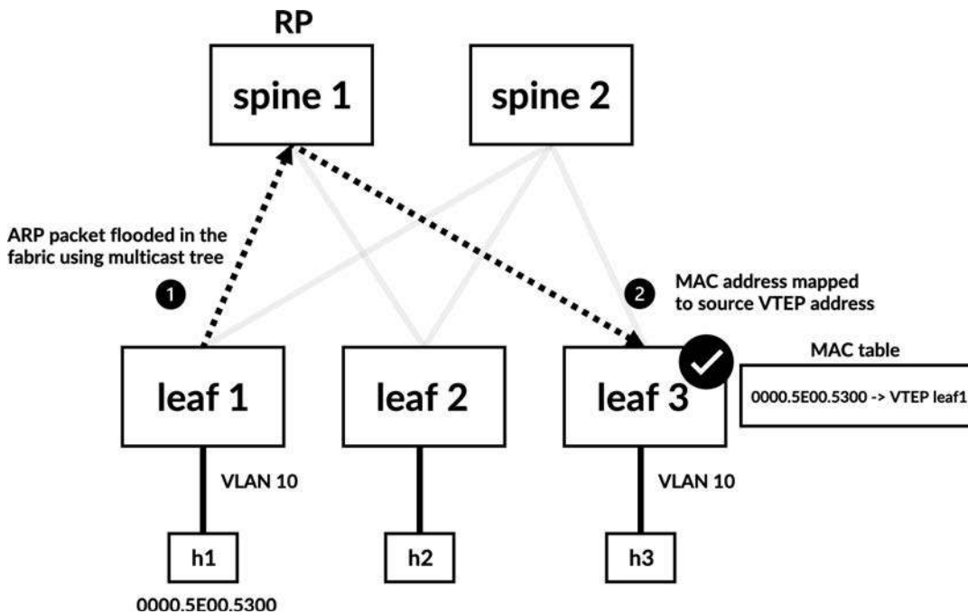
Figure 4-7 ARP packet flooded using a multicast tree in VXLAN flood-and-learn deployments
