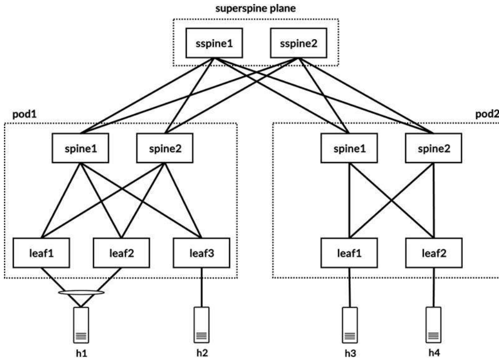
Figure 2-13 5-stage fabric with two pods
