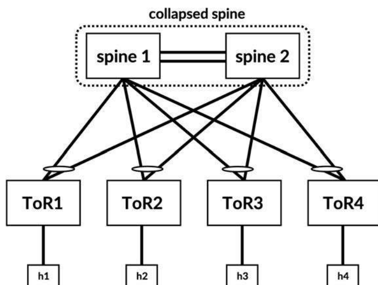
Figure 2-15 Collapsed spine design for EVPN VXLAN
