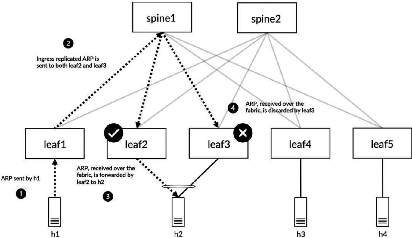
Figure 5-31 Visualization of BUM traffic, received over the fabric, dropped by nDF leaf3
