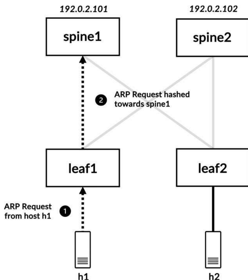
Figure 7-10 ARP request from h1 hashed toward spine1
