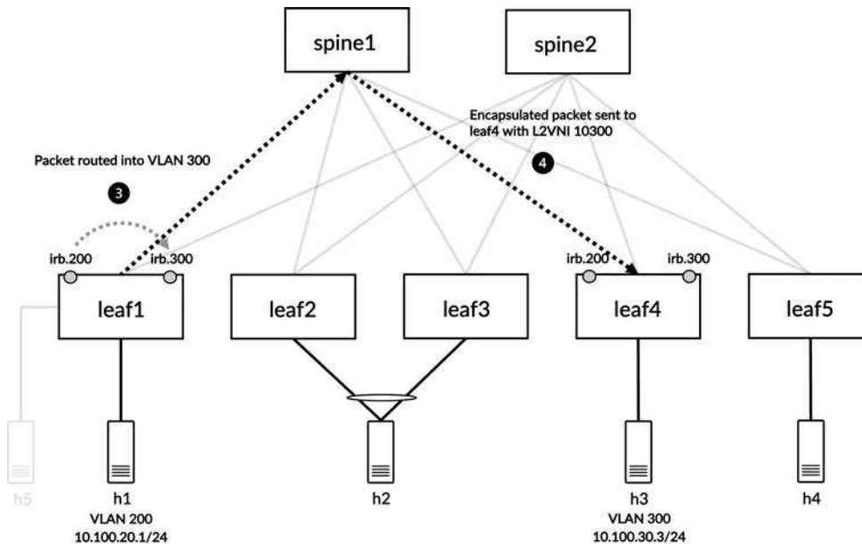
Figure 8-12 Encapsulated VXLAN packet with L2VNI 10300
