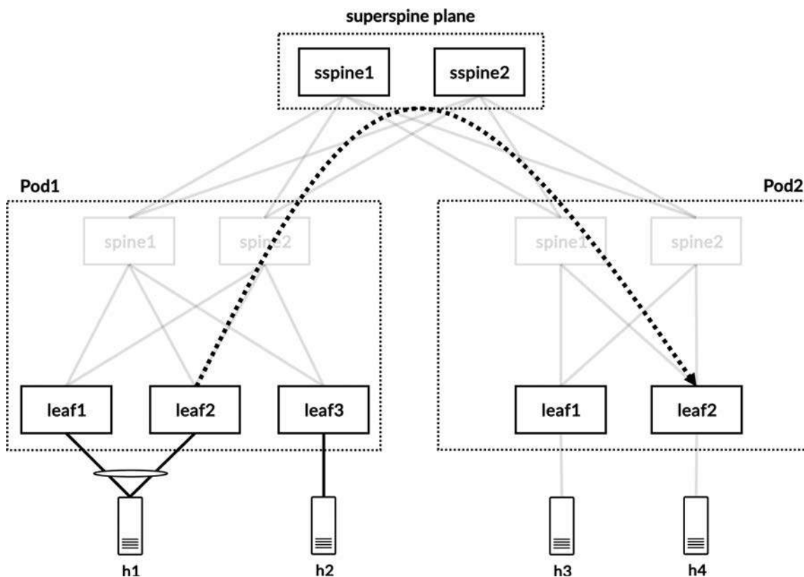
Figure 15-9 Inter-pod communication in a 5-stage Clos fabric deployed by Apstra
