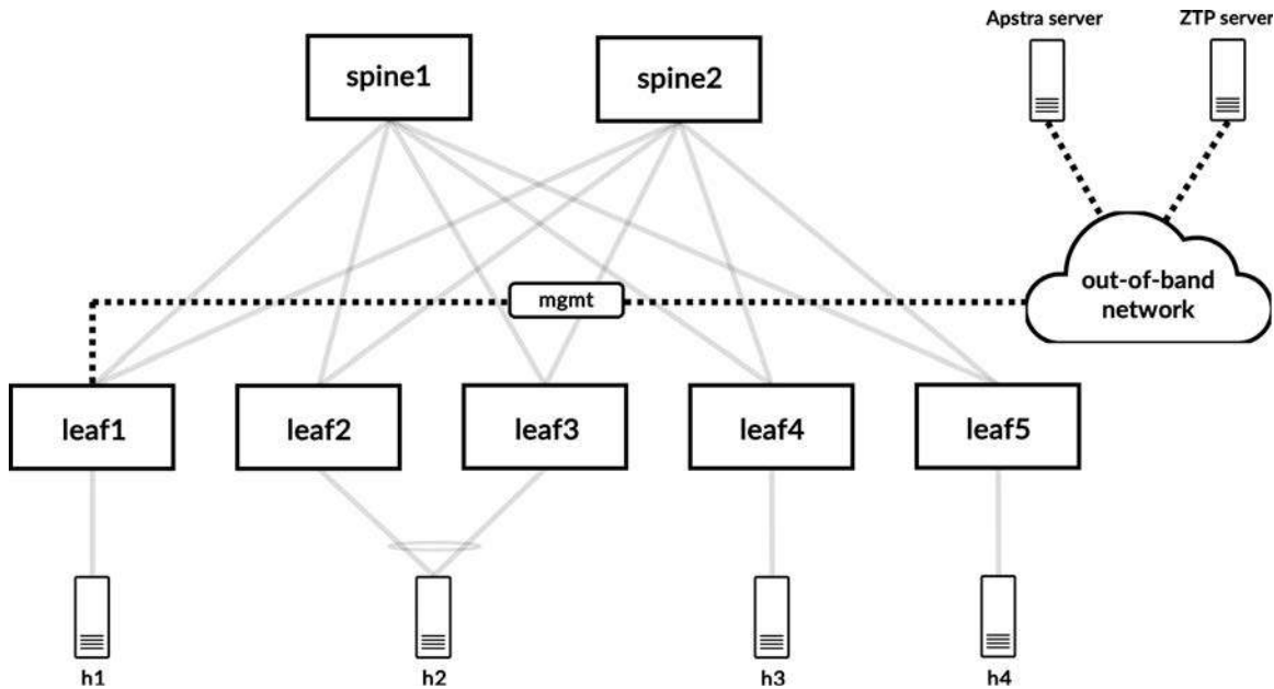
Figure 12-12 Topology for ZTP with Apstra
