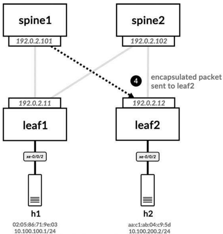
Figure 7-25 Packet routed into irb.200, encapsulated and sent toward leaf2
