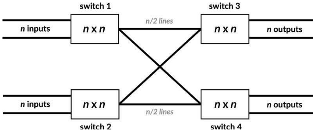
Figure 2-5 2-stage crossbar interconnection
