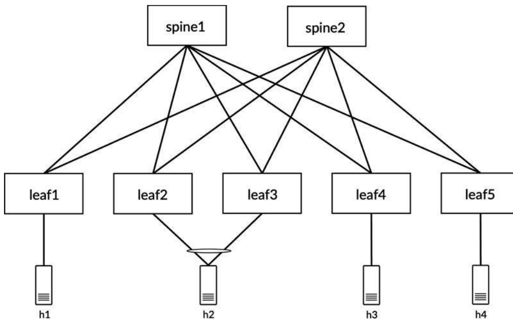
Figure 6-5 Reference topology for VLAN-Based MAC-VRFs
