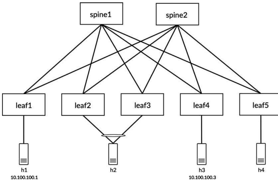
Figure 5-5 Reference topology for packet flow in a bridged overlay fabric
