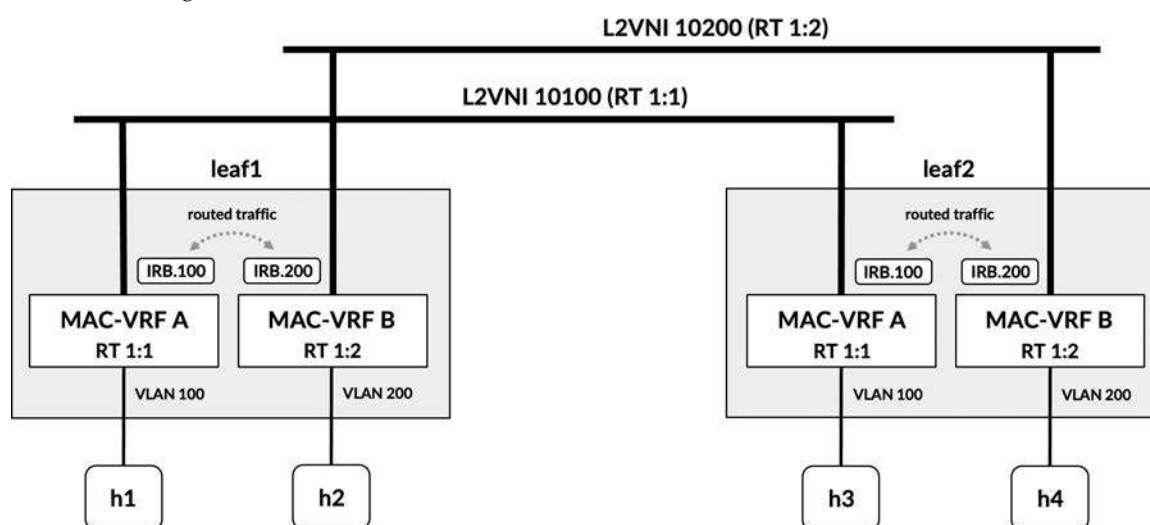
Figure 8-2 Asymmetric IRB with VLAN-Based MAC-VRFs
