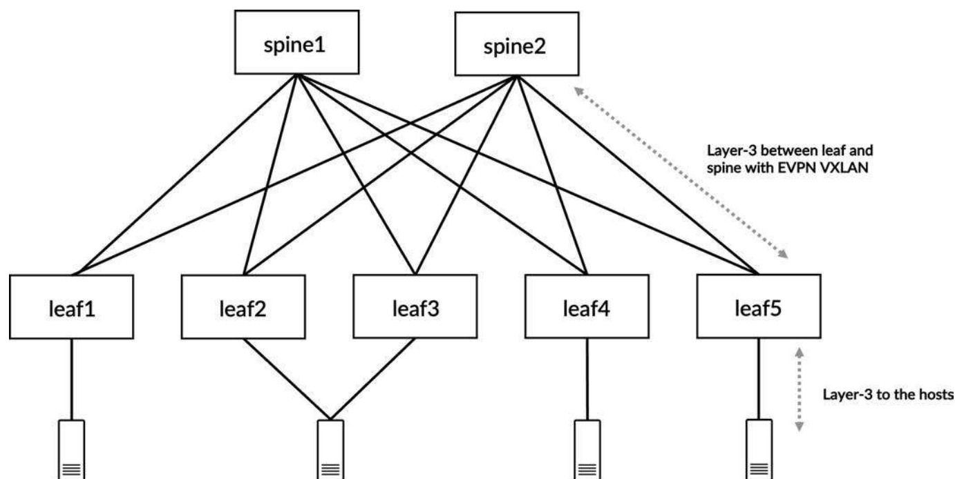
Figure 9-1 L2/L3 demarcation brought down to the hosts in a routed overlay design
