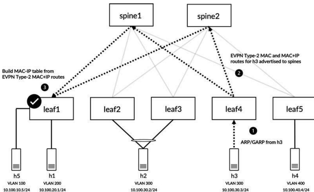
Figure 8-9 Host h3's address advertised via EVPN Type-2 routes
