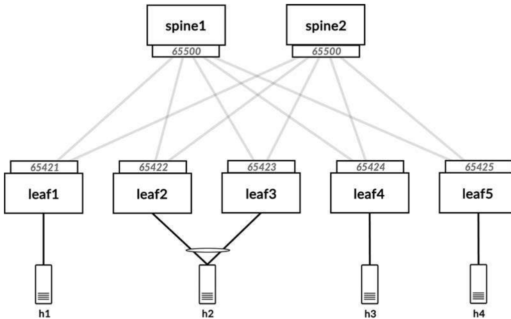
Figure 5-3 BGP AS design for a bridged overlay
