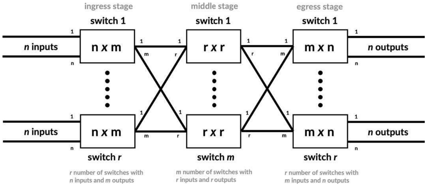
Figure 2-7 3-stage Clos network for telephony systems
