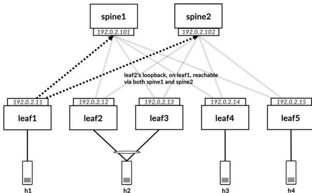
Figure 5-4 ECMP for underlay paths, shown as an example, on leaf1
