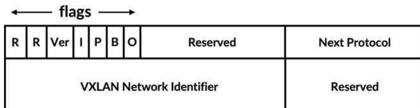
Figure 4-5 VXLAN-GPE header, as defined in VXLAN-GPE IETF draft
