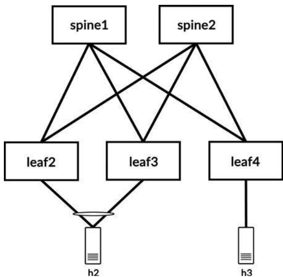
Figure 14-1 Visual representation of virtual network topology deployed by Containerlab
