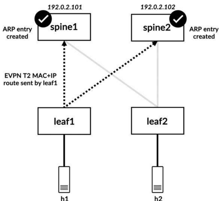
Figure 7-11 Leaf1 sending a MAC+IP Type-2 EVPN route to spines
