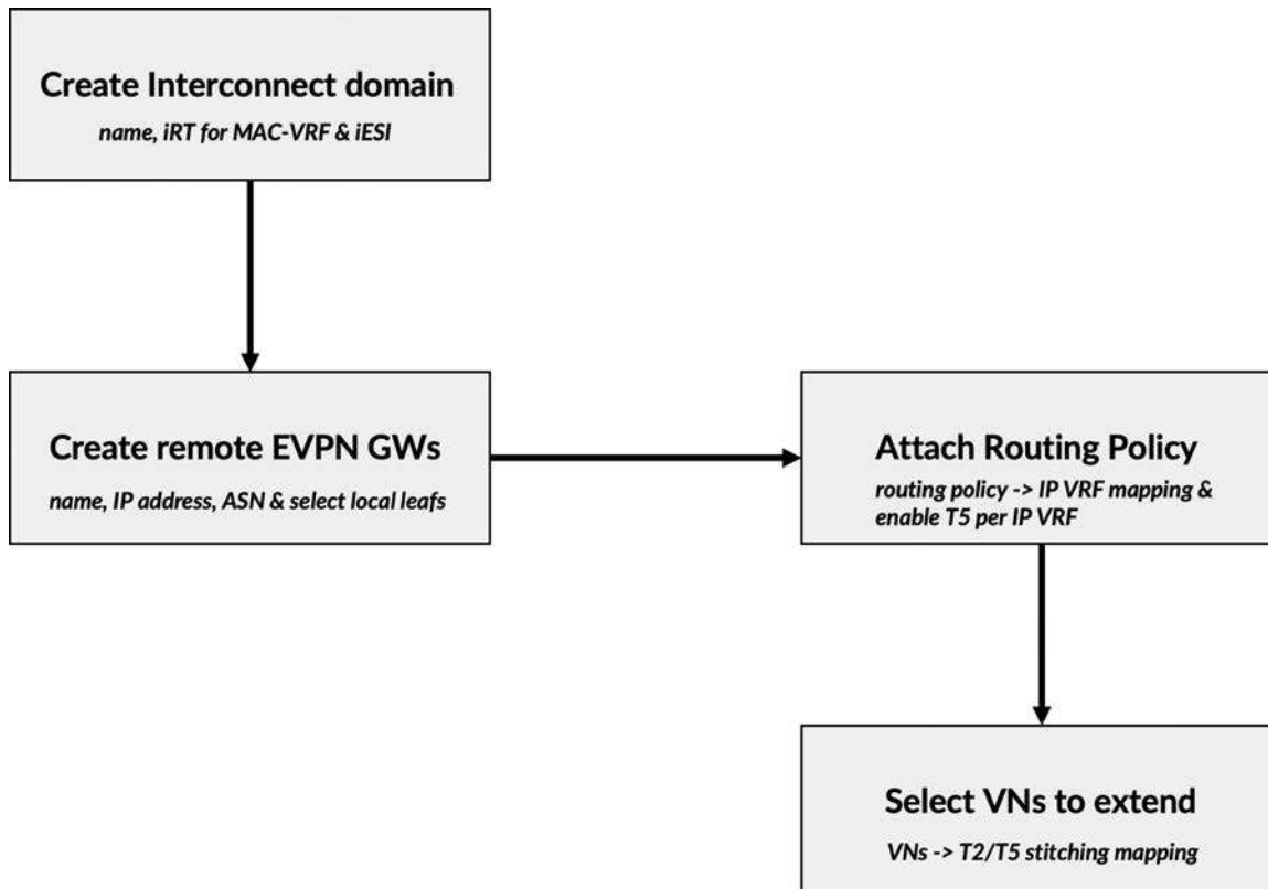
Figure 13-44 Steps to configure Integrated Interconnect in Apstra
