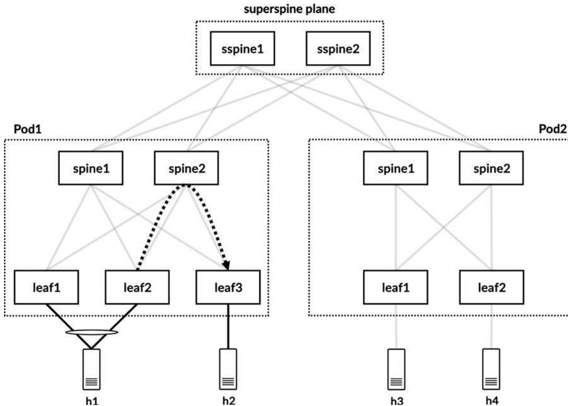
Figure 15-8 Intra-pod communication in a 5-stage Clos fabric deployed by Apstra
