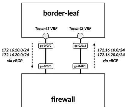
Figure 15-17 Border leaf to firewall connectivity scheme
