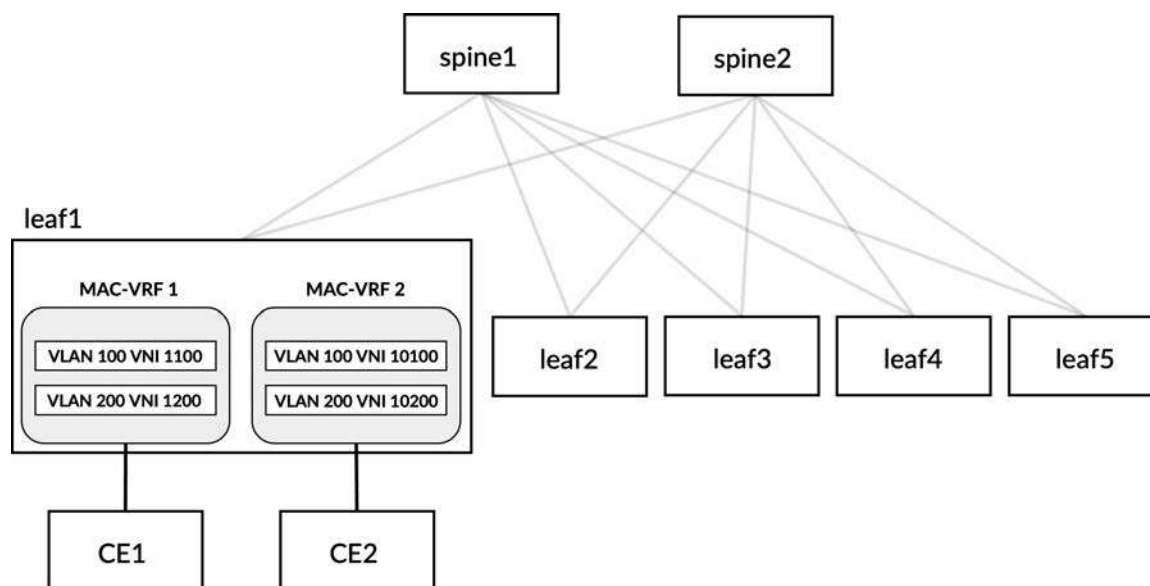
Figure 6-14 Overlapping VLANs between MAC-VRFs on leaf1
