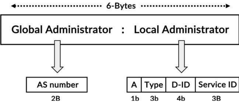
Figure 5-42 Auto-derived route-target breakdown
