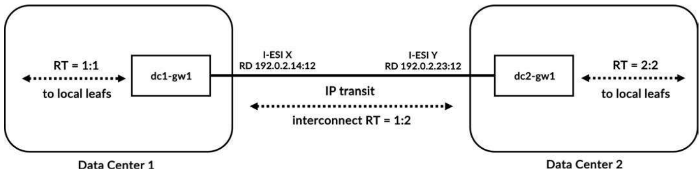
Figure 11-13 Interconnect details for VXLAN stitching between DC1 and DC2
