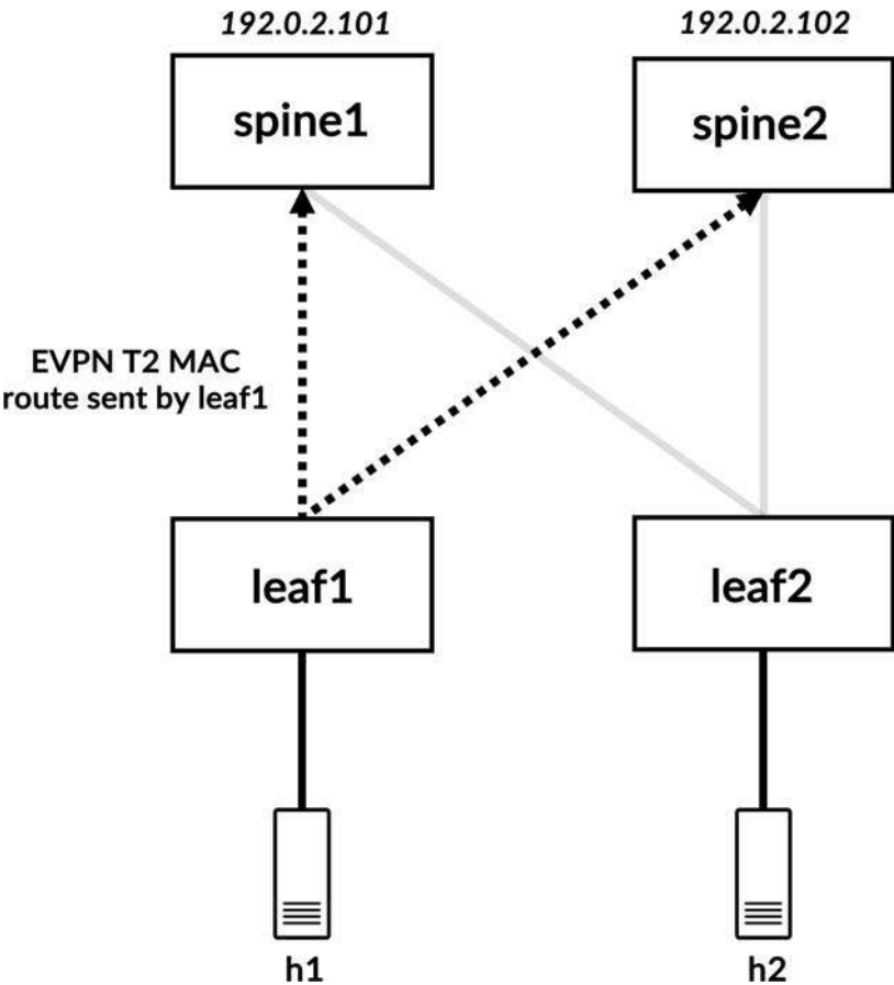
Figure 7-9 EVPN Type-2 MAC route sent to spine1 and spine2 by leaf1
