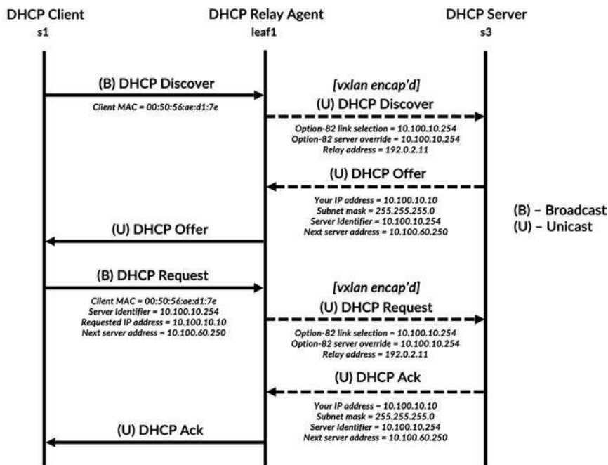
Figure 10-15 Packet flow of DHCP messages with a DHCP relay agent
