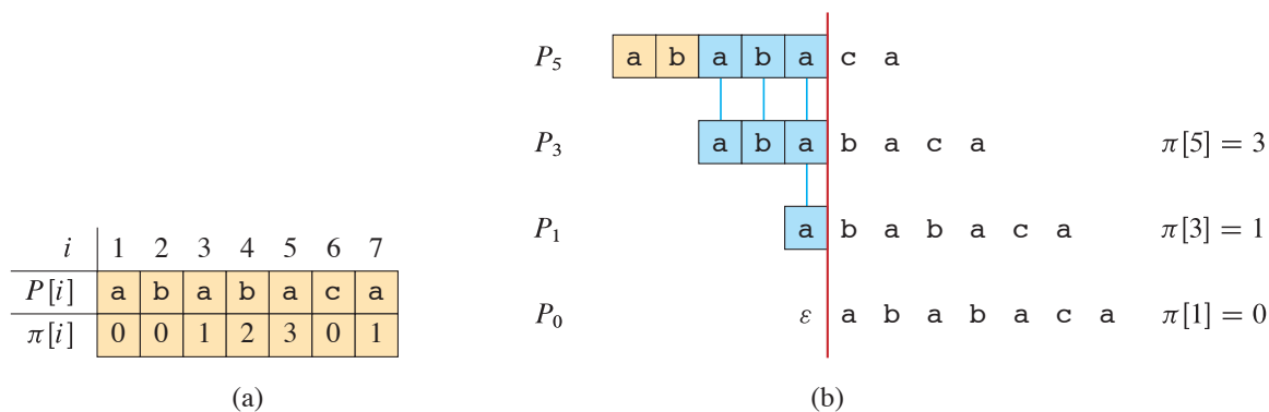
Figure 32.10 An illustration of Lemma 32.5 for the pattern P = ababaca and q = 5 . (a) The \pi function for the given pattern. Since \pi[5] = 3 , \pi[3] = 1 , and \pi[1] = 0 , iterating \pi gives \pi^*[5] = \{3, 1, 0\} . (b) Sliding the template containing the pattern P to the right and noting when some prefix P[:k] of P matches up with some proper suffix of P[:5] . Matches occur when k = 3, 1 , and 0 . In the figure, the first row gives P , and the vertical red line is drawn just after P[:5] . Successive rows show all the shifts of P that cause some prefix P[:k] of P to match some suffix of P[:5] . Successfully matched characters are shown in blue. Blue lines connect aligned matching characters. Thus, \{k : k < 5 \text{ and } P[:k] \sqsupseteq P[:5]\} = \{3, 1, 0\} . Lemma 32.5 claims that \pi^*[q] = \{k : k < q \text{ and } P[:k] \sqsupseteq P[:q]\} for all q .
