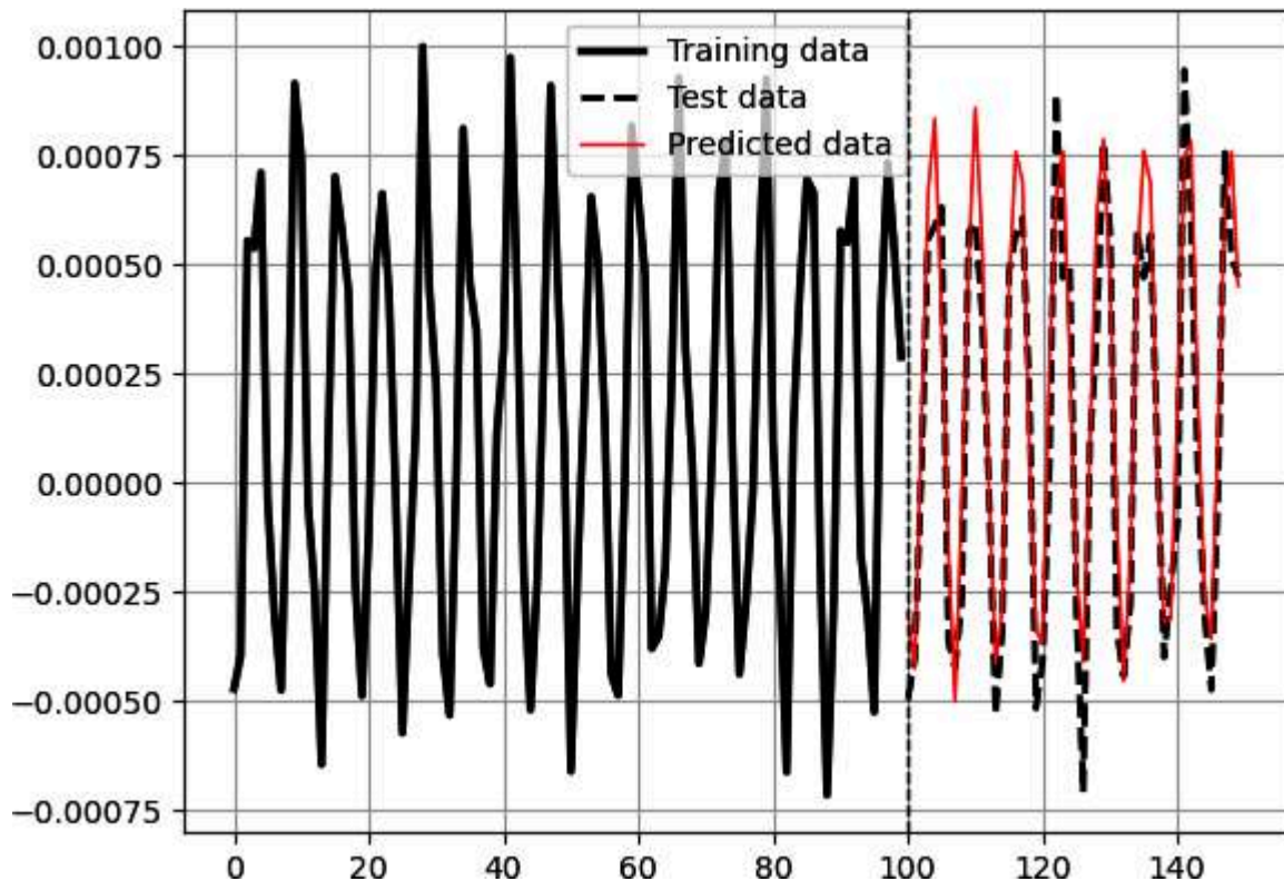
Figure 8-17. Prediction over the differenced time series using MLP.
