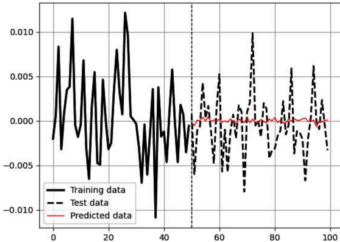
Figure 9-5. Predicting using the continuous retraining technique
