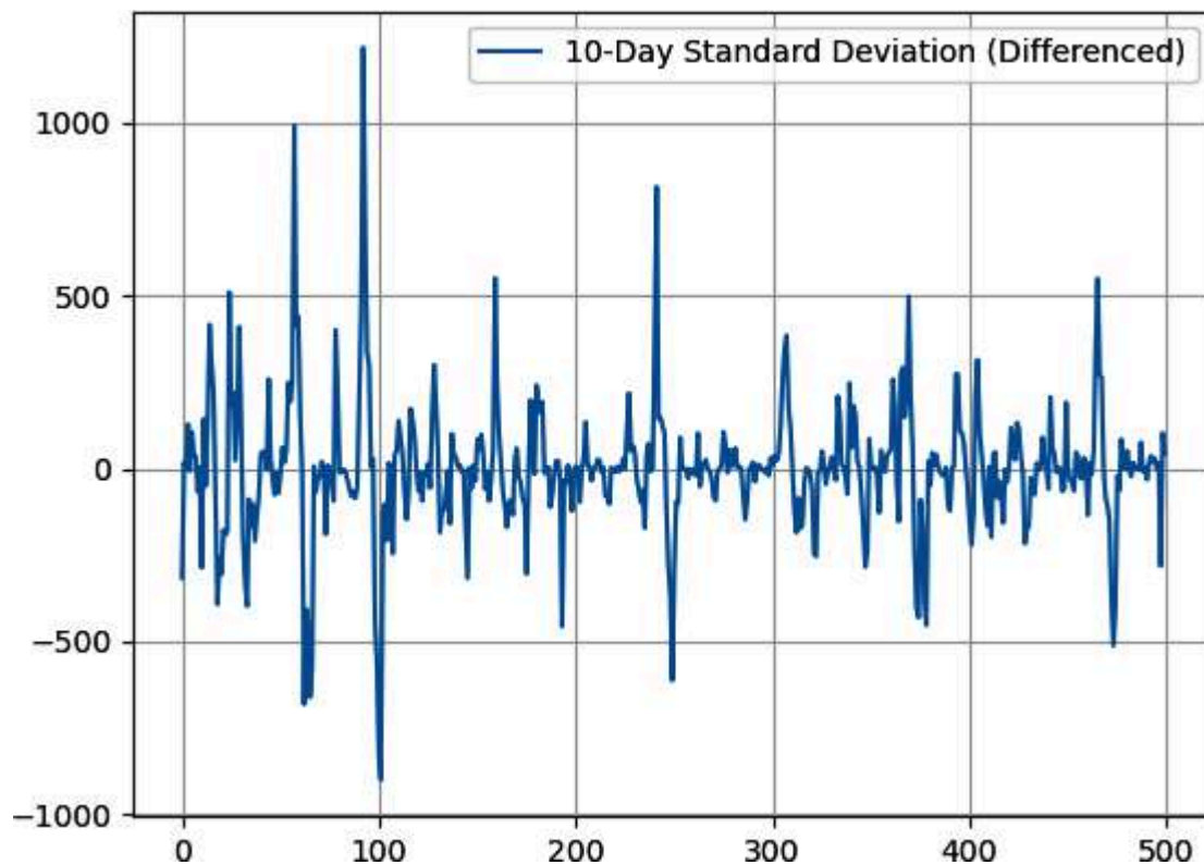
Figure 11-10. Bitcoin's rolling 10-day standard deviation (differenced).
