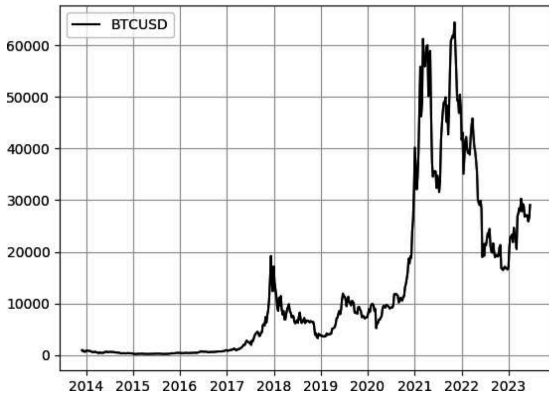
Figure 11-7. Historical evolution of BTCUSD since 2014 in a linear scale.
