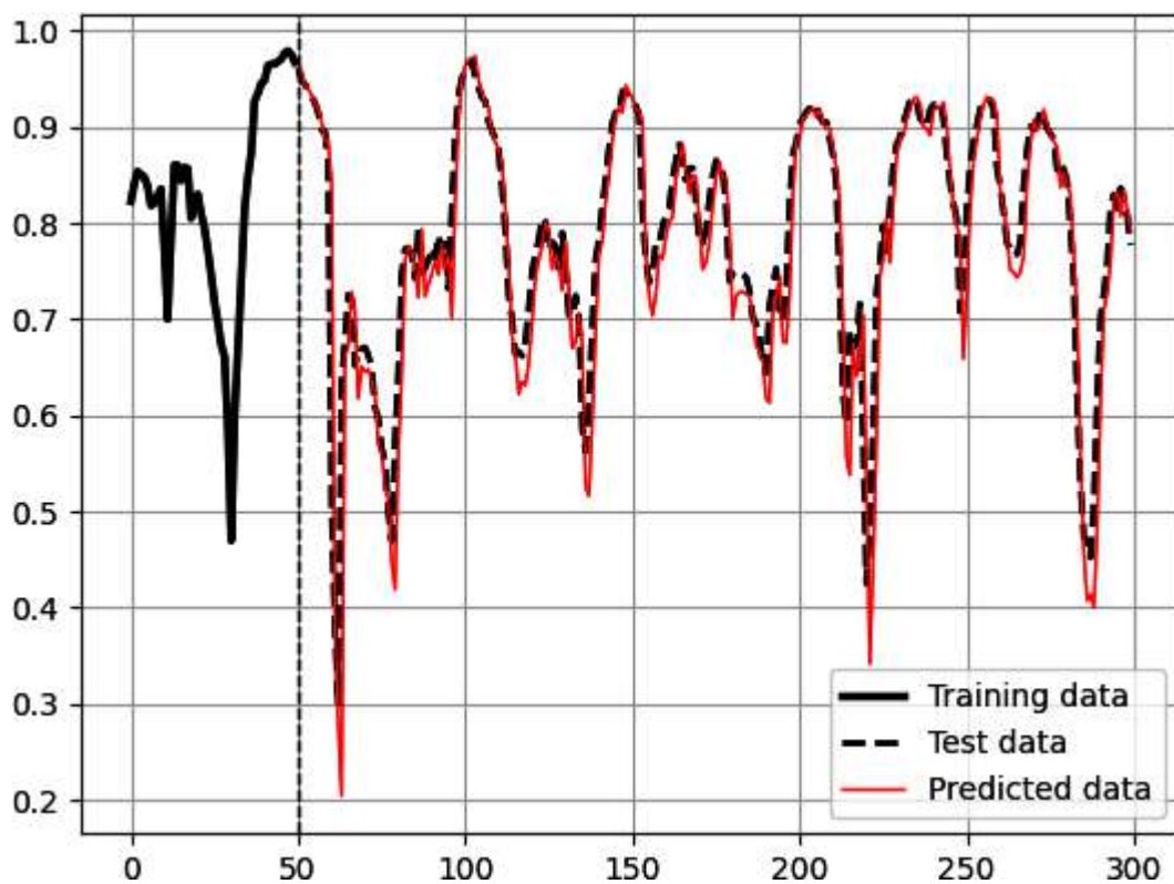
Figure 9-16. Predicting correlation
