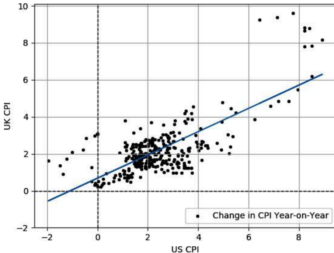
Figure 3-10. Scatterplot of UK CPI data versus US CPI data with a best-fit line
