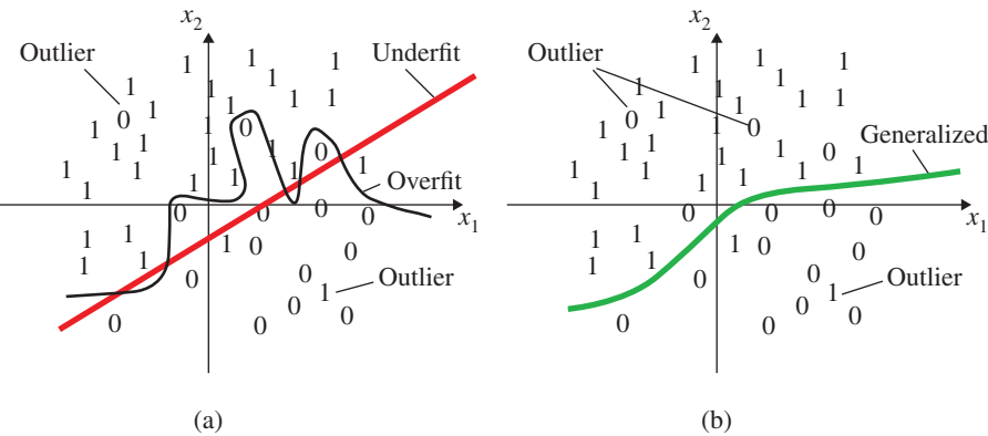
Figure 8.10 Effect of overfitting, underfitting, and generalization. (a) overfitting and underfitting, and (b) generalized result.
