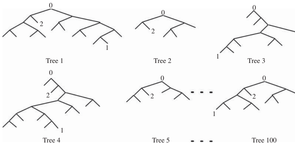
Figure 11.7 Illustration of random tree generation for Isolation Forest.
