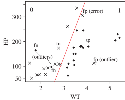
Figure 9.8 Examples of different logical cases involving outliers and errors.
