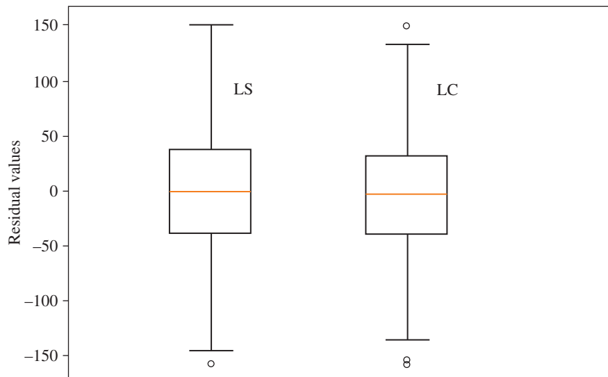
Figure 6.7 Boxplots of residuals from LS and LC for diabetes dataset.
