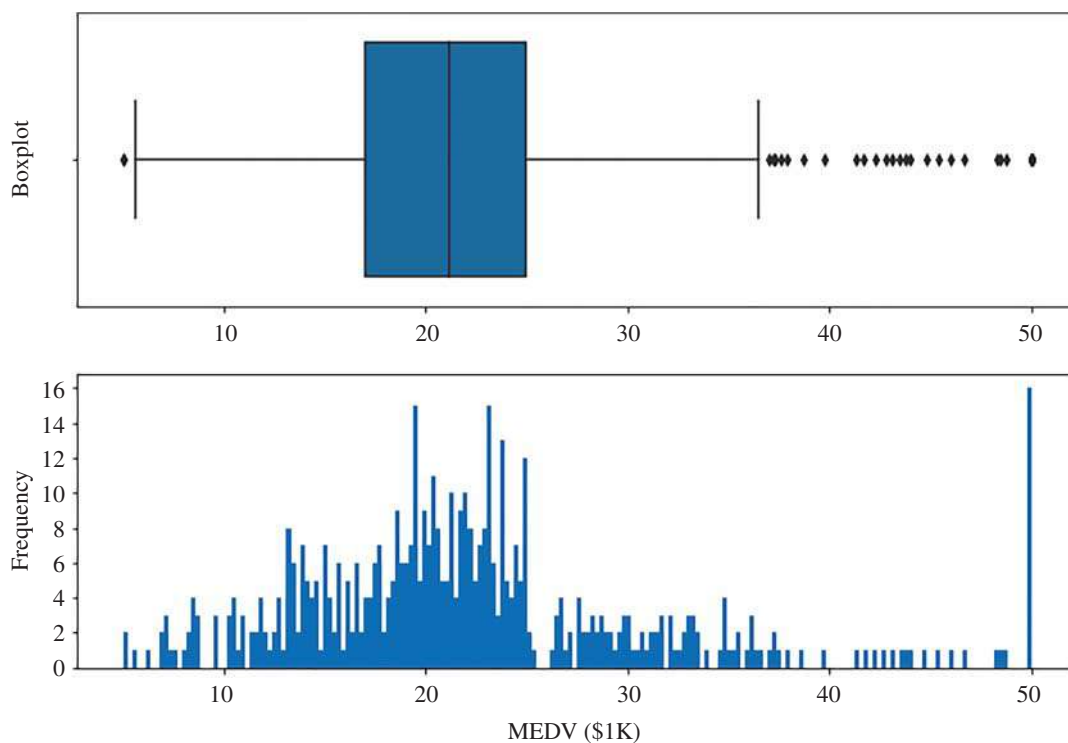
Figure 12.1 Relationship between boxplot and histogram of MEDV indicating suspected outliers and a large spike at $50K.
