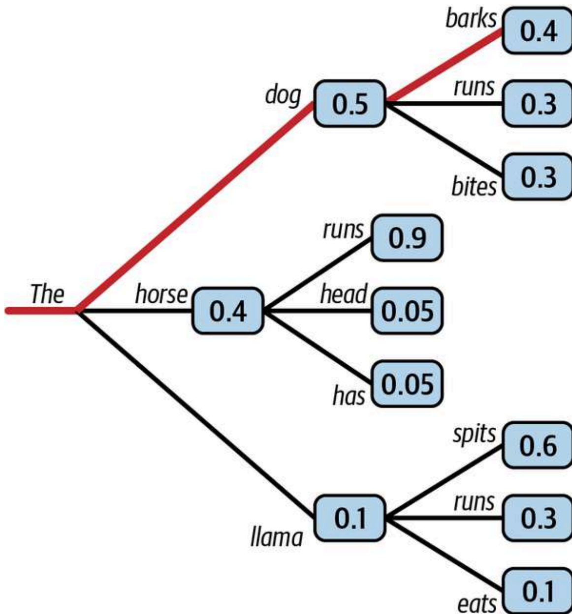
Figure 2-4. This greedy decoding example generates “The dog barks” because “dog” is the most likely second token with a probability of 0.5, and “barks” is the most likely token following “The dog”
