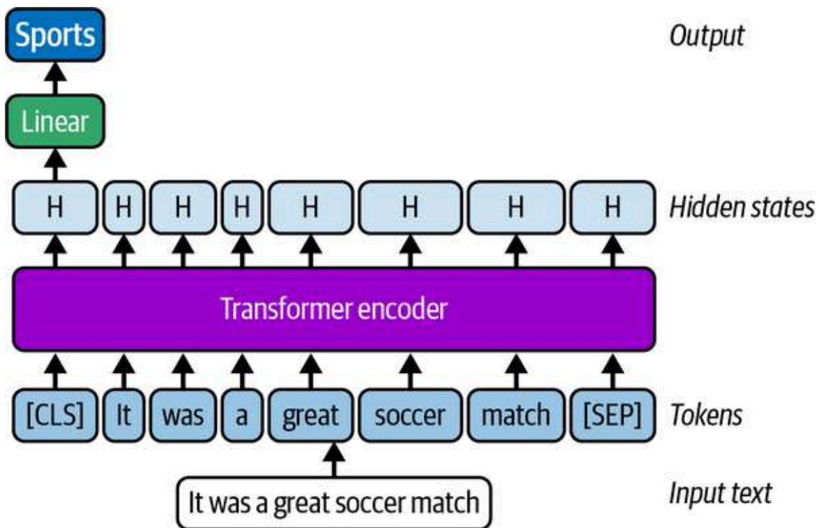
Figure 6-2. BERT with a classification head. In practice, the embedding corresponding to CLS is used as the pooled embedding and can be used for classification tasks.
