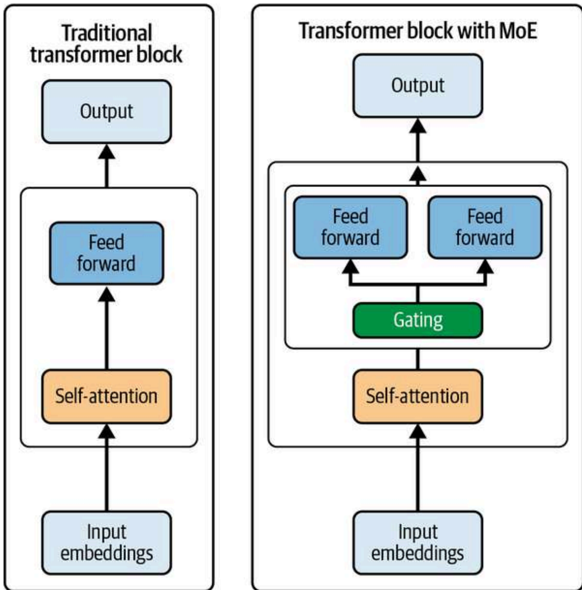
Figure 10-4. A simplified traditional transformer block and its MoE equivalent having two experts
