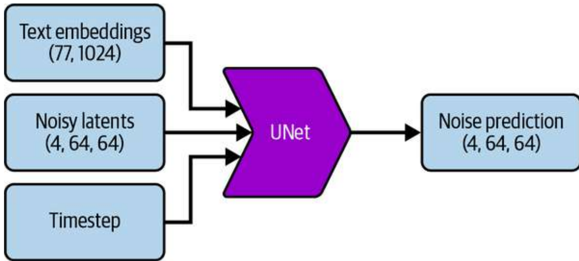
Figure 5-2. The UNet can be conditioned on multiple inputs, such as the timestep, the class label, or the text embeddings
