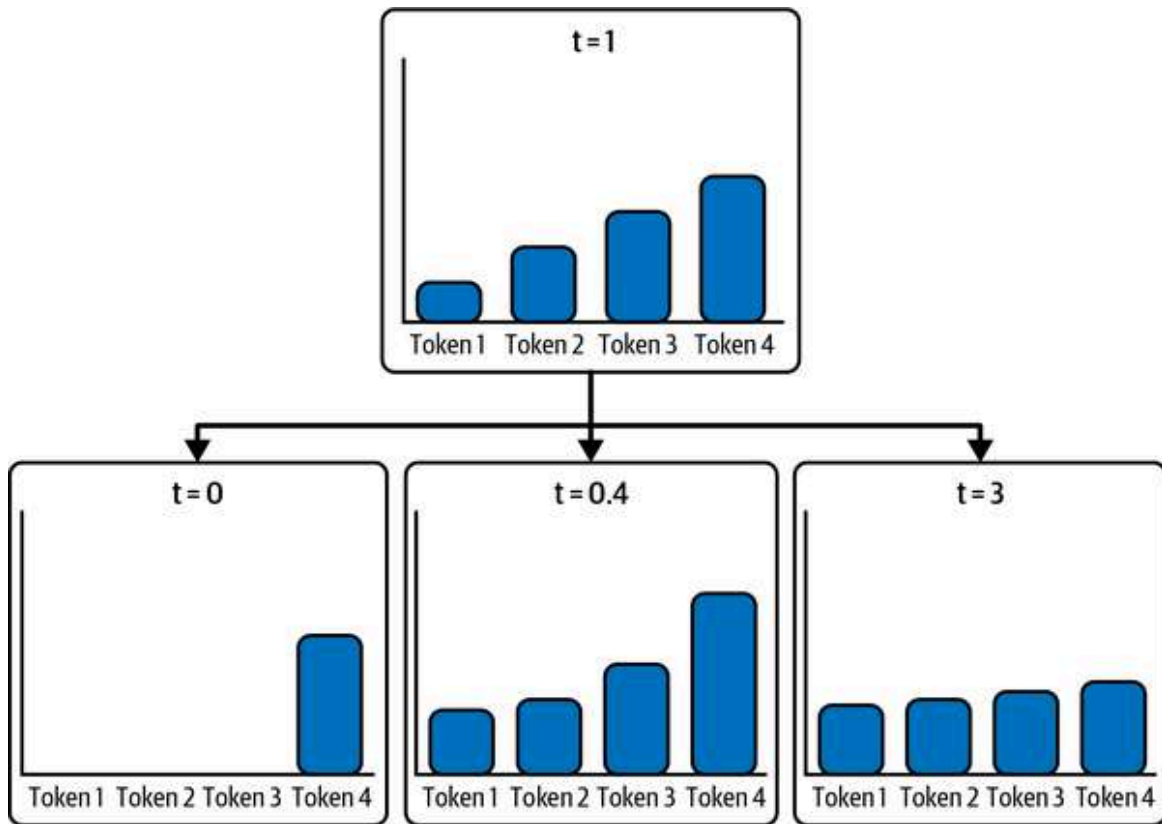
Figure 2-7. Effect of temperature on the token probability distribution
