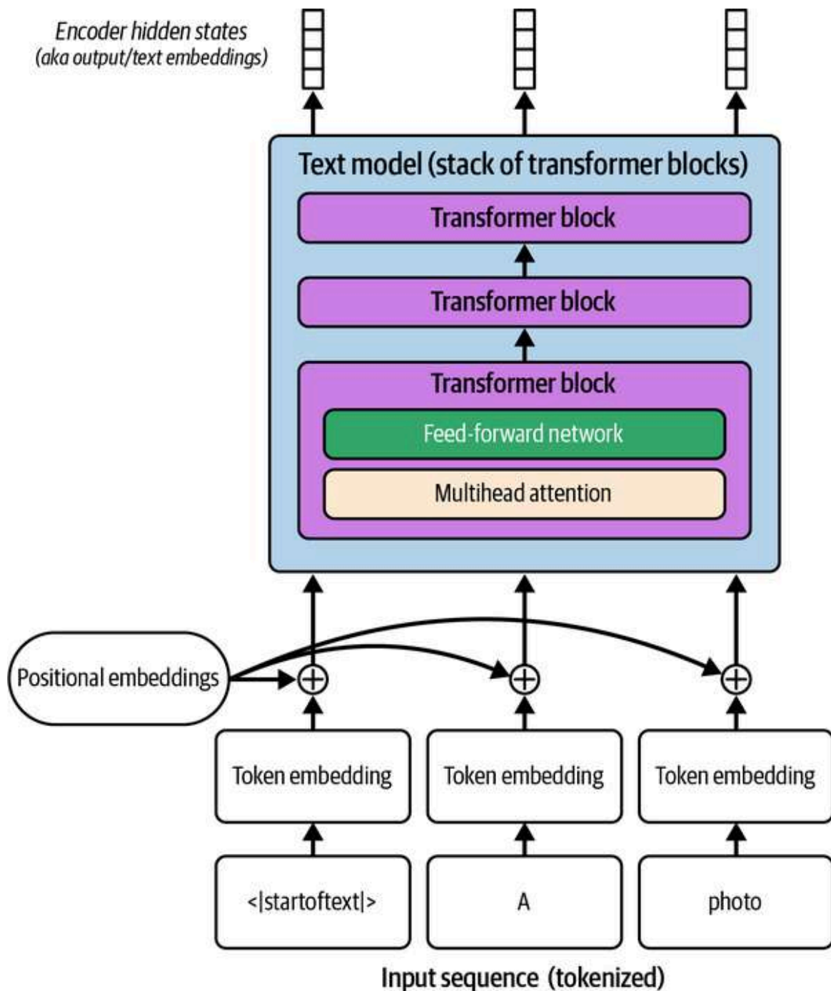
Figure 5-3. The text-encoding process transforms the input prompt into a set of text embeddings (the encoder hidden states), which can then be fed in as conditioning to the UNet
