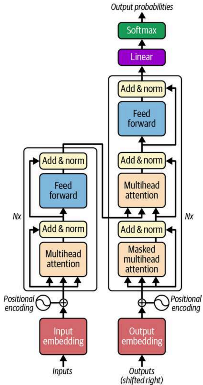
Figure 2-10. The encoder-decoder transformer (adapted from an image in the original transformer paper )
