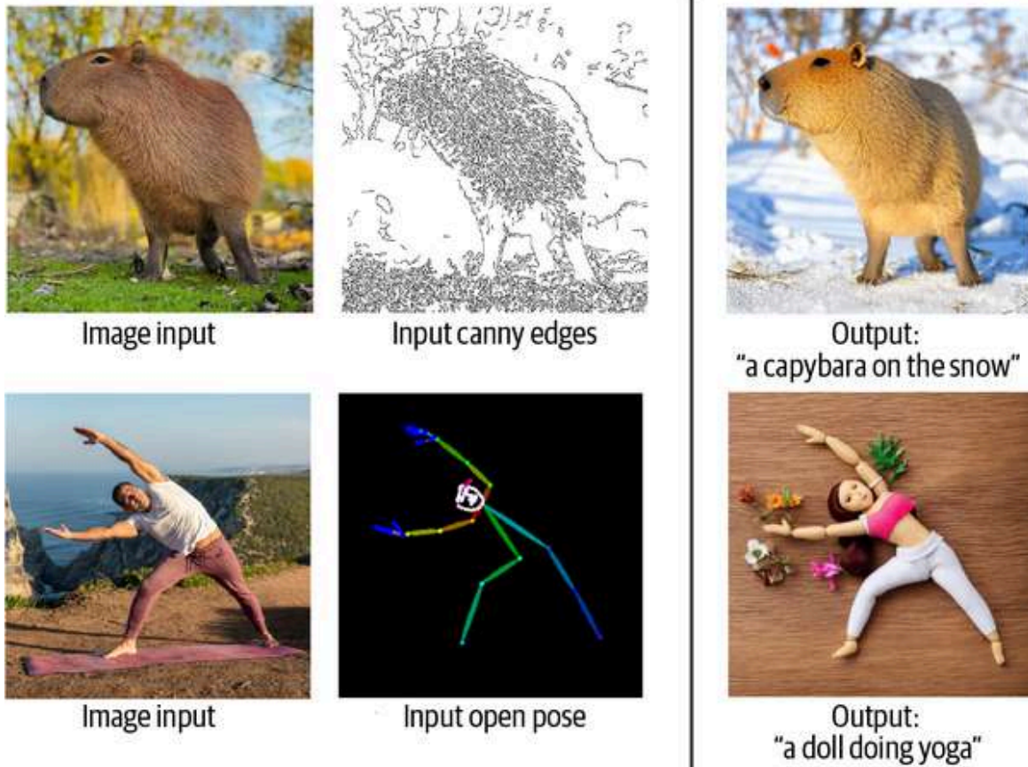
Figure 8-4. ControlNet examples with image input, canny edges, and open pose conditionings, and the generated output
