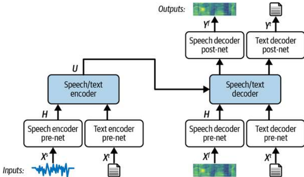
Figure 9-9. Architecture of the SpeechT5 model (adapted from an image in the original paper )
