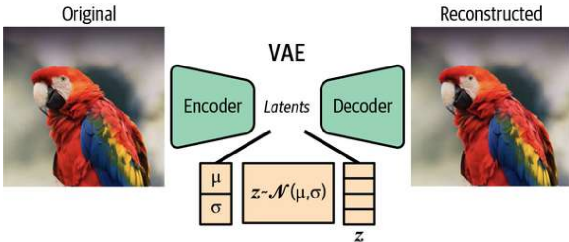
Figure 3-4. VAEs learn Gaussian representations of the features and describe them through their means and variances. Points z in the latent space are sampled from the predicted Gaussian distributions.
