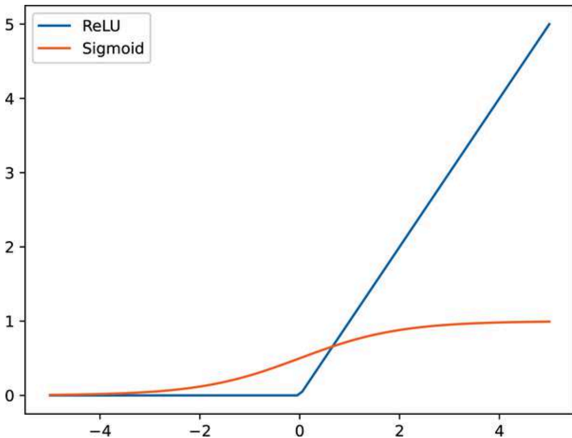
Figure 3-3. Activation functions: ReLU versus Sigmoid
