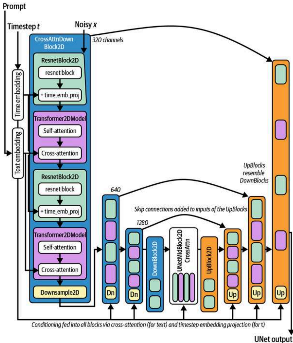
Figure 5-5. Conditioned UNet architecture
