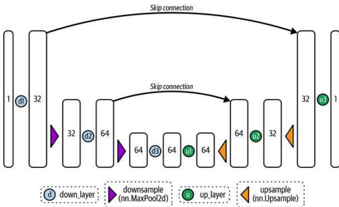
Figure 4-3. Architecture of a simplified UNet
