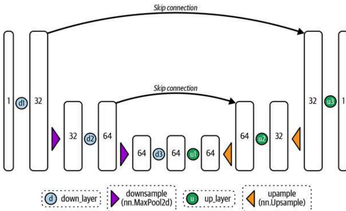
Figure 4-7. Architecture of a basic UNet
