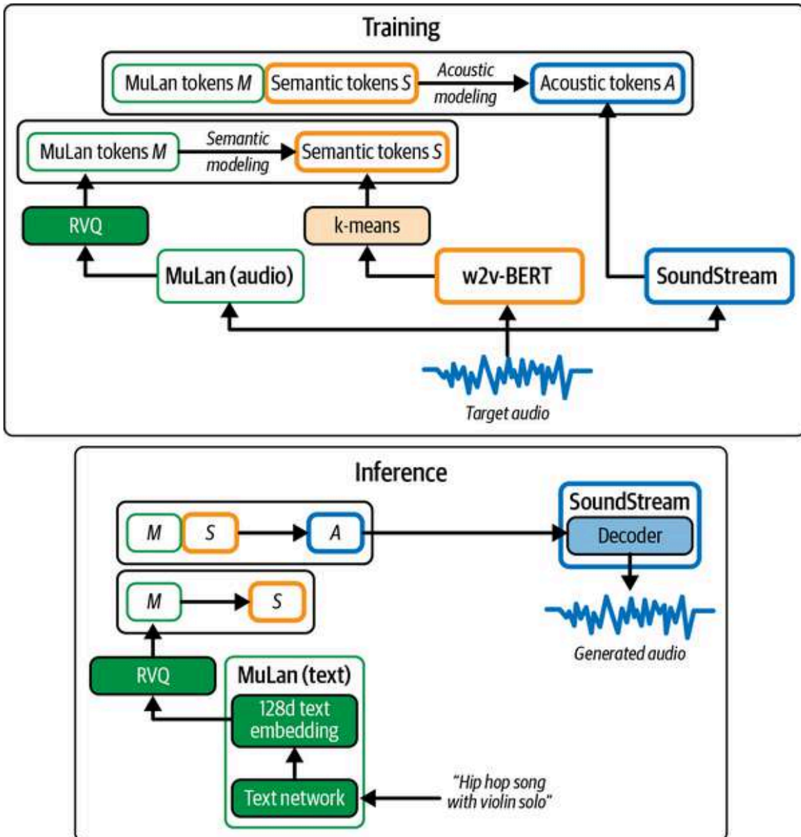
Figure 9-12. MusicLM incorporates text conditioning to the AudioLM architecture, to generate audio based on a prompt (adapted from an image in the original paper )
