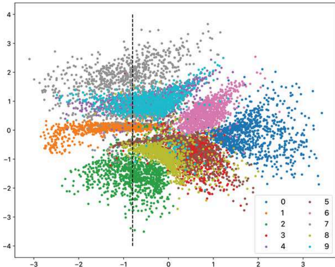
Figure 3-6. VAE latent space focusing on samples where x = -0.8
