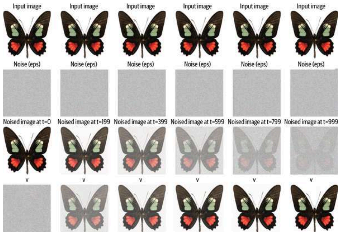
Figure 4-11. Comparing eps versus x0 versus v objectives: eps tries to predict the noise added at each timestep, x0 predicts the denoised image, and v uses a mixture of the two
