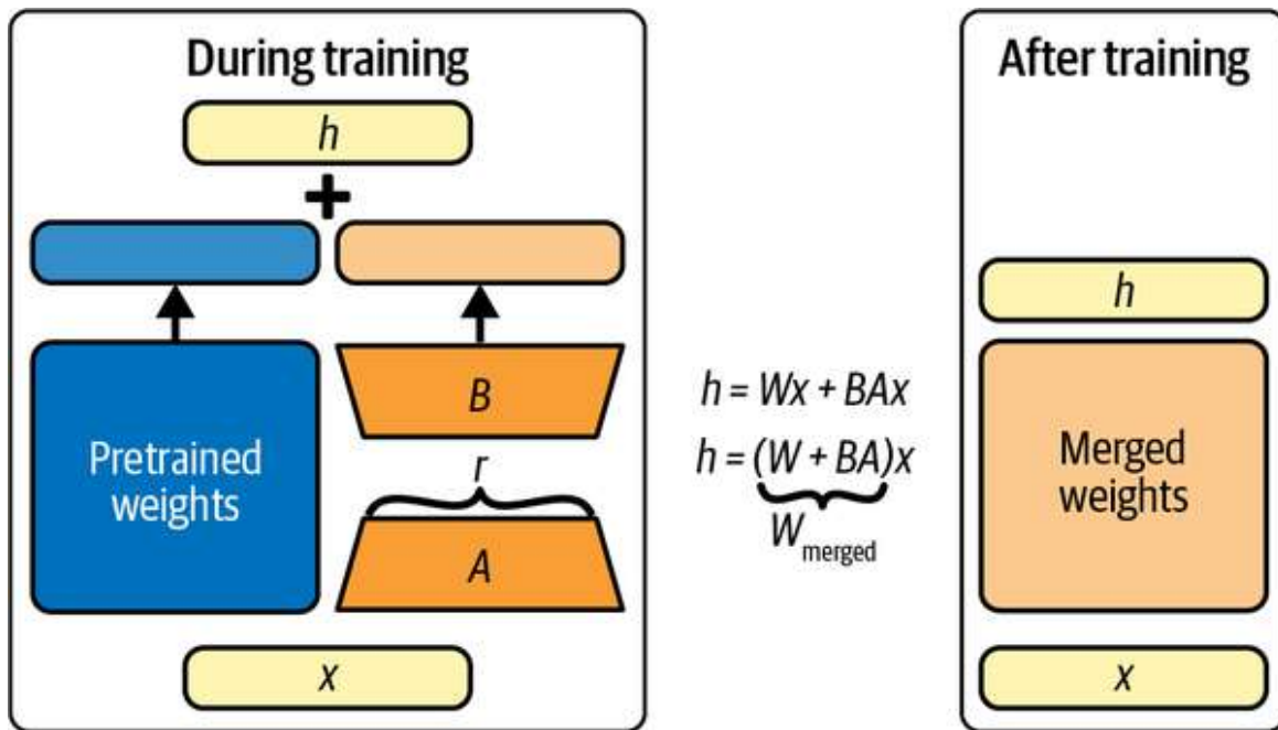
Figure 7-5. LoRA architecture flow
