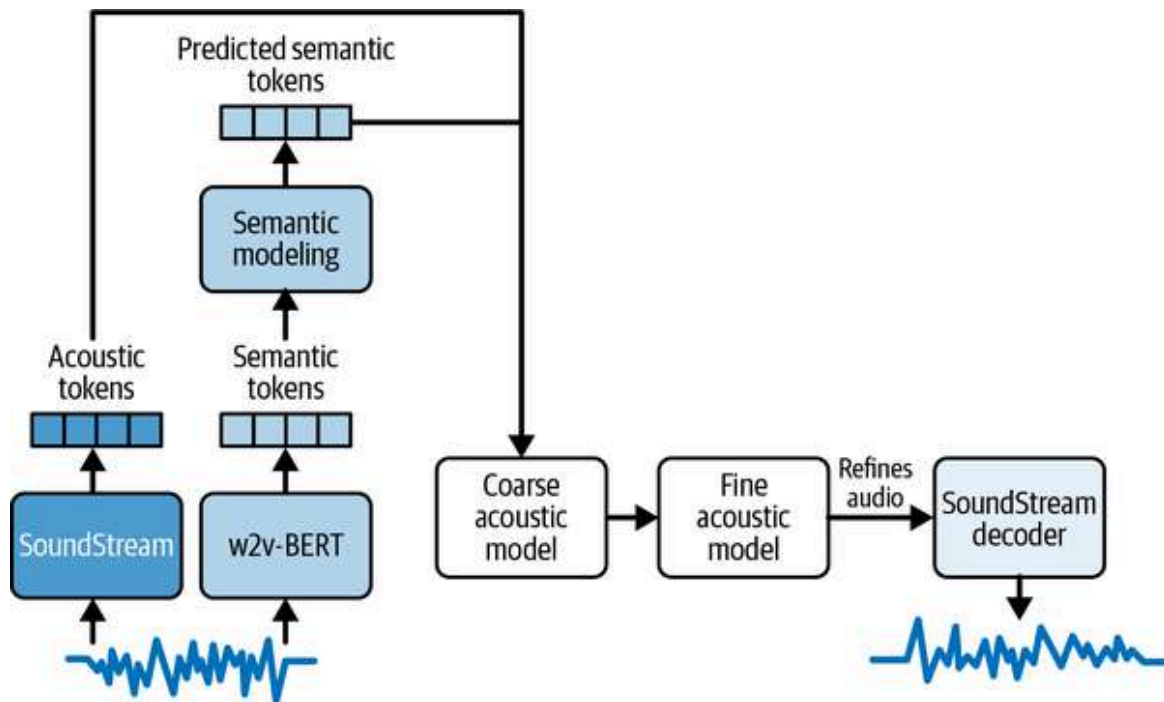
Figure 9-11. In the AudioLM model pipeline, AudioLM converts the input audio to a sequence of tokens and performs audio generation using language-modeling techniques (adapted from an image in the original paper )
