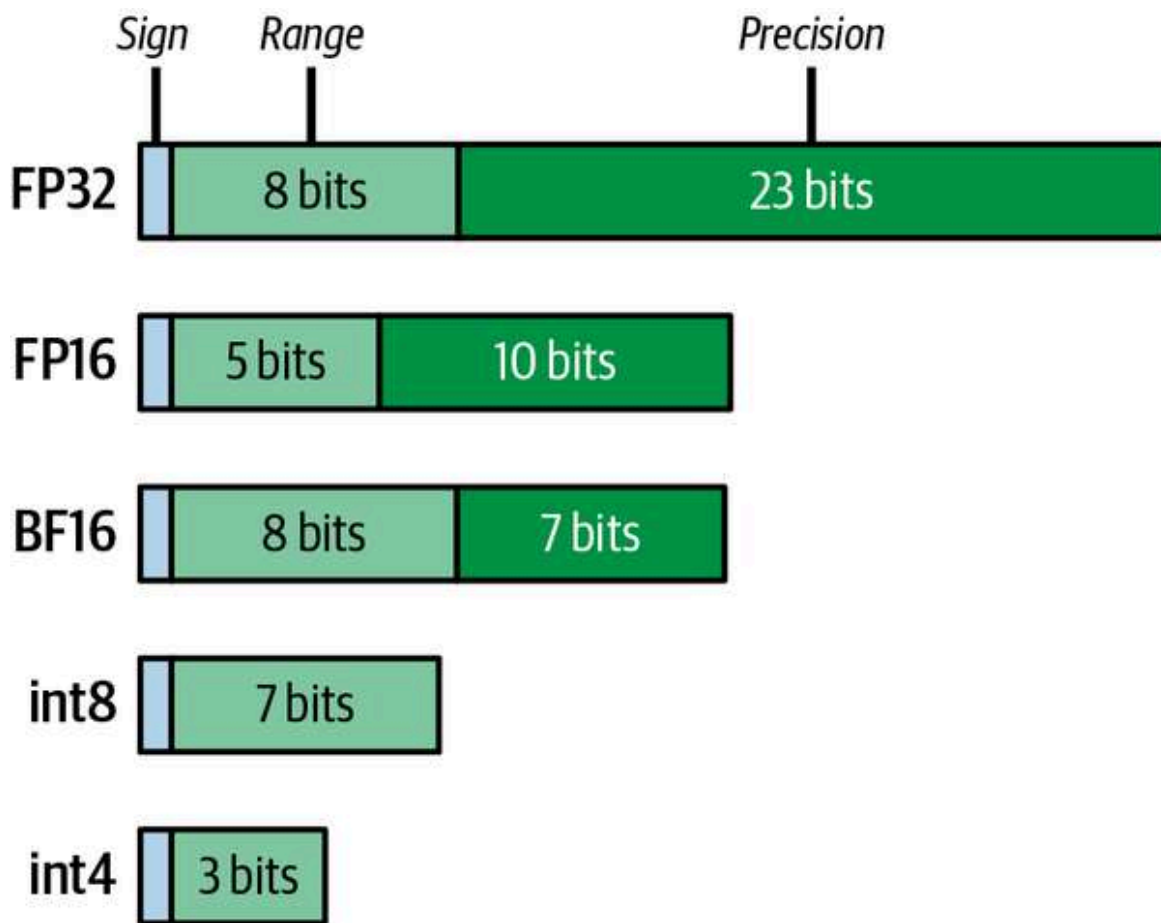
Figure 6-5. How different precisions are represented
