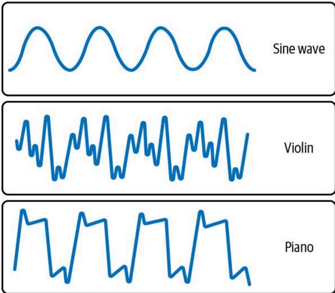
Figure 9-5. The same note played by several instruments has the same pitch (frequency) and amplitude, but it sounds different because of the waveform's shape variations. A pure note is a perfect sine wave.
