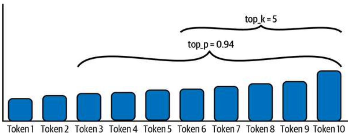
Figure 2-8. Effect of top_k and top_p on the token probability distribution. With top_k=5 , only the five most likely tokens are considered. With top_p=0.94 , we include all tokens until they cumulatively have a probability of 0.94.
