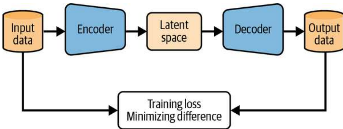
Figure 3-2. AutoEncoder architecture
