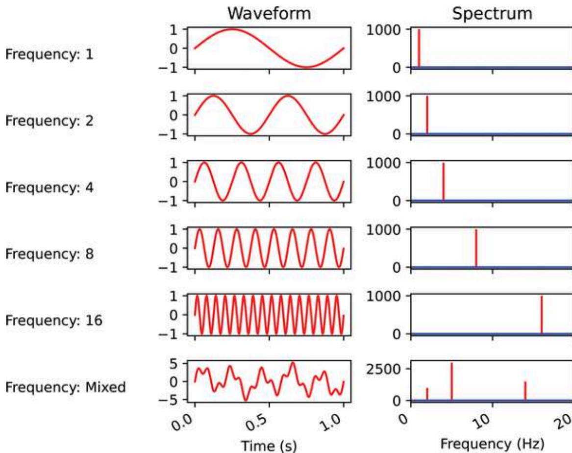
Figure 9-6. Some sinusoidal functions and their frequency spectrums. Pure notes (sine waves) have a single peak at the sine period, whereas more-complex sounds show several peaks in the frequency domain.
