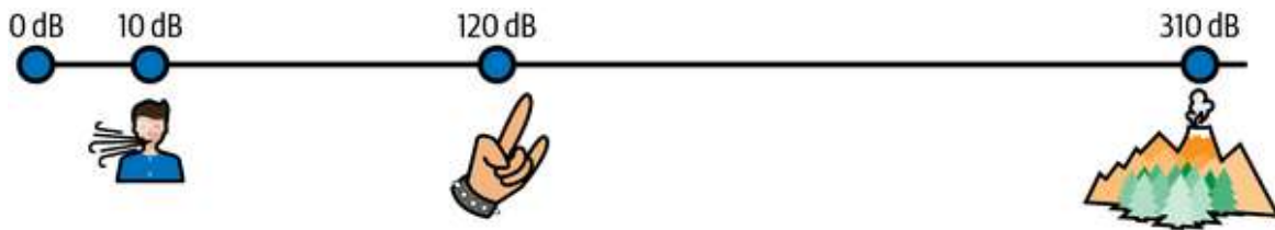
Figure 9-3. The amplitude of some sounds in the dB scale
