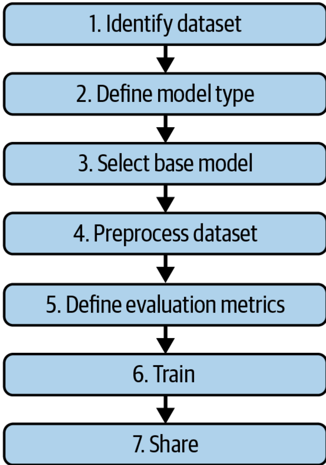
Figure 6-1. The usual steps of a fine-tuning workflow
