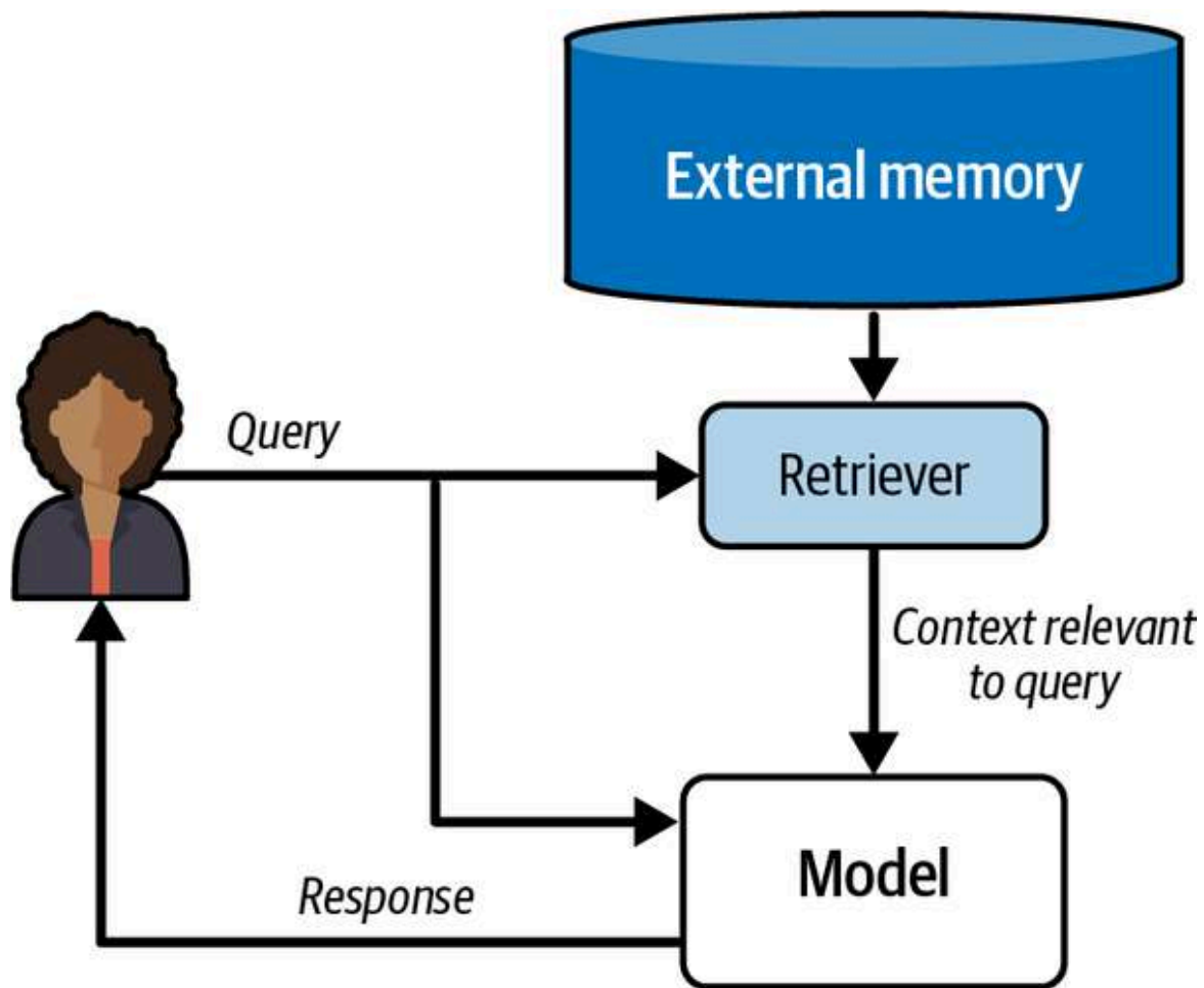
Figure C-1. A simplified RAG pipeline
