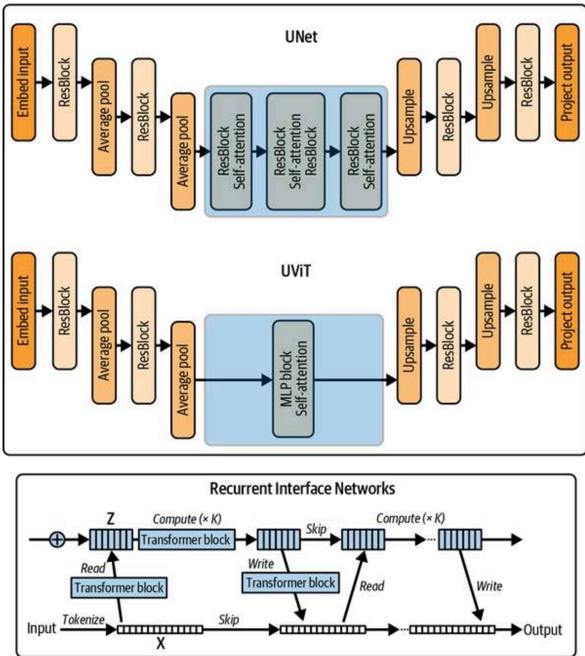
Figure 4-10. Comparison of UNet with UViT and RIN
