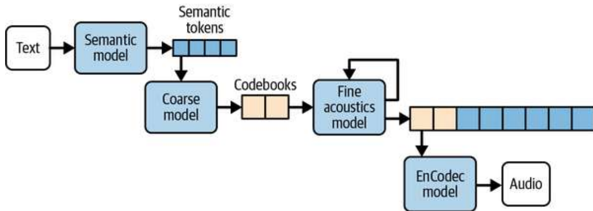
Figure 9-10. The Bark pipeline uses three components: text-to-semantic tokens, semantic-to-coarse tokens, and coarse-to-fine tokens
