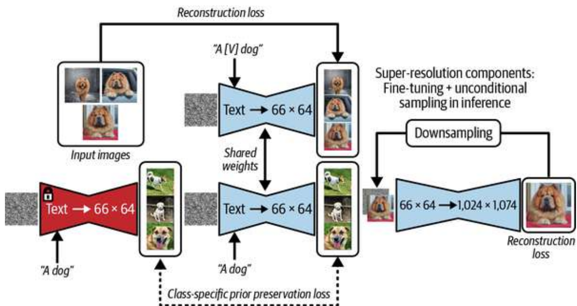
Figure 7-2. The DreamBooth architecture flow
