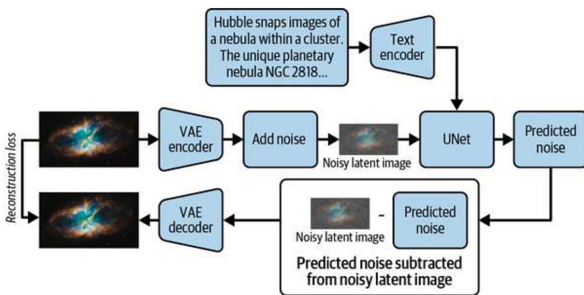
Figure 7-1. Stable Diffusion fine-tuning architecture
