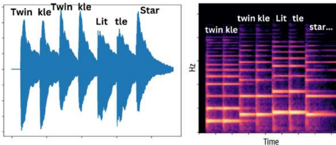
Figure 9-4. Waveform (left) and mel spectrogram (right) representing the same audio clip
