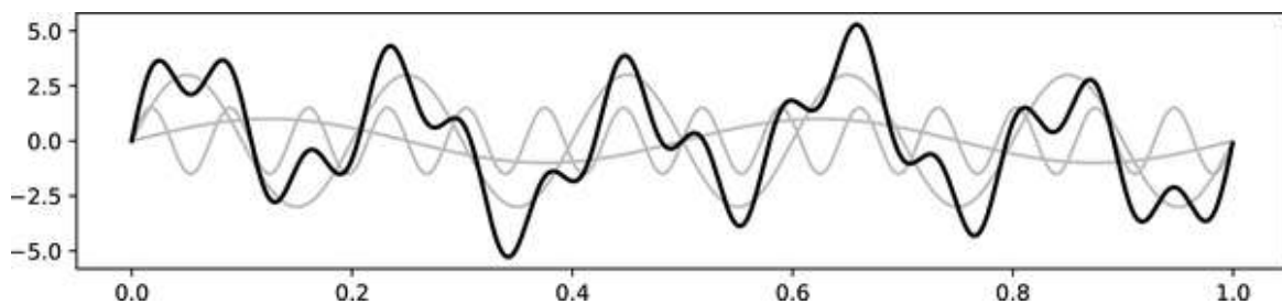
Figure 9-7. A complex sound wave can be decomposed into sinusoidal frequencies by analyzing the spectrum representation
