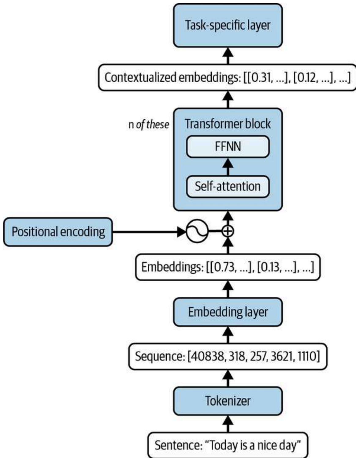
Figure 2-9. Architecture of a transformer-based language model
