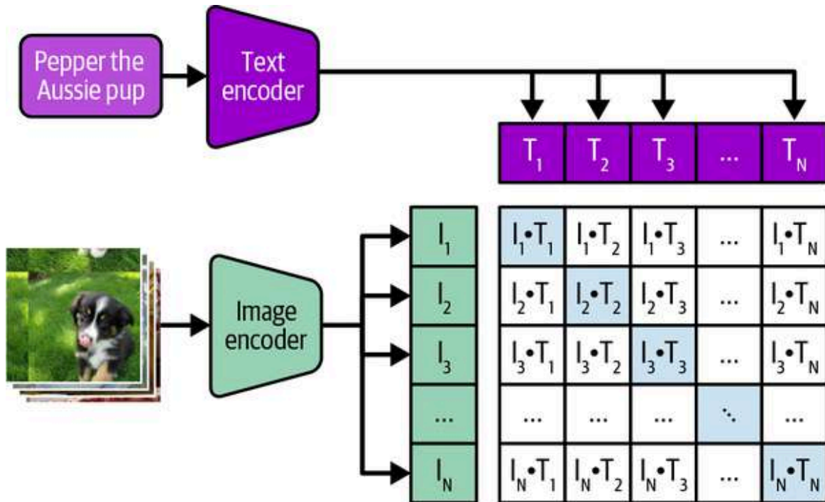
Figure 3-7. CLIP (adapted from an image by OpenAI )
