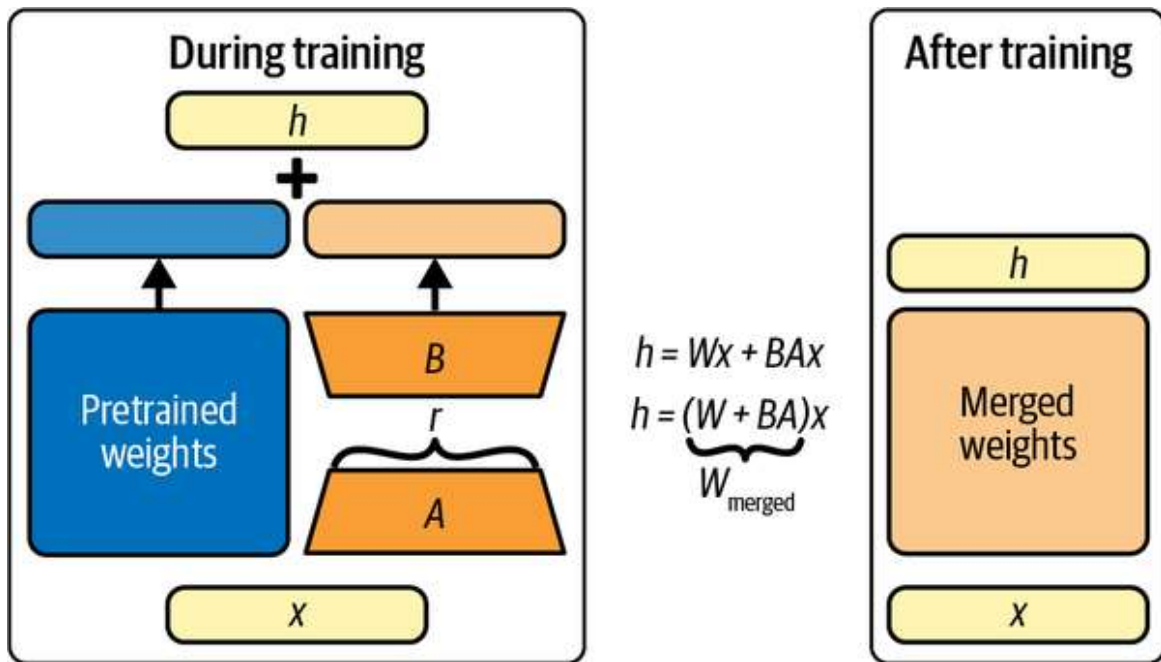
Figure 6-4. LoRA reduces the number of trainable weights. Once trained, the LORA weights can be merged back into the original model.
