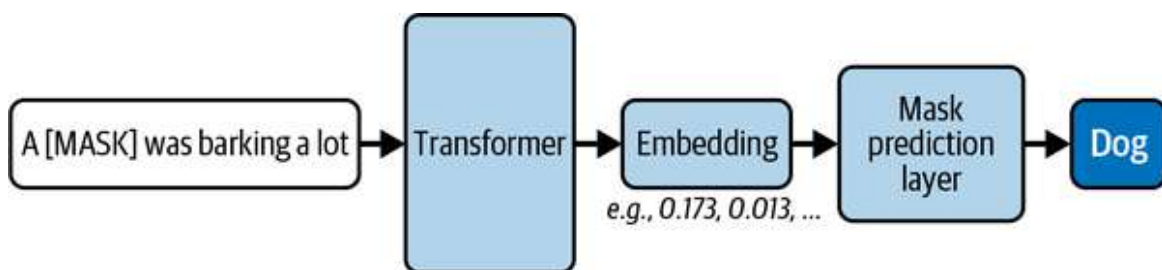
Figure 2-11. Encoder models output semantic embeddings that can be used to solve tasks such as predicting a token in the middle of a sequence
