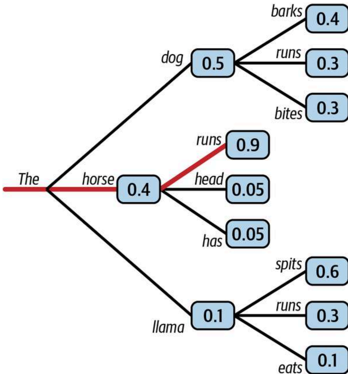
Figure 2-5. This beam search example finds a more likely sequence: “The dog barks” has a total probability of 0.5 \times 0.4 = 0.2 , while “The horse runs” has a probability of 0.4 \times 0.9 = 0.36
