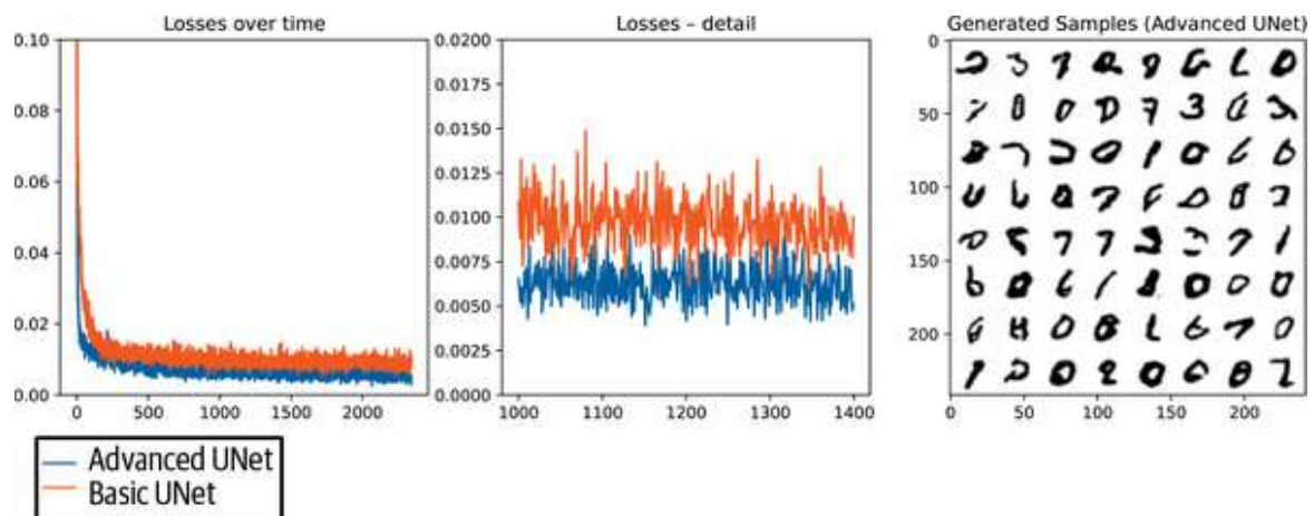
Figure 4-9. Loss and generations from the diffusers UNet, with several improvements over the basic architecture
