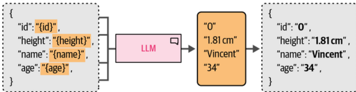
Figure 6-20. Use an LLM to generate only the pieces of information we do not know beforehand.
