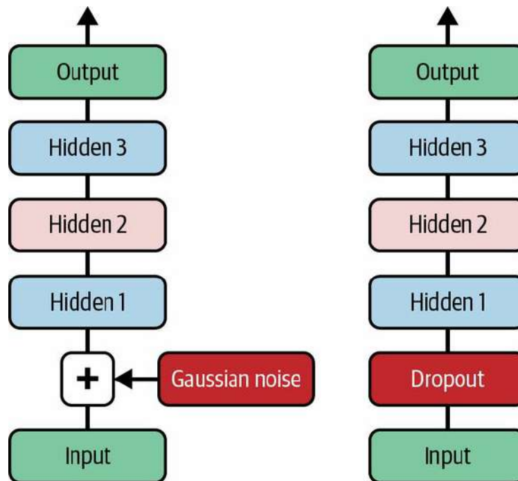
Figure 17-8. Denoising autoencoders, with Gaussian noise (left) or dropout (right)
