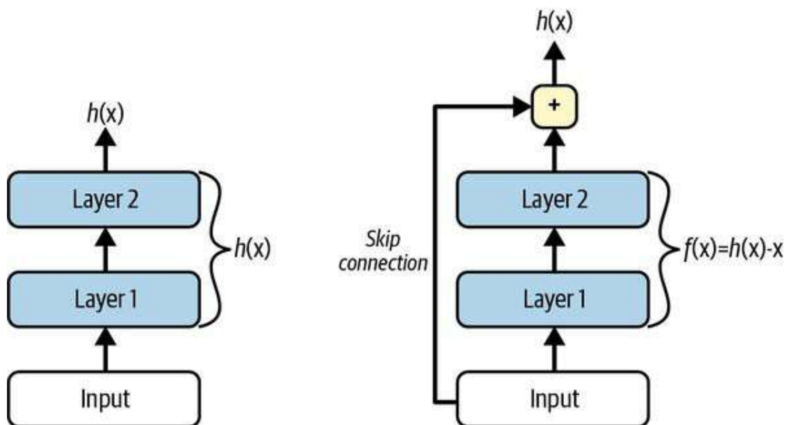
Figure 14-16. Residual learning
