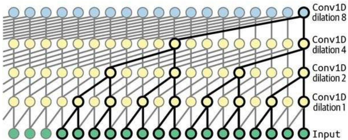
Figure 15-14. WaveNet architecture
