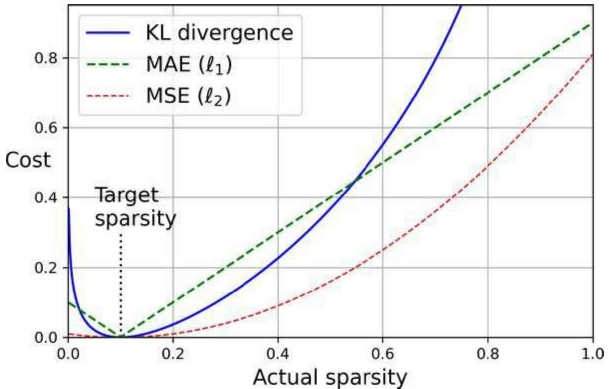
Figure 17-10. Sparsity loss
