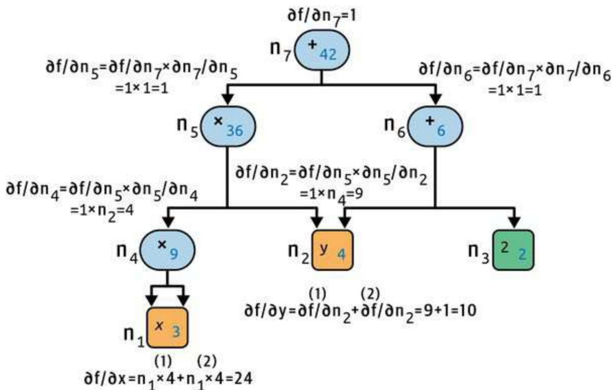
Figure B-3. Reverse-mode autodiff
