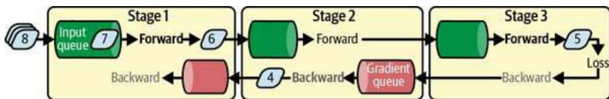
Figure 19-17. PipeDream's pipeline parallelism
