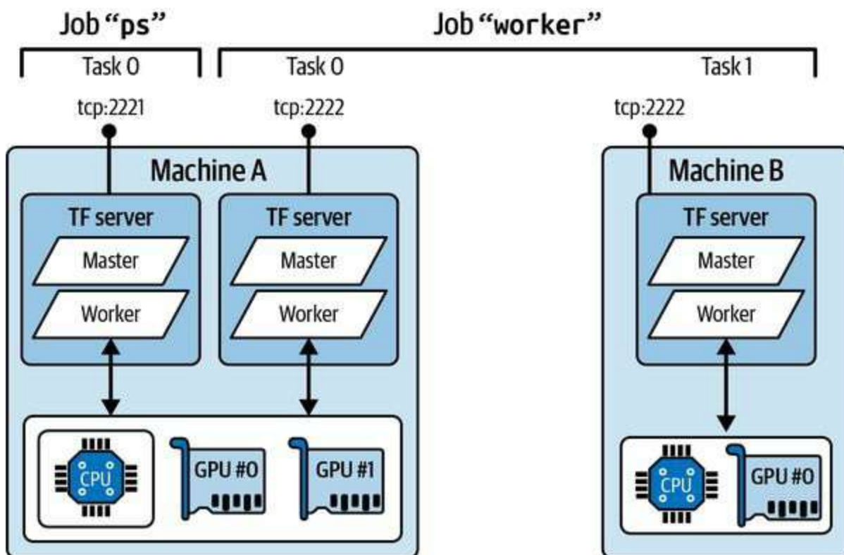
Figure 19-18. An example TensorFlow cluster
