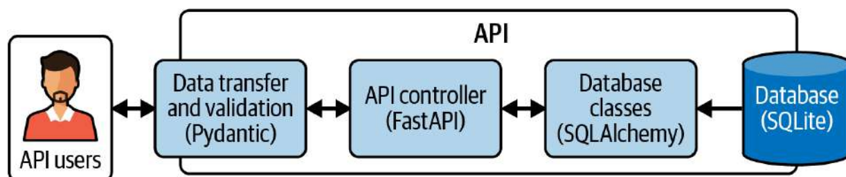
Figure 3-1. API components
