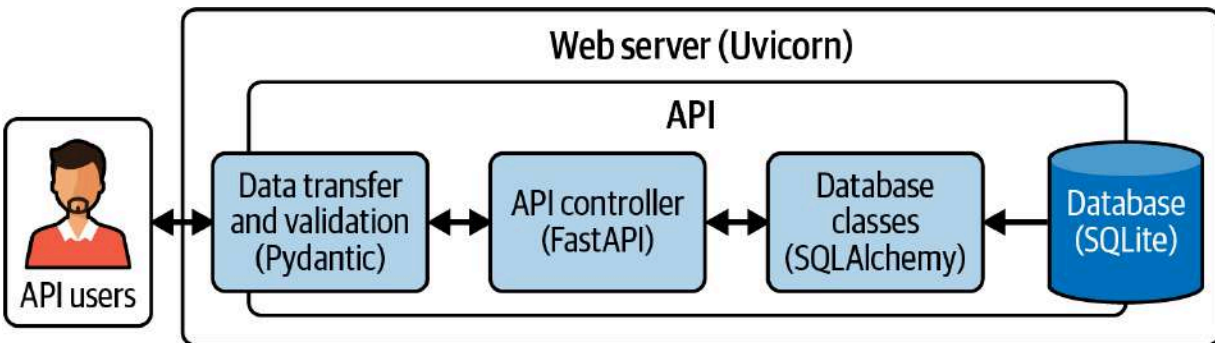
Figure 4-1. API components with Uvicorn
