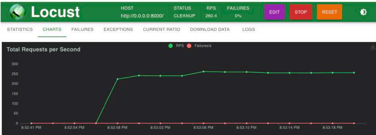
Figure 8-3. Example Locust load test report
