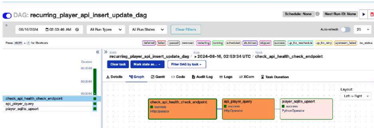
Figure 10-10. Successful DAG run
