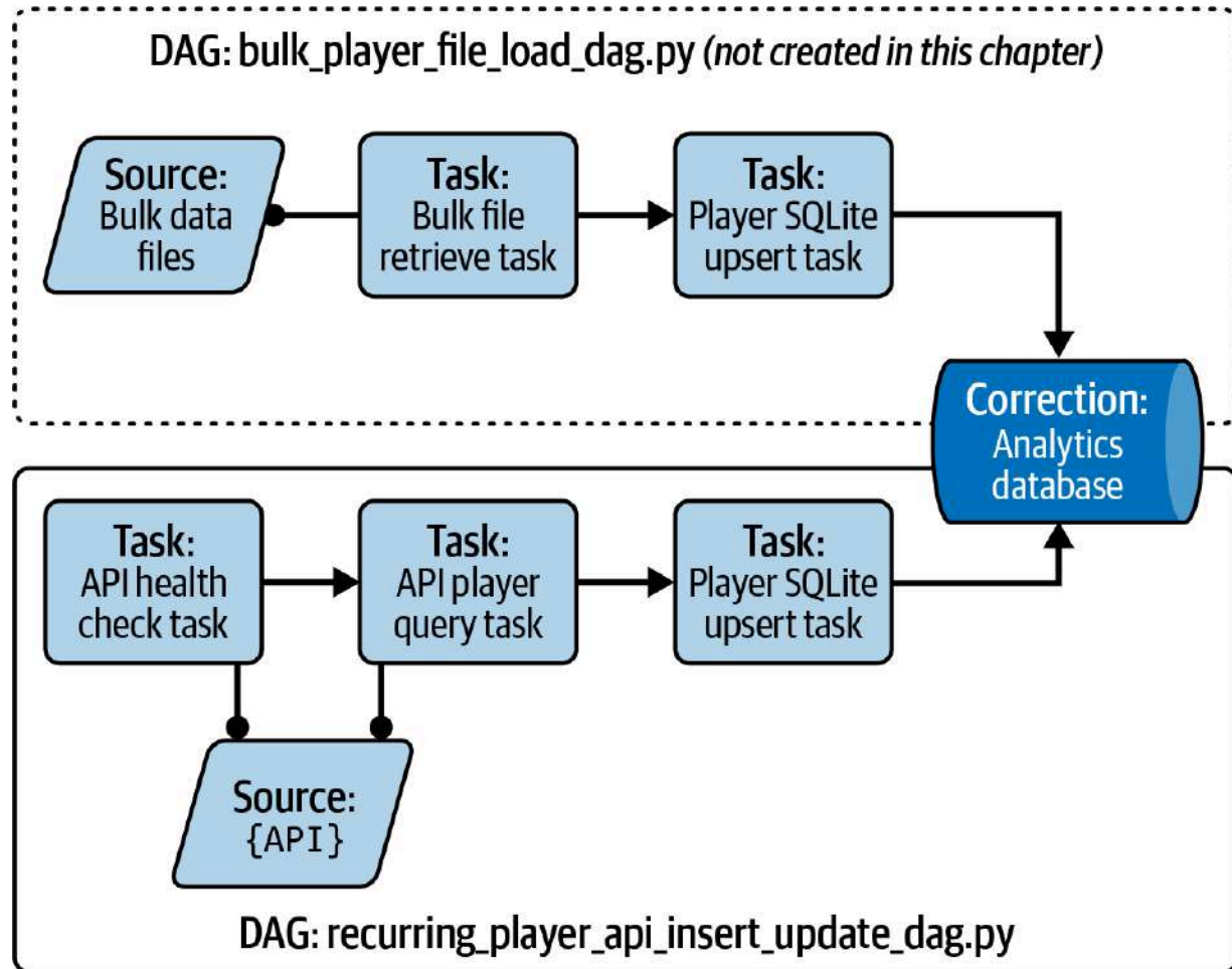
Figure 10-7. Airflow components of your data pipeline
