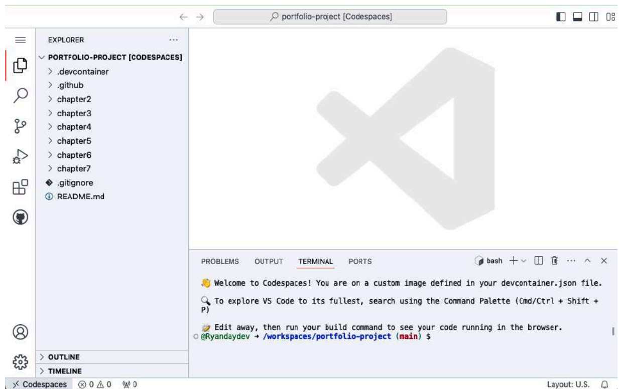
Figure 2-3. New GitHub Codespace
