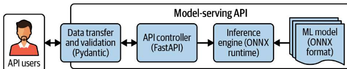
Figure 13-3. Model-serving API components
