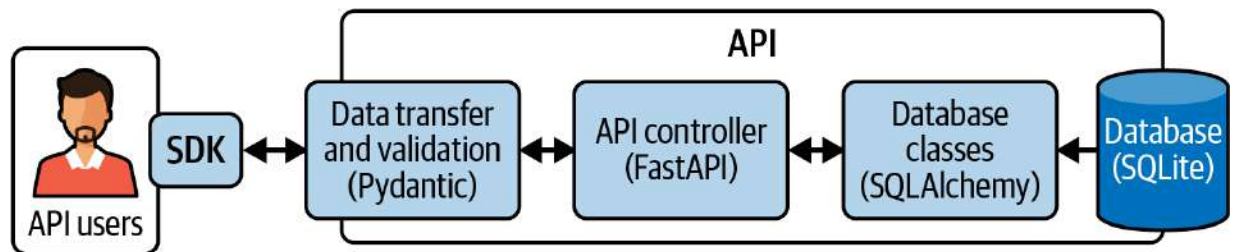
Figure 7-1. SDK interacting with the API
