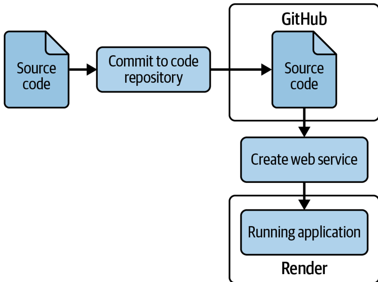
Figure 6-3. Deploying your API to Render
