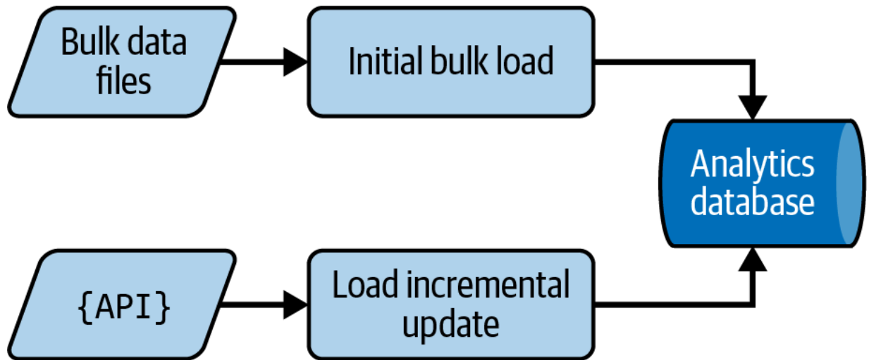
Figure 10-1. Plan for your data pipeline
