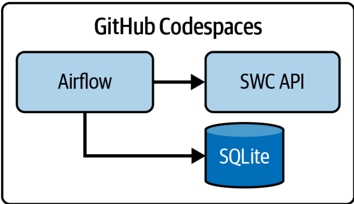
Figure 10-3. Architecture of the Airflow project
