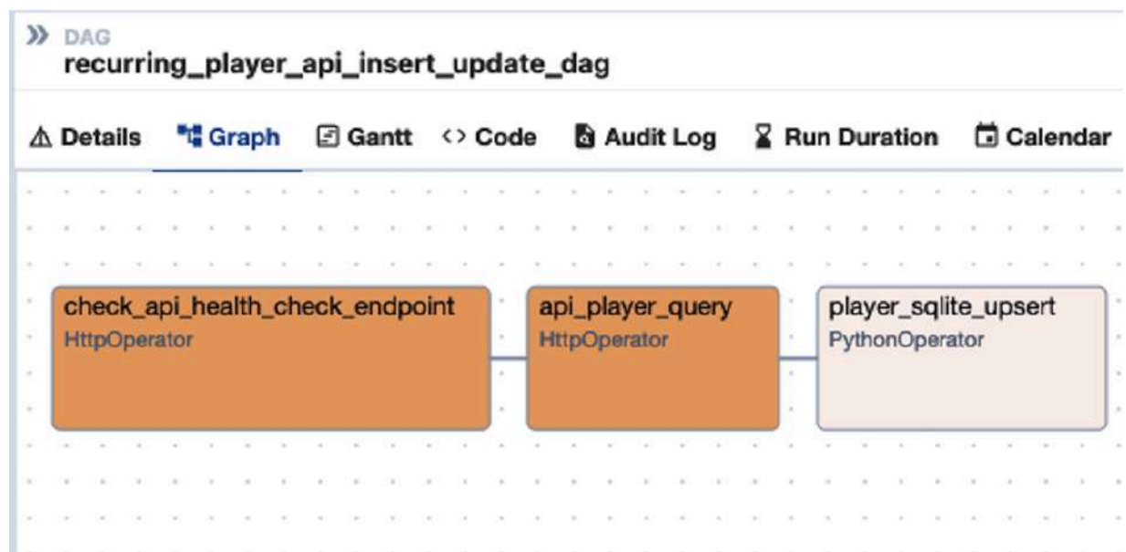
Figure 10-9. Graph view of the first DAG
