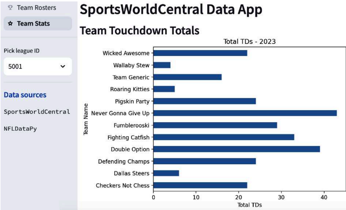
Figure 11-6. Team Stats page
