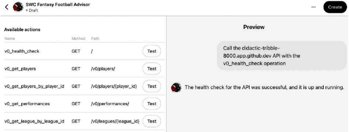
Figure 15-13. GPT calling health check endpoint
