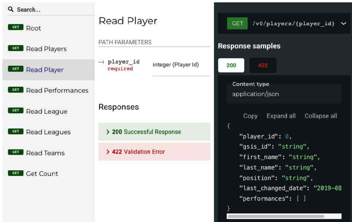
Figure 5-12. Redoc documentation page
