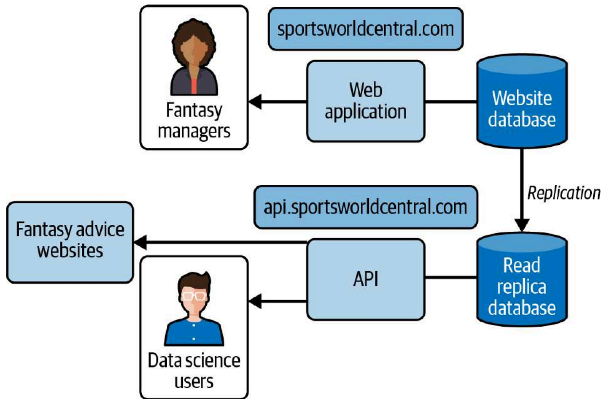
Figure 2-2. Future state application architecture
