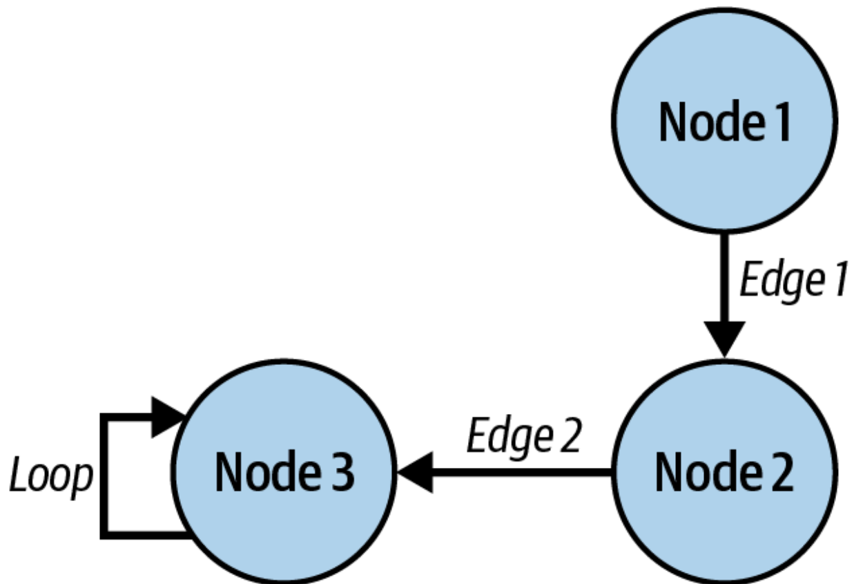
Figure 14-2. Directed cyclic graph
