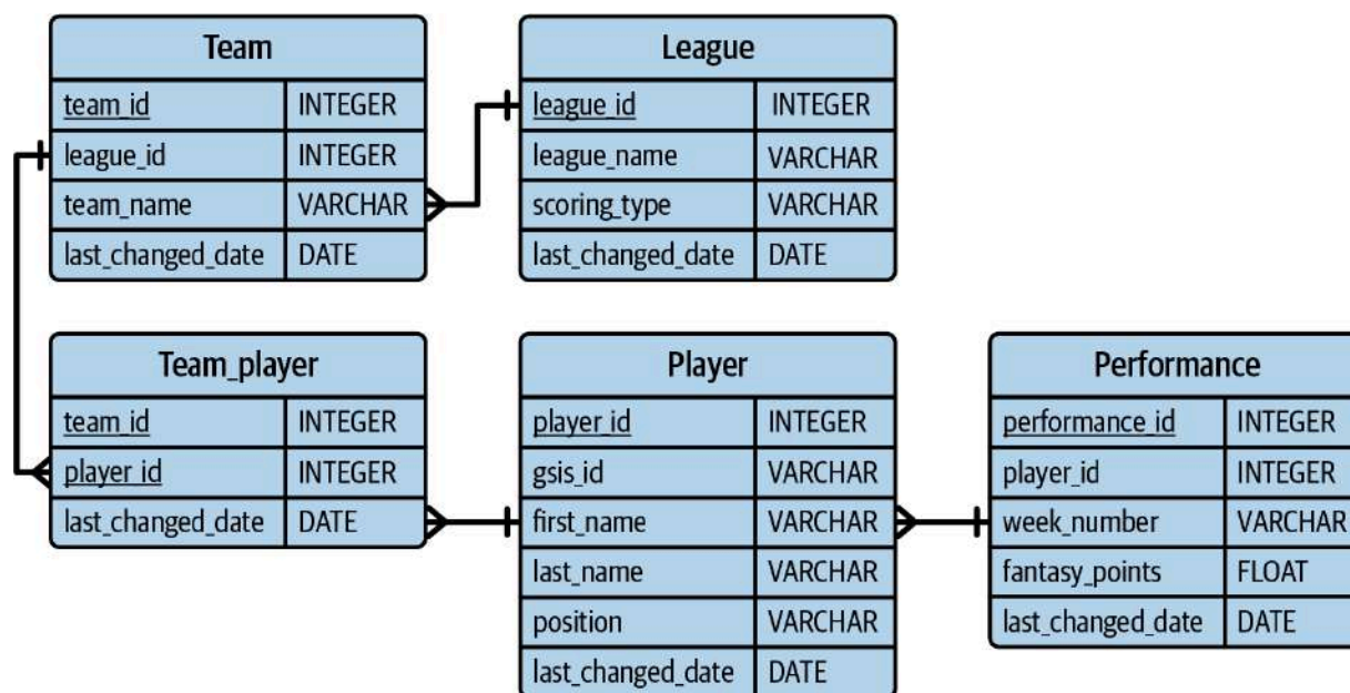
Figure 3-2. Database table structure
