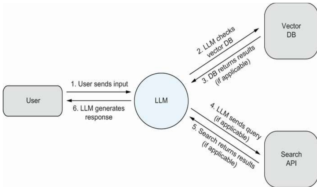
Figure 8.4 A schematic diagram for an LLM accessing data stored in a vector database and retrieving search results from the web
