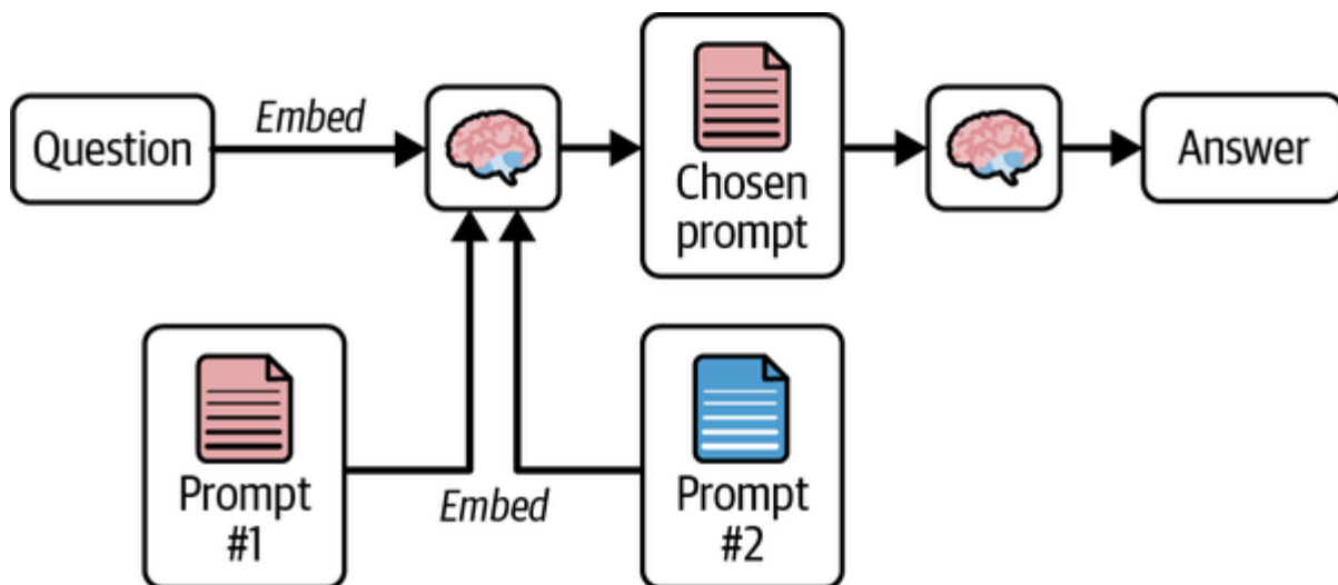
Figure 3-9. Semantic routing to improve the accuracy of retrieved documents
