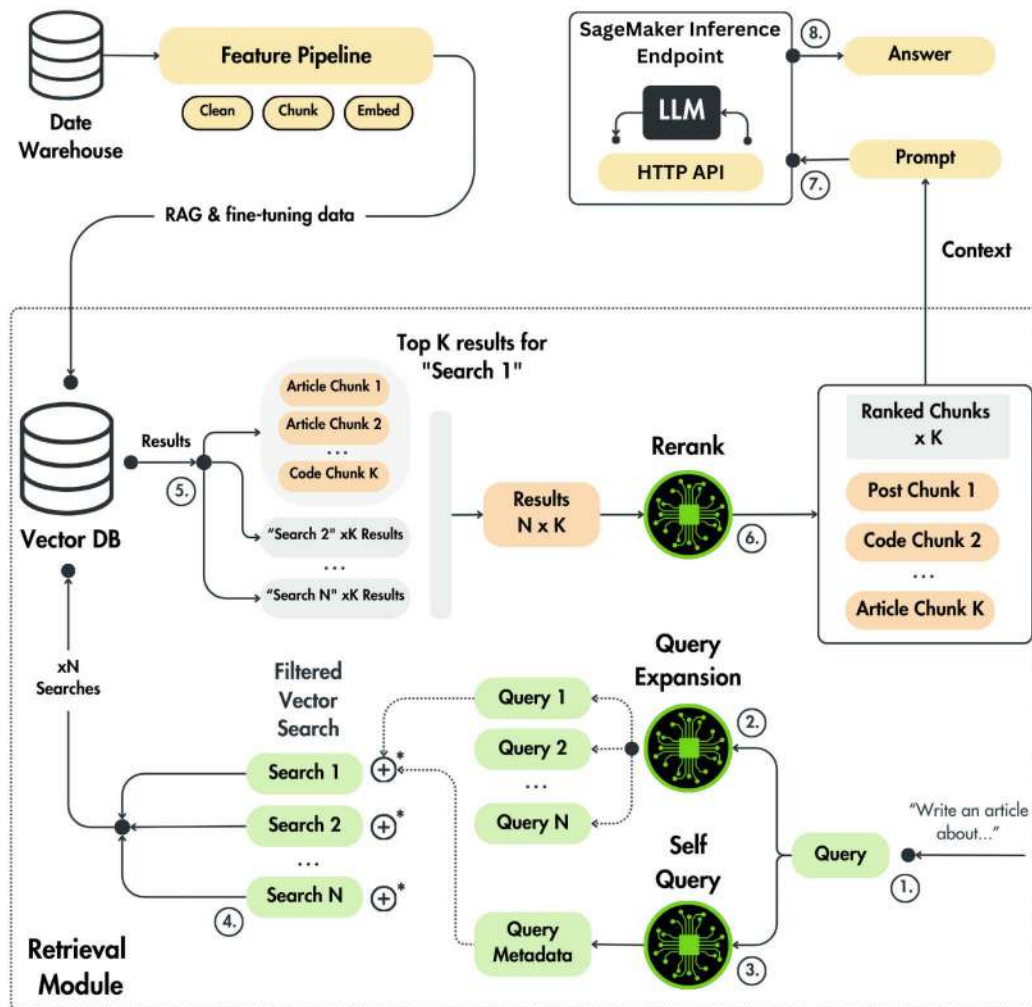
Figure 9.1: RAG inference pipeline architecture
