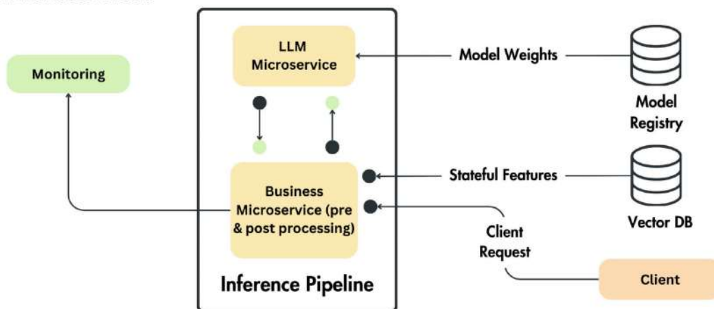
Figure 10.2: Monolithic versus microservices architecture in model serving
