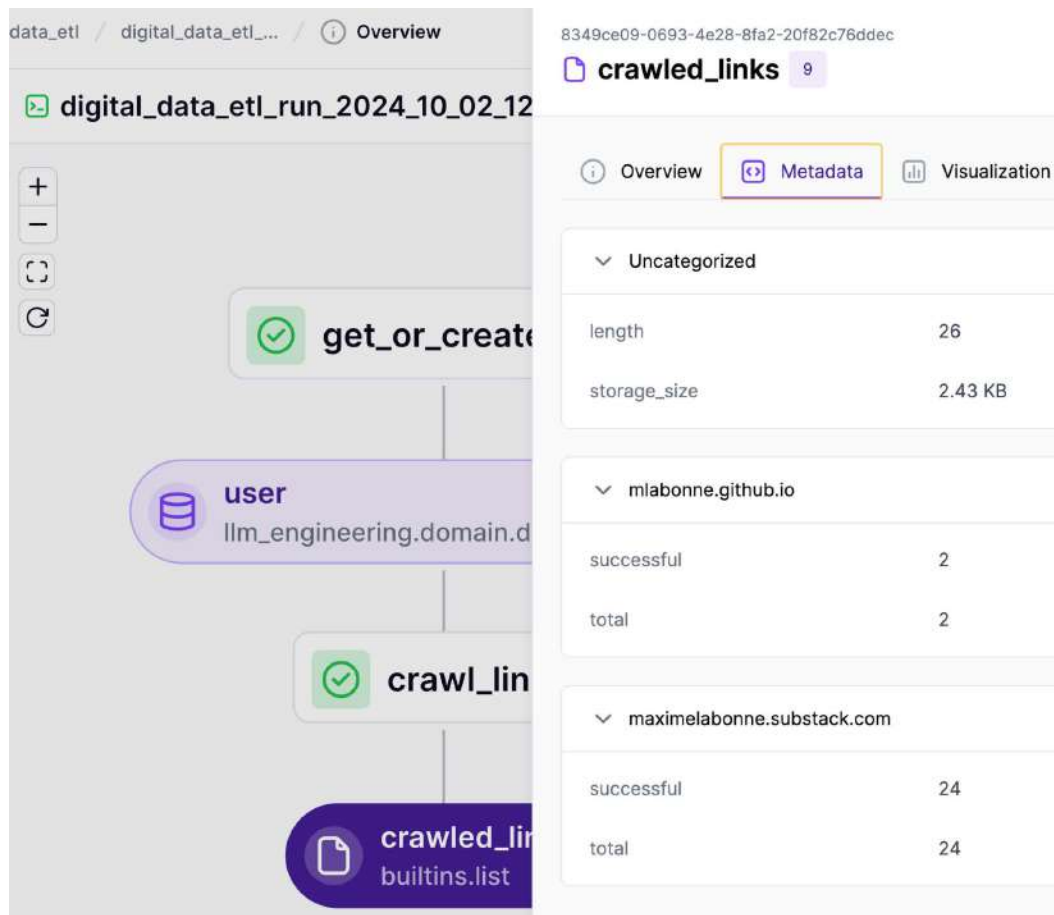
Figure 3.6: Example of the crawled_links output artifact after running the data collection pipeline using Maxime's configuration file
