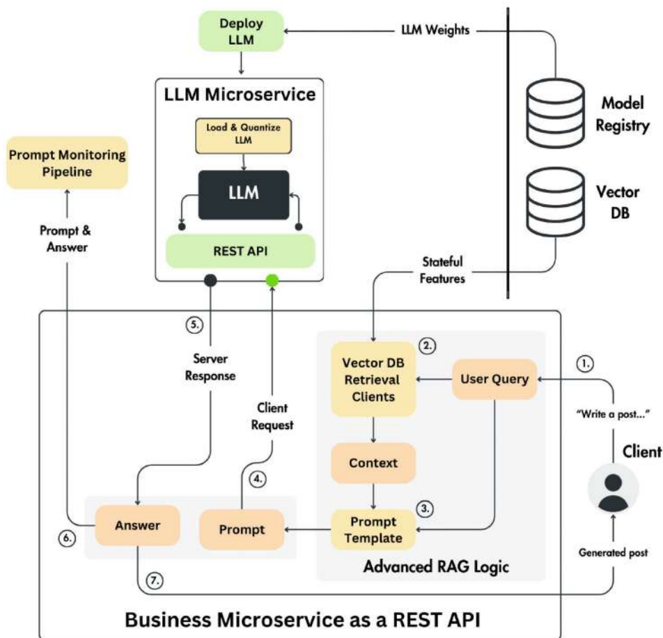
Figure 11.21: Inference pipeline serving architecture
