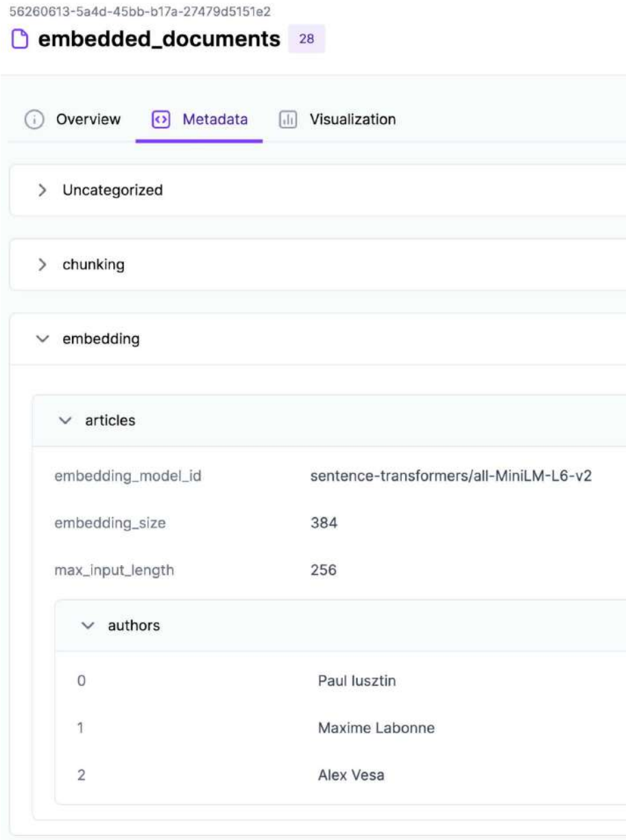
Figure 4.15: Metadata of the embedding and chunking ZenML step, detailing the embedding dropdown
