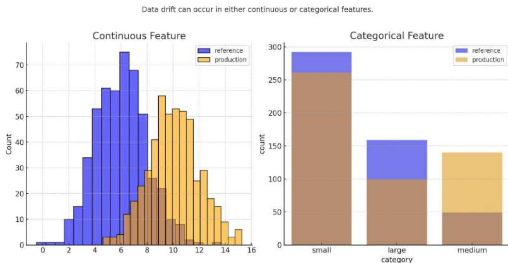
Figure A.3: Data drift examples
