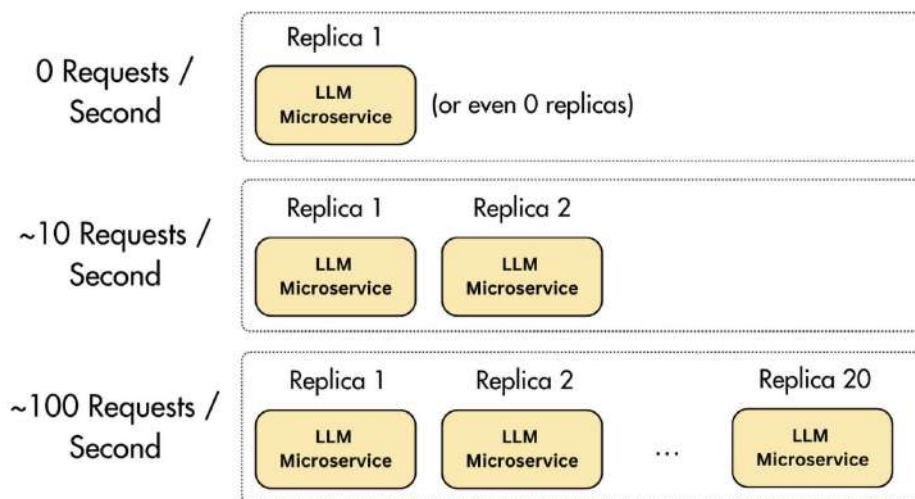
Figure 10.8: Autoscaling possible use cases
