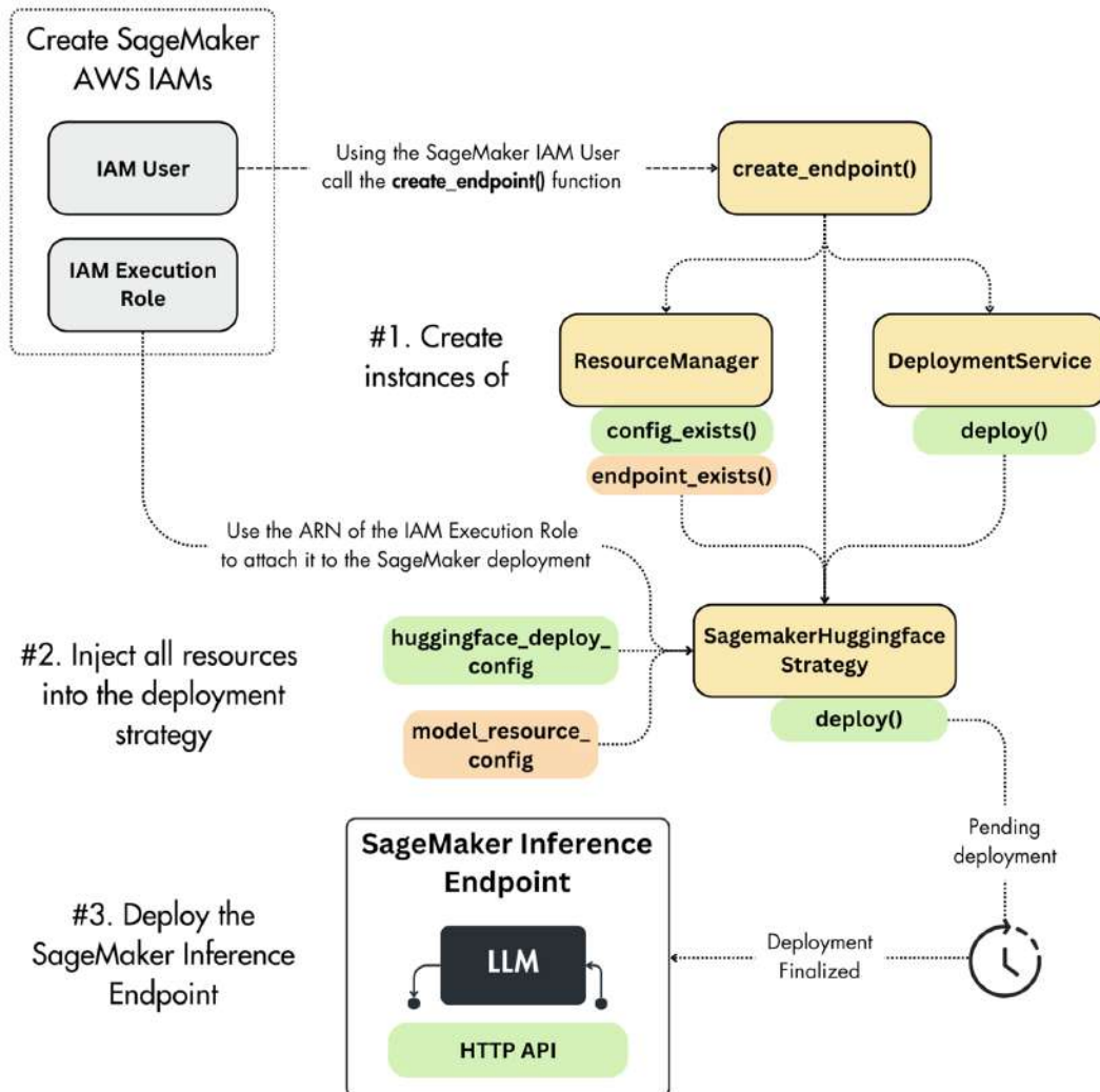
Figure 10.5: AWS SageMaker deployment steps
