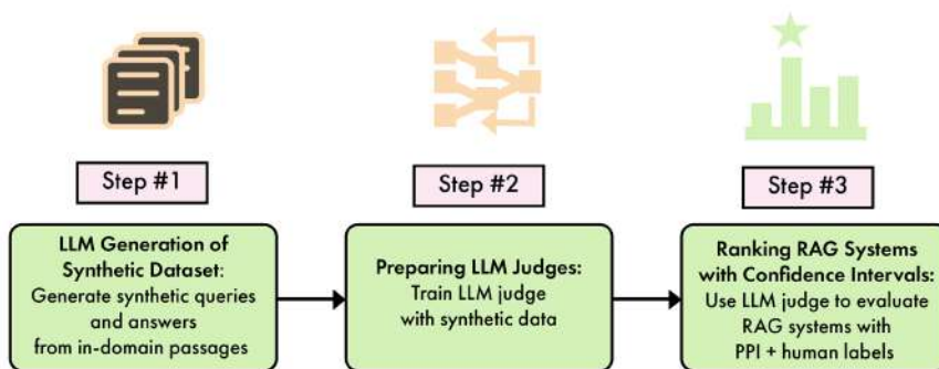
Figure 7.2: Overview of the ARES evaluation framework
