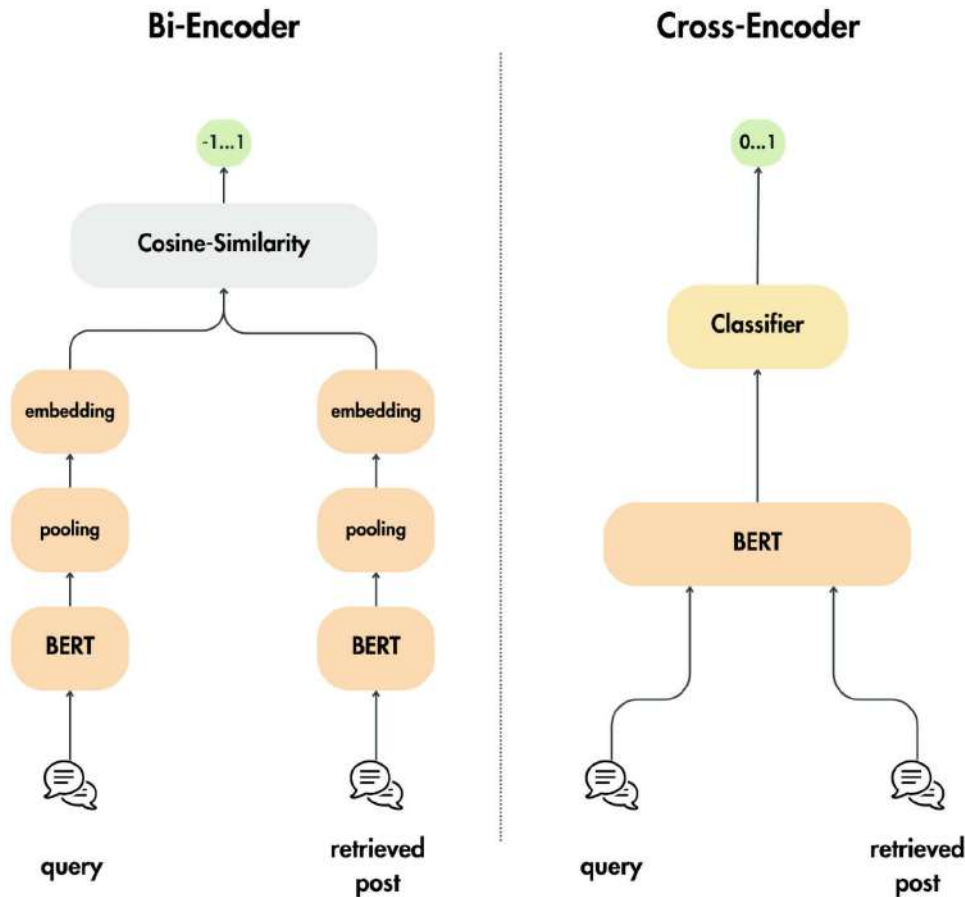
Figure 4.7: Bi-encoder (the standard embedding model) versus cross-encoder
