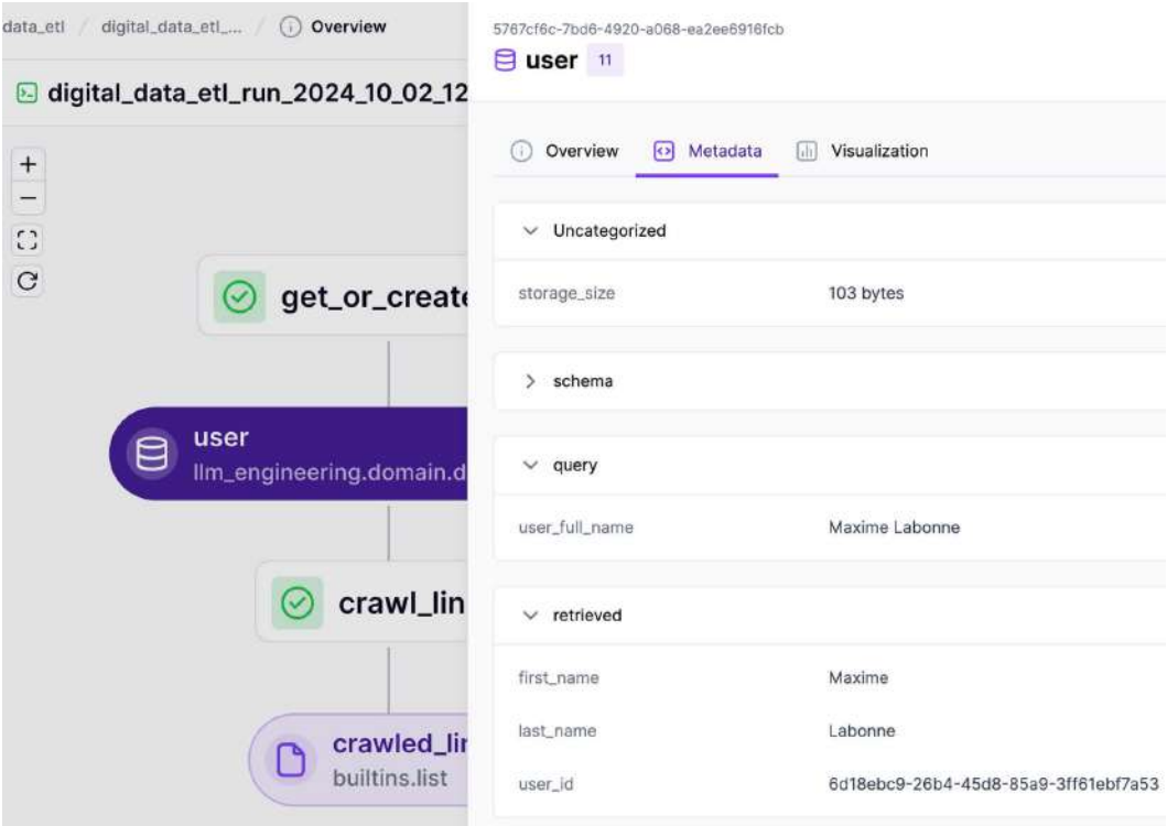
Figure 3.5: Example of the user output artifact after running the data collection pipeline using Maxime’s configuration file
