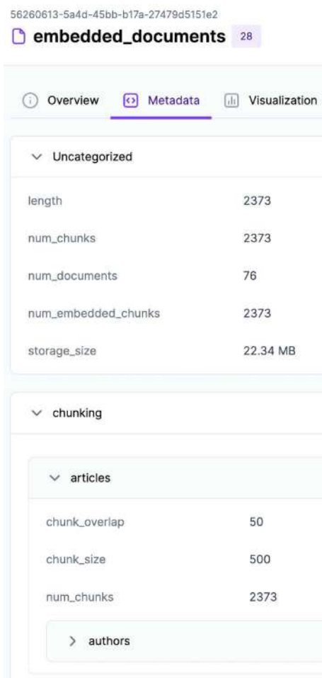
Figure 4.14: Metadata of the embedding and chunking ZenML step, detailing the uncategorized and chunking dropdowns
