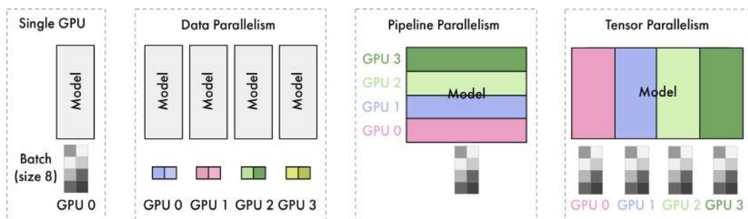
Figure 8.8 – Illustration of the different model parallelism techniques
