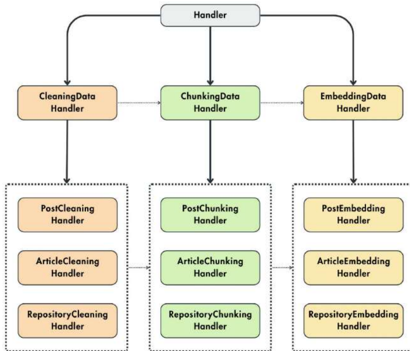
Figure 4.17: Handler class hierarchy and their interaction
