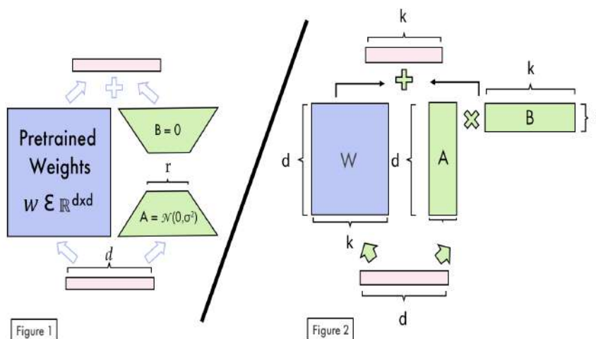
Figure 5.10 – LoRA adds the two trainable matrices A and B and keeps the pre-trained weights W frozen
