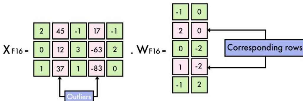
Figure 8.11 – Example of outliers in a weight matrix
