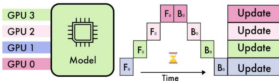
Figure 8.5 – Illustration of pipeline parallelism with four GPUs
