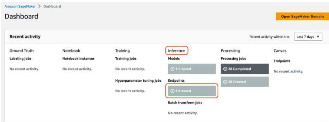
Figure 10.6: AWS SageMaker Inference endpoints example
