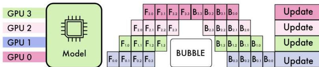
Figure 8.6 – Illustration of pipeline parallelism with micro-batching.
