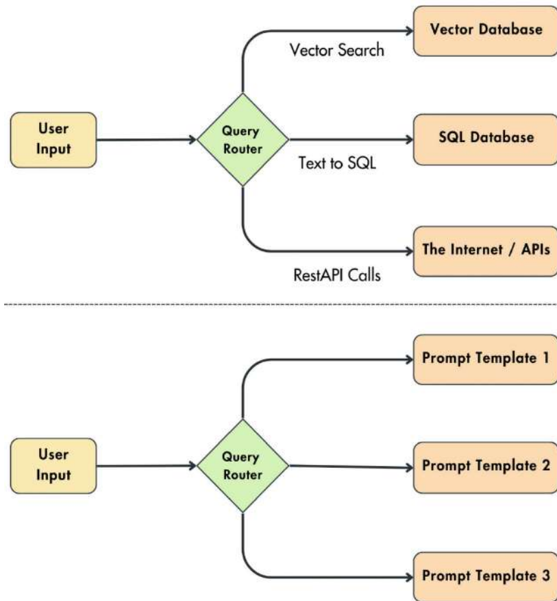
Figure 4.6: Query routing
