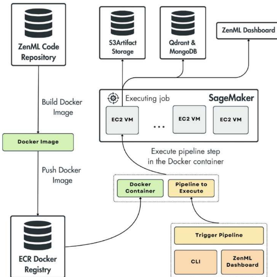
Figure 11.5: Infrastructure flow
