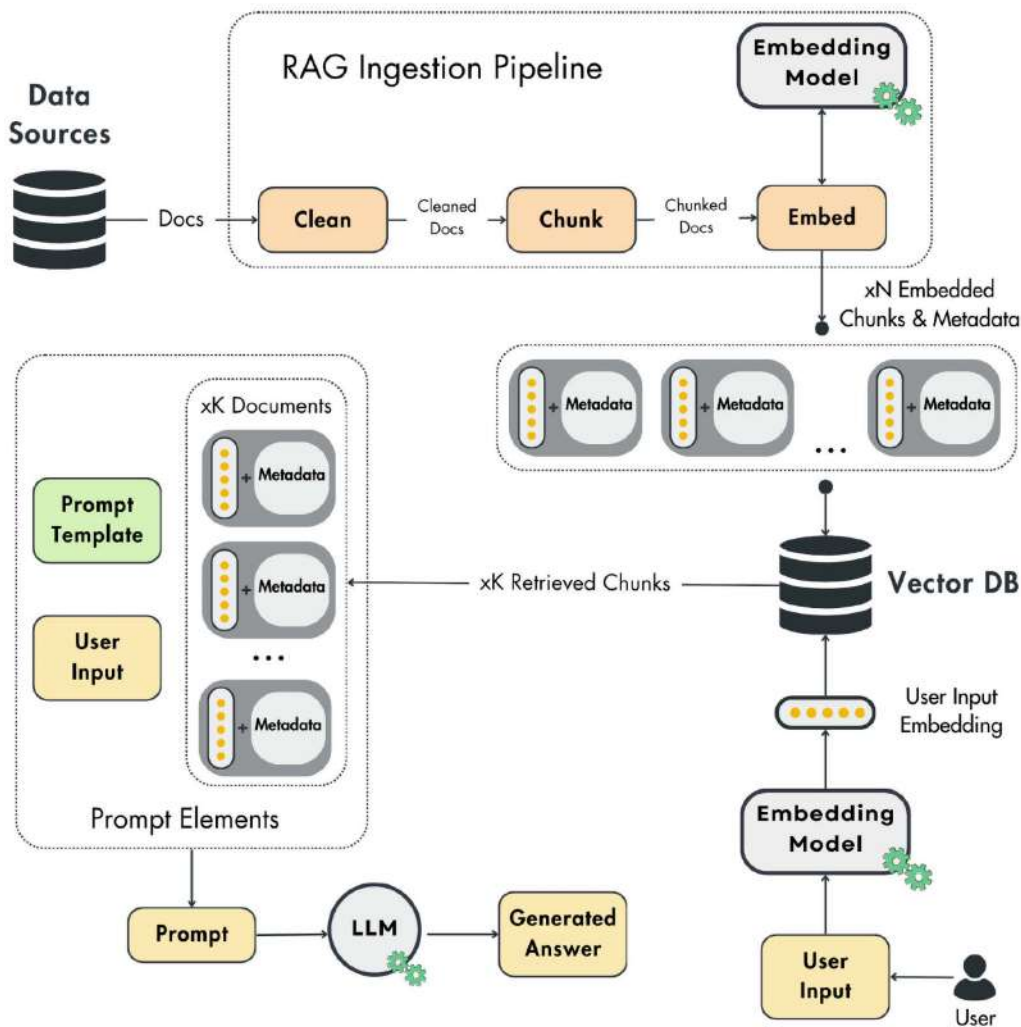
Figure 4.1: Vanilla RAG architecture
