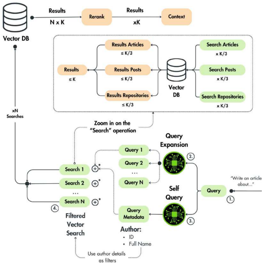
Figure 9.2: Search logic of the RAG retrieval module
