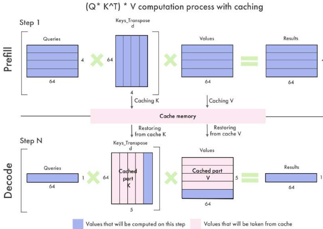
Figure 8.2 – Illustration of the KV cache
