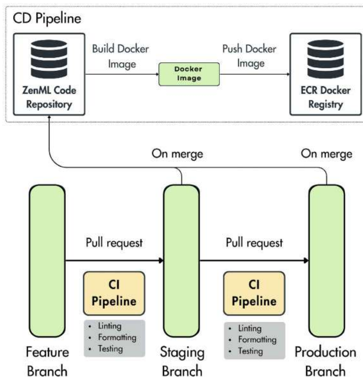
Figure 11.14: CI/CD pipelines flow
