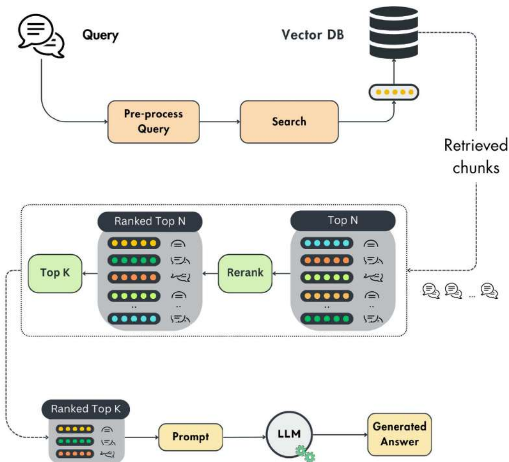
Figure 4.8: The re-ranking algorithm
