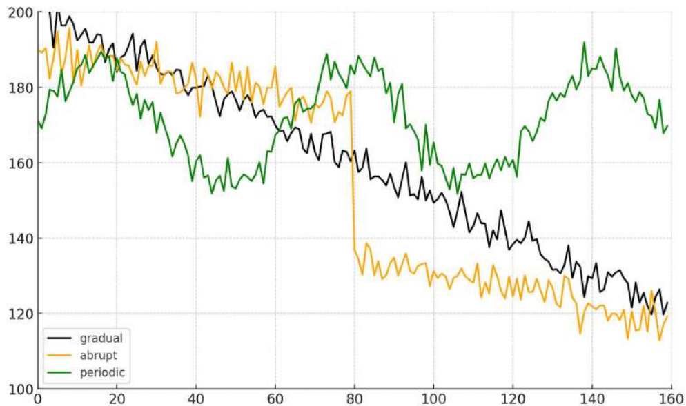
Figure A.4: Concept drift examples
