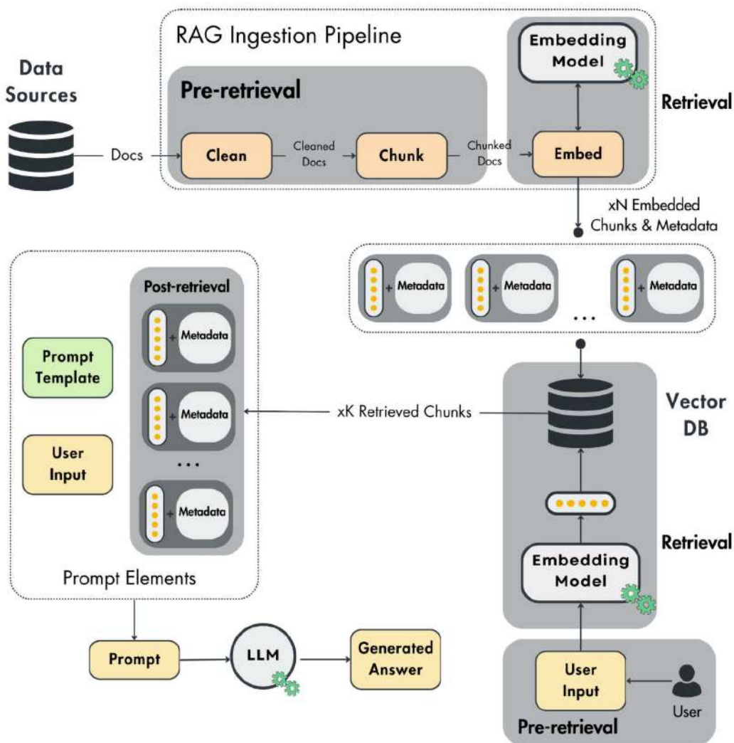
Figure 4.5: The three stages of advanced RAG
