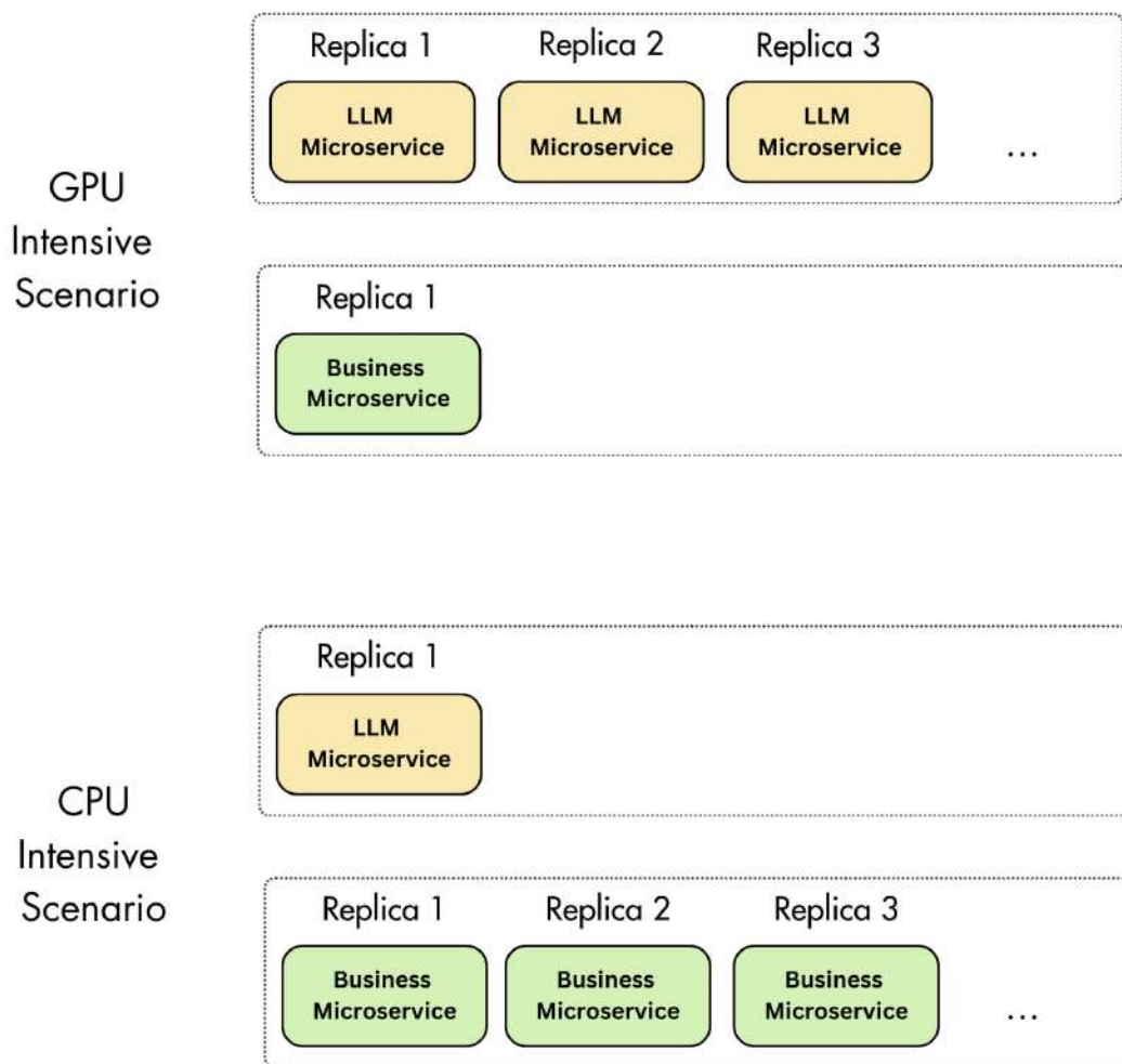
Figure 10.3: Scaling microservices independently based on compute requirements
