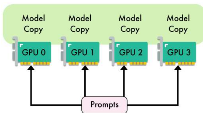
Figure 8.4 – Illustration of data parallelism with four GPUs
