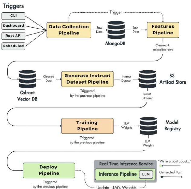
Figure 11.19: CT pipeline
