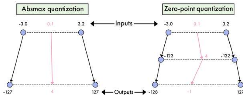
Figure 8.10 – Quantization of 0.1 in a [-3.0, 3.2] range with absmax quantization and zero-point quantization
