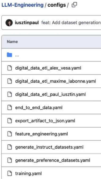
Figure 2.10: ZenML pipeline configs
