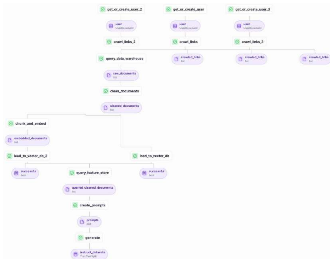
Figure 11.20: End-to-end pipeline illustrated in ZenML's dashboard
