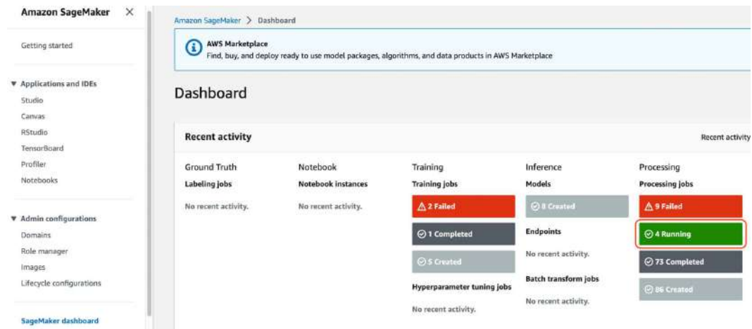
Figure 11.12: SageMaker dashboard
