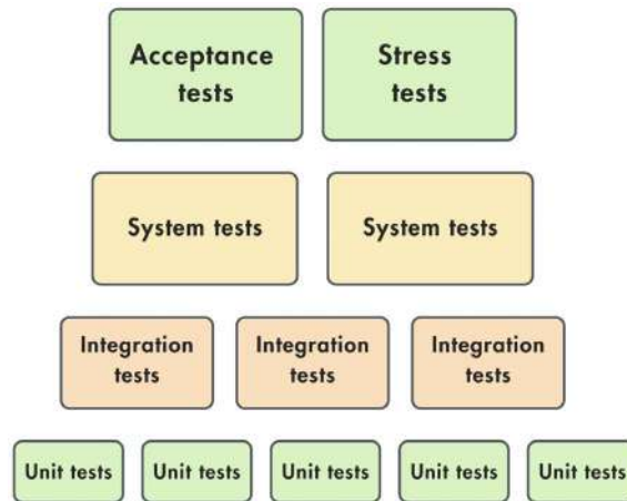
Figure A.2: Test types
