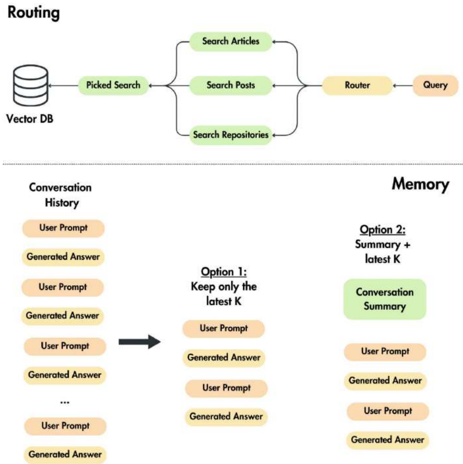
Figure 9.4: Routing and memory examples
