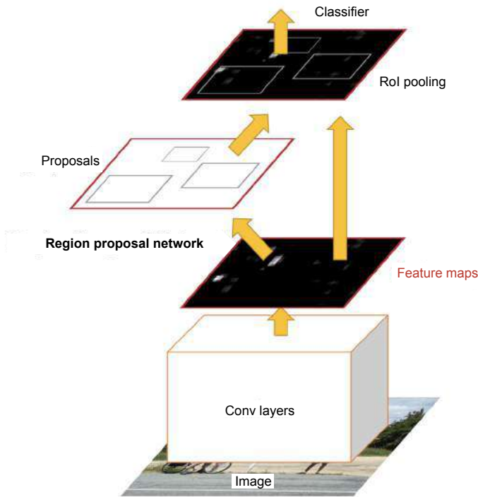
Figure 11.12 Faster R-CNN architecture. (Source: “Faster R-CNN: Toward real-time object detection with region proposal networks”; https://arxiv.org/abs/1506.01497 .)
