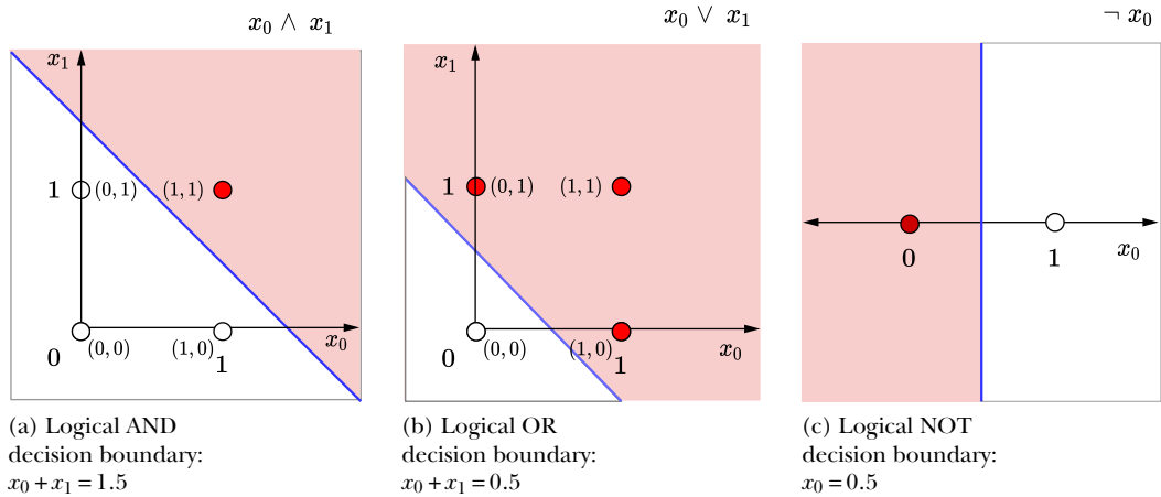
Figure 7.11 Geometrical views for the perceptrons in figure 7.10. Each dot represents an input point (a \begin{bmatrix} x_0 & x_1 \end{bmatrix} vector). The shaded dots map to an output value of 1, and the unshaded dots map to an output value of 0. The thick line indicates the decision boundary.
