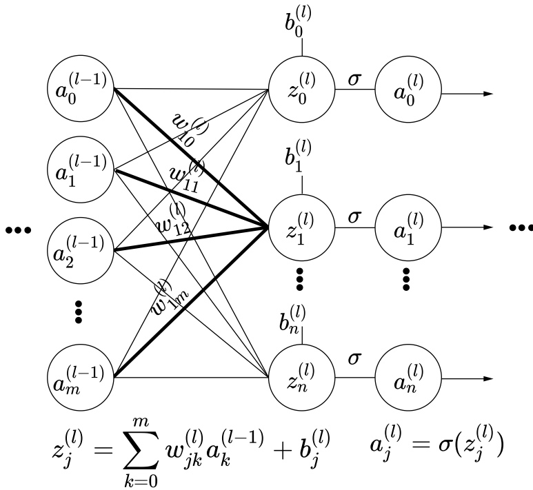
Figure 8.6 Linear layer outputting layer l from layer (l-1) . The weights belonging to row 1 of the weight matrix (coming from all the input neurons, layer (l-1) , which sum together to form output neuron 1) are shown in bold.
