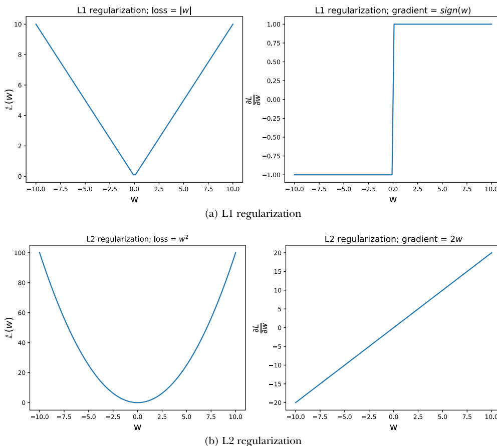
Figure 9.12 L1 and L2 regularization
