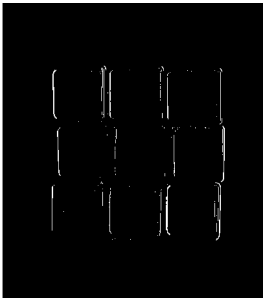
(b) Vertical edges detected by applying 2D convolution \begin{bmatrix} -0.25 & 0.25 \\ -0.25 & 0.25 \end{bmatrix} to figure 10.11a
