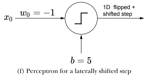
Figure 7.15 Generating a 1D tower with perceptrons. (Figure continued on next page)
