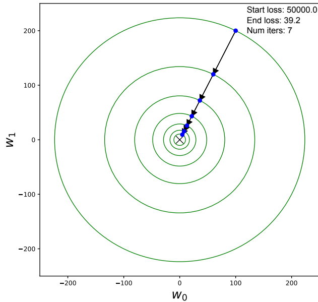
(a) A trajectory through constant loss contours for gradient descent without momentum
