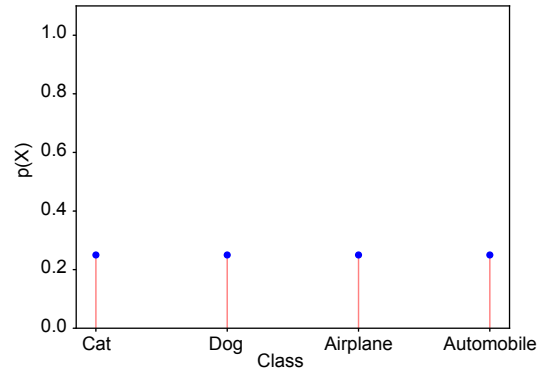
(c) Bad prediction: probabilities dissimilar to ground truth. Cross-entropy loss = 1.38.
