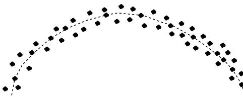
Figure 14.4 A 2D data distribution with a curved underlying pattern. It is impossible to find a straight line or vector such that all points are near it. PCA will not do well.
