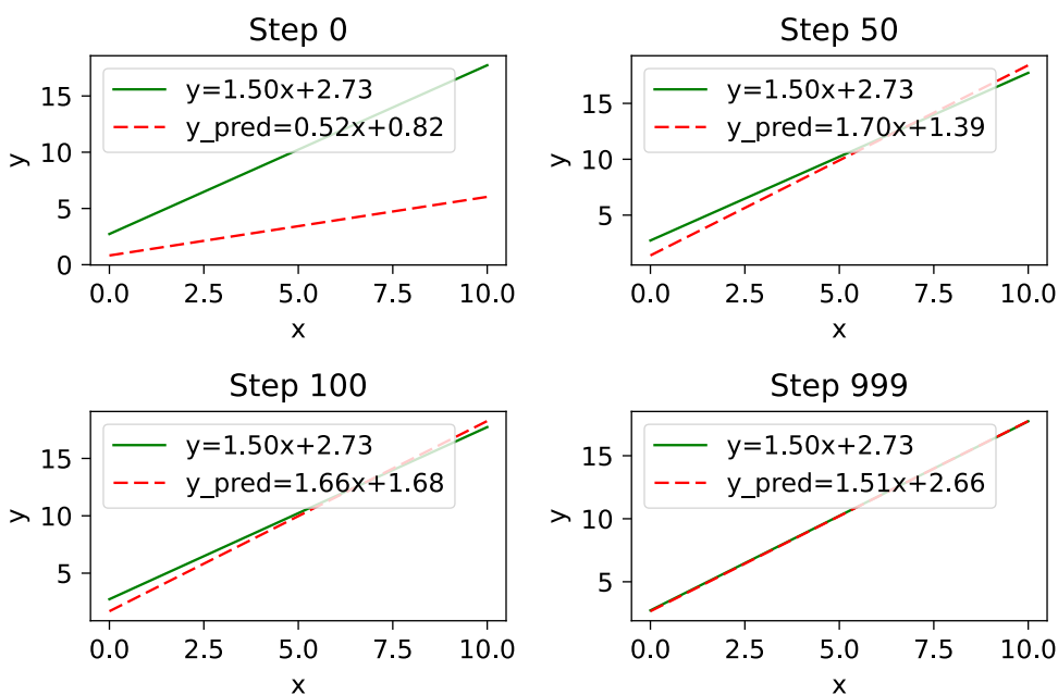
Figure 3.11 Linear approximation of linear data. By step 1,000, the model has more or less converged to the true underlying function.
