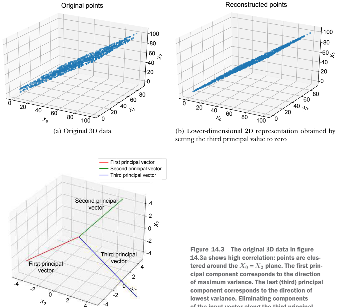
(c) The principal vectors of the original data. The third principal vector is normal to X_0 = X_2 plane; the other two are in-plane.
