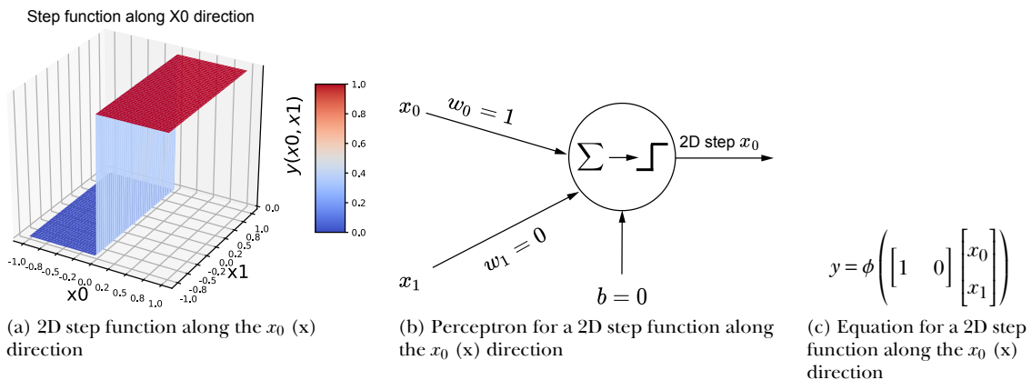
Figure 7.16 Generating 2D steps and waves with perceptrons. (Figure continued on next page)
