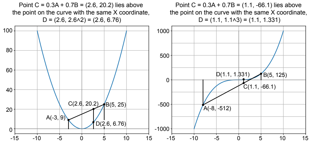
Figure 3.16 Convex and nonconvex curves. A and B are a pair of points on the curve. C = 0.3A + 0.7B is a weighted average of the coordinates of A and B , with weights summing to 1. C lies on the line joining A and B . The left-hand curve is convex: C lies above the corresponding curve point D . The right-hand curve is nonconvex: C lies below the corresponding curve point D .
