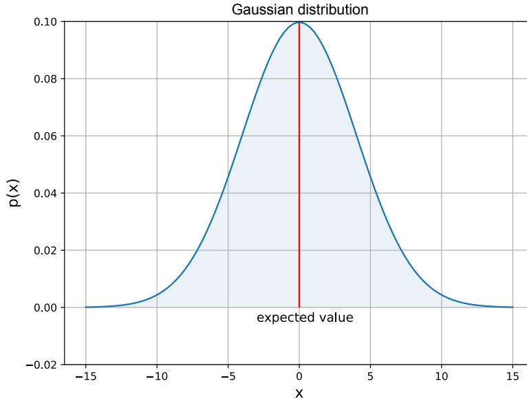
Figure 5.9 Univariate (single-variable) normal (Gaussian) random probability density function, \mu = 0 and \sigma = 4 . The solid line in the middle indicates the expected value.
