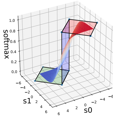
(b) Softmax: differential approximation of the step function
