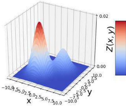
(c) \pi_1 = 0.7, \pi_2 = 0.3
