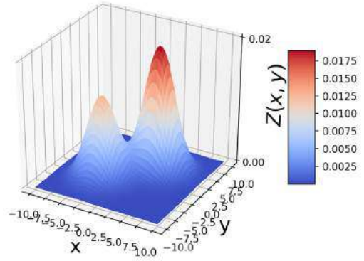
(b) \pi_1 = 0.4, \pi_2 = 0.6
