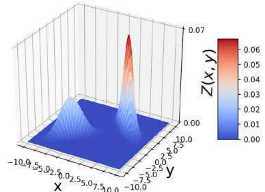
Figure 6.9 Two-dimensional GMMs with circular bases, (\Sigma_1 = \Sigma_2 = \begin{bmatrix} 5 & 0 \\ 0 & 5 \end{bmatrix}) , \vec{\mu}_1 = \begin{bmatrix} -3 \\ -3 \end{bmatrix} , \vec{\mu}_2 = \begin{bmatrix} 3 \\ 3 \end{bmatrix} .
