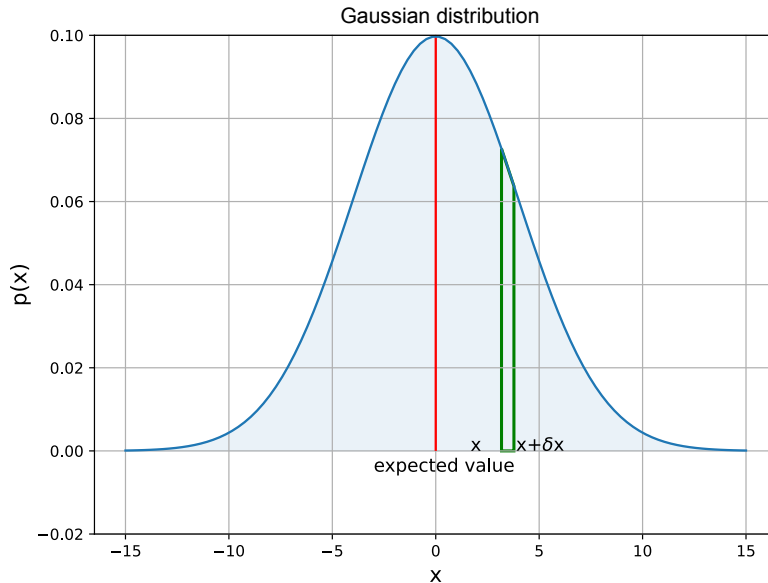
Figure 5.7 Univariate Gaussian random probability density function, \mu = 0 and \sigma = 4 . The bell-shaped curve is highest at the center and decreases more and more as we move away from the center, approaching zero asymptotically. The value x = 0 has the highest probability, corresponding to the center of the probability density function. Note that the curve is symmetric. Thus, for instance, the probability of a random sample being in the vicinity of -5 is the same as that of 5 ( 0.04 ): that is, p(-5) = p(5) = 0.04 . An interactive visualization (where you can change the parameters and observe how the graph changes as a result) can be found at http://mng.bz/NYJX .
