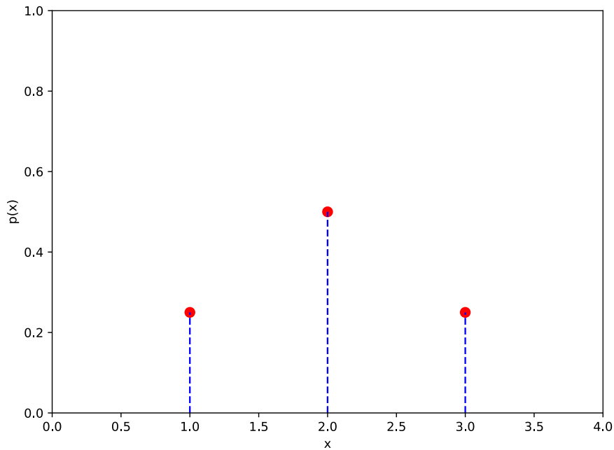
Figure 5.2 Probability distribution graph for the weights of adults in Statsville, corresponding to table 5.2. Event E_1 \equiv X = 1 \Rightarrow a weight in the range S_1 , Event E_2 \equiv X = 2 \Rightarrow a weight in the range S_2 , and Event E_3 \equiv x = 3 \Rightarrow a weight in the range S_3 .
