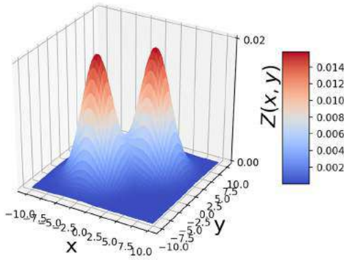
(a) \pi_1 = 0.5, \pi_2 = 0.5
