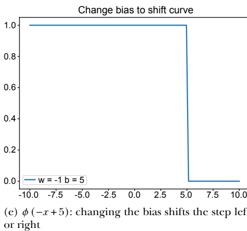
Figure 7.15 Generating a 1D tower with perceptrons. (Figure continued on next page)
