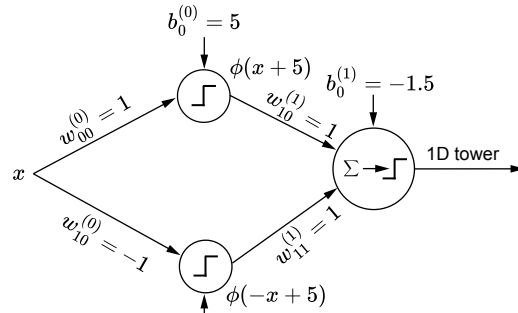
(h) MLP for a 1D tower
