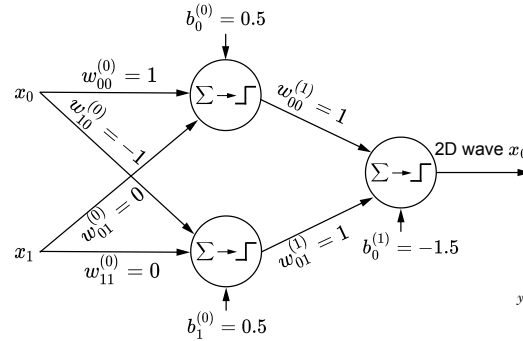
(h) MLP for a 2D wave along the x_0 (x) direction
