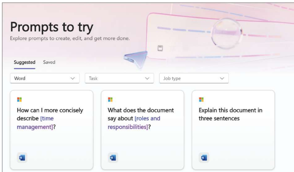
Figure 3.2: Viewing prompts
