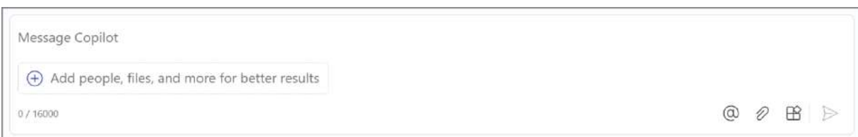
Figure 3.1: Copilot Lab
