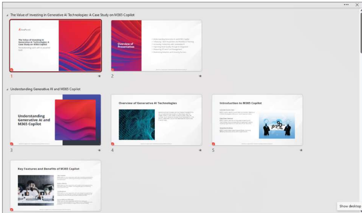
Figure 16.8: Copilot-generated slides
