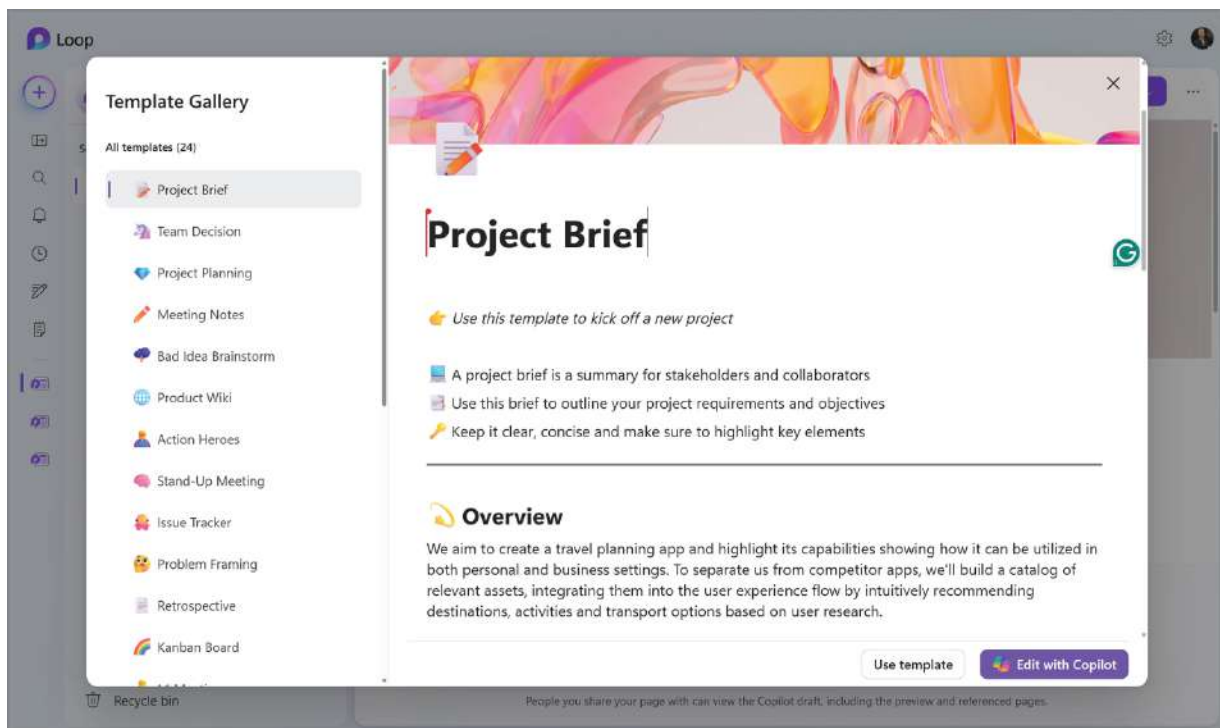
Figure 11.4: Template Gallery
