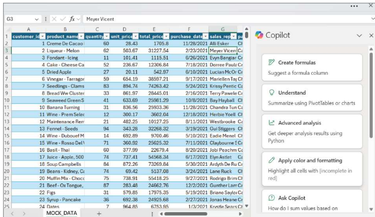
Figure 16.9: The Advanced analysis prompt
