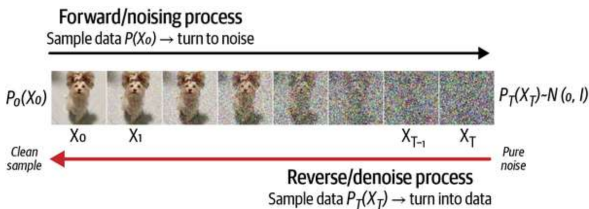
Figure 7-1. Diffusion schematics
