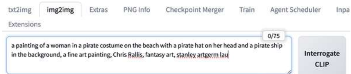
Figure 9-14. Interrogate CLIP
