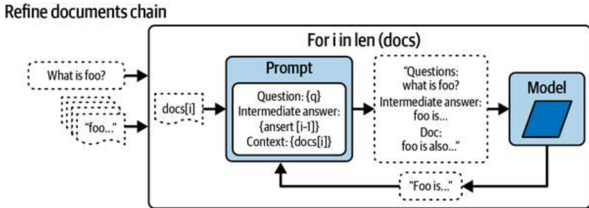
Figure 4-6. Refine documents chain
