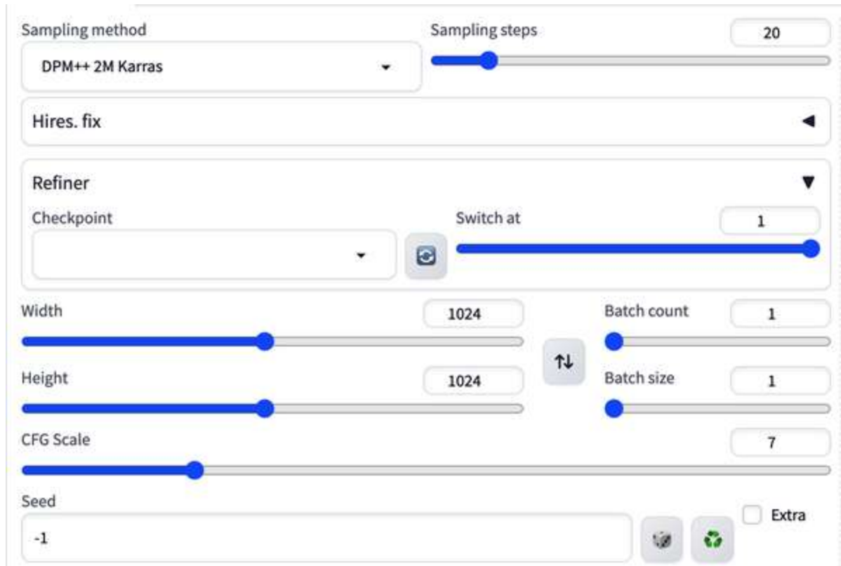
Figure 9-5. Standard settings for SDXL
