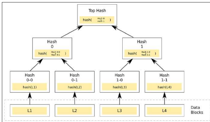
FIGURE 4-1: A Merkle tree.
