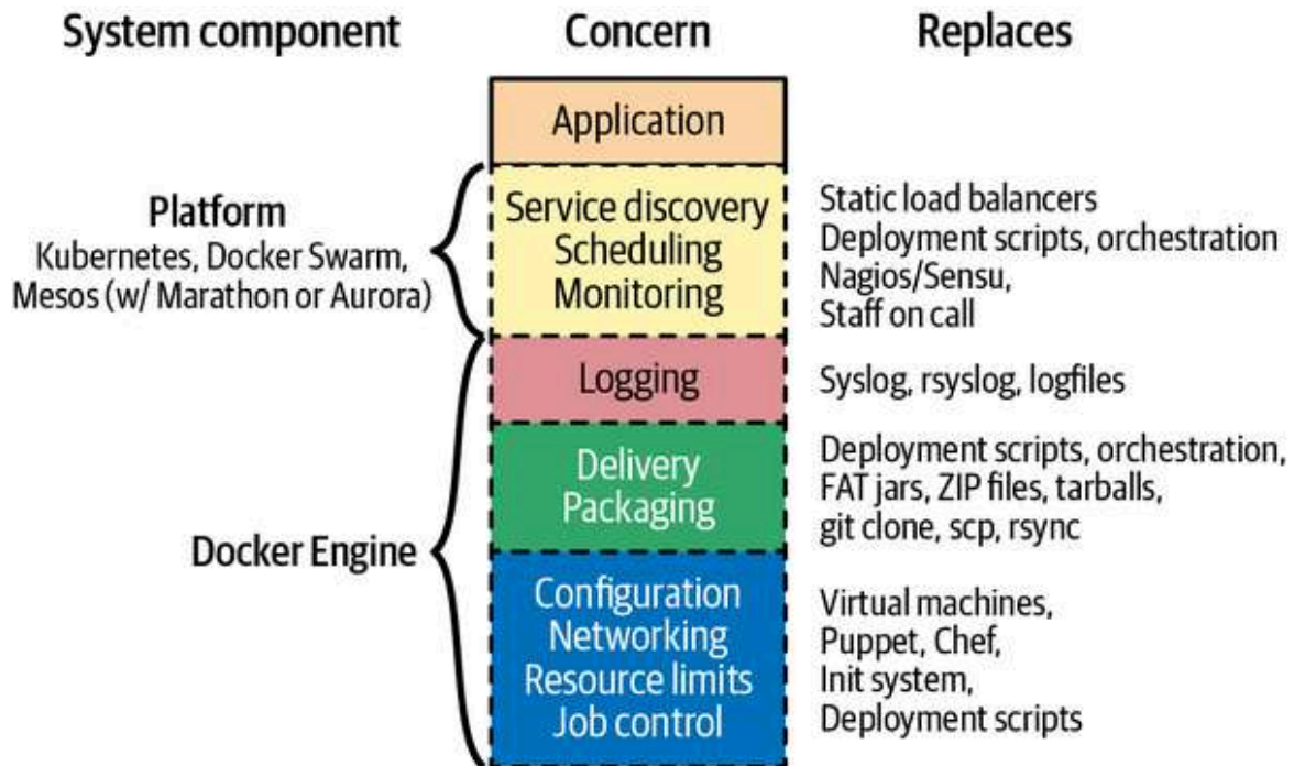
Figure 9-1. Docker's role in a production system
