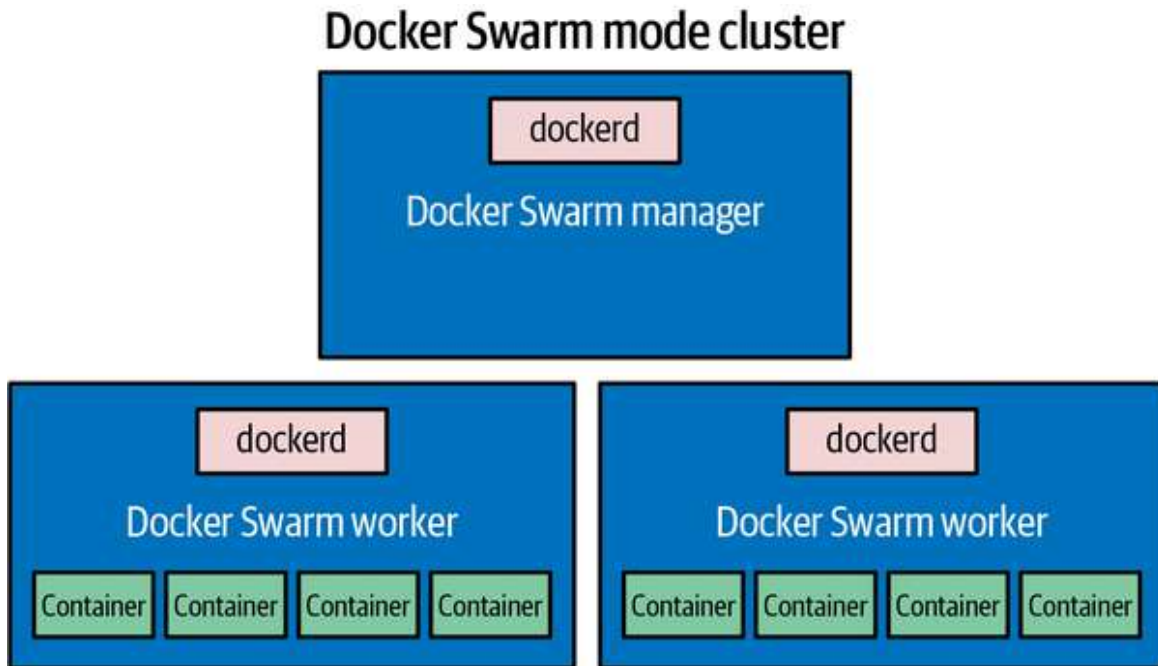
Figure 10-1. Simple Docker Swarm mode cluster
