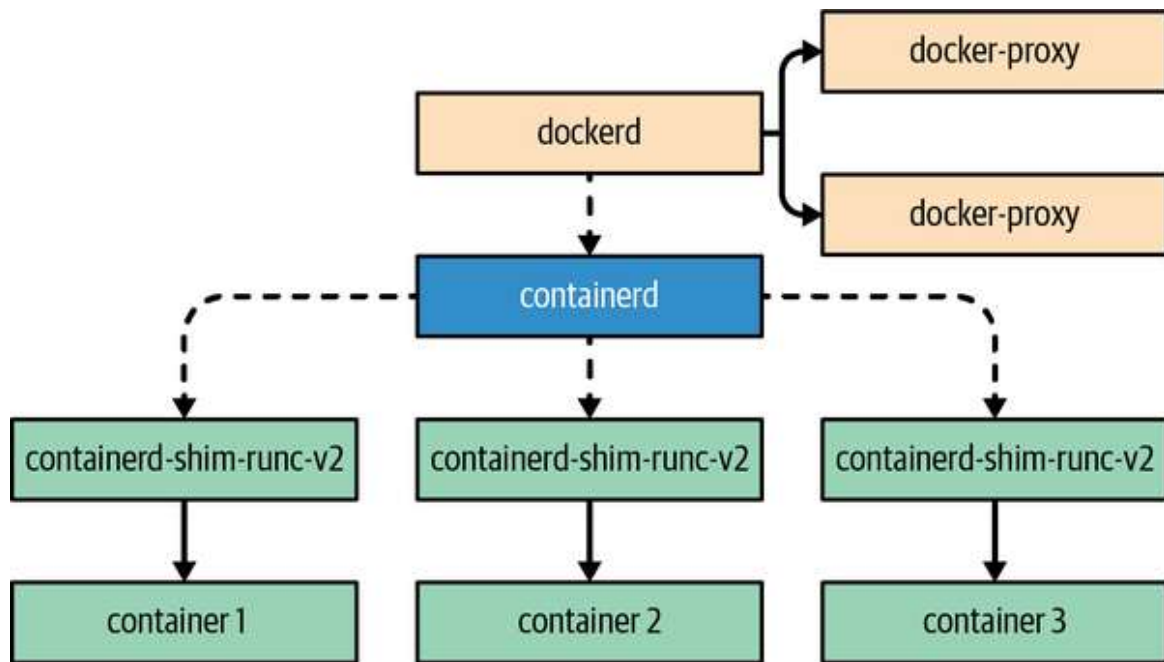
Figure 11-2. Structure of Docker
