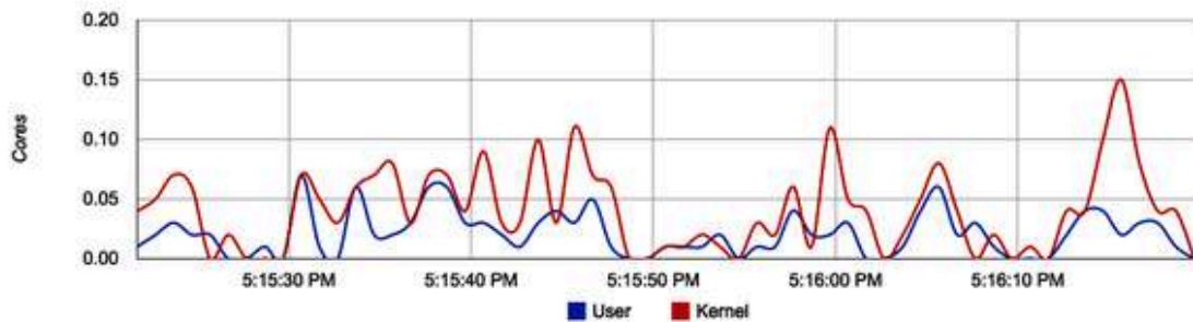
Figure 6-1. cAdvisor CPU graphs (example)
