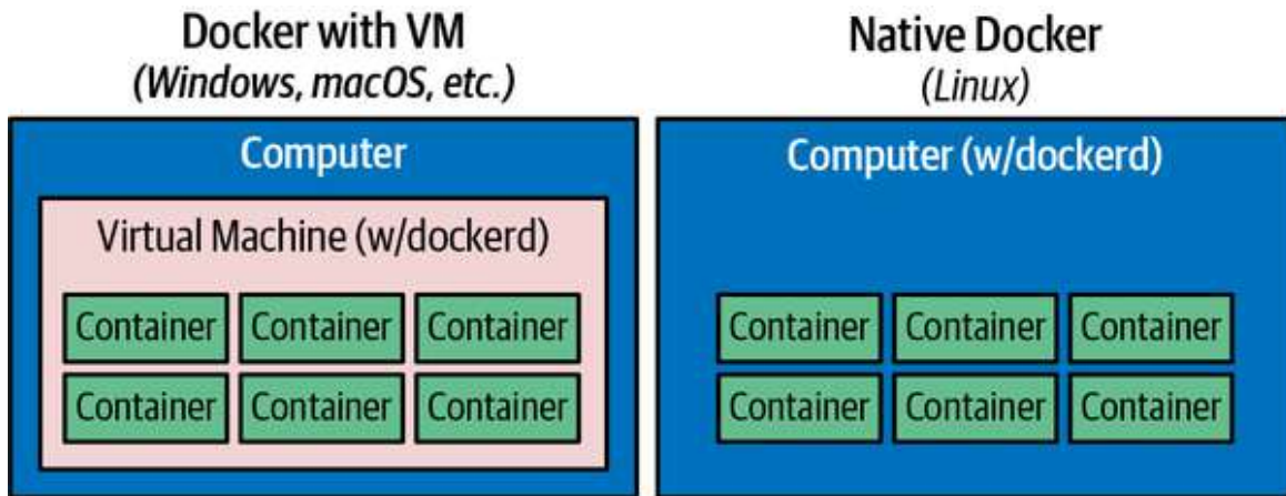
Figure 2-5. Typical Docker installations
