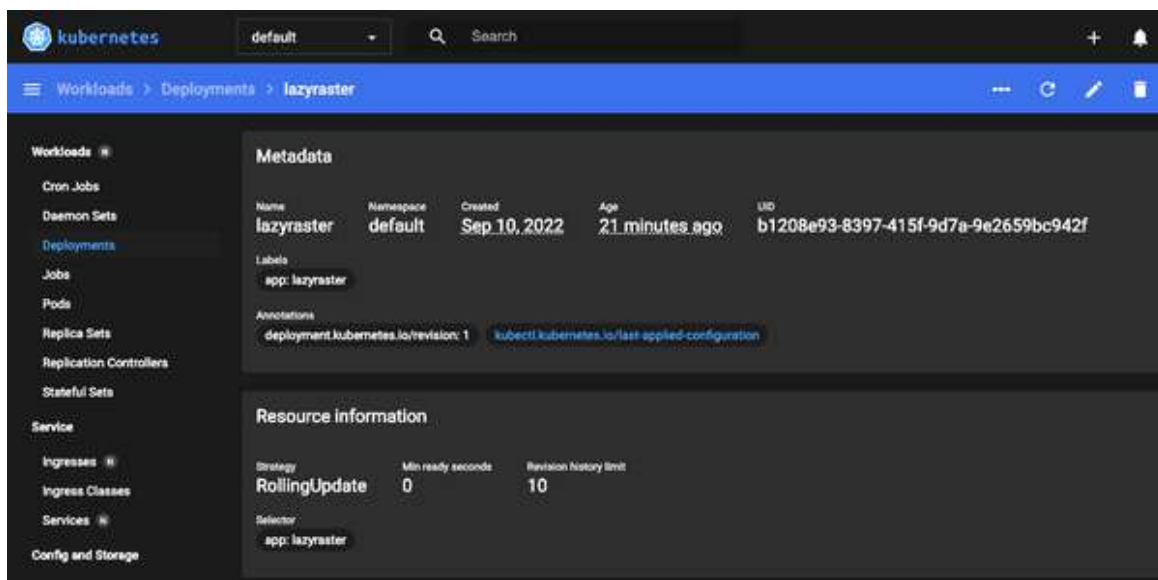
Figure 10-3. lazyraster service dashboard (example)
