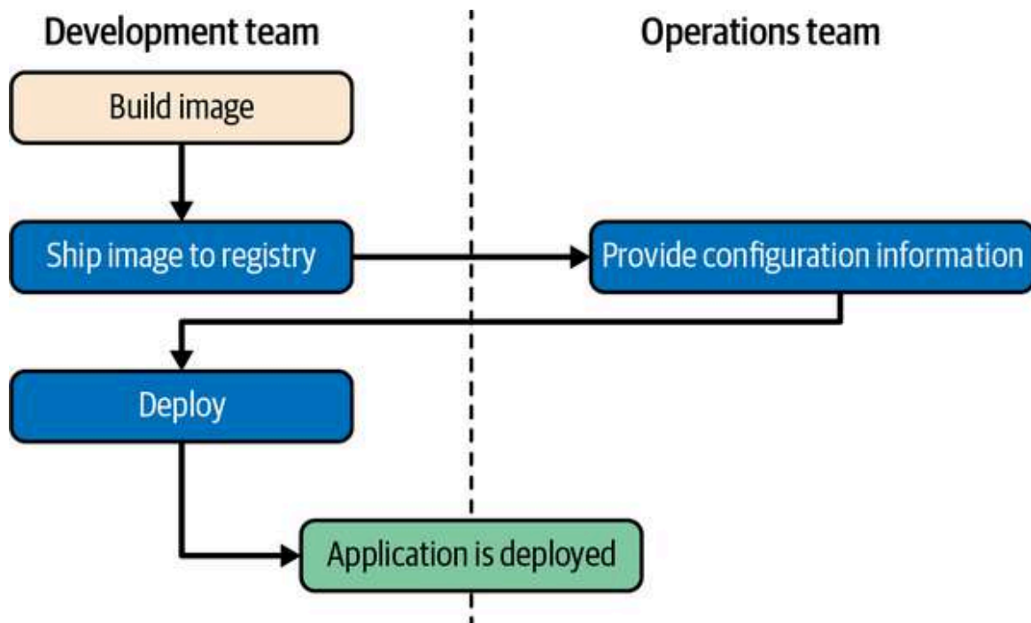
Figure 2-2. A Docker deployment workflow
