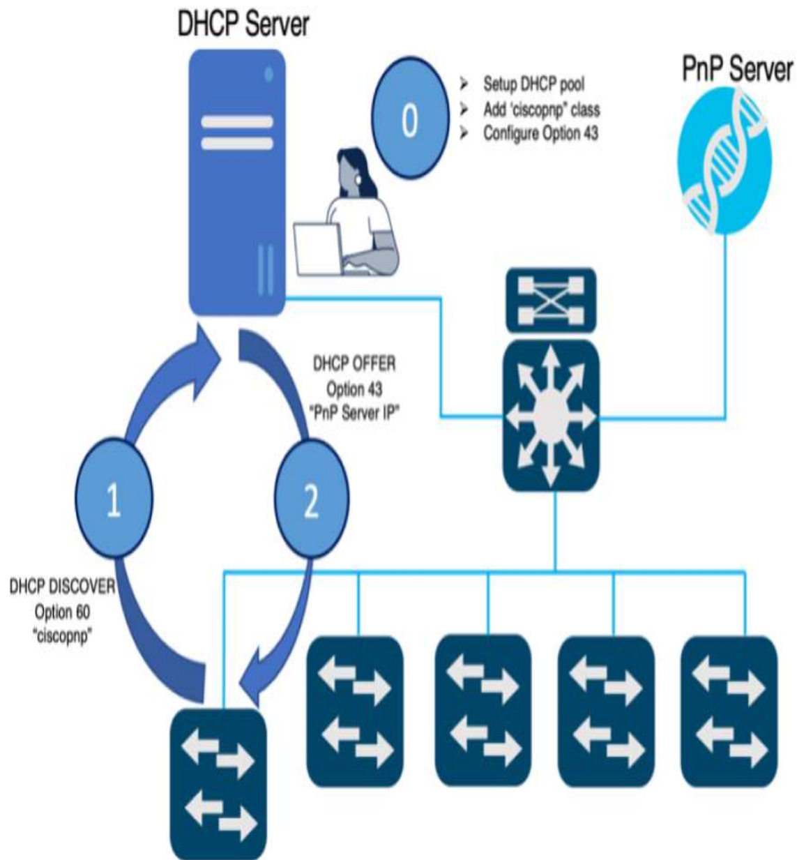
Figure 7-9 DHCP Option 60 Flow in PnP
