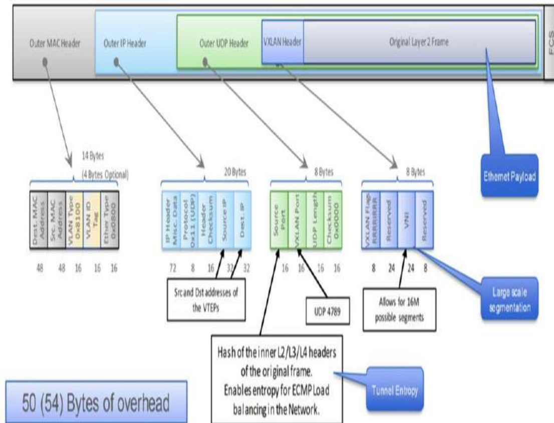
Figure 22-7 VXLAN-GPO
