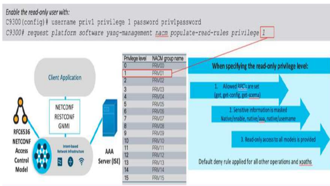
Figure 23-7 NAMC Mappings for User Privilege
