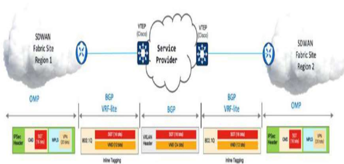
Figure 22-6 Inter Region Policy Propagation
