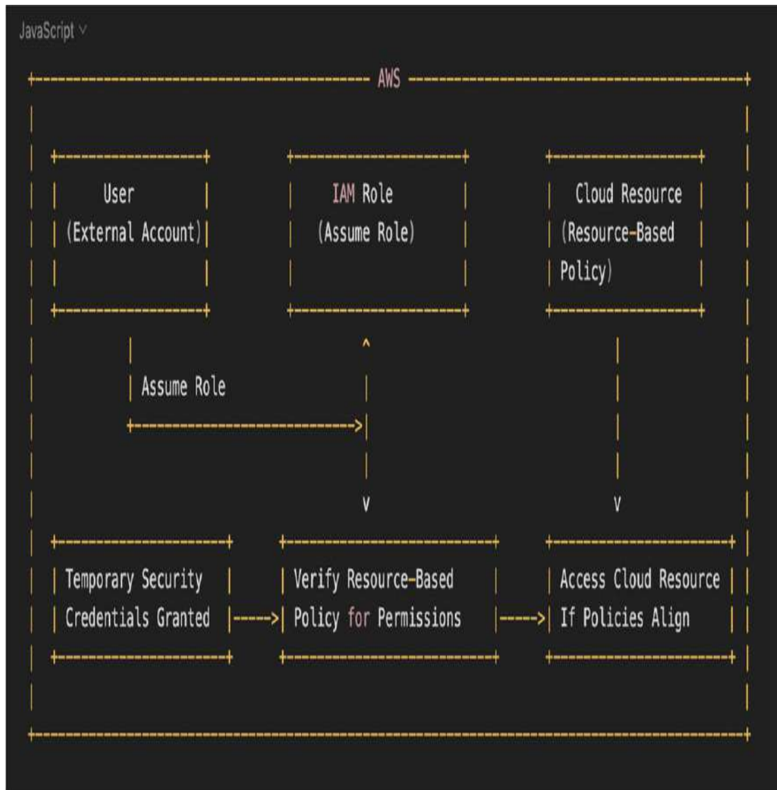
Figure 19-9 AWS Example: IAM Role with Resource-Based Policy
