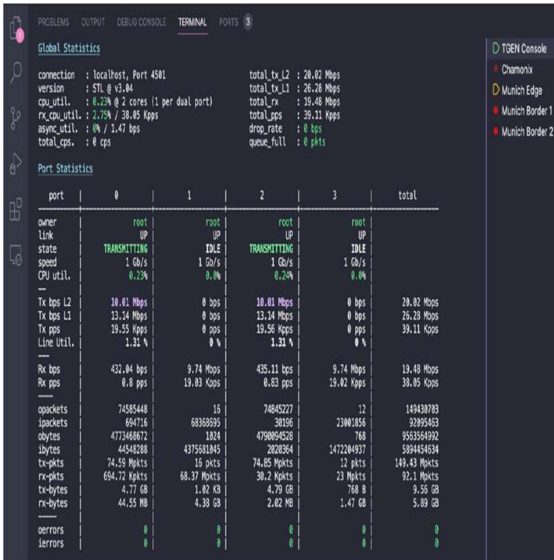
Figure 11-22 TReX Transmitting Data Without Dropping Any Data
