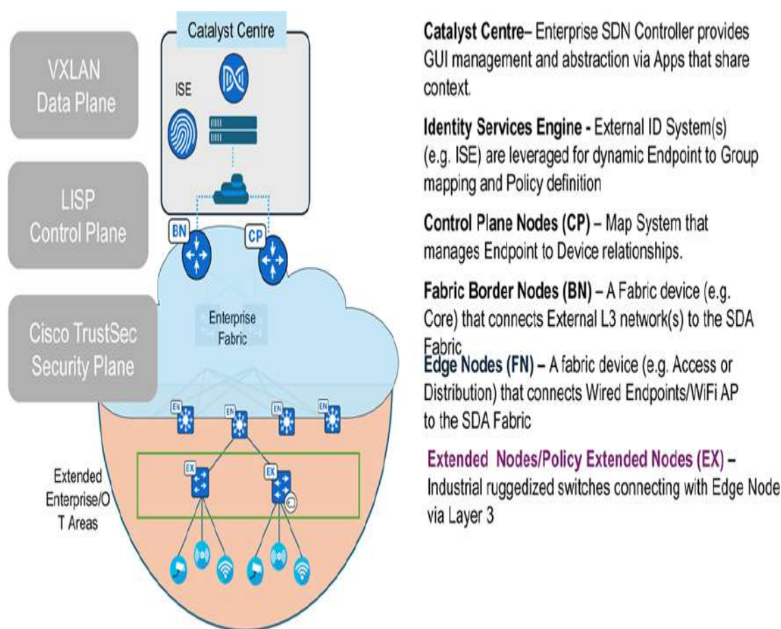
Figure 21-12 Cisco SD-Access Extended Network Components
