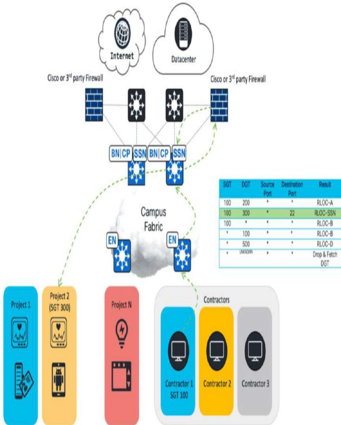
Figure 22-15 R&D Environment and Secure Service Insertion
