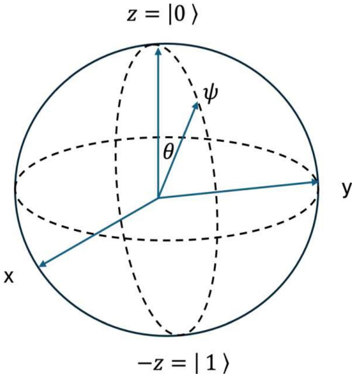
Figure 10-1 Bloch Sphere
