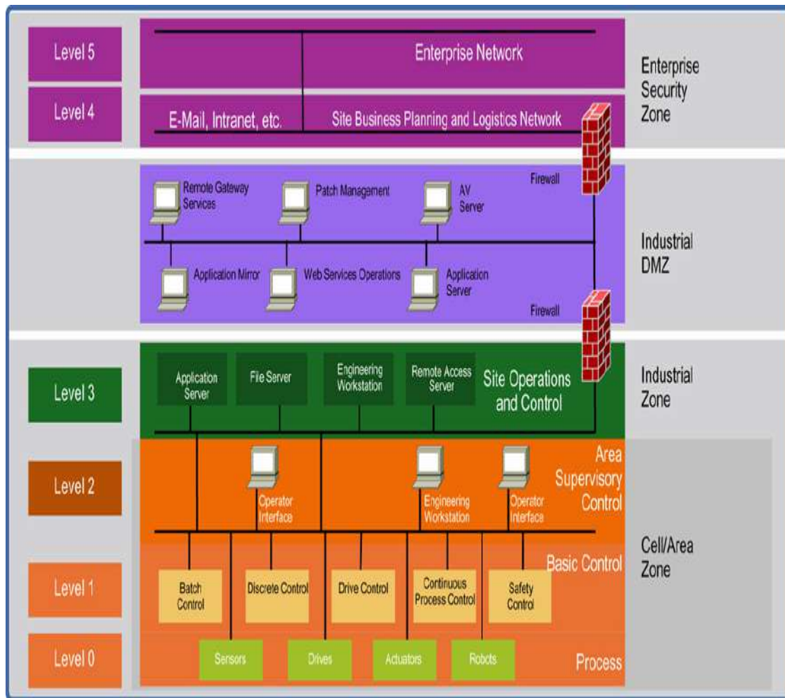
Figure 21-2 Purdue Model
