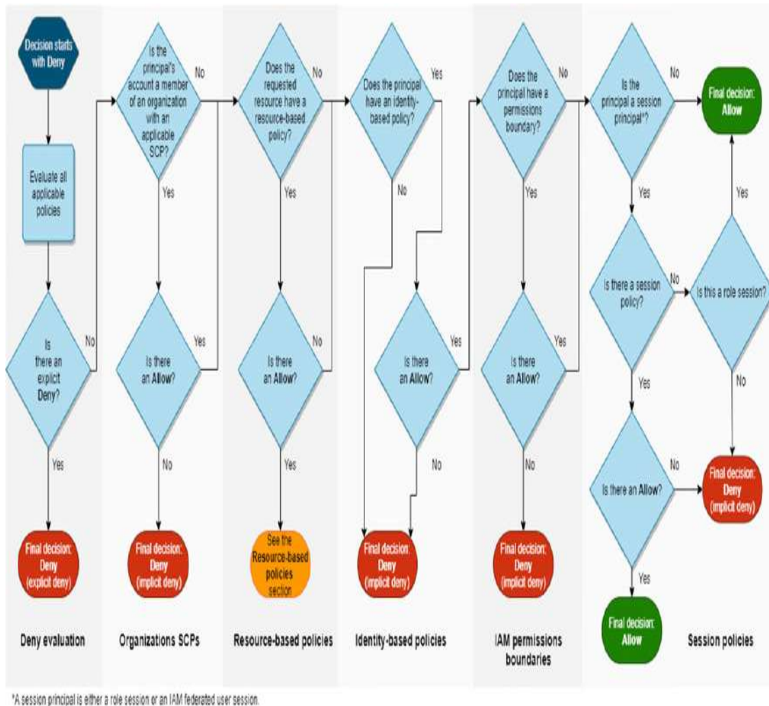
Figure 19-12 AWS Policy Evaluation Flow Chart
