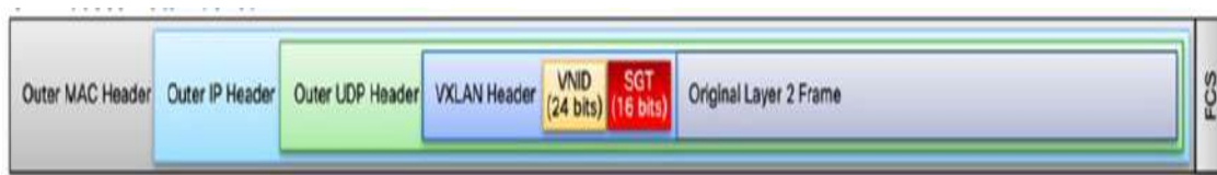
Figure 8-3 VXLAN Encapsulated Packet
