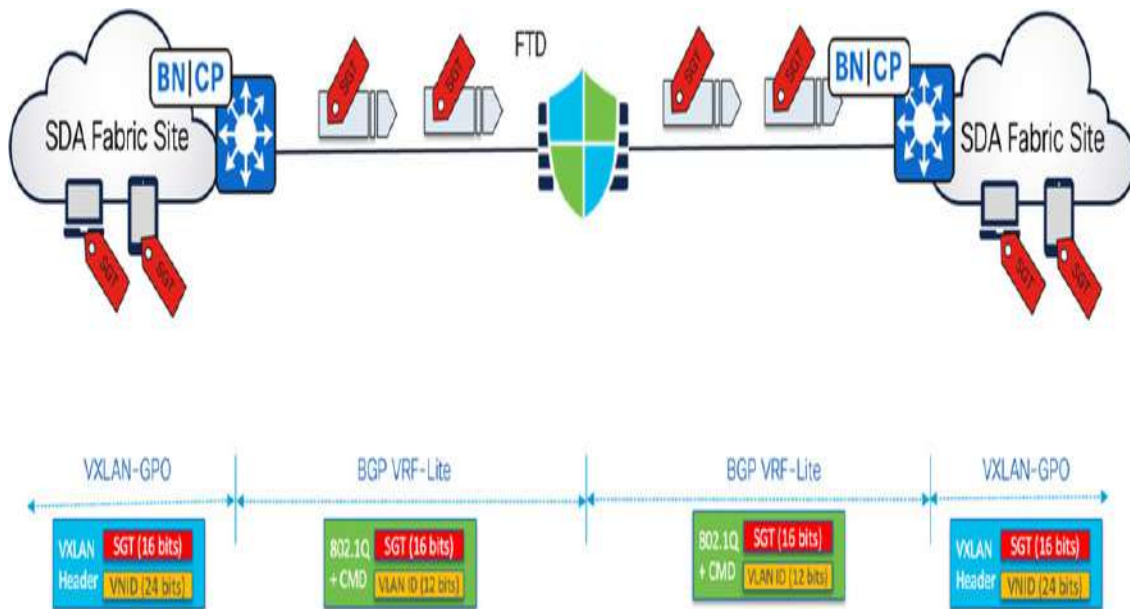
Figure 22-18 CMD Inline Tagging SGT Propagation Across Firewall
