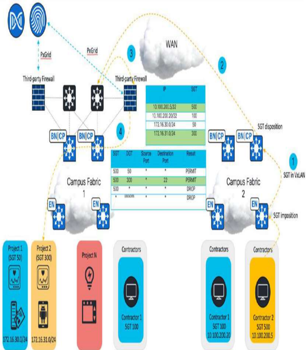
Figure 22-19 Third-Party Vendor Firewall Integration Packet Flow
