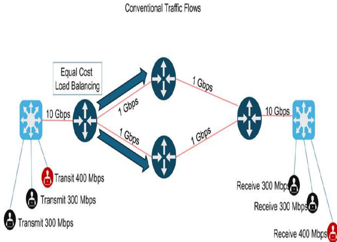
Figure 11-14 Equal-Cost Multipath Flows of Traffic over a Network
