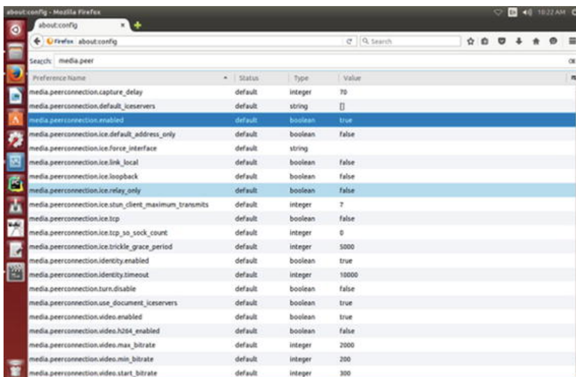
Figure 28-3. Check “media.peerconnection.enabled” true or false
