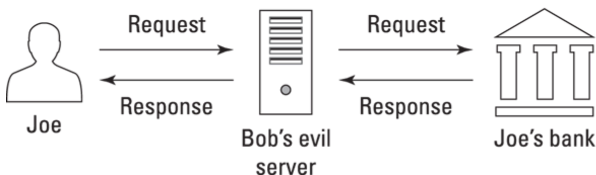
FIGURE 2-2: A man-in-the-middle interception.
