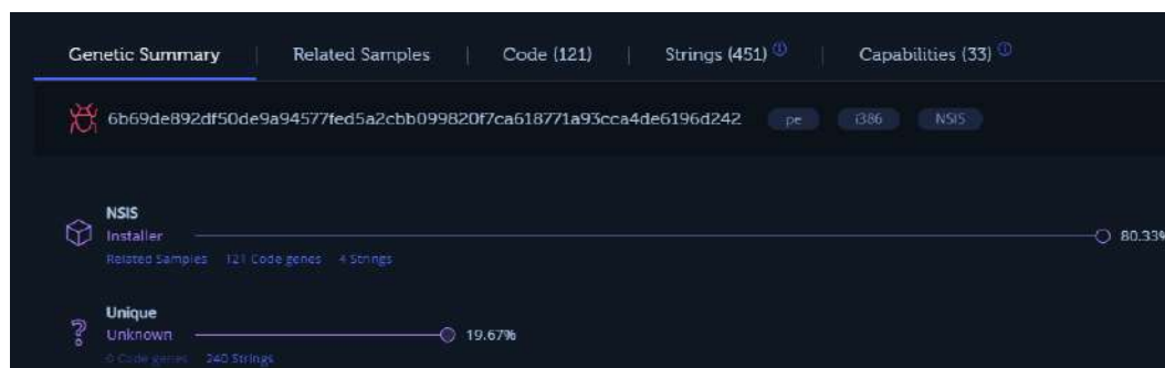
Figure 16.12 – Intezer metadata
