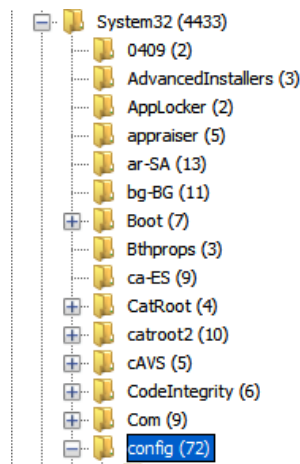
Figure 11.38 – Registry location
