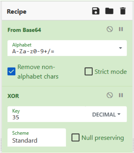
Figure 15.24 – Base64 XOR recipe
