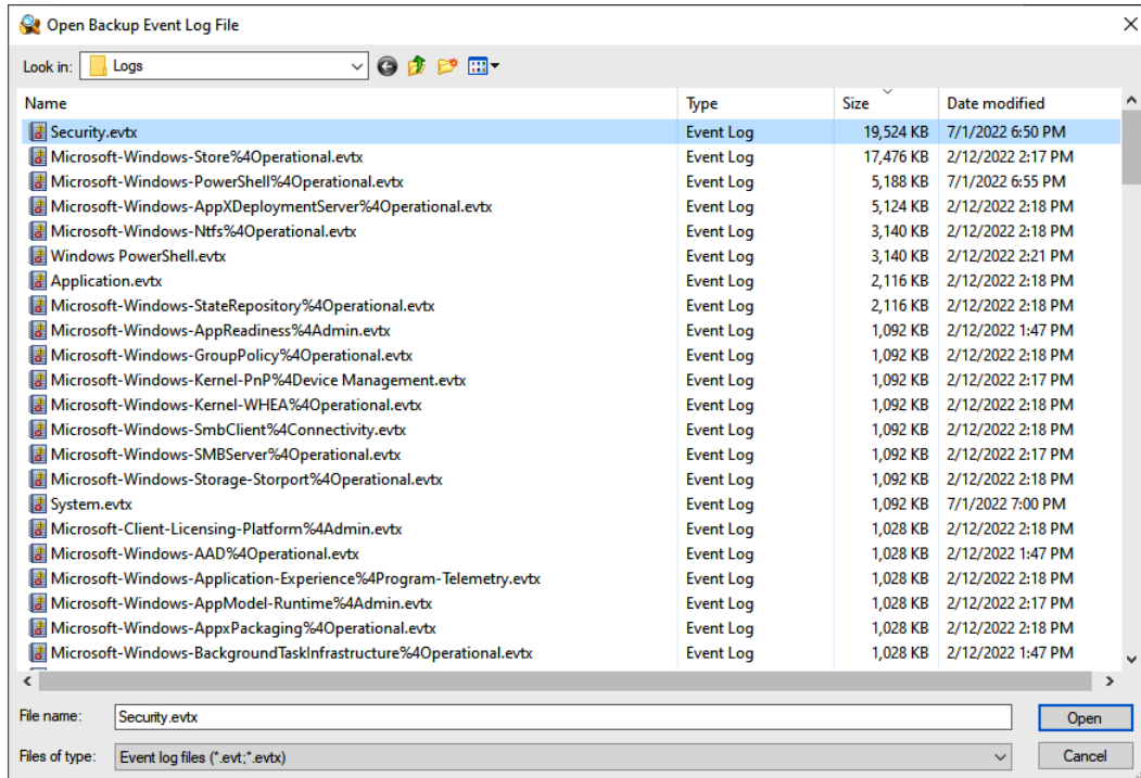
Figure 12.14 – Opening Windows event logs
