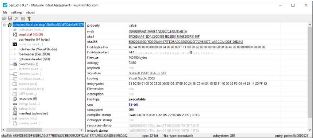
Figure 16.3 – PEStudio metadata view
