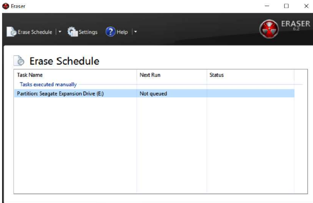
Figure 8.7 – Erase Schedule
