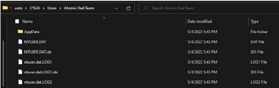
Figure 7.25 – Acquired evidence
