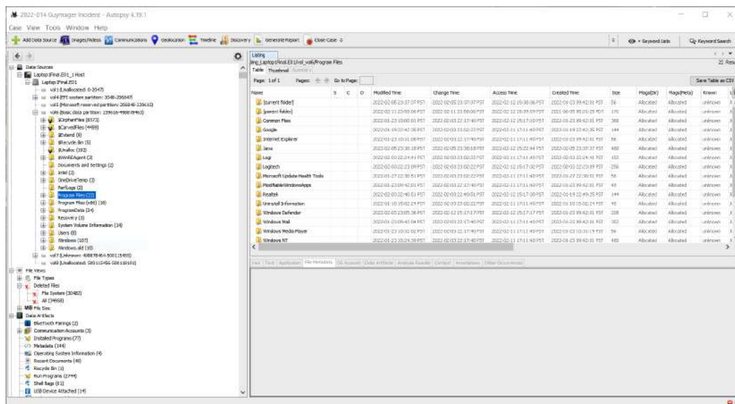
Figure 11.12 – Autopsy GUI
