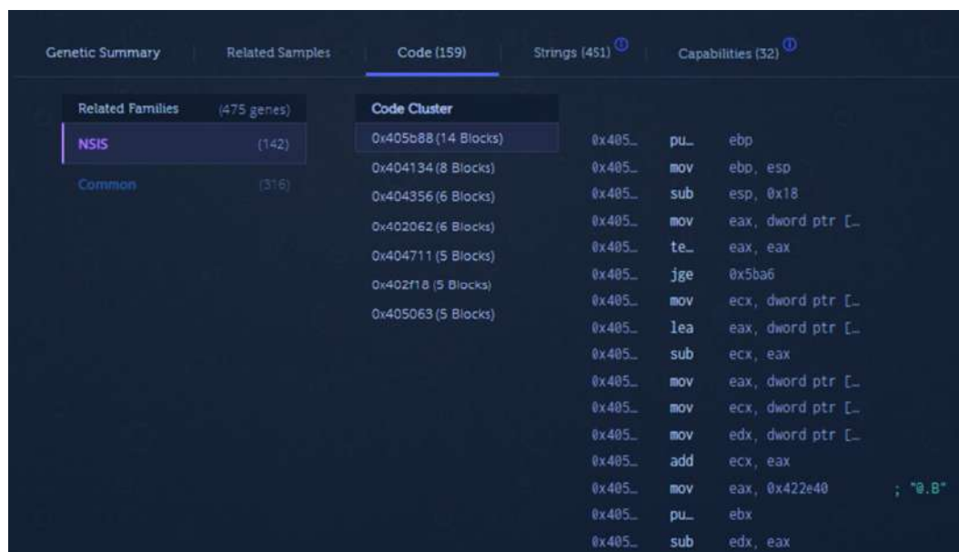
Figure 16.16 – Code analysis
