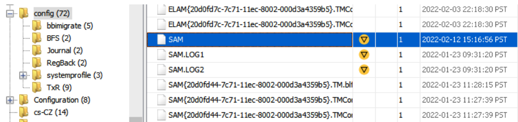
Figure 11.39 – SAM location
