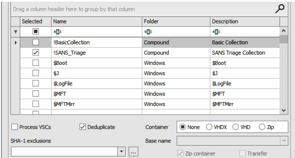
Figure 6.20 – SANS_Triage target
