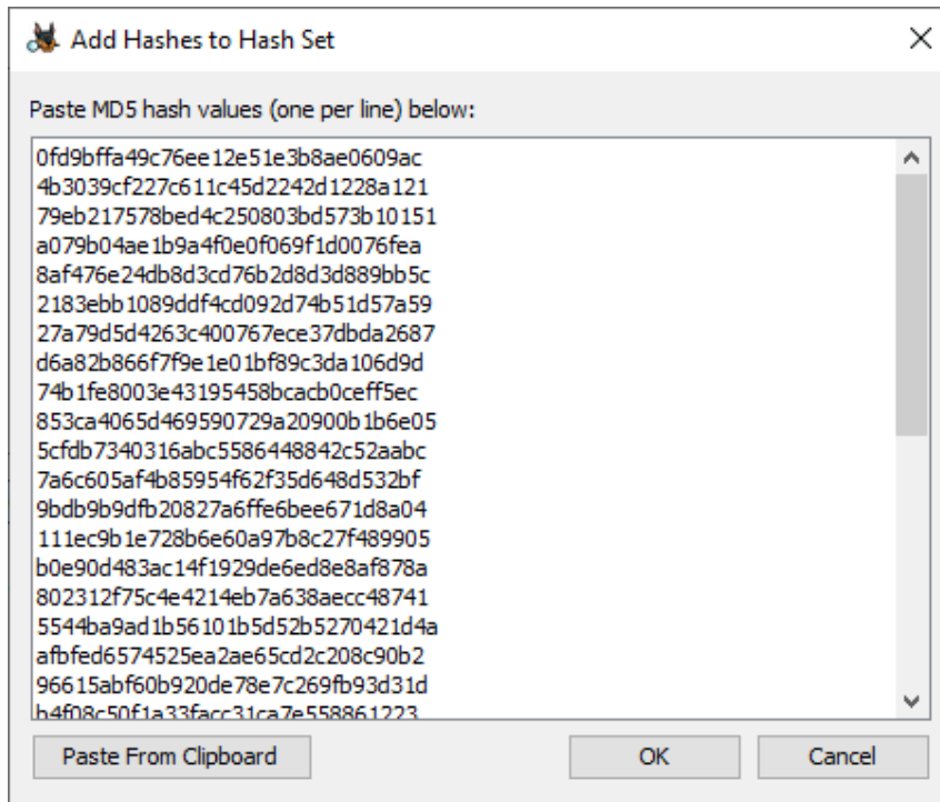
Figure 17.25 – Hash values
