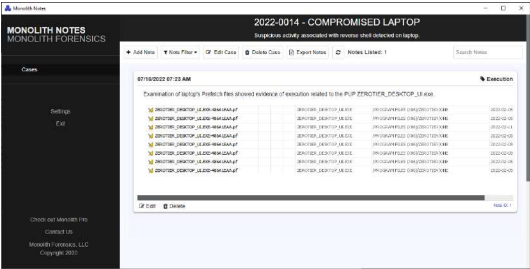
Figure 13.9 – Completed note
