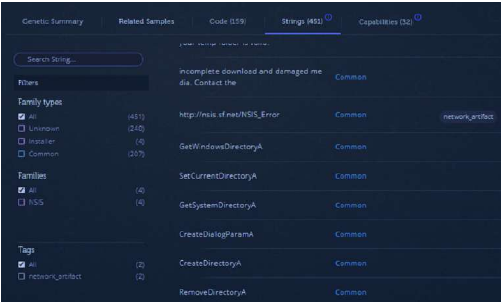
Figure 16.17 – Strings
