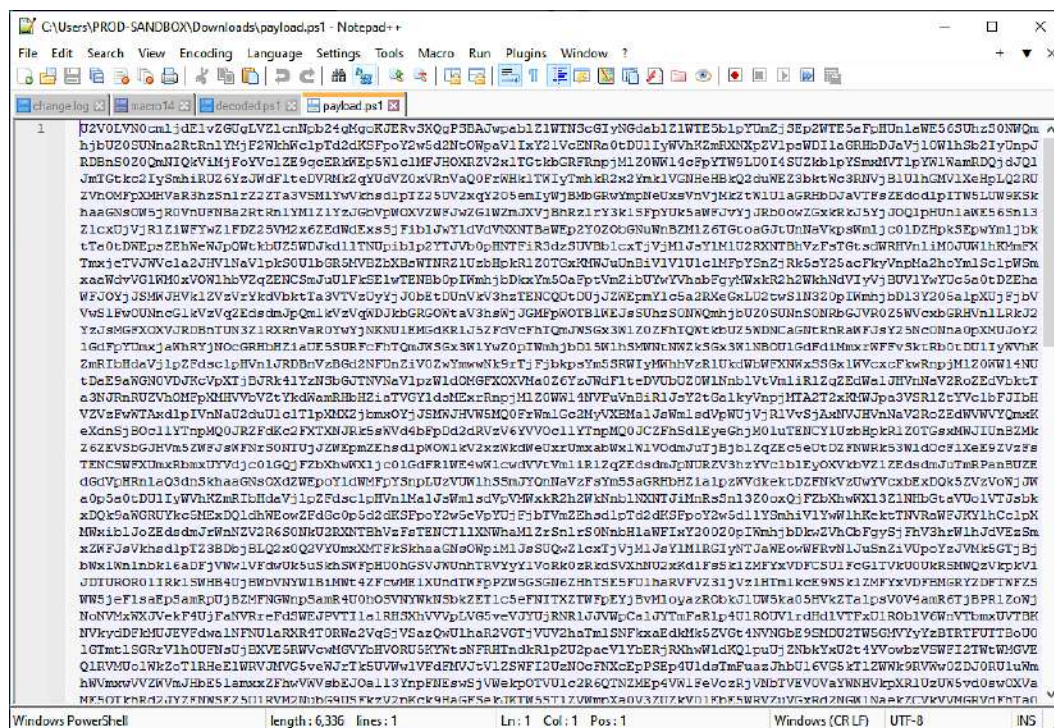
Figure 15.21 – Cobalt Strike Base64-encoded script
