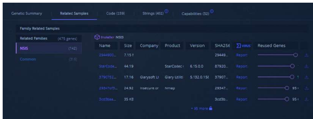
Figure 16.15 – Reused genes
