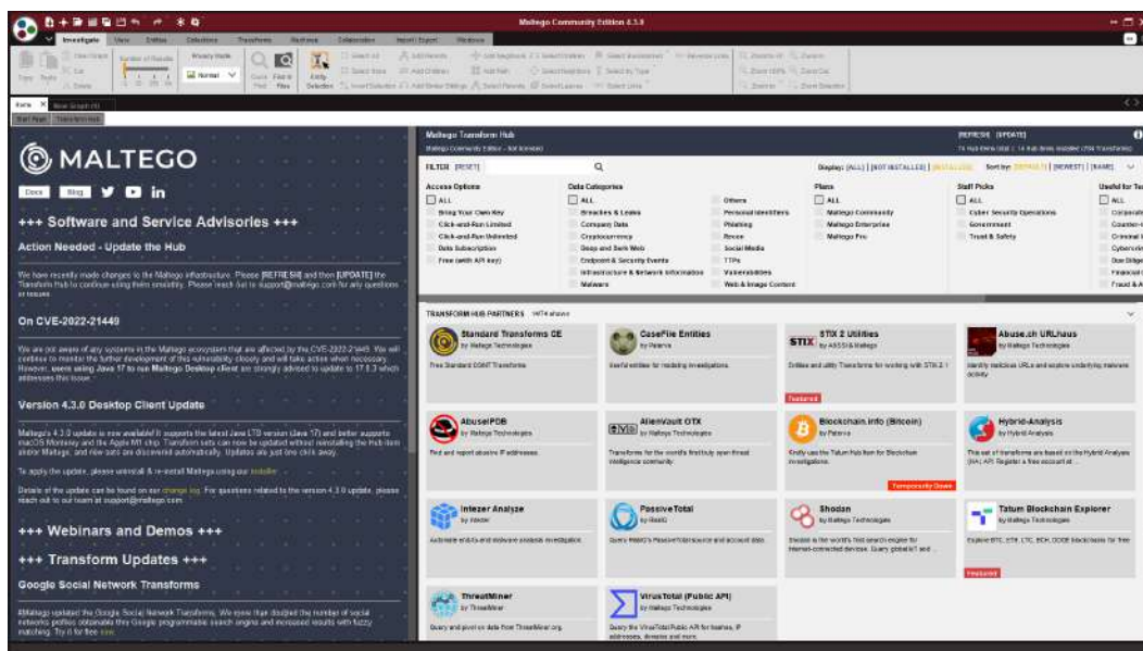
Figure 17.27 – Maltego GUI
