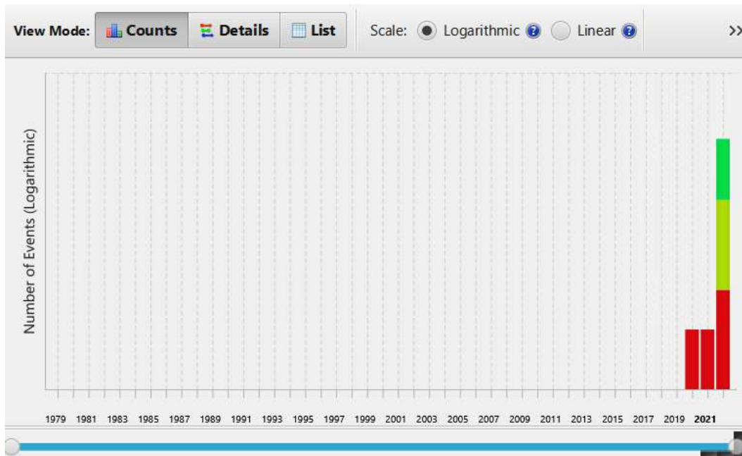
Figure 11.34 – Keyword timeline
