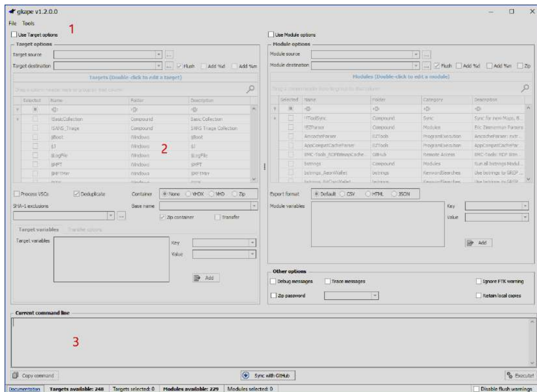
Figure 6.18 – KAPE GUI
