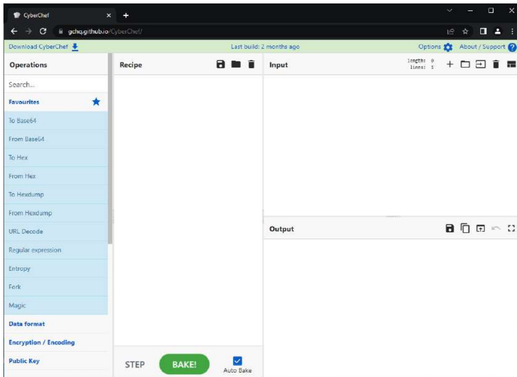
Figure 15.9 – CyberChef interface
