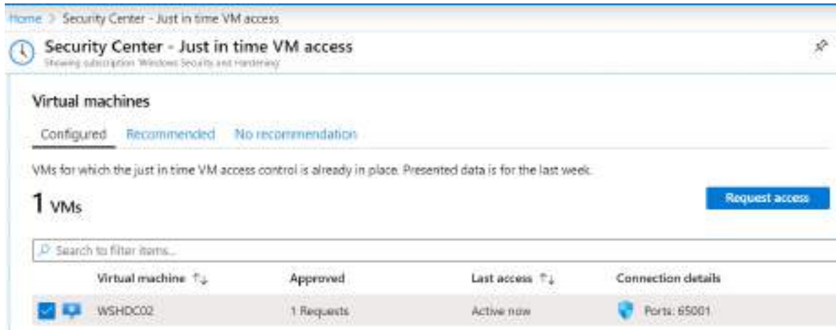
Figure 11.22 – JIT access rule over port 65001 showing as active
