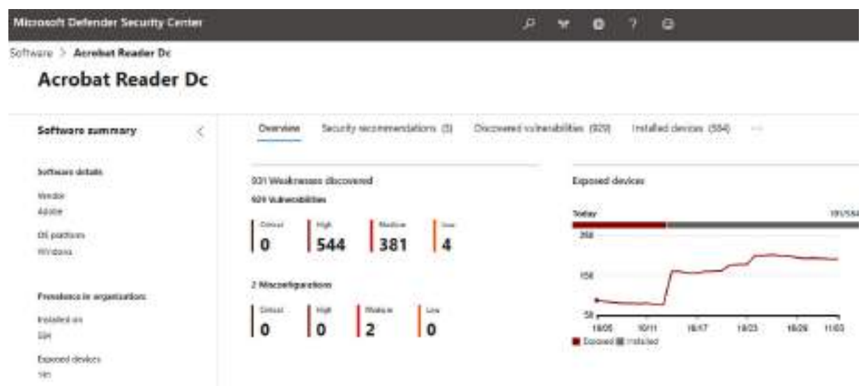
Figure 1.9 – Acrobat Reader DC identified vulnerabilities
