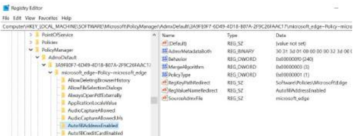
Figure 9.5 – ADMX ingestion of Microsoft Edge policies
