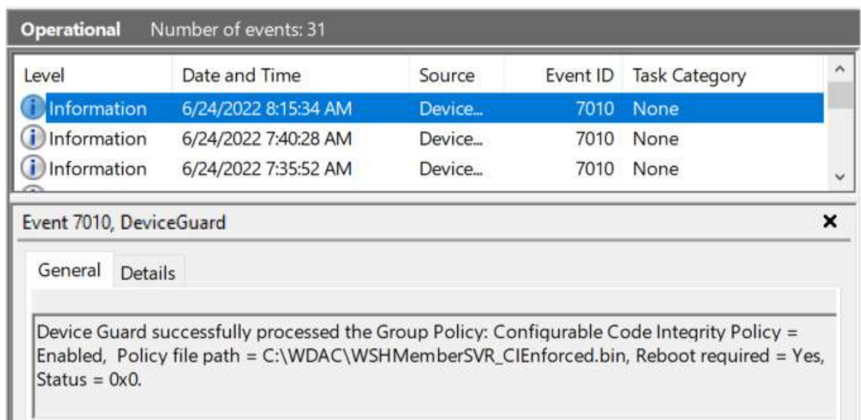
Figure 12.43 – DeviceGuard – Operational logs
