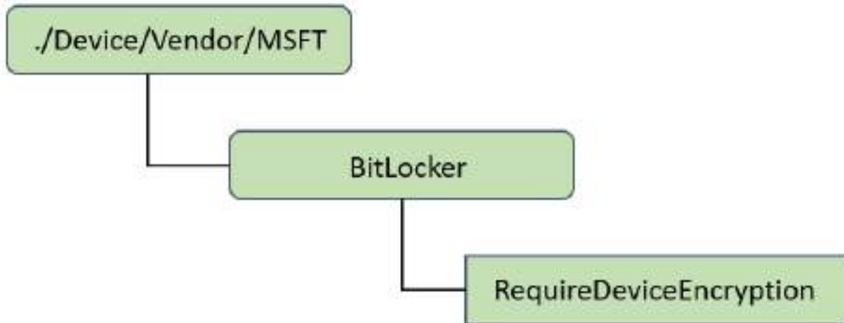
Figure 6.18 – CSP diagram for the BitLocker RequireDeviceEncryption setting
