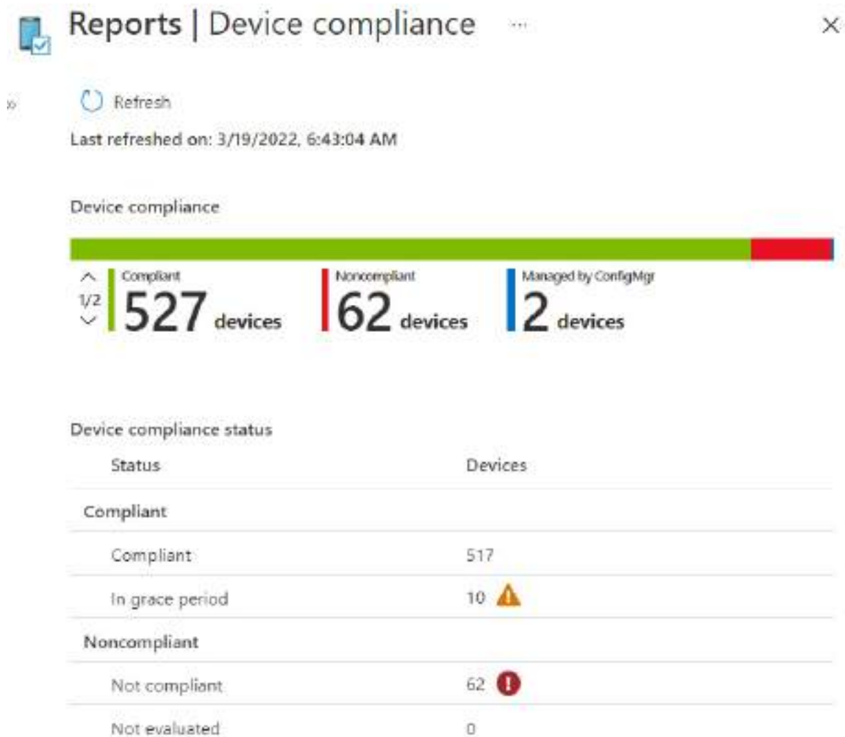
Figure 13.24 – Device compliance summary report
