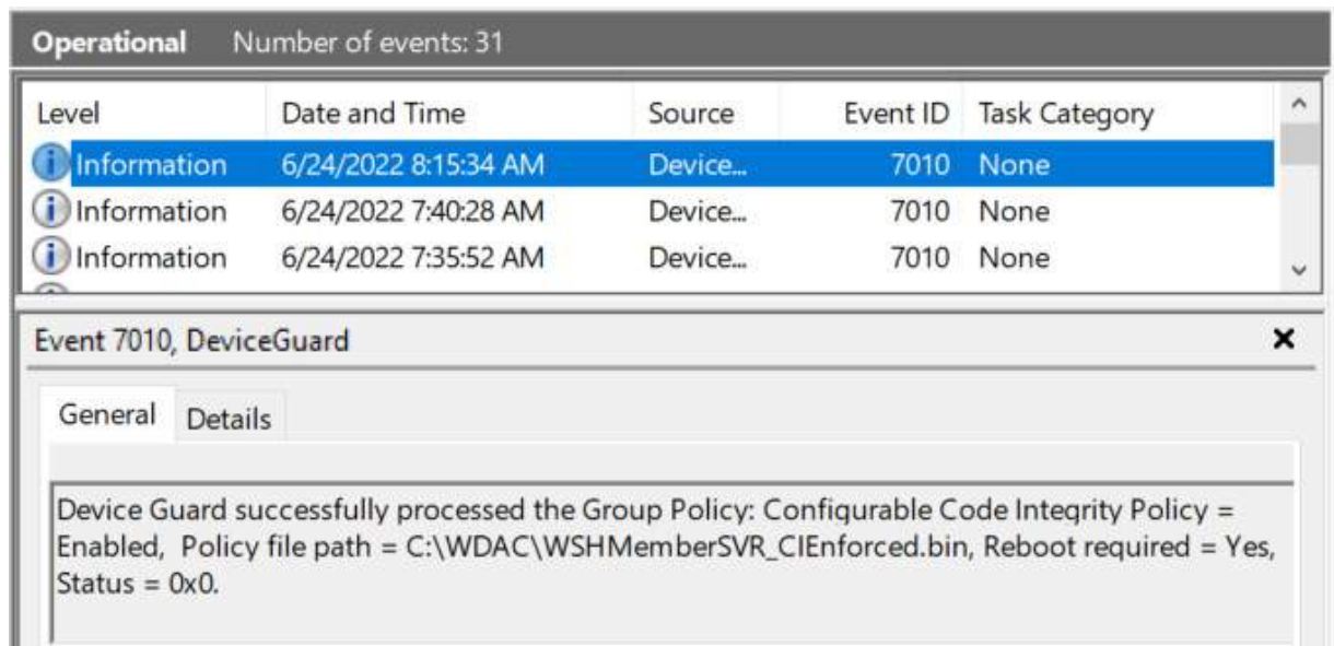
Figure 10.45 – Device Guard – Operational logs in Event Viewer
