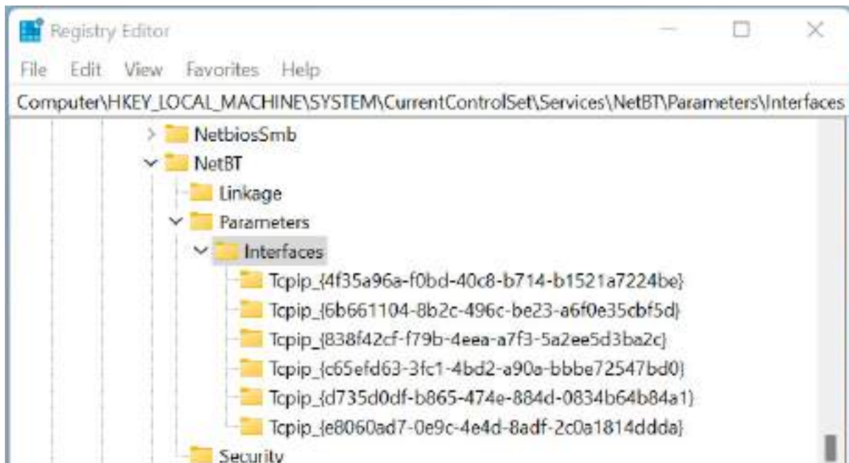
Figure 10.5 – The TCPIP_GUID values of network adapters
