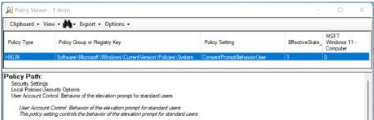
Figure 8.28 – Policy Analyzer comparison
