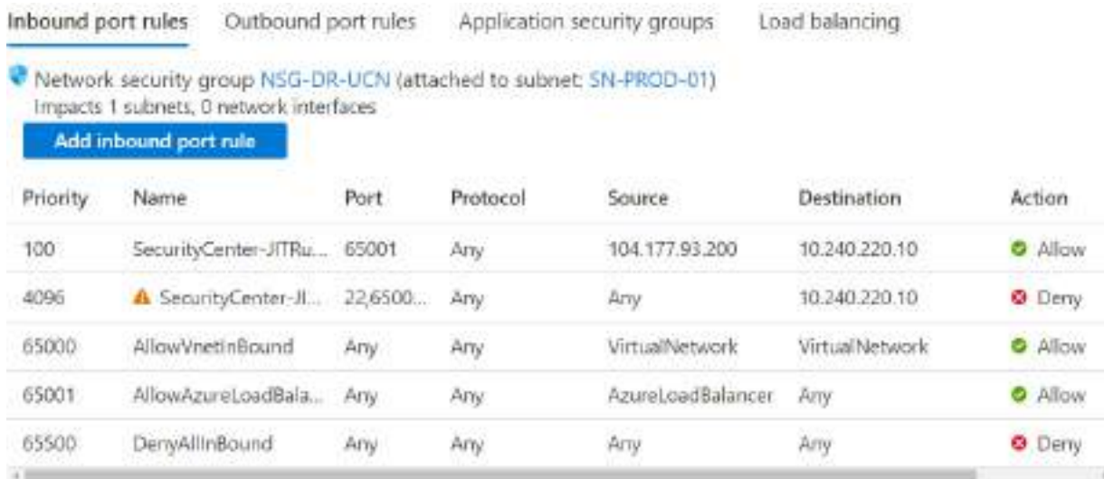
Figure 11.23 – Active JIT rule
