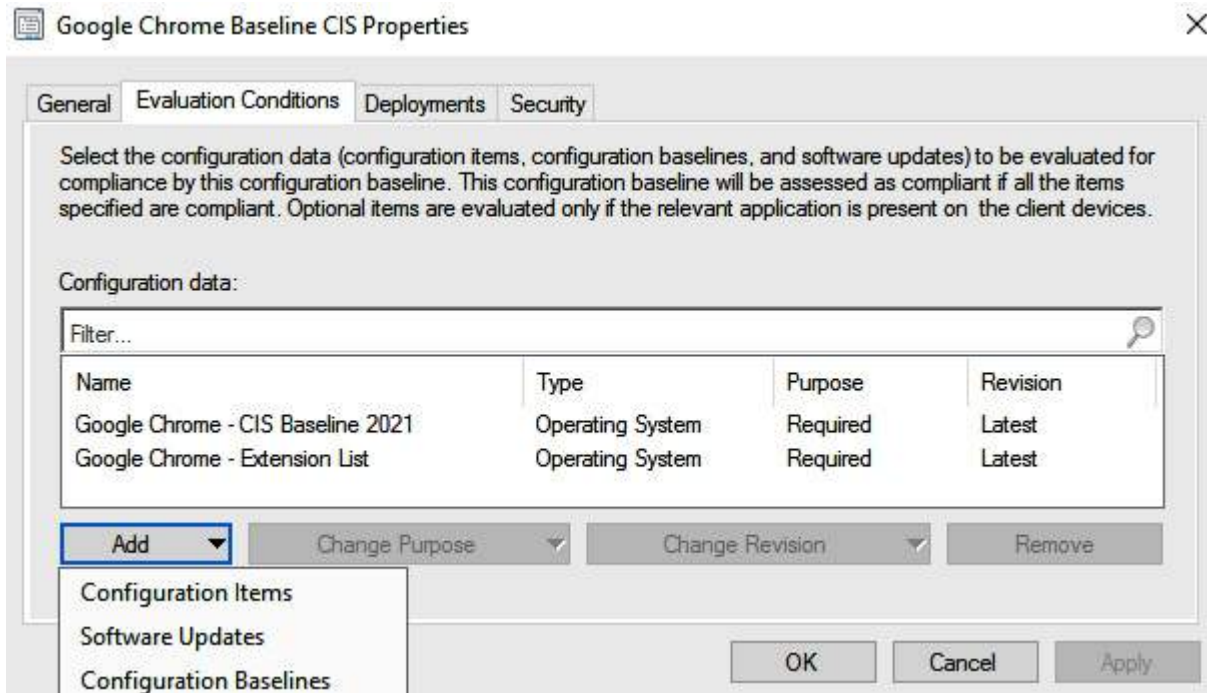
Figure 6.14 – Configuration baseline properties
