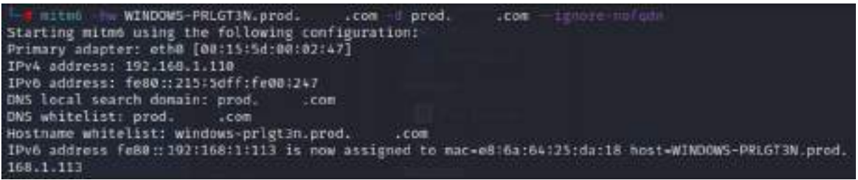
Figure 10.25 – MiTM attack on IPv6
