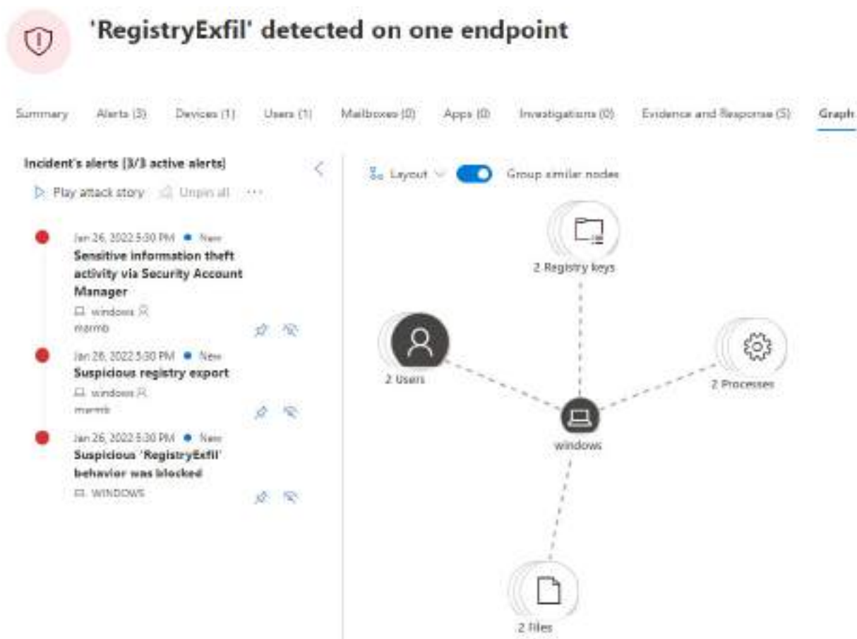
Figure 14.14 – The Graph view of the alert story
