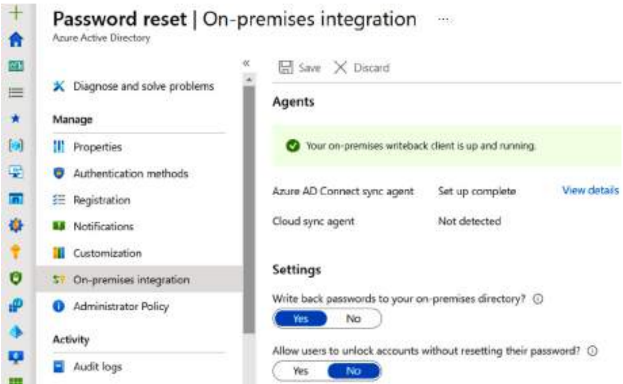
Figure 5.14 – On-premises AD integration
