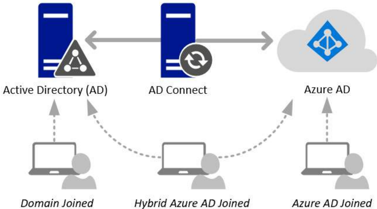
Figure 6.2 – Domain-joined, hybrid, and Azure AD-joined examples
