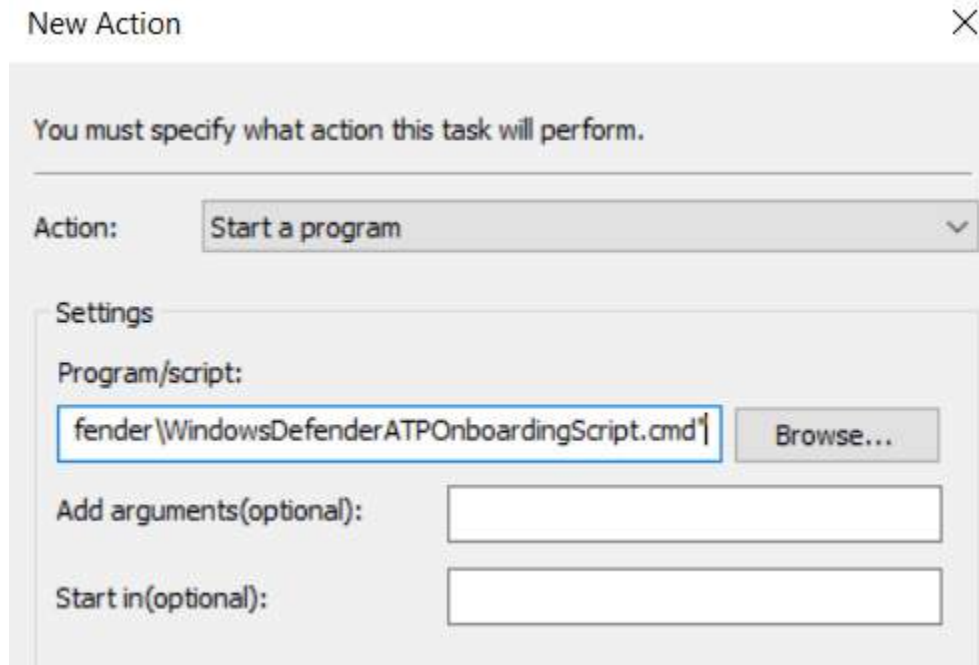
Figure 12.17 – Configuring a new action for a scheduled task
