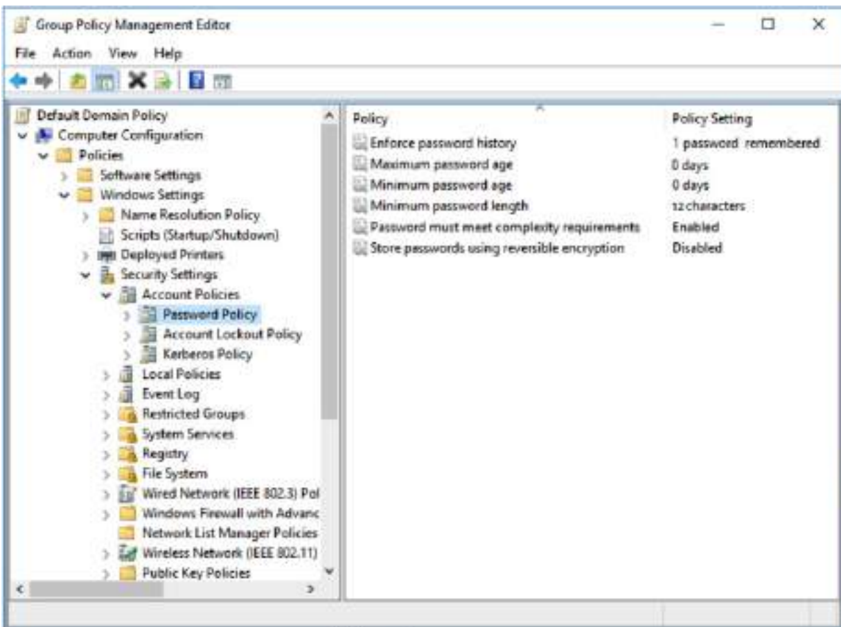
Figure 5.11 – The default AD domain password policy
