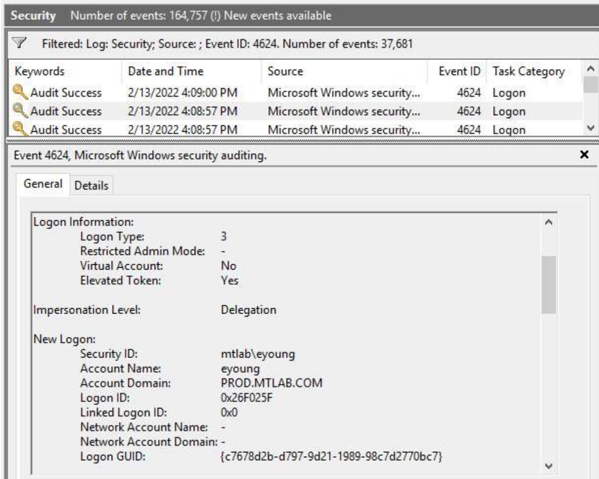
Figure 11.9 – Event 4624: successful login in Event Viewer
