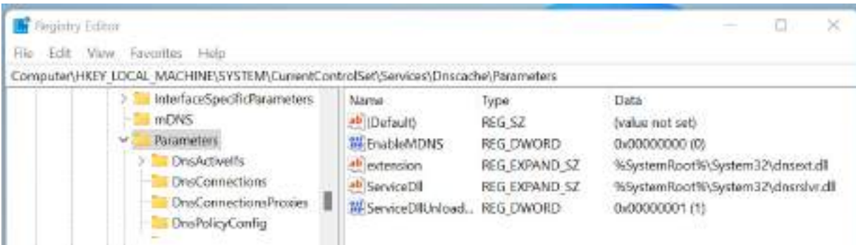
Figure 10.14 – Disabling mDNS for Windows
