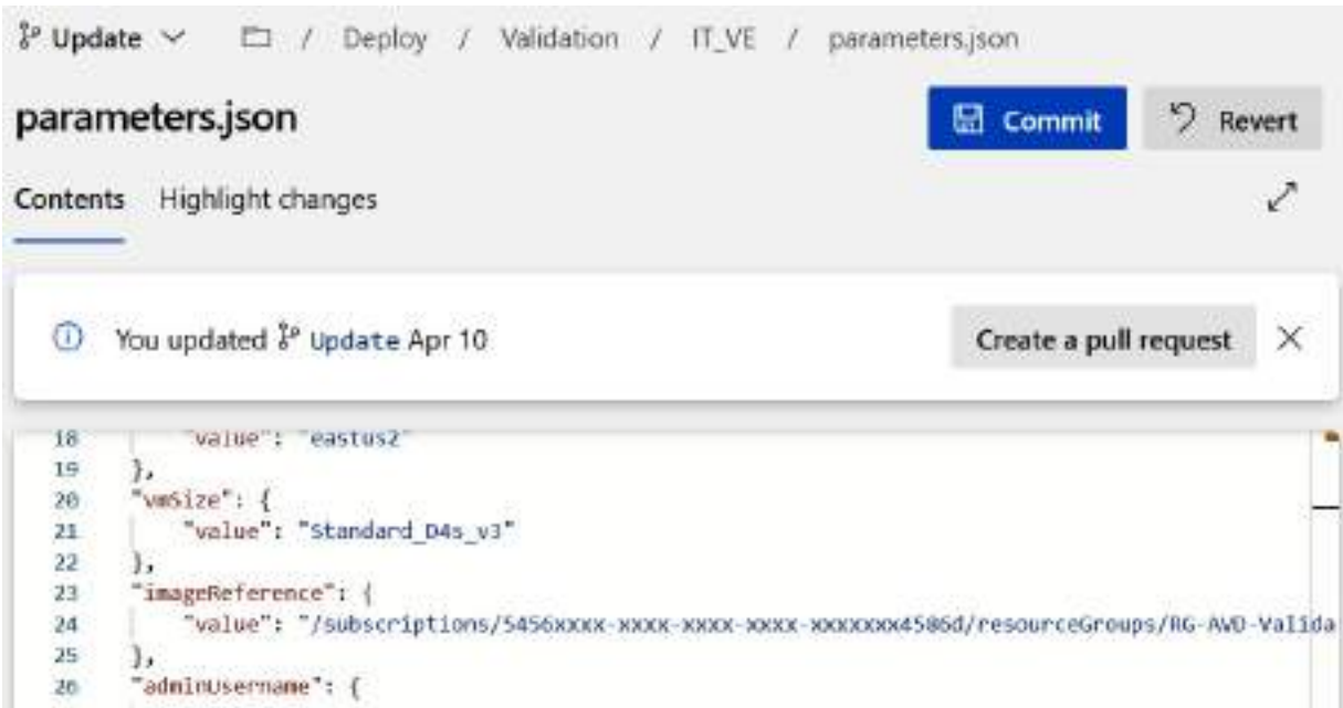
Figure 7.16 – Azure DevOps deployment for AVD
