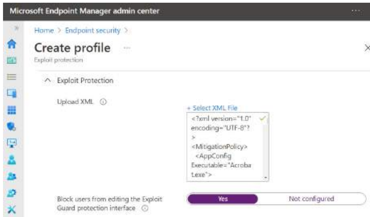
Figure 9.39 – Exploit protection profile in Endpoint security
