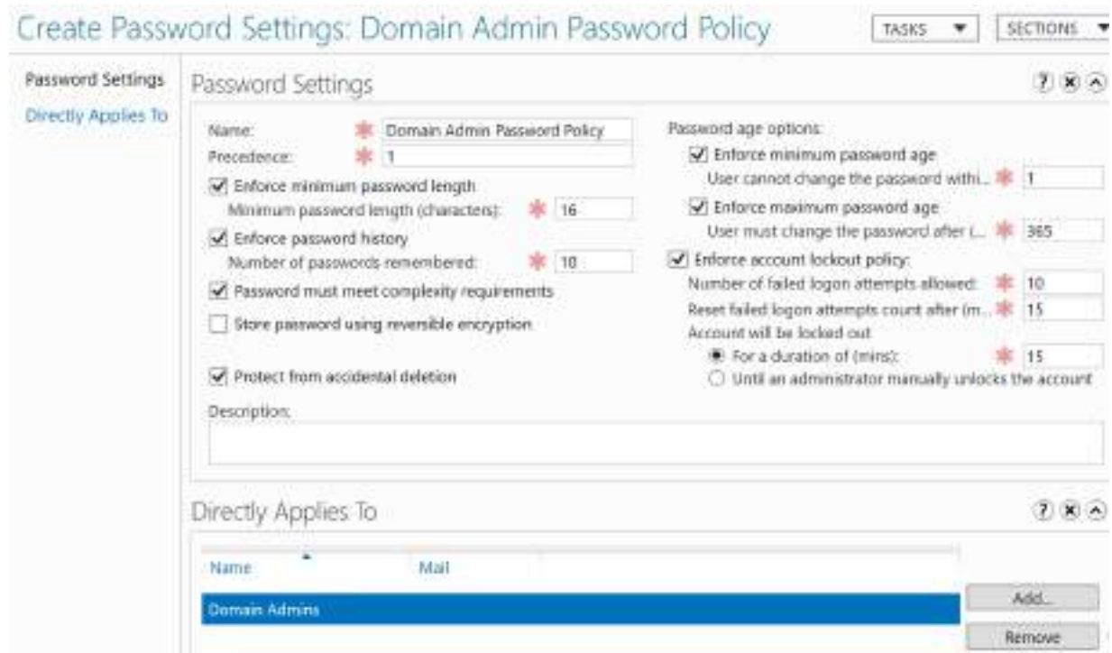
Figure 12.27 – Fine-grained password policy in Active Directory
