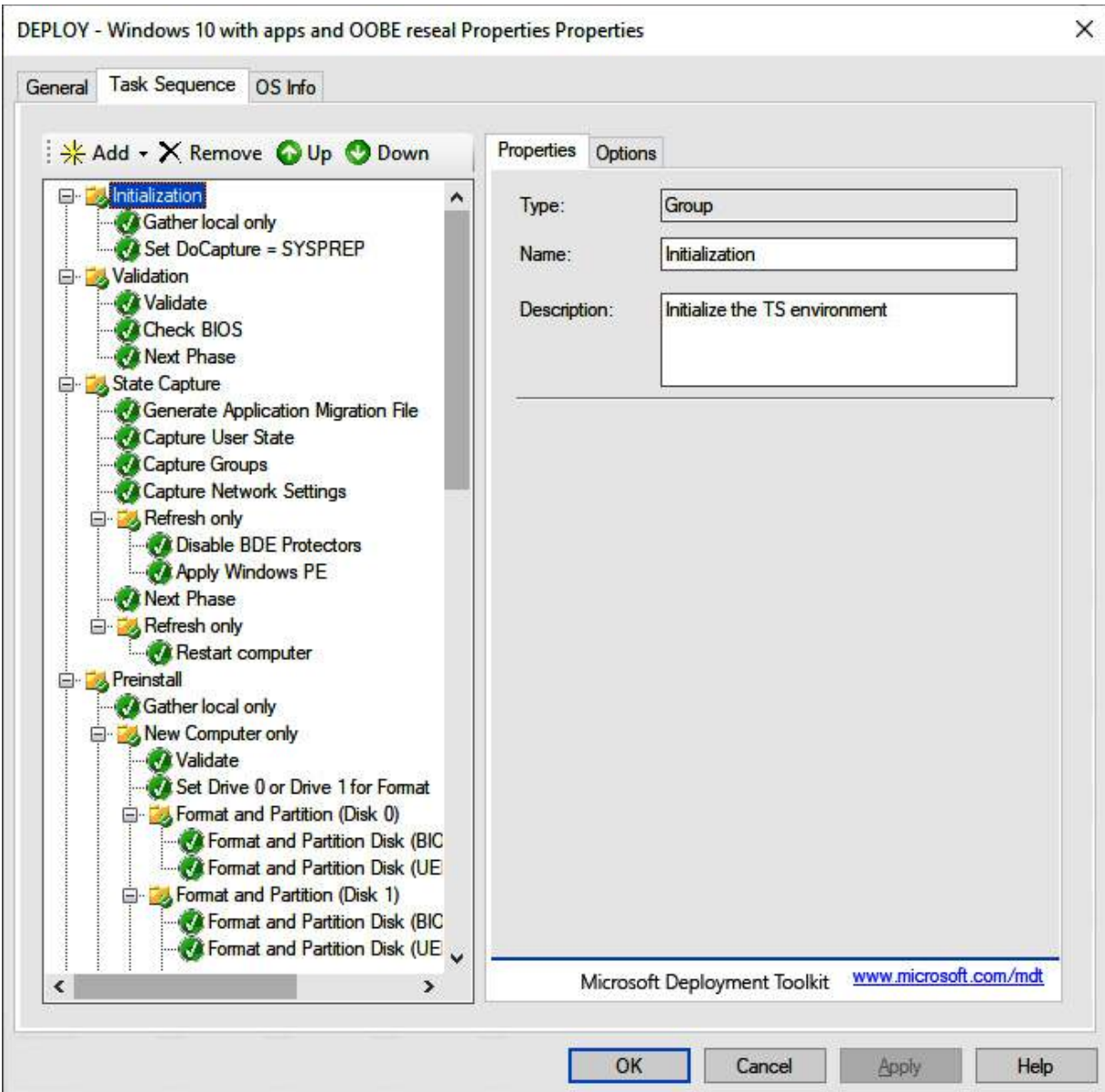
Figure 7.8 – Custom MDT task sequence
