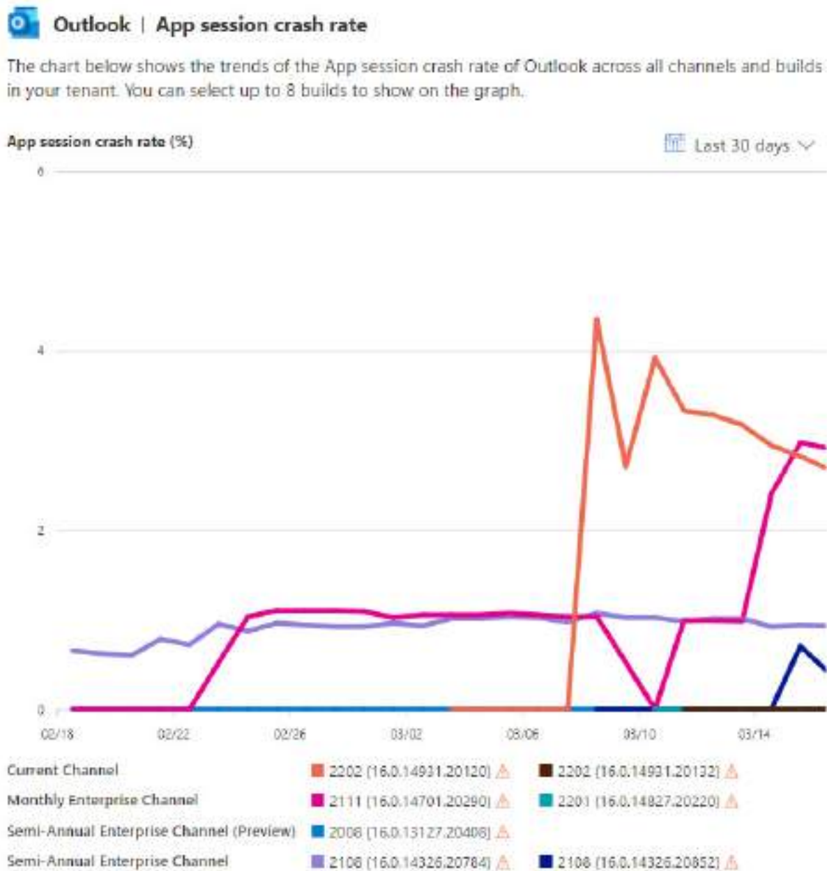
Figure 13.32 – App metrics for Outlook
