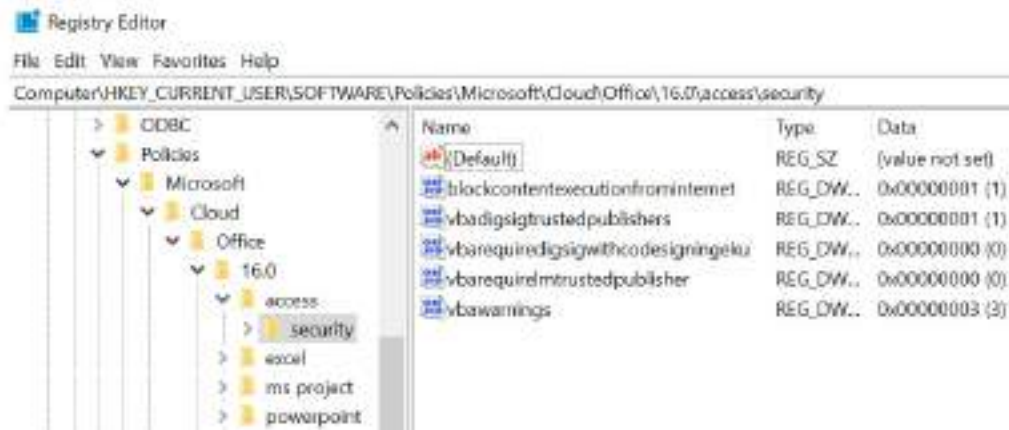
Figure 9.25 – Office cloud policy service policies
