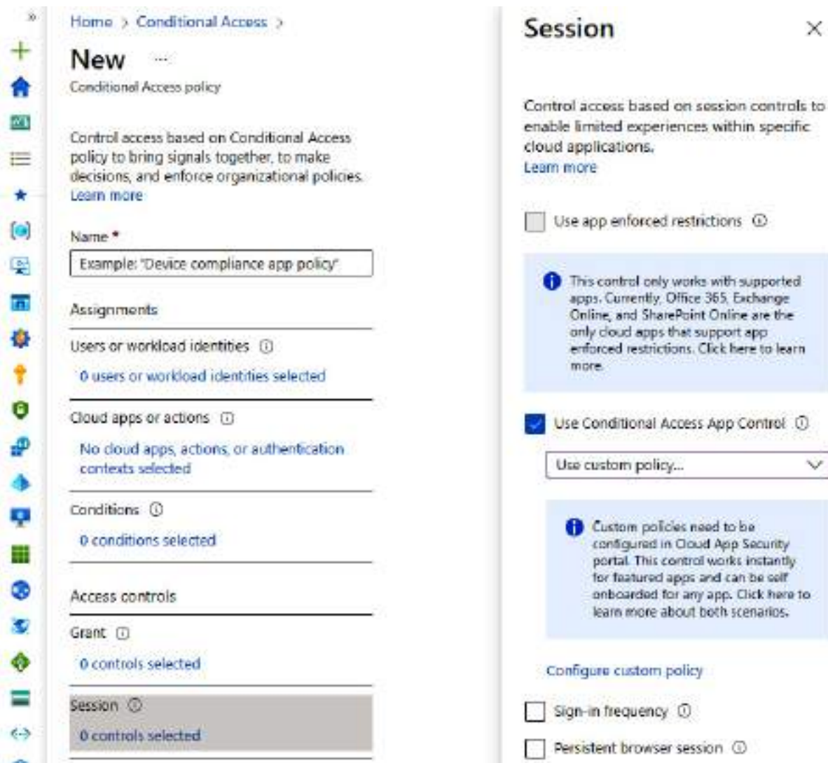
Figure 14.29 – Onboarding apps into MDCA using conditional access
