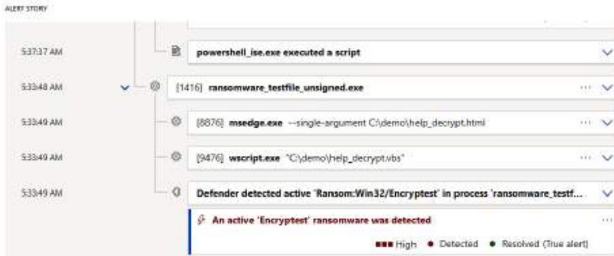
Figure 14.10 – The MDE alert story
