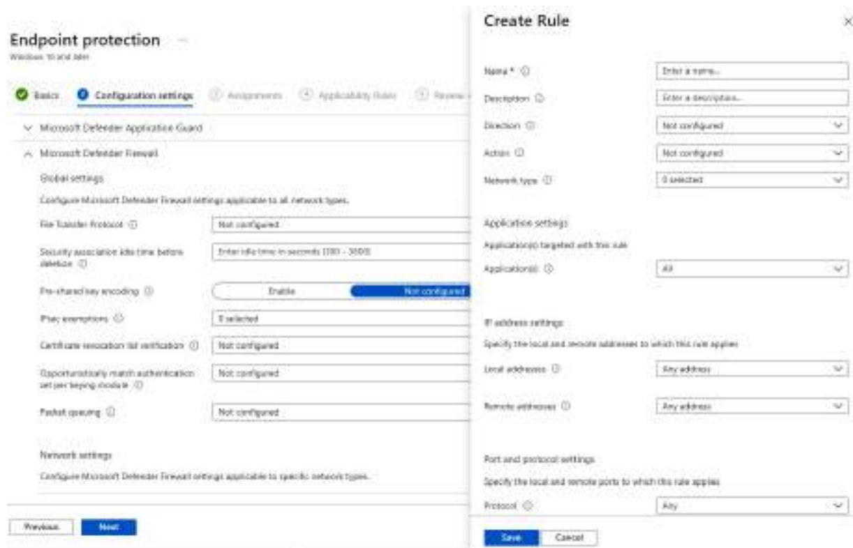
Figure 4.13 – Microsoft Defender Firewall template in Intune
