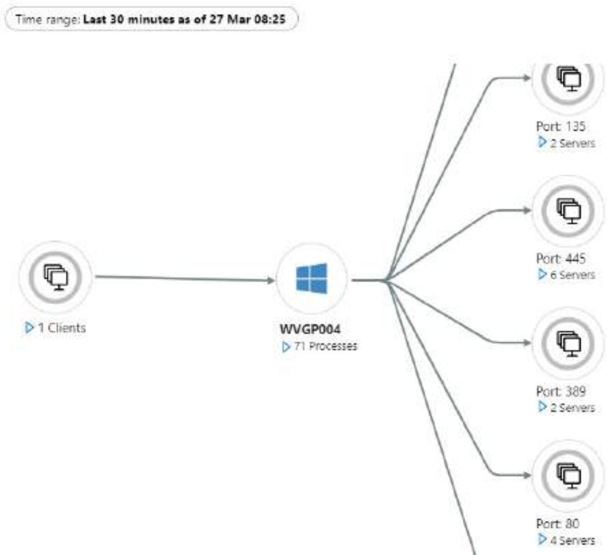
Figure 13.15 – Service Map solution
