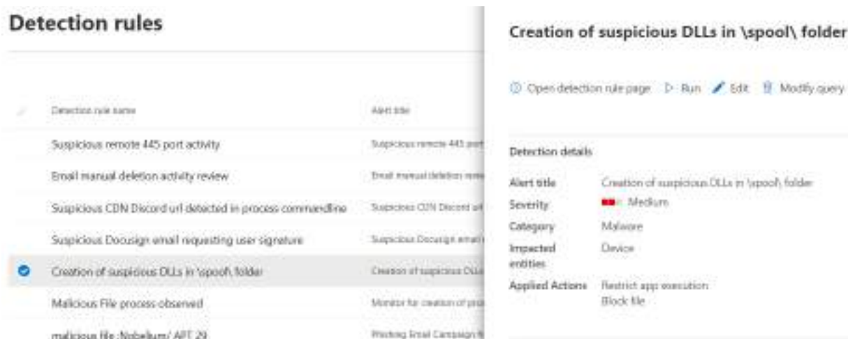
Figure 14.19 – Custom detection rules
