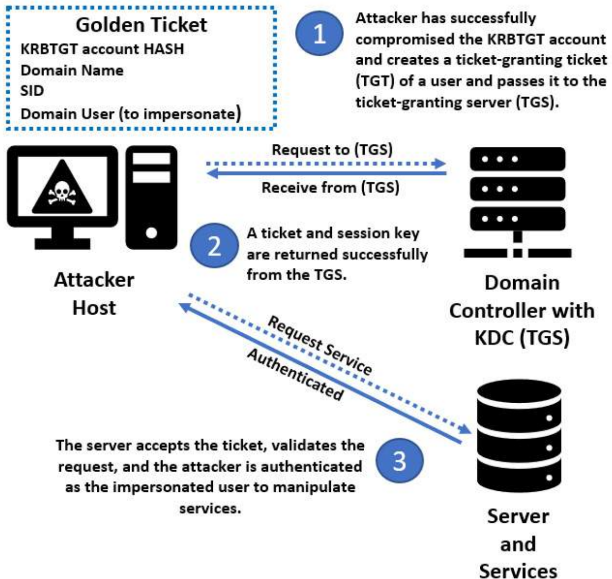
Figure 10.35 – Golden ticket attack
