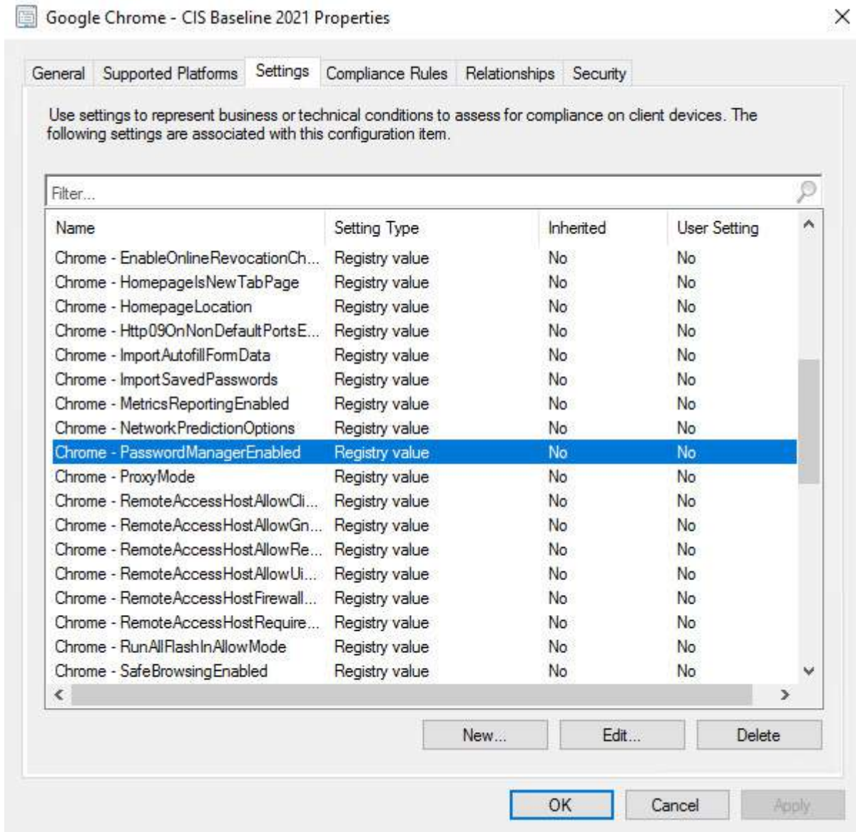
Figure 8.9 – Configuration Item settings
