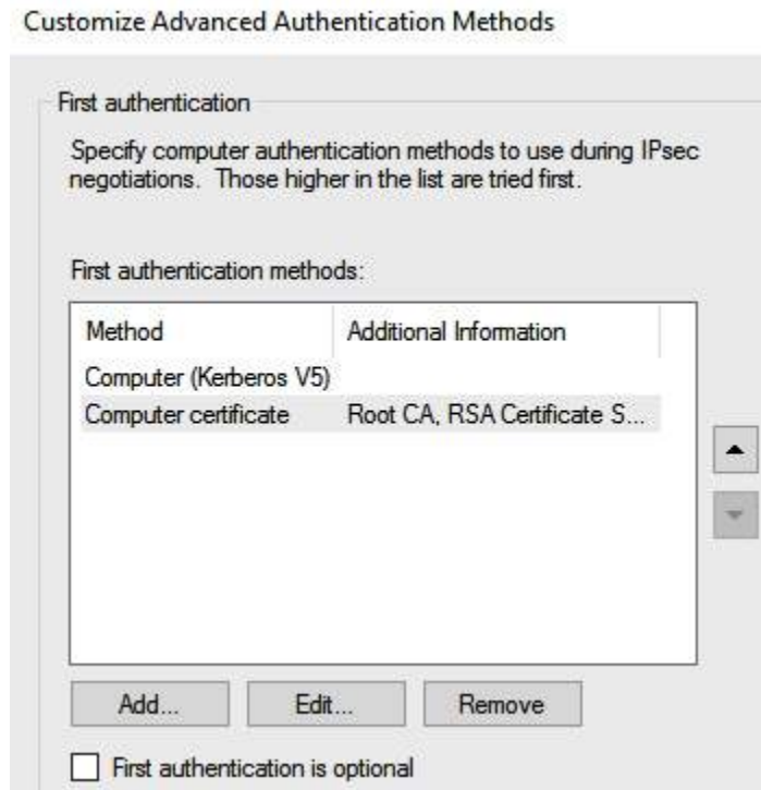
Figure 12.40 – Connection methods in Windows Defender Firewall
