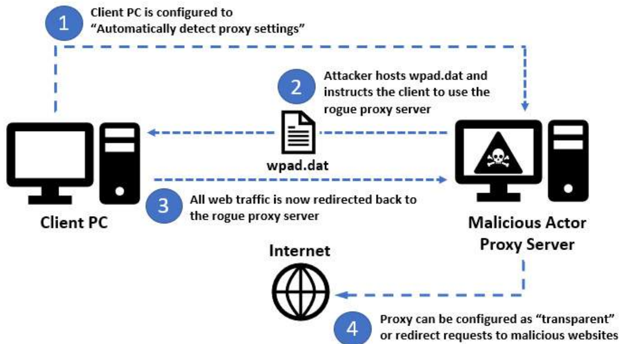
Figure 10.15 – Malicious proxy server
