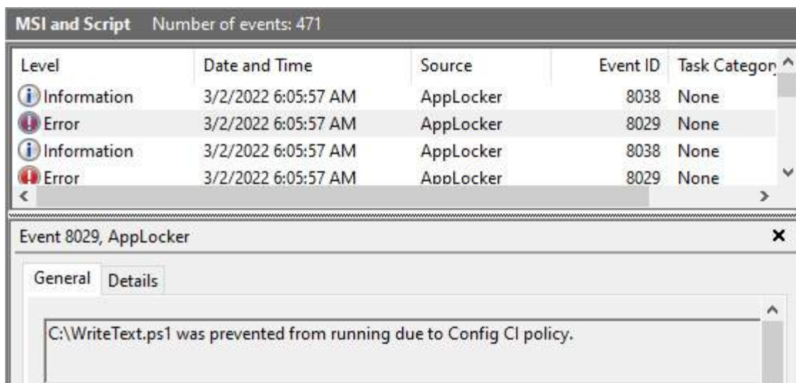
Figure 12.47 – AppLocker logs in Event Viewer
