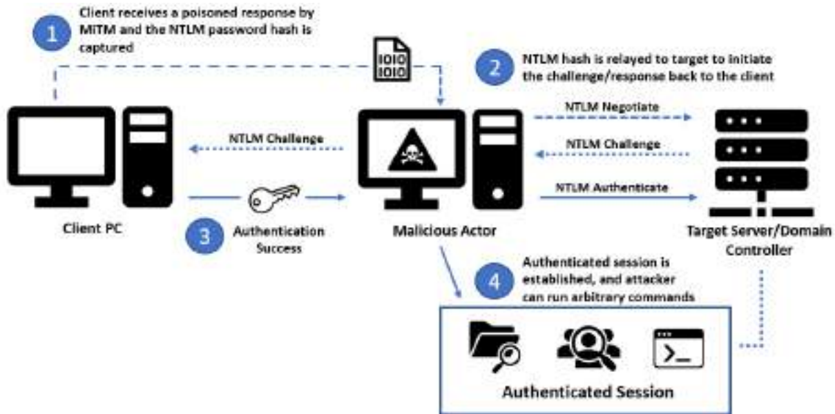
Figure 10.20 – NTLM relay attack
