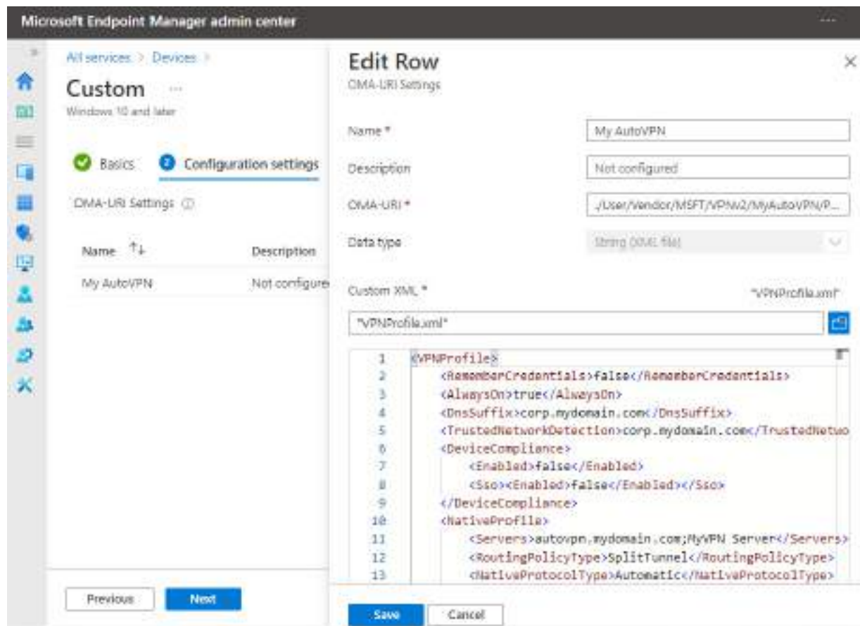
Figure 4.9 – Always On VPN in Intune
