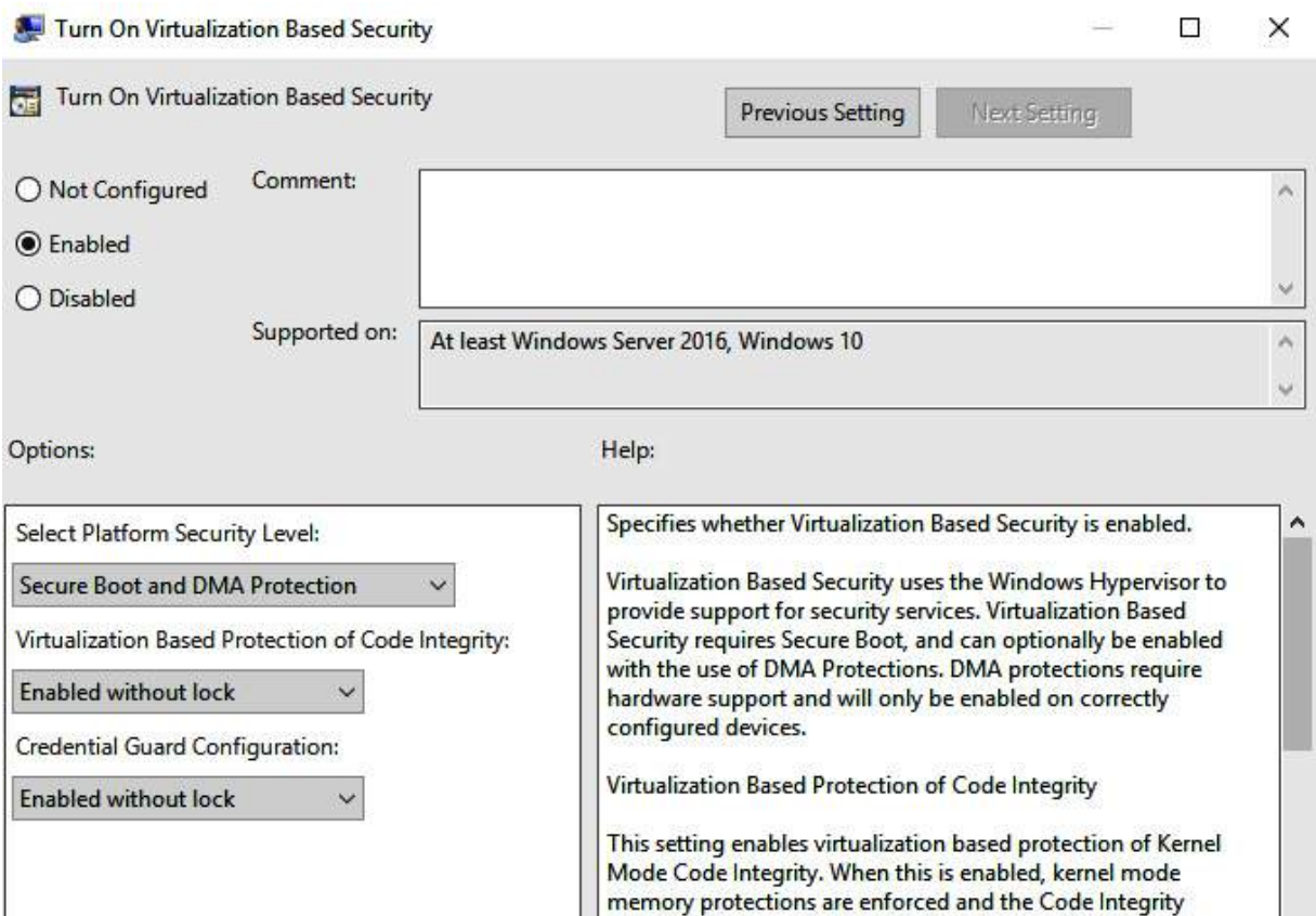
Figure 3.17 – Group Policy for HVCI and VBS features
