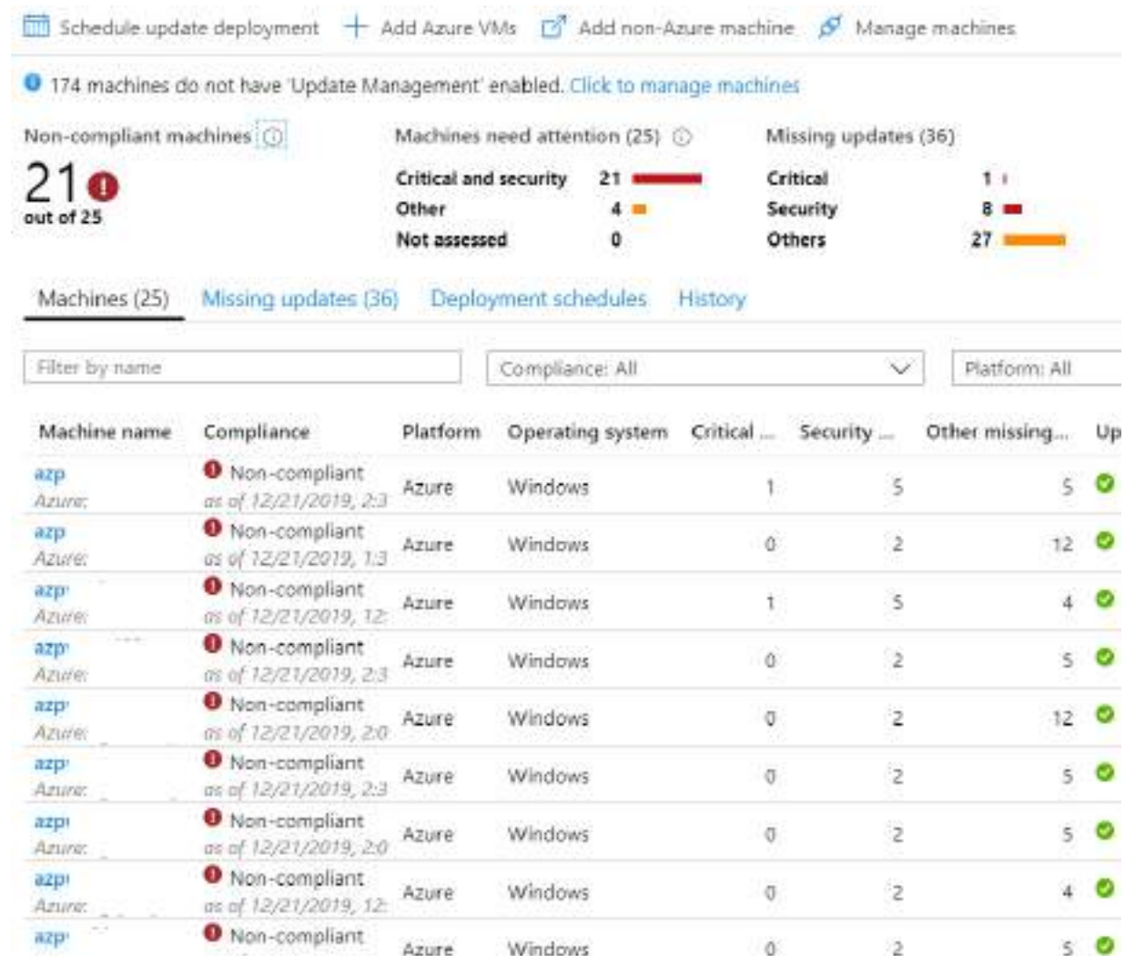
Figure 11.18 – Azure Automation Update Management
