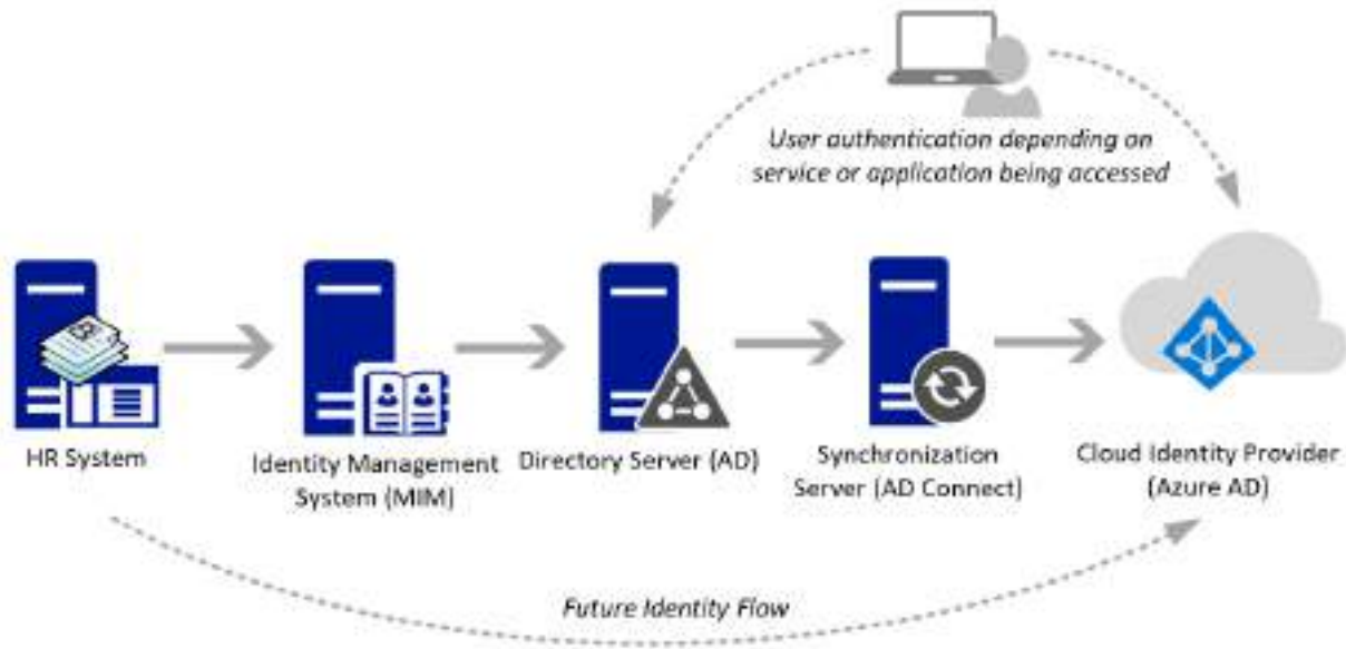
Figure 5.4 – The identity life cycle architecture example
