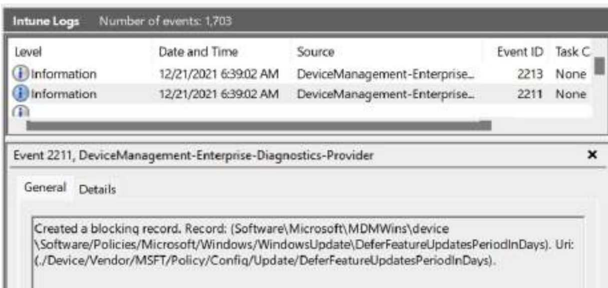
Figure 8.17 – MDM blocking record
