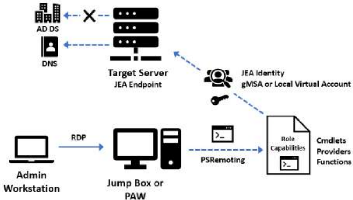
Figure 12.49 – Just Enough Administration
