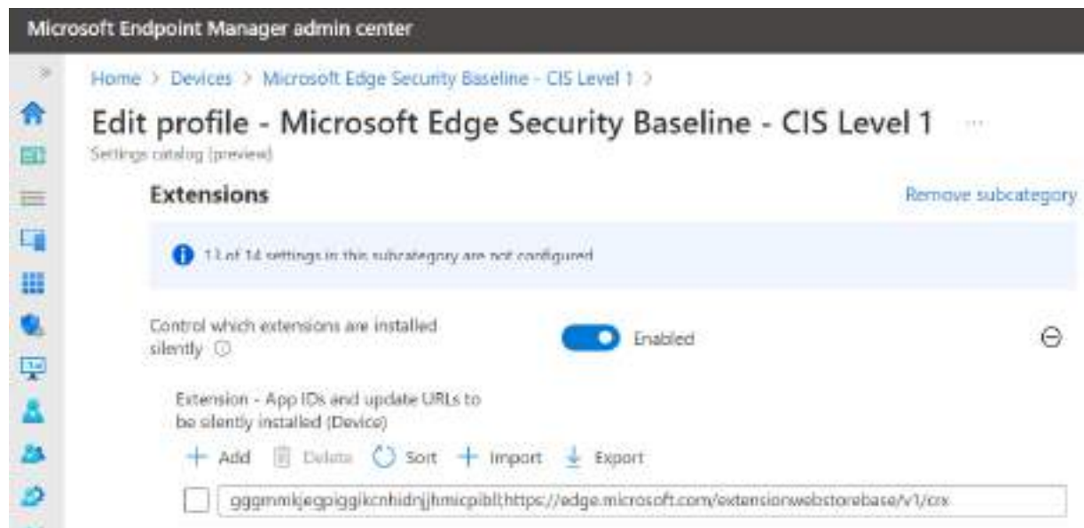
Figure 9.6 – Microsoft Edge extension policy
