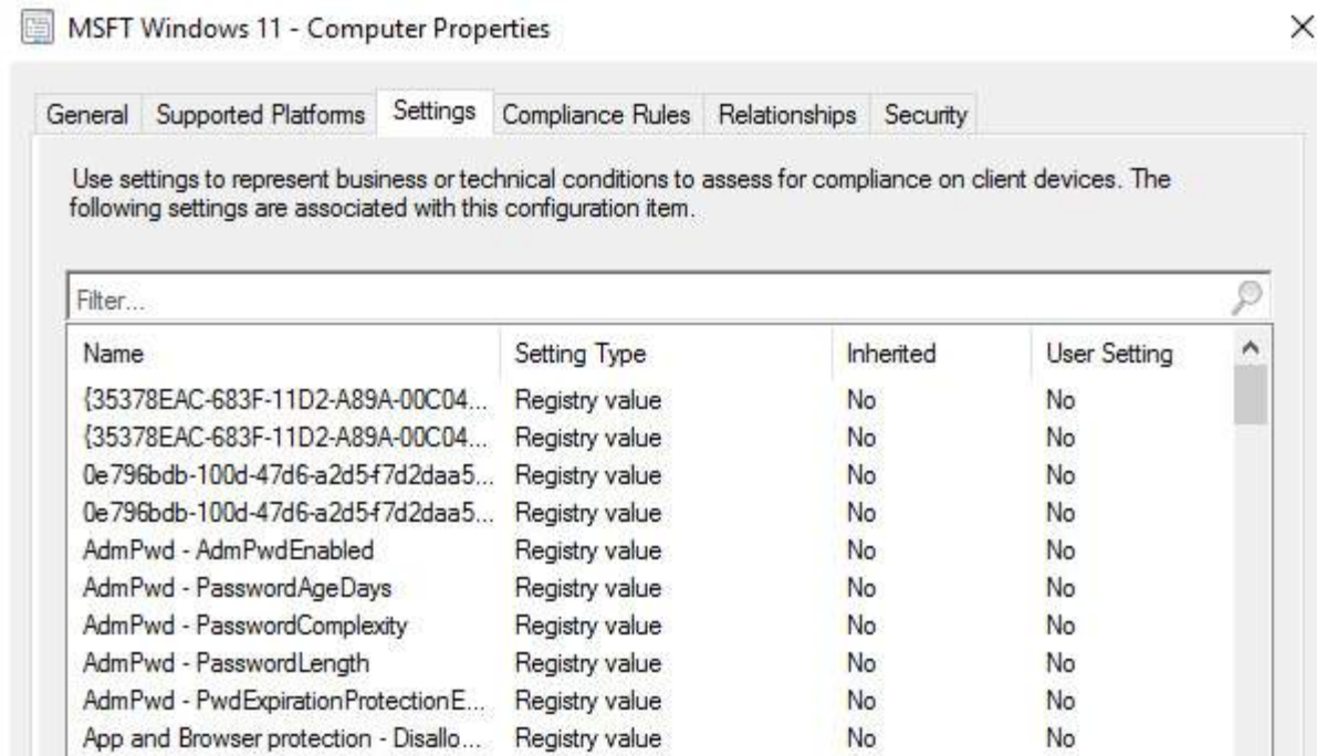
Figure 8.31 – The Settings tab of a Configuration Item
