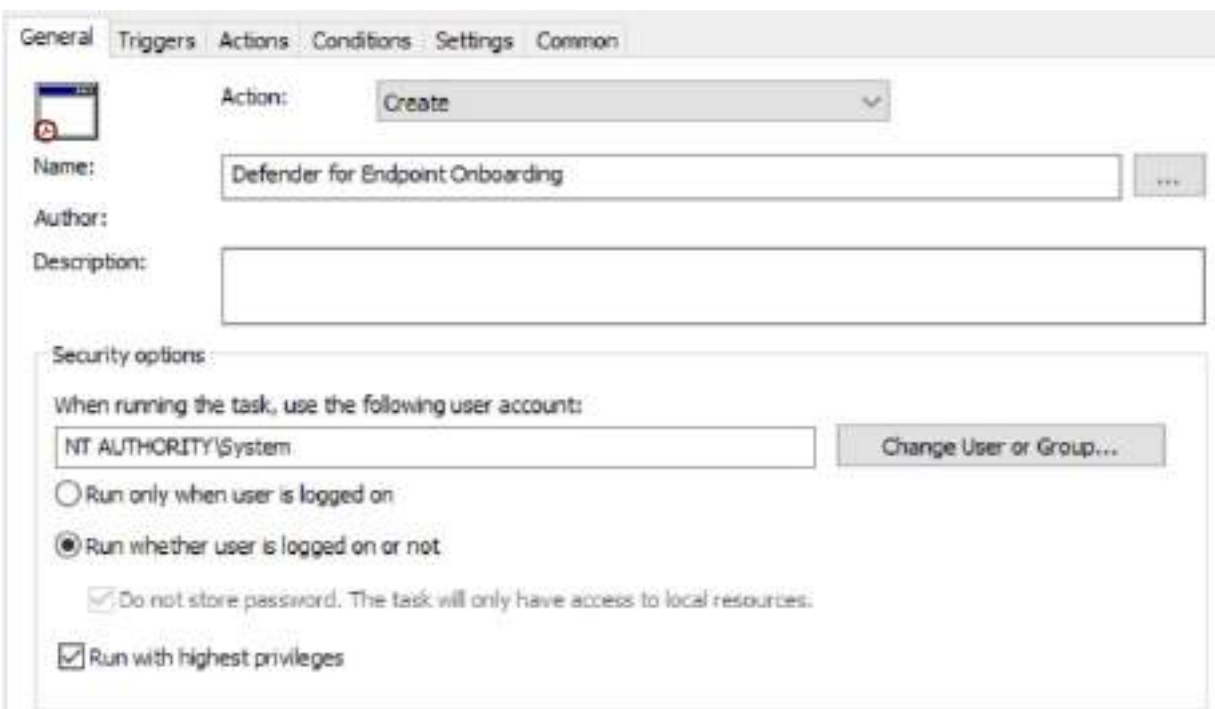
Figure 12.16 – Creating a scheduled task with Group Policy
