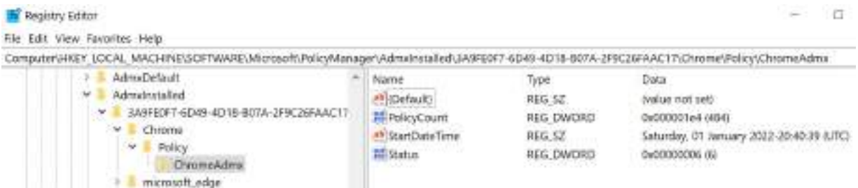
Figure 9.10 – ADMX ingested into the registry
