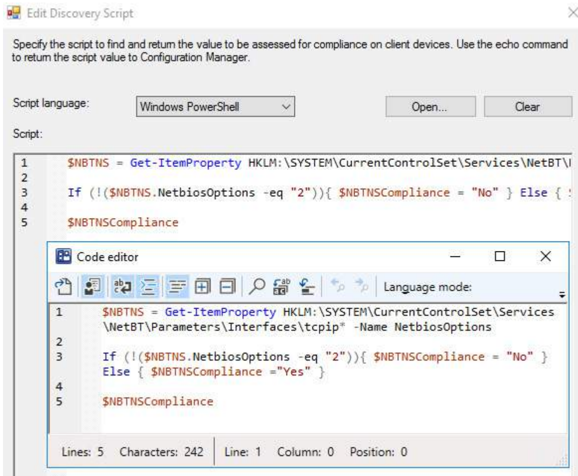
Figure 10.6 – Edit Discovery Script
