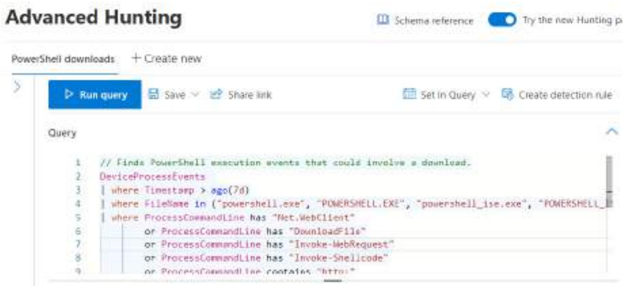
Figure 14.18 – Create detection rule
