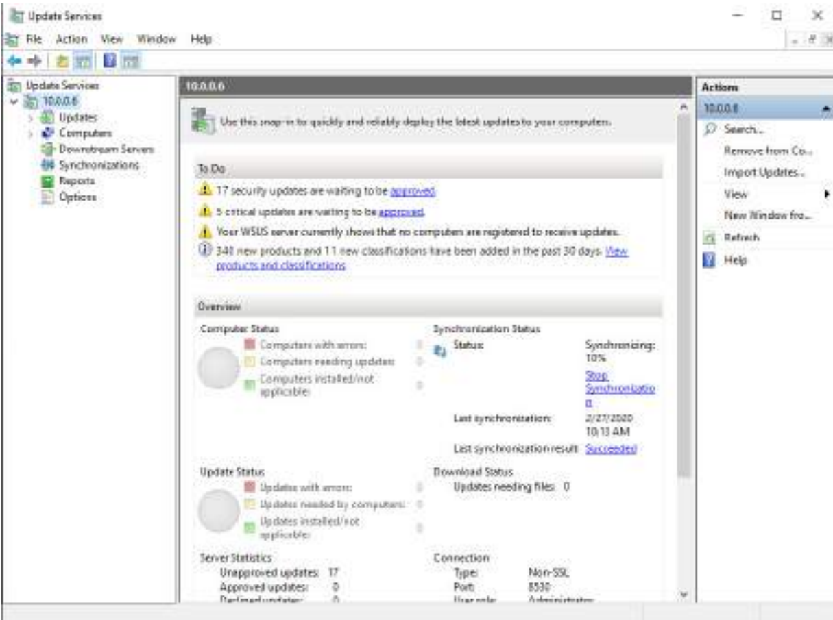
Figure 12.4 – WSUS management console
