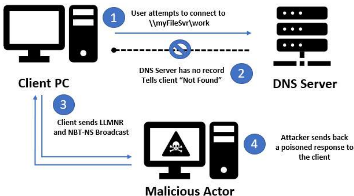
Figure 10.1 – Multicast response communication flow
