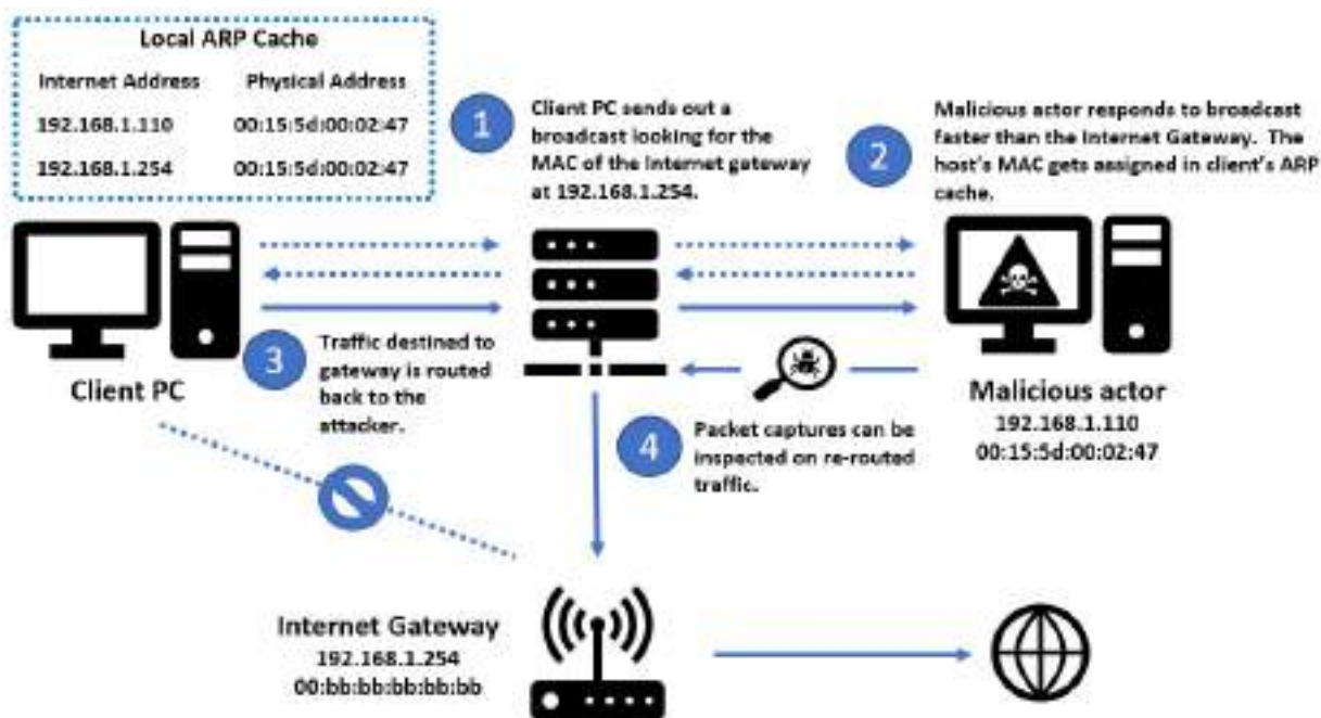
Figure 10.29 – ARP cache poisoning
