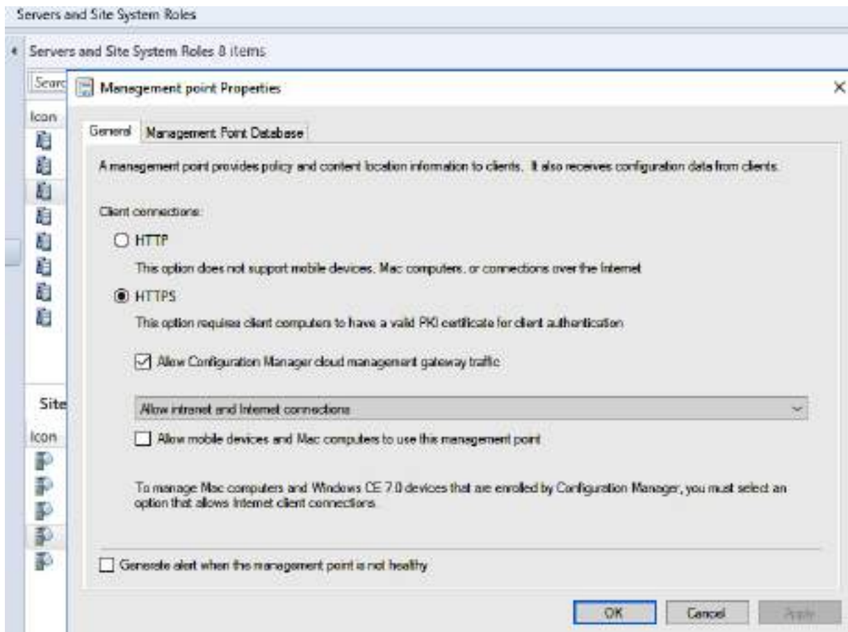
Figure 6.6 – MP client communication settings in Configuration Manager
