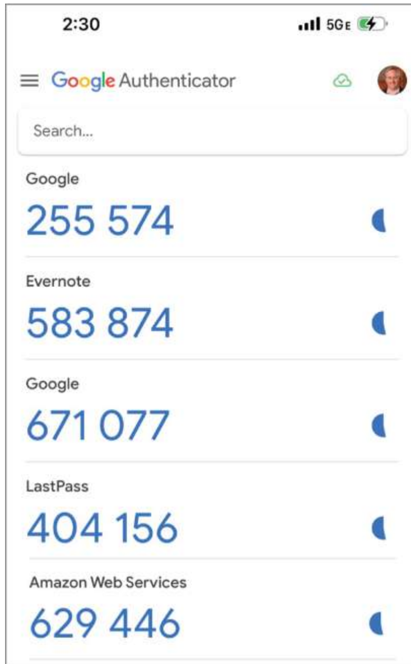
FIGURE 13.2 Software authenticator
