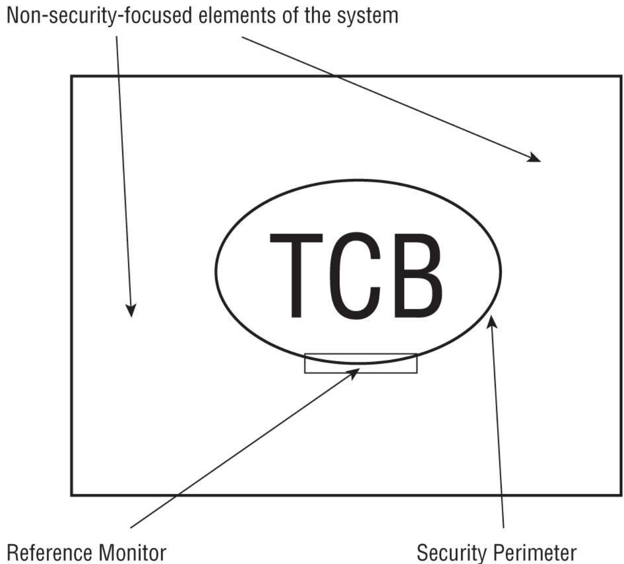
FIGURE 8.2 The TCB, security perimeter, and reference monitor
