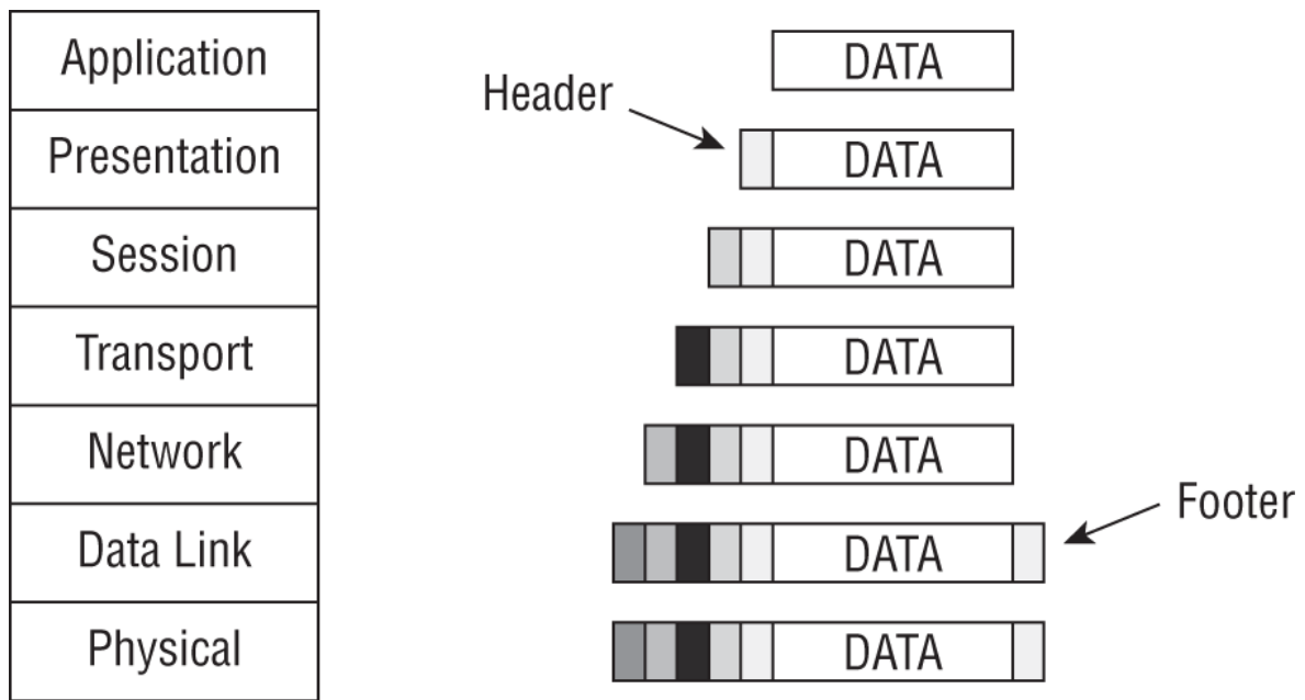
FIGURE 11.2 OSI model encapsulation
