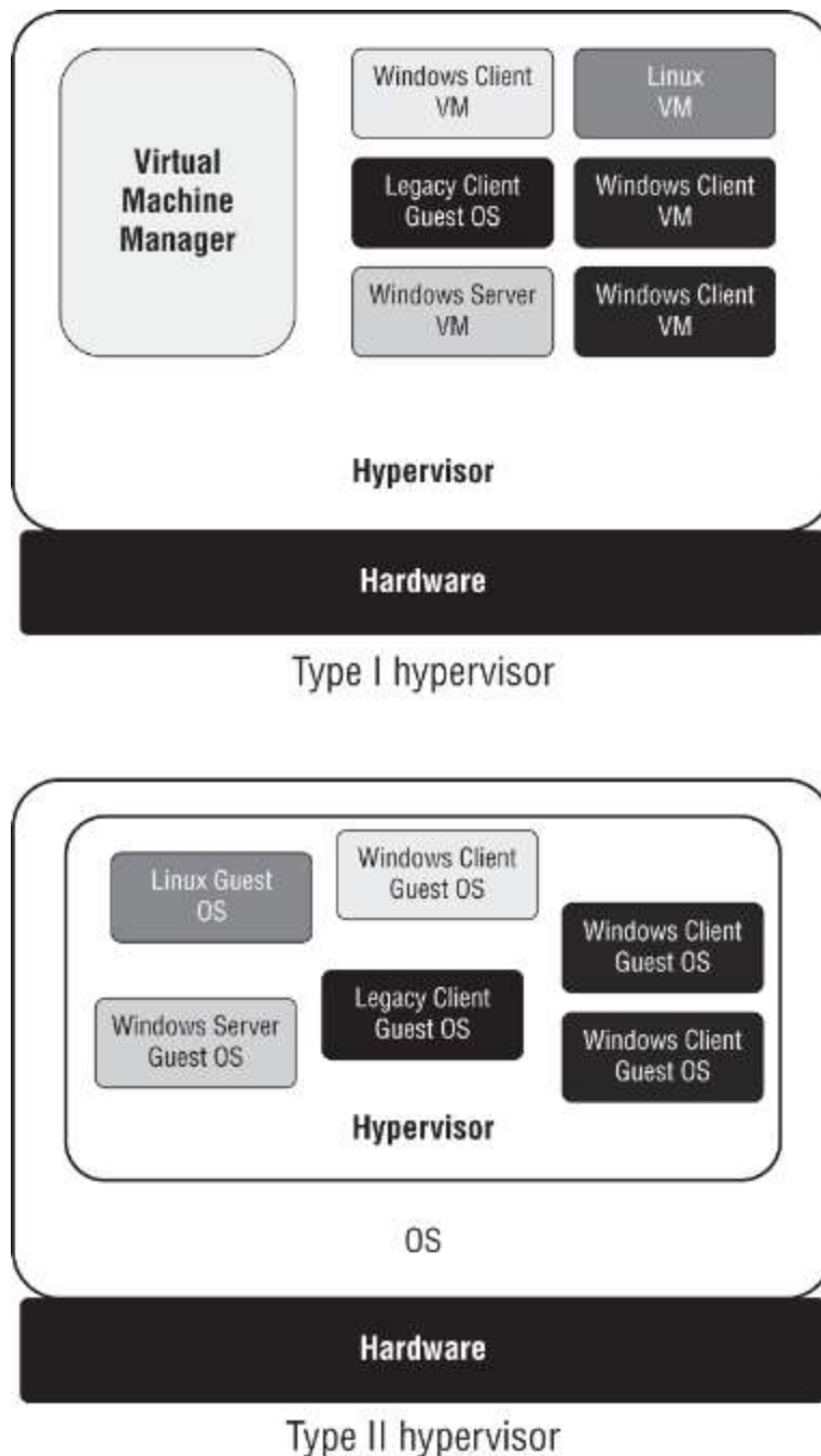
FIGURE 9.3 Types of hypervisors
