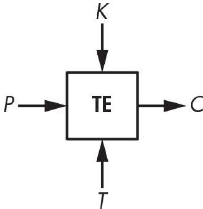
Figure 1-6: Tweakable encryption
