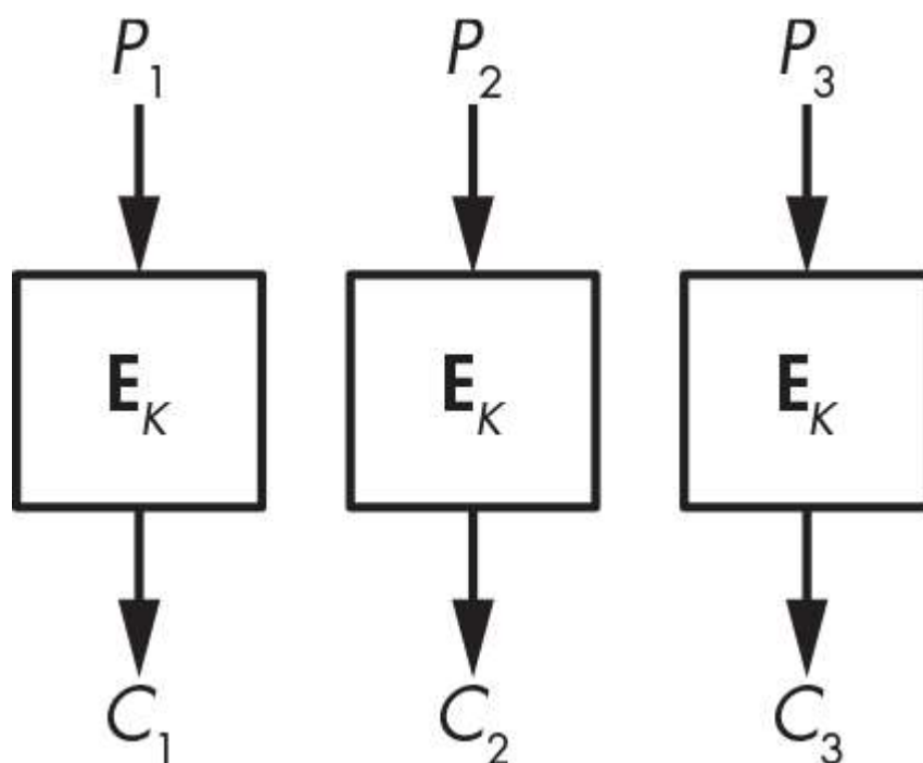
Figure 4-6: ECB mode
