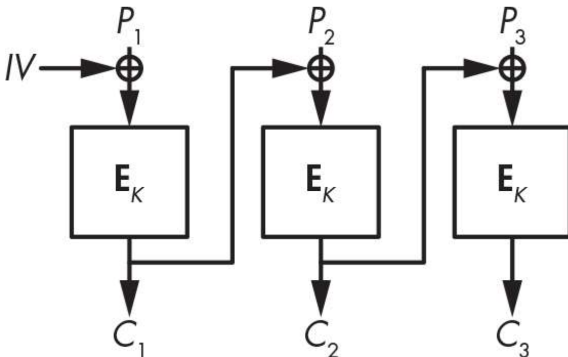
Figure 4-8: CBC mode
