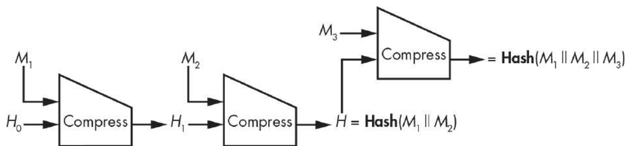
Figure 6-9: The length-extension attack
