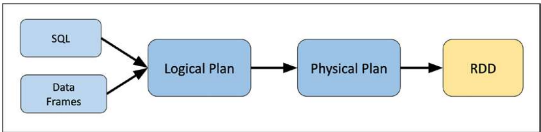
Figure 4-6. Catalyst optimizer
