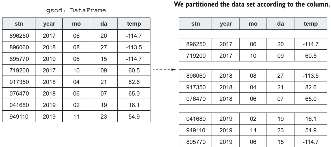
Figure 10.2 We partition the gsod data frame according to the year column and compute the minimum temperature for each partition. Each record belonging to the partition gets the minimum temperature appended. The resulting data frame contains the same number of records, but with a new column, min_temp , that contains the coldest temperature for the year.
