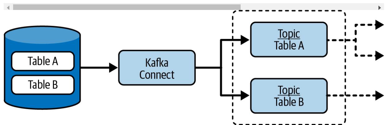
Figure 2-3. Debezium architecture in a nutshell, showing a Kafka Connect consumer leveraging the database commit logs and writing all matching datasets to dedicated Apache Kafka topics
