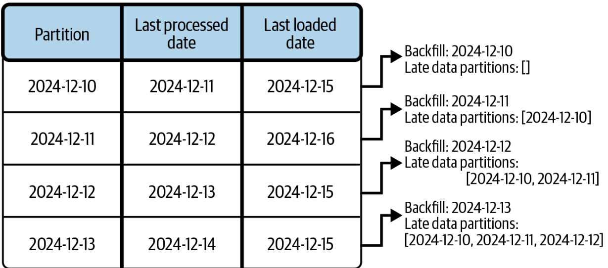
Figure 3-9. Late data integration concurrency problem
