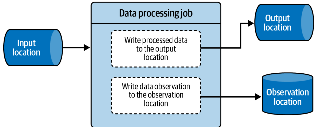
Figure 9-6. Online data observer for a streaming job
