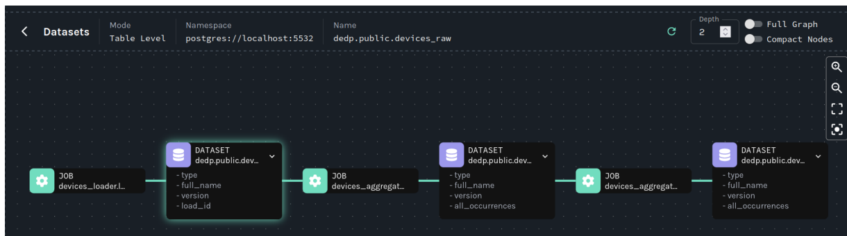
Figure 10-5. Apache Airflow DAG's lineage visualization in the Marquez UI
