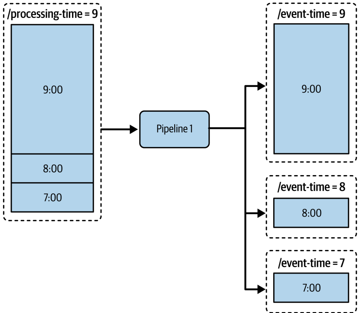
Figure 3-5. Shifting the late data problem
