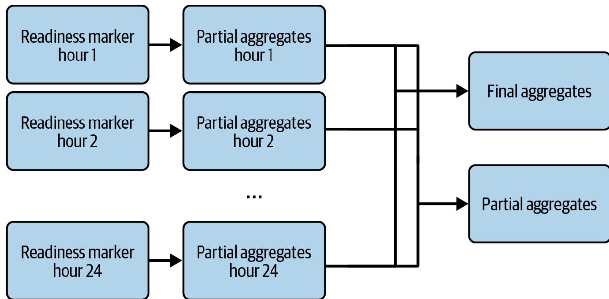
Figure 6-4. Confusing Unaligned Fan-In example
