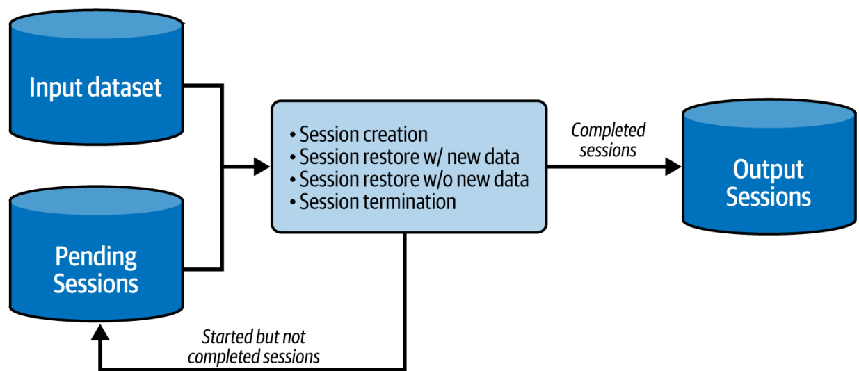
Figure 5-6. Incremental Sessionizer with three storage spaces
