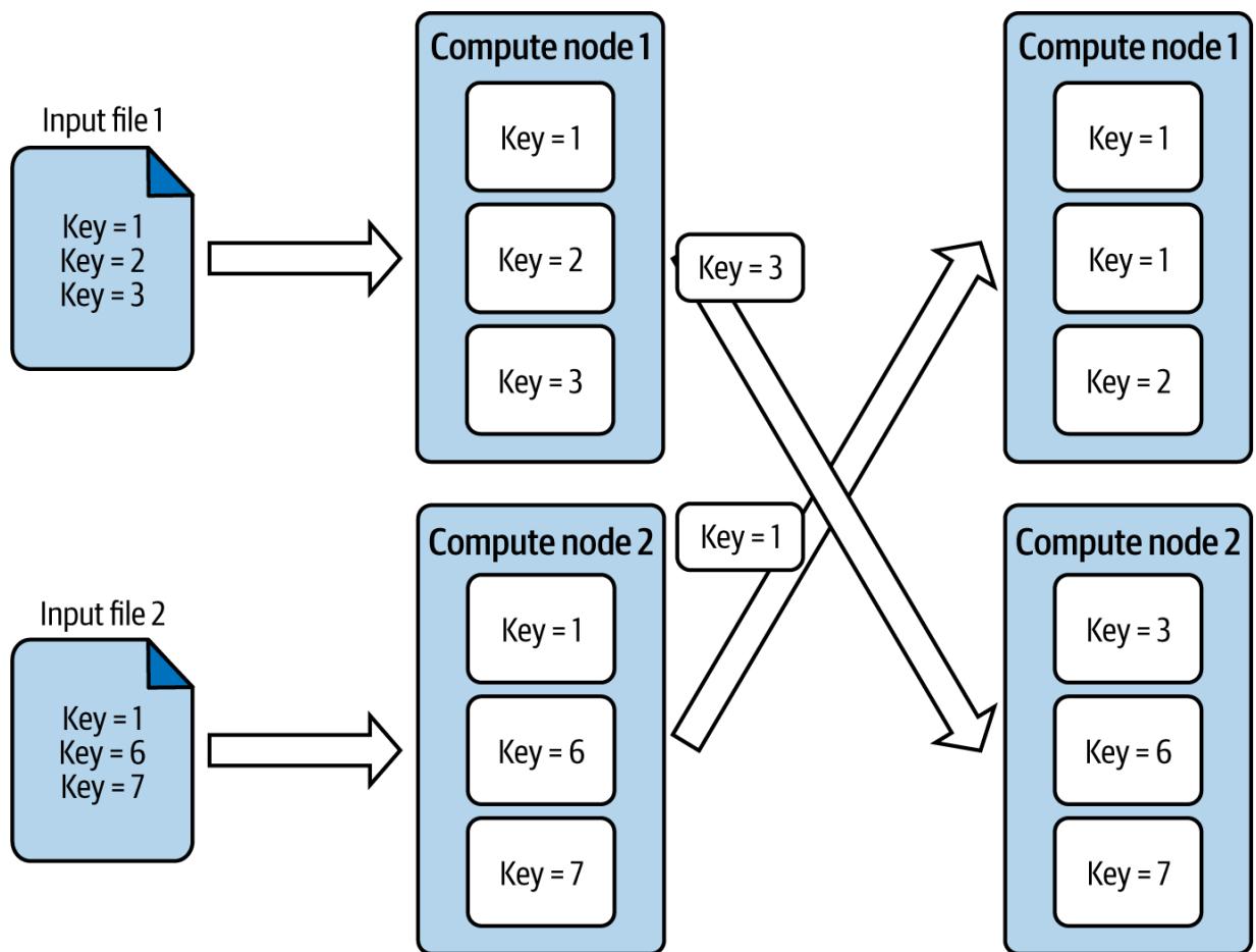
Figure 5-5. Data exchange in Distributed Aggregator
