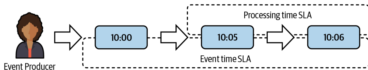
Figure 10-2. Processing time and event time SLAs illustrated
