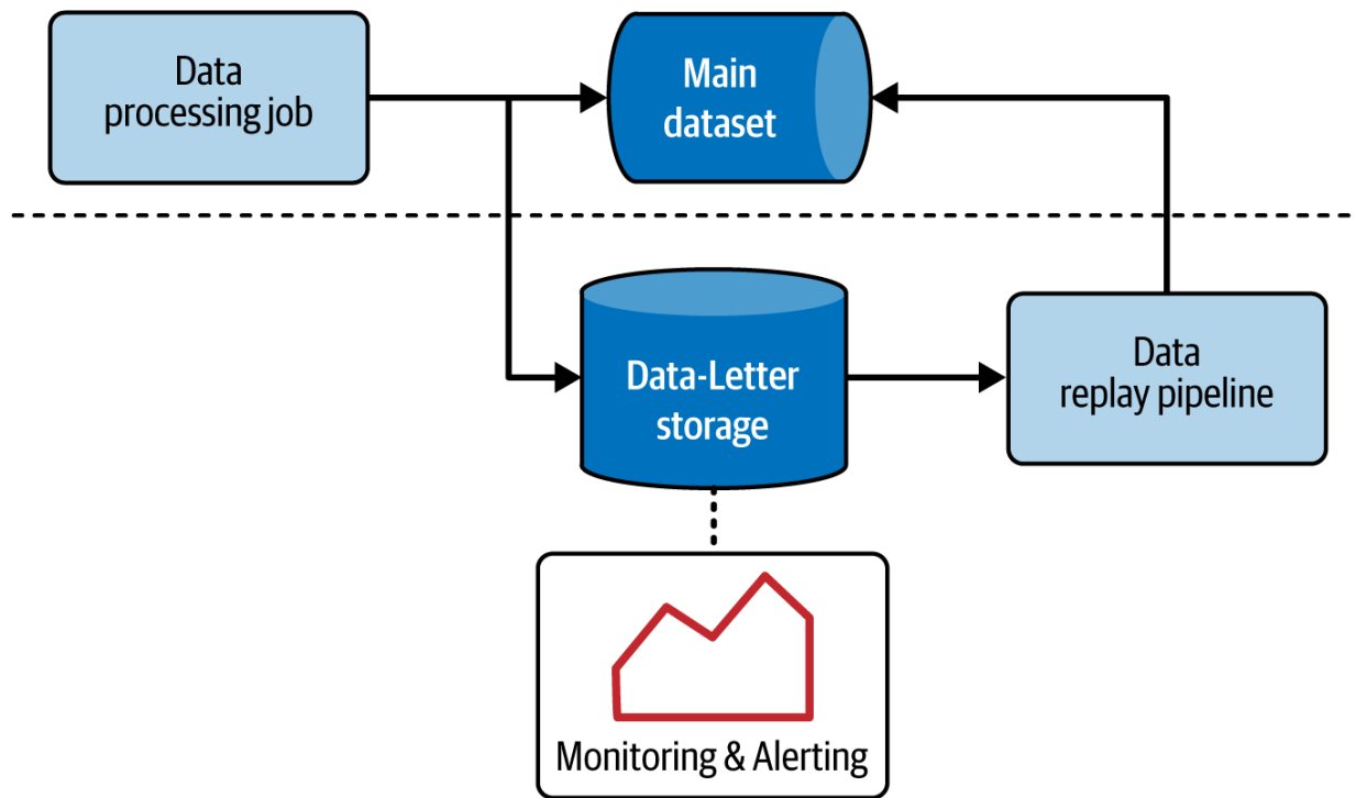
Figure 3-1. Components involved in the Dead-Letter pattern
