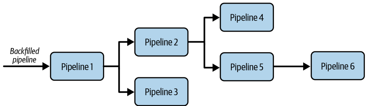
Figure 3-2. Snowball backfilling effect where backfilling Pipeline 1 triggers the same process for all downstream consumers
