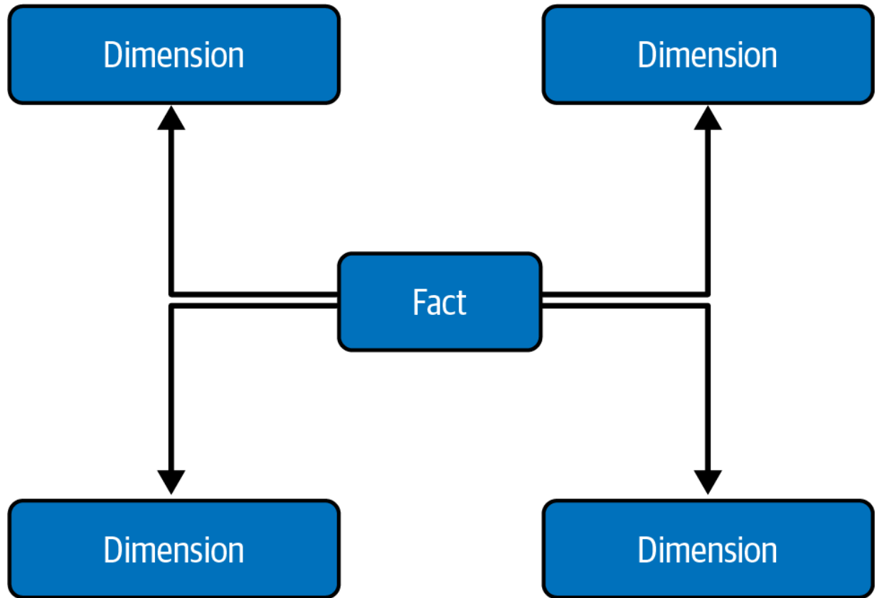
Figure 8-10. Star model with only one dimension table level
