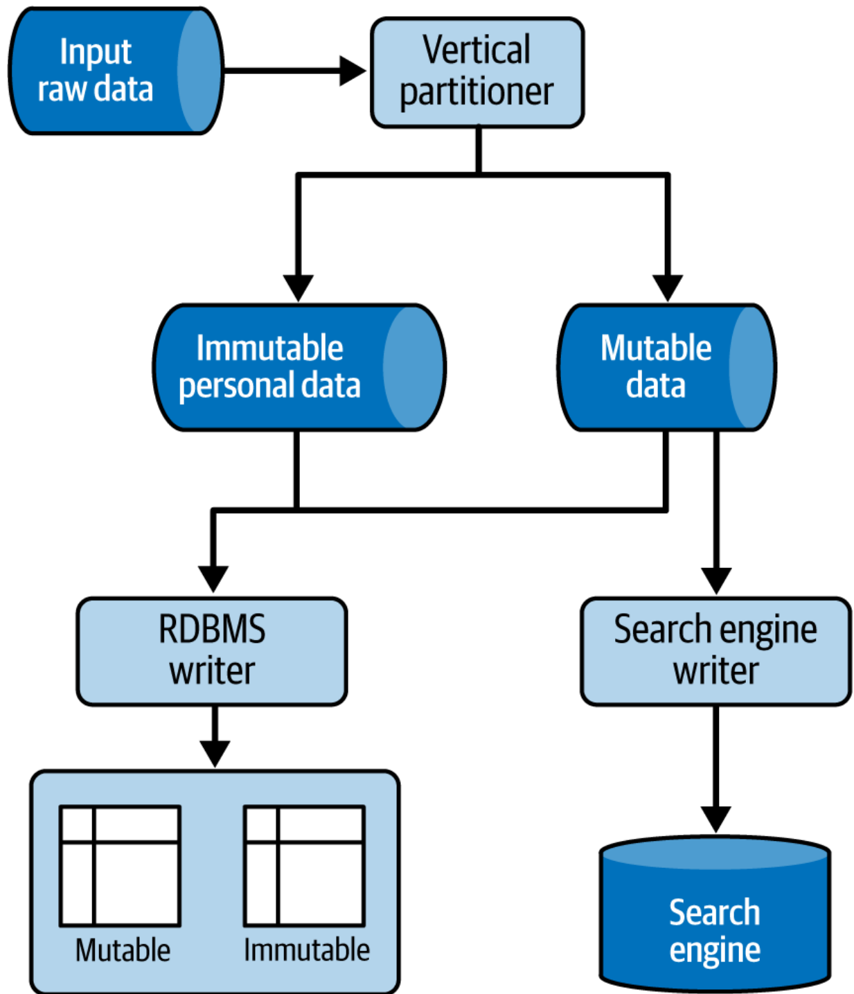
Figure 7-2. Polyglot persistence with vertical partitioning
