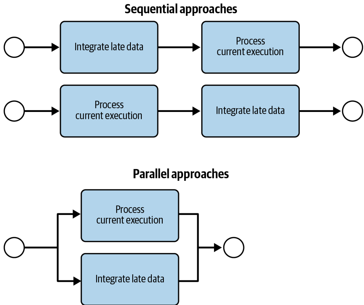
Figure 3-6. Strategies to include late data integration in pipelines
