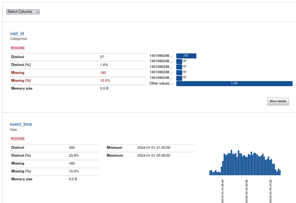
Figure 9-4. A data profile for the observed dataset
