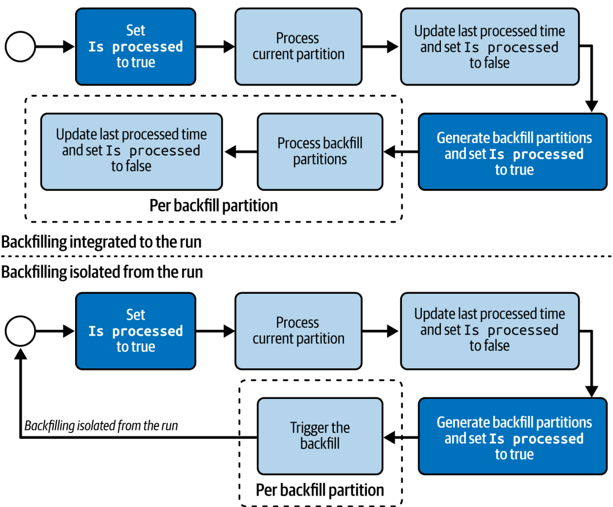
Figure 3-10. Late Data Integrator for concurrent pipelines
