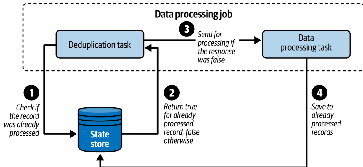
Figure 3-3. Windowed Deduplicator for a streaming job
