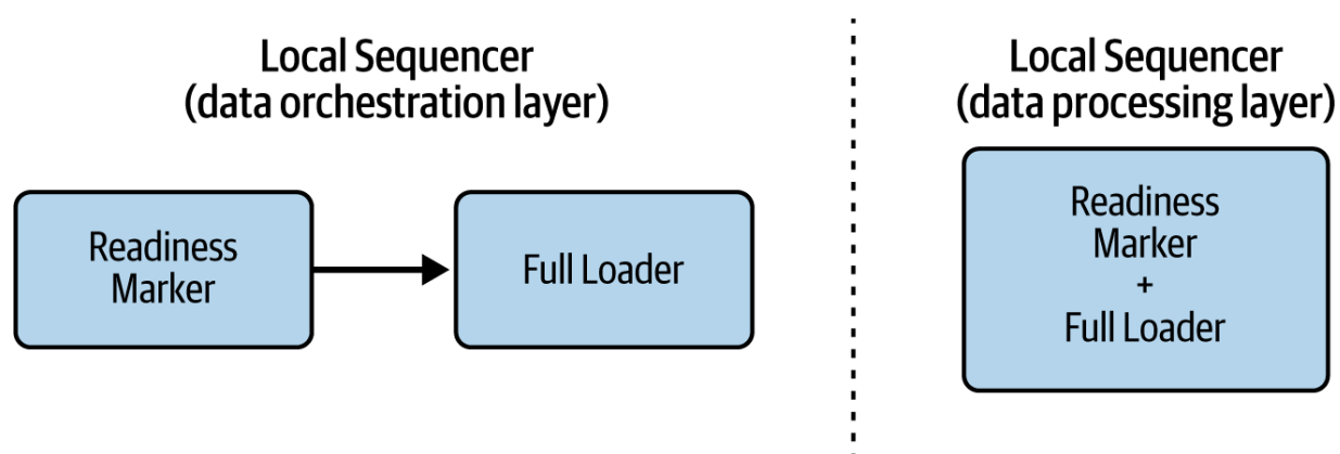
Figure 6-1. Local Sequencer versus single task
