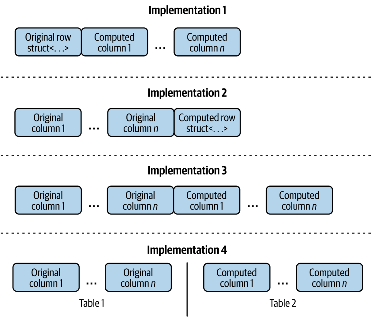
Figure 5-4. Possible Wrapper implementations for structured data
