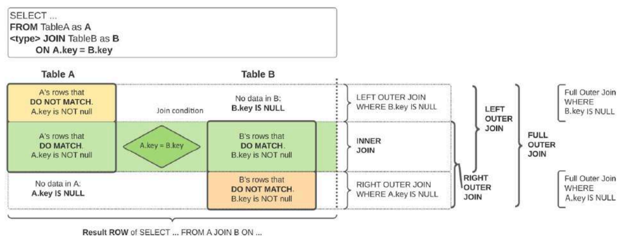
Figure 1.7: Visual representation of different JOIN types between tables A and B
