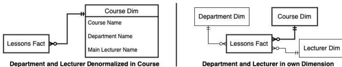
Figure 10.7: An alternative modeling of department and lecturer information
