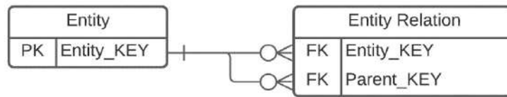
Figure 3.18: Many-to-many hierarchical relationship
