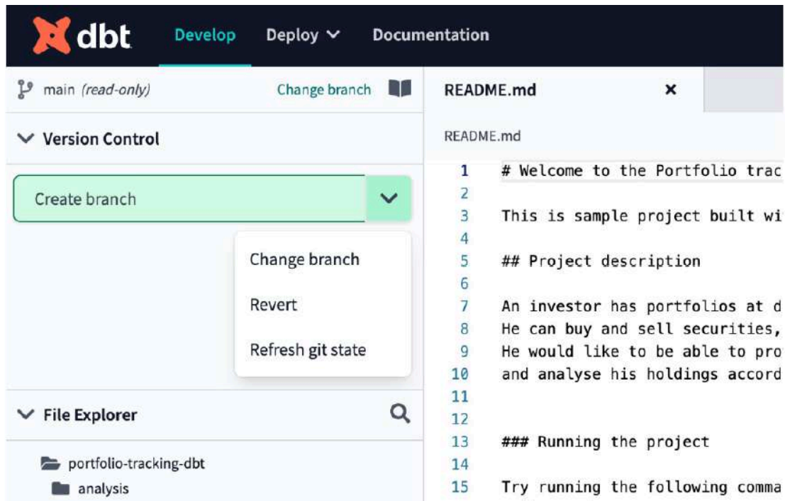
Figure 11.1: Available Git actions on the master branch
