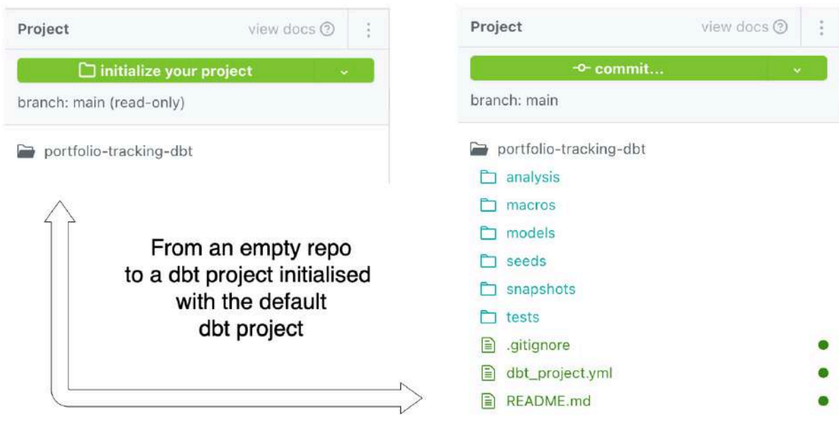
Figure 5.4: The dbt Cloud UI with the project content
