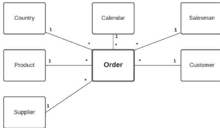
Figure 3.23: Example of a star schema
