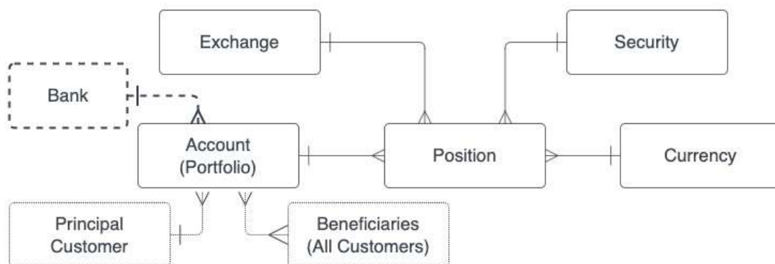
Figure 7.1: Conceptual data model of our sample project
