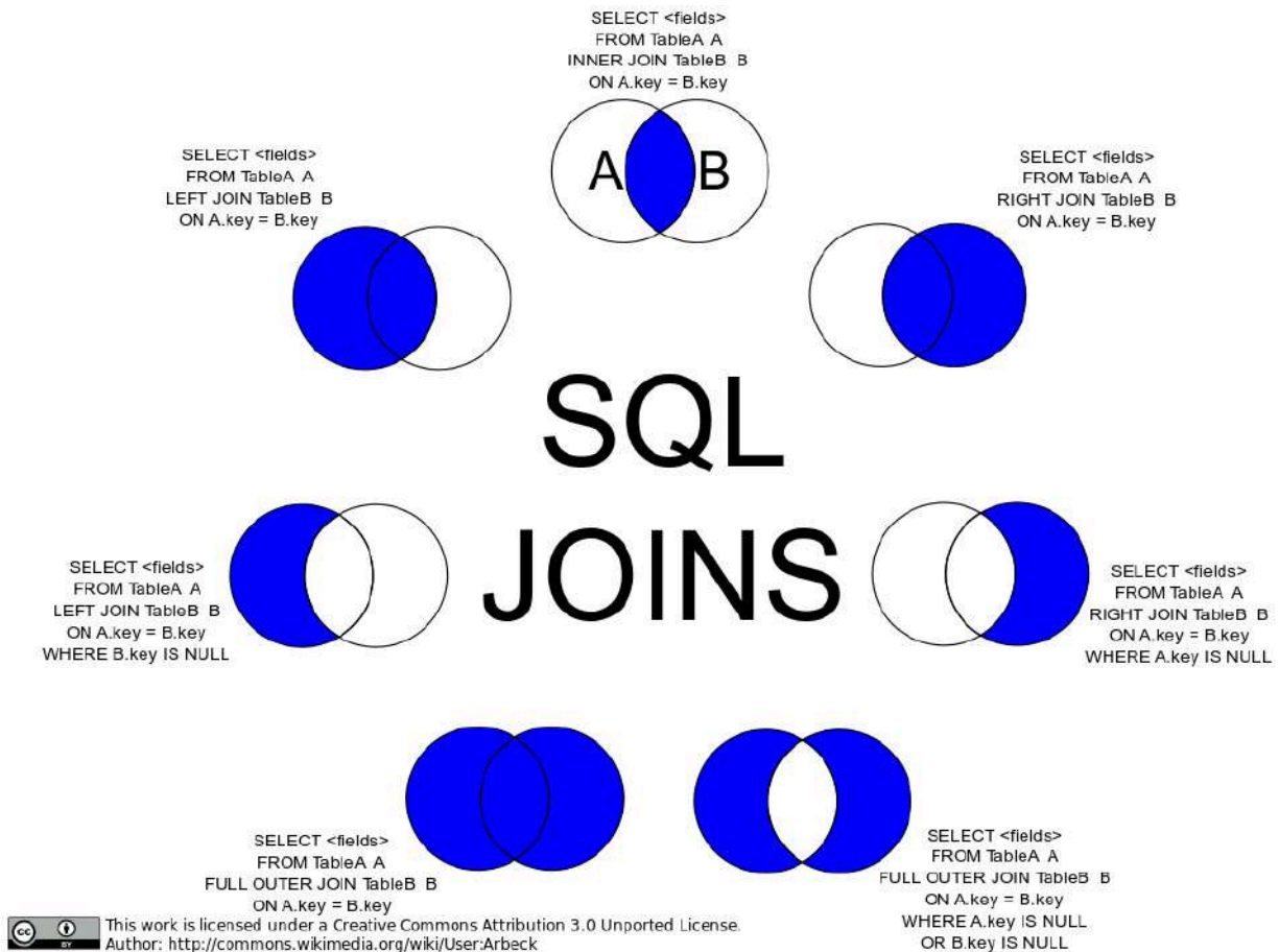
Figure 1.10: Visual representation of SQL JOIN types with an ON clause, as set operations
