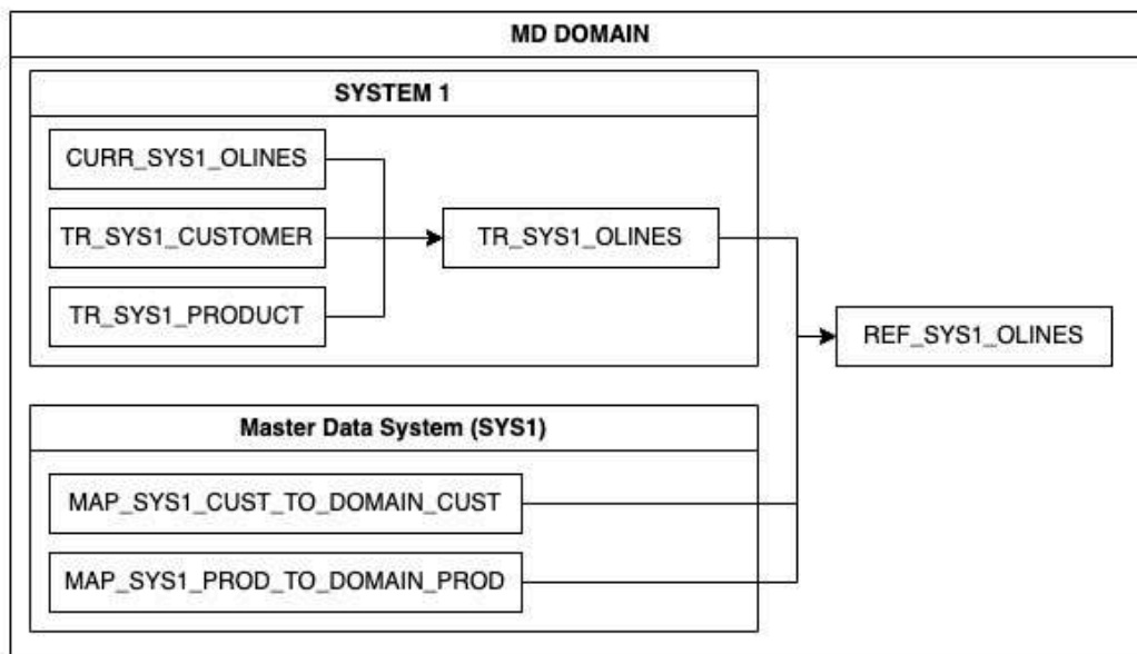
Figure 13.4: Transformations to apply MD when the source data uses surrogate keys
