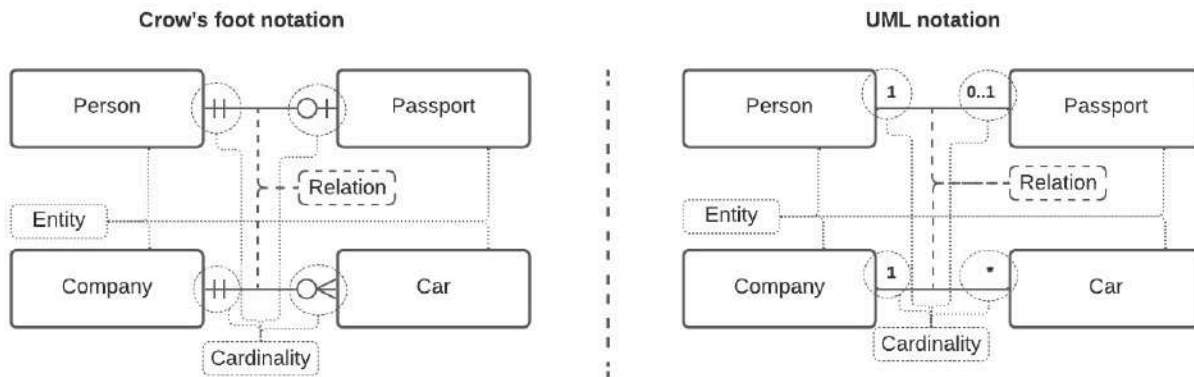
Figure 3.4: E-R notation basics
