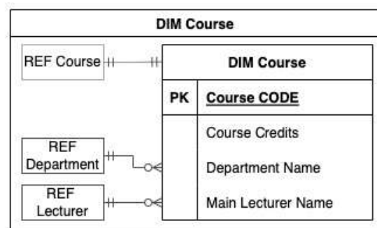
Figure 10.10: An example of an enriched dimension
