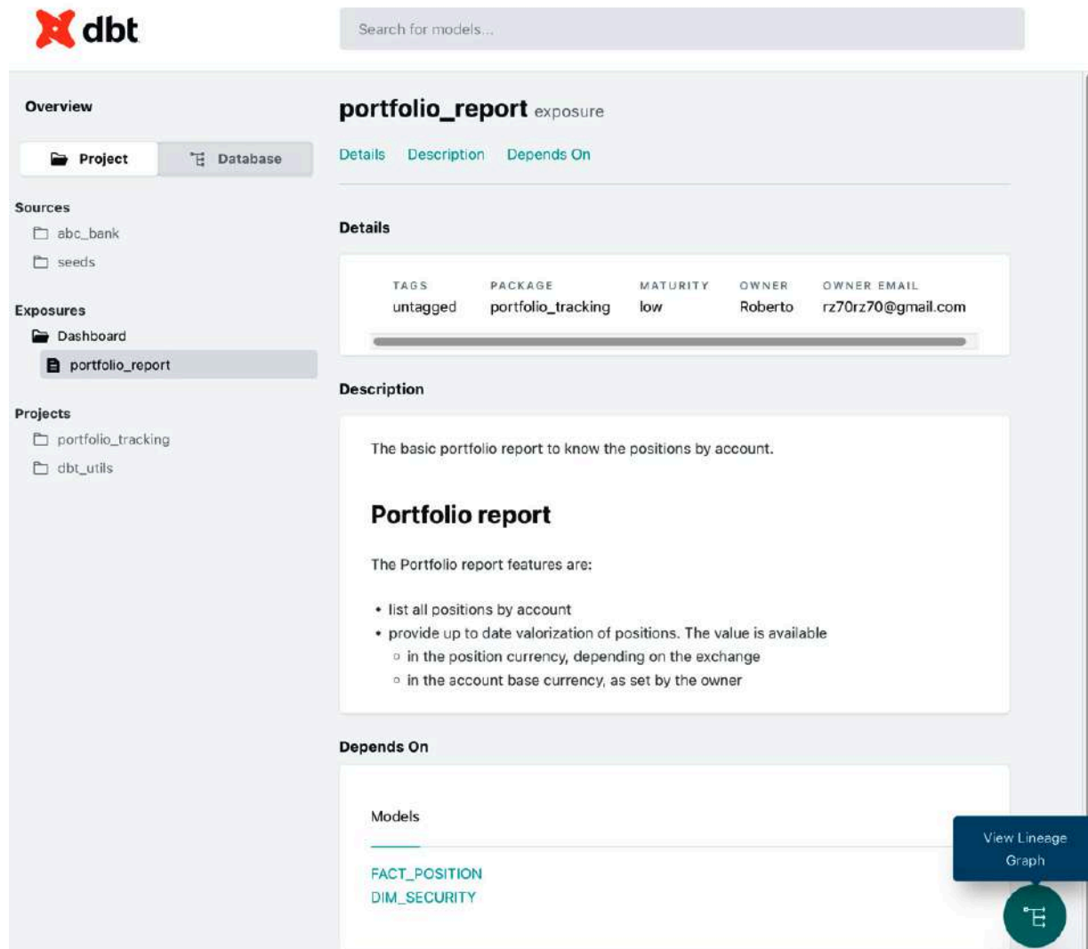
Figure 12.33: Generated documentation for an exposure
