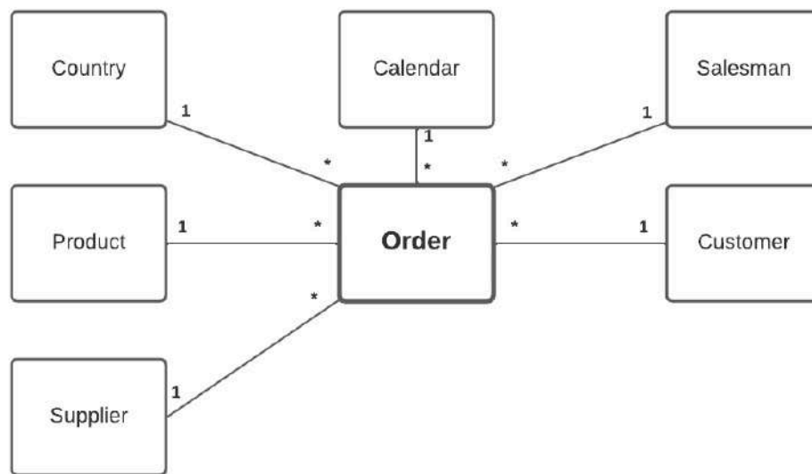
Figure 10.4: An example of a generic star schema
