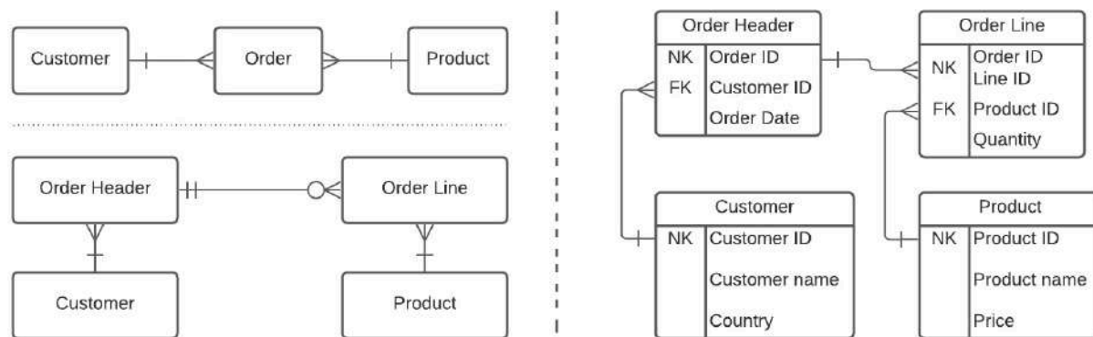
Figure 3.15: Different abstraction levels for an E-R model
