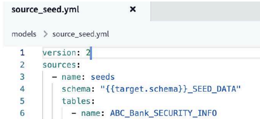
Figure 7.8: The definition of a source system to read our seed files
