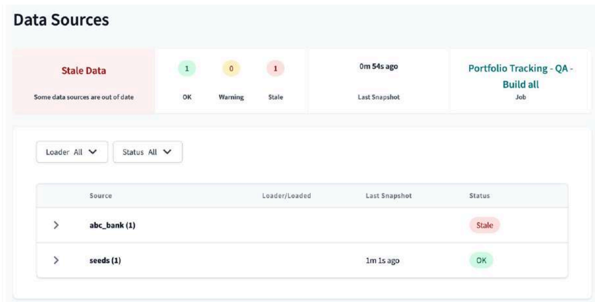
Figure 12.29: Data source freshness report, by system
