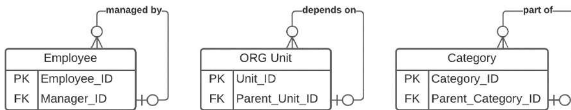
Figure 3.17: Examples of hierarchical relationships
