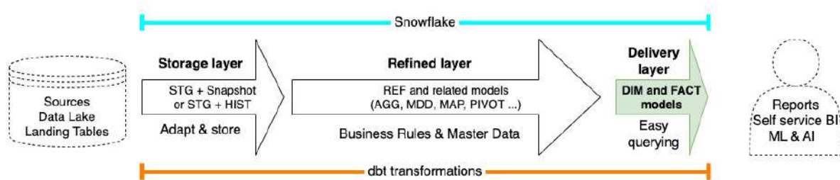
Figure 6.5: The delivery layer highlighted in the Pragmatic Data Platform
