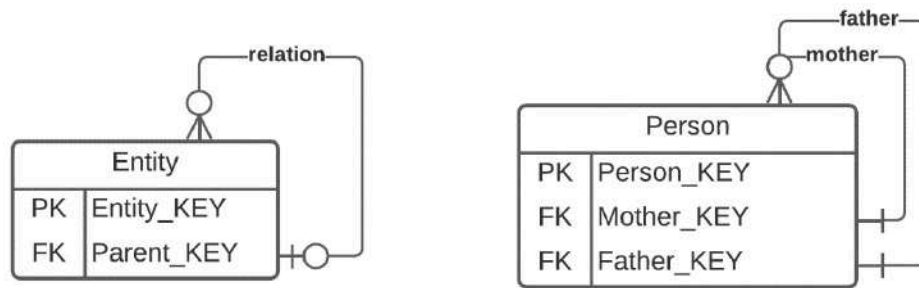
Figure 3.16: Single and multiple hierarchical relationships
