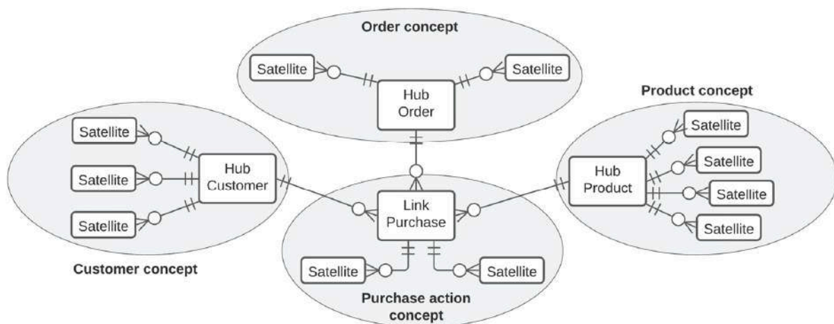
Figure 3.27: Example of a DV model
