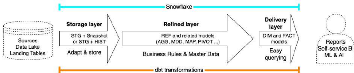
Figure 7.7: The layers of the Pragmatic Data Platform
