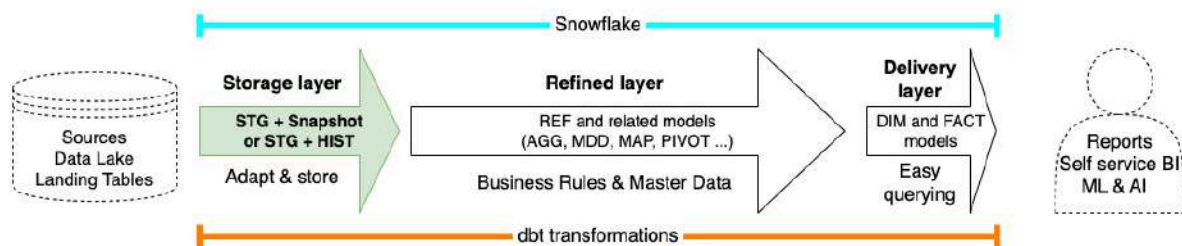
Figure 13.6: Storage layer highlighted in the context of the Pragmatic Data Platform
