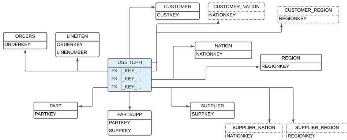
Figure 3.25: The star schema for the USS super fact of the TPCB database
