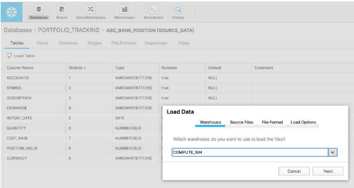
Figure 5.6: The Load Data wizard in Snowflake
