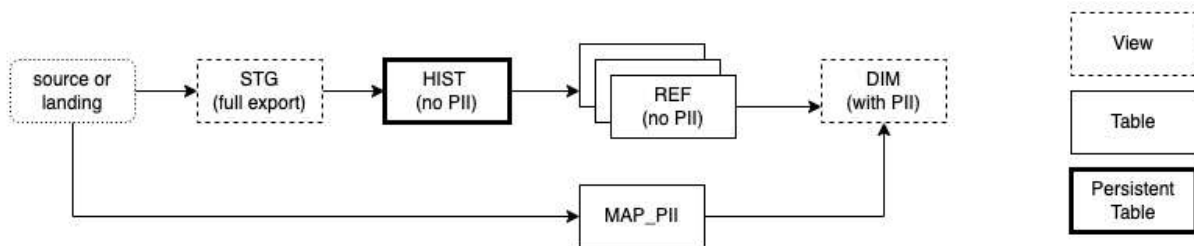
Figure 15.1: PII workflow for full exports
