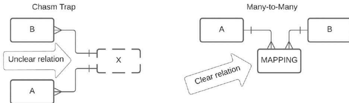
Figure 3.21: Chasm trap and a correct many-to-many relationship model
