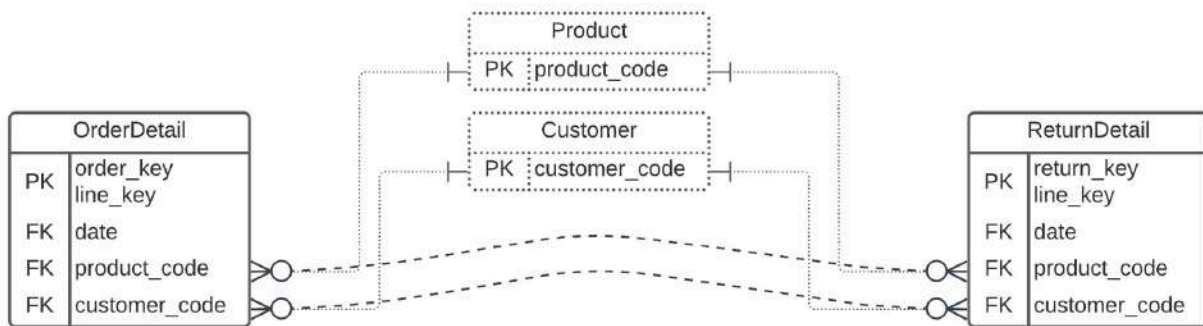
Figure 3.22: Example of chasm traps between facts with shared dimensions
