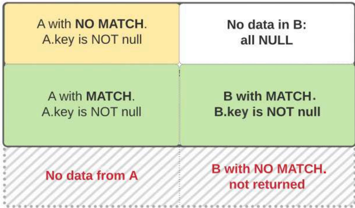
Figure 1.9: Visual representation of a LEFT OUTER JOIN
