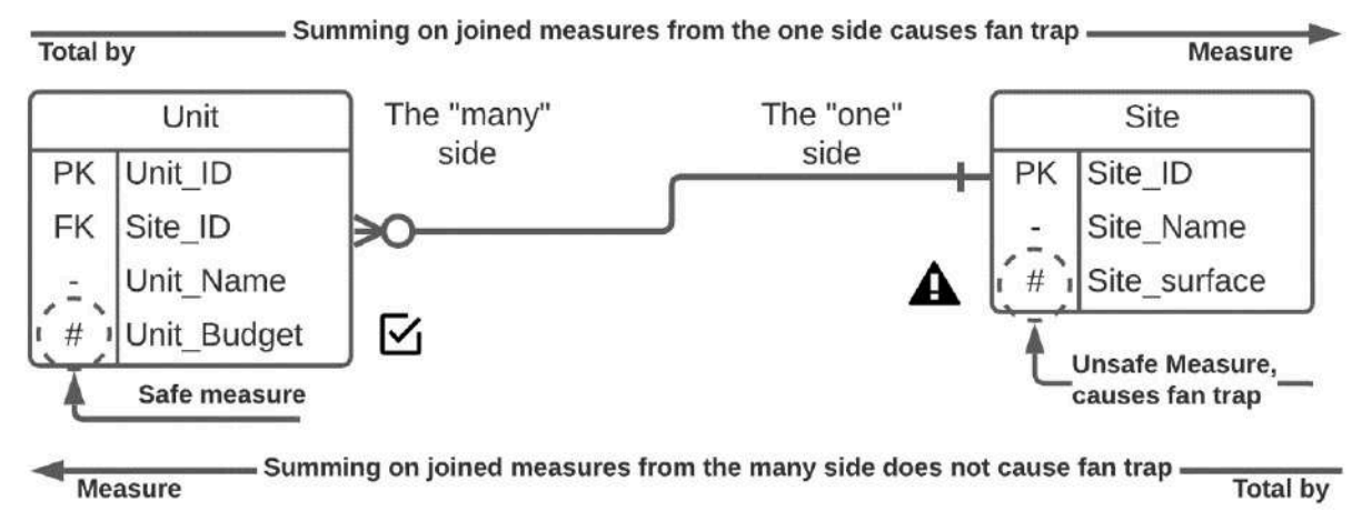
Figure 3.20: Data model with potential for a fan trap
