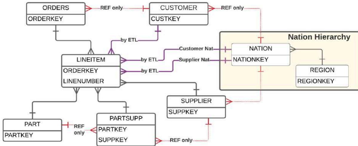
Figure 10.3: The lightweight data mart data model for TPCCH
