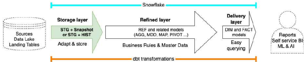
Figure 6.2: The staging layer highlighted in the Pragmatic Data Platform
