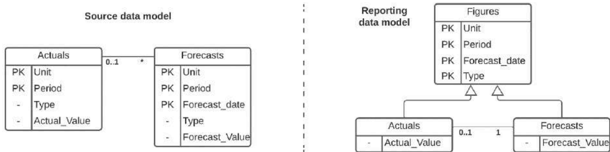
Figure 3.19: Data models for Actuals and Forecasts
