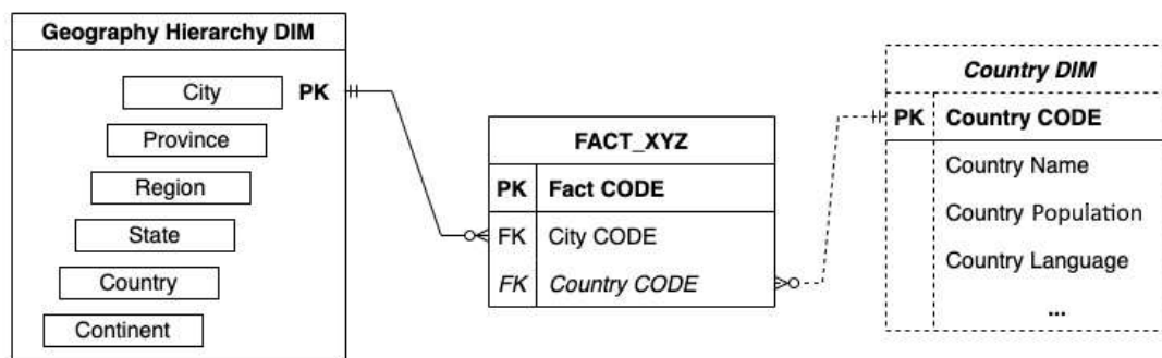
Figure 10.5: Hierarchical dimension modeling, with extra country dimension
