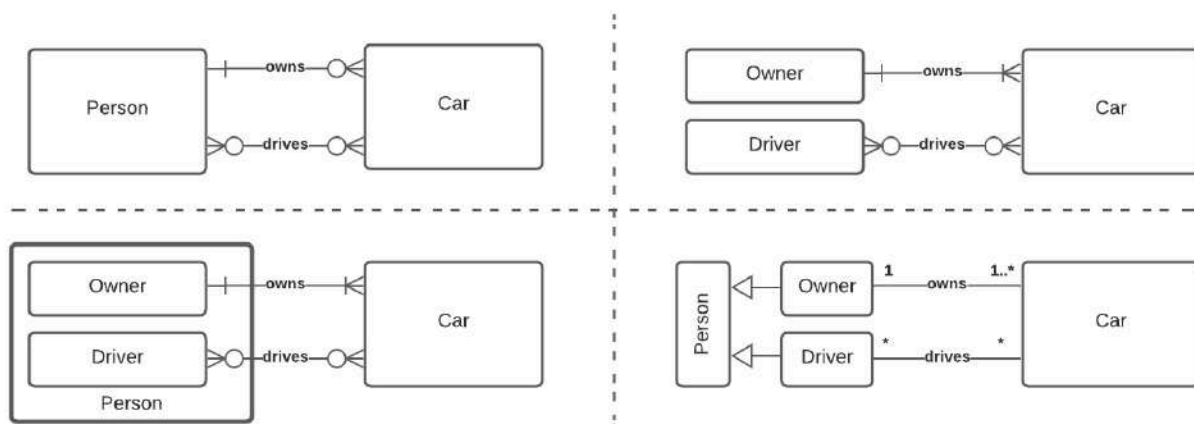
Figure 3.14: Different ways to express the same Person-Car model in E-R diagram models
