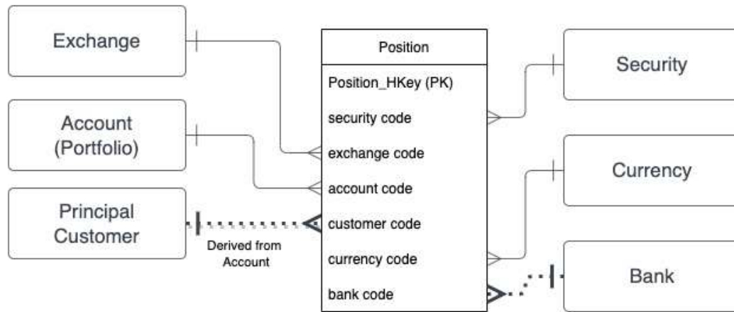
Figure 7.2: Star schema data model for our sample project
