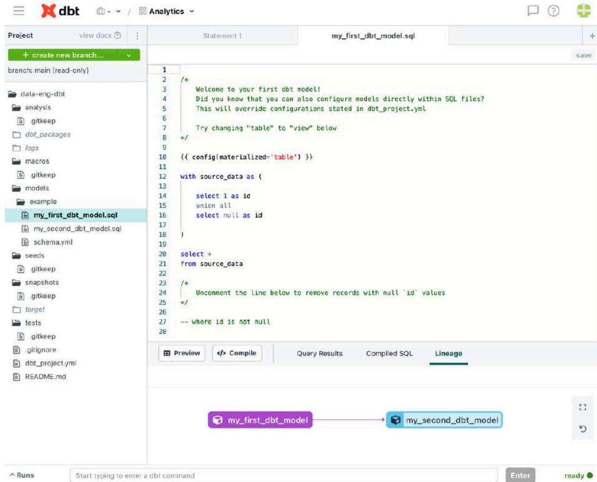
Figure 2.33: dbt IDE open for editing a SQL file
