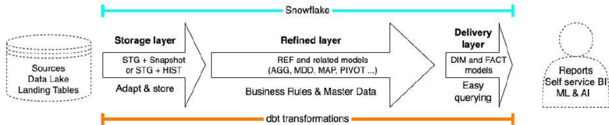
Figure 7.10: The layers of the Pragmatic Data Platform
