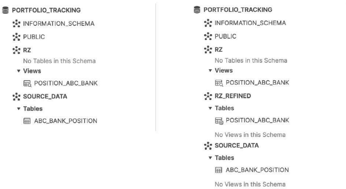
Figure 5.11: The content of our Snowflake database before and after re-running the project
