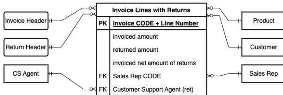
Figure 10.8: The data mart for invoices with returns
