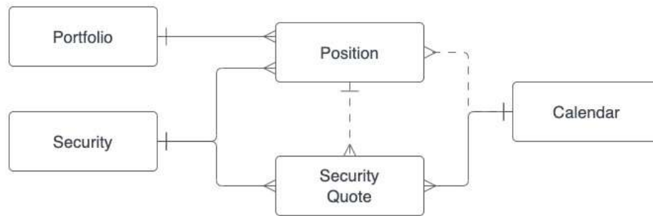
Figure 5.3: The initial data model for the portfolio tracking project
