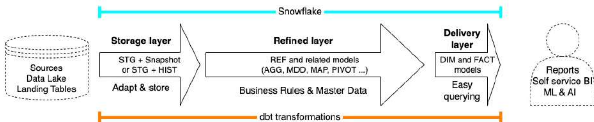
Figure 6.1: The layers that make up the Pragmatic Data Platform
