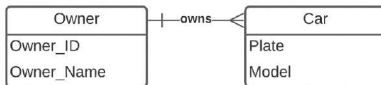
Figure 3.1: A sample E-R diagram
