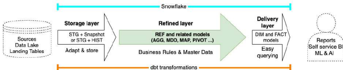
Figure 6.4: The refined layer highlighted in the Pragmatic Data Platform
