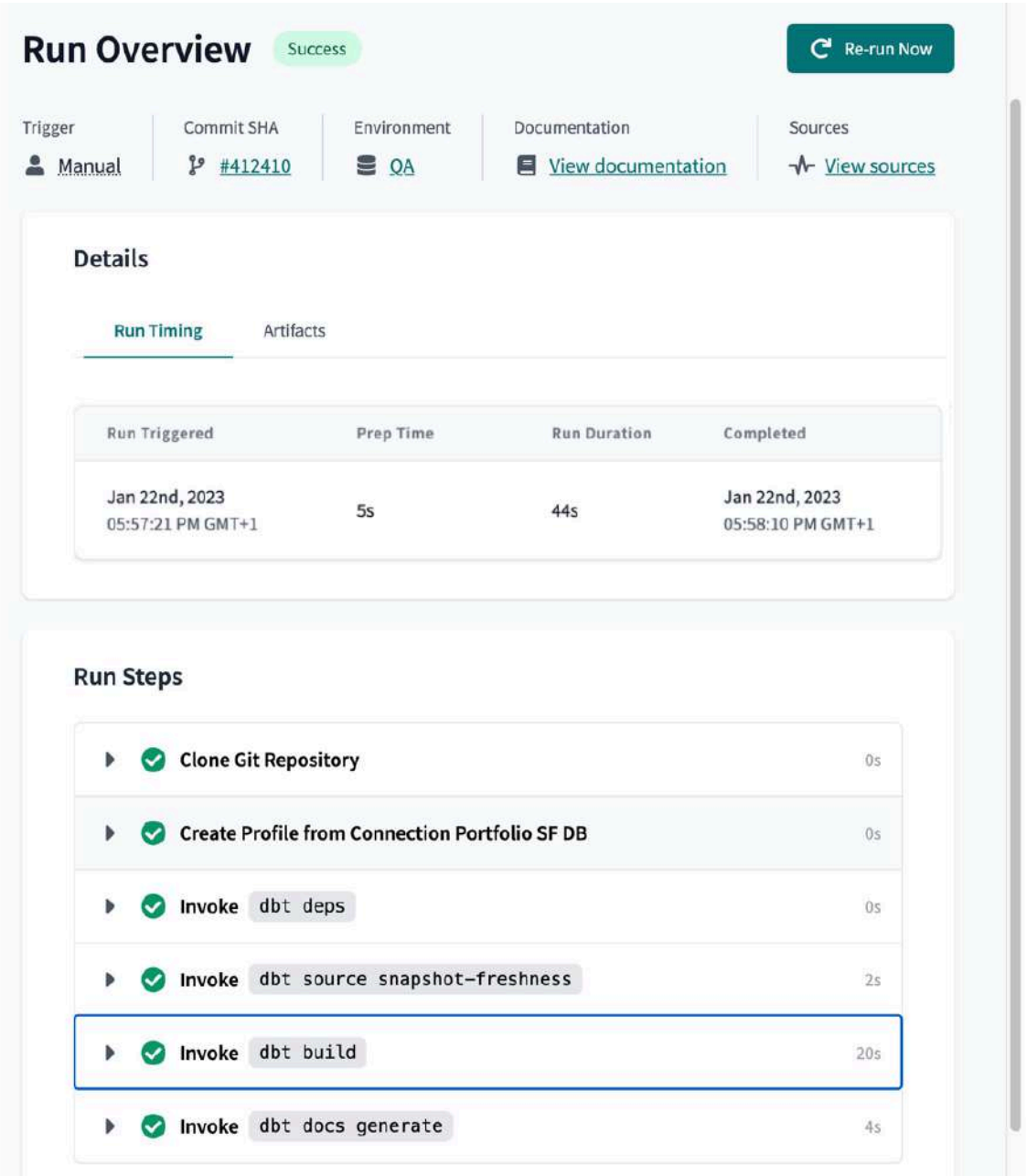
Figure 12.15: A job's Run Overview page
