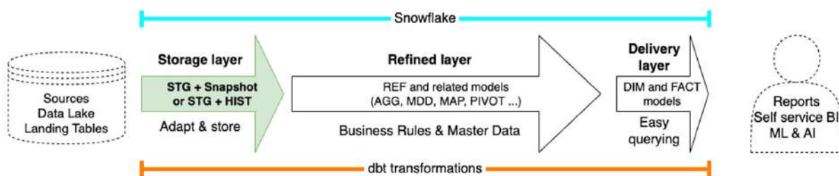
Figure 6.6: The storage layer highlighted in the Pragmatic Data Platform
