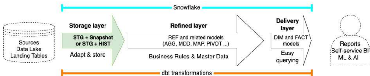
Figure 7.9: The storage layer highlighted in the Pragmatic Data Platform
