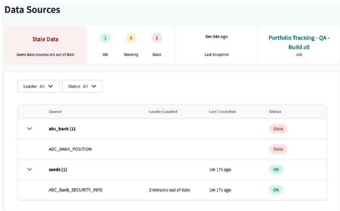
Figure 12.30: The freshness report per system
