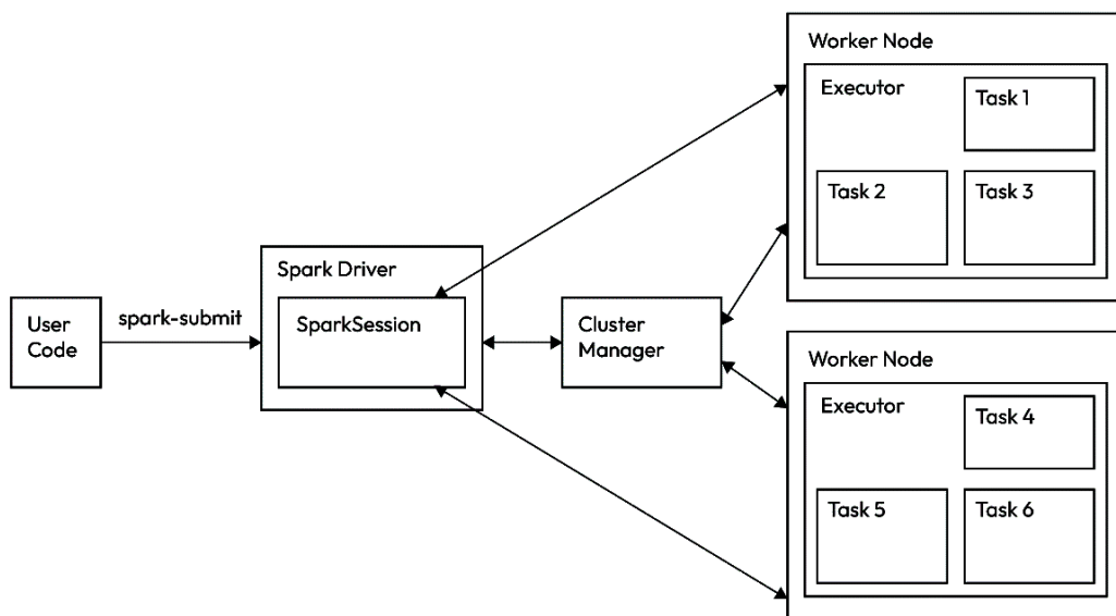
Figure 3.1: Spark architecture
