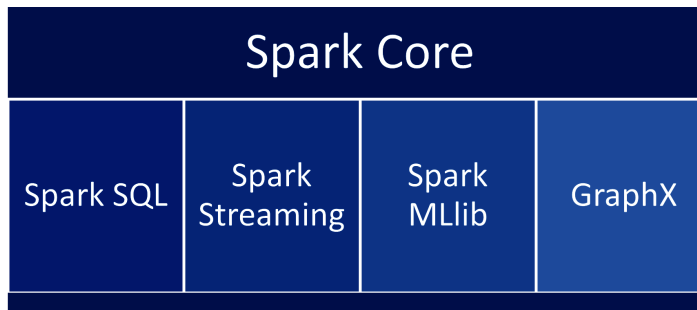
Figure 2.1: Spark components
