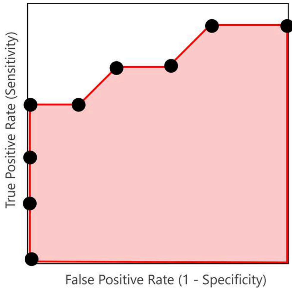
Figure 6-20. A receiver operator characteristic curve
