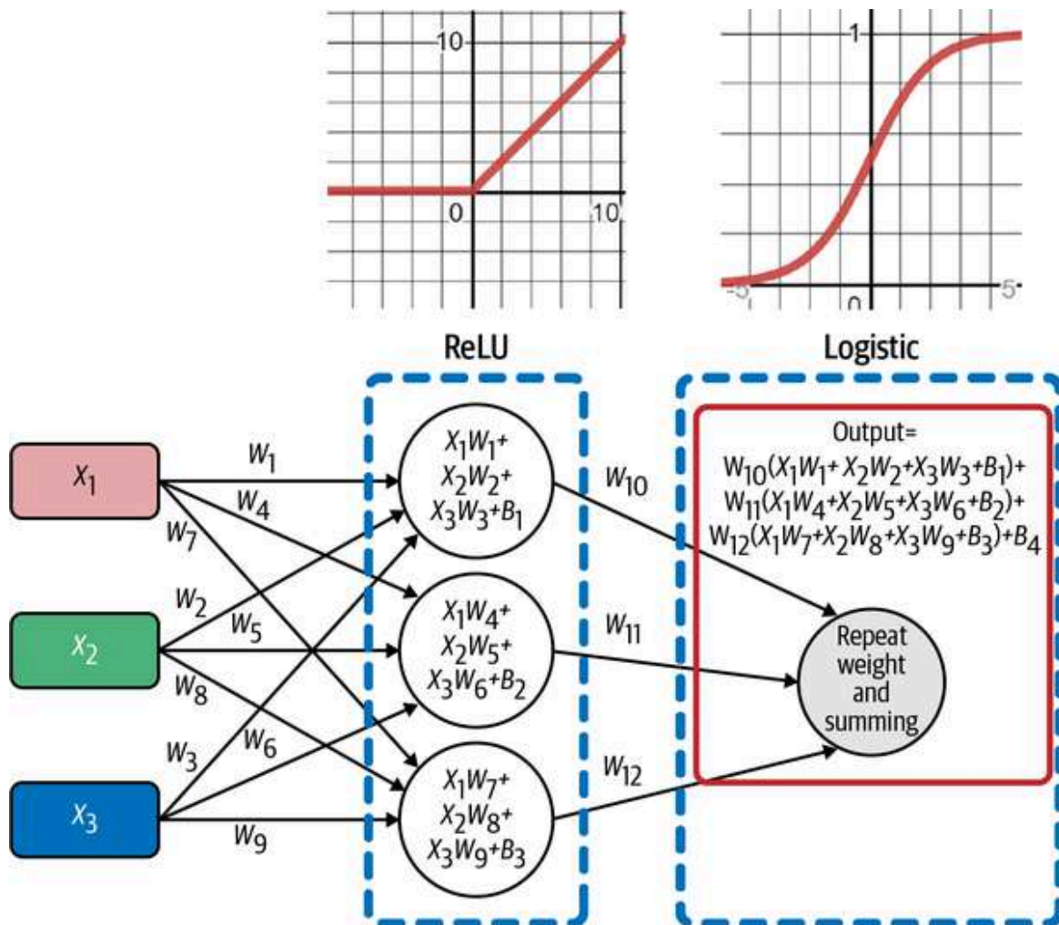
Figure 7-5. Applying activation functions
