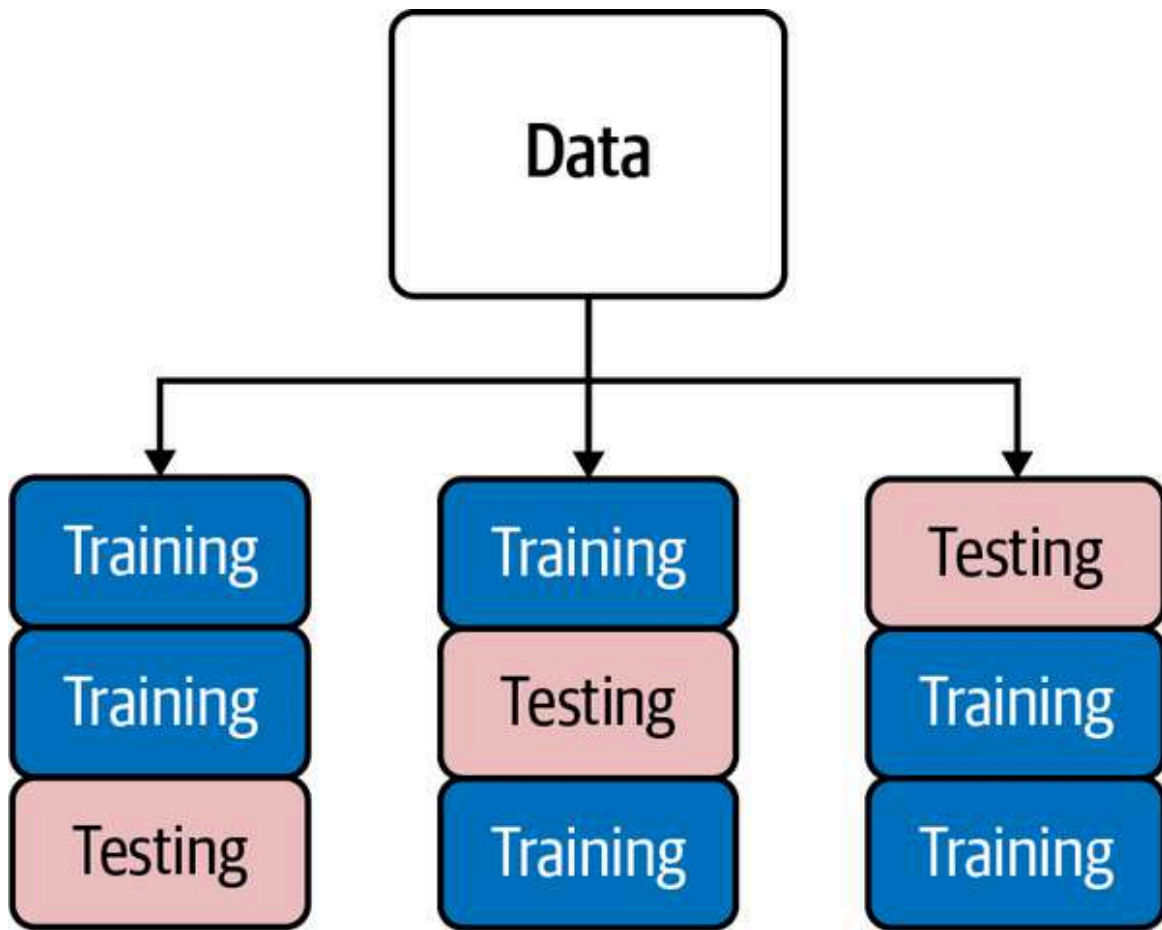
Figure 5-20. A visualization of cross-validation with three folds
