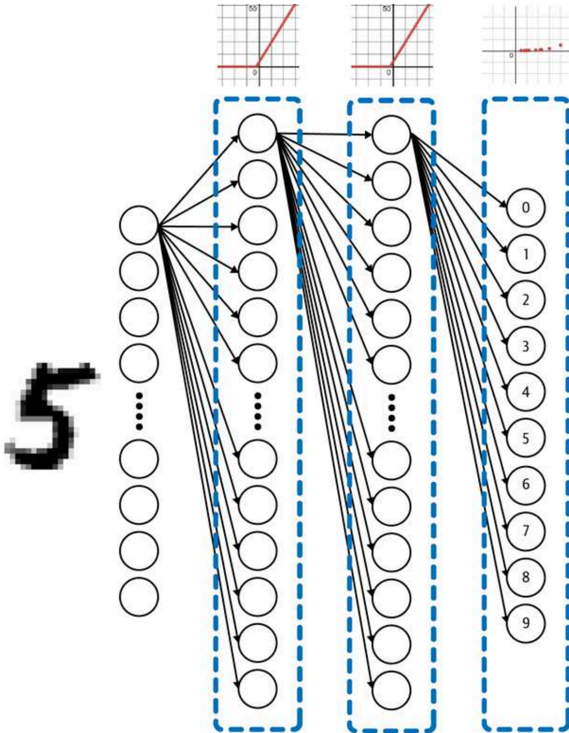
Figure 7-8. A neural network that takes each pixel as an input and predicts what digit the image contains
