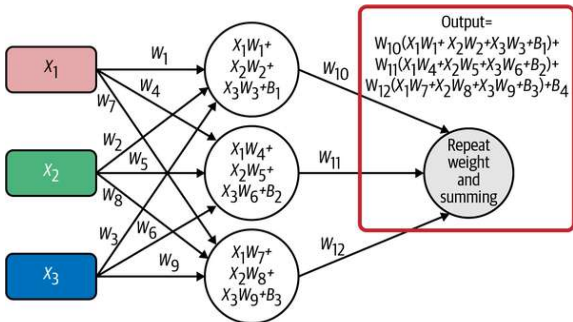
Figure 7-4. The hidden layer of the neural network applies weight and bias values to each input variable, and the output layer applies another set of weights and biases to that output
