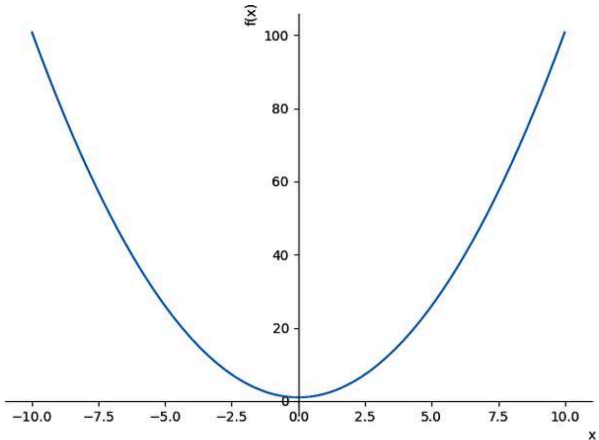
Figure 1-3. Using SymPy to graph a function involving an exponent
