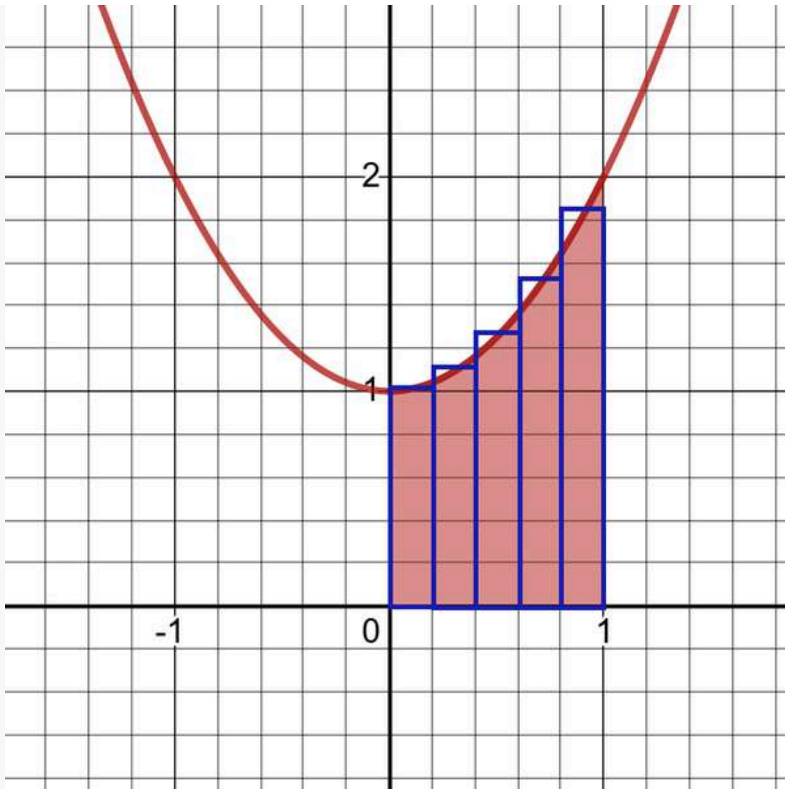
Figure 1-11. Packing rectangles under a curve to approximate area
