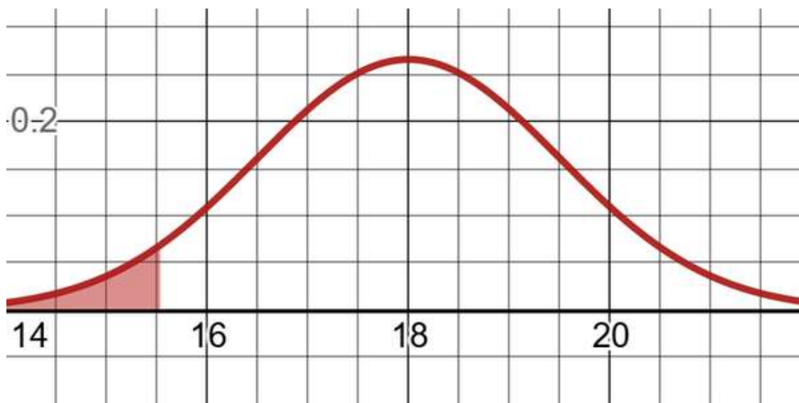
Figure 3-18. Getting the x-value with 5% of area behind it
