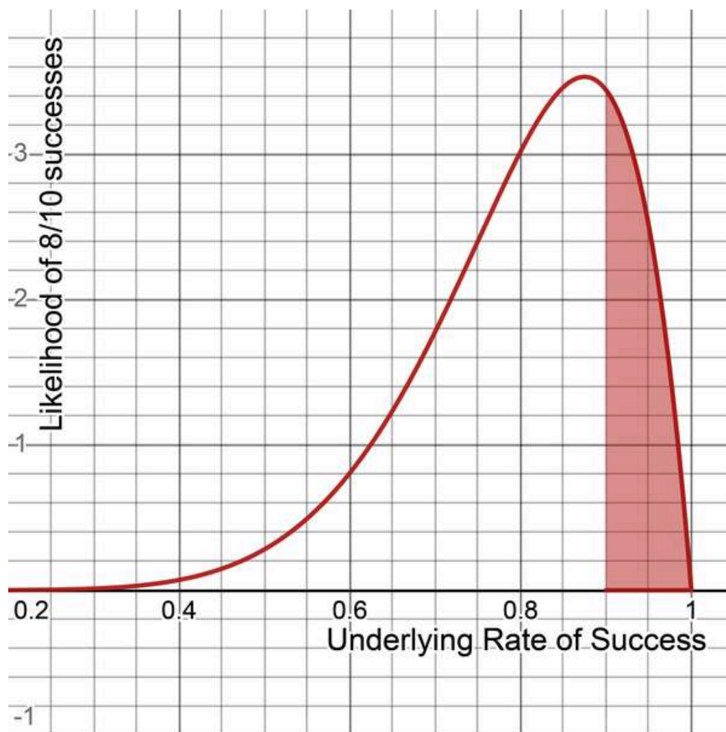
Figure 2-5. The probability of success being 90% or more
