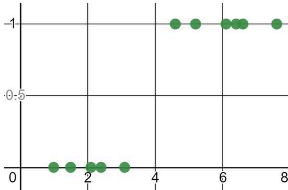
Figure 6-1. Plotting whether patients showed symptoms (1) or not (0) over x hours of exposure
