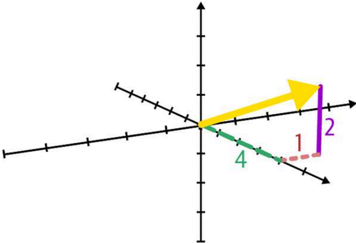
Figure 4-3. A three-dimensional vector
