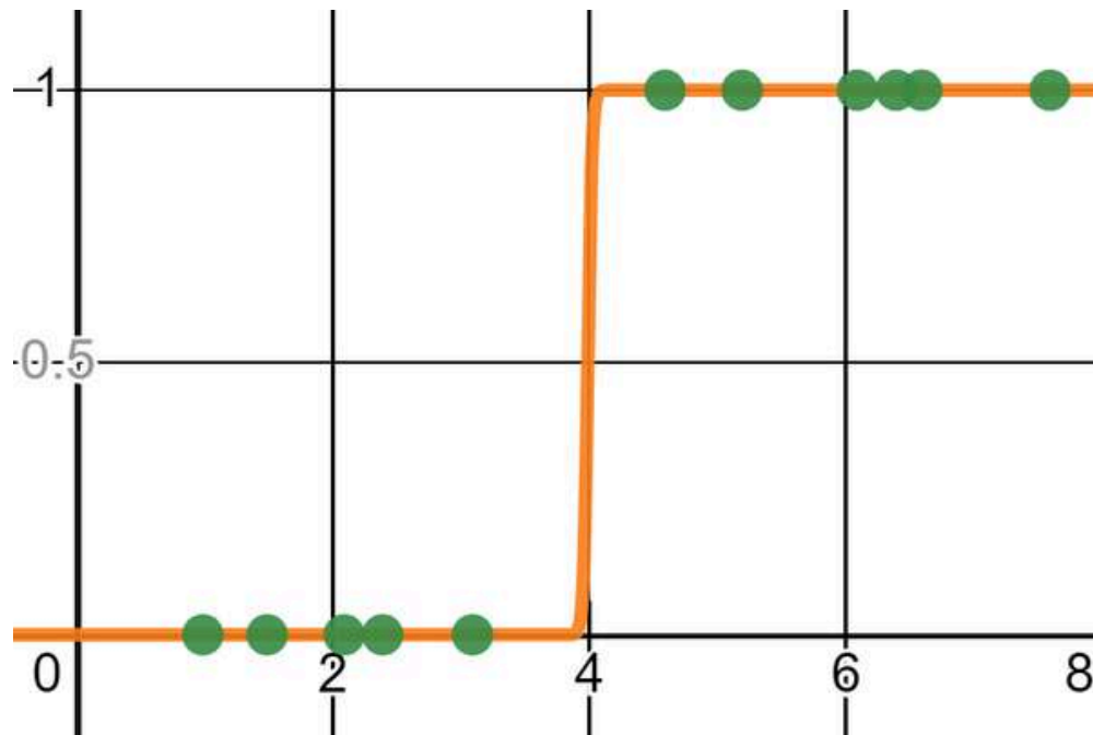
Figure 6-2. After four hours, we see a clear jump where patients start showing symptoms
