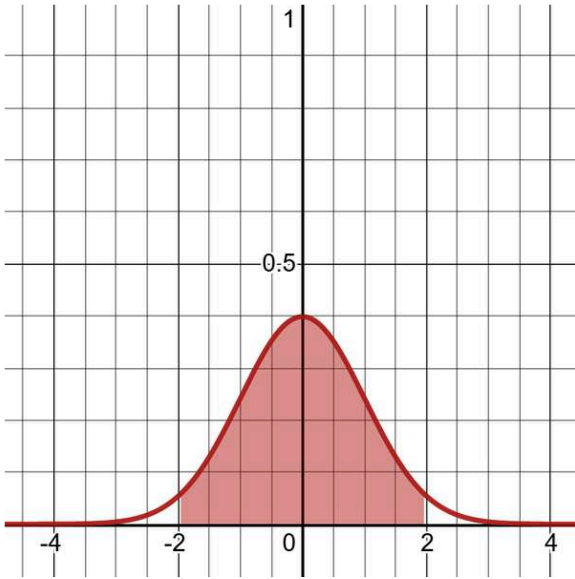
Figure 3-14. 95% symmetrical probability in the center of a standard normal distribution
