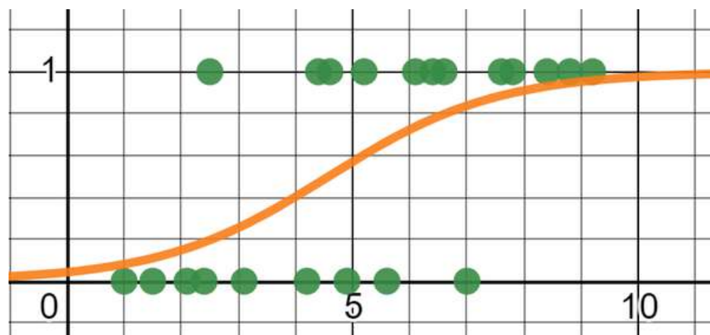
Figure 6-4. Fitting a logistic function to the data
