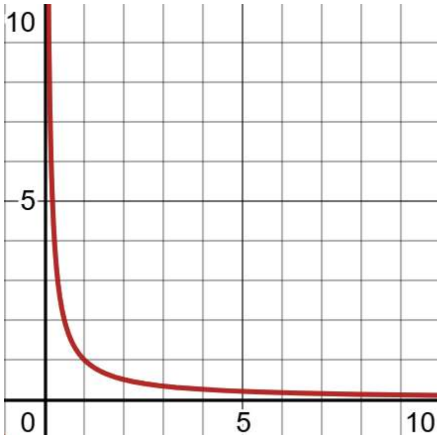
Figure 1-5. A function that forever approaches 0 but never reaches 0
