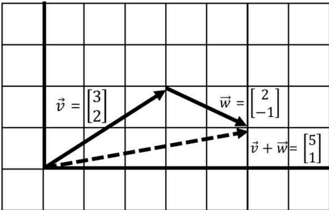
Figure 4-5. Adding two vectors into a new vector
