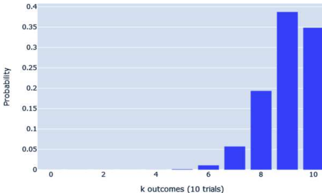
Figure 2-1. A binomial distribution
