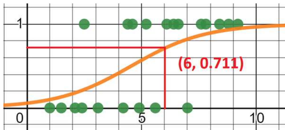
Figure 6-5. We can expect a patient exposed for six hours to be 71.1% likely to have symptoms, and because that's greater than a threshold of 50% we predict they will show symptoms
