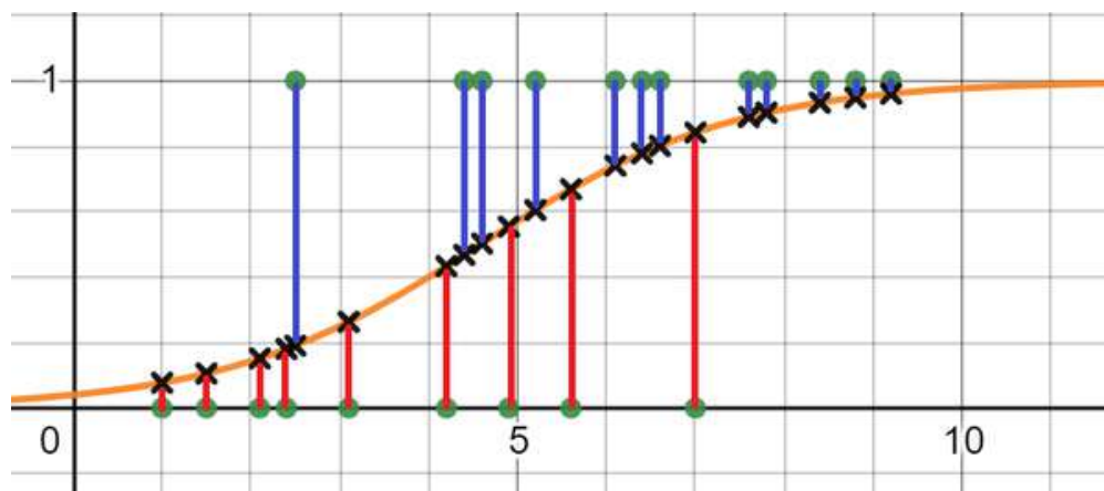
Figure 6-8. Every input value has a corresponding likelihood on the logistic curve
