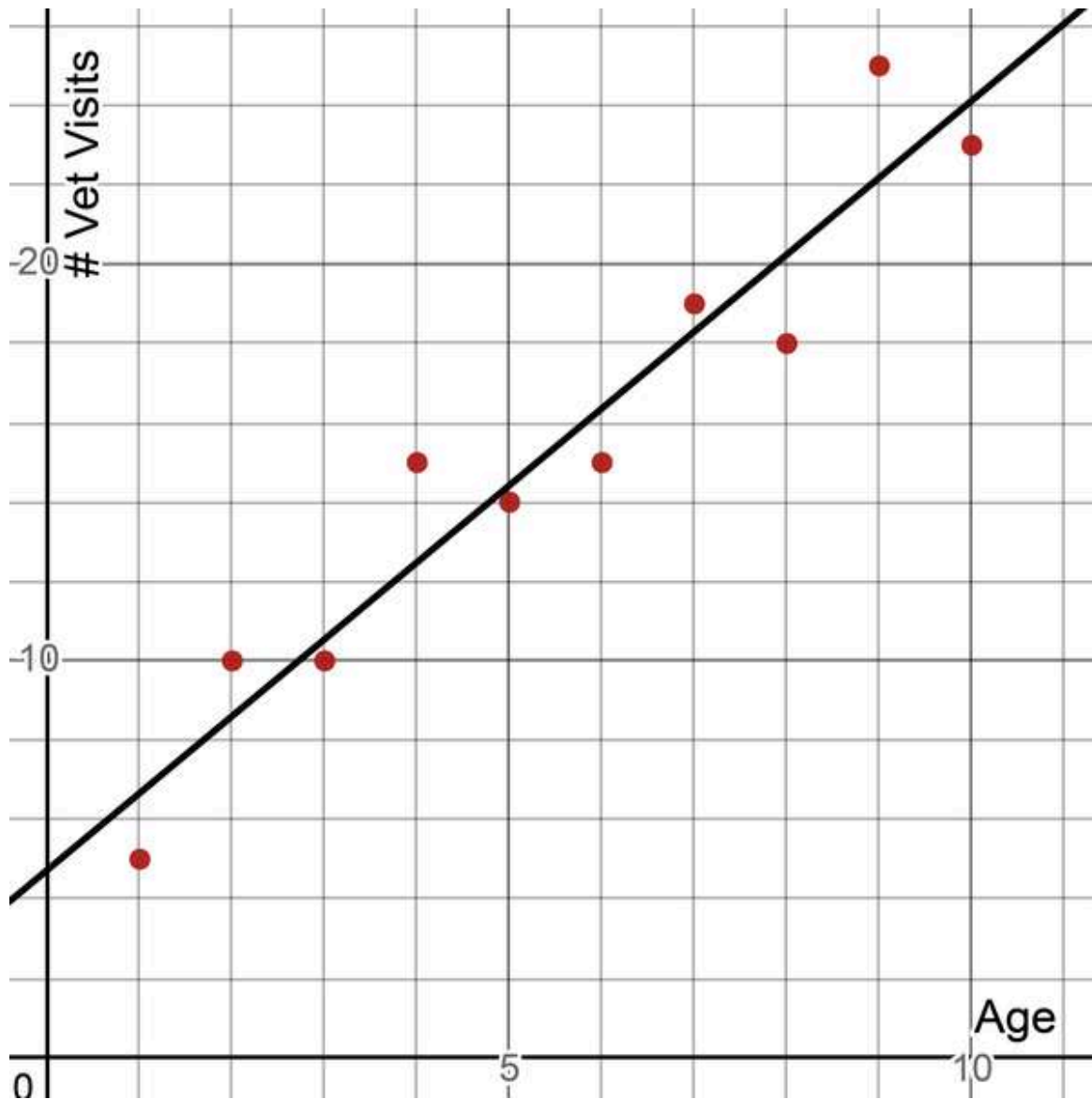
Figure 5-3. Fitting a line through our data
