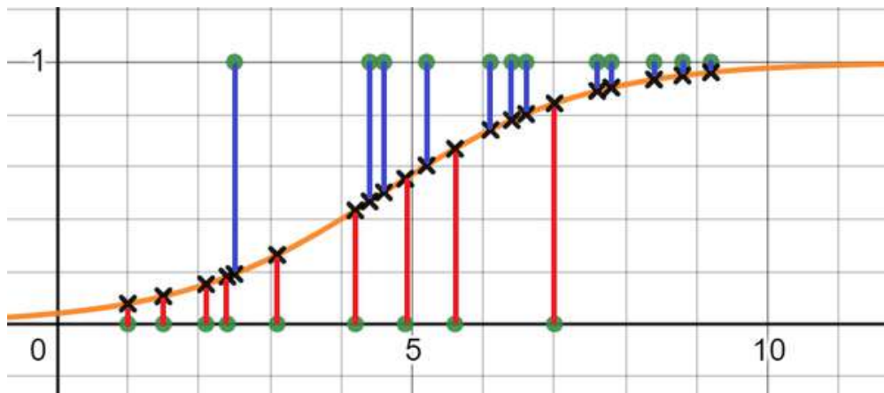
Figure 6-11. Projecting the output values back onto the logistic curve
