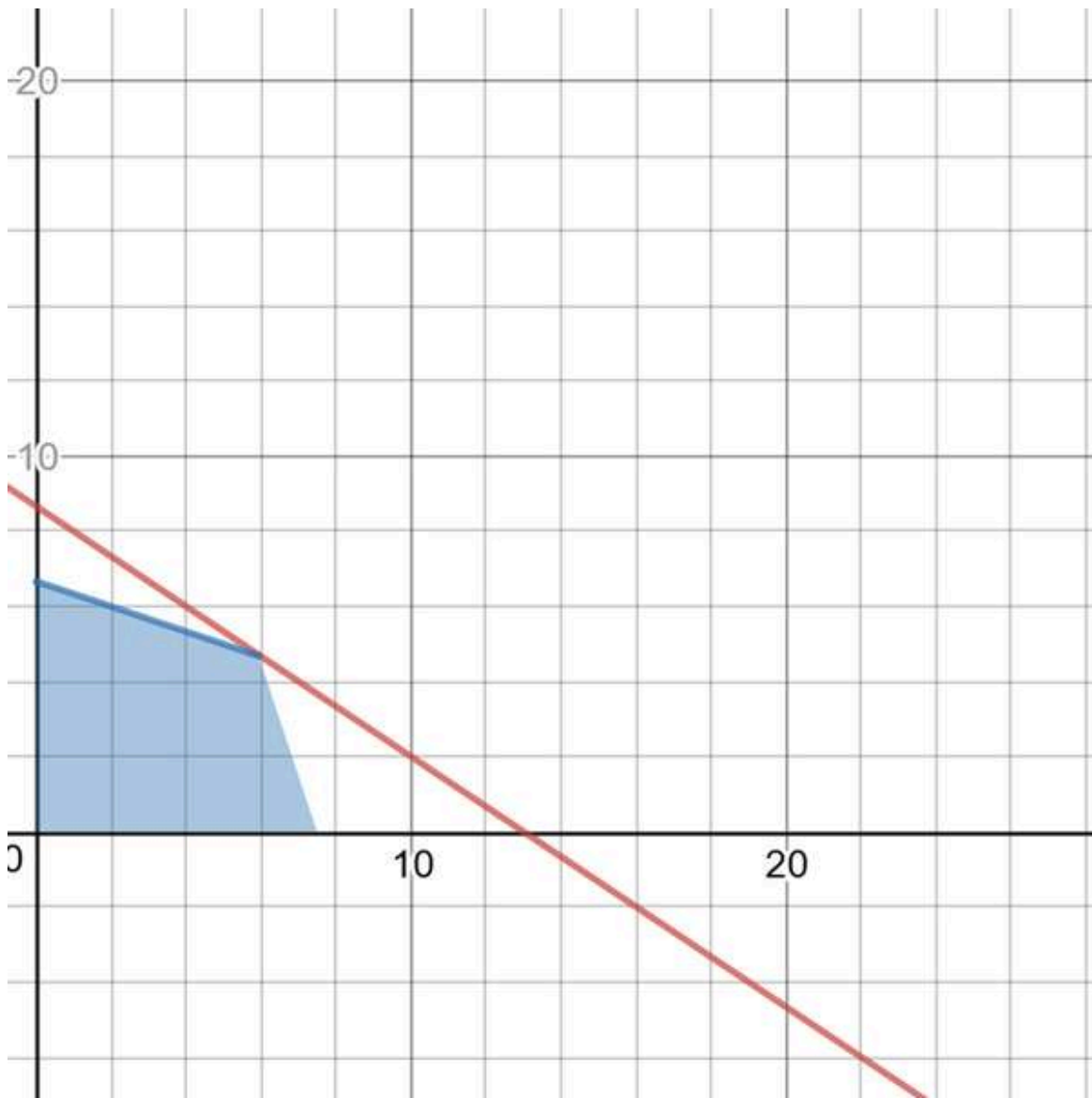
Figure A-8. Maximized objective for our linear programming system
