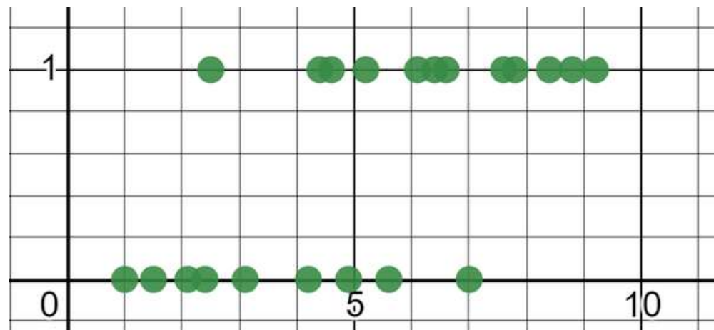
Figure 6-3. A mix of patients who show symptoms (1) and do not show symptoms (0) exists in the middle
