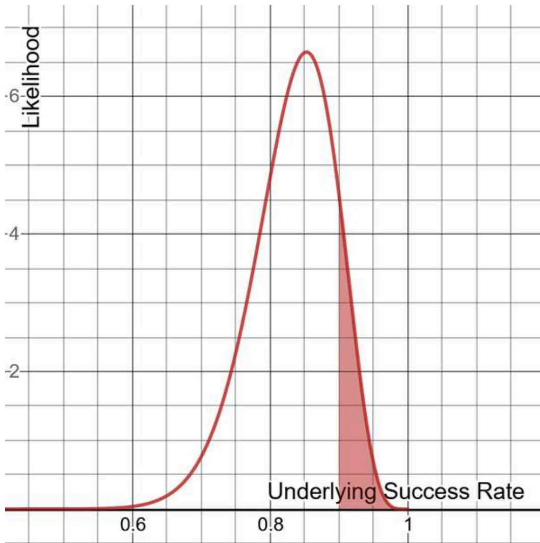
Figure 2-7. Beta distribution after 30 successes and 6 failures
