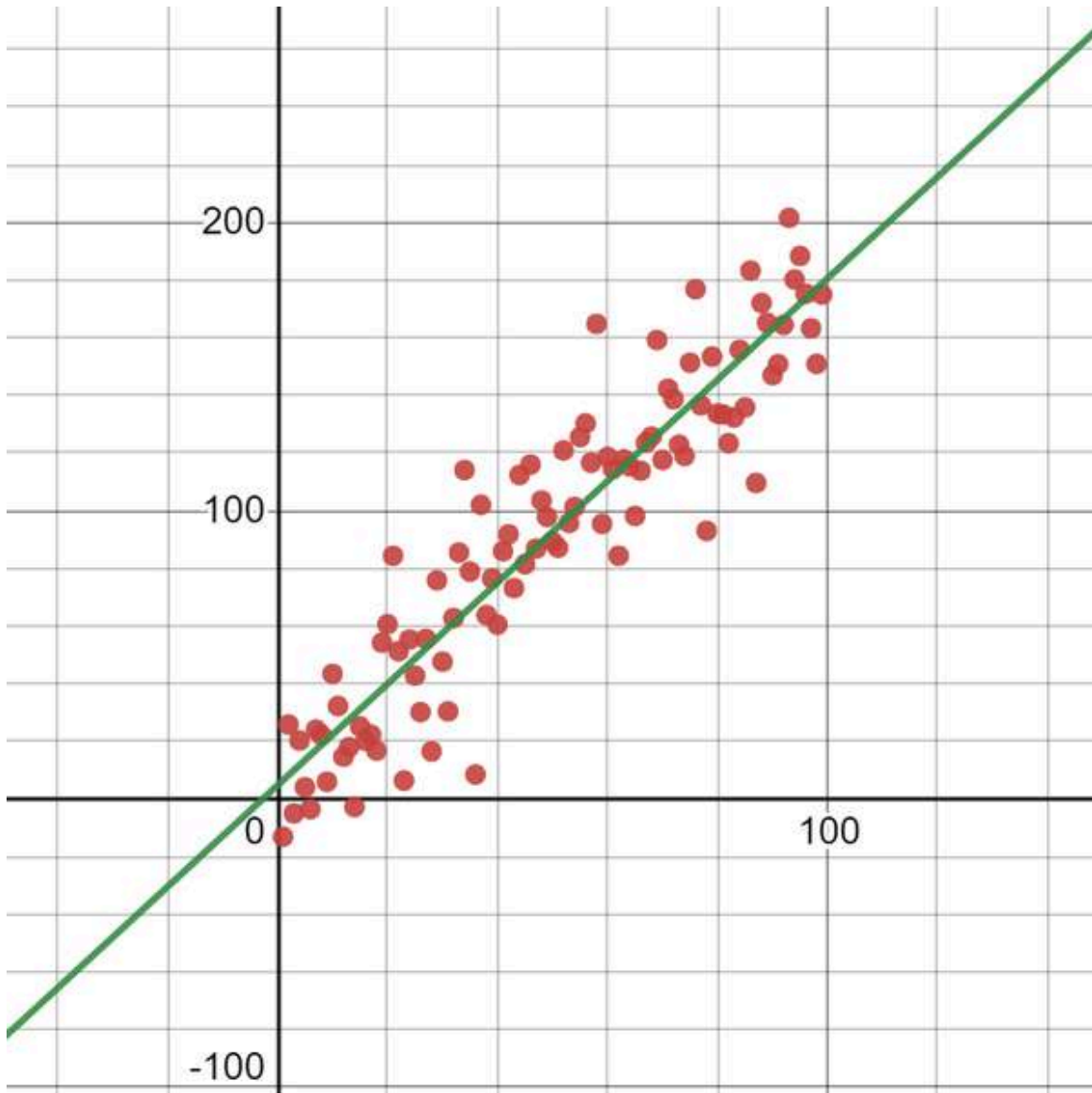
Figure 5-1. Example of a linear regression, which fits a line to observed data
