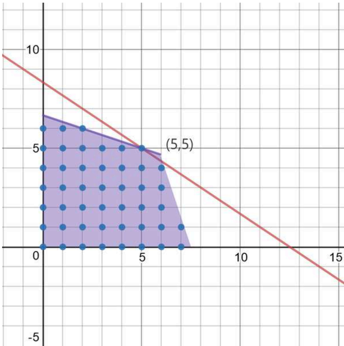
Figure A-9. A discrete linear programming system
