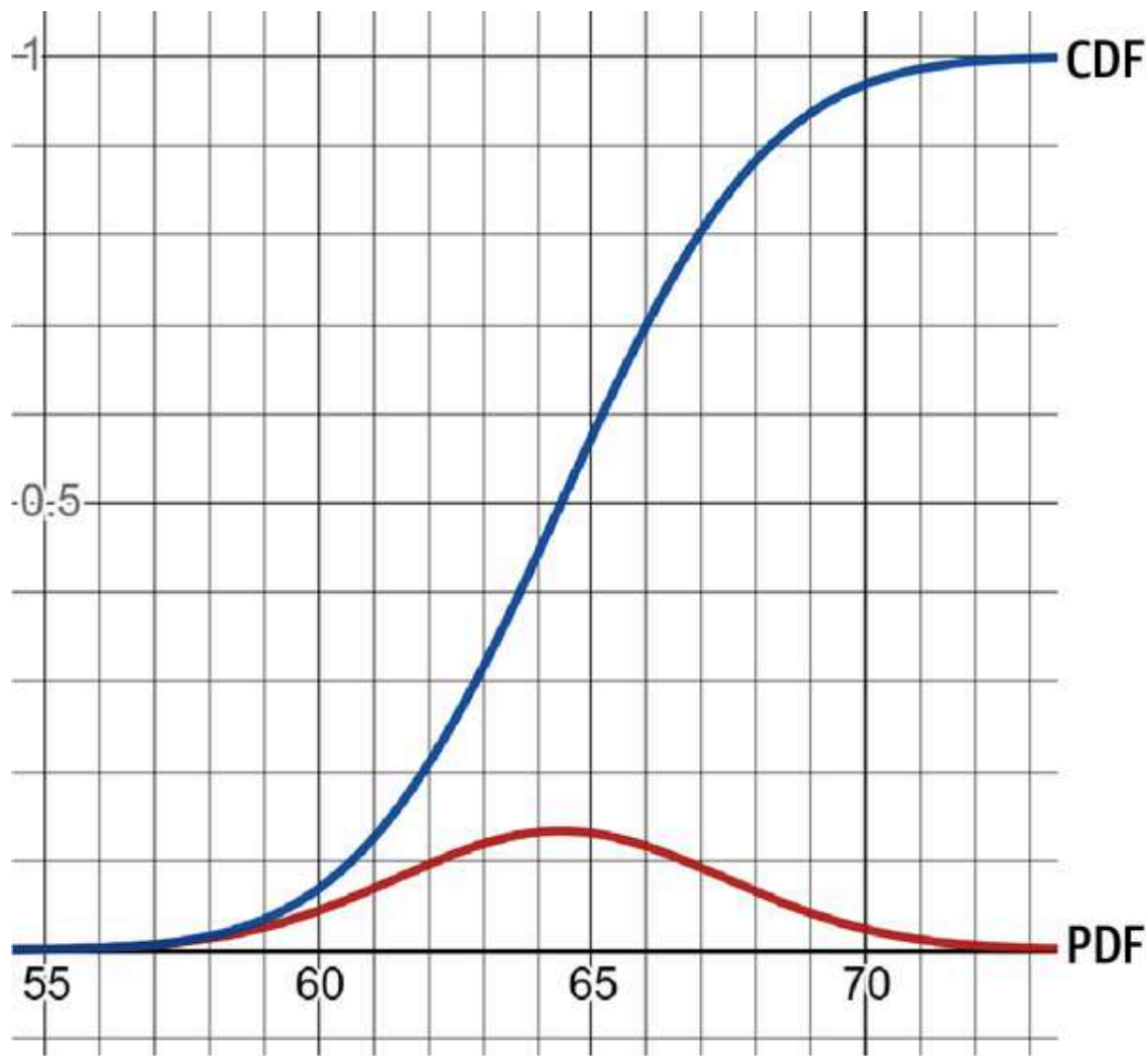
Figure 3-8. A PDF alongside its CDF
