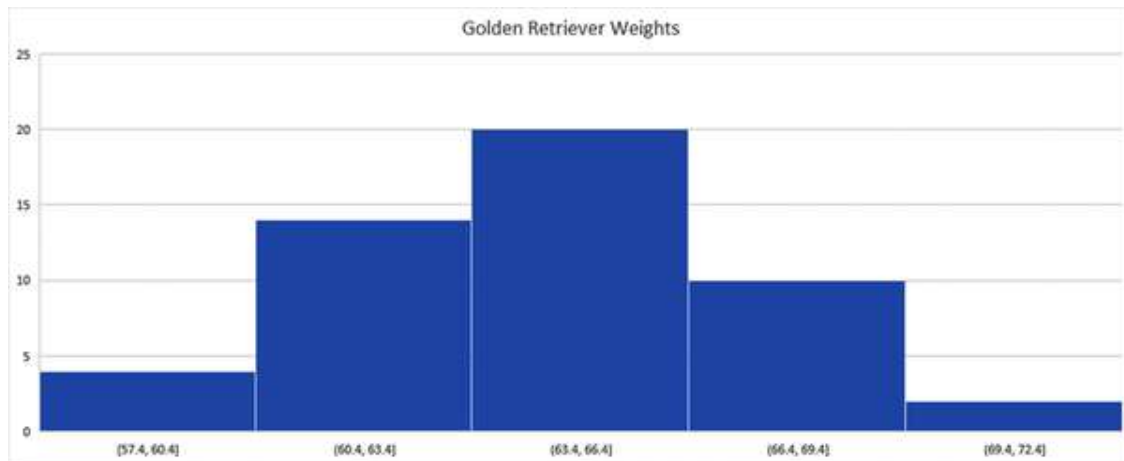
Figure 3-5. A more productive histogram
