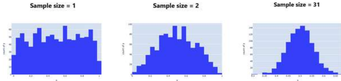
Figure 3-13. Larger sample sizes approach the normal distribution
