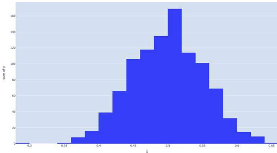
Figure 3-12. Taking the means of samples (each of size 31) and plotting them
