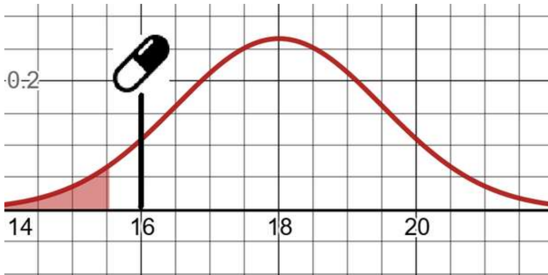
Figure 3-19. We have failed to prove our drug test result is statistically significant
