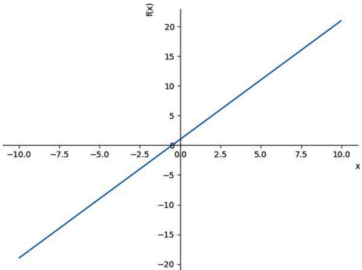
Figure 1-2. Using SymPy to graph a linear function
