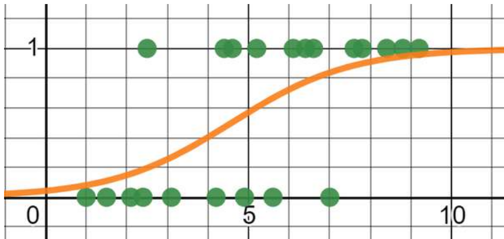
Figure 6-12. Our data has a mediocre R^2 of 0.30645 because there is a lot of variance in the middle of our curve
