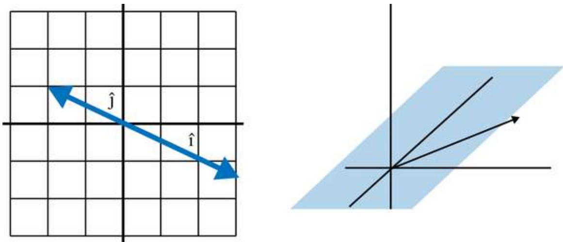
Figure 4-23. Linear dependence in 2D and 3D
