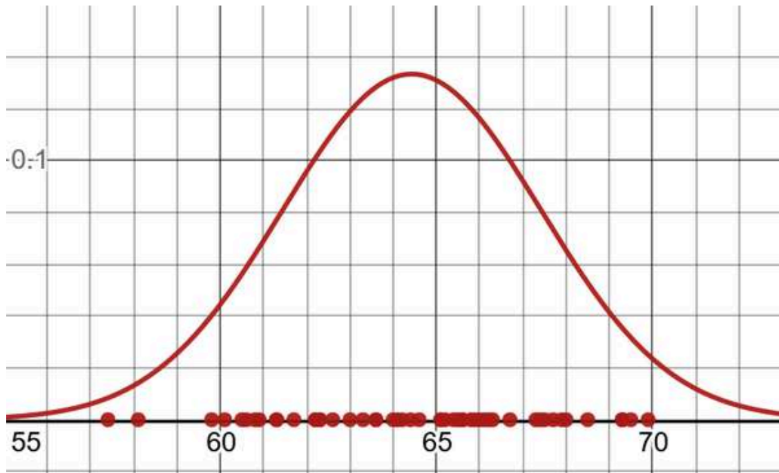
Figure 3-6. A normal distribution fitted to data points
