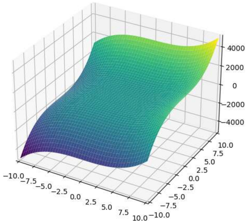
Figure 1-8. Plotting a three-dimensional exponential function
