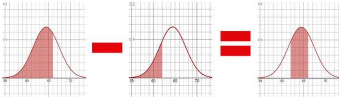
Figure 3-10. Finding a middle range of probability
