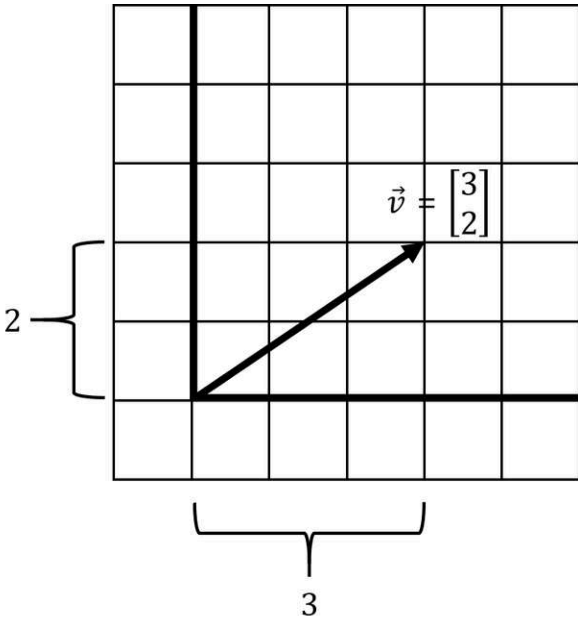
Figure 4-1. A simple vector
