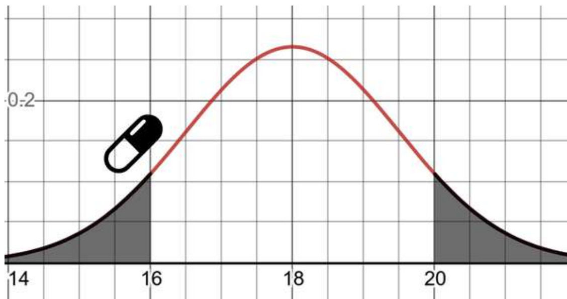
Figure 3-23. The p-value adds symmetrical sides for statistical significance
