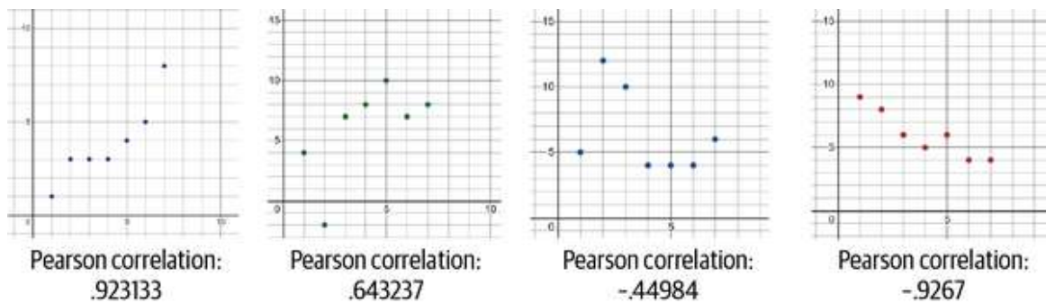
Figure 5-12. Correlation coefficients for four scatterplots
