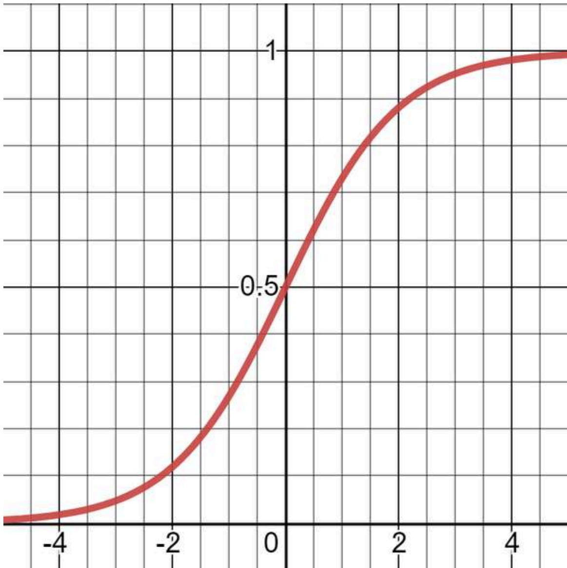
Figure 7-7. Logistic activation function
