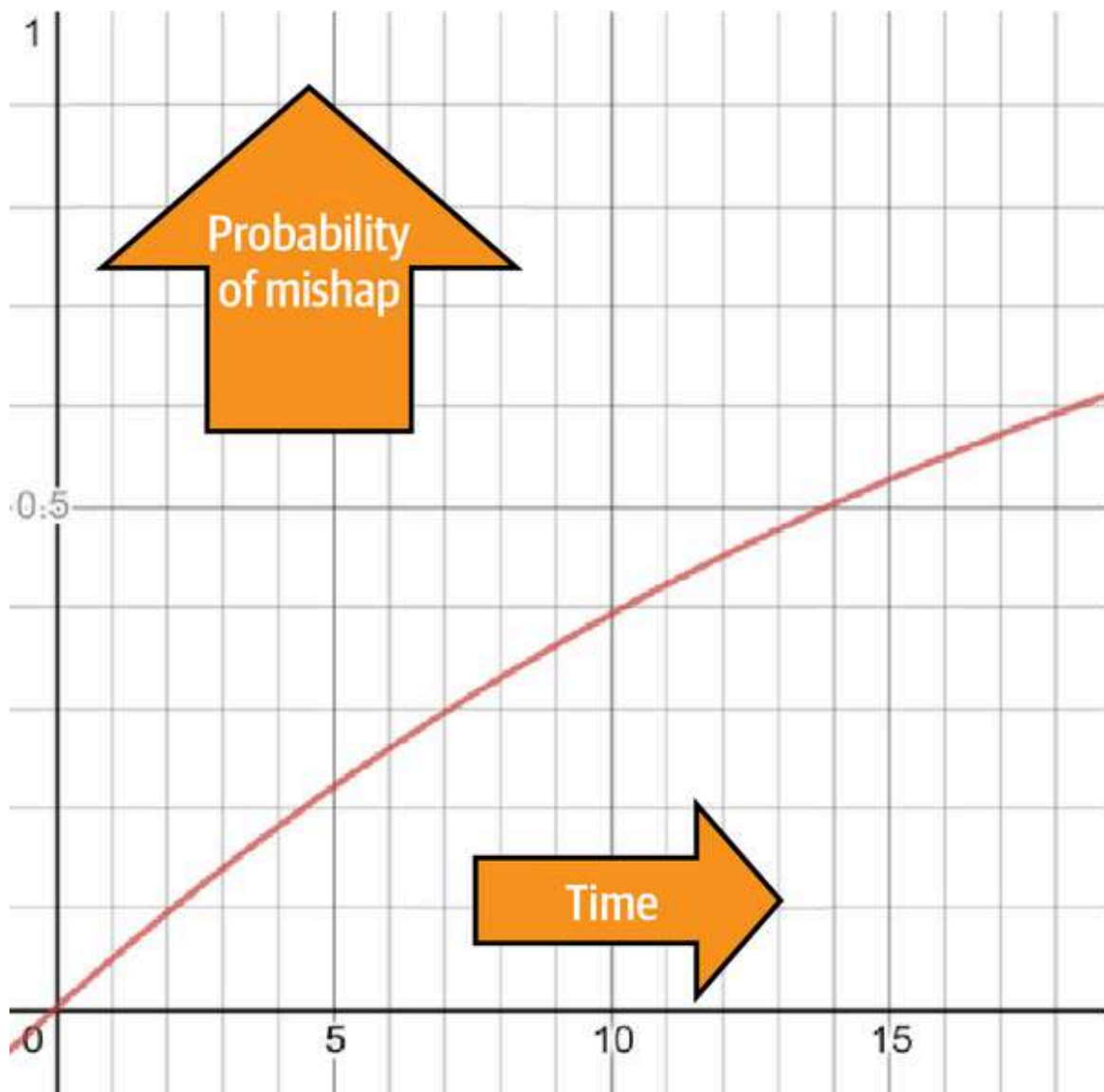
Figure A-3. Predicting the probability of a leak over time
