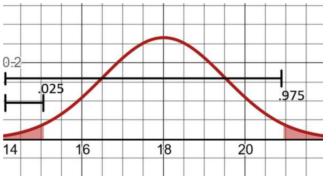
Figure 3-21. Calculating the central 95% of normal distribution area
