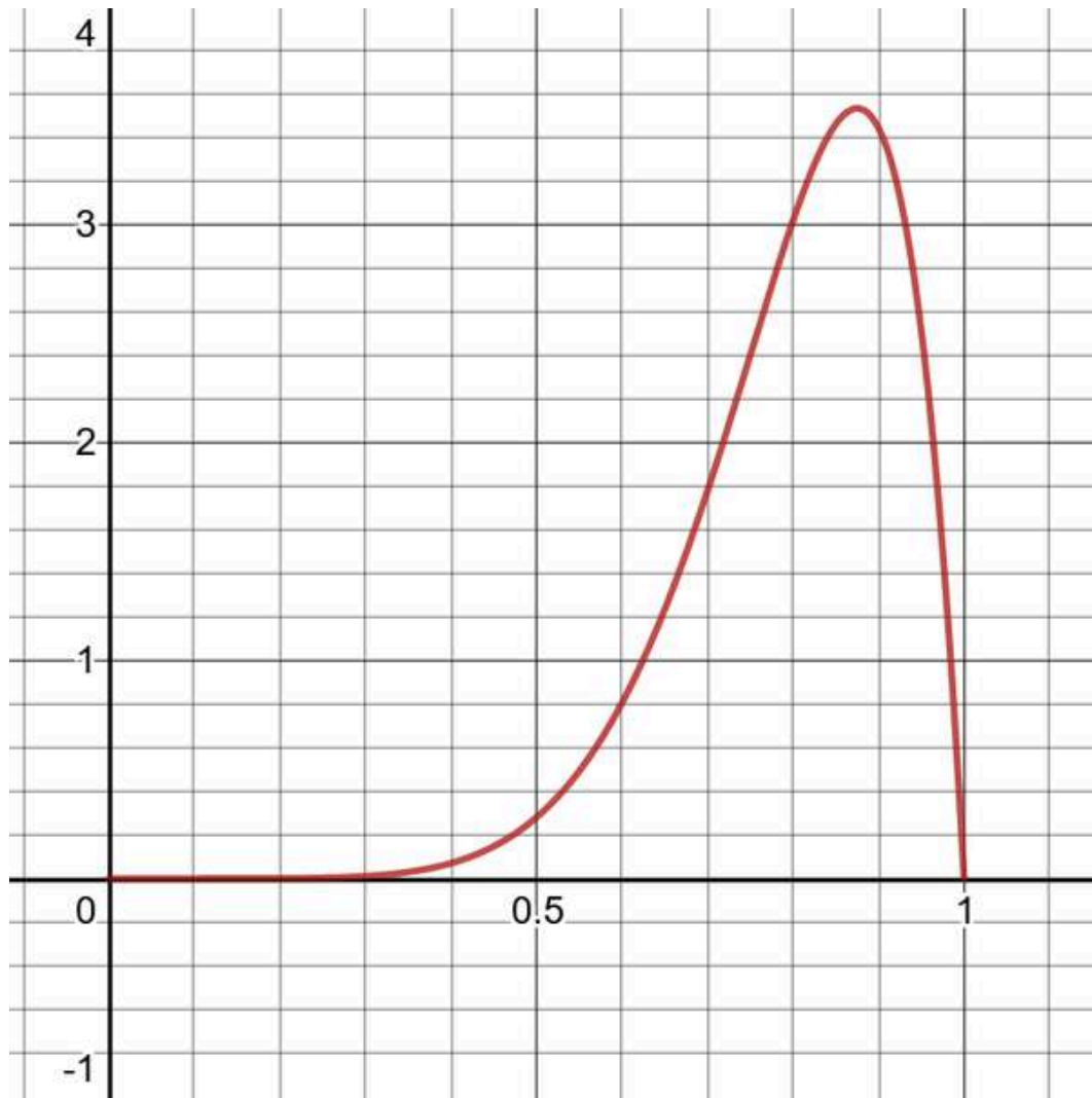
Figure 2-2. Beta distribution
