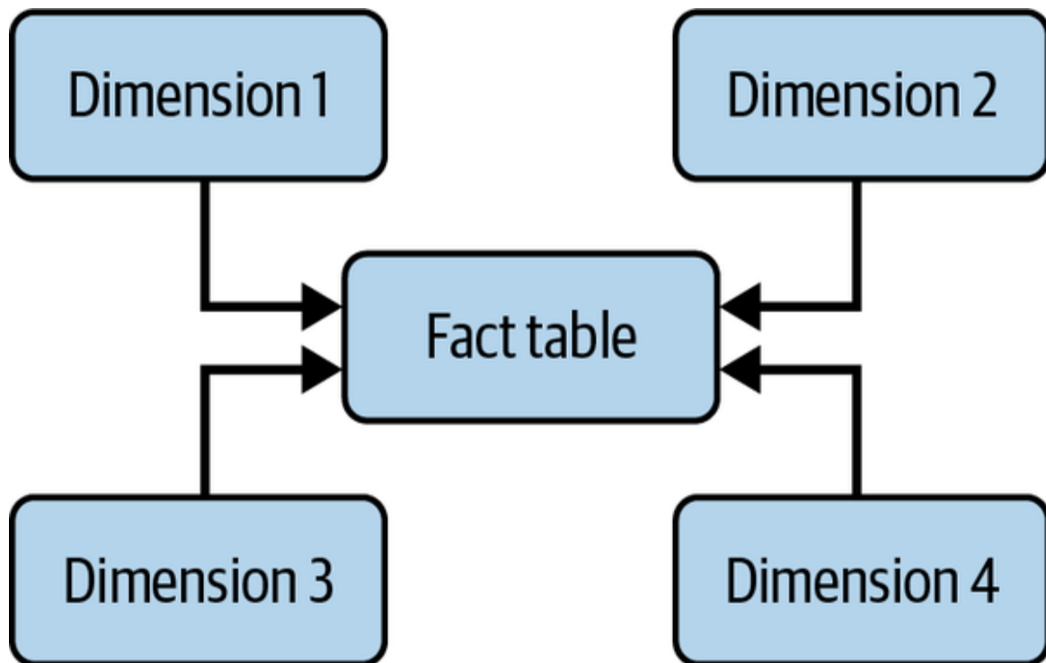
Figure 8-14. A Kimball star schema, with facts and dimensions
