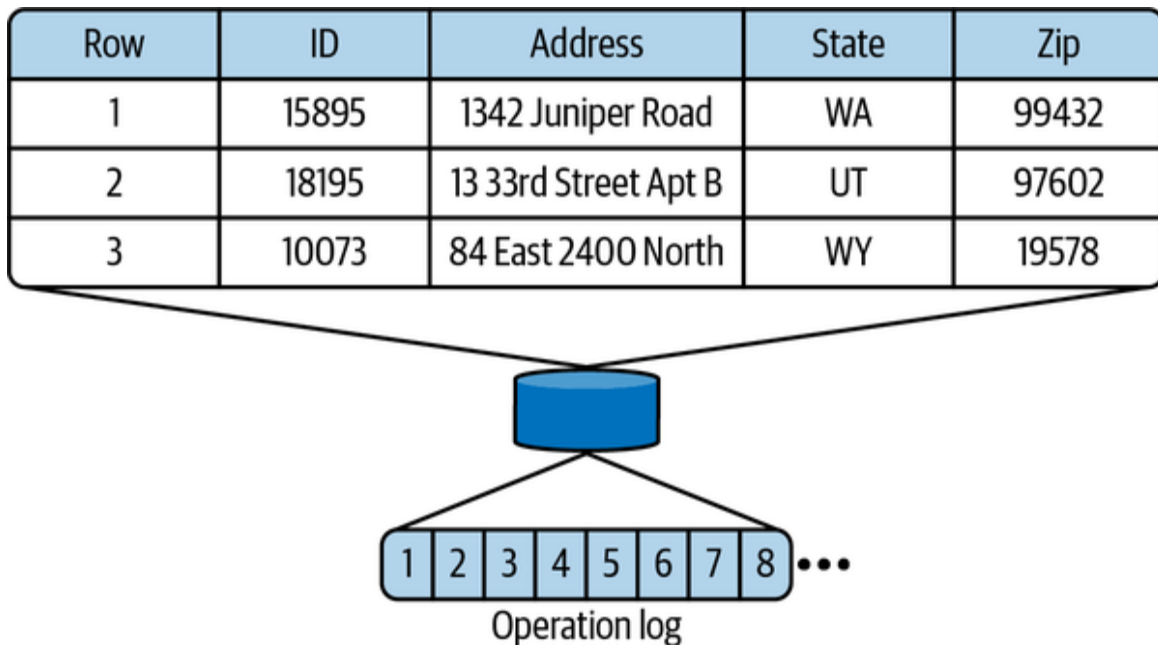
Figure 5-3. Database logs record operations on a table
