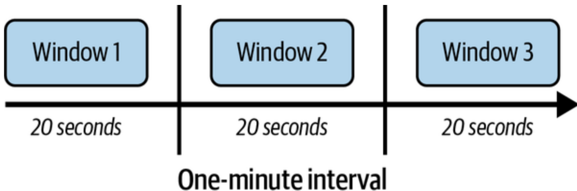
Figure 8-6. Tumbling/fixed window
