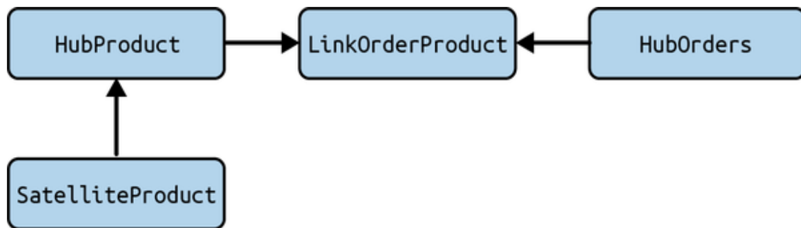
Figure 8-16. The Data Vault for orders and products
