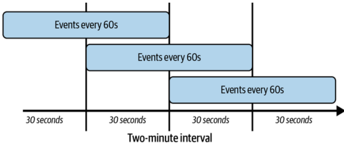
Figure 8-7. Sliding windows
