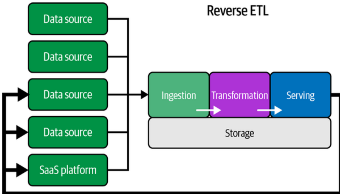
Figure 9-5. Reverse ETL
