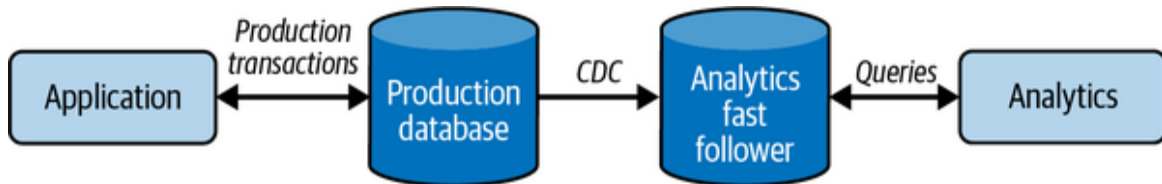
Figure 8-3. CDC with a fast-follower analytics database
