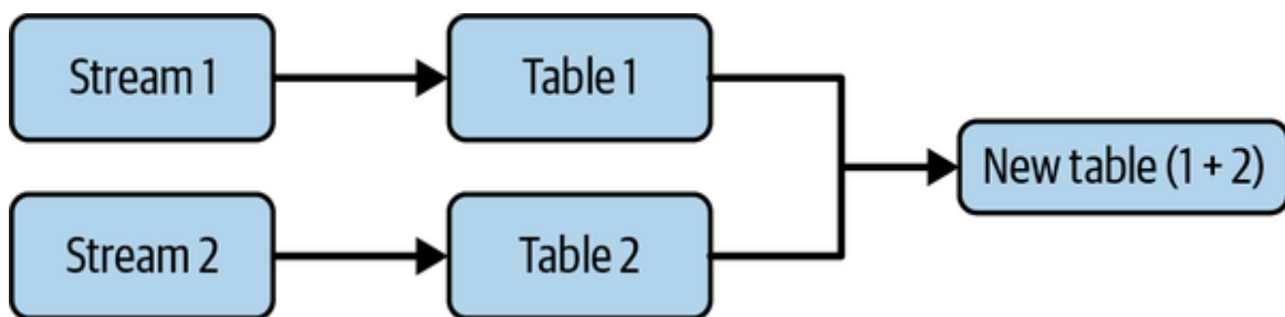
Figure 8-9. Joining two tables fed by streams
