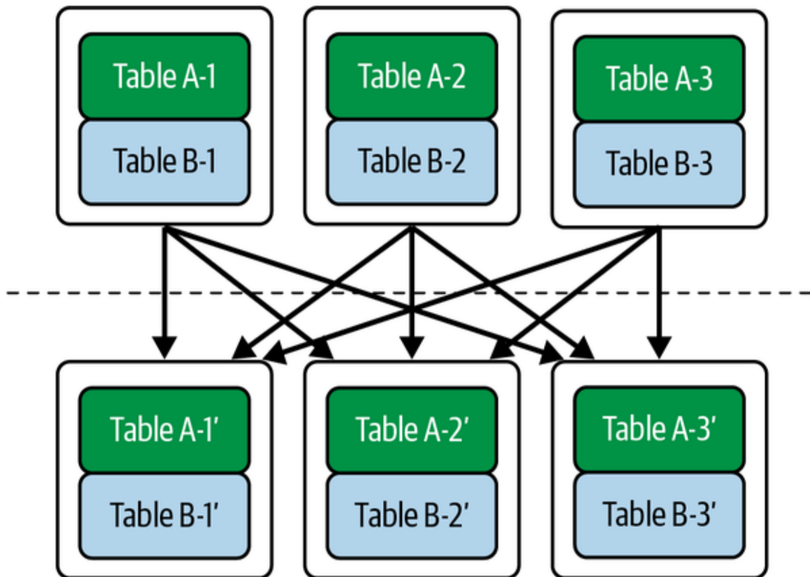
Figure 8-18. Shuffle hash join
