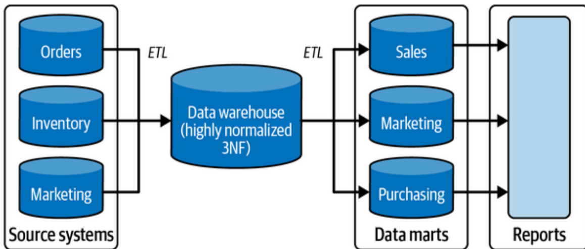
Figure 8-13. An ecommerce data warehouse
