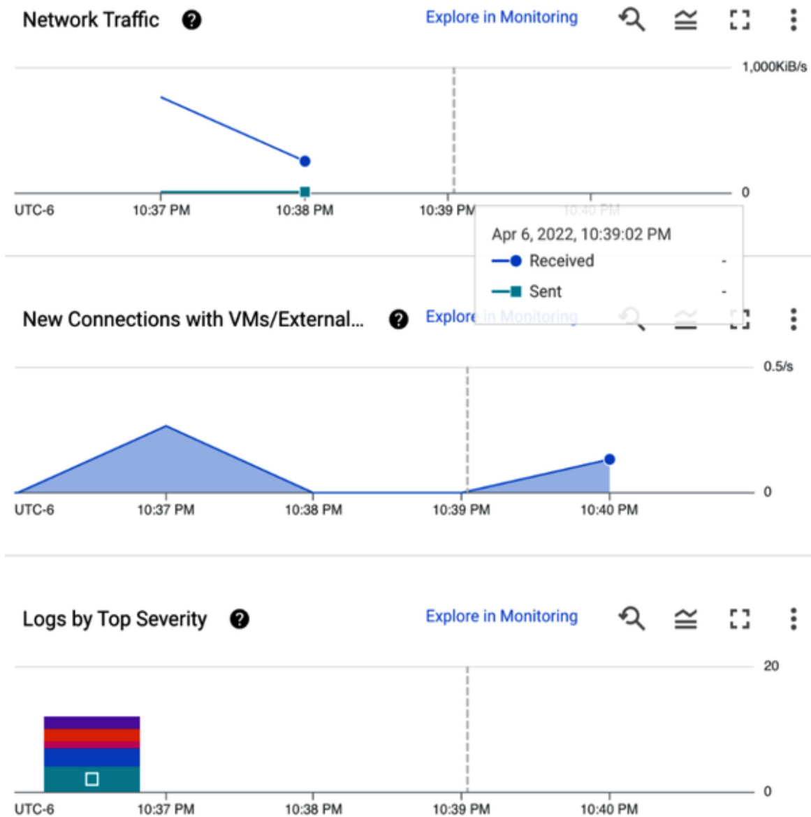
Figure 9-2. An operational analytics dashboard showing some key metrics from Google Compute Engine
