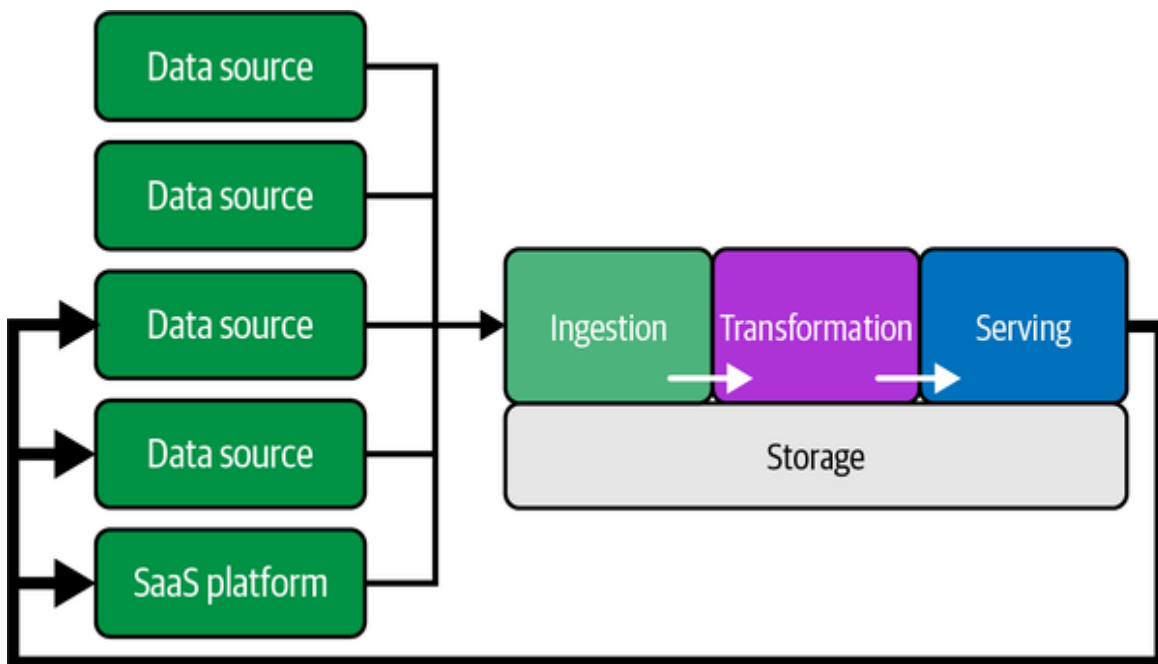
Figure 2-6. Reverse ETL
