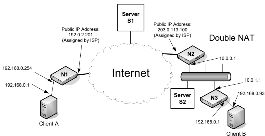
Figure 7-7 Applications running on clients behind a NAT may require help from a server to engage in direct communication. In hole punching, a server, often specialized for a specific application, provides rendezvous information among clients that first establish NAT state and then perform direct communication, if possible. Some applications attempt to “fix” (determine and maintain) the addresses (and port numbers) their traffic will be assigned when passing through a NAT using standard generic protocols. These methods may encounter troubles in certain situations such as environments with multiple levels of NAT. In this example, client A’s external address visible at S1 is 192.0.2.201 and client B’s is 203.0.113.100. At S2, however, B’s external address is 10.0.1.1.
