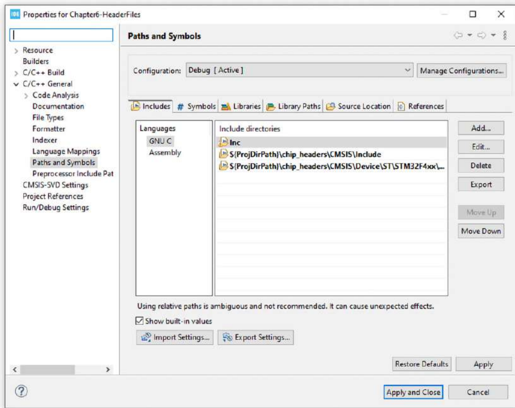
Figure 6.2: The Includes tab in the project properties window
