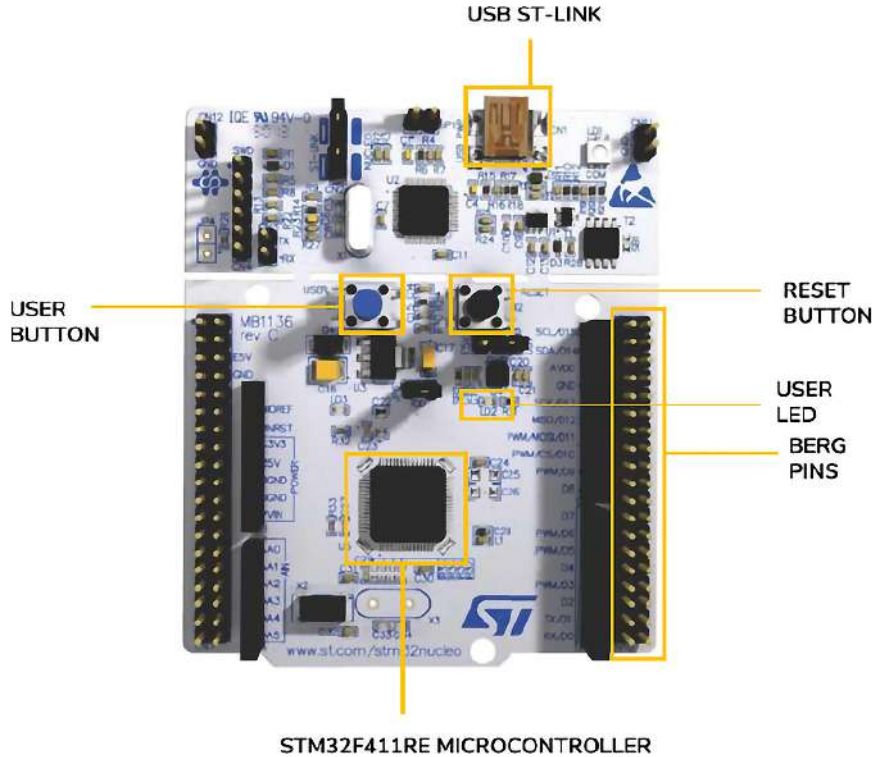
Figure 1.13: The NUCLEO-F411 development board
