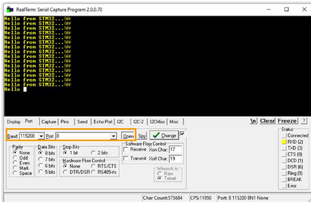
Figure 10.5: Realterm settings
