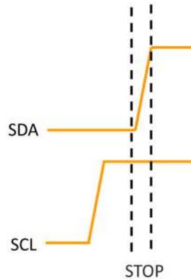
Figure 13.4: The stop condition
