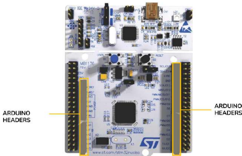
Figure 2.8: This NUCLEO-F411 development board with Arduino headers highlighted
