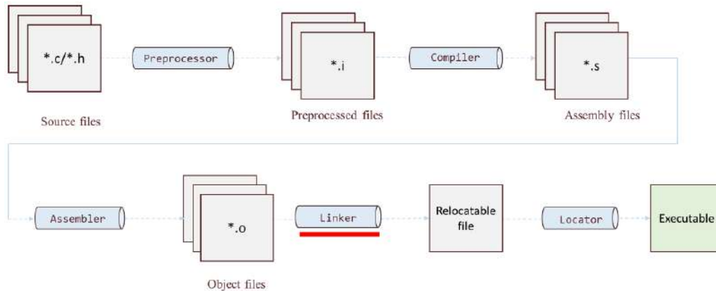
Figure 4.2: The build process with the linker highlighted
