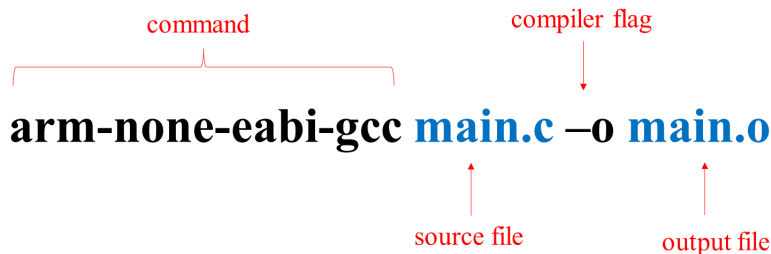
Figure 3.2: Usage of the arm-none-eabi-gcc command
