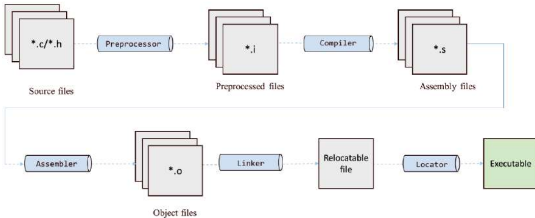
Figure 3.1: The build process, detailing the input and output files for each stage and the specific tools used
