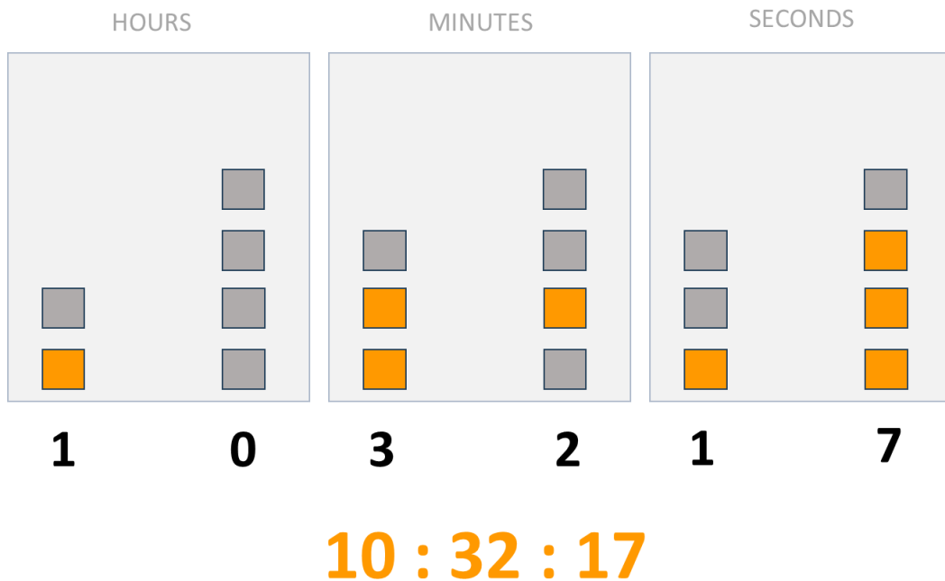
Figure 15.7: Display with BCD format
