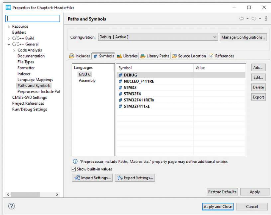
Figure 6.3: The Symbols tab in the project properties window
