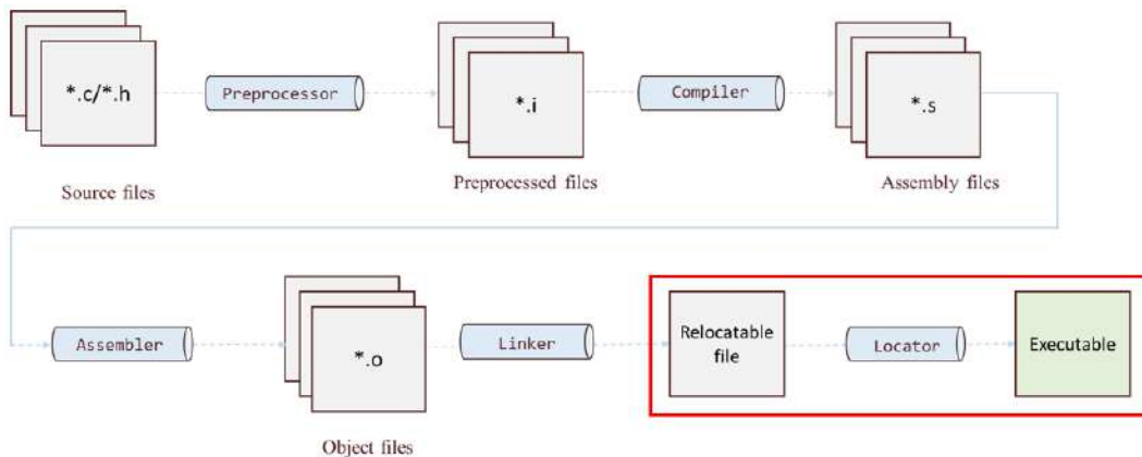
Figure 4.3: The build process, highlighting the relationship between the relocatable file, the locator, and the final executable output
