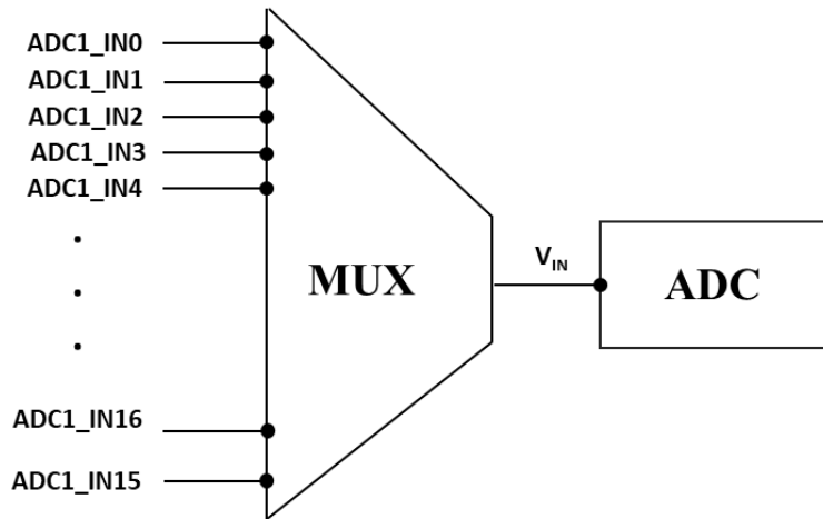
Figure 11.3: ADC channel multiplexing
