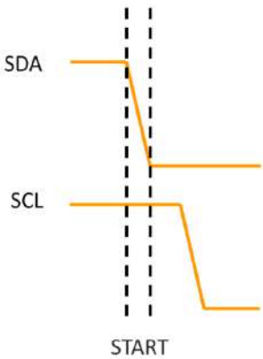
Figure 13.3: The start condition
