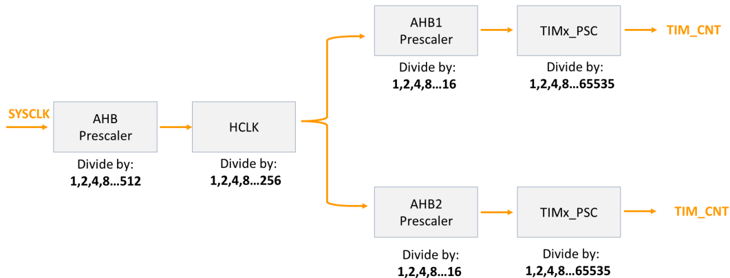
Figure 9.1: Timer clock prescaling
