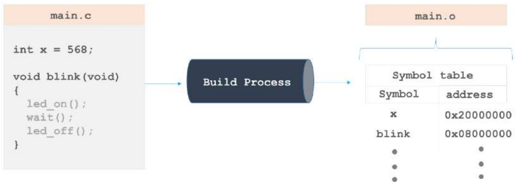
Figure 4.6: Representation of functions and variables from the source file in the symbol table of the output object file
