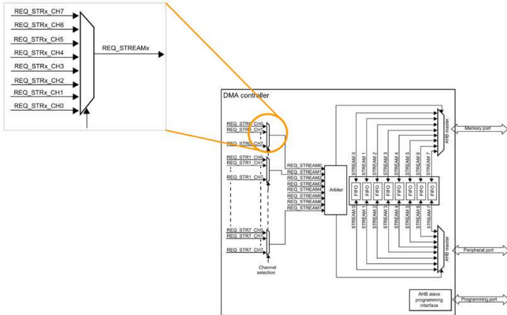
Figure 17.3: The DMA module, with channels zoomed in
