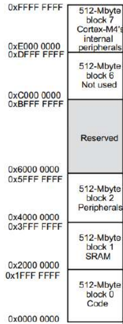
Figure 2.11: Memory map
