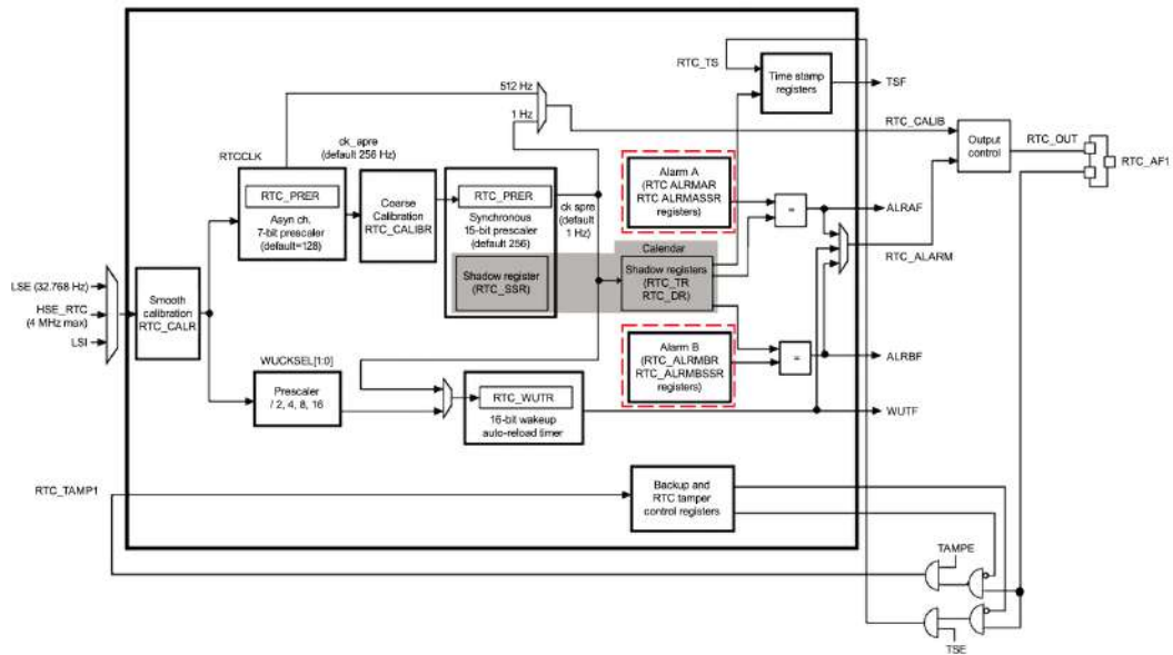
Figure 15.4: RTC block diagram – alarms
