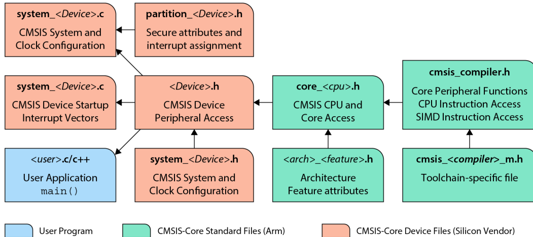
Figure 6.1: The CMSIS-Core files
