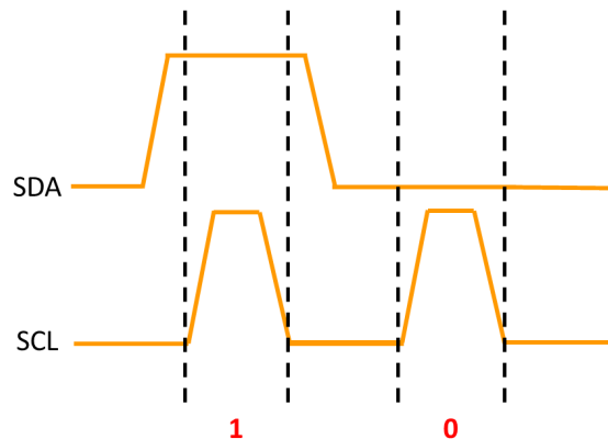
Figure 13.5: The data transmission process
