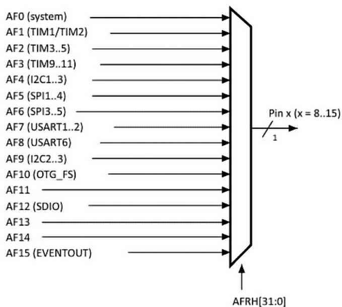
Figure 7.5: Alternate function selection
