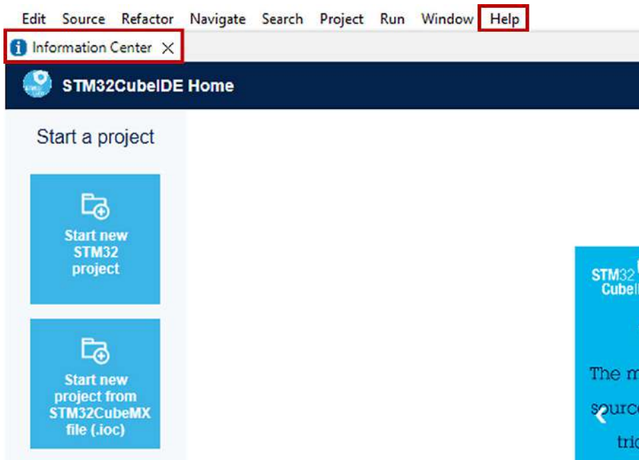
Figure 1.15: Information Center
