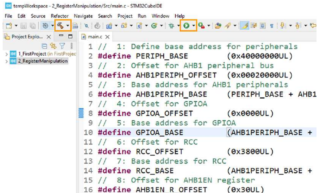
Figure 2.20: The build and run icons
