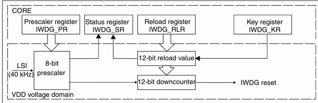
Figure 16.1: IWDG block diagram
