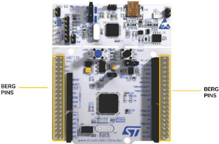
Figure 2.7: This is the NUCLEO-F411 development board with berg pins highlighted
