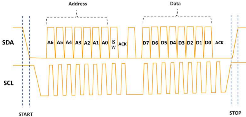
Figure 13.6: The complete packet
