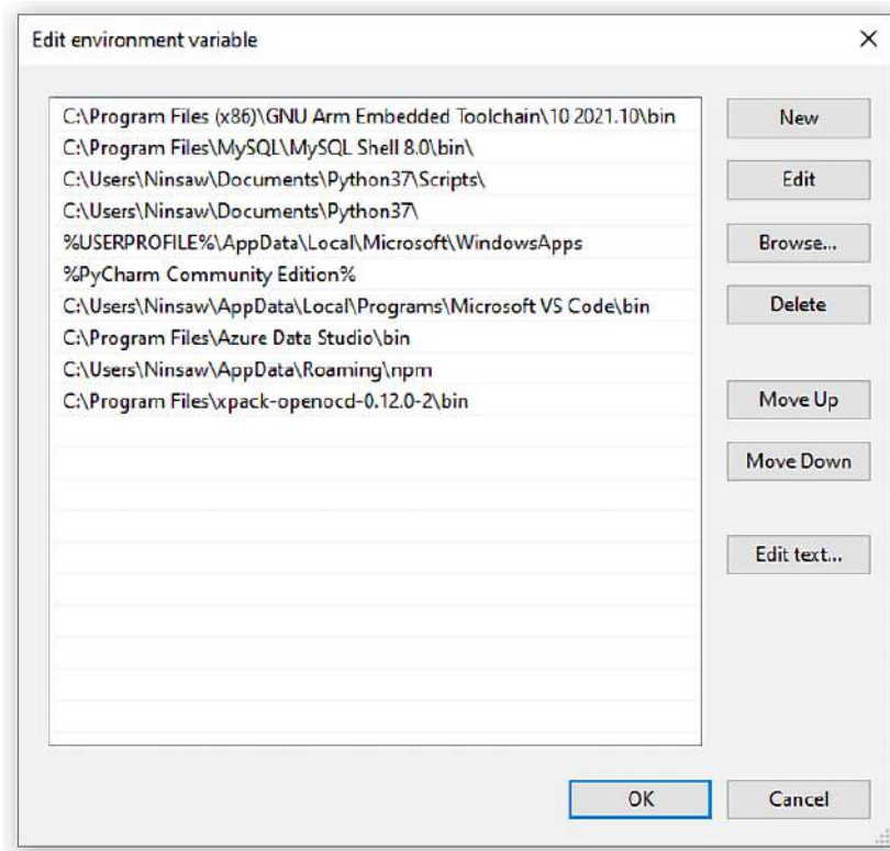
Figure 1.12: The Edit environment variable popup
