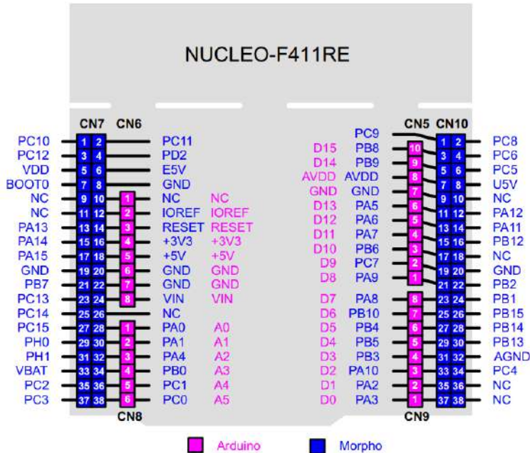
Figure 2.9: Pinout of the NUCLEO-F411 development board
