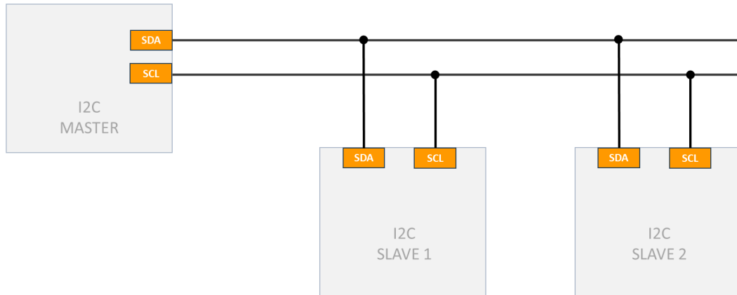
Figure 13.1: The I2C interface – multiple slaves
