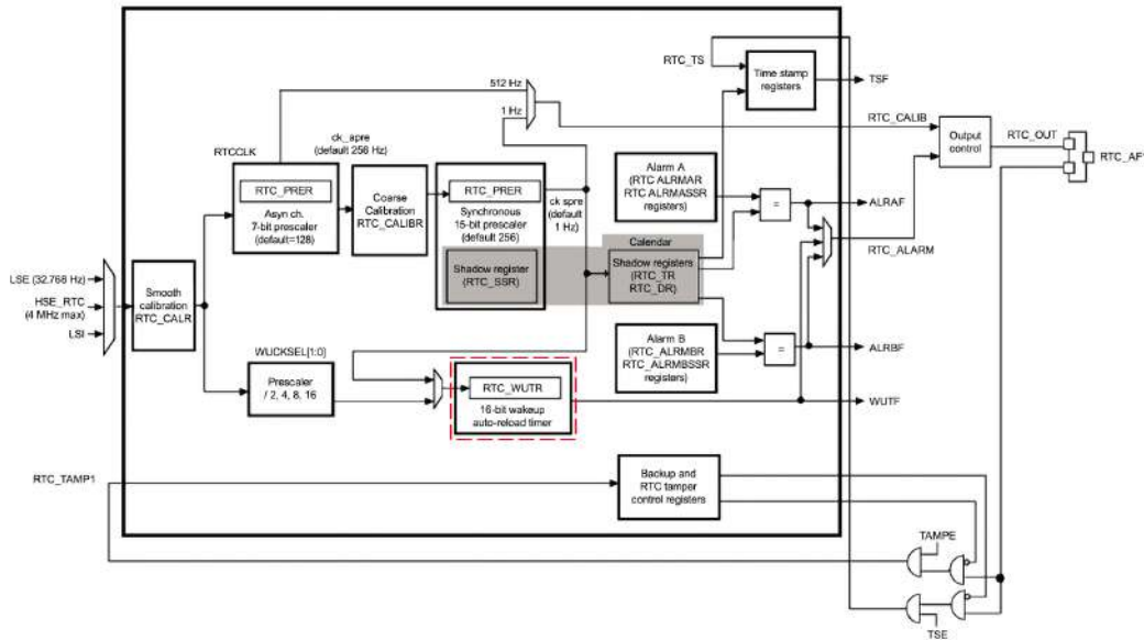
Figure 15.5: RTC block diagram – wakeup timer
