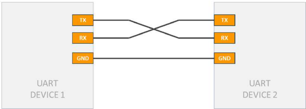
Figure 10.1: The UART interface
