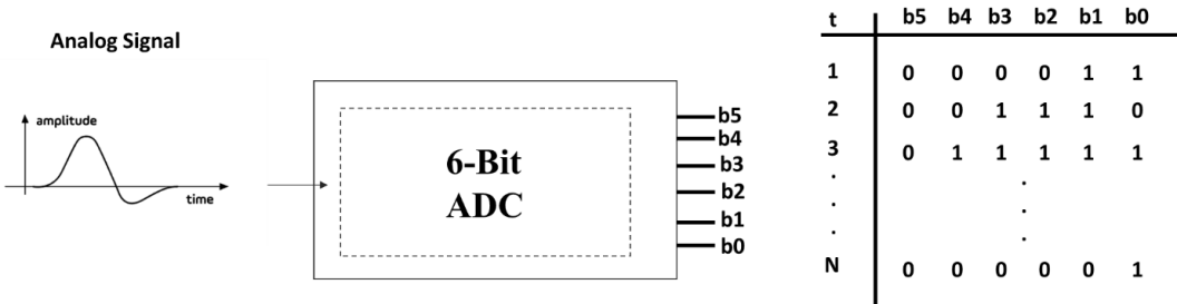
Figure 11.2: The encoding process
