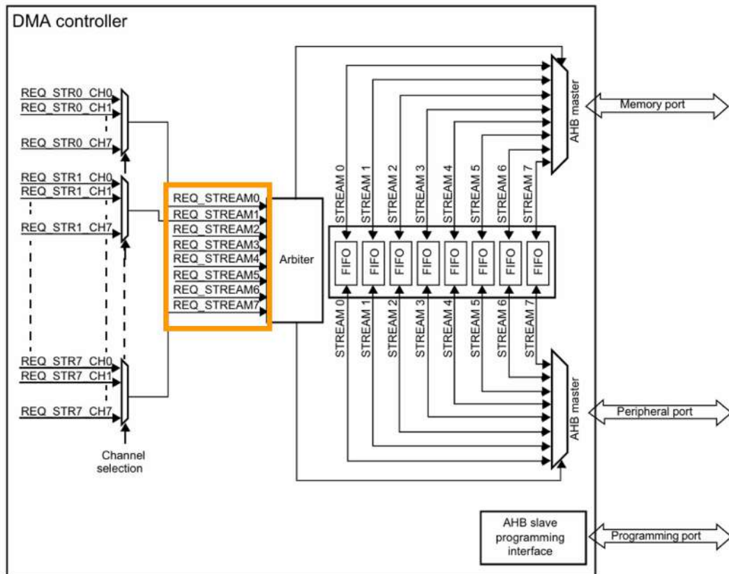
Figure 17.2: The DMA module, indicating the streams
