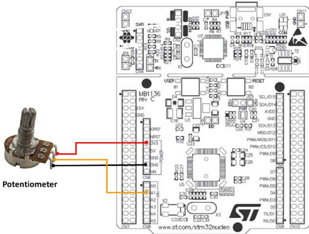
Figure 11.5: Potentiometer connection
