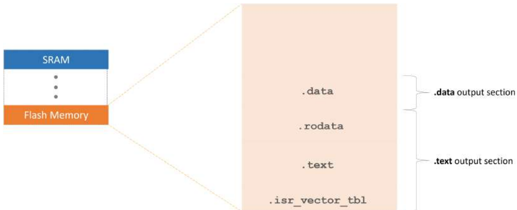
Figure 4.7: The flash memory area showing the order in which sections should be placed
