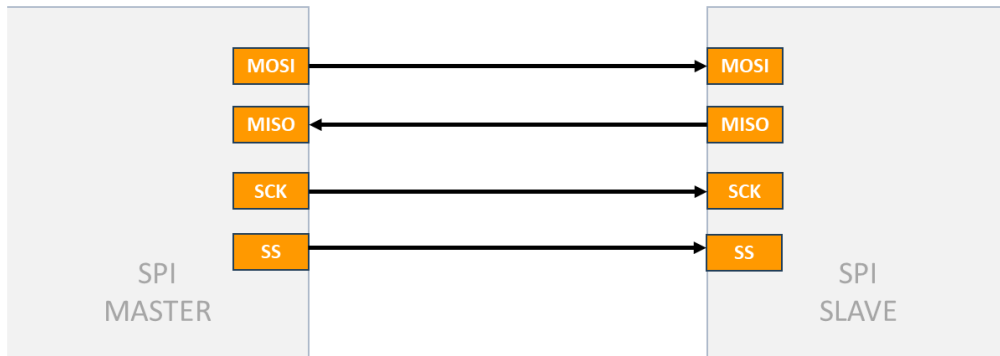
Figure 12.1: The SPI interface
