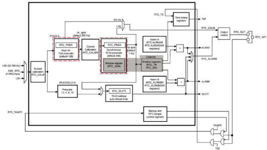
Figure 15.2: RTC block diagram – asynchronous and synchronous prescalers
