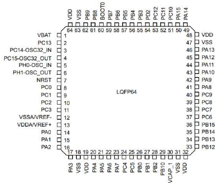
Figure 2.10: STM32F411 pinout
