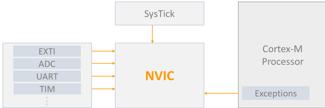
Figure 14.1: The NVIC
