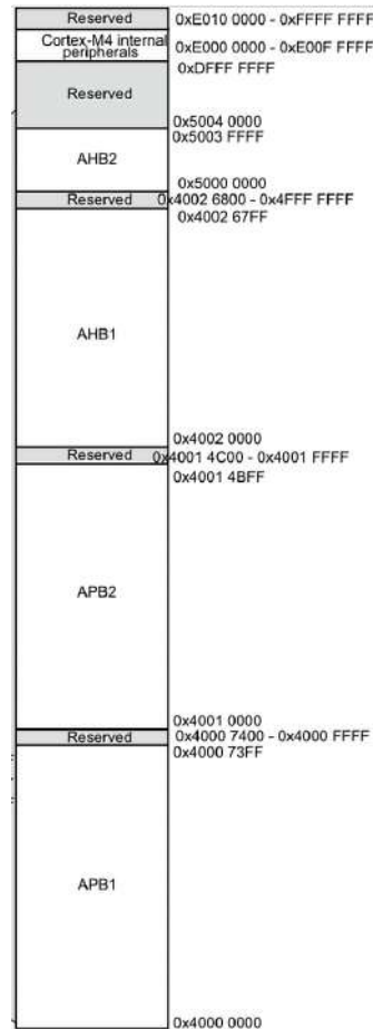
Figure 2.12: Peripherals memory map
