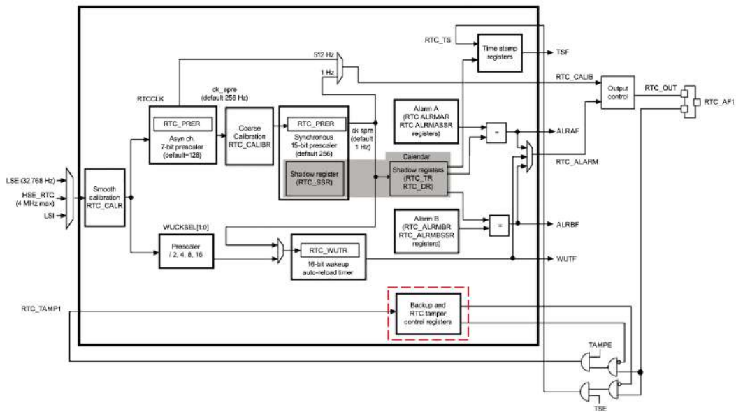
Figure 15.6: RTC block diagram – backup and control registers
