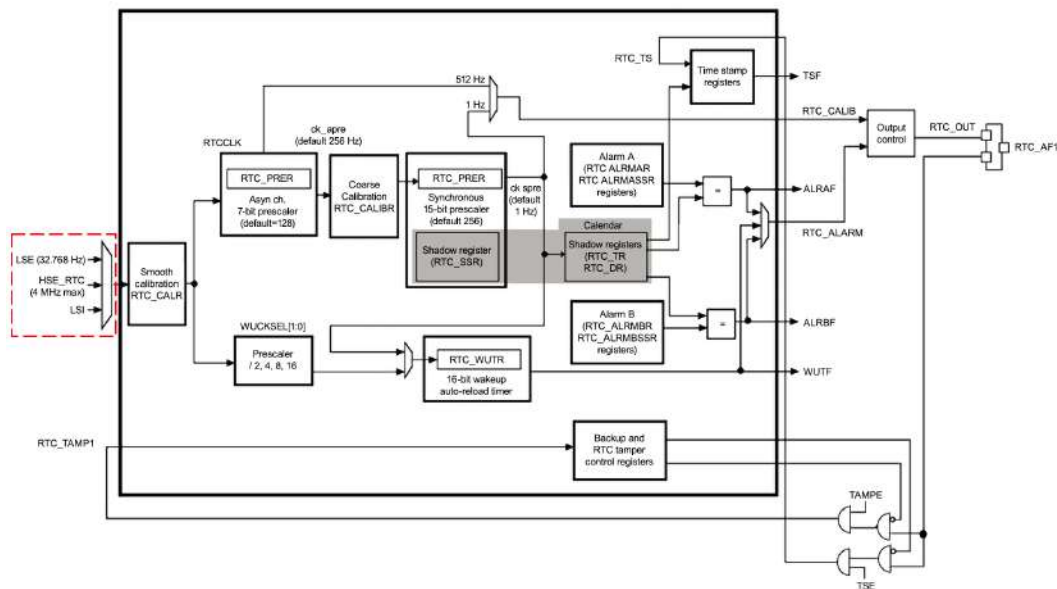
Figure 15.1: RTC block diagram with clock sources highlighted
