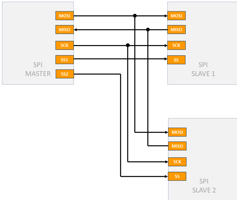
Figure 12.2: The SPI interface – multiple slaves
