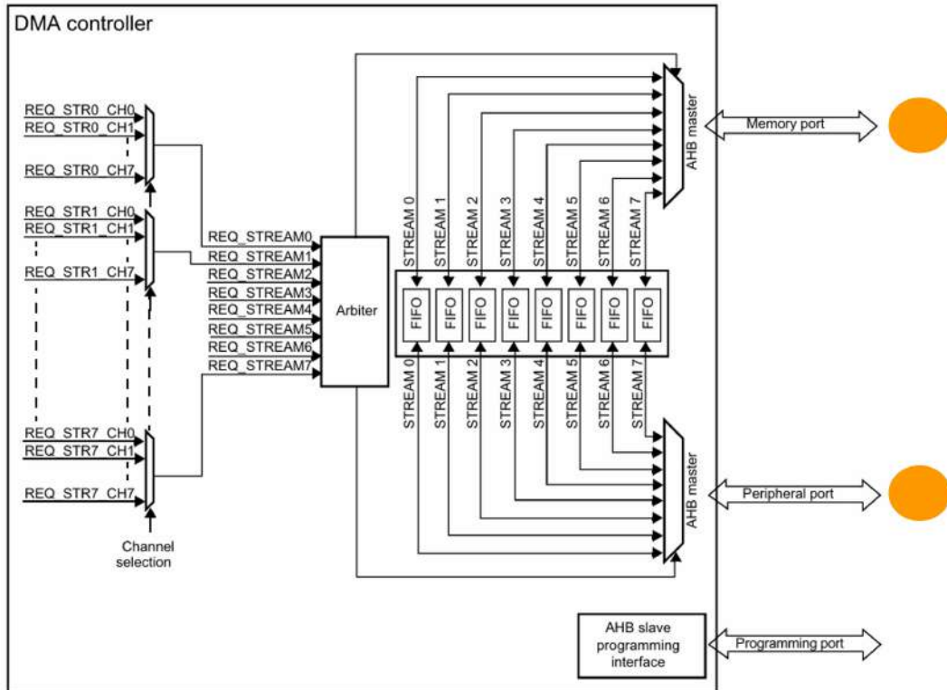
Figure 17.1: The DMA module, indicating the data transfer ports
