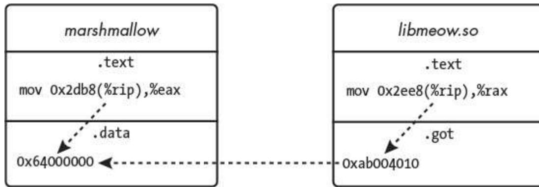
Figure 17-2: The references between object files after relocation
