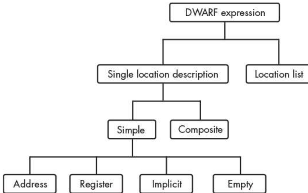
Figure 19-1: The taxonomy of DWARF expressions
