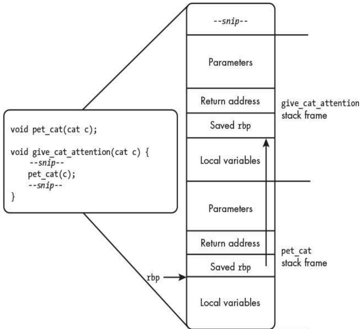
Figure 14-1: A simplified x64 stack with base pointers
