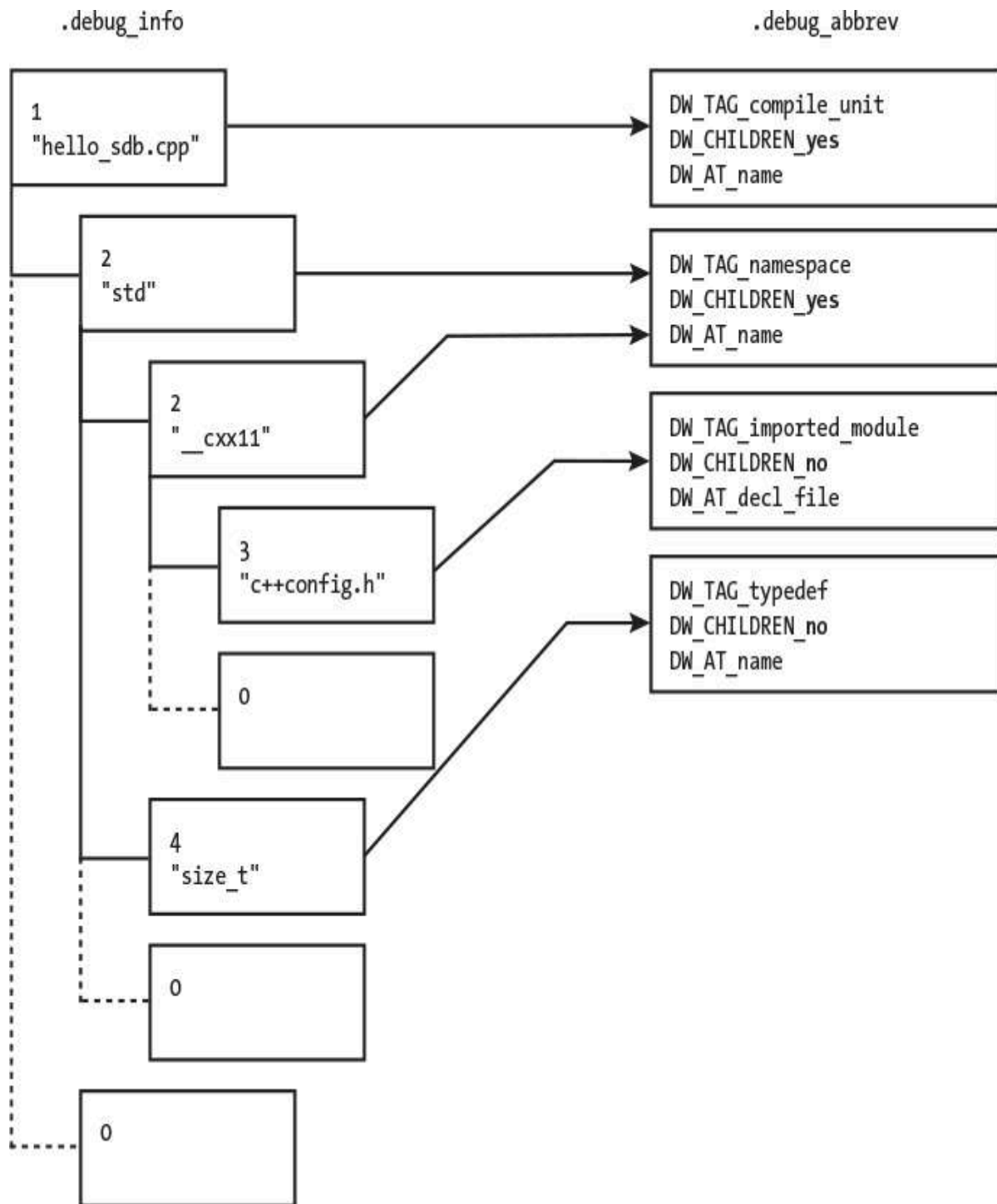
Figure 12-1: A simplified visualization of the DIE tree's encoding
