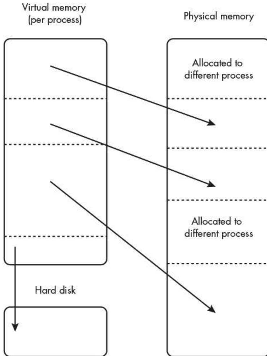
Figure 2-4: Virtual memory translation
