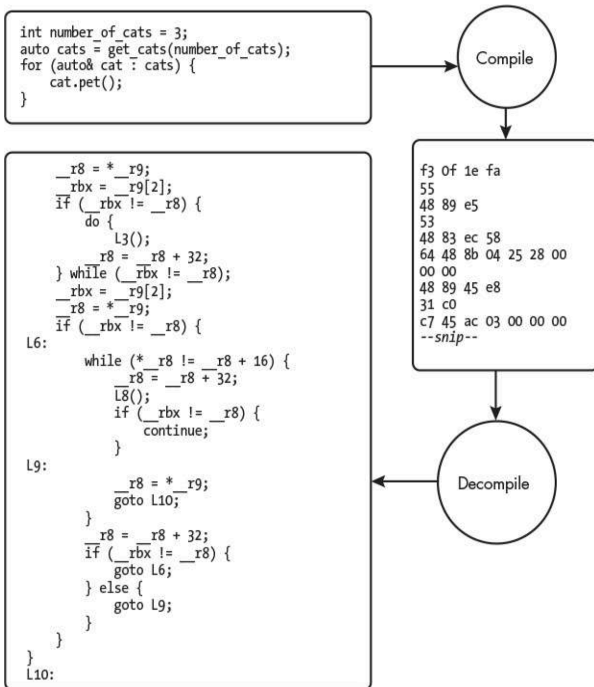
Figure 2-1: Compilation is a lossy process.
