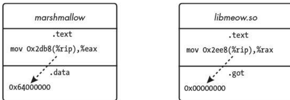
Figure 17-1: The references between object files before relocation
