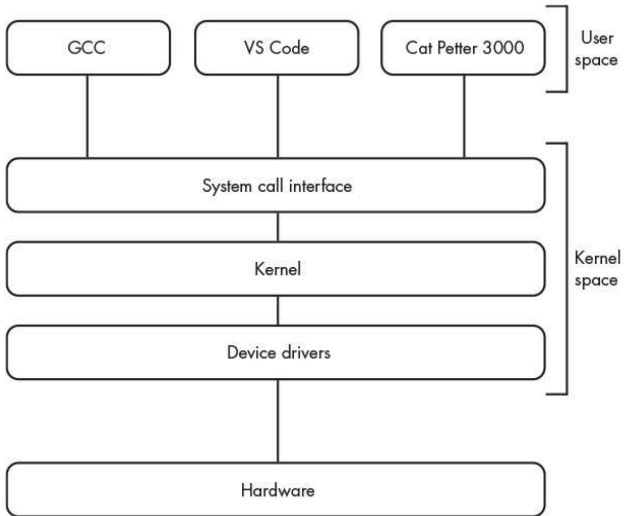
Figure 2-3: The separation of user space and kernel space
