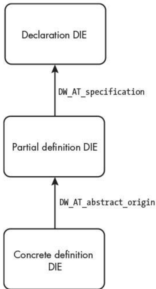
Figure 21-1: A chain of member function DIEs
