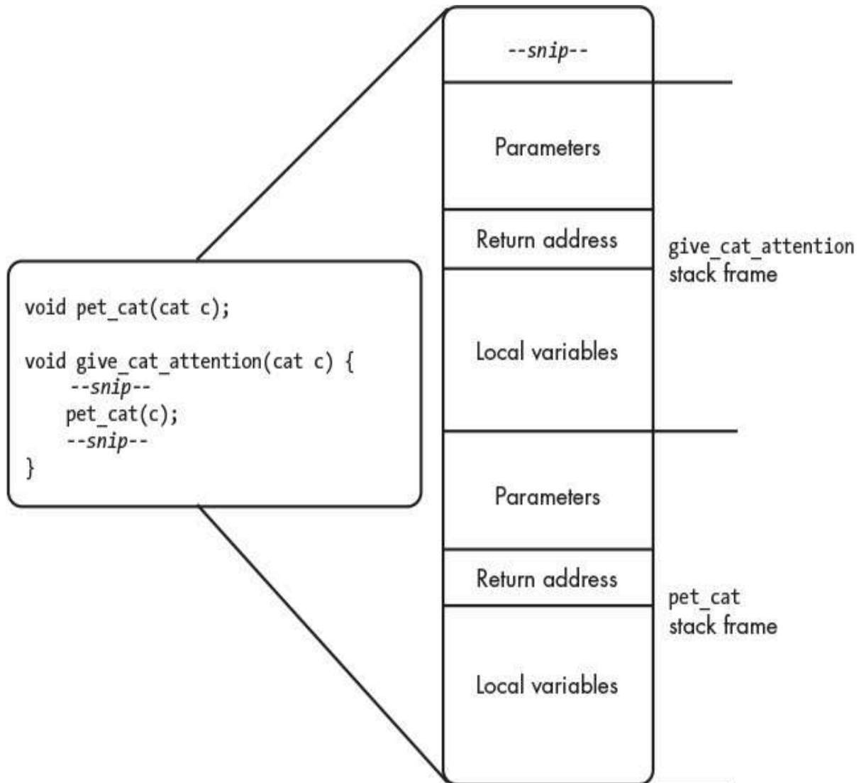
Figure 2-5: A simplified stack
