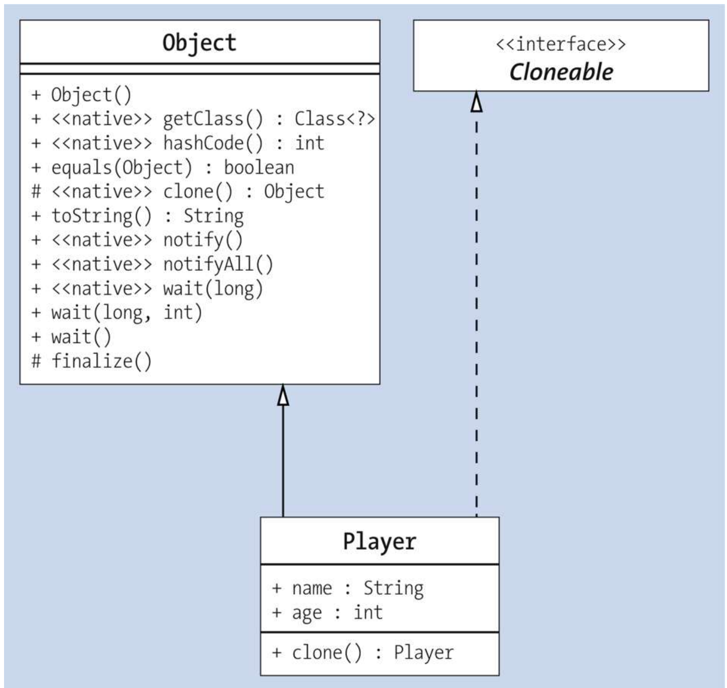
Figure 11.2 Player Extends Object and Implements Cloneable
