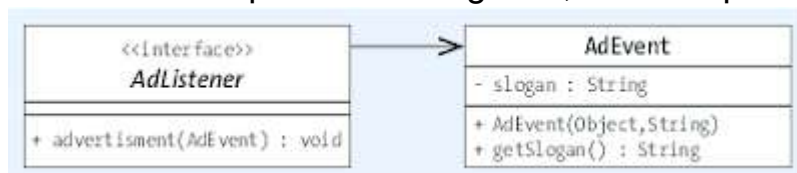
Figure 14.2 UML Class Diagram of AdListener Referencing AdEvent
