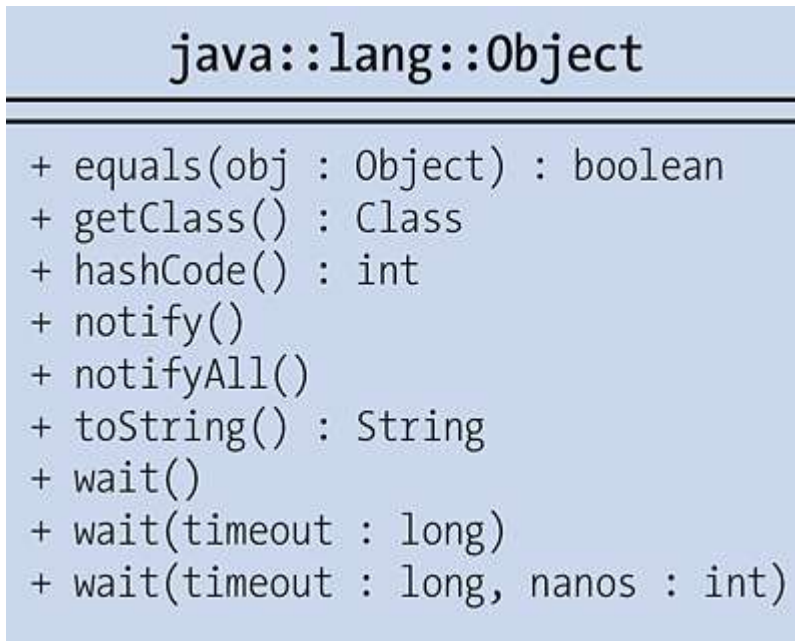
Figure 11.1 Unified Modeling Language (UML) Diagram of Object, the Absolute Base Class
