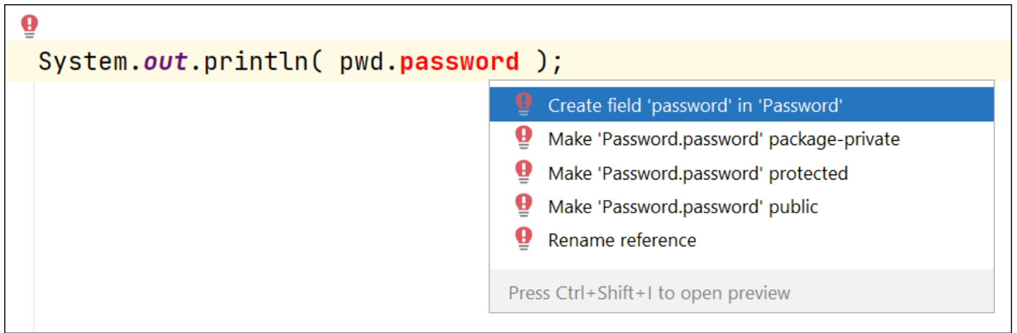
Figure 6.7 With an Error Caused by the Wrong Visibility, IntelliJ Can Change Visibility via Ctrl+Enter
