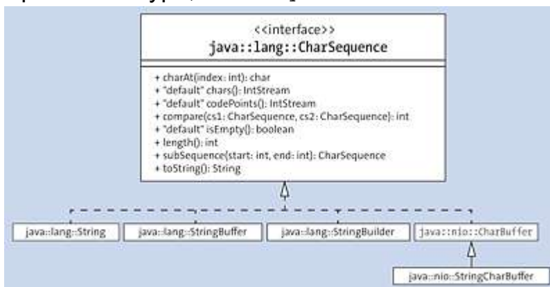
Figure 5.3 Some Implementing Classes of the CharSequence Interface
