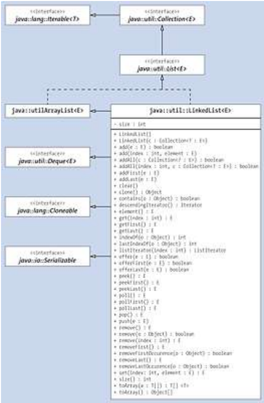
Figure 18.1 Unified Modeling Language (UML) Class Diagram of LinkedList with Inheritance Relationships
