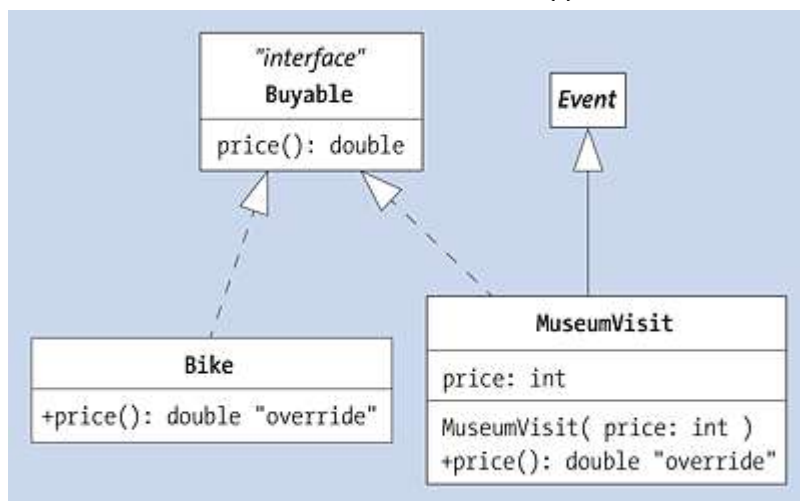
Figure 8.1 UML Diagram of the Buyable Interface and the Bike and MuseumVisit Implementations
