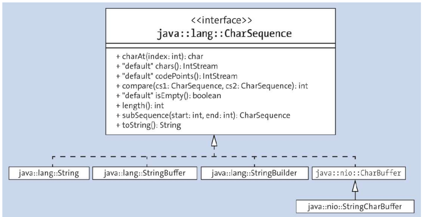
Figure 5.3 Some Implementing Classes of the CharSequence Interface
