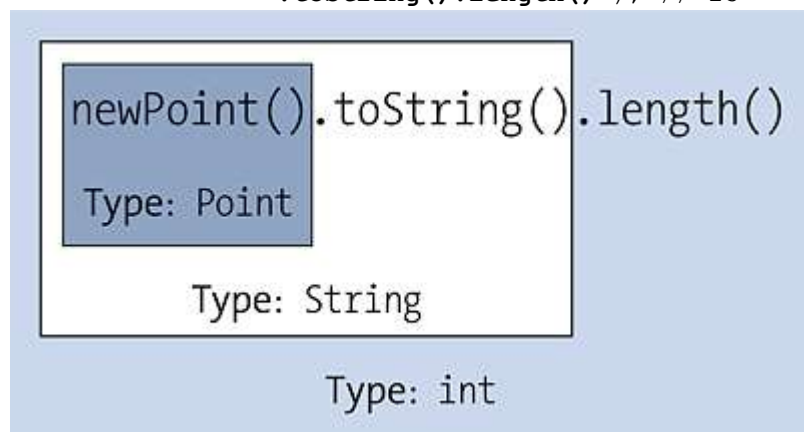
Figure 3.5 Each Nesting Results in a New Type
