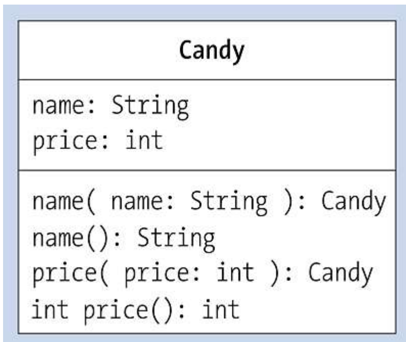
Figure 6.5 UML Class Diagram for Candy with the Fluent API
