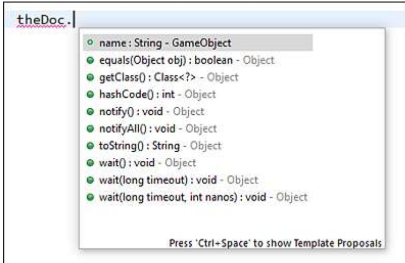
Figure 7.9 Methods from the Absolute Superclass java.lang.Object
