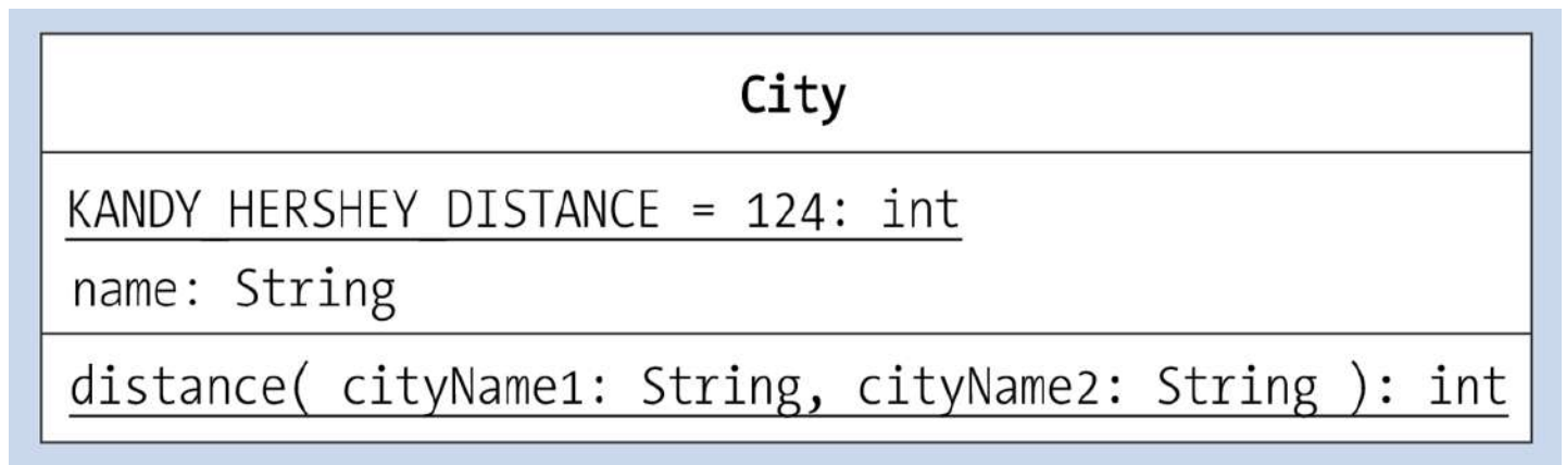
Figure 6.8 UML Diagram with Static Members Underlined
