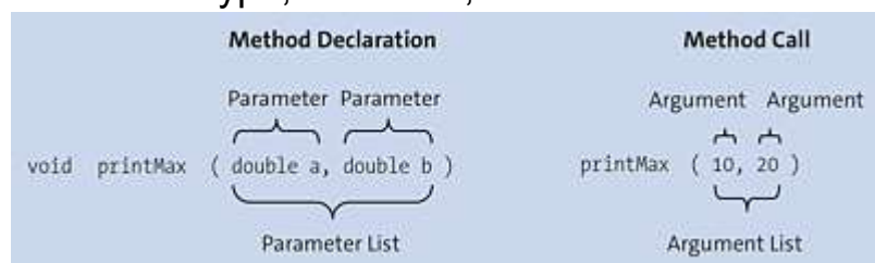
Figure 2.12 The Terms “Parameter” and “Argument”
