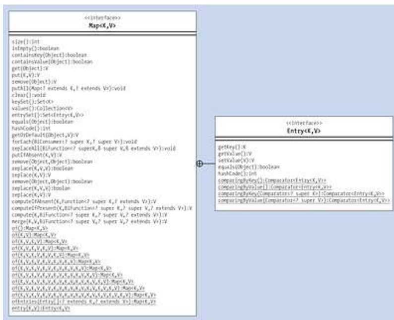
Figure 18.2 UML Class Diagram of the Map Interface
