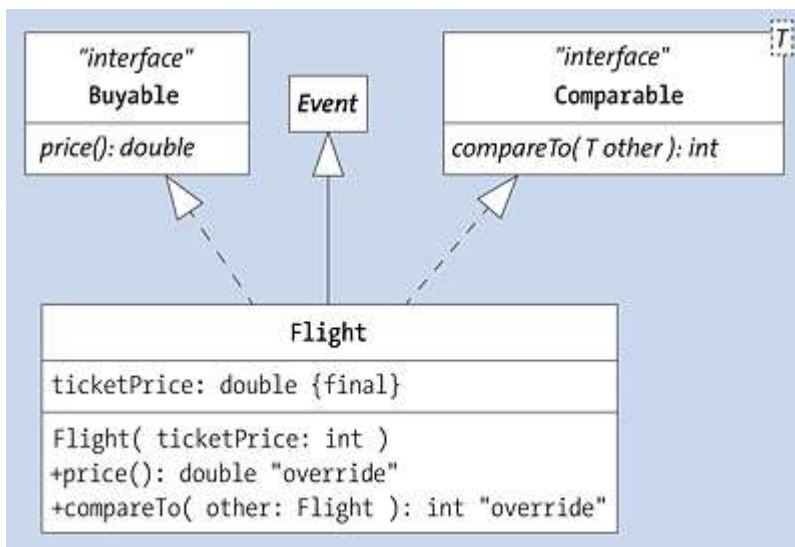
Figure 8.2 The Flight Class with Various Supertypes
