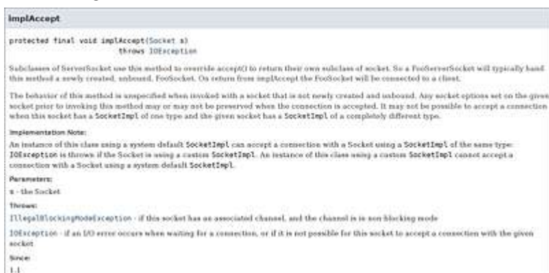
Figure 2.11 Extract from the API Documentation for the java.net.ServerSocket Class
