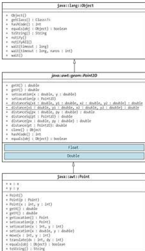
Figure 3.6 Inheritance Hierarchy in Point2D
