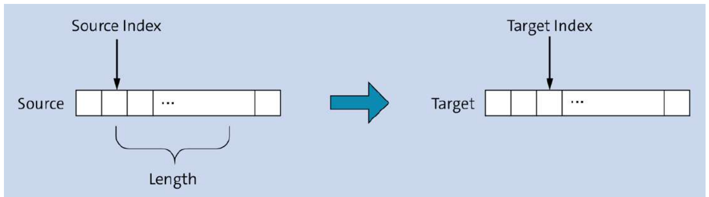
Figure 4.2 Copying the Elements from One Array to Another
