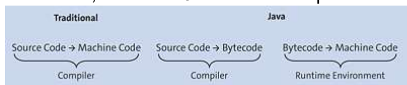
Figure 1.3 The Traditional Compiler and the Java Compiler with the Runtime Environment
