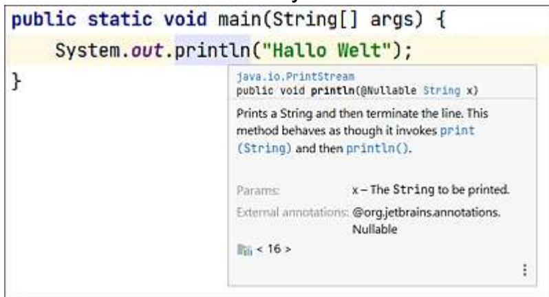
Figure 2.2 IntelliJ Displaying API Documentation in a Small Dialog Box via the Shortcut Ctrl+Q
