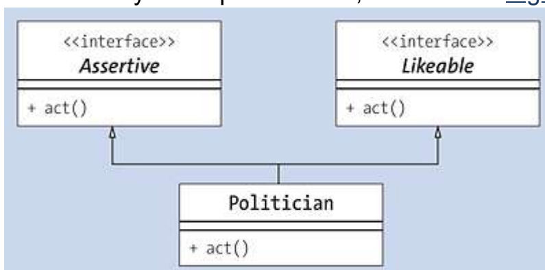
Figure 8.3 A Class Inheriting the Same Operation from Two Interfaces
