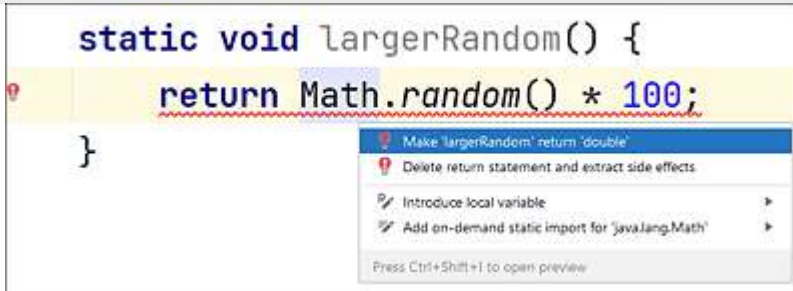
Figure 2.13 IntelliJ Detects If a Return Type Is Missing and Suggests a Suitable Type When Pressing Ctrl+Enter
