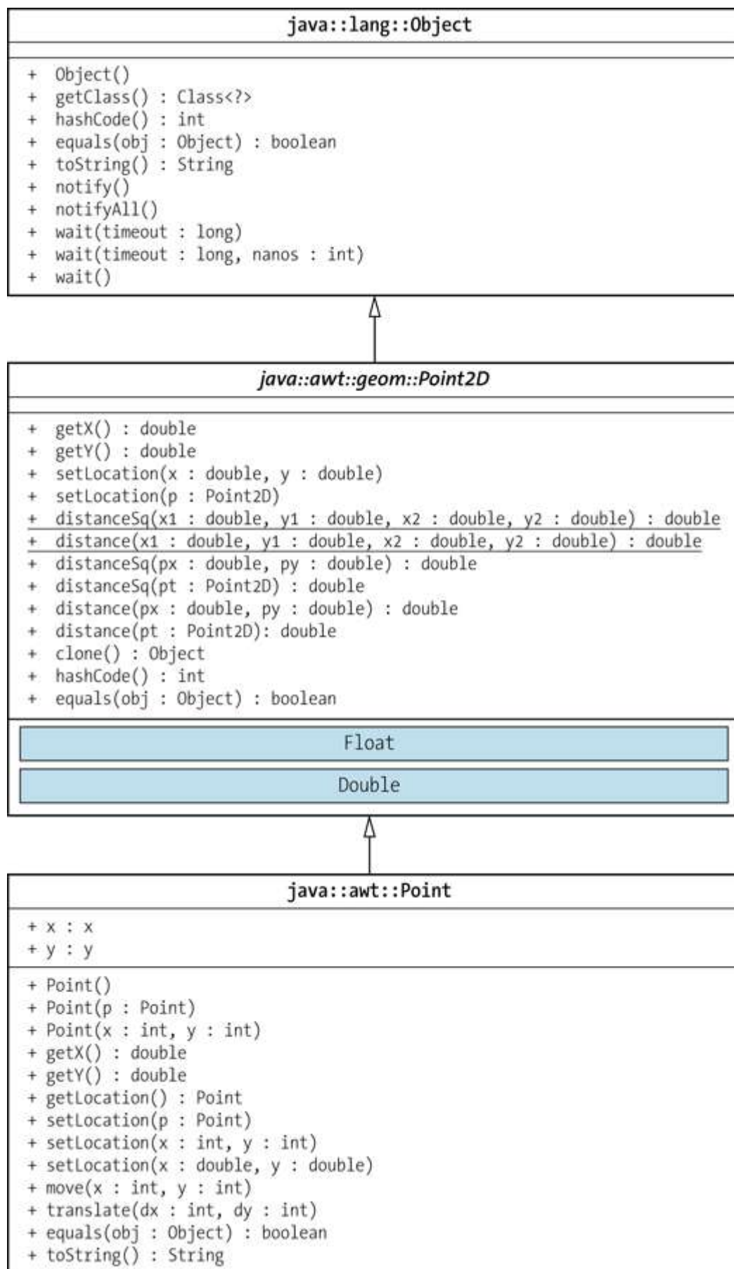
Figure 3.6 Inheritance Hierarchy in Point2D
