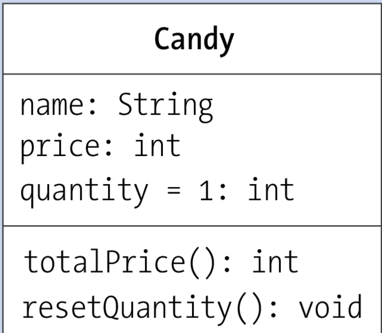
Figure 6.4 UML Class Diagram of Candy with Three Object Variables and Two Methods
