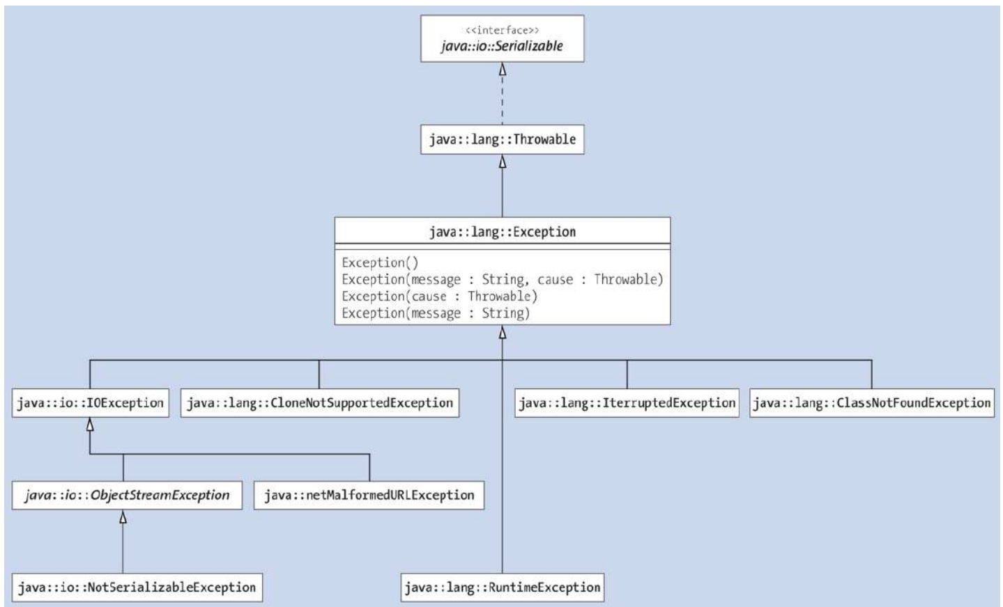
Figure 9.5 Selected Subclasses of the Exception Class
