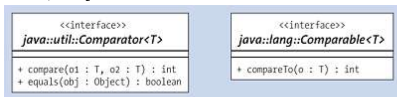
Figure 11.3 Simplified UML Diagram of Comparator and Comparable
