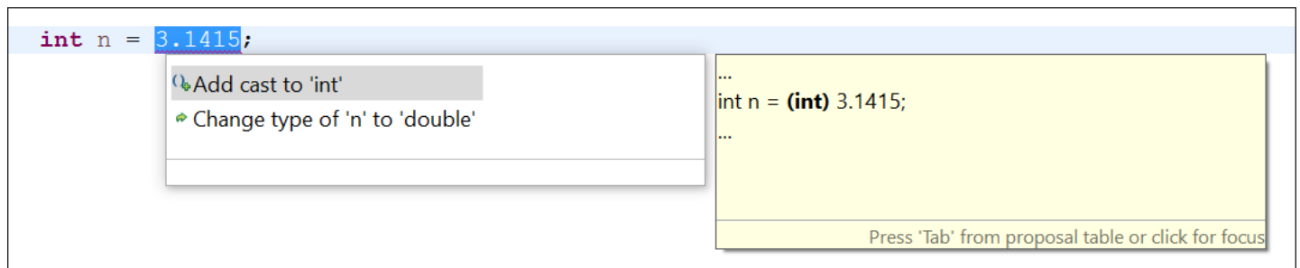
Figure 2.6 If the Type of an Expression Doesn't Fit, Press Ctrl+1
