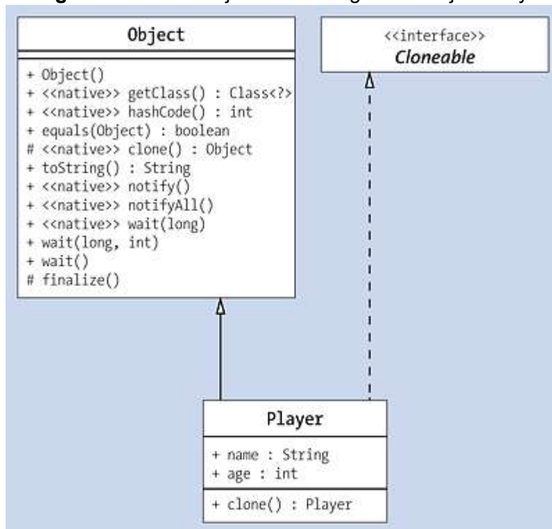
Figure 11.2 Player Extends Object and Implements Cloneable
