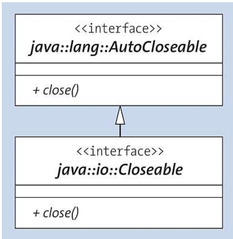
Figure 19.4 Unified Modeling Class (UML) Class Diagram Showing the Inheritance Relationship between Closeable and AutoCloseable
