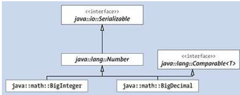
Figure 21.1 The Inheritance Relationship of BigInteger and BigDecimal
