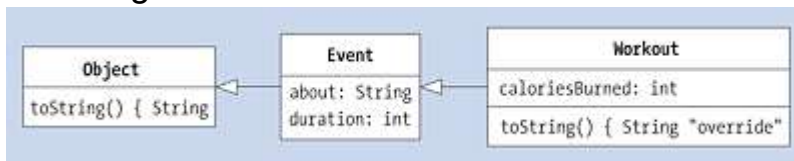
Figure 7.11 Workout as a Subclass of Event and Has Its Own toString() . The UML Stereotype Identifies the Override.
