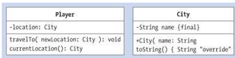
Figure 7.2 UML Diagram of Association via Attributes
