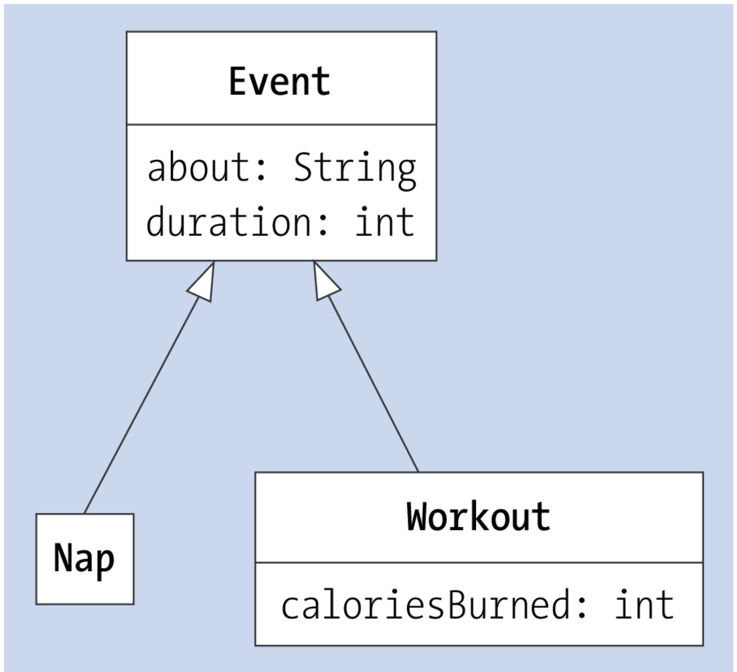
Figure 7.8 Nap and Workout Classes as Two Subclasses of the Event Class
