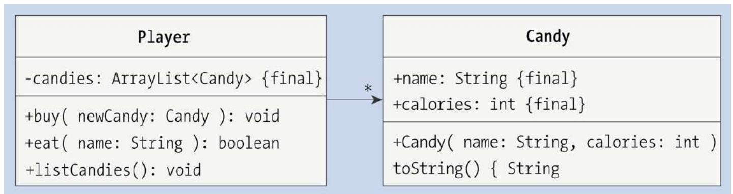
Figure 7.6 UML Diagram where the Player References Any Number of Candies
