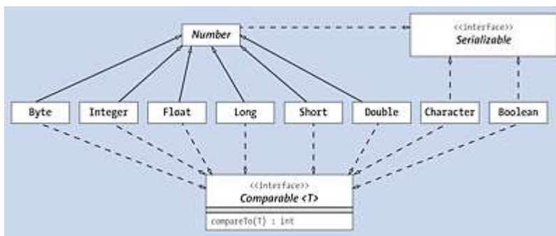
Figure 11.5 Essential Type Relationships of Wrapper Classes: Character Doesn't Extend Number
