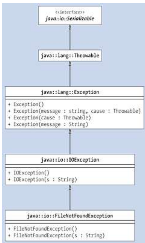
Figure 9.6 IOException in the Class Diagram
