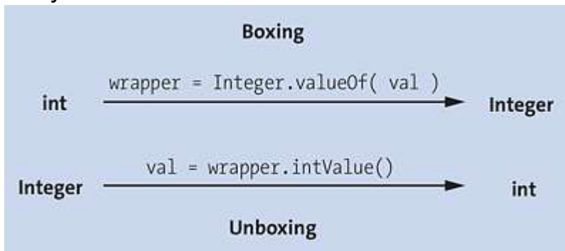
Figure 11.7 Autoboxing of int/Integer
