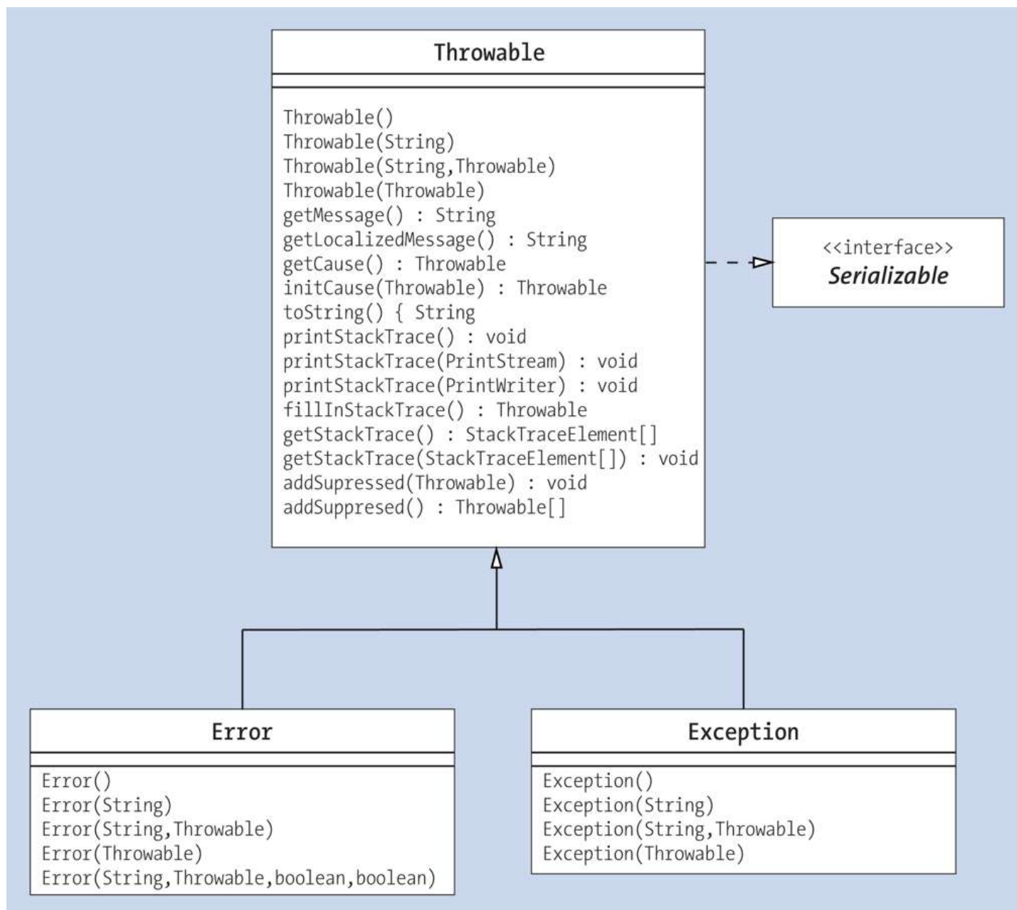
Figure 9.4 Unified Modeling Language (UML) Diagram of the Important Throwable Superclass
