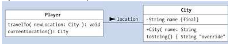
Figure 7.3 UML Diagram of Directed Association
