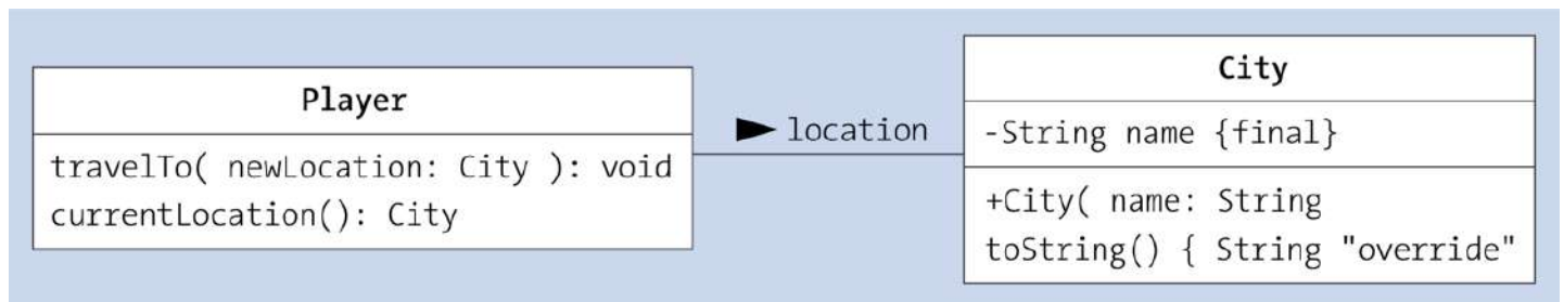
Figure 7.3 UML Diagram of Directed Association
