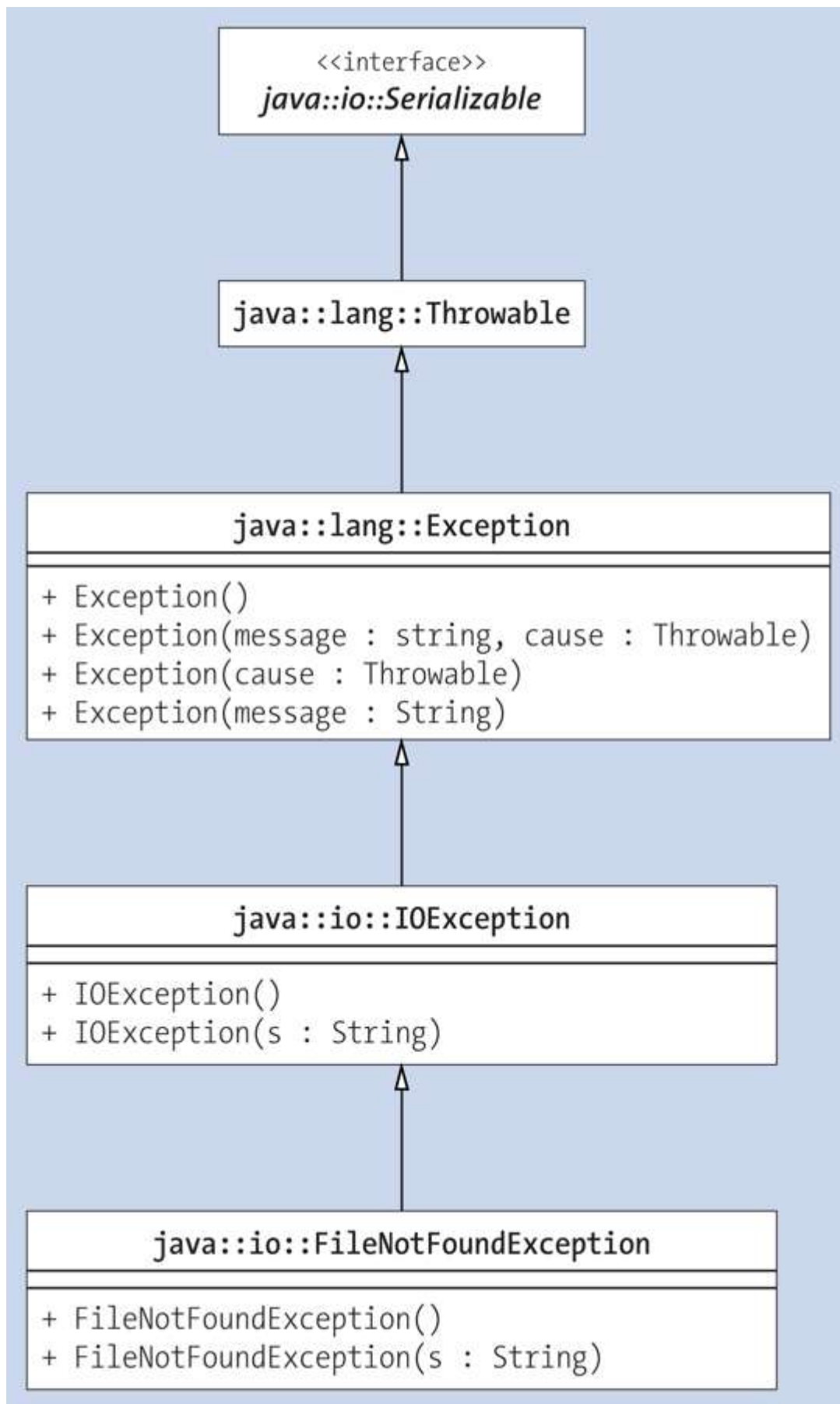
Figure 9.6 IOException in the Class Diagram
