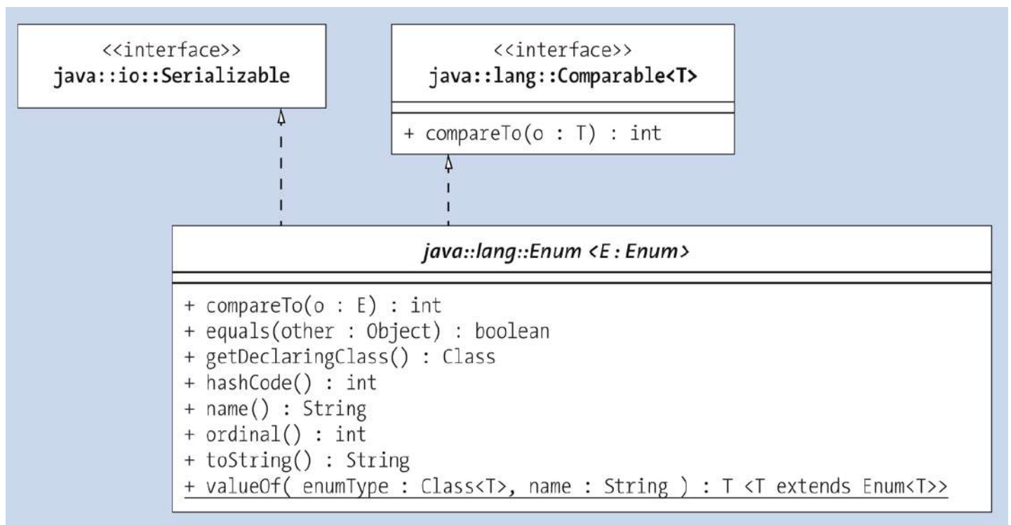
Figure 8.4 Type Relationship of Enum
