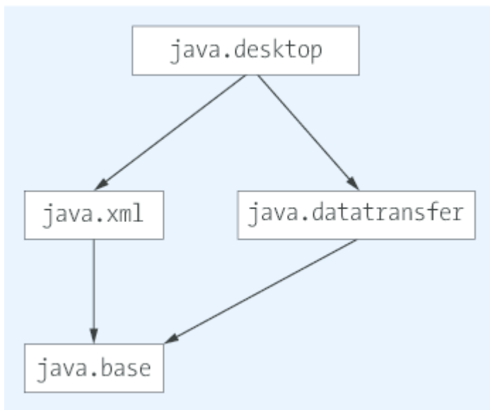
Figure 16.2 Dependencies of the java.desktop Module
