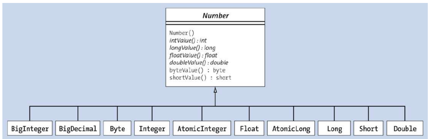
Figure 11.6 UML Diagram of Number
