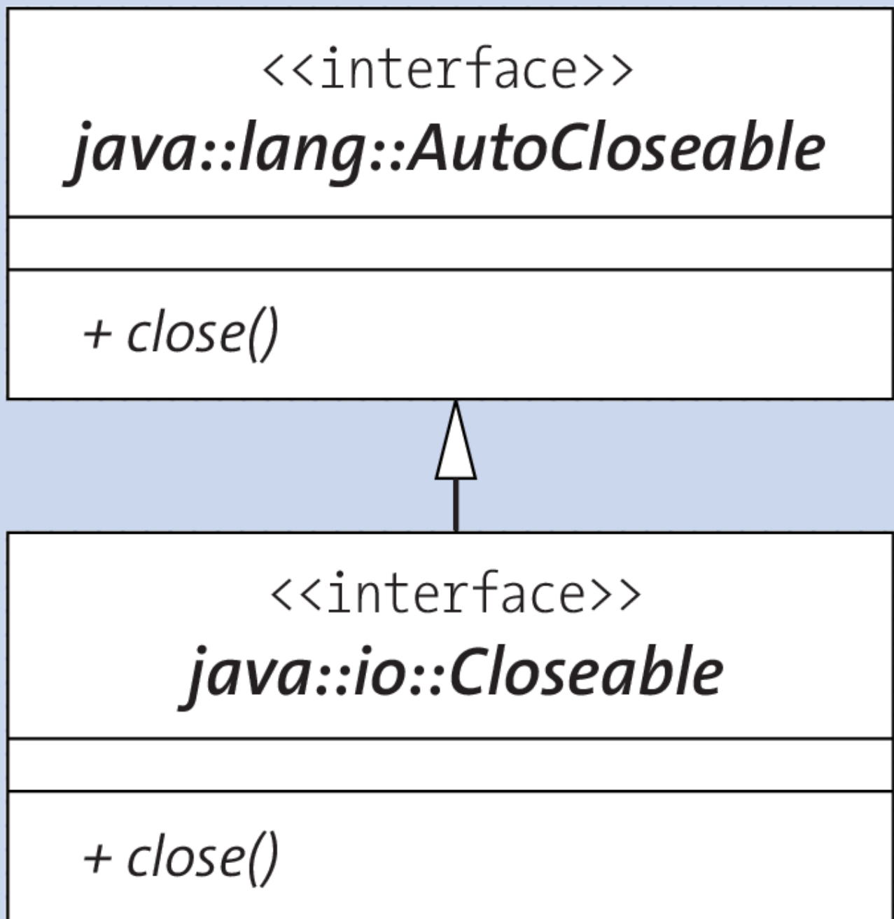
Figure 19.4 Unified Modeling Class (UML) Class Diagram Showing the Inheritance Relationship between Closeable and AutoCloseable
