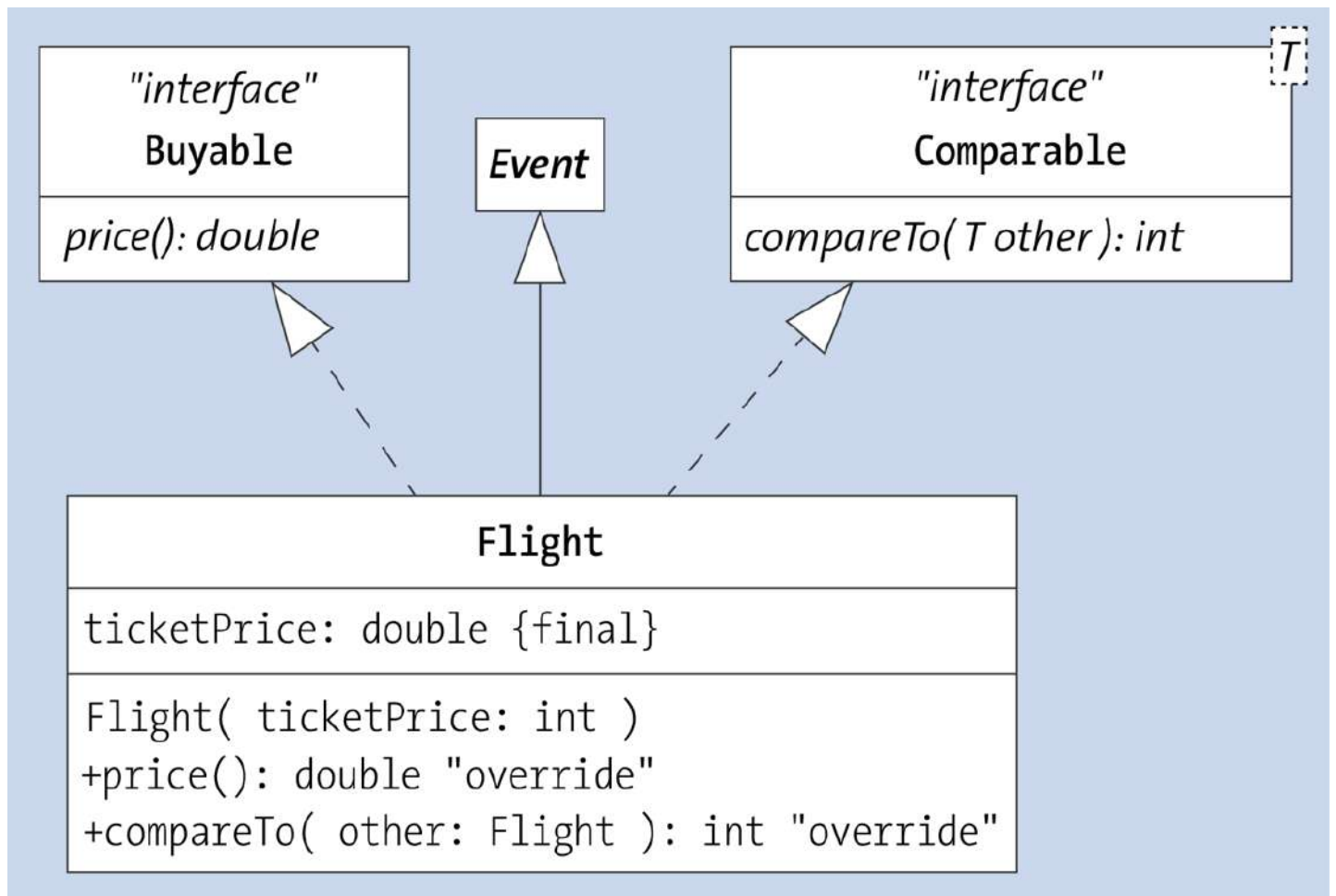
Figure 8.2 The Flight Class with Various Supertypes
