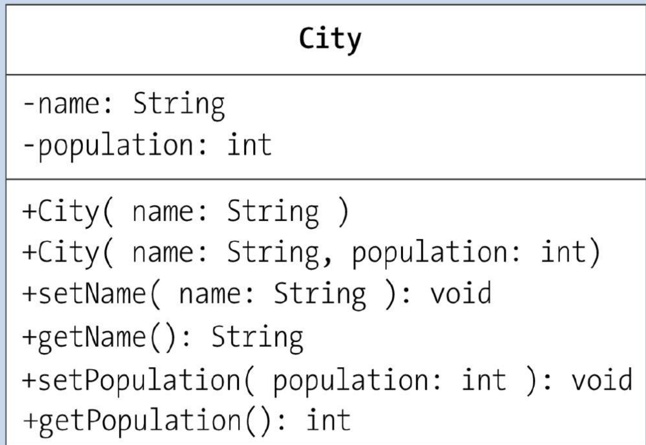
Figure 6.12 UML Diagram for City with Two Constructors
