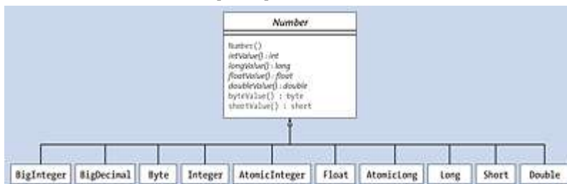
Figure 11.6 UML Diagram of Number
