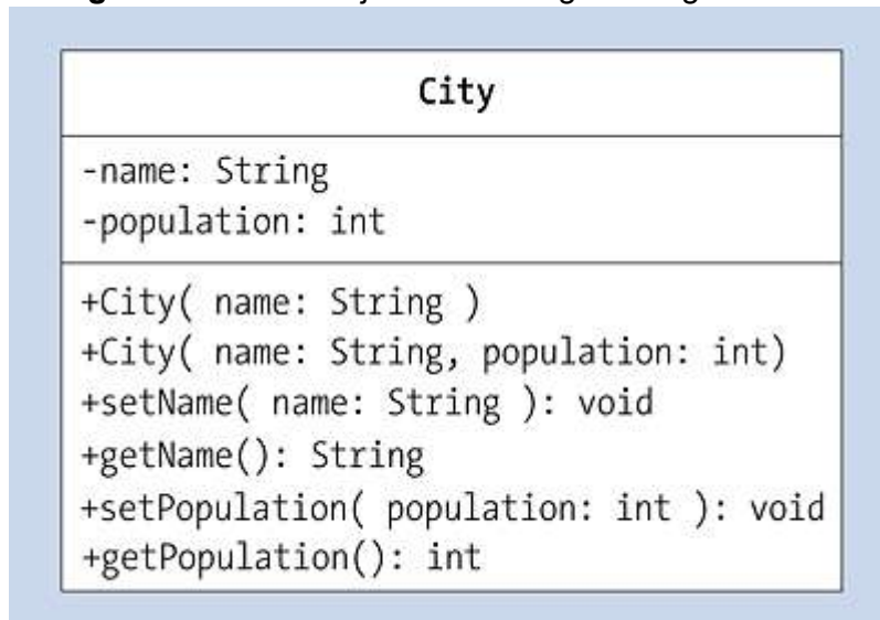
Figure 6.12 UML Diagram for City with Two Constructors
