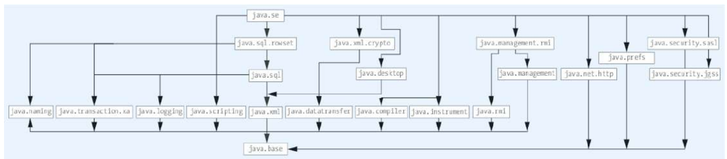
Figure 16.3 Dependencies of the java.se Module
