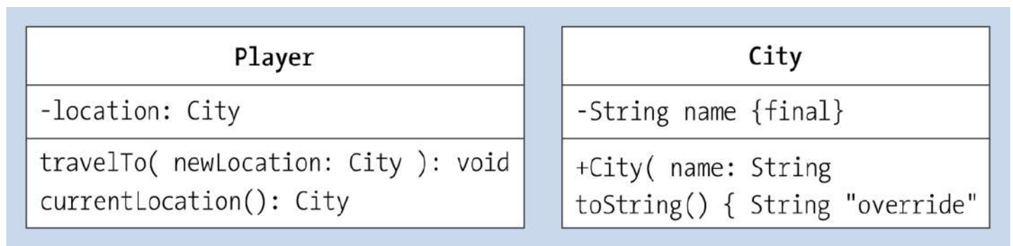
Figure 7.2 UML Diagram of Association via Attributes
