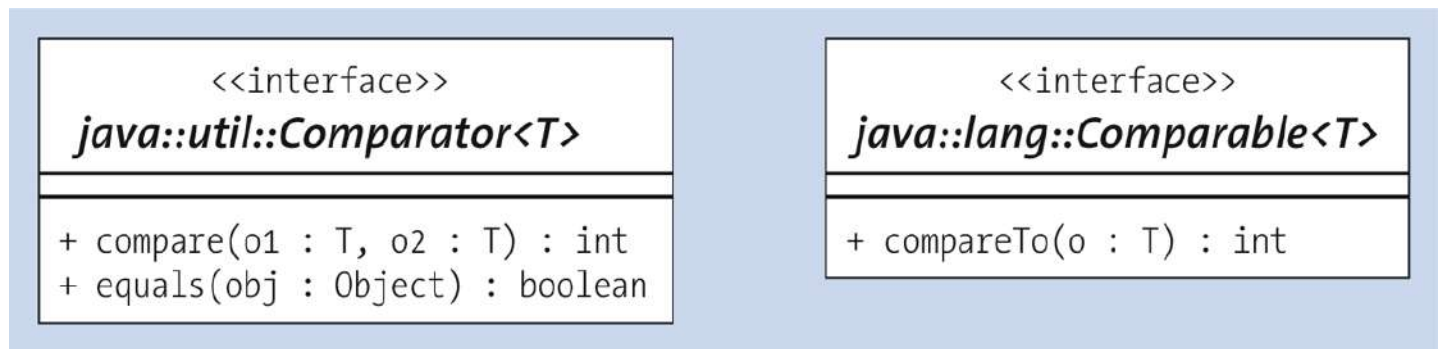
Figure 11.3 Simplified UML Diagram of Comparator and Comparable
