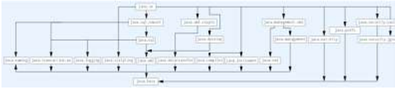
Figure 15.2 Module Dependencies of the java.se Module
