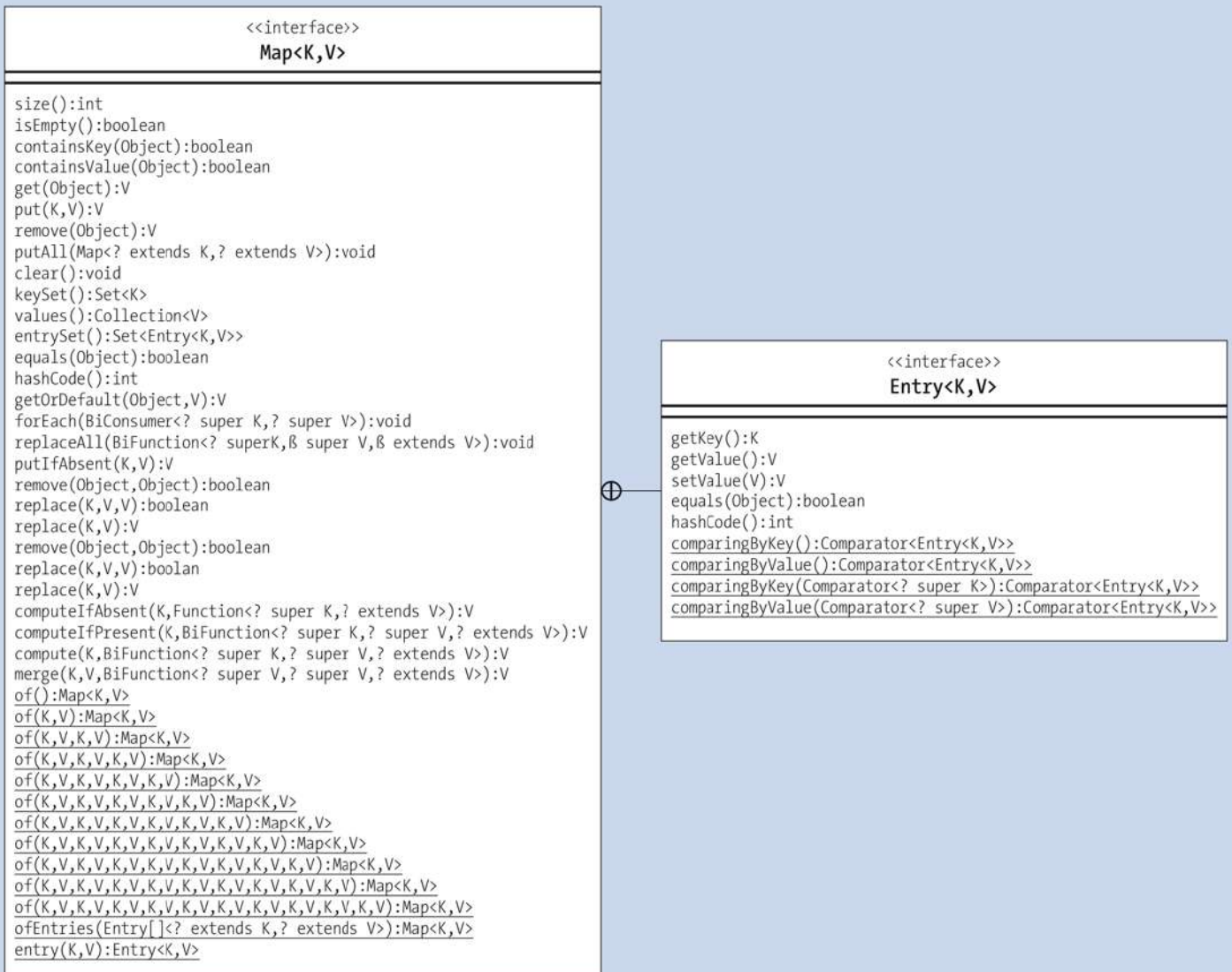
Figure 18.2 UML Class Diagram of the Map Interface
