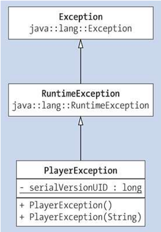
Figure 9.9 UML Diagram for PlayerException package com.tutego.insel.exception.v2 ;
