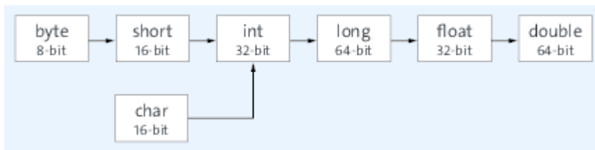
Figure 2.5 Graphical Representation of Automatic Typecasting
