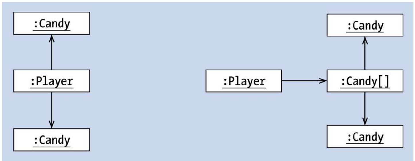
Figure 7.5 The Player Takes over Storage of an Array
