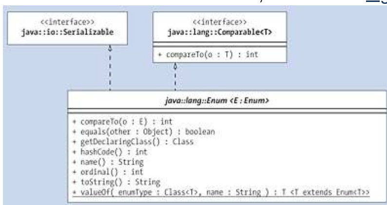
Figure 8.4 Type Relationship of Enum
