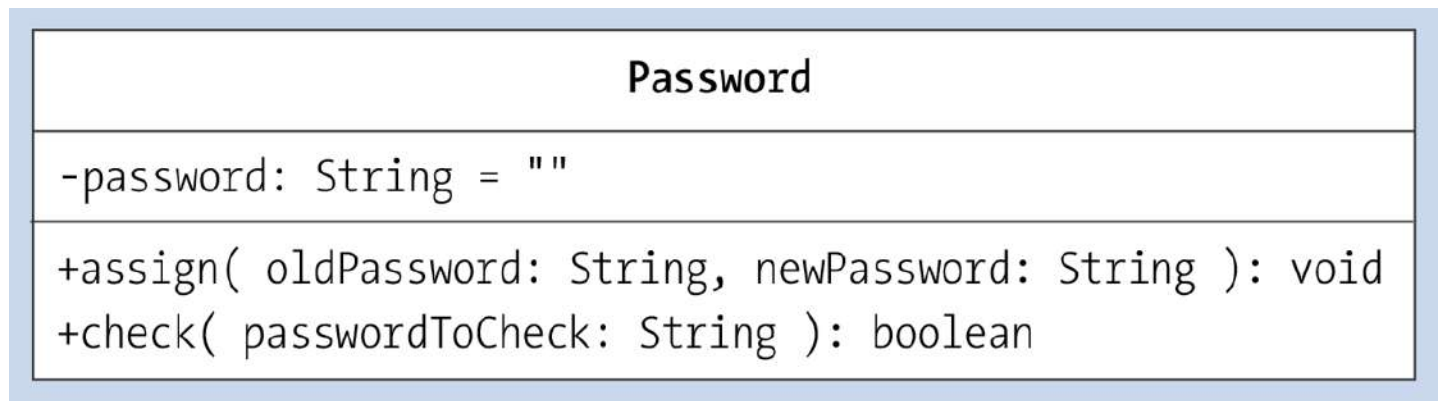
Figure 6.6 UML Diagram Showing Private Members (Minus Signs) and Public Members (Plus Signs)
