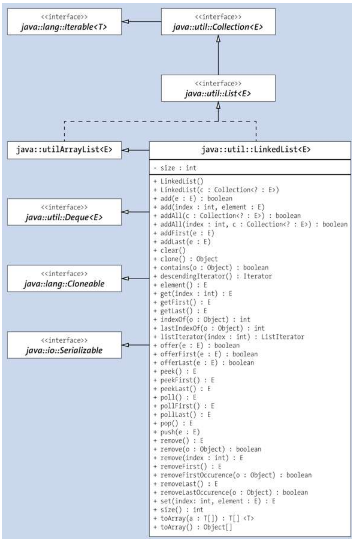
Figure 18.1 Unified Modeling Language (UML) Class Diagram of LinkedList with Inheritance Relationships
