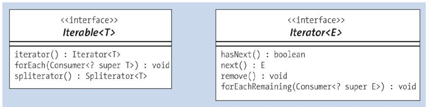
Figure 11.8 UML Diagram of Iterable and Iterator
