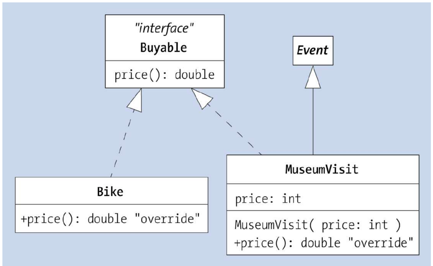
Figure 8.1 UML Diagram of the Buyable Interface and the Bike and MuseumVisit Implementations
