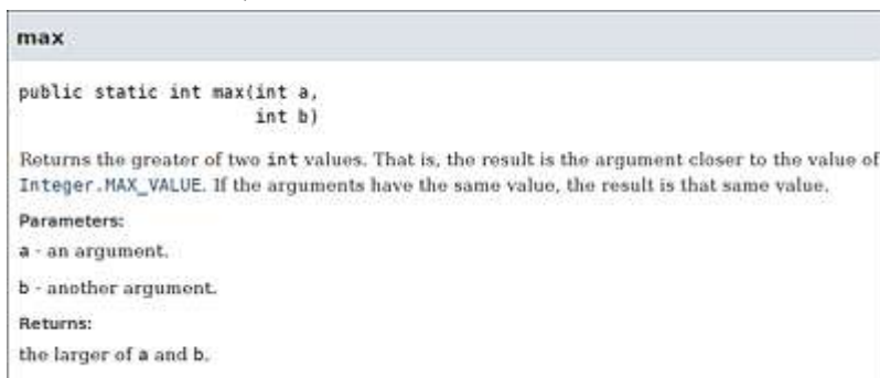
Figure 2.10 The Online API Documentation for Math.max()
