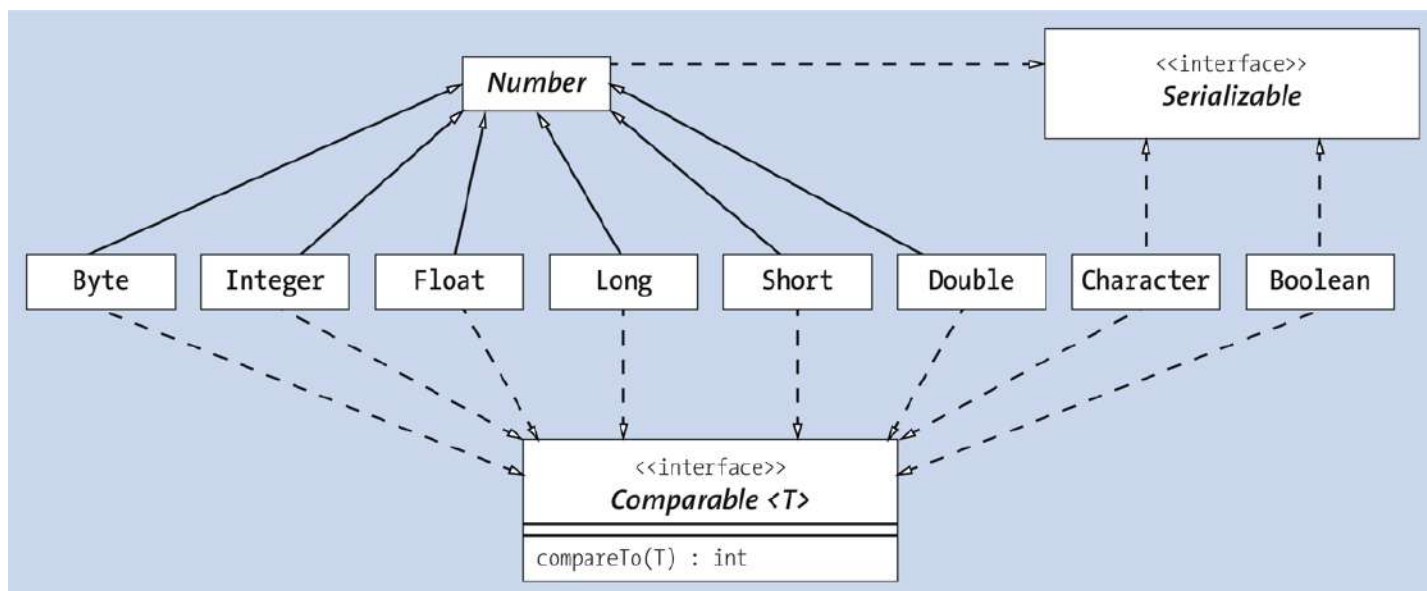
Figure 11.5 Essential Type Relationships of Wrapper Classes: Character Doesn't Extend Number
