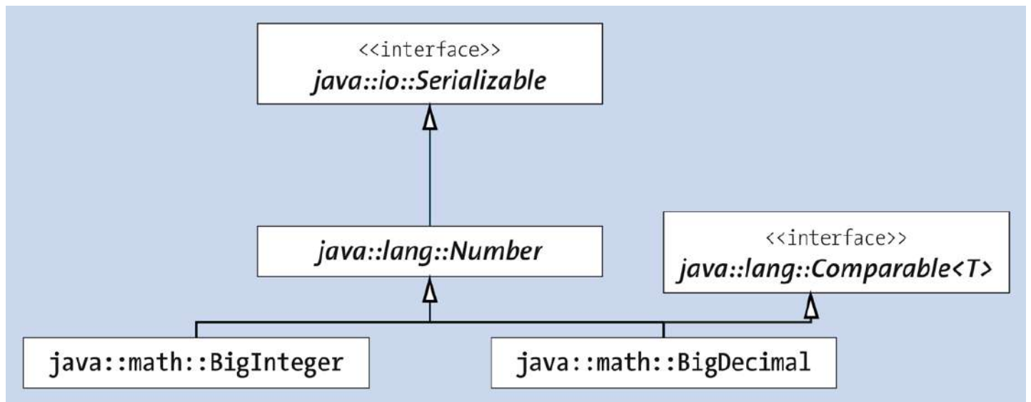
Figure 21.1 The Inheritance Relationship of BigInteger and BigDecimal
