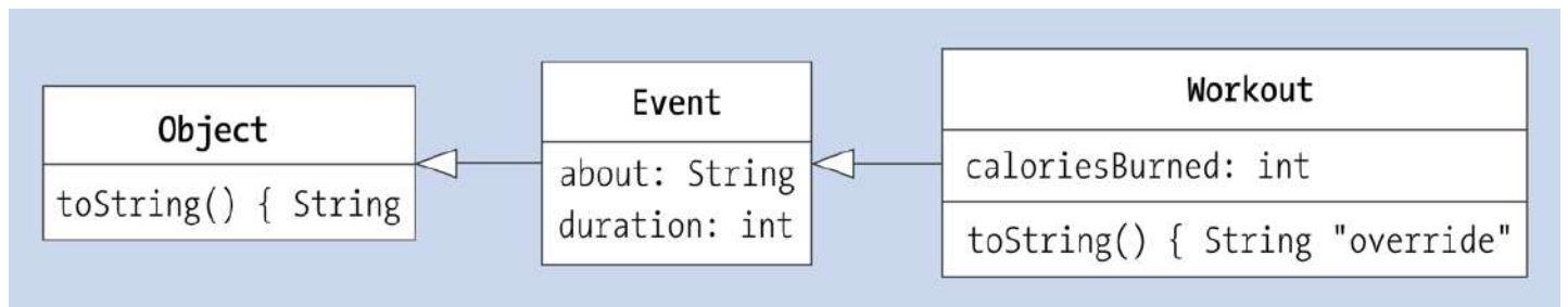
Figure 7.11 Workout as a Subclass of Event and Has Its Own toString() . The UML Stereotype Identifies the Override.
