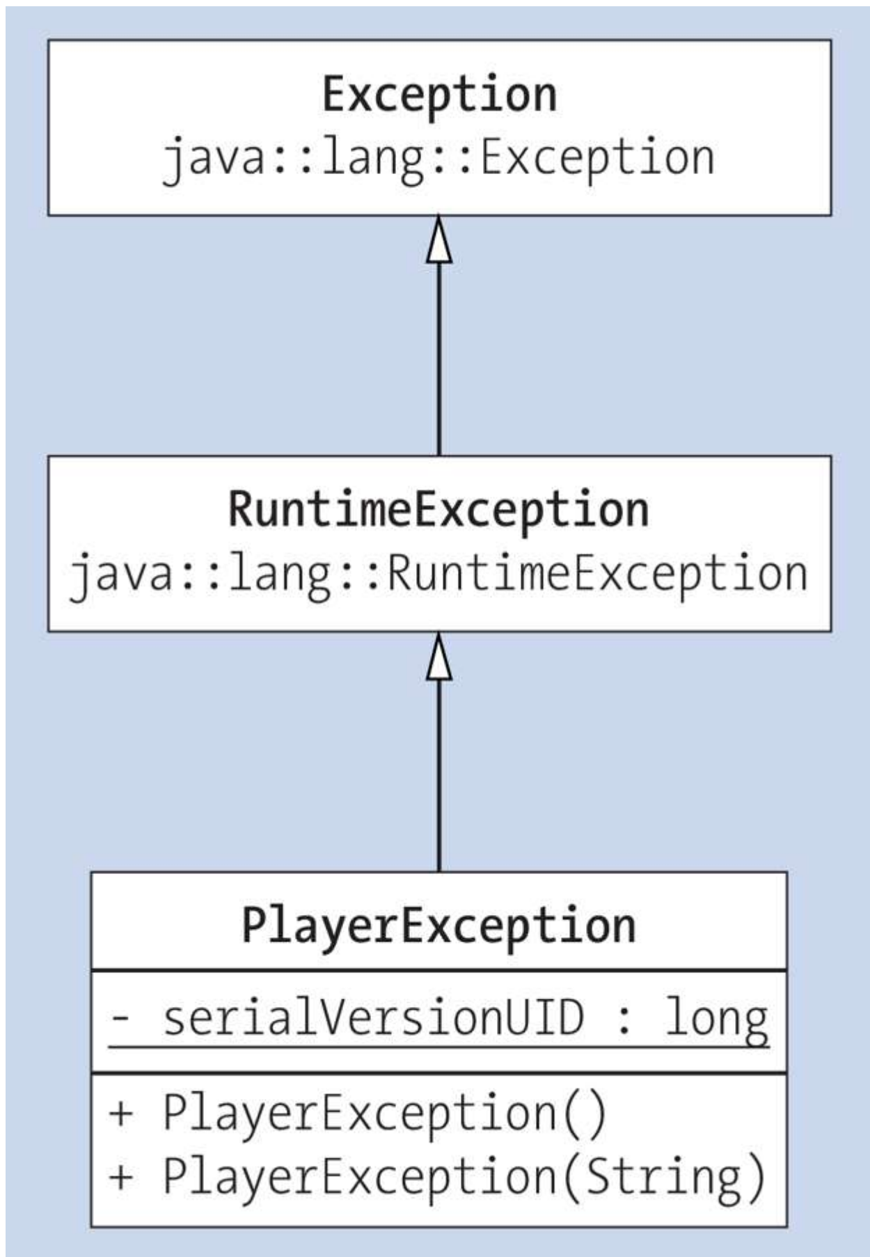
Figure 9.9 UML Diagram for PlayerException
