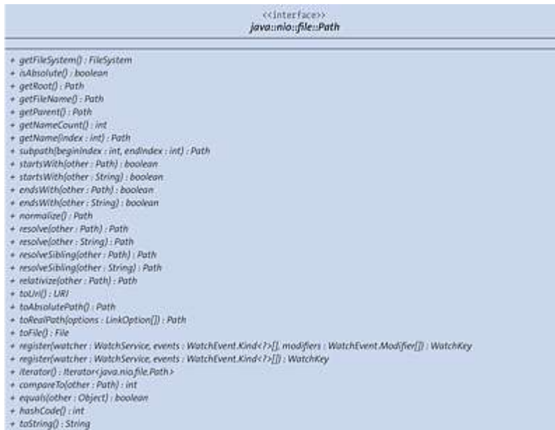
Figure 19.2 The Class Diagram of Path
