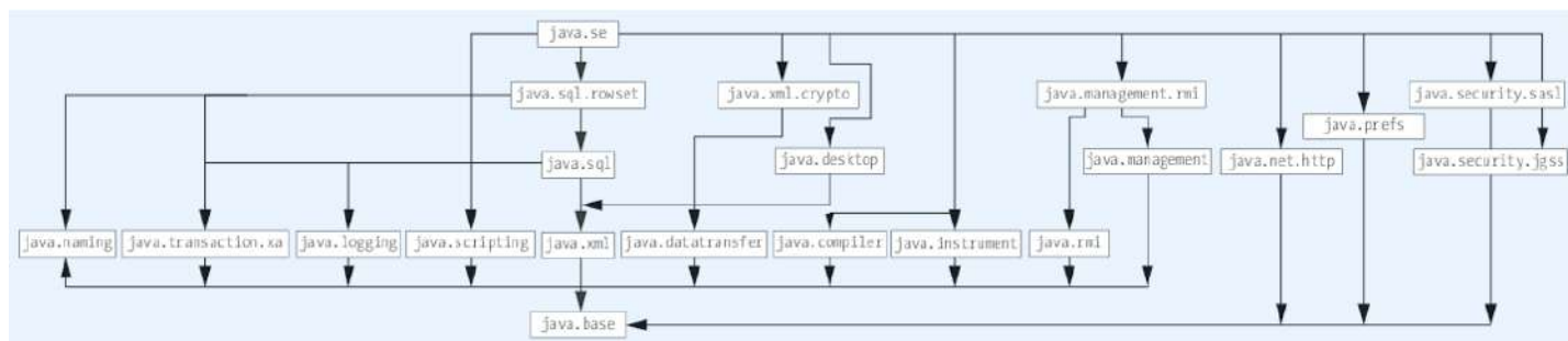
Figure 15.2 Module Dependencies of the java.se Module
