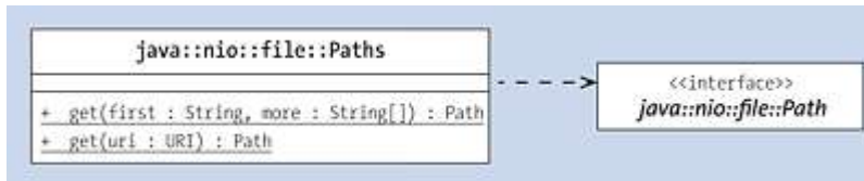
Figure 19.1 Dependencies of the Paths and Path Types
