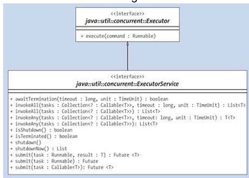
Figure 17.5 The ExecutorService Interface Extends Executor
