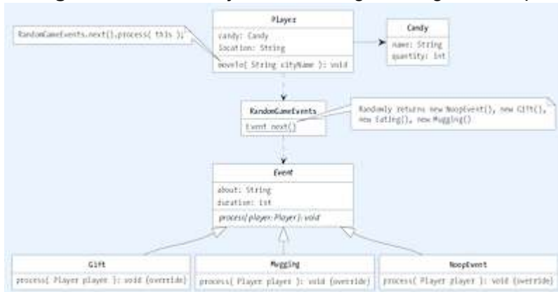
Figure 7.12 UML Diagram Showing the Names of Abstract Classes as Italicized. Subclasses Override the Abstract Method of the Superclass.
