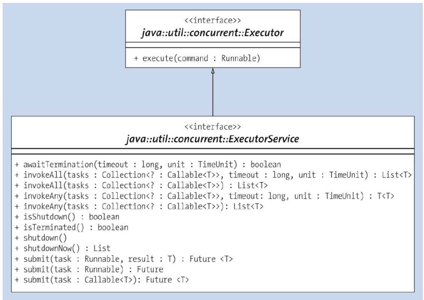
Figure 17.5 The ExecutorService Interface Extends Executor
