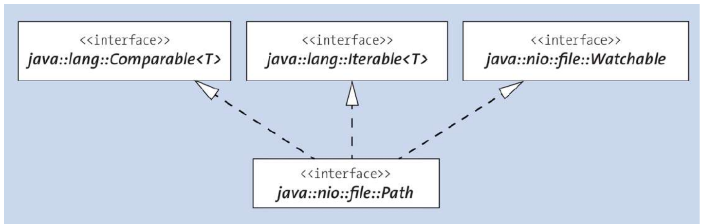
Figure 19.3 The Inheritance Relationship of Path
