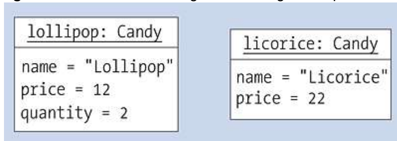
Figure 6.3 UML Object Diagram Showing the Two Candy Instances
