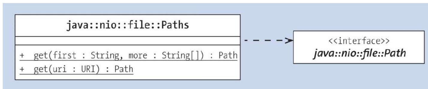
Figure 19.1 Dependencies of the Paths and Path Types
