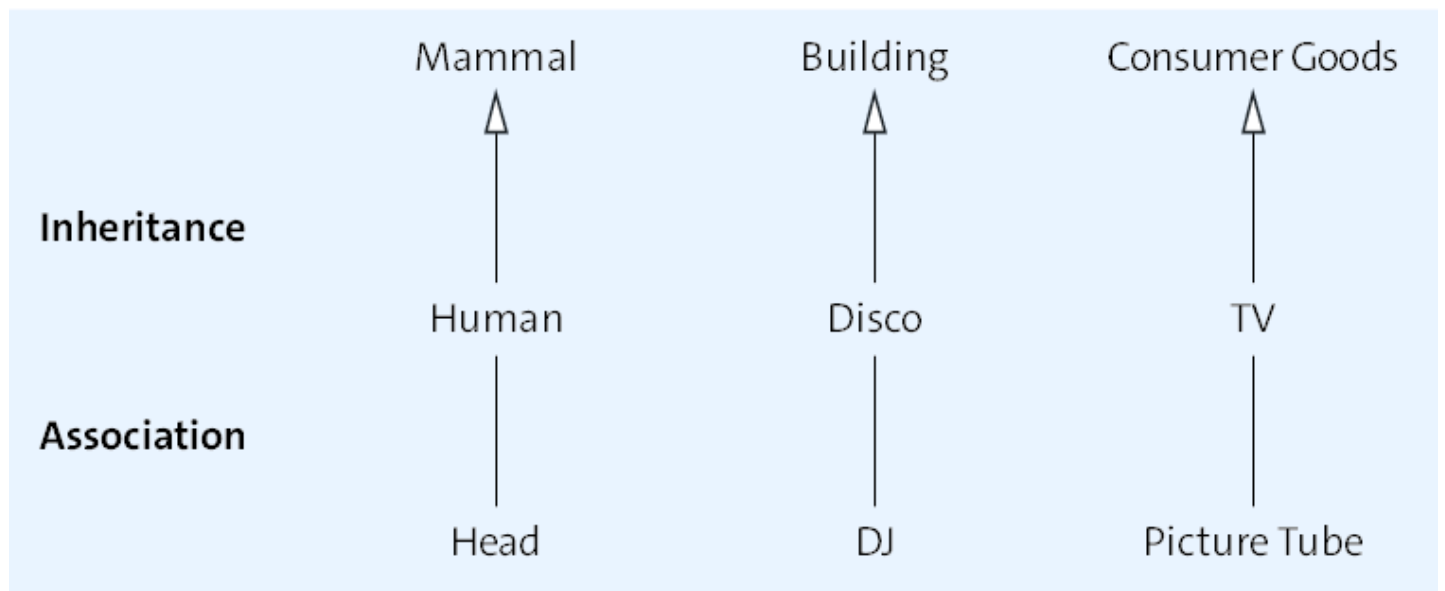
Figure 7.7 Examples of Inheritance and Association
