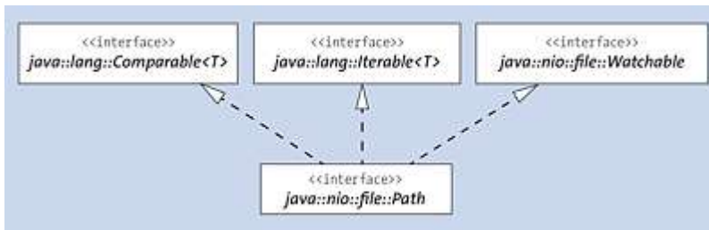
Figure 19.3 The Inheritance Relationship of Path
