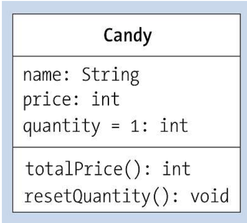
Figure 6.4 UML Class Diagram of Candy with Three Object Variables and Two Methods
