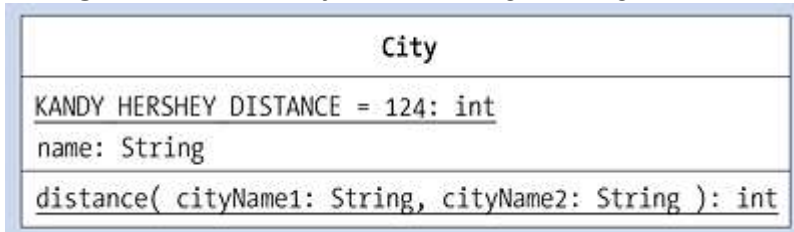
Figure 6.8 UML Diagram with Static Members Underlined
