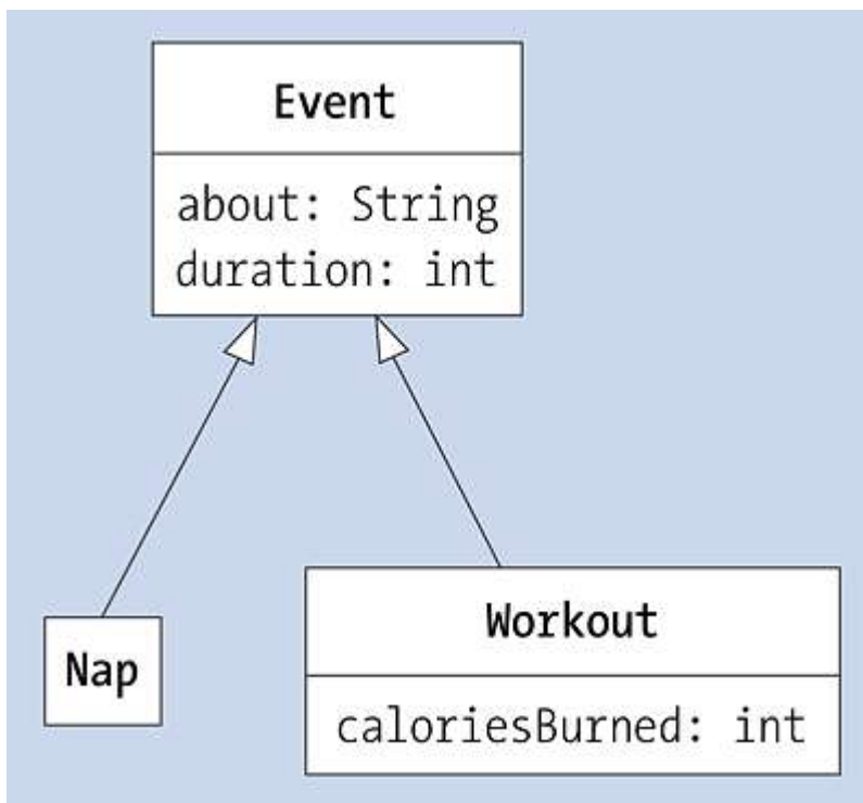
Figure 7.8 Nap and Workout Classes as Two Subclasses of the Event Class
