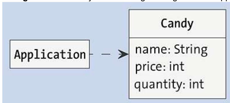
Figure 6.2 UML Class Diagram Showing the Dependencies of Application and Candy
