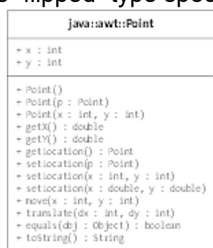
Figure 3.1 The java.awt.Point Class in a UML Representation
