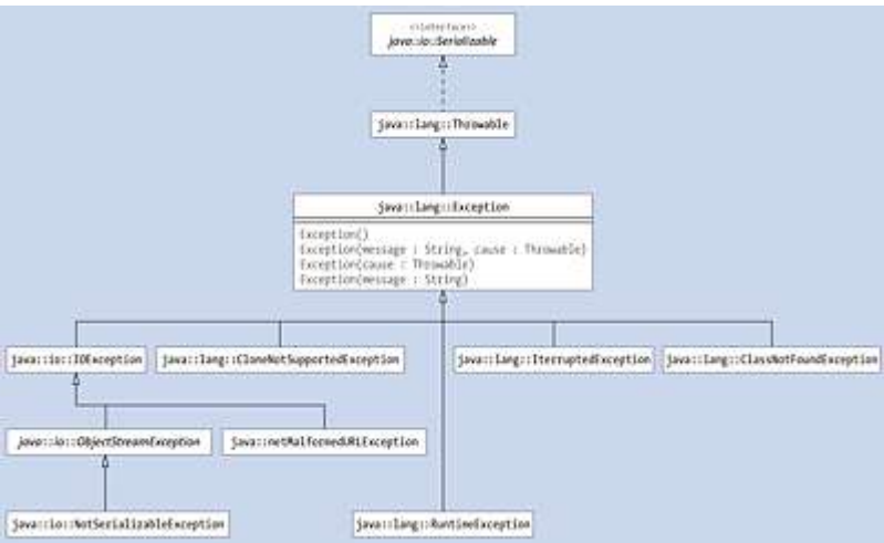
Figure 9.5 Selected Subclasses of the Exception Class
