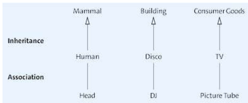
Figure 7.7 Examples of Inheritance and Association
