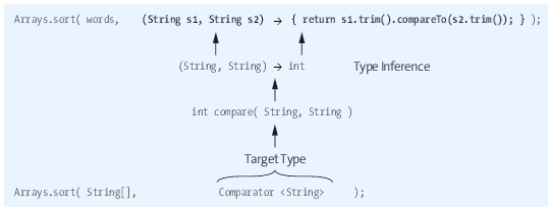
Figure 13.1 Type Inference of the Compiler
