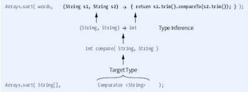
Figure 13.1 Type Inference of the Compiler
