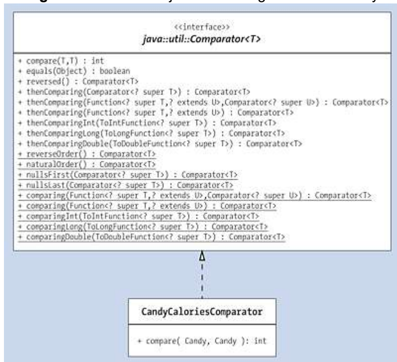
Figure 11.4 The Custom Comparator Must Merely Override compare(...) from the Interface
