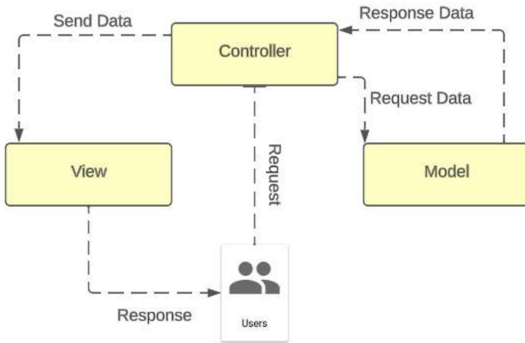
Figure 2.15: Example of MVC design pattern
