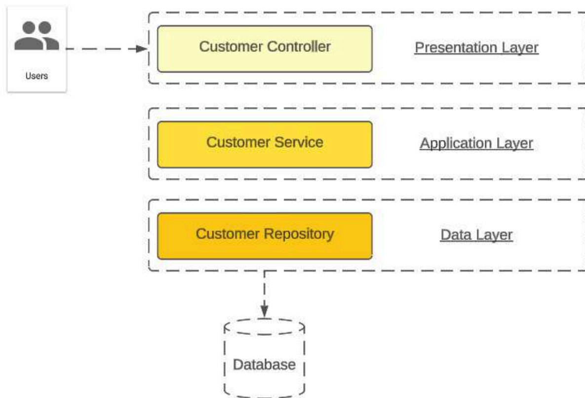
Figure 2.14: Example of the Layered design pattern
