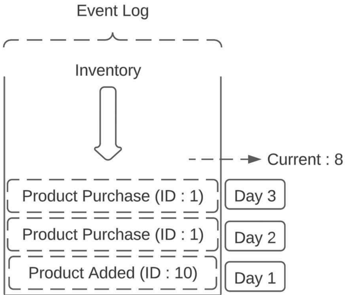
Figure 2.6: Event log – detailed example
