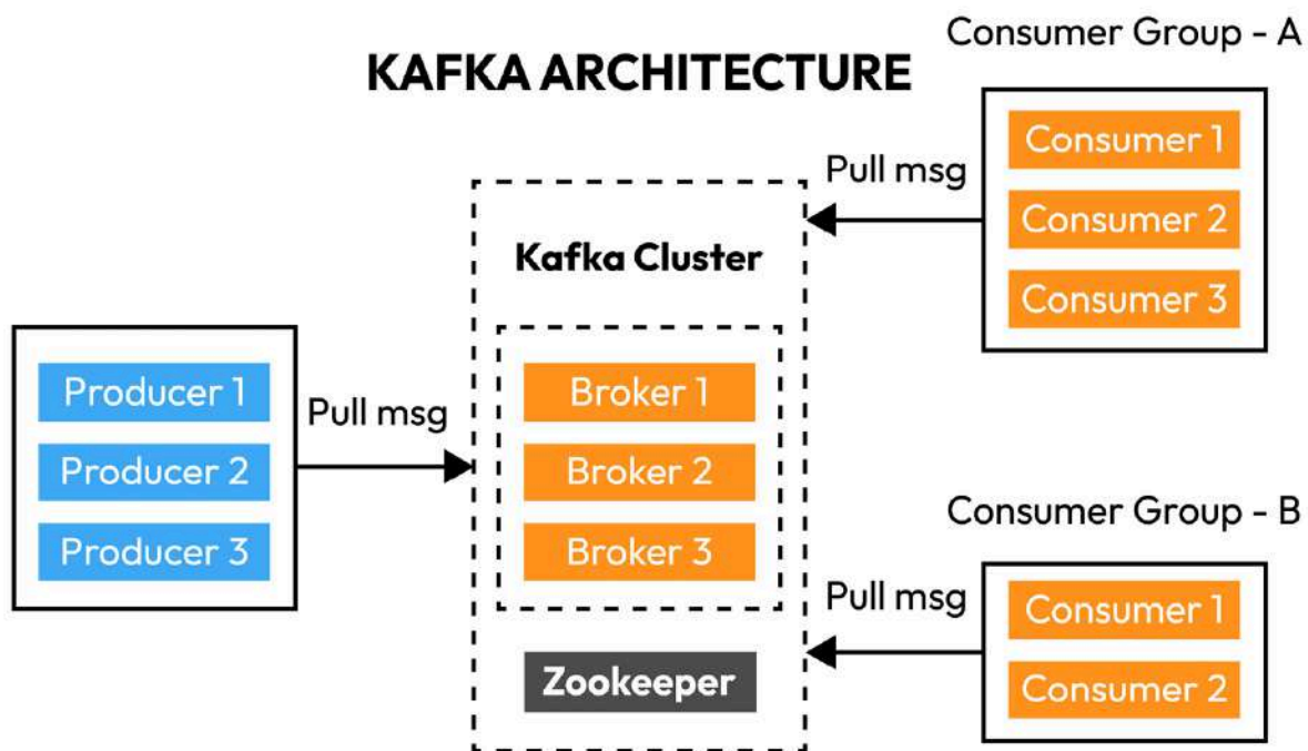
Figure 8.1: Kafka cluster architecture
