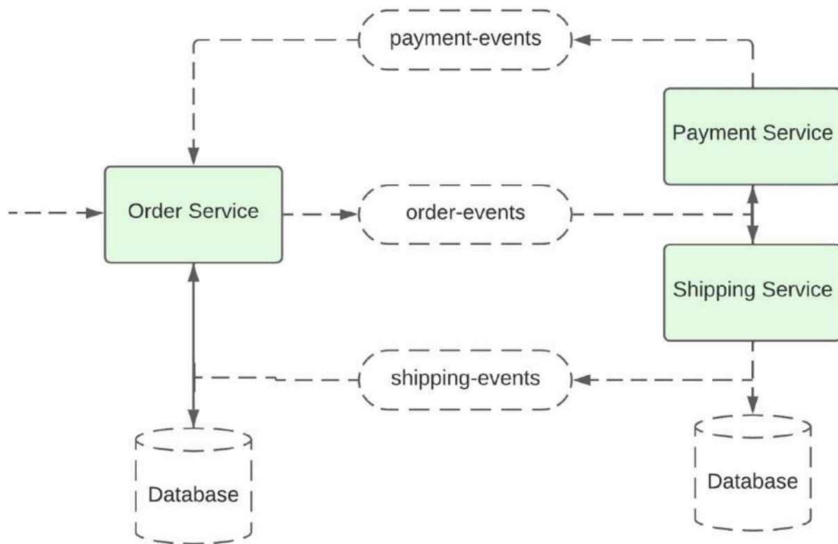
Figure 2.16: Example of the Saga design pattern
