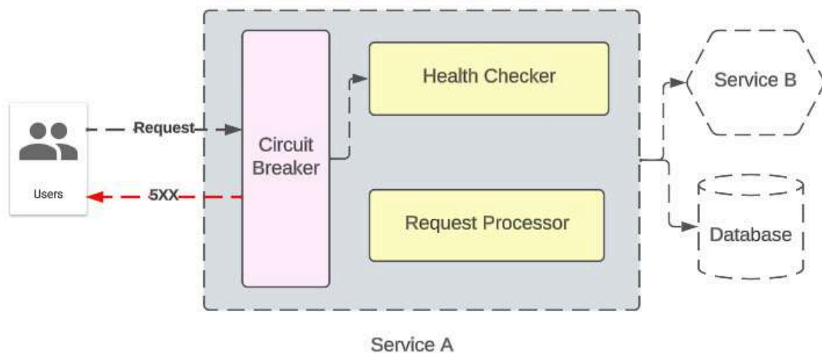
Figure 2.13: Example of the Circuit Breaker pattern
