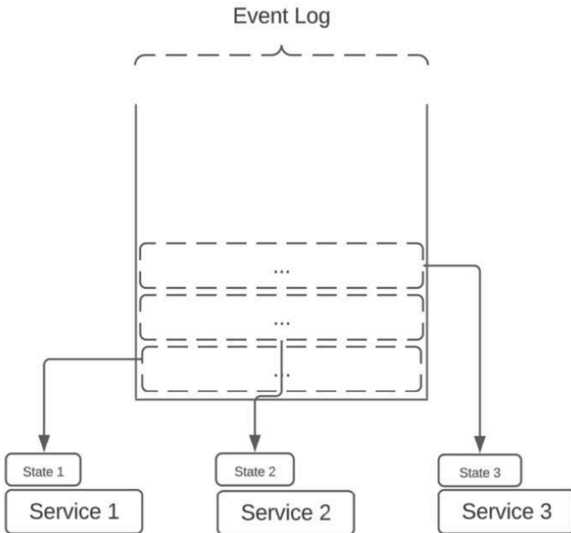
Figure 2.7: Parallel processing feature
