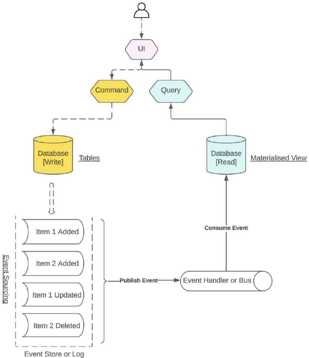
Figure 2.10: Event Sourcing pattern with CQRS
