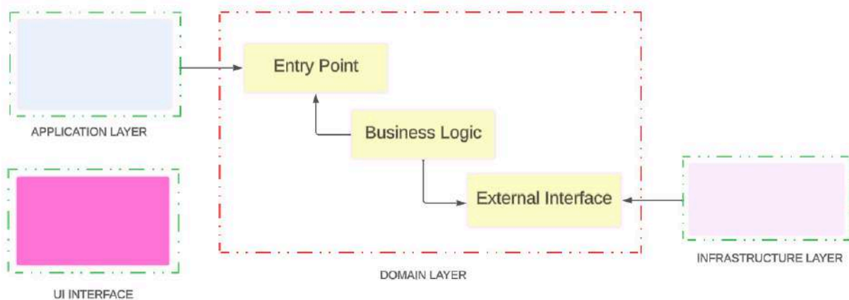
Figure 2.2: Relationship between the DDD layers
