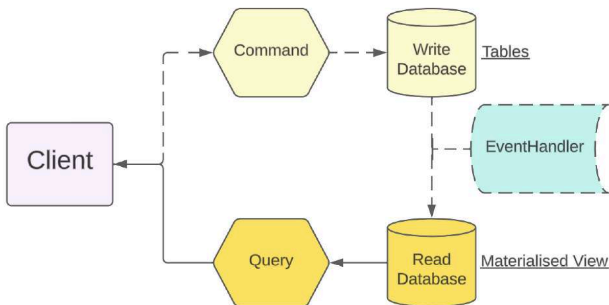
Figure 2.8: Representation of CQRS pattern
