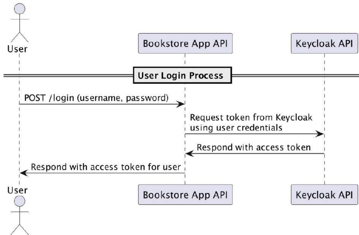
Figure 5.5: User login process with Keycloak server
