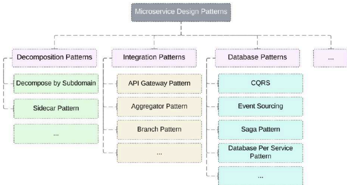
Figure 2.1: Common microservice design patterns
