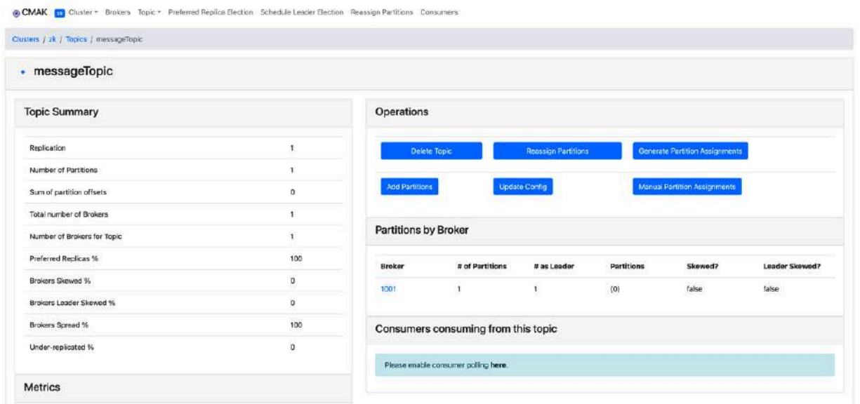
Figure 8.5: Kafka Manager screen for our topic
