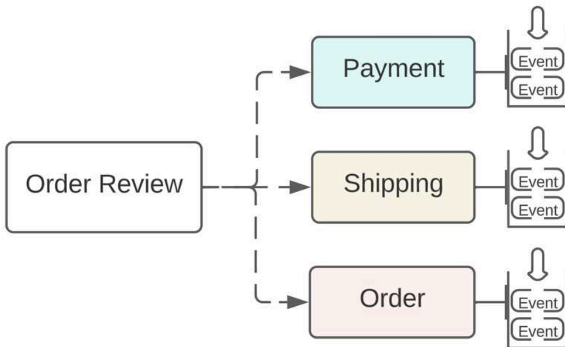
Figure 2.9: Zoom in on the service side
