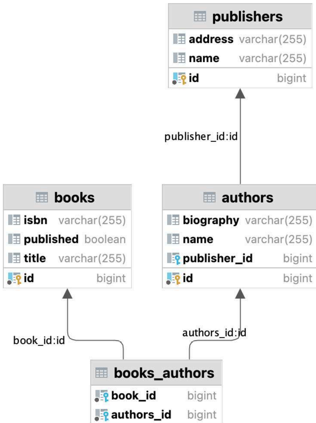
Figure 4.1 – Database diagram of the tables
