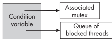
Figure 16-3: A schematic representation of a condition variable
