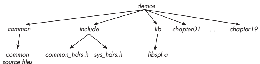
Figure 3-1: The structure of the demo program directories with common code
