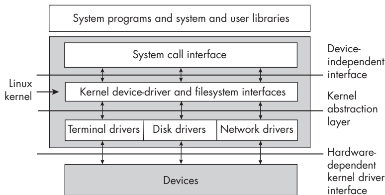
Figure 6-4: The layering of interfaces from the hardware up to user space applications
