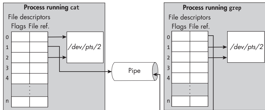
Figure 13-7: The file descriptor tables of the cat and grep processes with the set-up pipe
