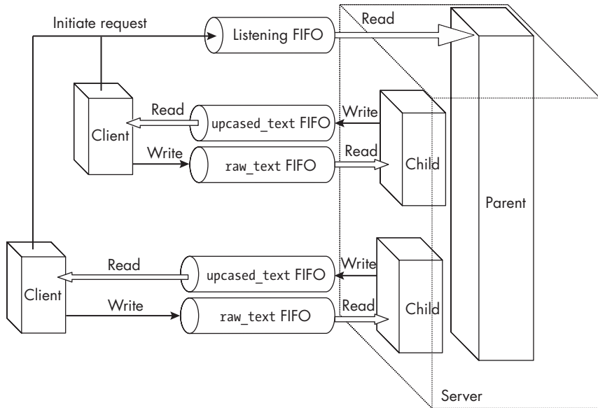
Figure 14-2: Concurrent server and client communication
