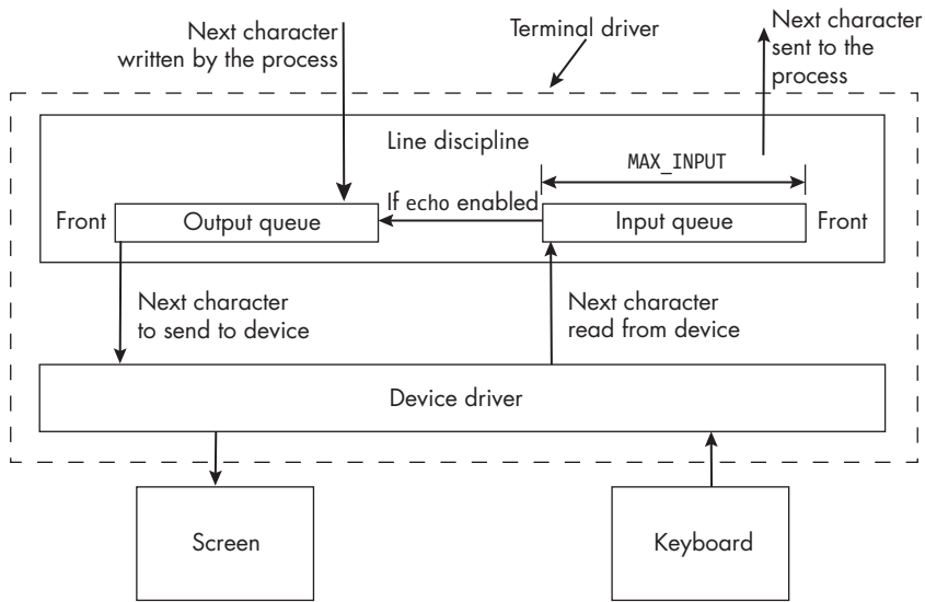
Figure 18-2: The Unix implementation of a terminal showing some of the internal queues of the terminal driver
