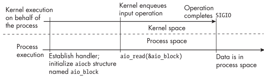
Figure 17-4: A timeline depicting the relative points in time at which events take place for an AIO input request
