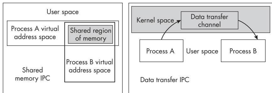
Figure 12-1: Shared memory-based IPC in comparison to data transfer-based IPC
