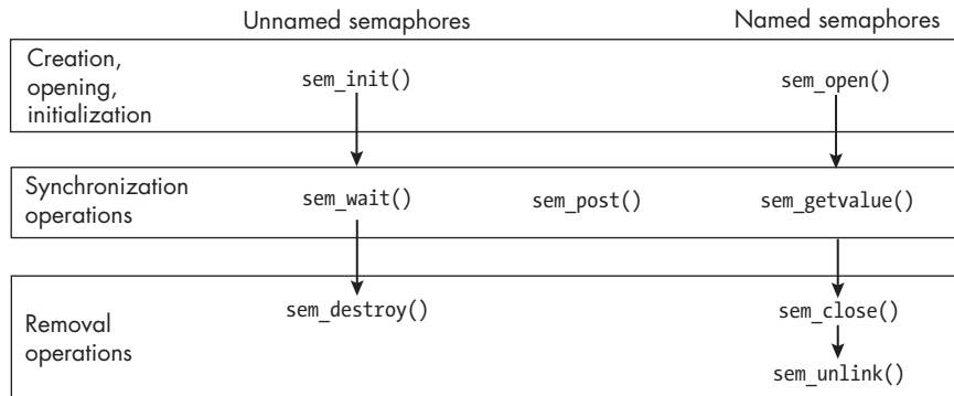
Figure 12-5: A comparison of the sequence of steps for using named and unnamed POSIX semaphores
