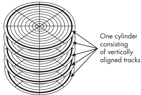
Figure 6-2: A schematic representation of a cylinder for a five-platter disk
