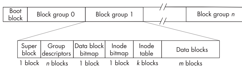
Figure 6-6: Layout of an Ext2 partition with n block groups and an exploded view of one block group
