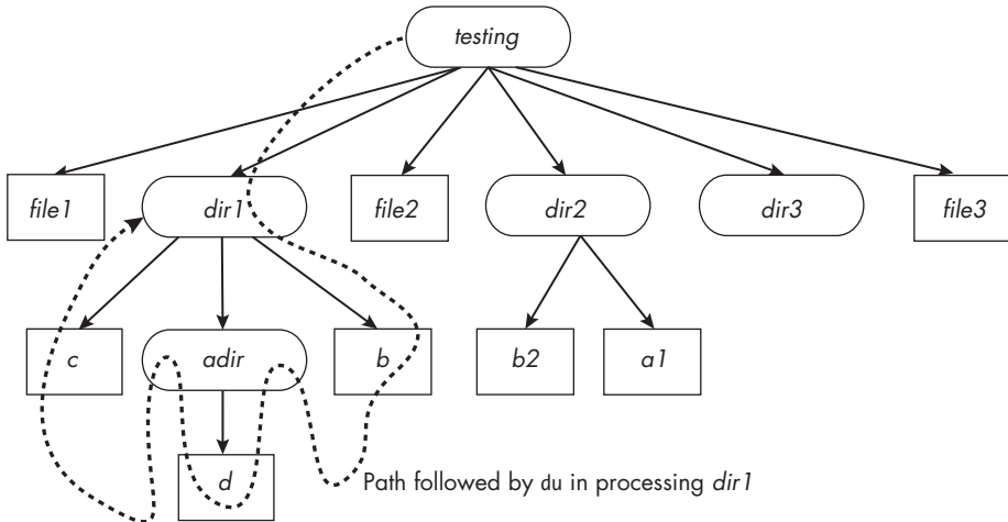
Figure 7-7: A portion of the path taken by du -a on the testing directory
