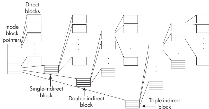
Figure 6-7: The structure of a inode, showing pointers to direct and indirect blocks
