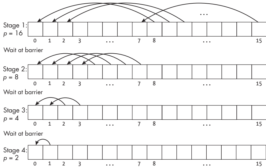
Figure 16-5: The four stages of parallel reduction of an array with a size of 16 by 16 threads
