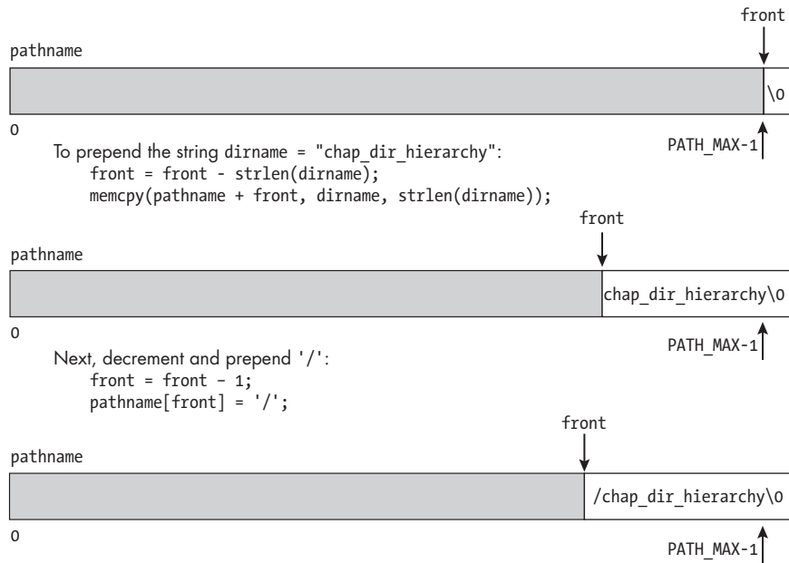
Figure 7-9: The steps to build the pathname in a right-to-left direction by prepending each new parent directory
