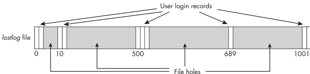
Figure 5-5: The structure of the lastlog file
