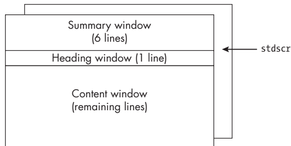
Figure 19-5: Tiled windows of spl_top.c program
