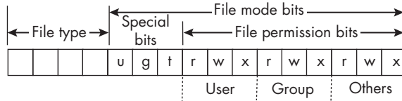
Figure 6-9: The file mode bits in the st_mode member
