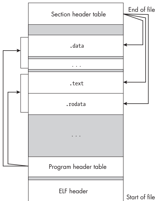
Figure 10-2: The overlapping views of the ELF file, showing that multiple sections may be part of a single segment
