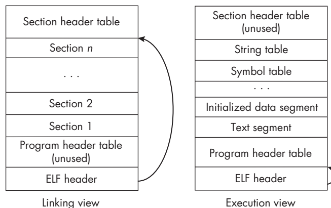
Figure 10-1: The linking and execution views of an ELF file with low addresses at the bottom
