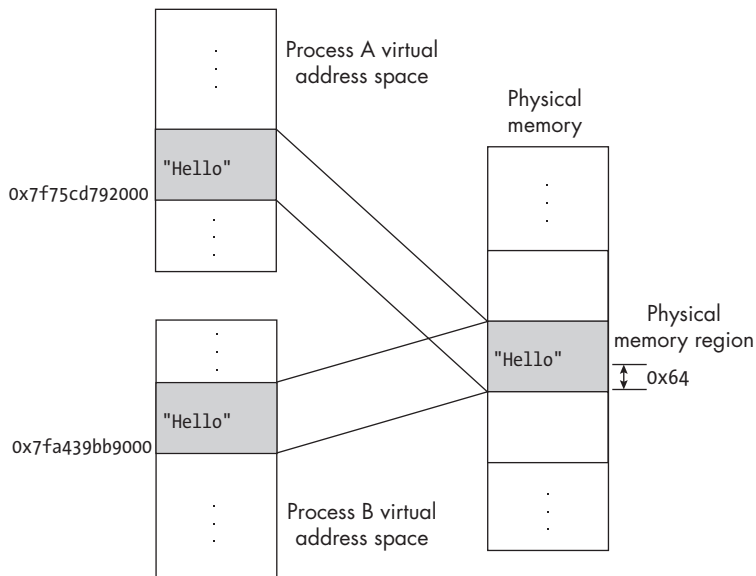
Figure 12-3: Two processes sharing a mapped memory region, showing that the starting address of the region is different in each process
