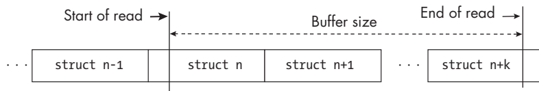
Figure 5-1: The positions at the start and end of a read operation with respect to structures in a file
