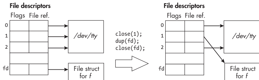
Figure 13-6: The redirection of standard output to a file f referred to by descriptor fd , using dup()
