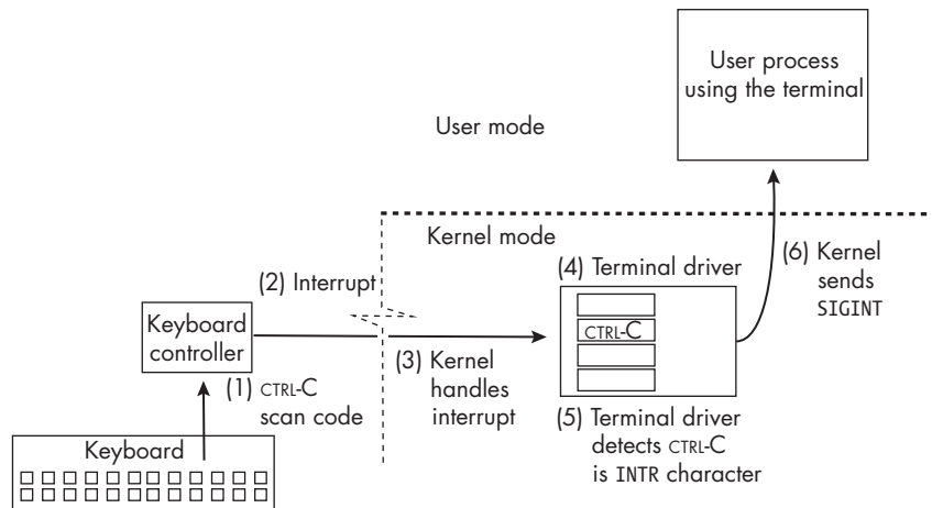
Figure 8-1: The steps taken to transform CTRL-C entered on a terminal's keyboard to a SIGINT delivered to processes using that terminal
