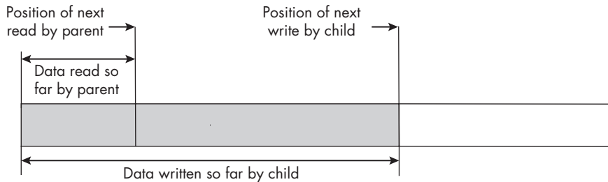
Figure 11-3: The two different positions that the shared file offset must have for parent and child processes
