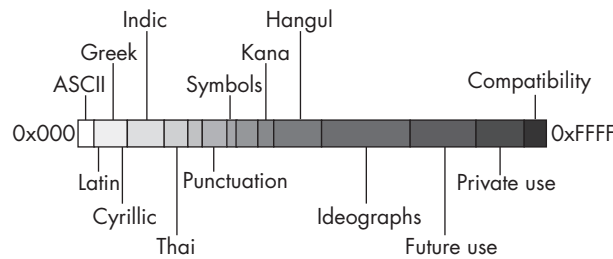
Figure B-1: Unicode layout
