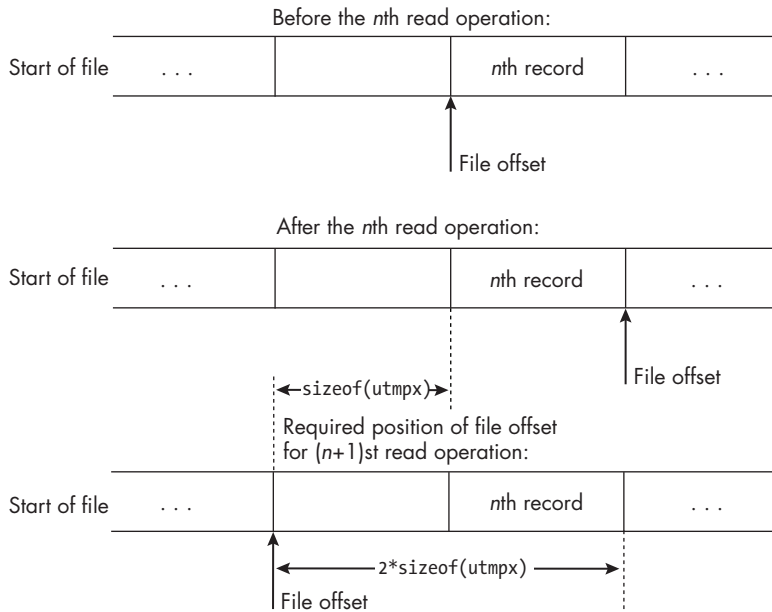
Figure 5-7: Where the file offset has to be repositioned after a read when reading backward in the file
