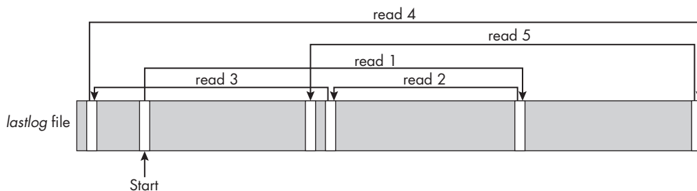
Figure 5-6: The order of reads in the lastlog file using the passwd structures returned by successive calls to getpwent() on a hypothetical host
