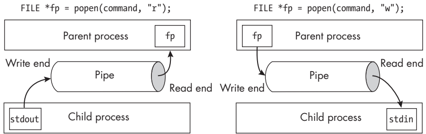
Figure 13-8: The two different methods of establishing communication with popen()
