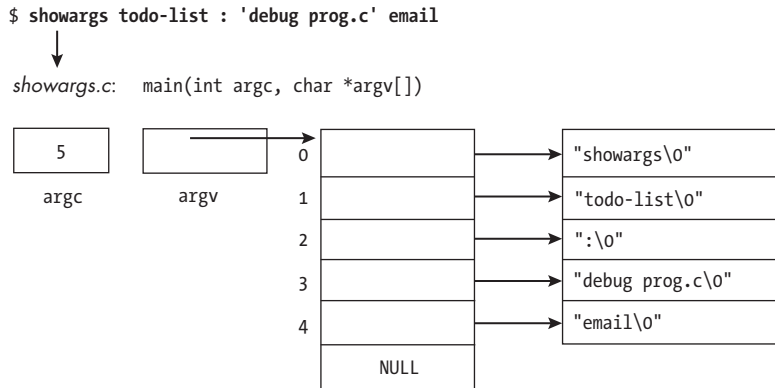
Figure 2-4: How command line arguments are passed to a program
