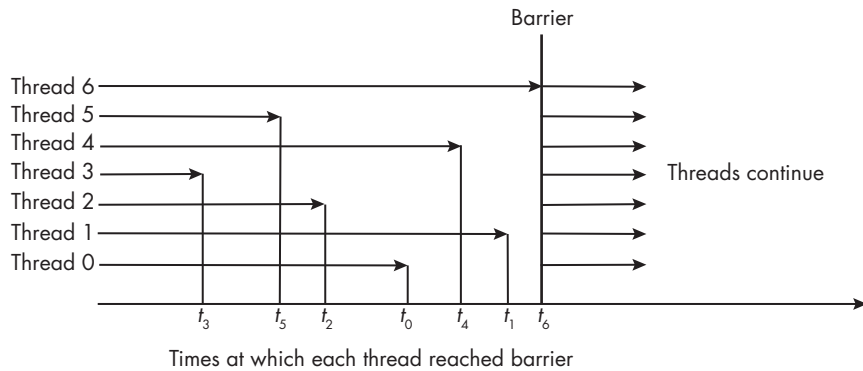
Figure 16-4: A conceptualization of a barrier synchronization point showing what time each thread reached it and that they all resume at the same time when the last thread arrives at it
