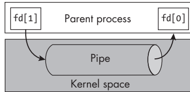
Figure 13-2: The pipe immediately after creation by the parent process
