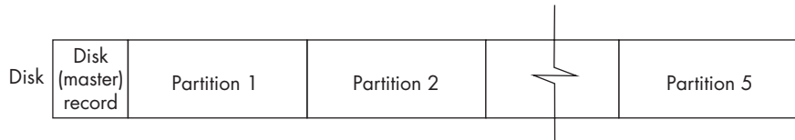
Figure 6-5: The layout of a disk with five partitions
