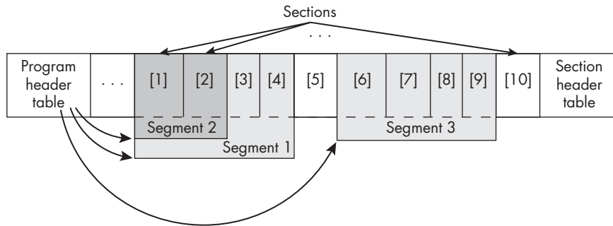
Figure 10-3: Illustration of how sections are part of segments and may be in more than one segment
