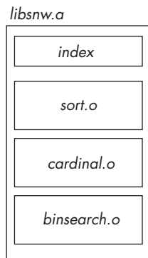
Figure 2-1: A small object library with three modules and an index that serves as a table of contents
