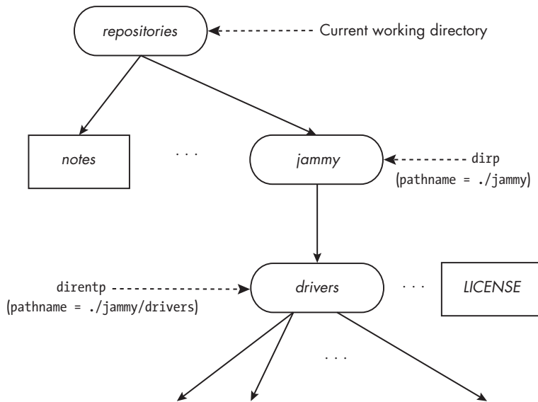
Figure 7-6: A directory being processed by opendir() and readdir()
