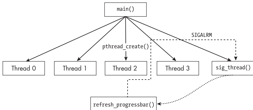
Figure 16-2: A schematic representation of threaded_progbar.c showing four compute threads and one signal handling thread
