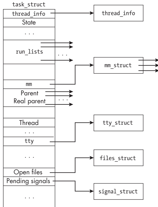
Figure 10-5: Fragments of the Linux process descriptor of type task_struct
