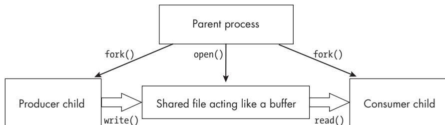
Figure 11-6: The structure of the producer-consumer program in which the main program forks two children that act as producer and consumer
