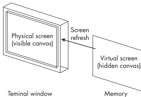
Figure 19-2: Screen refreshing in which the contents of a hidden canvas are applied to the visible canvas on the screen
