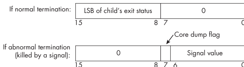
Figure 11-5: A traditional arrangement of bits of the status available from the call wait(&status)
