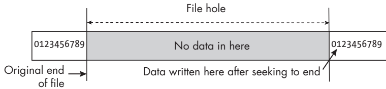
Figure 5-3: A file hole created by seeking past the end of a file and writing data there
