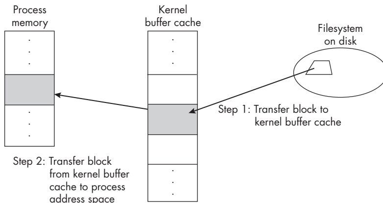
Figure 4-4: The transfer of data during a read() call from the filesystem on disk to the kernel's buffer cache and then to the process's address space
