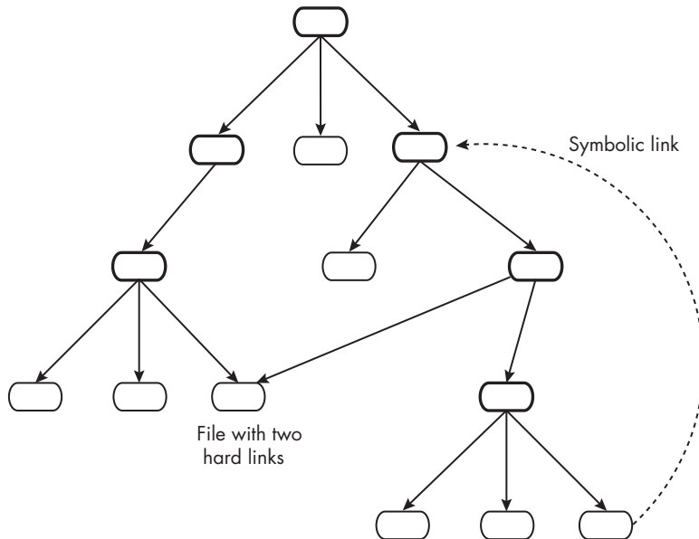
Figure 7-2: A portion of the directory hierarchy with a symbolic link creating a cycle
