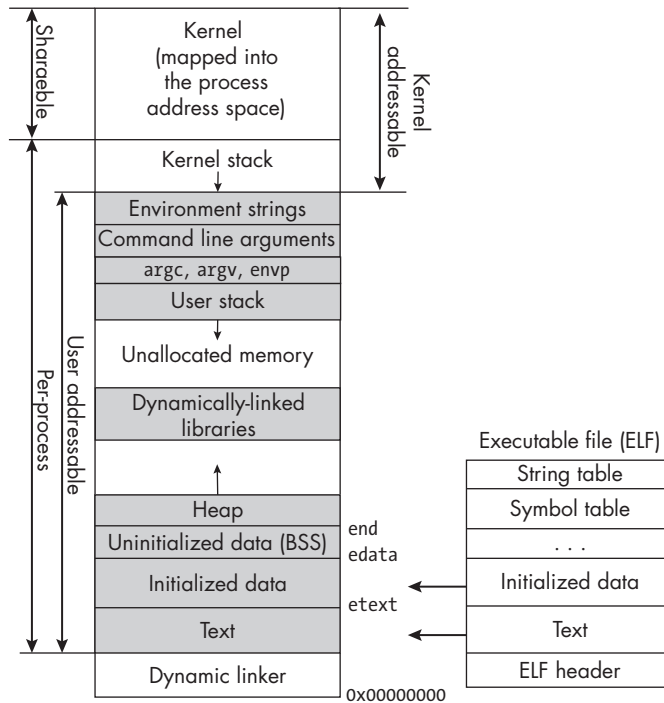
Figure 10-4: The layout of a process in its virtual address space for a typical Linux system, showing the correspondence between the ELF file's segments and the process's segments
