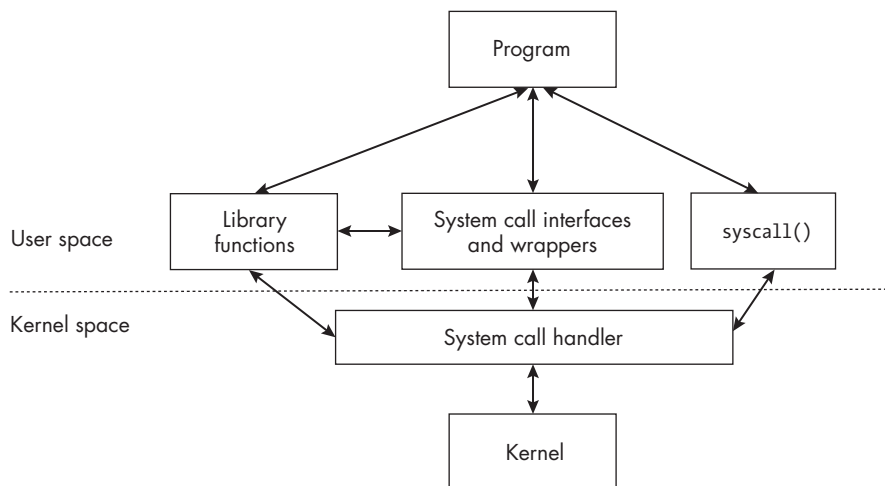
Figure 2-3: The different control paths for obtaining services, showing the relationship between library function calls and system calls
