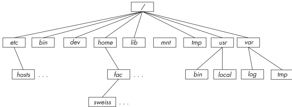
Figure 1-7: A portion of the top of a typical UNIX directory hierarchy
