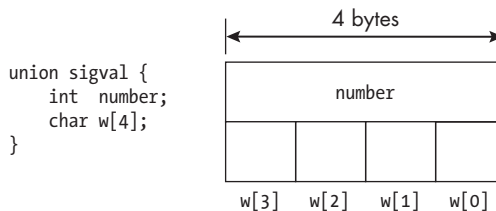
Figure 8-4: A C union with a 4-byte integer and a four-character string
