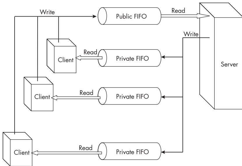
Figure 14-1: The FIFOs used in the iterative server
