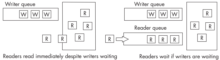
Figure 16-6: Two scenarios when writers are waiting for the read-write-lock while readers are “in the room” and readers arrive
