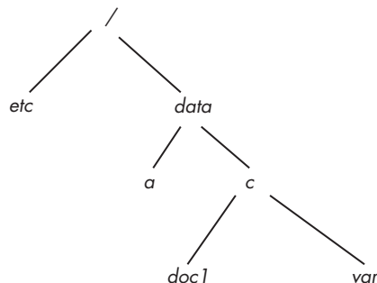
Figure 7-3: The initial file hierarchy without any mounts
