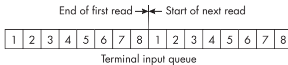
Figure 8-5: A read of eight characters from the terminal, showing where the next read operation will start
