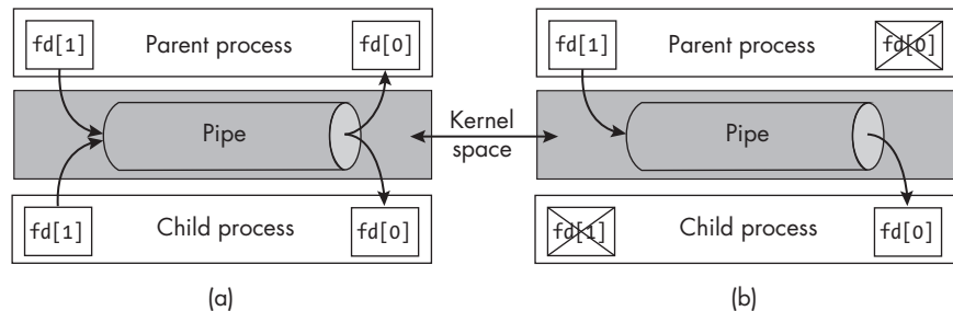
Figure 13-3: The pipe after the parent forks the child. (a) The state of the pipe before parent and child close their respective read and write descriptors. (b) Its state after.
