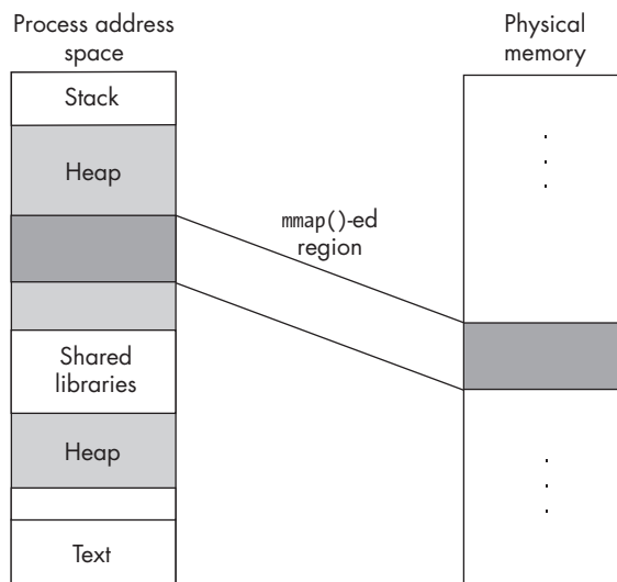
Figure 12-2: The effect of mmap() on a shared memory object
