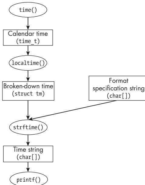
Figure 3-2: The program flow of spl_date1.c
