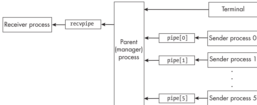
Figure 17-8: A schematic representation of select_demo.c showing the sources of input and output monitored by the parent process using select()
