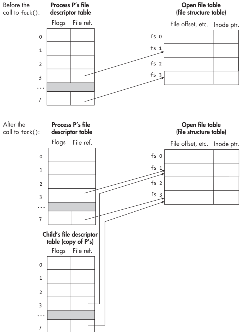
Figure 11-2: The before and after of the duplication of a process's open file descriptor table in the new child process
