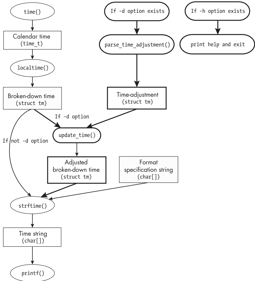
Figure 3-3: The control flow of spl_date3.c
