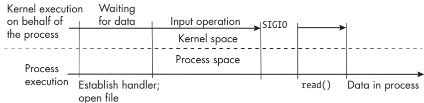
Figure 17-2: A timeline depicting the relative points in time at which events take place for signal-driven input
