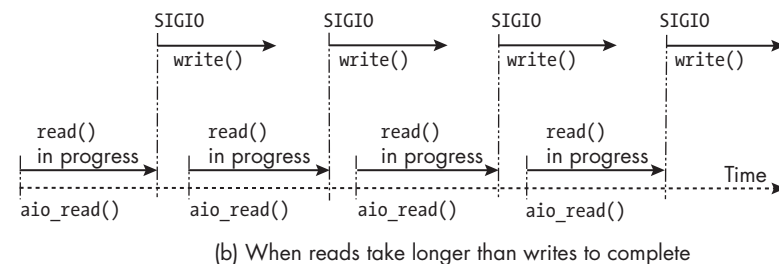
Figure 17-7: Overlapped, asynchronous reads using aio_read() and synchronous writes using write() to copy a source file to a target file
