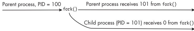
Figure 11-1: A conceptualization of the fork() system call
