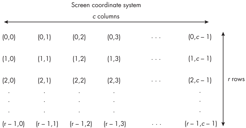
Figure 19-1: The Curses coordinate system
