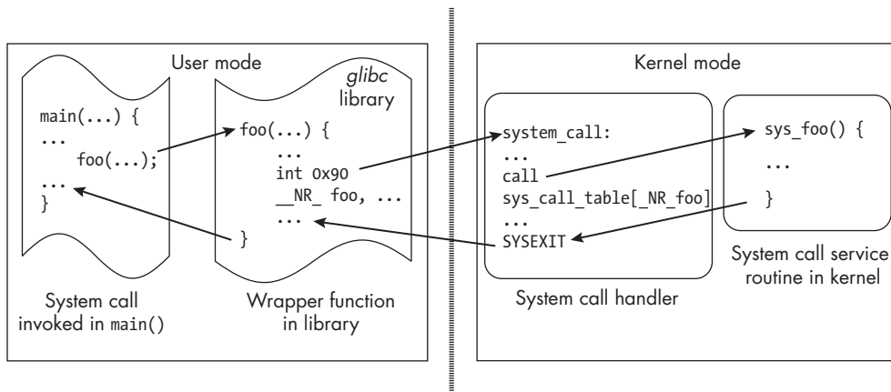
Figure 2-2: A sample detailed system call execution flow
