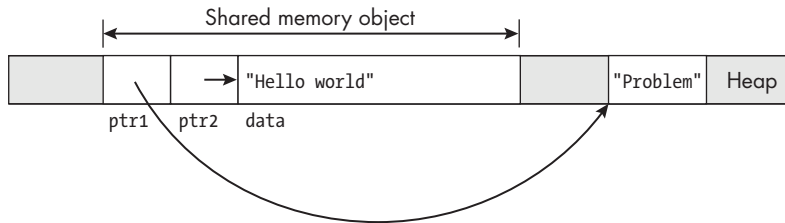
Figure 12-4: The arrangement of data in the shared memory created by shm_creator_demo2.c
