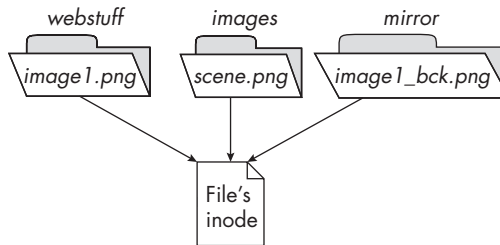
Figure 1-6: A file with three names
