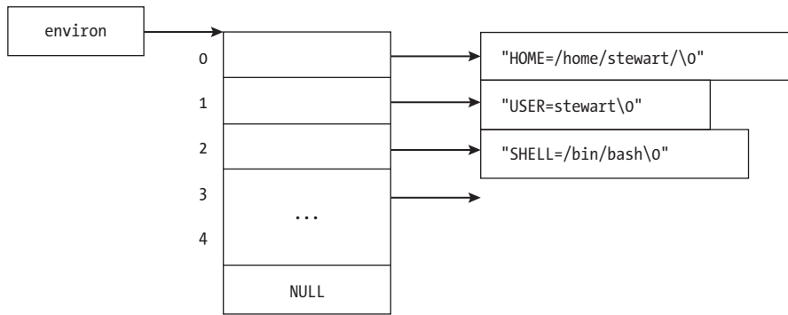
Figure 2-5: The environ pointer
