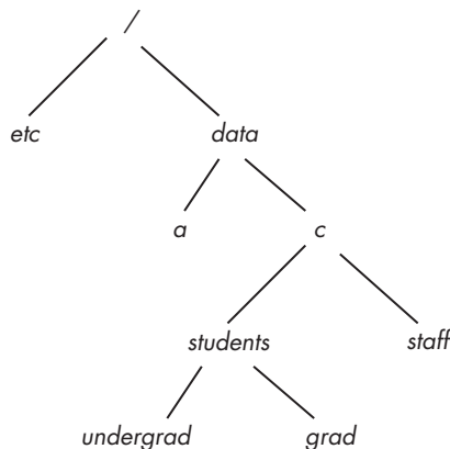
Figure 7-5: The directory hierarchy after the mount of /dev/hdb onto /data/c
