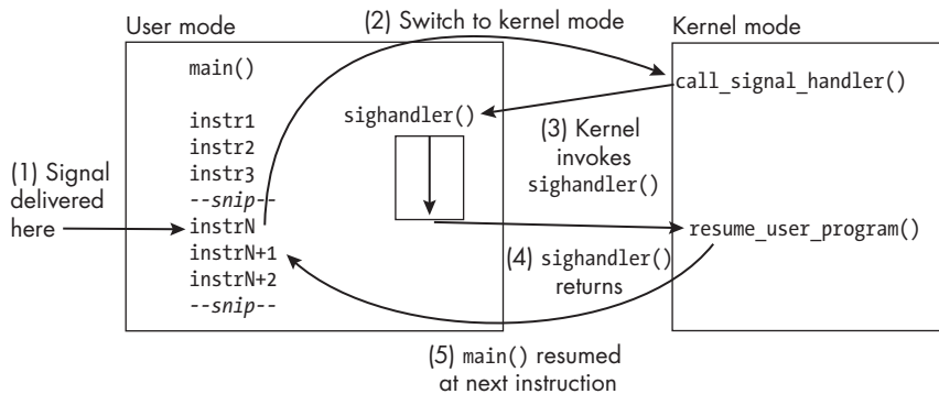
Figure 8-2: A schematic representation of the steps that occur when a process receives a signal for which it has registered a signal handler named sighandler()
