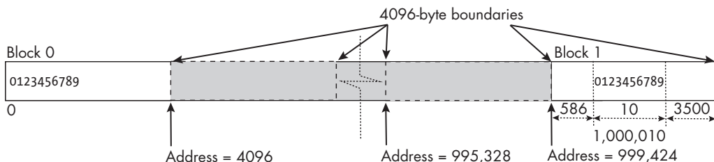
Figure 5-4: A not-to-scale diagram of the disk blocks allocated to the file with holes that is depicted in Figure 5-3
