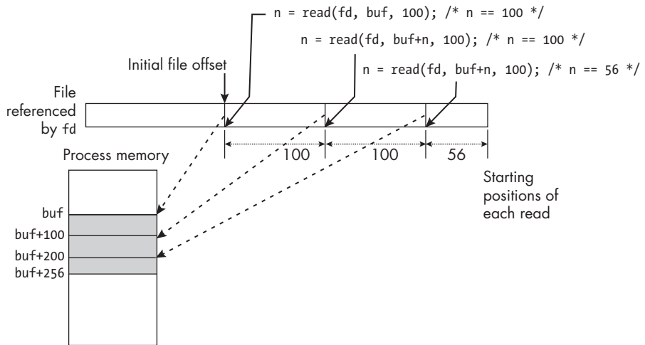
Figure 4-3: Three successive reads with the third returning fewer bytes than requested
