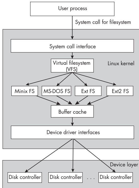
Figure 6-8: A schematic representation of the Linux VFS incorporating the Ext2 filesystem
