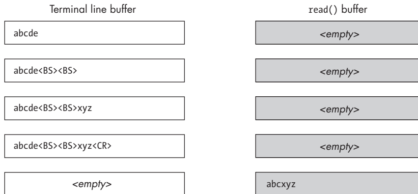
Figure 18-1: A schematic representation of the processing of an edited input line
