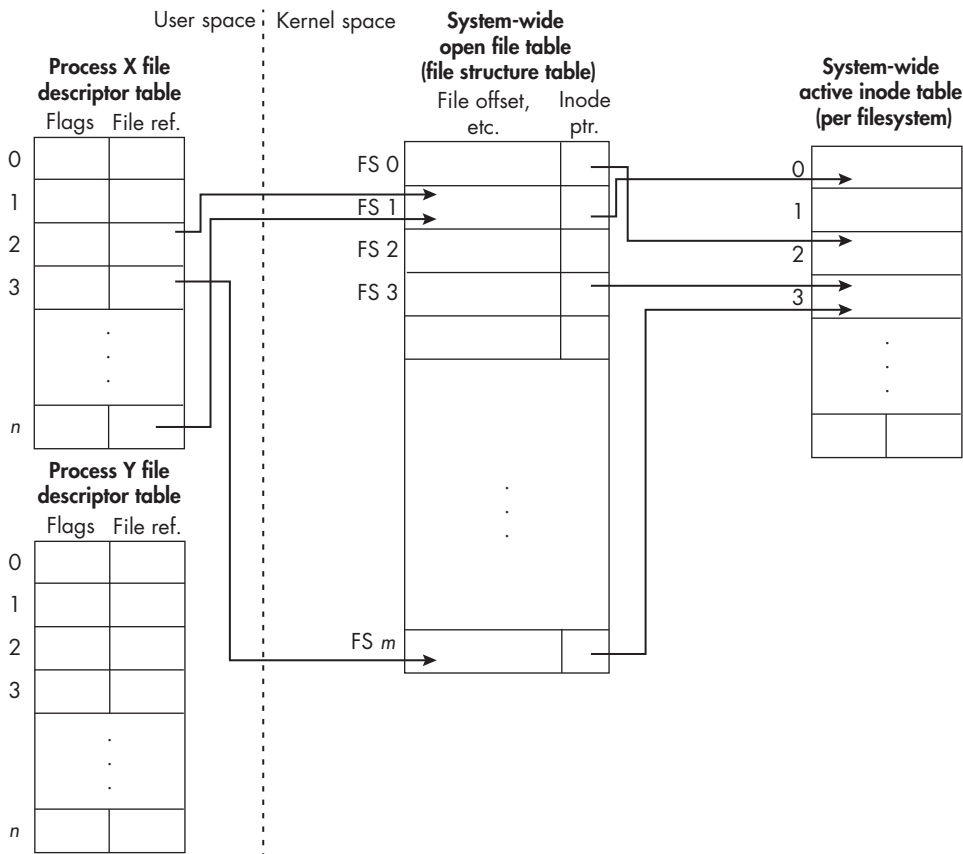
Figure 4-1: The tables used to manage files opened by processes
