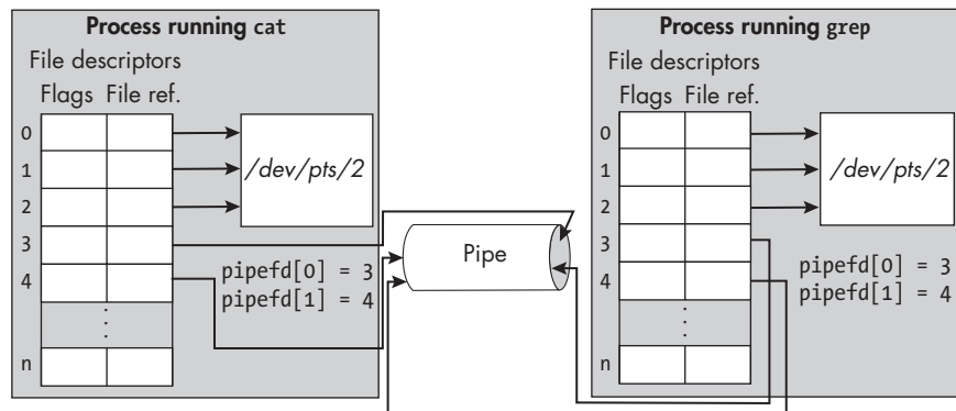
Figure 13-5: The state of the pipe and file descriptors immediately after bash created the pipe
