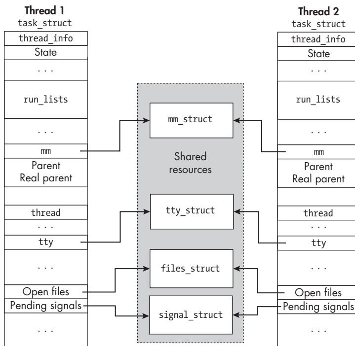
Figure 15-1: A schematic representation of how the process descriptors of two threads that are part of the same process facilitate sharing of memory, open files, and other shared data of the parent process
