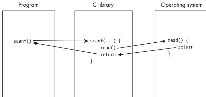
Figure 1-1: The execution flow of input operation
