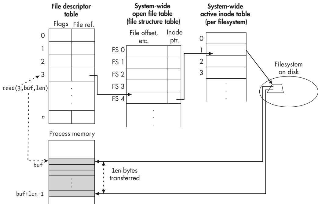
Figure 4-2: A read of len bytes by a process from the file with file descriptor 3 to memory location buf
