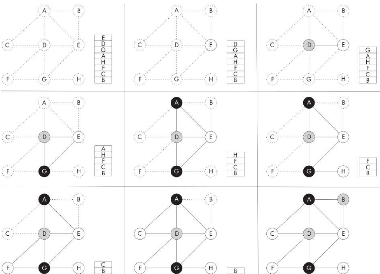
Figure 20-11: Adding nodes back to the graph and assigning colors Description
