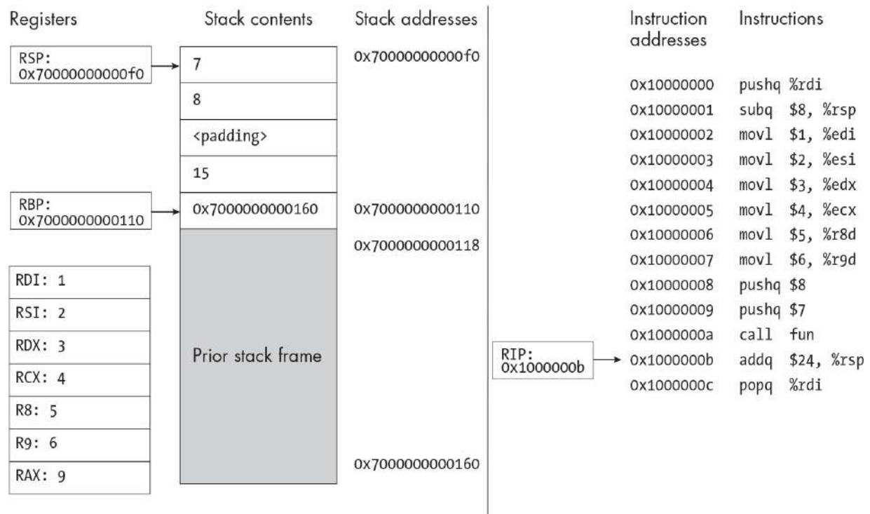
Figure 9-6: The state of the program just after returning to the caller Description
