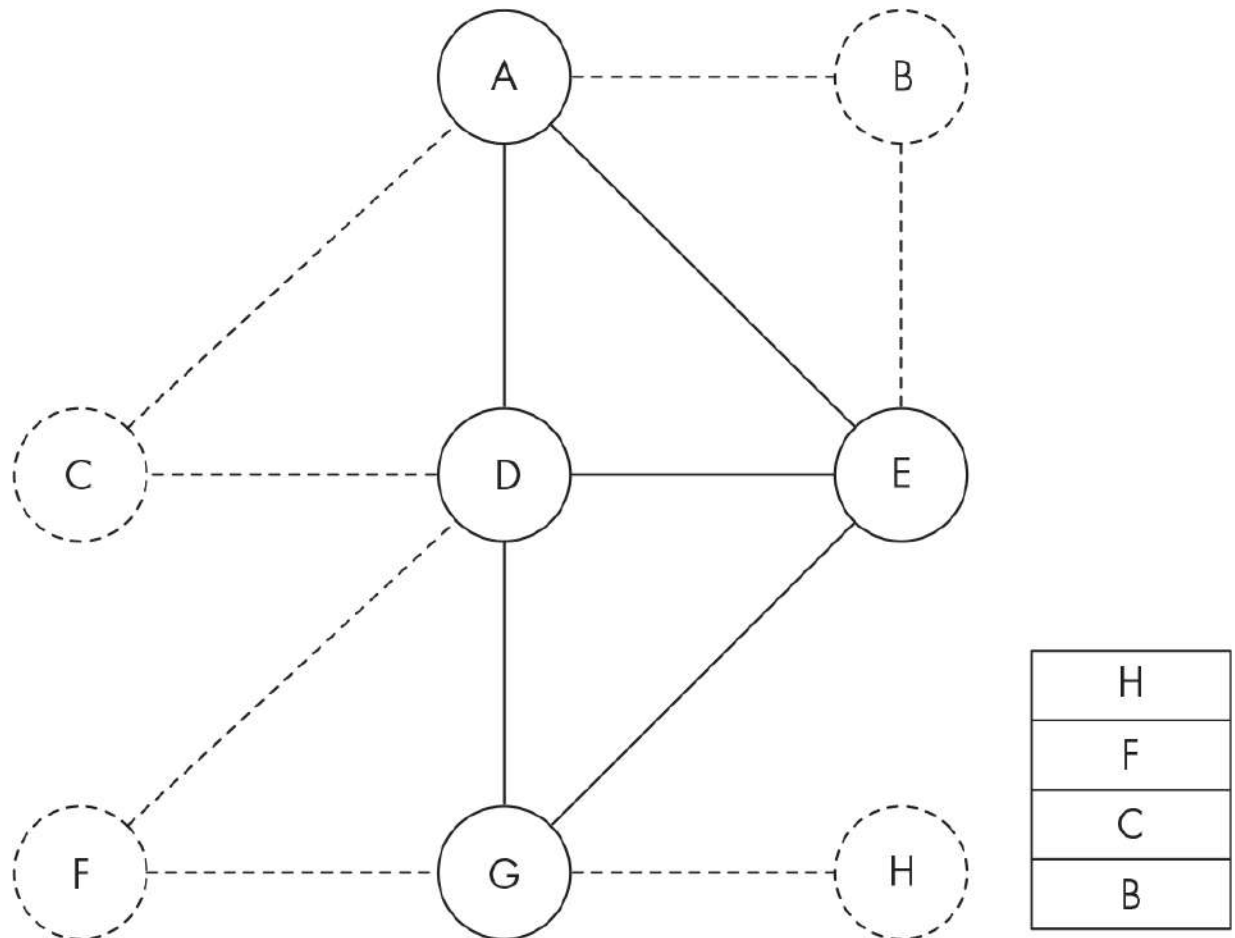
Figure 20-8: The graph from Figure 20-7 with low-degree nodes removed Description
