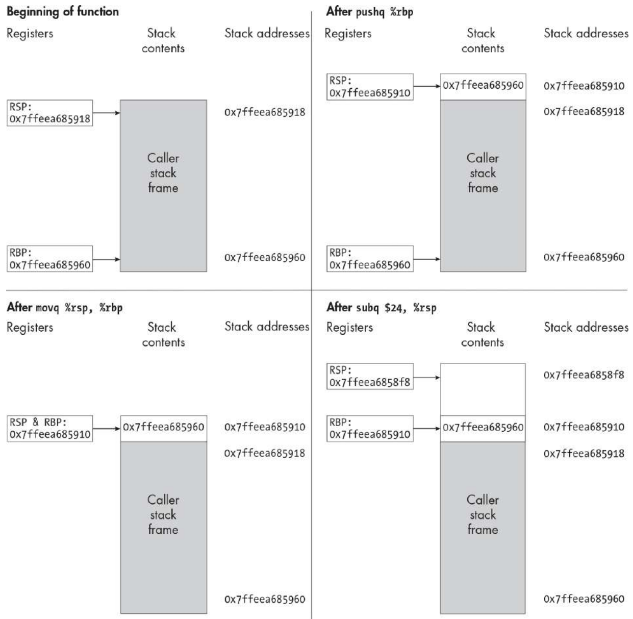
Figure 2-2: The state of the stack at each point in the function prologue Description
