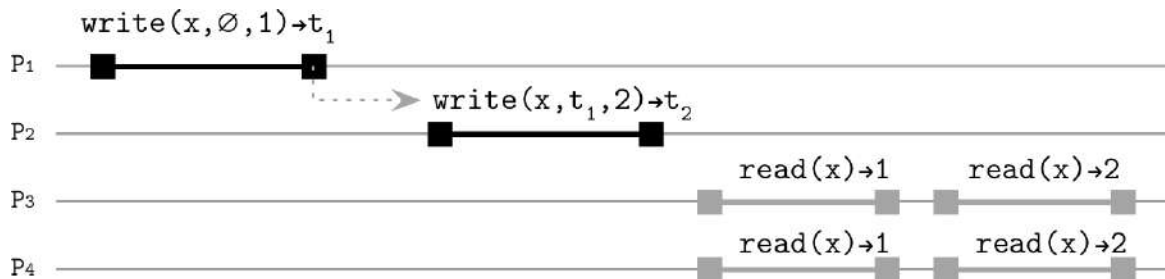
Figure 11-8. Write operations with causal relationship
