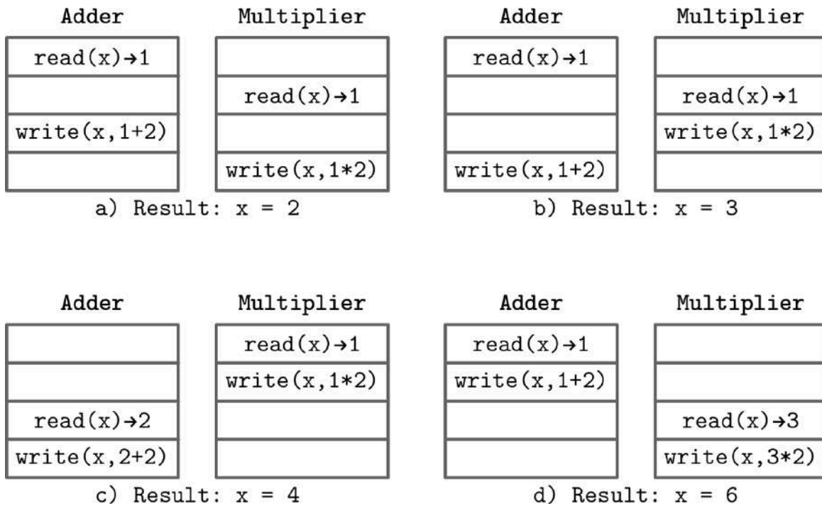
Figure 8-1. Possible interleavings of concurrent executions
