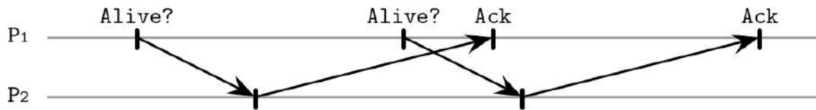
Figure 9-2. Pings for failure detection: responses are delayed, coming after the next message is sent
