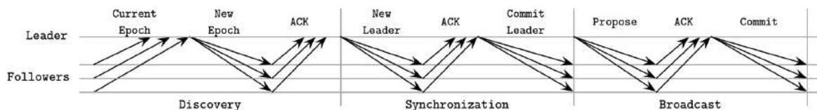
Figure 14-2. ZAB protocol summary
