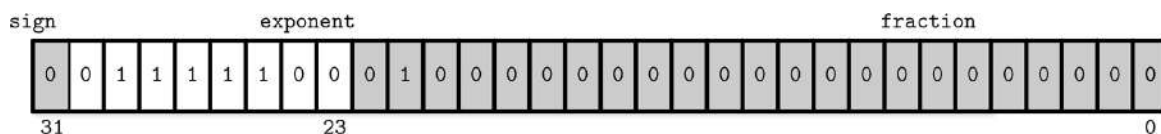
Figure 3-2. Binary representation of single-precision float number
