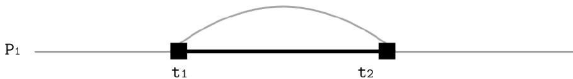
Figure 11-3. Time bounds of a linearizable operation
