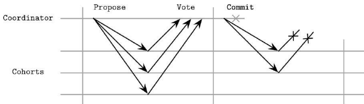
Figure 13-3. Coordinator failure after the propose phase
