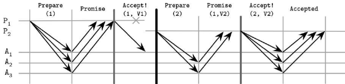
Figure 14-5. Paxos failure scenario: proposer failure, deciding on the new value
