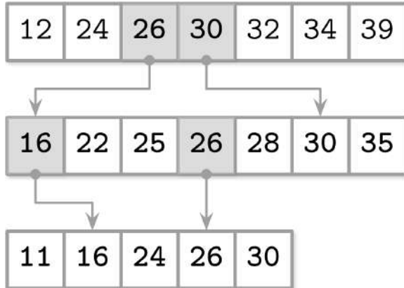
Figure 6-5. Fractional cascading
