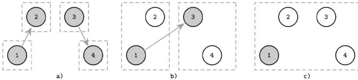
Figure 10-4. Invitation algorithm
