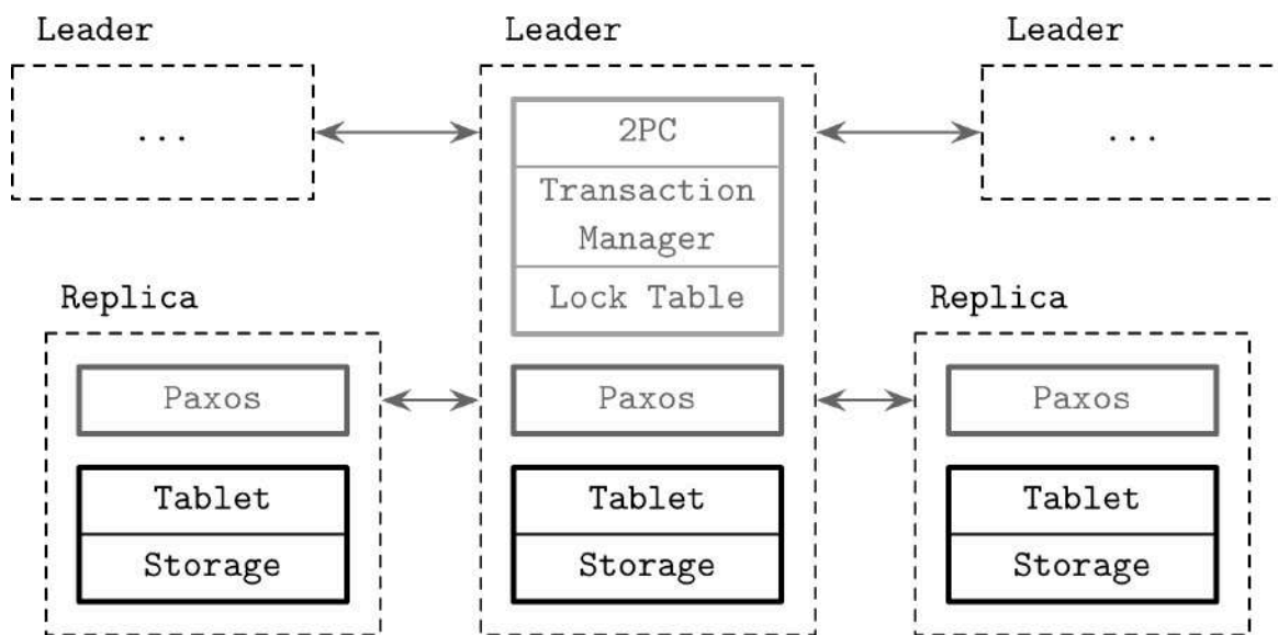
Figure 13-8. Spanner architecture
