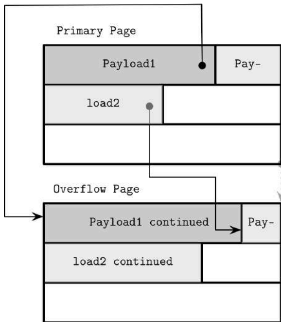
Figure 4-6. Overflow pages
