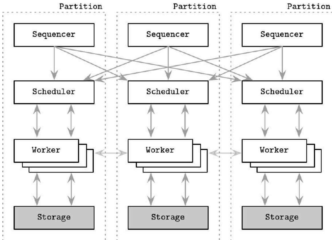
Figure 13-7. Calvin architecture
