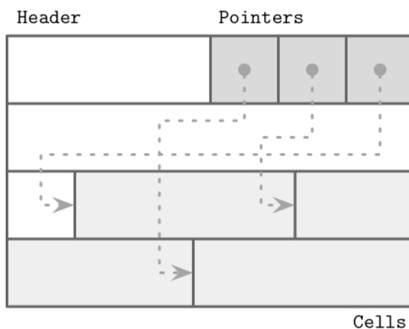
Figure 3-5. Slotted page
