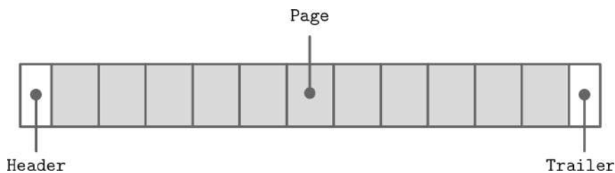
Figure 3-3. File organization
