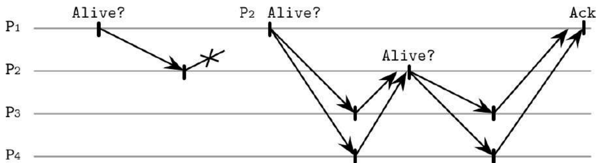
Figure 9-3. “Outsourcing” heartbeats
