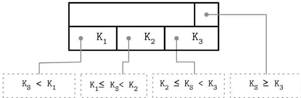
Figure 4-2. Rightmost pointer
