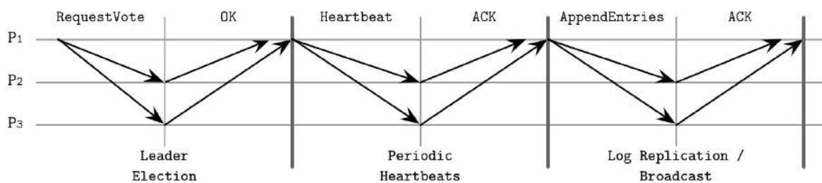
Figure 14-10. Raft consensus algorithm summary
