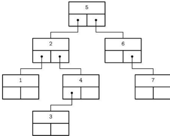
Figure 2-8. Alternative representation of a binary tree
