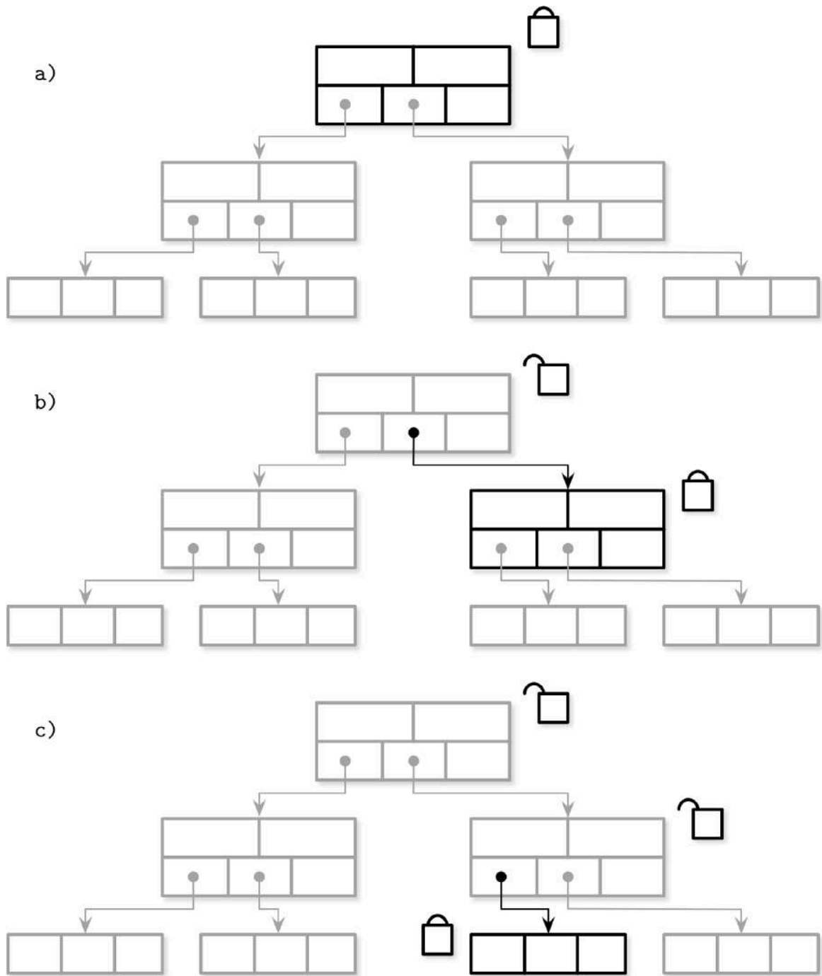
Figure 5-9. Latch crabbing during insert
