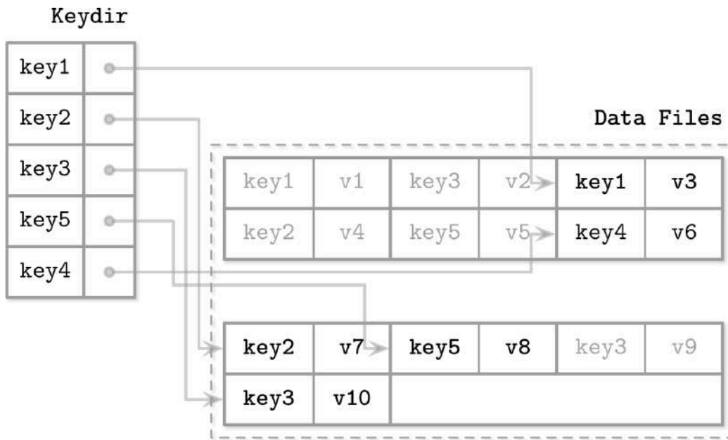
Figure 7-11. Mapping between keydir and data files in Bitcask. Solid lines represent pointers from the key to the latest value associated with it. Shadowed key/value pairs are shown in light gray.
