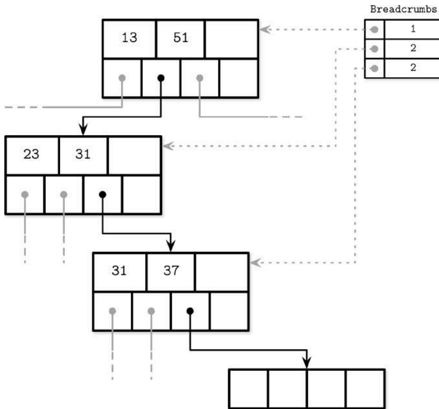
Figure 4-8. Breadcrumbs collected during lookup, containing traversed nodes and cell indices. Dotted lines represent logical links to visited nodes. Numbers in the breadcrumbs table represent indices of the followed child pointers.
