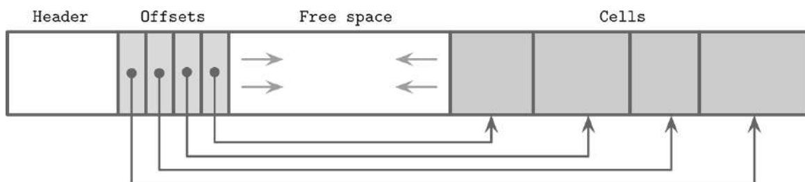
Figure 3-6. Offset and cell growth direction
