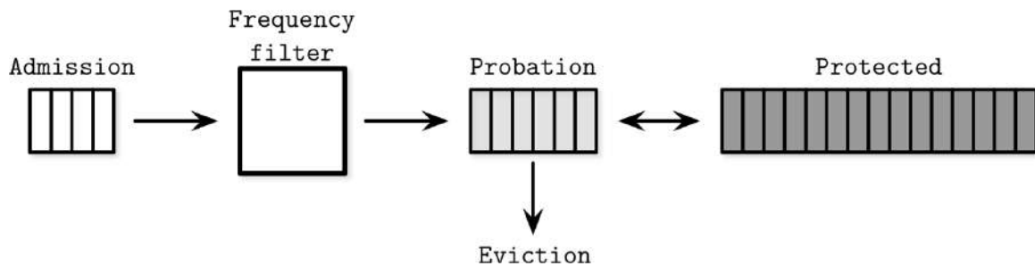
Figure 5-3. TinyLFU admission, protected, and probation queues
