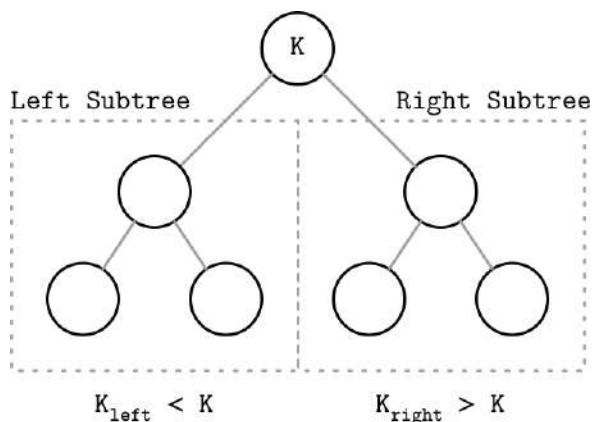
Figure 2-2. Binary tree node invariants
