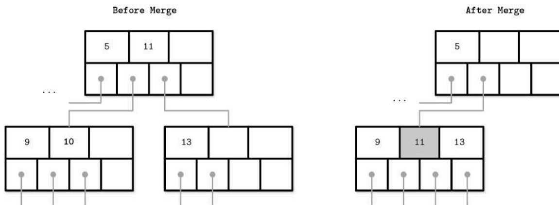
Figure 2-14. Nonleaf node merge
