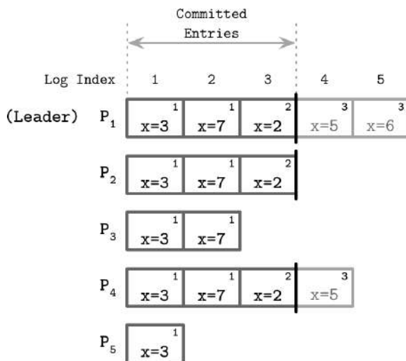
Figure 14-12. Raft state machine
