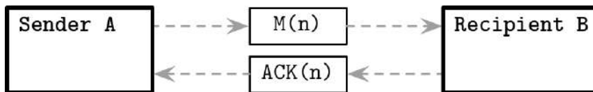
Figure 8-3. Sending a message with an acknowledgment
