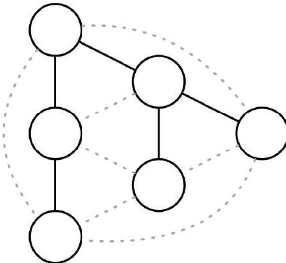
Figure 12-5. Lazy and eager push networks. Solid lines represent a broadcast tree. Dotted lines represent lazy gossip connections.
