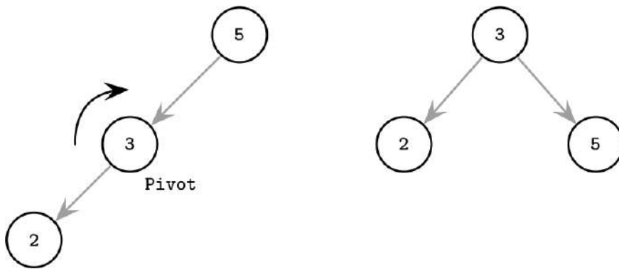
Figure 2-4. Rotation step example
