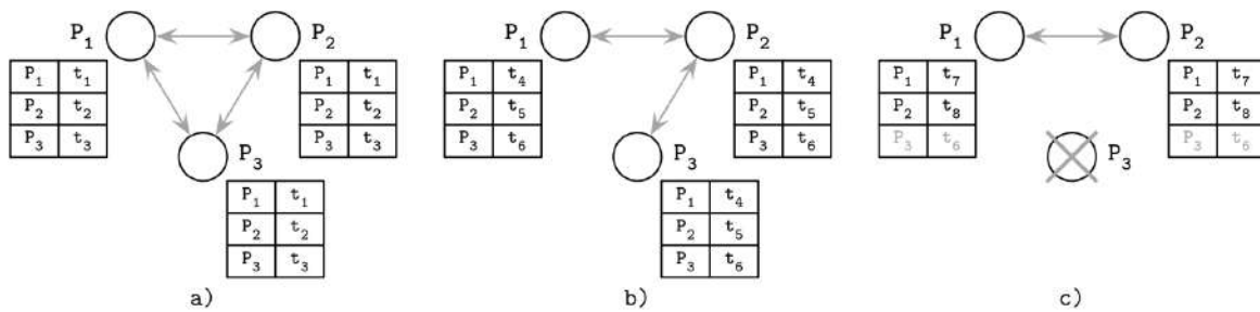
Figure 9-4. Replicated heartbeat table for failure detection
