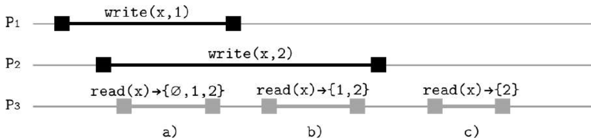
Figure 11-2. Example of linearizability
