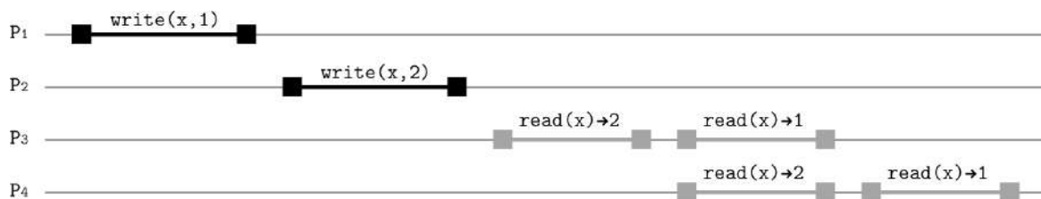
Figure 11-5. Ordering in sequential consistency
