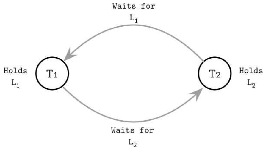
Figure 5-6. Example of a deadlock
