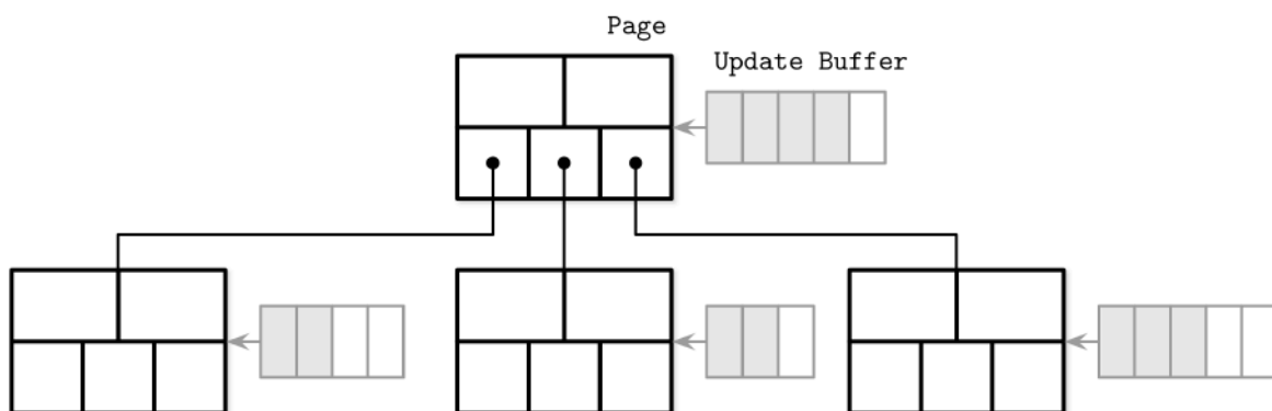
Figure 6-2. WiredTiger: high-level overview
