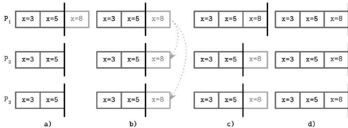
Figure 14-11. Procedure of a commit in Raft with P_1 as a leader
