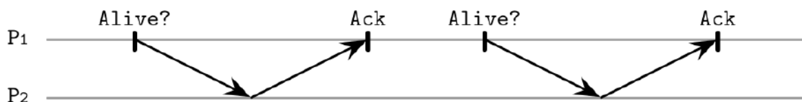
Figure 9-1. Pings for failure detection: normal functioning, no message delays
