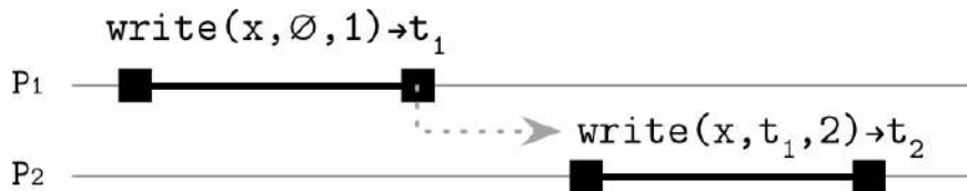
Figure 11-7. Causally related write operations
