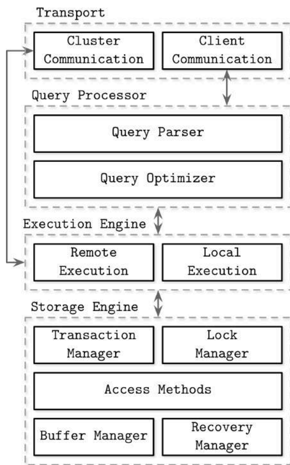
Figure 1-1. Architecture of a database management system
