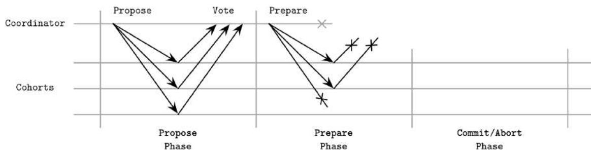
Figure 13-6. Coordinator failure during the second phase
