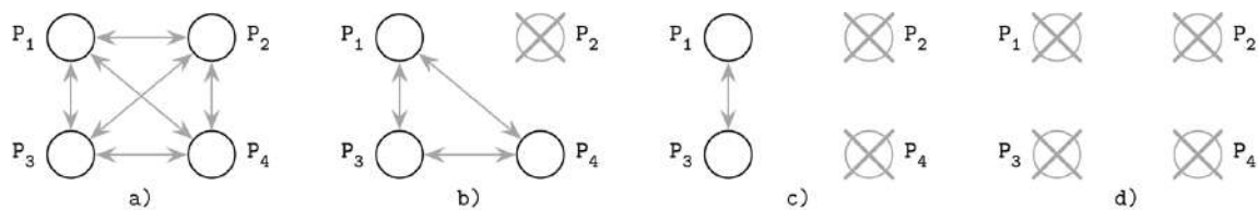
Figure 9-5. FUSE failure detection
