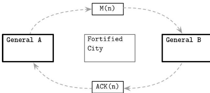
Figure 8-4. Two Generals' Problem illustrated
