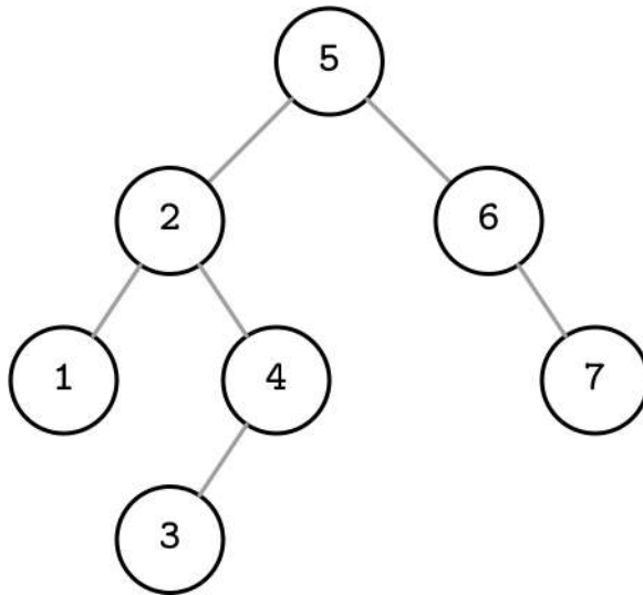
Figure 2-1. Binary search tree
