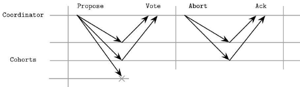
Figure 13-2. Cohort failure during the propose phase
