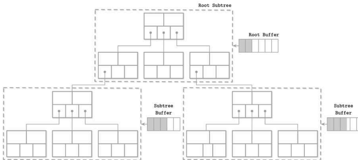
Figure 6-4. LA-Tree
