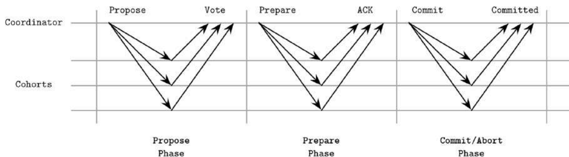
Figure 13-5. Three-phase commit
