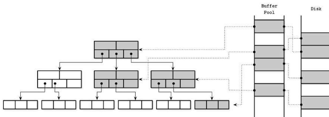
Figure 5-1. Page cache
