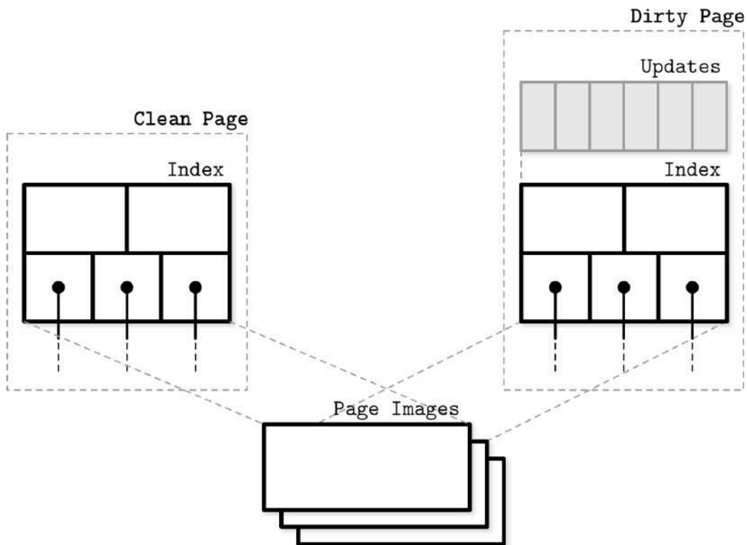
Figure 6-3. WiredTiger pages
