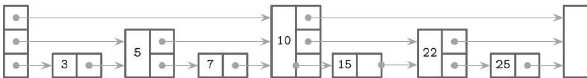
Figure 7-8. Skiplist
