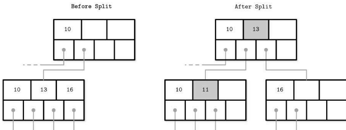
Figure 2-12. Nonleaf node split during the insertion of 11. New element and promoted key are shown in gray.
