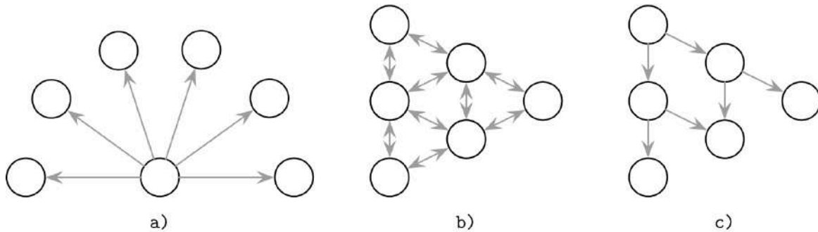
Figure 12-1. Broadcast (a), anti-entropy (b), and gossip (c)
