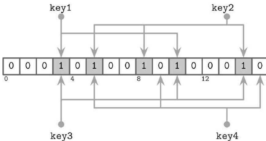
Figure 7-7. Bloom filter
