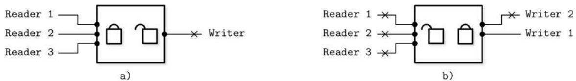
Figure 5-8. Readers-writer locks
