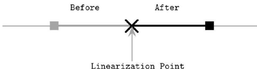
Figure 11-4. Linearization point
