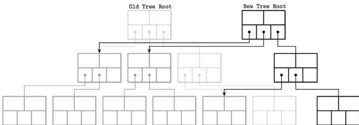
Figure 6-1. Copy-on-write B-Trees
