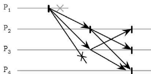
Figure 14-1. Broadcast
