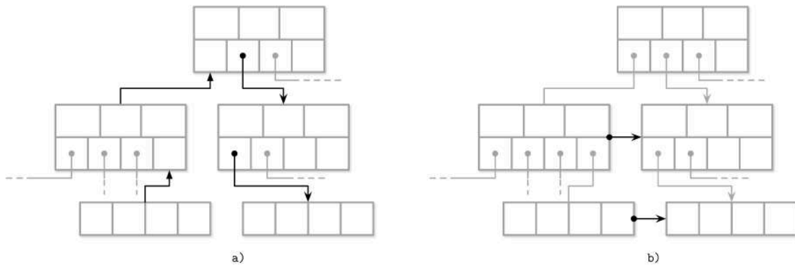
Figure 4-1. Locating a sibling by following parent links (a) versus sibling links (b)
