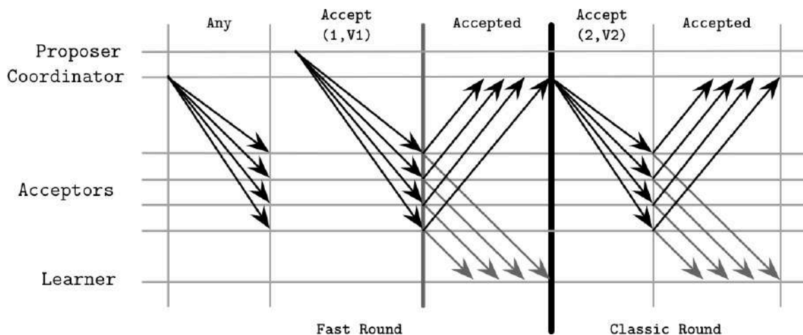
Figure 14-7. Fast Paxos algorithm: fast and classic rounds
