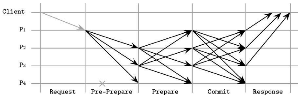
Figure 14-13. PBFT consensus, normal-case operation
