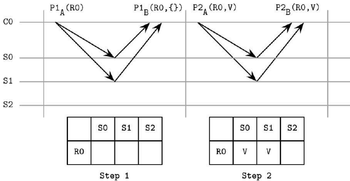
Figure 14-9. Generalization of Paxos
