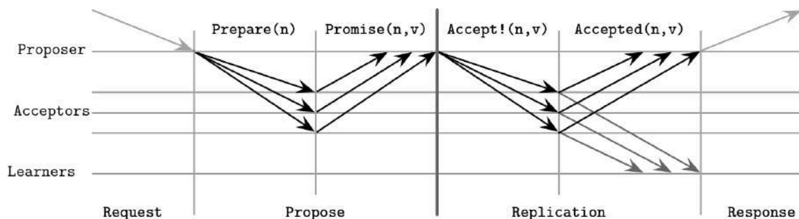
Figure 14-3. Paxos algorithm: normal execution
