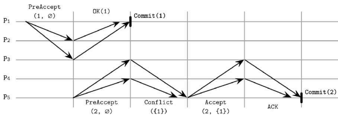
Figure 14-8. EPaxos algorithm run
