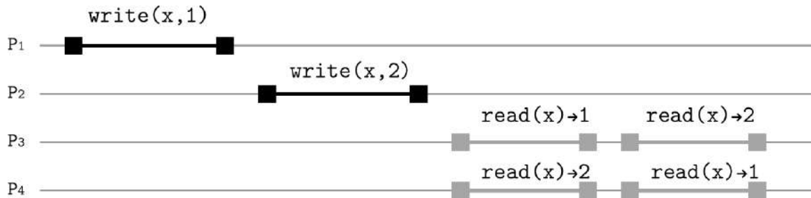
Figure 11-6. Write operations with no causal relationship
