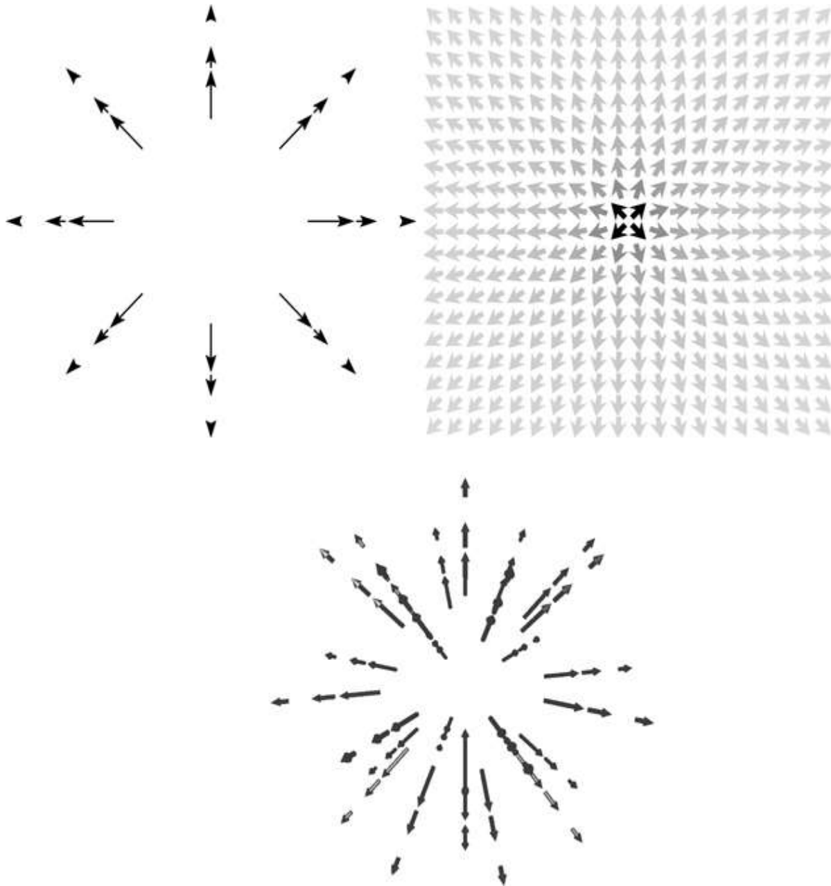
Figure 25-2: Three ways of visualizing the electric field \mathbf{eField\ protonOrigin} produced by a proton. The upper-left image is produced by eFieldPicProton2D , the upper-right image is produced by eFieldPicProtonGrad , and the lower picture is a screenshot of the 3D interactive image produced by eFieldPicProton3D .
