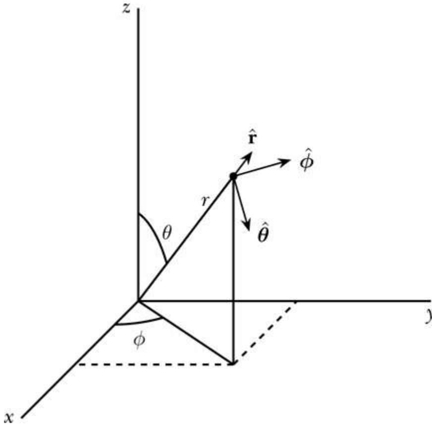
Figure 22-3: Spherical coordinates
