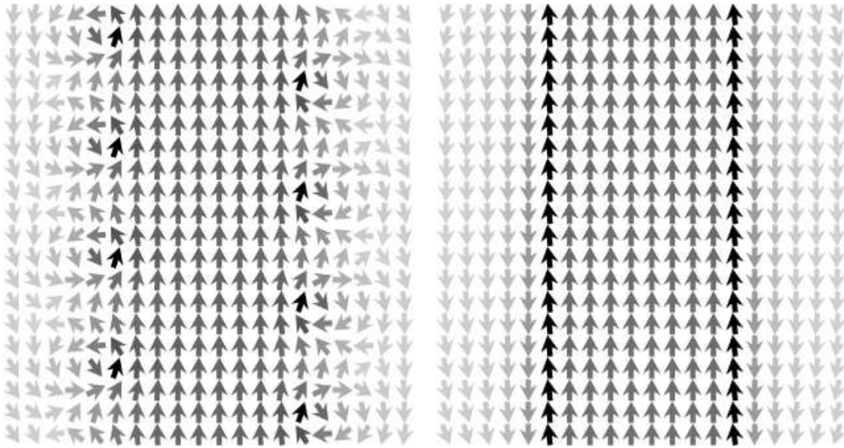
Figure 27-3: Magnetic fields produced by two solenoids. Both solenoids have a 1-cm radius, a 10-cm length, and a 10-A current. The solenoid on the left has 100 turns per meter, for a total of 10 turns. The solenoid on the right has 1,000 turns per meter, for a total of 100 turns. The pictures focus on a 4-cm \times 4-cm region at the center of the solenoid. The left image is produced by bFieldPicSolenoid10 ; the right image is produced by bFieldPicSolenoid100 .
