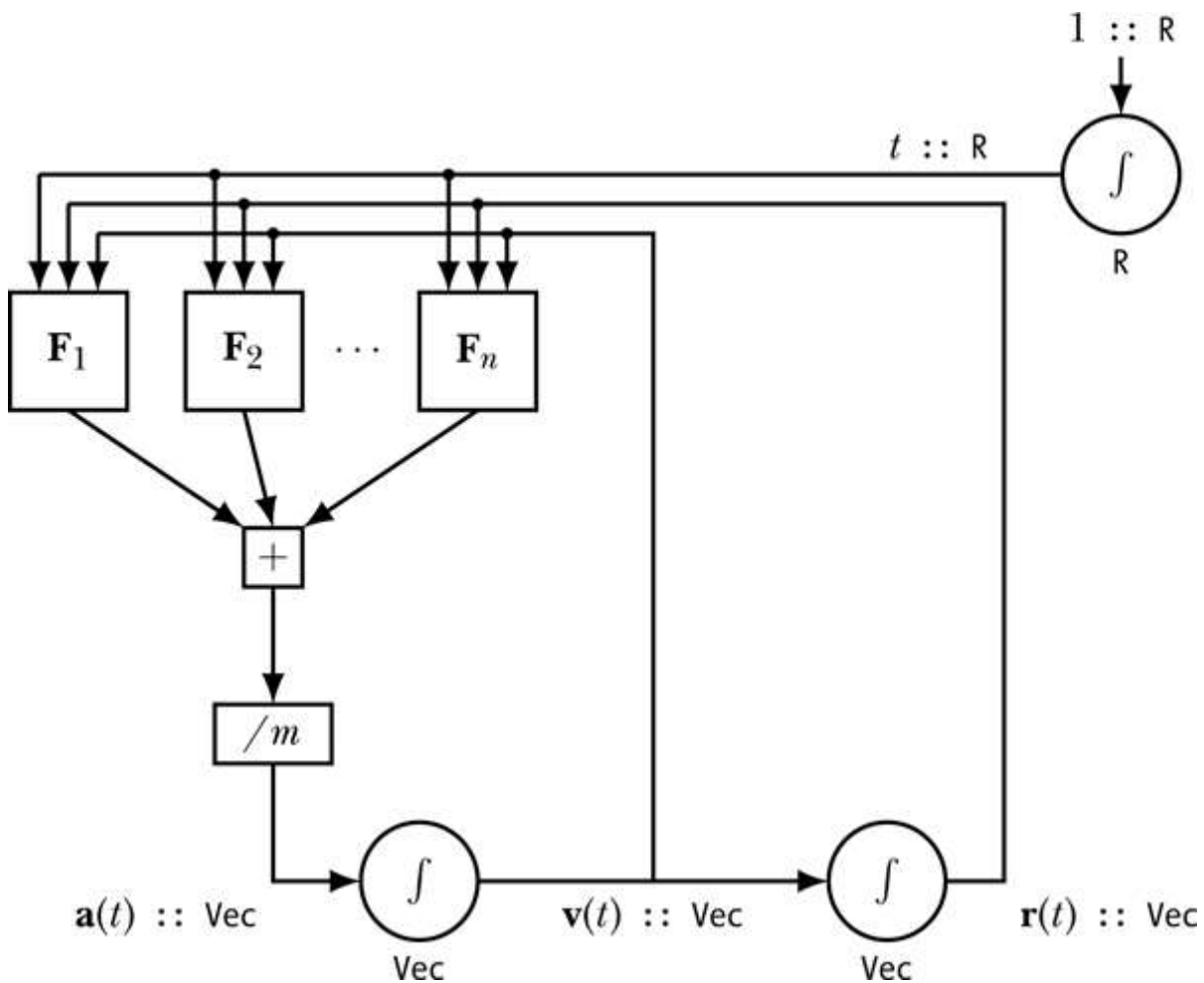
Figure 16-1: Schematic representation of Newton's second law
