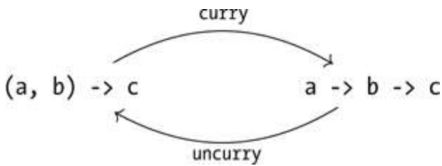
Figure 9-1: Two types for a function of two variables. The higher-order functions curry and uncurry transform a two-variable function of one type into the other type.
