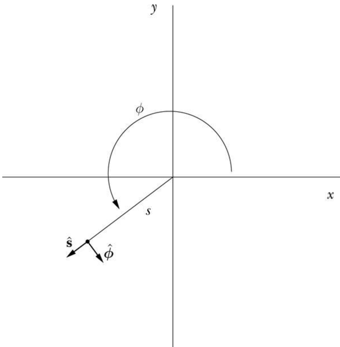
Figure 22-1: Polar coordinates
