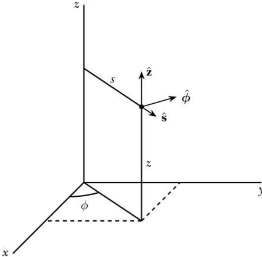
Figure 22-2: Cylindrical coordinates
