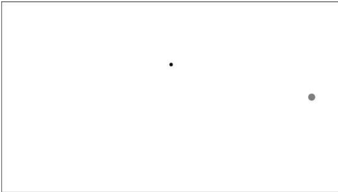
Figure 17-1: Halley's comet moving away from the sun
