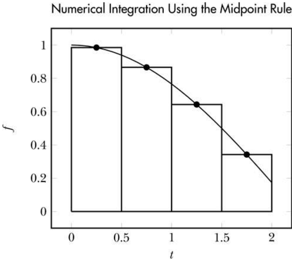
Figure 6-8: Numerical integration using the midpoint rule, \Delta t = 0.5
