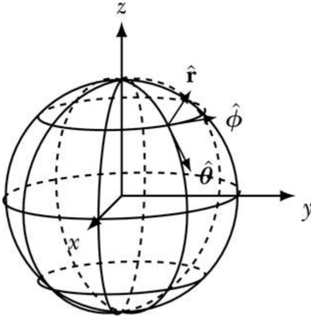
Figure 23-2: When the first parameter s is \theta and the second parameter t is \phi , the direction of orientation is \hat{\theta} \times \hat{\phi} , which is the same as \hat{\mathbf{r}} , so the orientation is outward.
