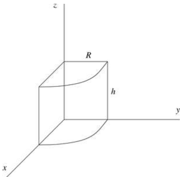
Figure 23-5: A volume representing a quarter cylinder
