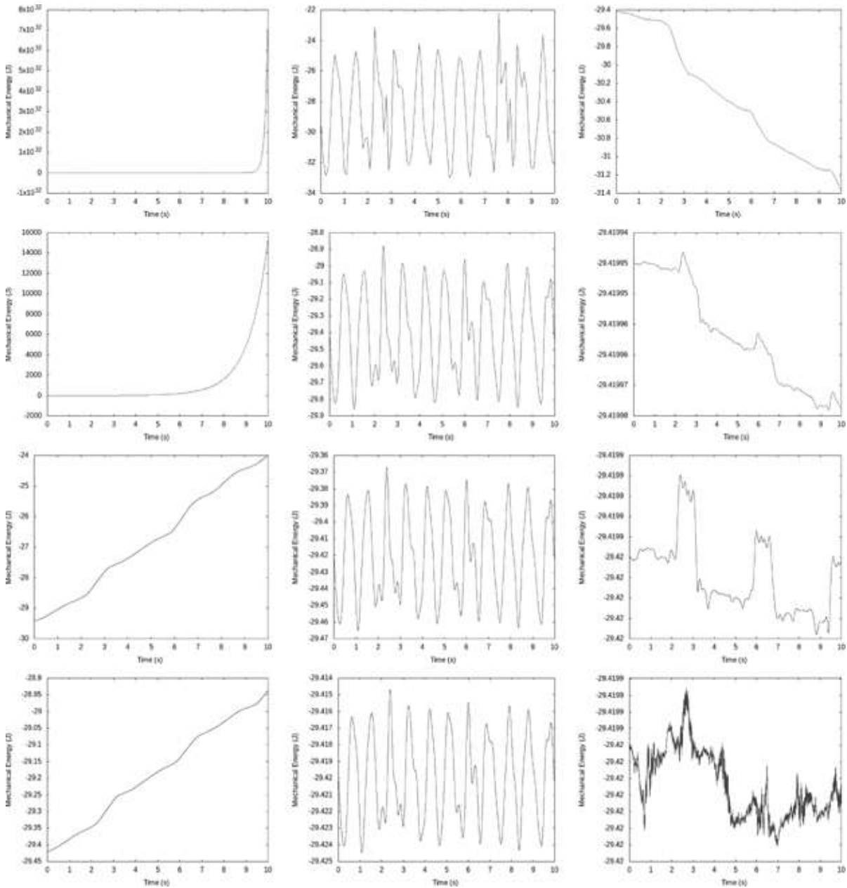
Figure 20-2: Mechanical energy as a function of time for different numerical methods. The change in mechanical energy is a measure of numerical inaccuracy.
