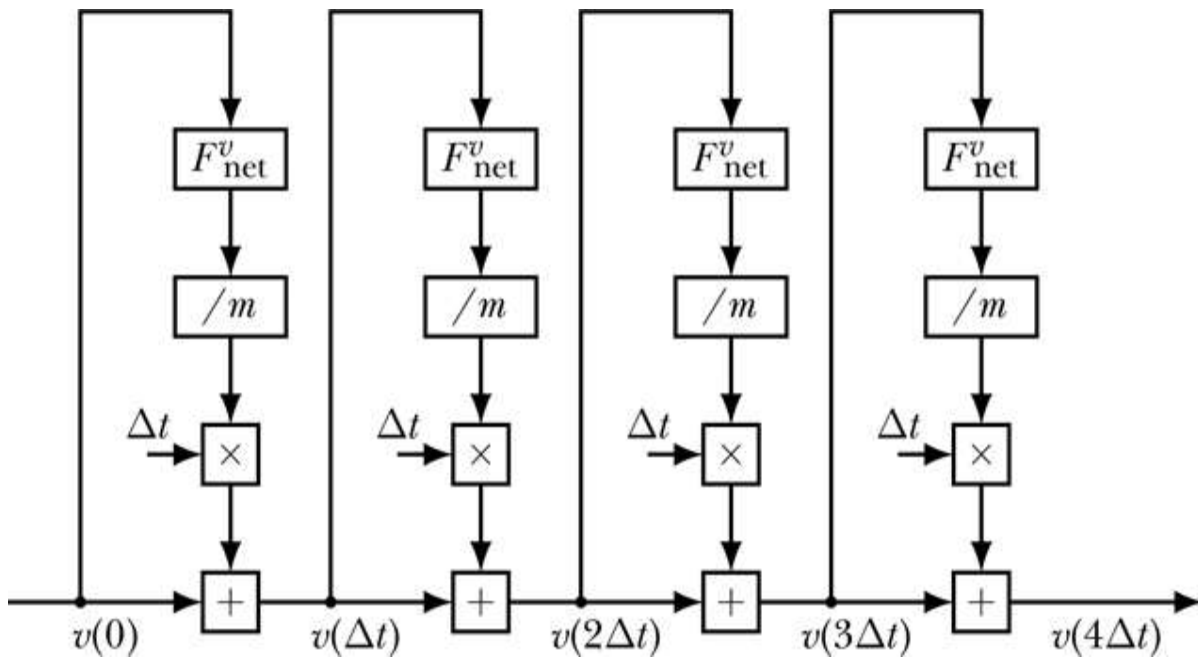
Figure 14-7: Euler method for Newton's second law in one dimension, for the special case in which net force depends only on velocity
