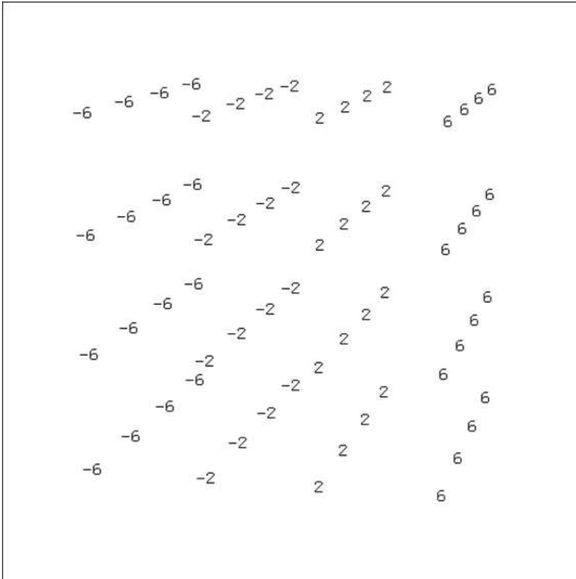
Figure 22-4: A screenshot of the y -coordinate scalar field y_{SF} produced with the program y_{SF}3D . The mouse and keyboard can be used to zoom in or out and rotate the visualization, a standard feature of the Vis module.
