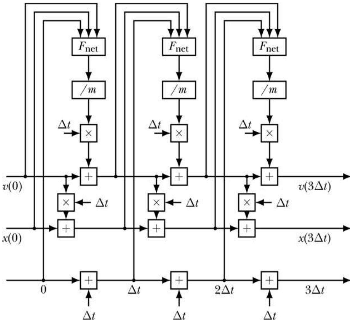
Figure 15-3: Euler method for Newton's second law in one dimension
