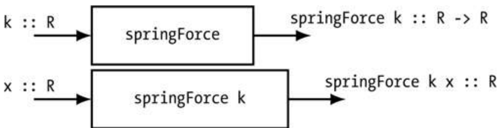
Figure 6-1: The higher-order function springForce takes a number as input and returns the function springForce k as output. The function springForce k then takes a number as input and returns a number as output.
