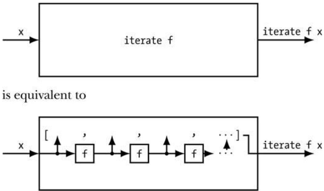
Figure 6-4: The function iterate f applies the function f to the input zero, one, two, three, and more times and collects the results in an infinite list.
