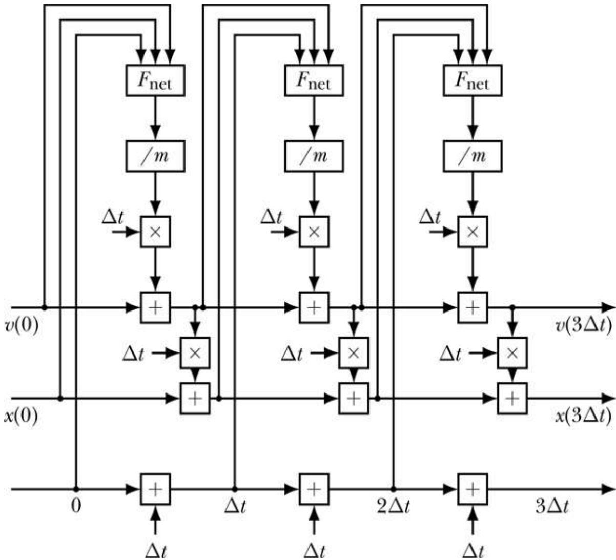
Figure 15-7: The Euler-Cromer method for Newton's second law in one dimension
