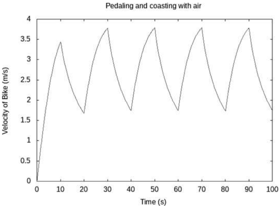
Figure 14-13: Pedaling and coasting with air resistance
