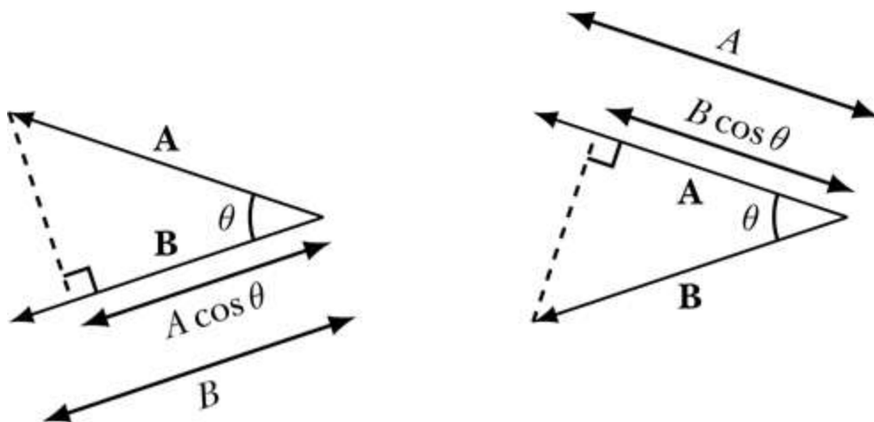
Figure 10-4: The dot product of two vectors is the product of the magnitude of one vector and the projection of the second vector onto the first.
