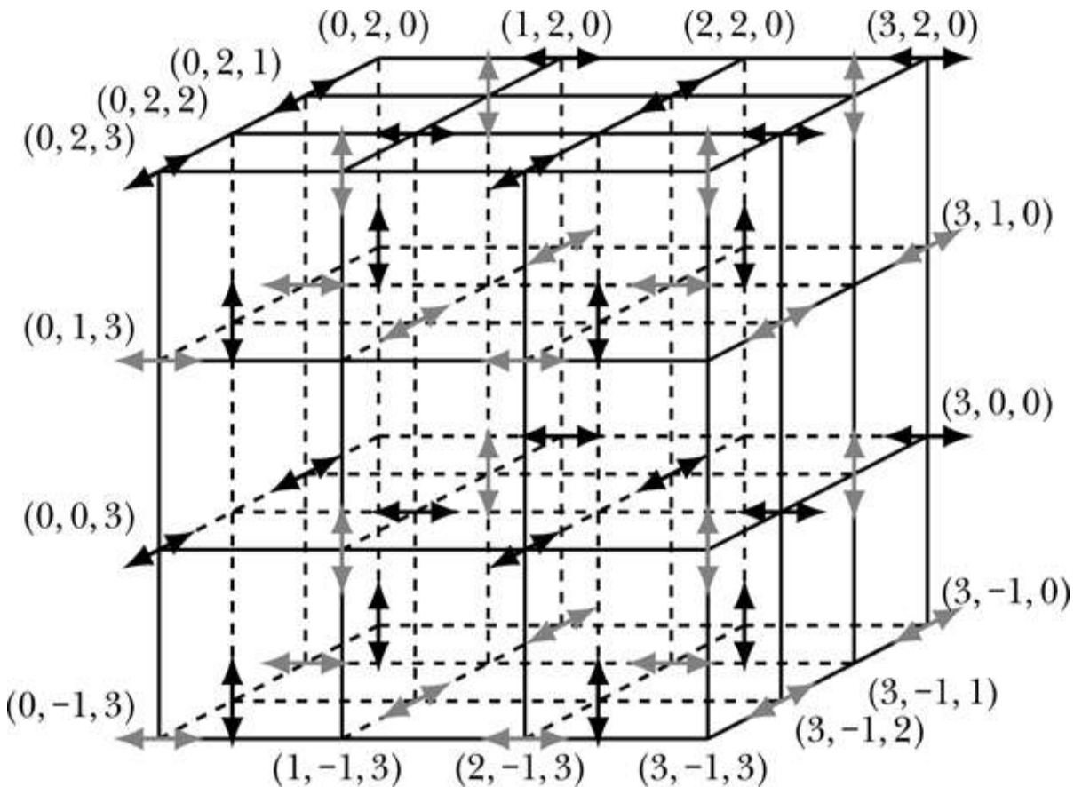
Figure 29-2: Yee cell showing where electric and magnetic field components are calculated
