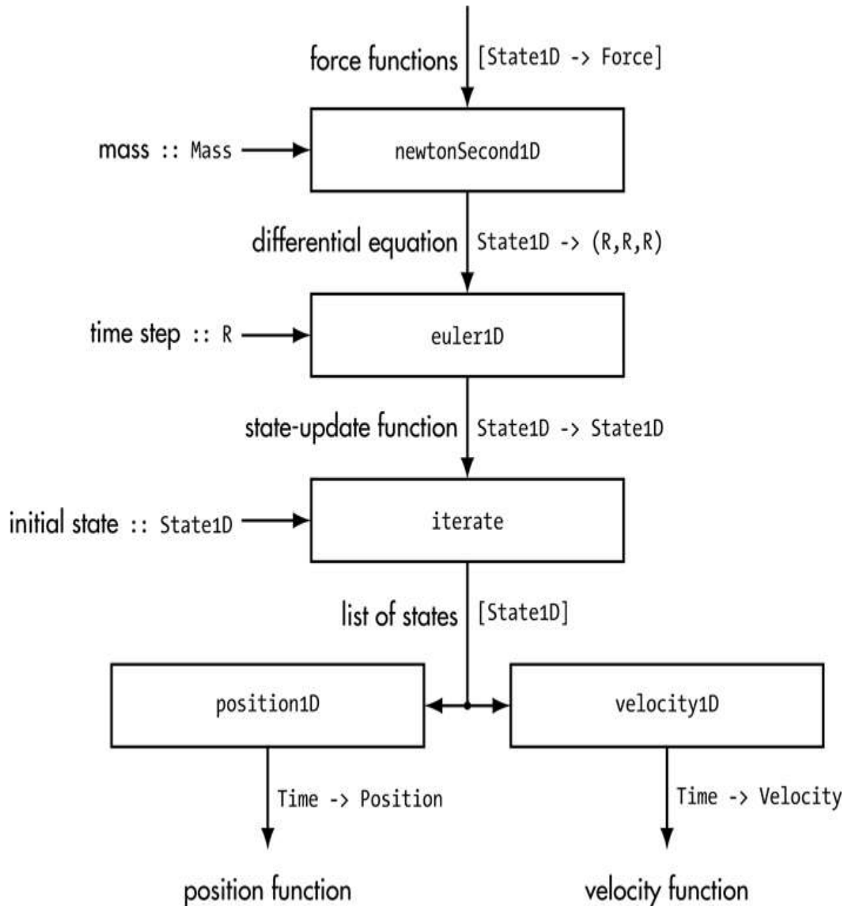
Figure 15-2: Data flow for solving a mechanics problem in one dimension. Functions transform the data through a sequence of five representations.
