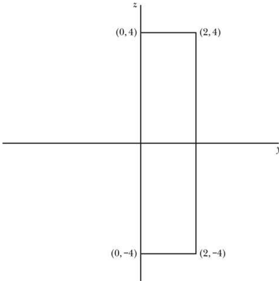
Figure 23-4: A surface in the yz -plane
