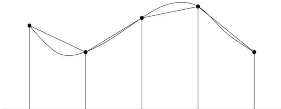
Figure 6-9: The trapezoidal rule
