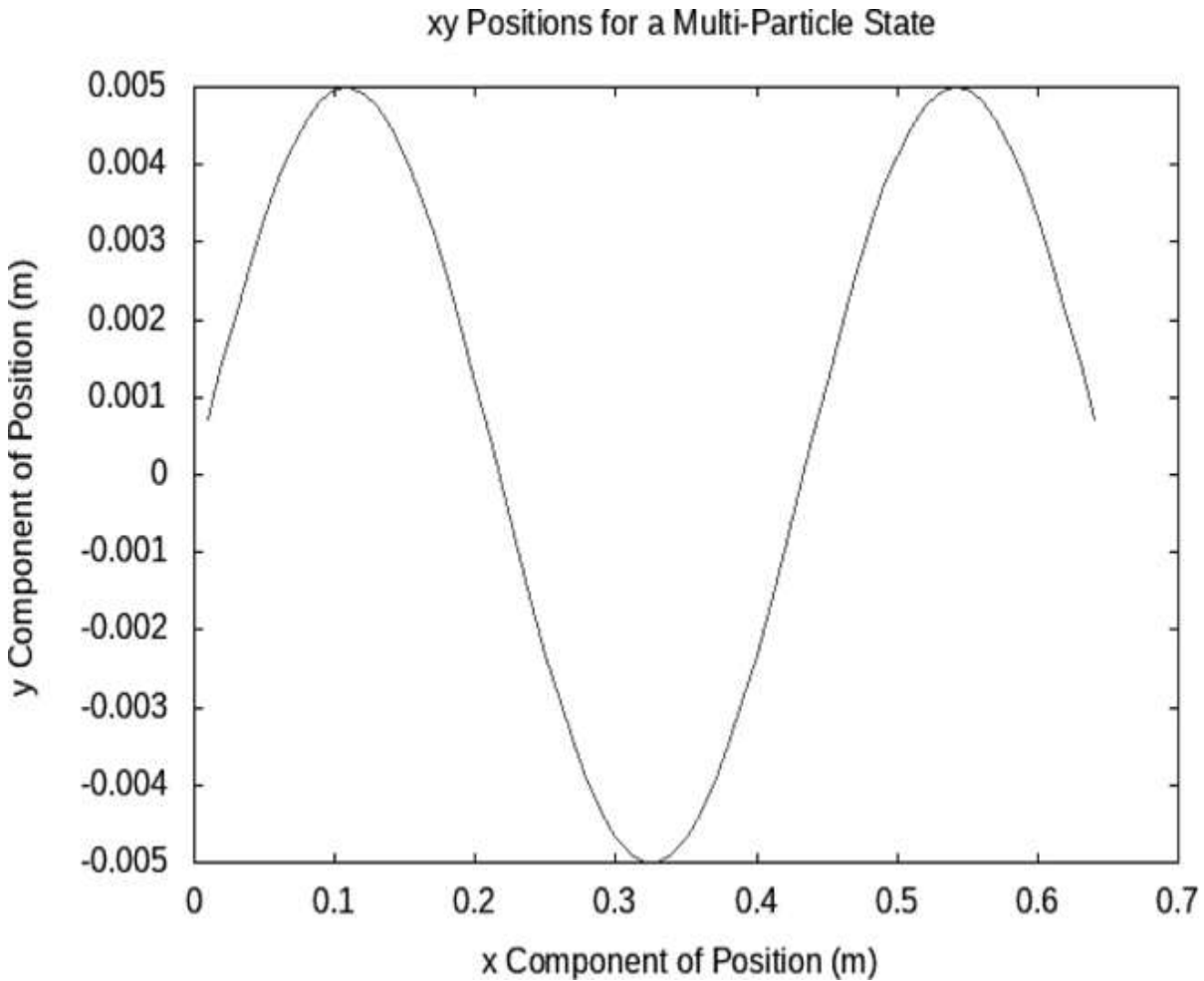
Figure 20-5: Initial state for the second overtone of a guitar string, given by stringInitialOvertone 3
