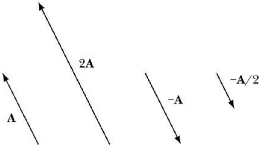
Figure 10-2: Scalar multiplication. Scaling A by 2, -1 , and -1/2 results in 2A , -A , and -A/2 , respectively.
