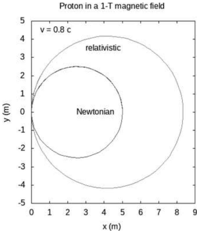
Figure 18-2: Proton in a magnetic field
