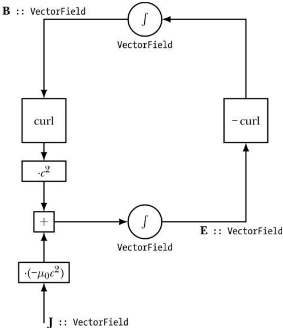
Figure 29-1: A schematic diagram representing the Maxwell equations
