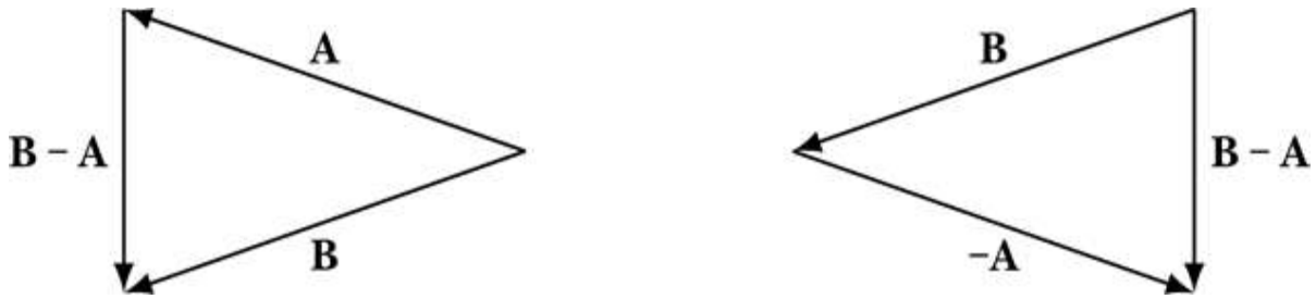
Figure 10-3: Vector subtraction. The vector \mathbf{B} - \mathbf{A} is the difference of vectors \mathbf{B} and \mathbf{A} .
