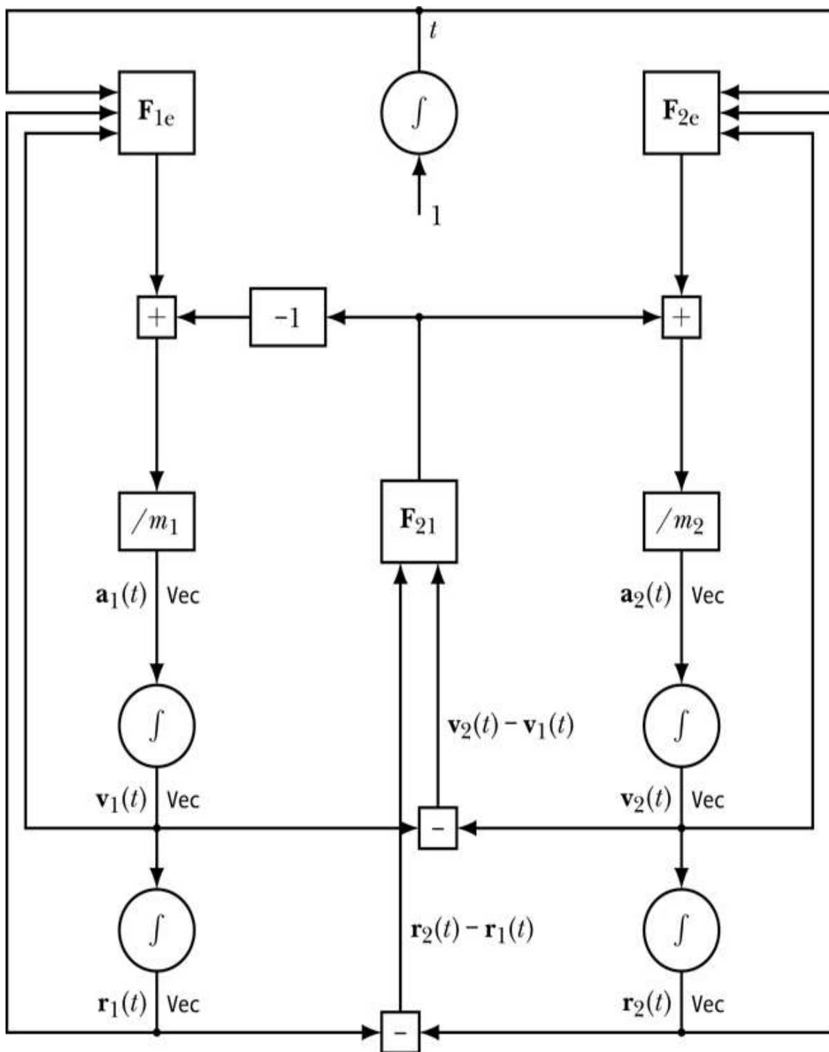
Figure 19-3: Schematic representation of Newton's second law and Newton's third law working together in a two-body situation. The two bodies interact with each other, and each body has external forces acting on it as well.
