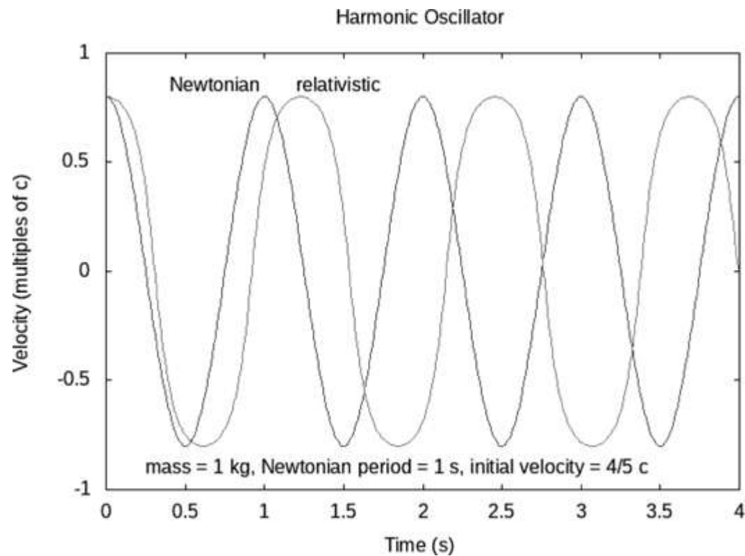
Figure 18-3: The relativistic harmonic oscillator
