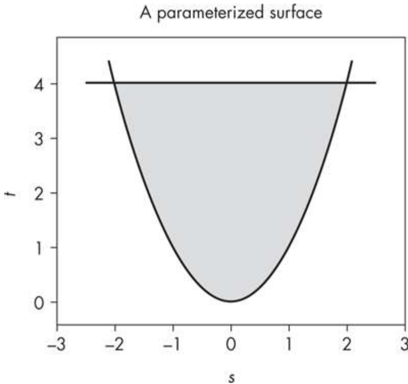
Figure 23-1: A parameterized surface
