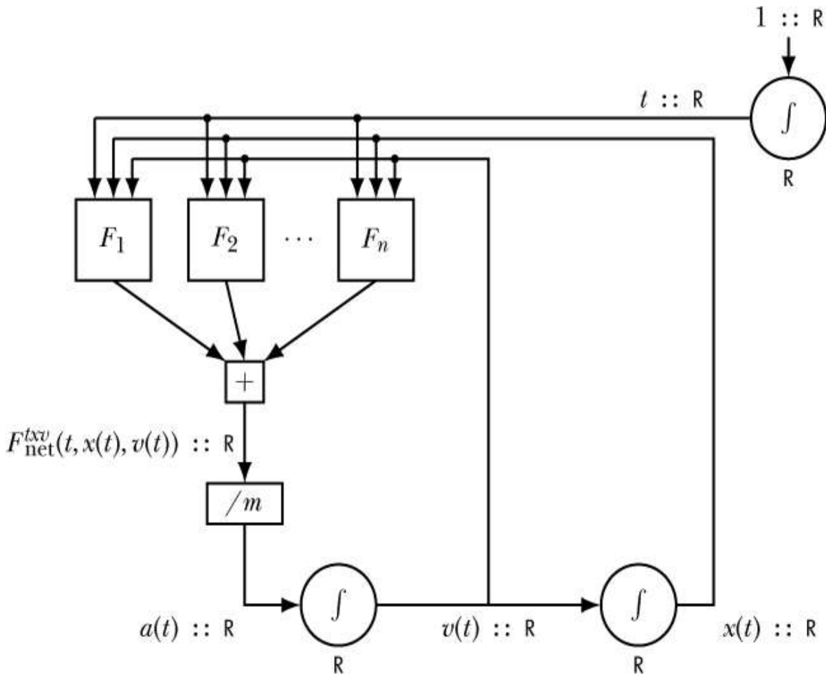
Figure 15-1: Newton's second law in one dimension. The forces depend on time, position, and velocity.
