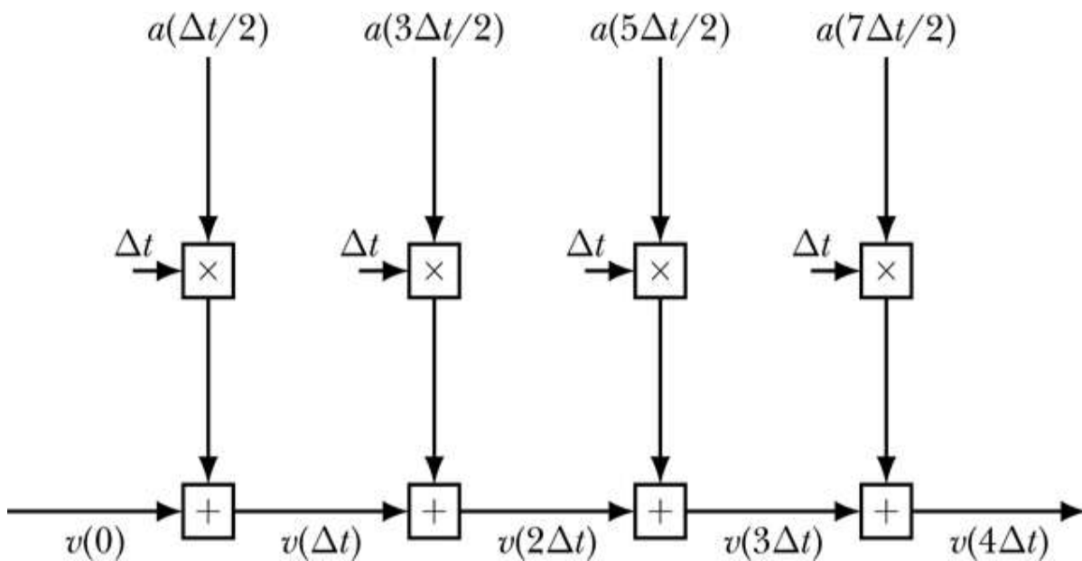
Figure 6-7: A functional model of an integrator that is discrete and state free. This integrator uses the midpoint rule.
