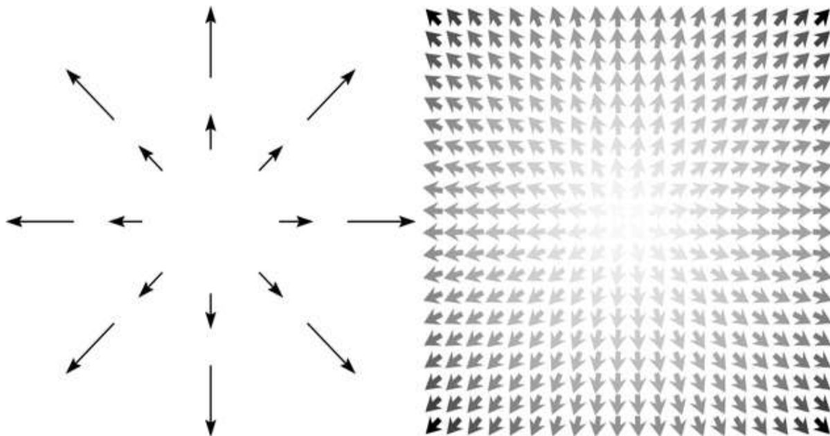
Figure 22-6: Two ways of visualizing the vector field \mathbf{r} , or rVF , in the xy -plane. The left image is produced by rVFpng ; the right image is produced by rVFGrad .
