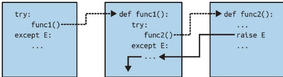
Figure 36-1. Nested try/except combinations
