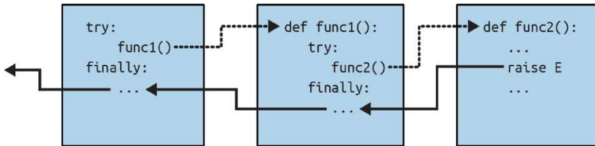
Figure 36-2. Nested try/finally combinations
