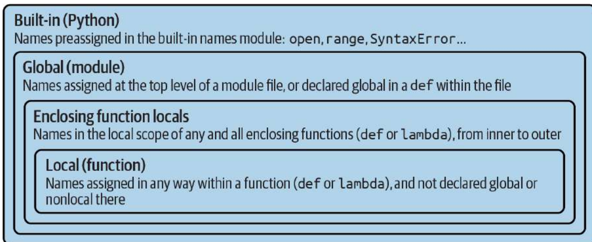
Figure 17-1. The LEGB scope lookup rule for names
