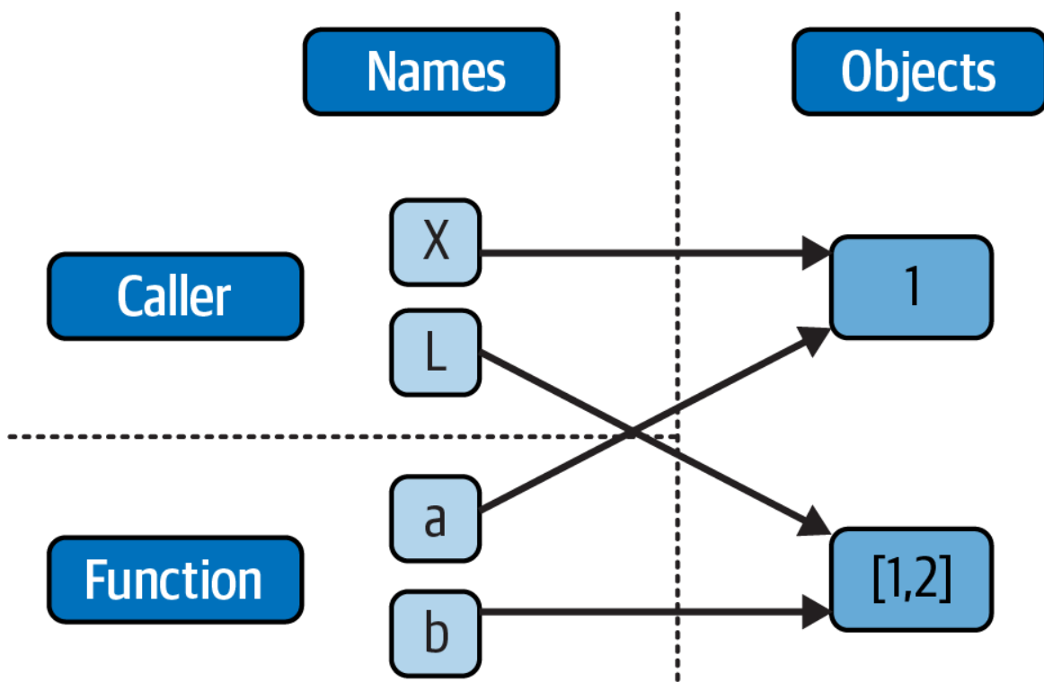
Figure 18-1. Function arguments and shared object references
