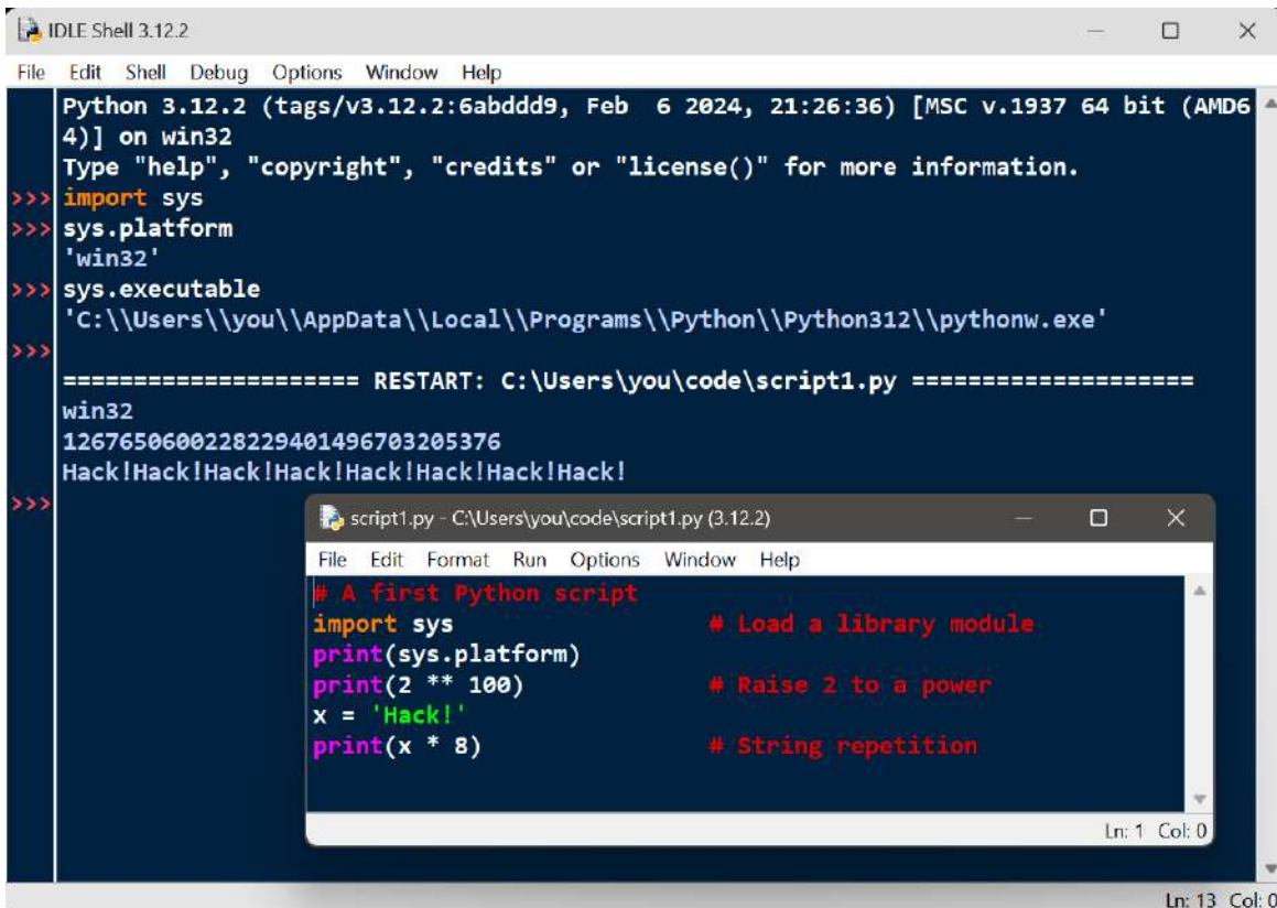
Figure 3-1. IDLE with its dark theme on Windows
