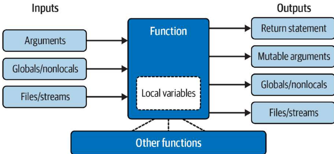
Figure 19-1. Function execution environment
