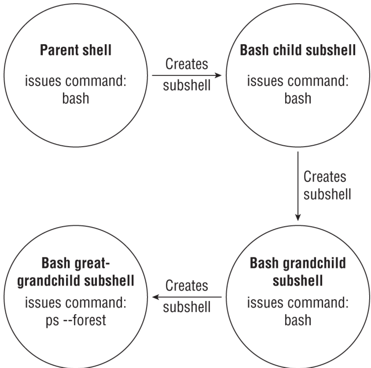
FIGURE 5-2 Subshell nesting
