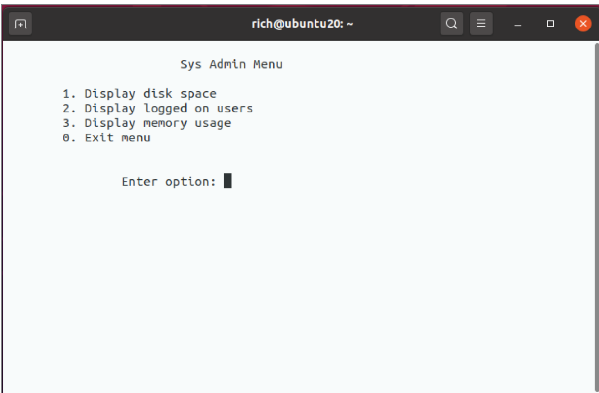
FIGURE 18-1 Displaying a menu from a shell script
