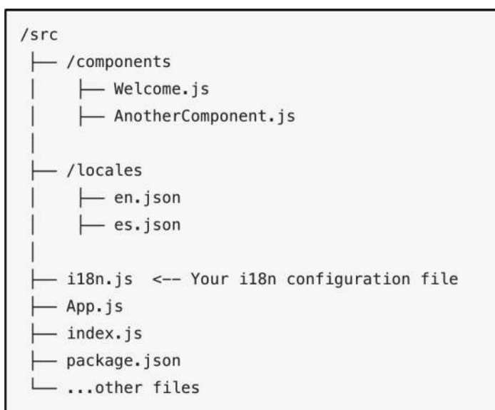
Figure 16-3. Recommended folder structure for locales and i18n.js
