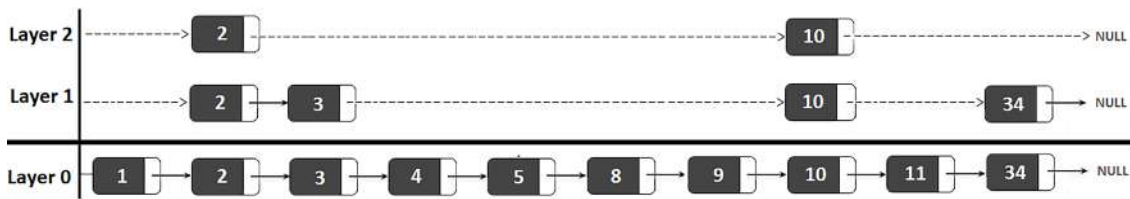
Figure 5.18: Skip List sample
