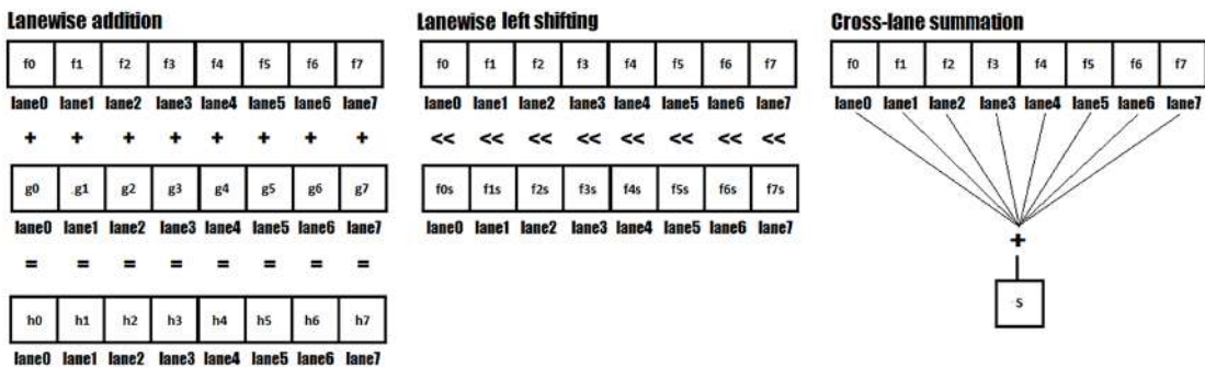
Figure 5.6: Lanewise and cross-lane operations
