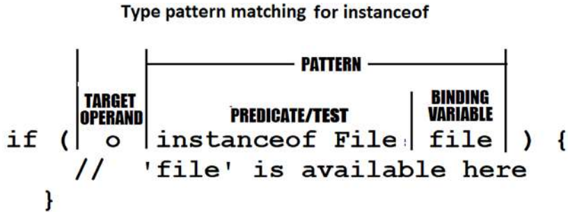
Figure 2.32: Type pattern matching for instanceof
