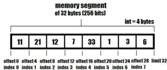
Figure 7.10: A memory segment of 8 integers
