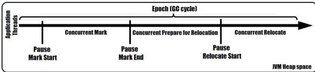
Figure 12.19: ZGC concurrency
