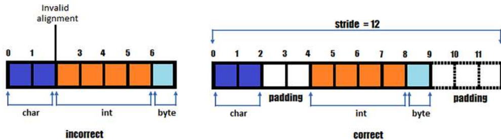
Figure 7.19: Incorrect/correct padding
