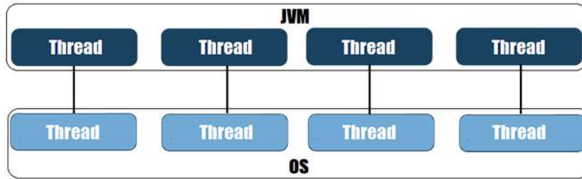
Figure 10.5: JVM to OS threads
