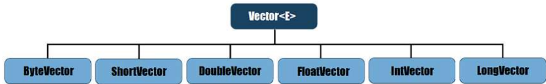
Figure 5.3: Specialized vector subtypes
