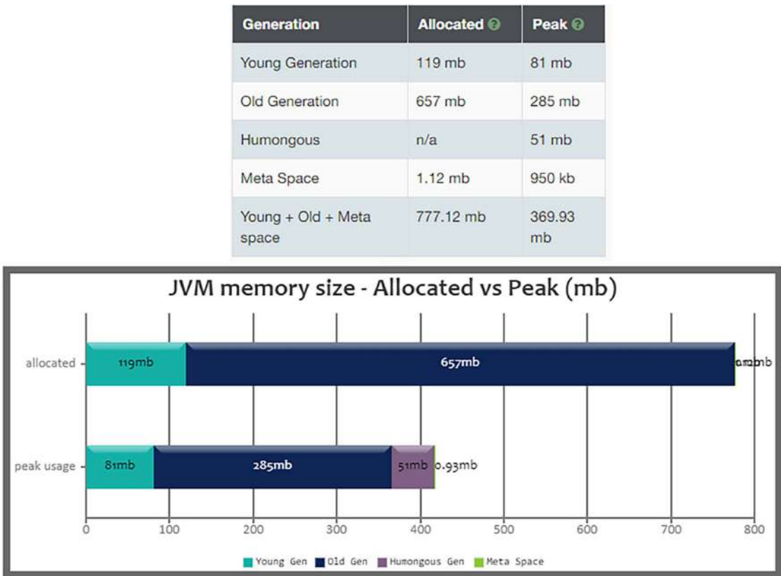
Figure 12.25: A screenshot from Universal GC Log Analyzer (GCEasy) report
