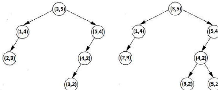
Figure 5.24: Inserting (3,2) and (5,2)
