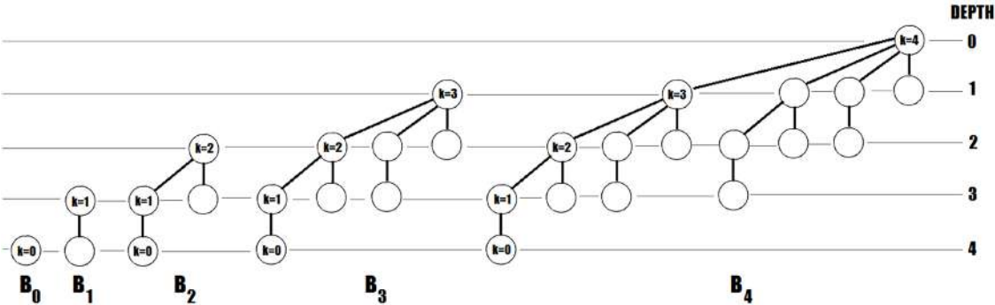
Figure 5.28: B_0 - B_4 Binomial Trees
