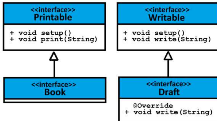
Figure 2.26: Interfaces: Printable , Writable , Draft , and Book
