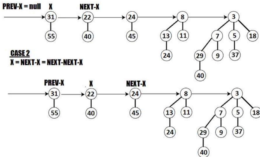
Figure 5.35: Applying Case 2
