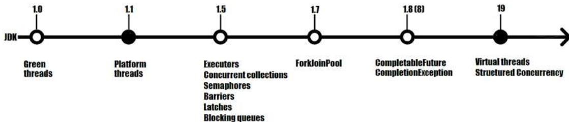
Figure 10.4: JDK multithreading evolution
