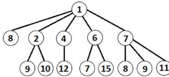
Figure 5.39: Fibonacci Heap sample
