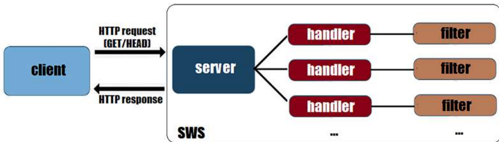
Figure 13.5: SWS key abstractions
