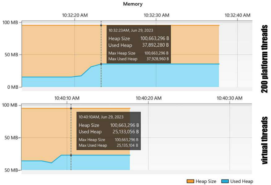
Figure 11.9: Memory usage (lock free)
