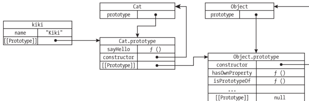
Figure 6-1: The prototype chain for kiki
