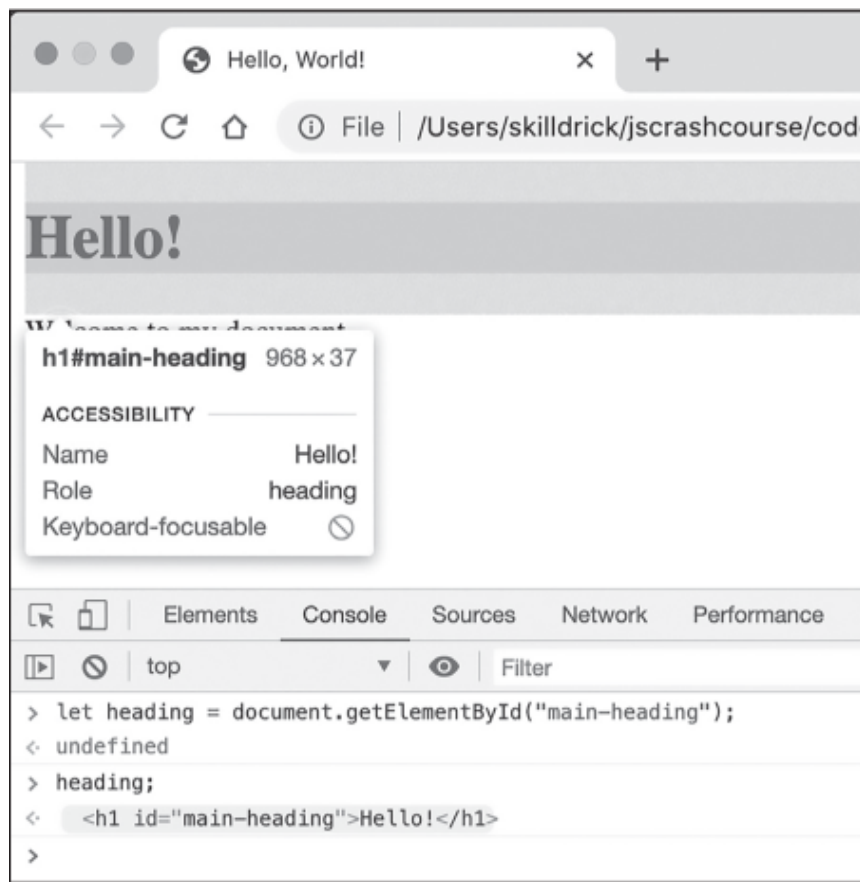
Figure 7-5: Chrome highlighting the h1 element on the page
