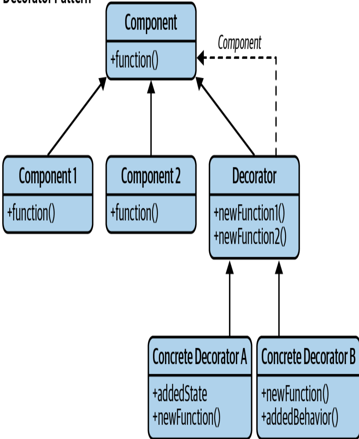
Figure 7-7. Decorator pattern
