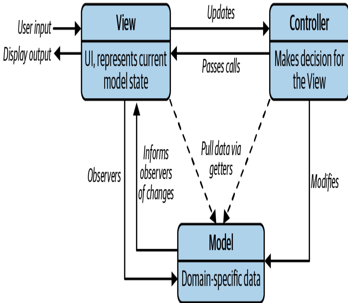
Figure 8-1. MVC pattern
