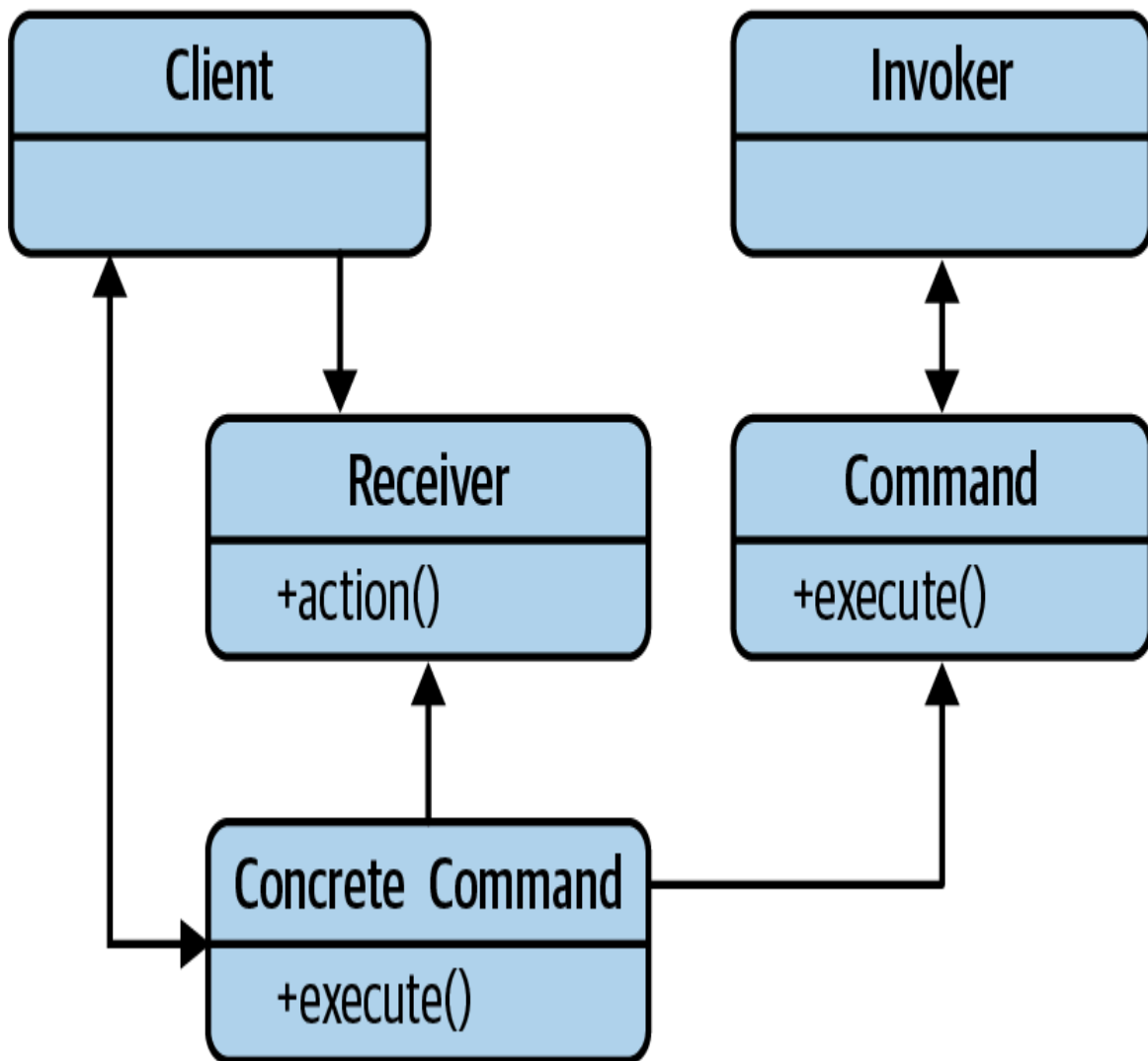
Figure 7-12. Command pattern
