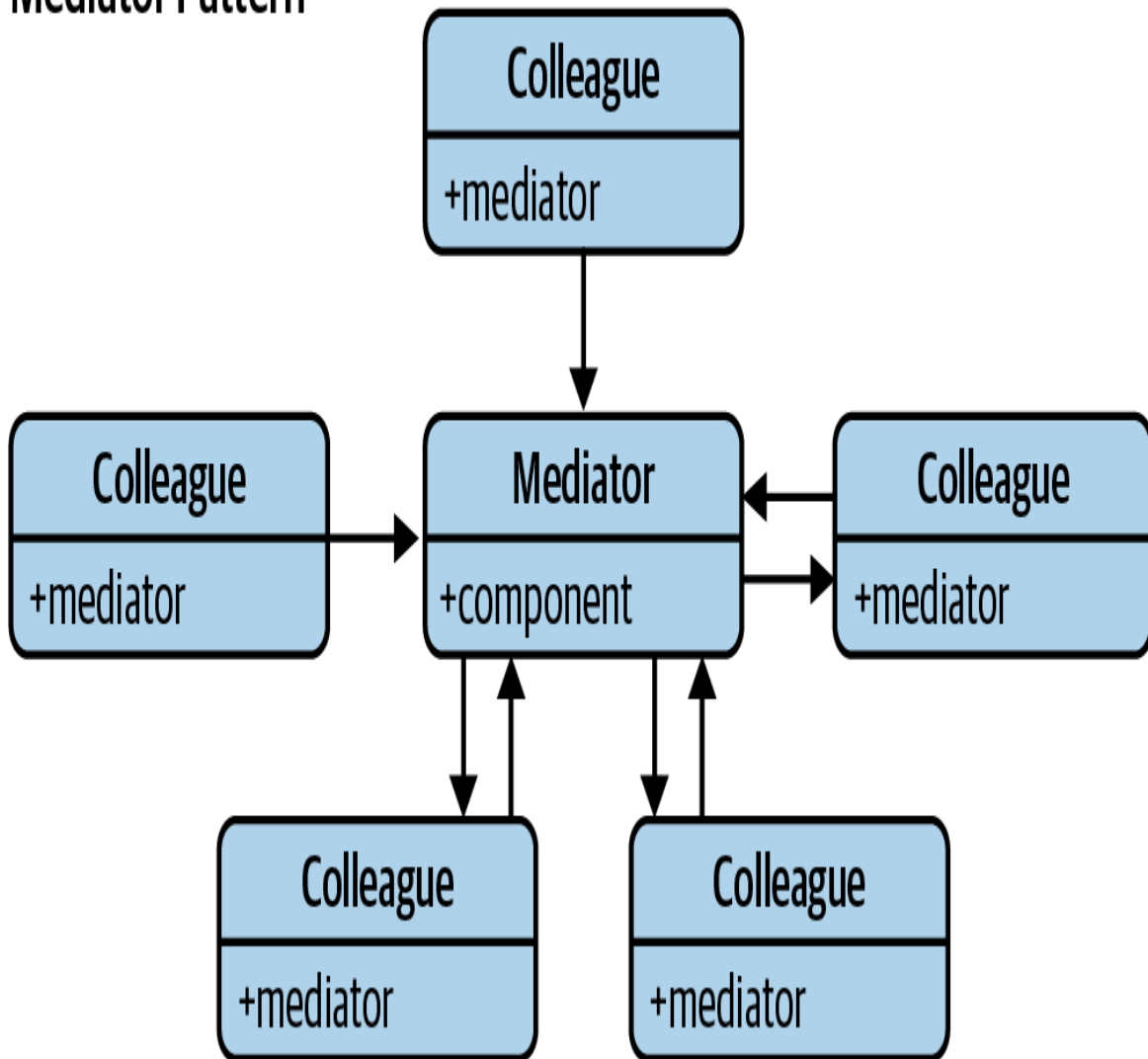
Figure 7-11. Mediator pattern
