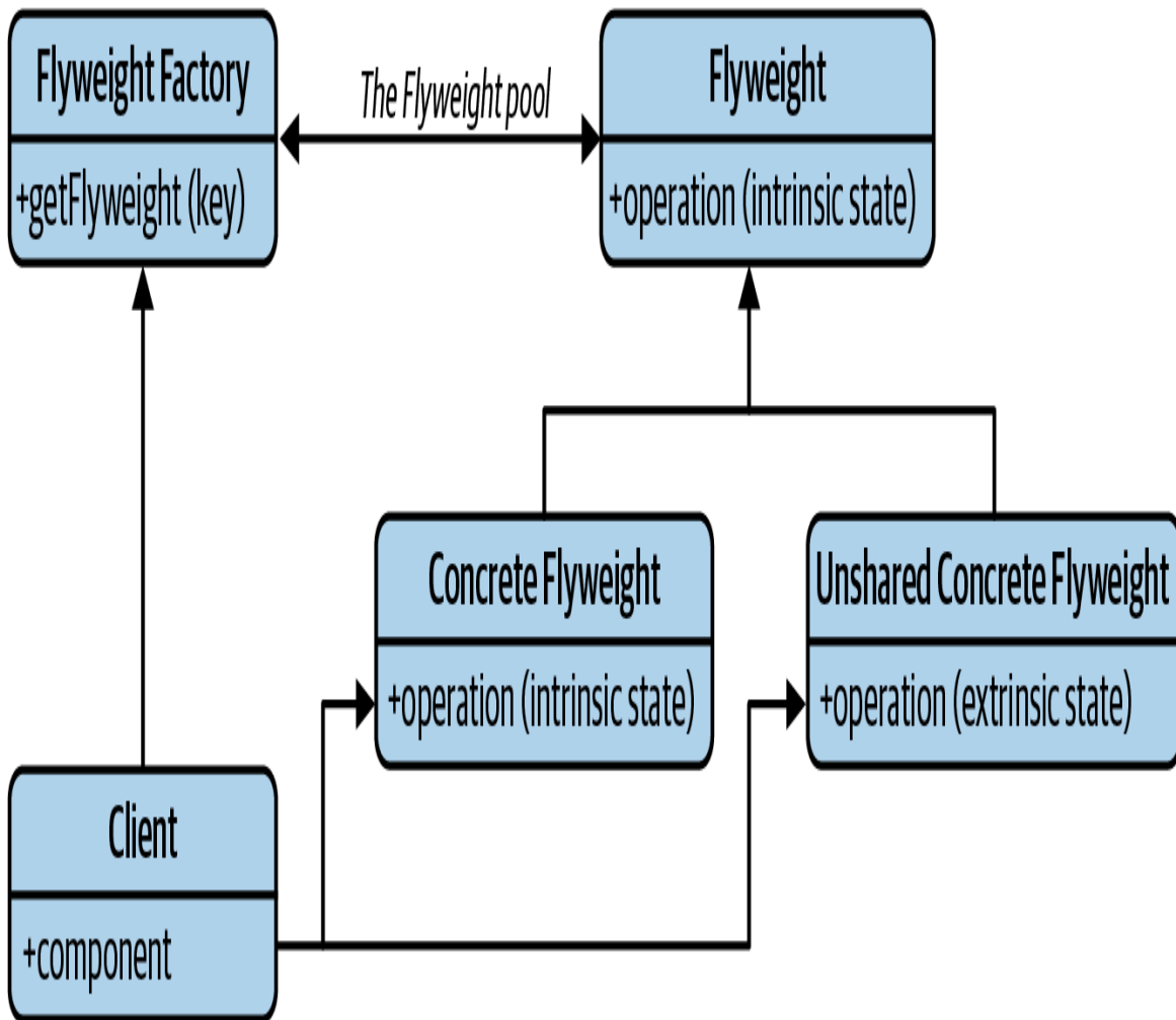
Figure 7-8. Flyweight pattern
