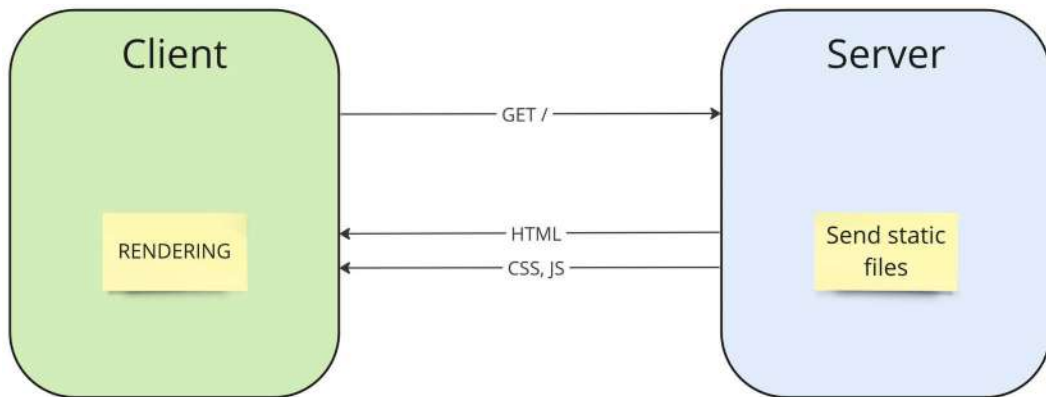
Figure 13.1: SPA application
