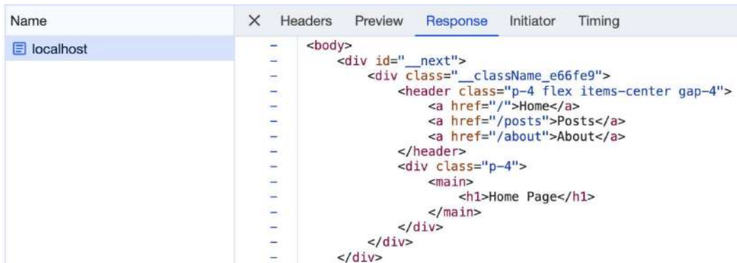
Figure 13.5: Home page response in Chrome DevTools
