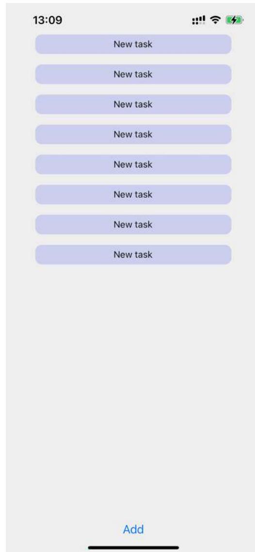
Figure 26.1: To-do list
