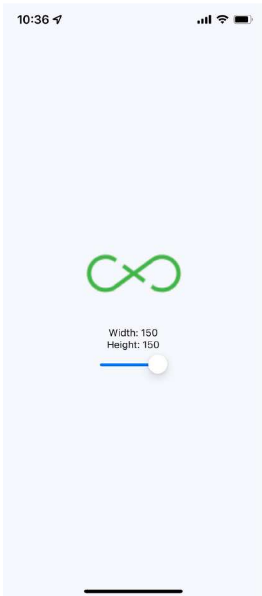
Figure 27.4: 150 x 150 image
