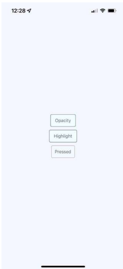
Figure 23.4: Pressable button
