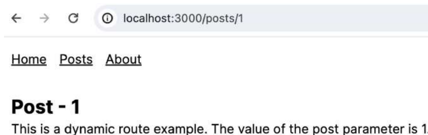
Figure 13.7: Post page
