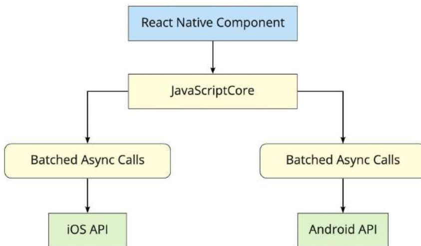
Figure 15.1: React Native workflow
