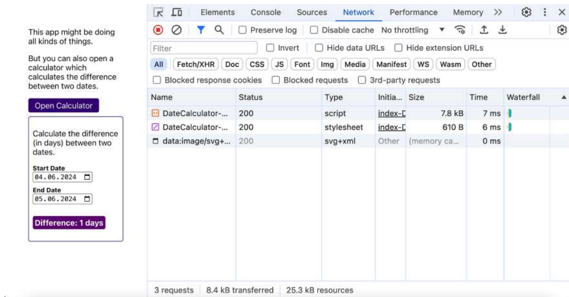
Figure 10.11: After clicking the button, an extra code file is downloaded
