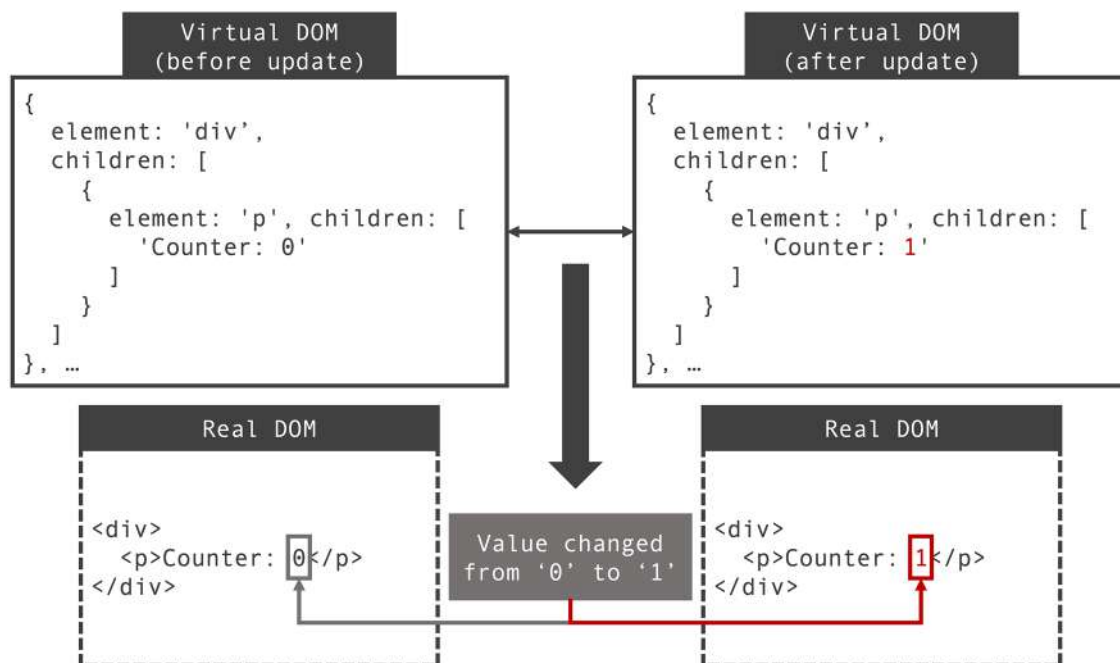
Figure 10.3: React detects required updates via the virtual DOM
