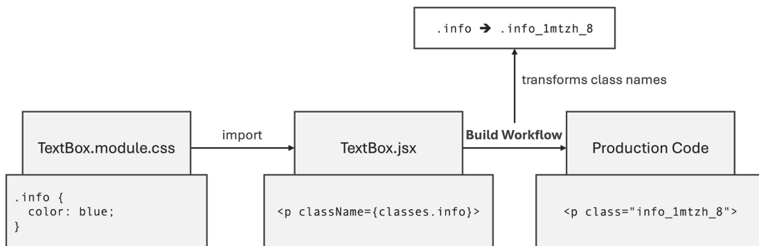
Figure 6.5: CSS modules in action. CSS class names are transformed into unique names during the build workflow
