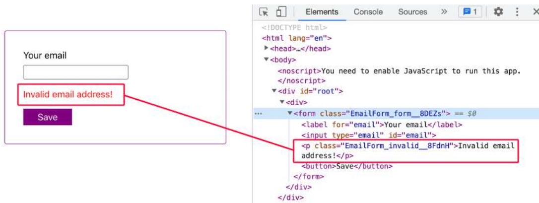
Figure 7.5: The error message DOM element sits right below the <input> it belongs to
