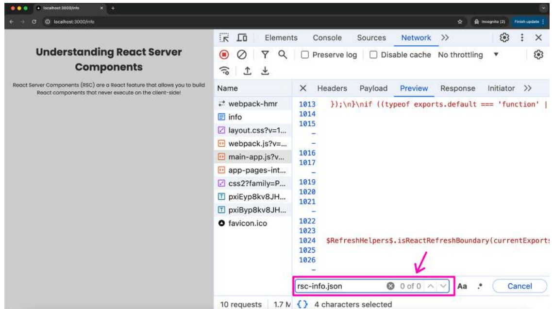
Figure 16.4: The data source filename that's included in the RSC code can't be found on the client side
