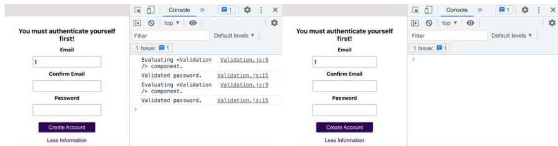
Figure 10.20: No console messages when clicking “More Information”
