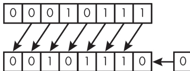
Figure 4-1: A logical left shift of 1 bit
