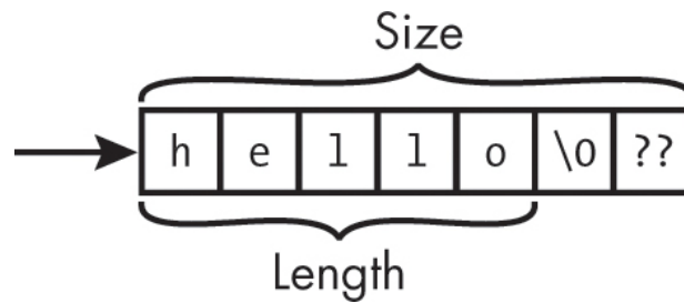
Figure 7-1: A sample narrow string
