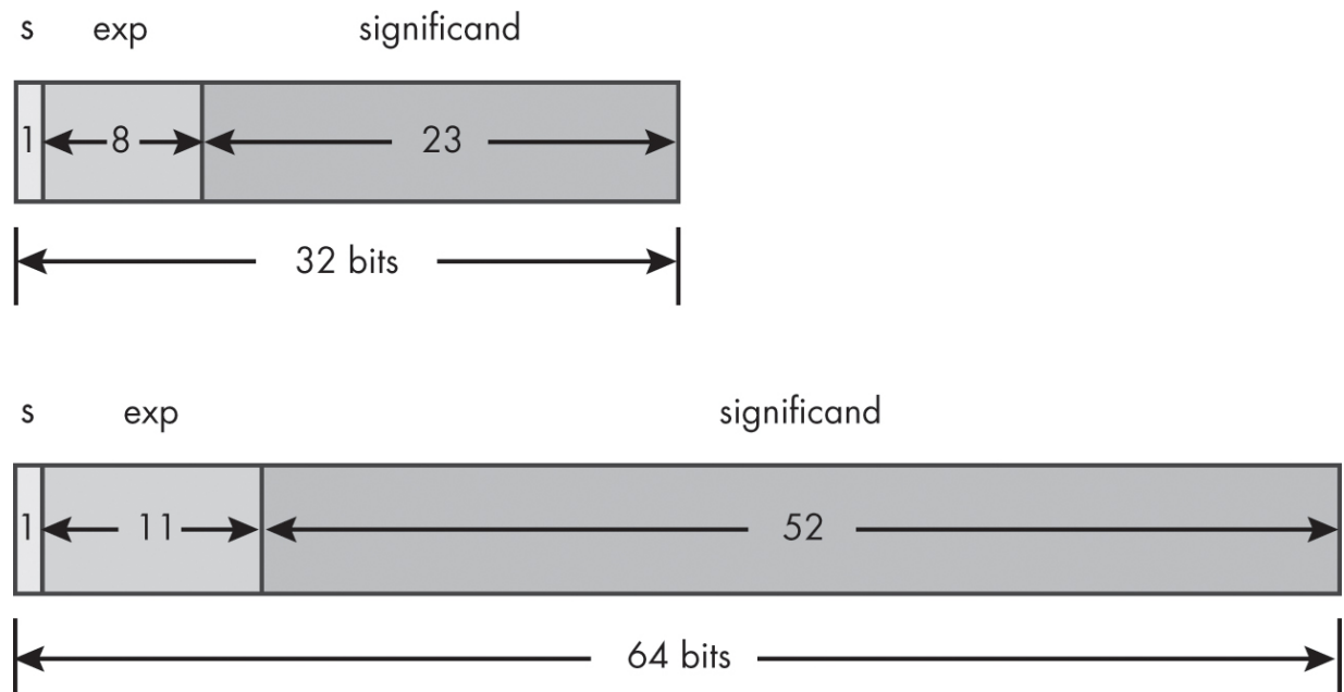
Figure 3-2: The float and double types
