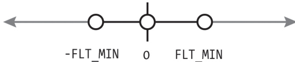
Figure 3-3: The domain of subnormal numbers
