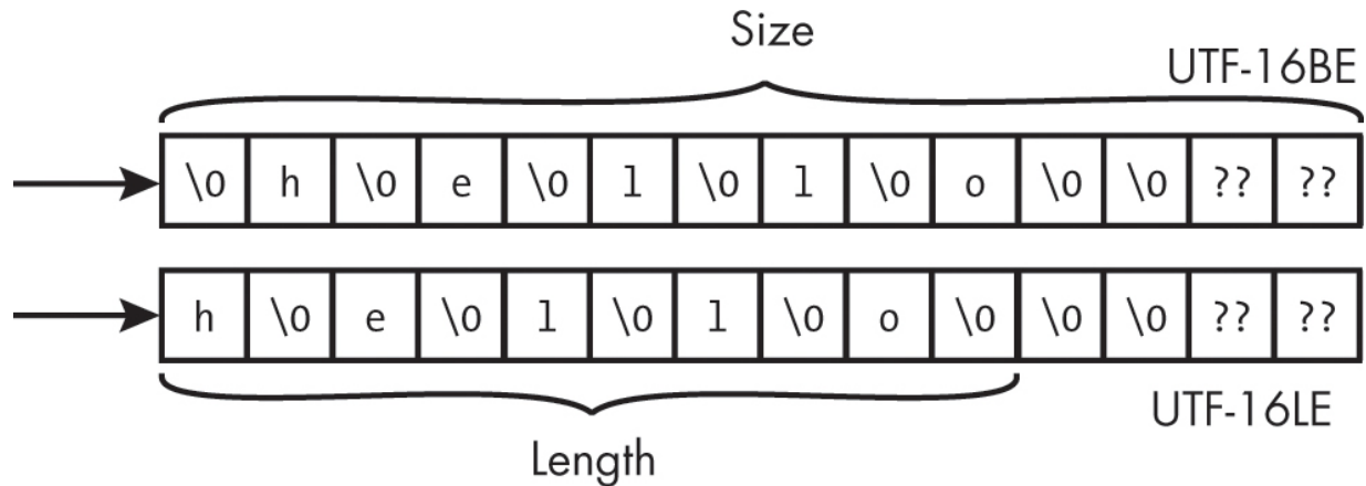
Figure 7-2: Sample UTF-16BE and UTF-16LE wide strings
